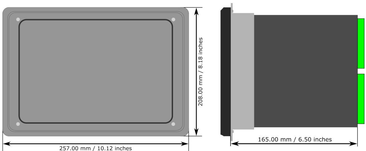
Figure. 7.5 - 128. Device dimensions.
