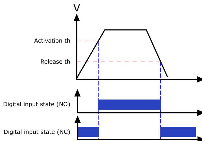
Figure. 7.4.1 - 114. Digital input state when energizing and de-energizing the digital input channels.
