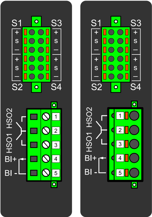
Figure. 7.4.6 - 119. Arc protection module. Can be equipped with standard screw terminals or spring cage terminals for connection.
