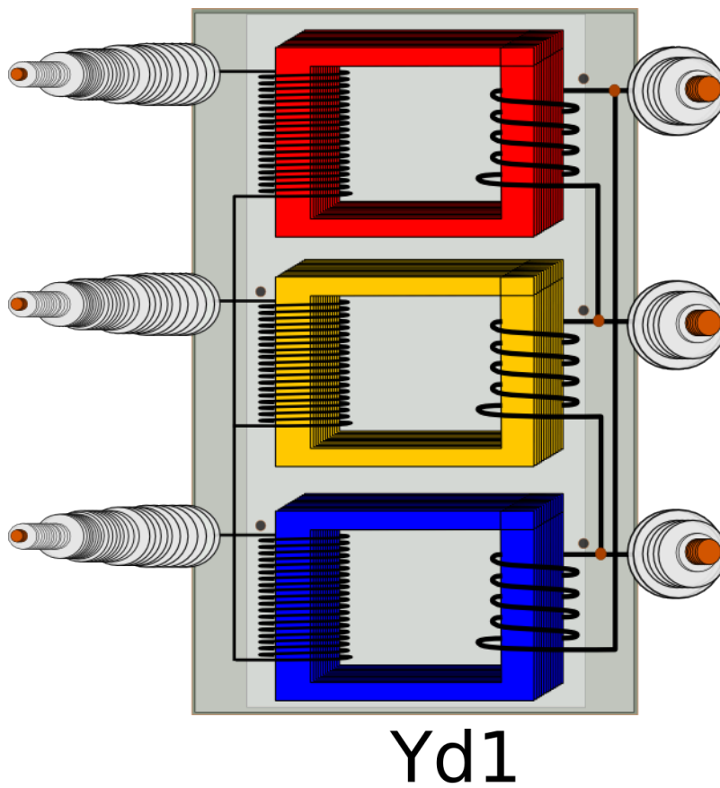
Figure. 4.4.7 - 39. Yd1 transformer's internal connection (in theory).
