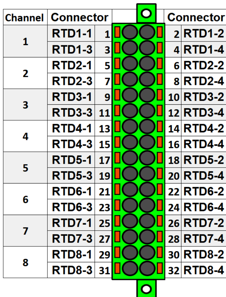
Figure. 7.4.7 - 120. RTD input module connectors.
