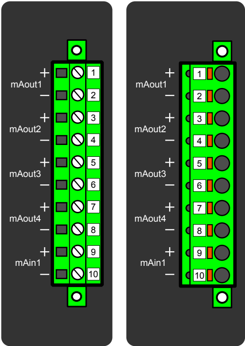
Figure. 7.4.4 - 117. Milliampere output (mA) I/O module connections. Can be equipped with standard screw terminals or spring cage terminals for connection.
