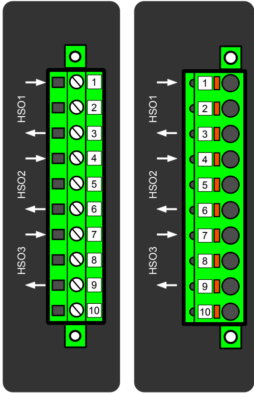
Figure. 7.4.3 - 116. High-speed and high-current output module with three add-on high-speed outputs. Can be equipped with standard screw terminals or spring cage terminals for connection.
