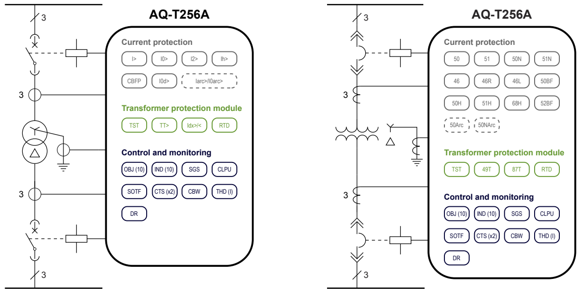
Figure. 6.1 - 106. AQ-T256 application example with function block diagram.
