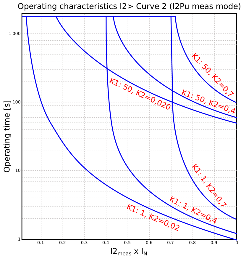
Figure. 4.4.3 - 19. Operation characteristics curve for I2> Curve2.
