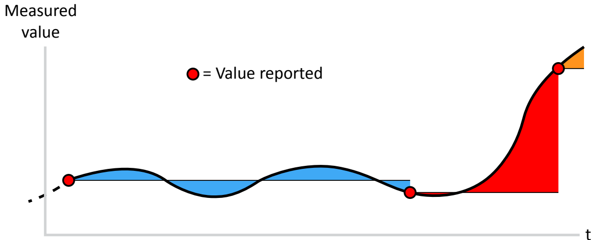
Figure. 5.3.9 - 102. Example graph showing how integration time affects measurement reporting. Small changes take longer to increase the integrated value over the deadband setting (blue area). Big changes meet the deadband criteria faster (red area).
