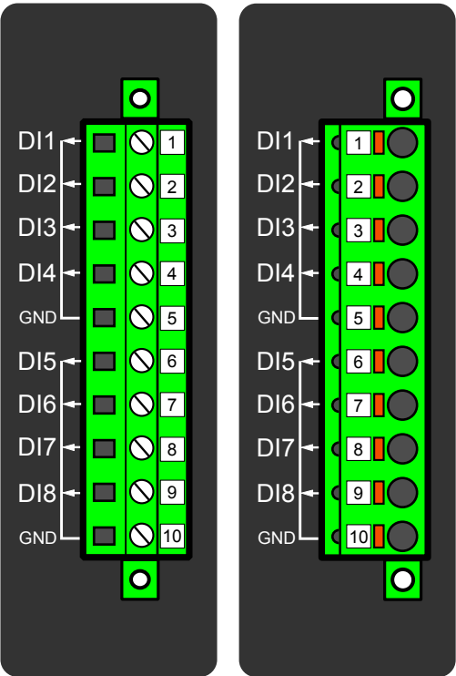
Figure. 7.4.1 - 113. Digital input module (DI8) with eight add-on digital inputs. Can be equipped with standard screw terminals or spring cage terminals for connection.
