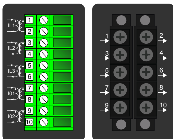
Figure. 7.3 - 112. Module connections with standard and ring lug terminals.
