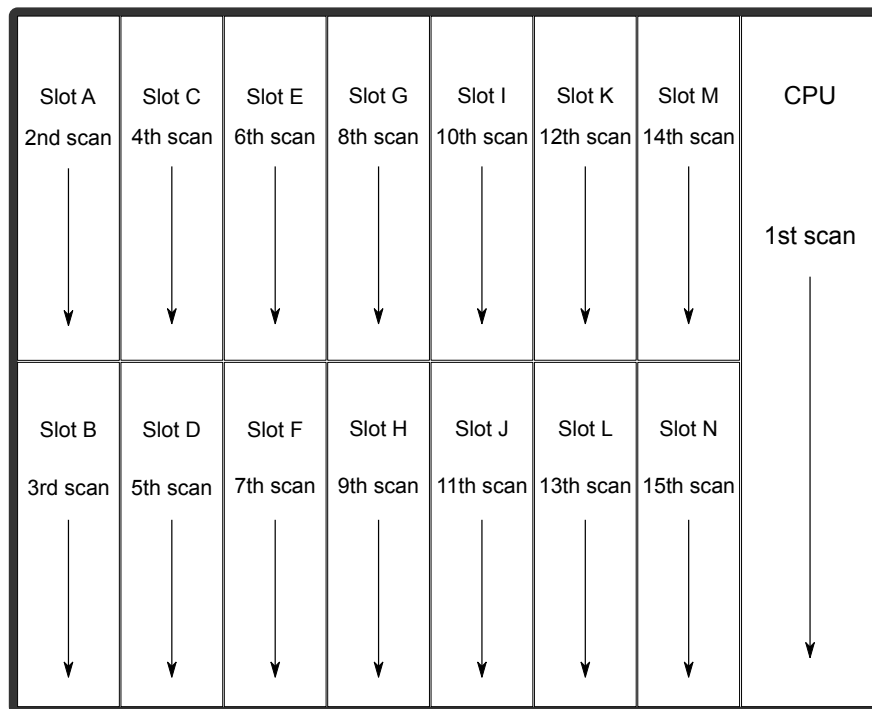
Figure. 7.1 - 110. AQ-X255 hardware scanning and I/O naming principles.
