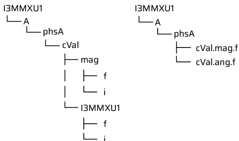
Figure. 5.3.8 - 100. Nested structure (left) and flat structure (right) comparison.
