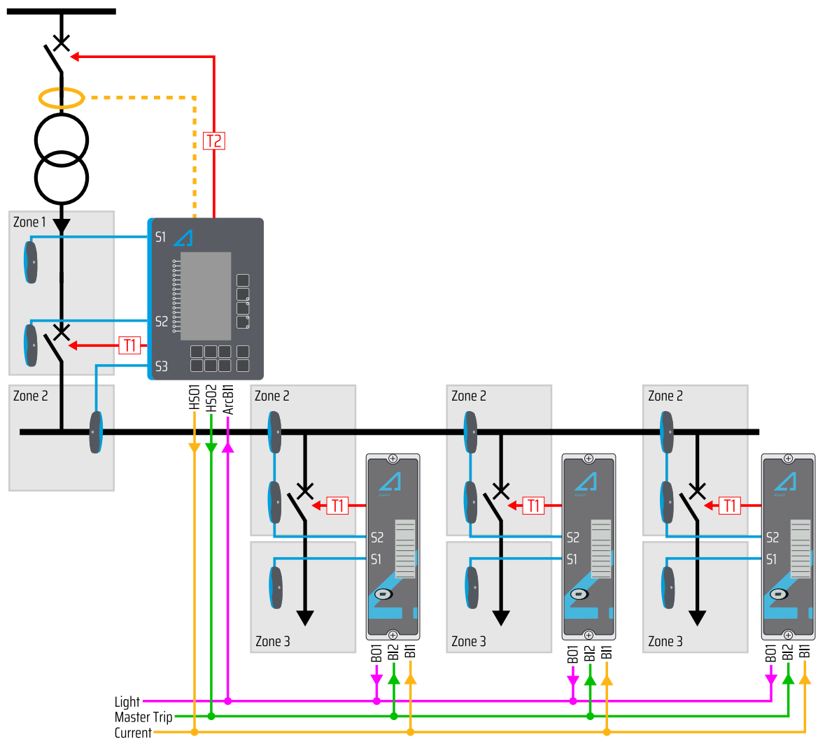
Figure. 4.4.11 - 56. Scheme with AQ-101 arc protection relays.
