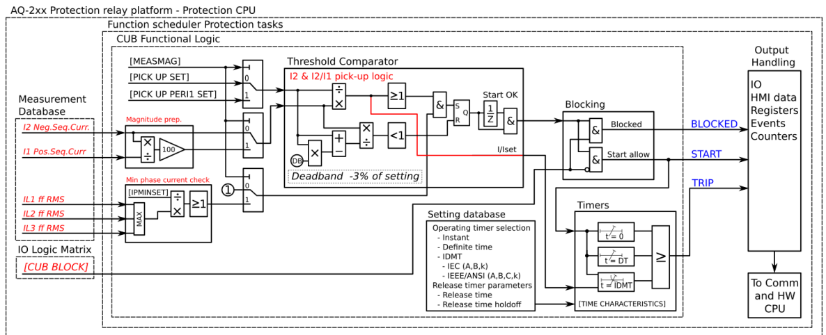
Figure. 4.4.3 - 18. Simplified function block diagram of the I2&gt; function.
