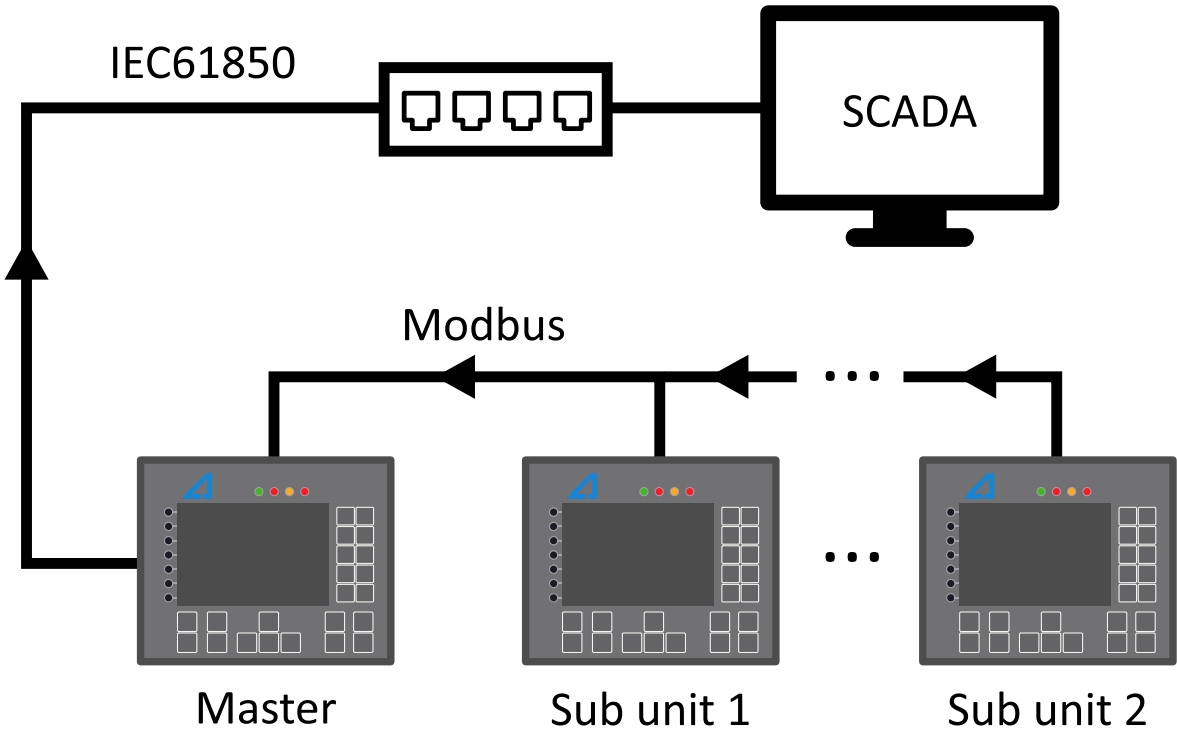
Figure. 5.5 - 105. Example setup of Modbus Gateway application.
