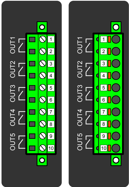
Figure. 7.4.2 - 115. Digital output module (DO5) with five add-on digital outputs. Can be equipped with standard screw terminals or spring cage terminals for connection.
