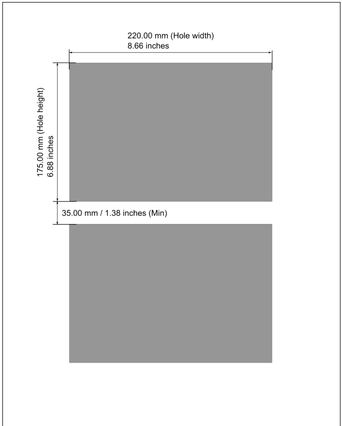
Figure. 7.5 - 130. Panel cut-out and spacing of the devices.
