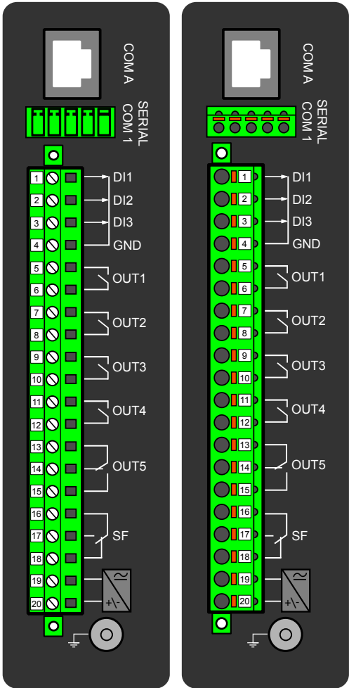
Figure. 7.2 - 111. CPU module can be equipped with standard screw terminals or spring cage terminals for connection.
