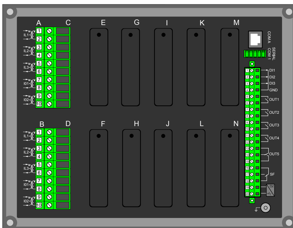
Figure. 7.1 - 108. Modular construction of AQ-X256-XXXXXXX-AAAAAAAAAA
