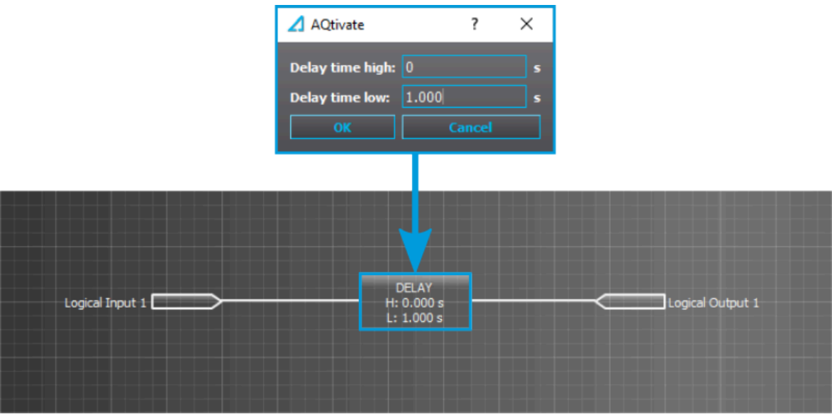
Figure. 4.5.12 - 79. Extending a logical input pulse.
