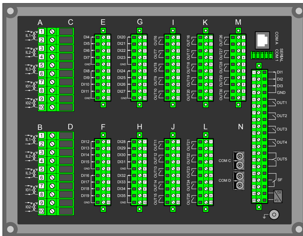
Figure. 7.1 - 109. Modular construction of AQ-X256-XXXXXXX-BBBBCCCCCJ
