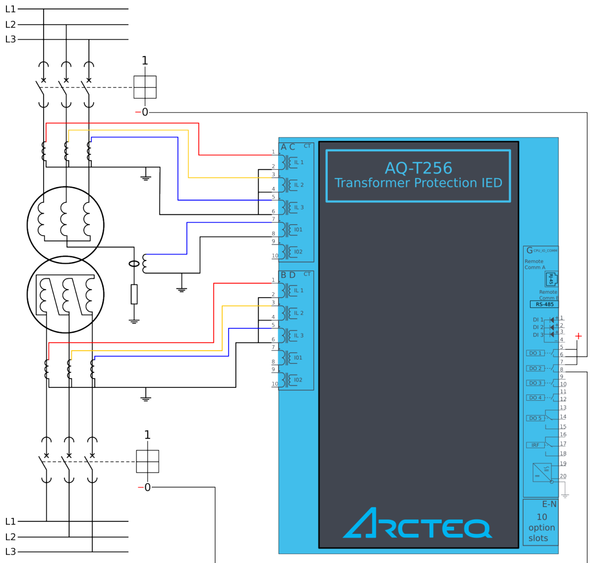
Figure. 6.2 - 107. Application example and its connections.
