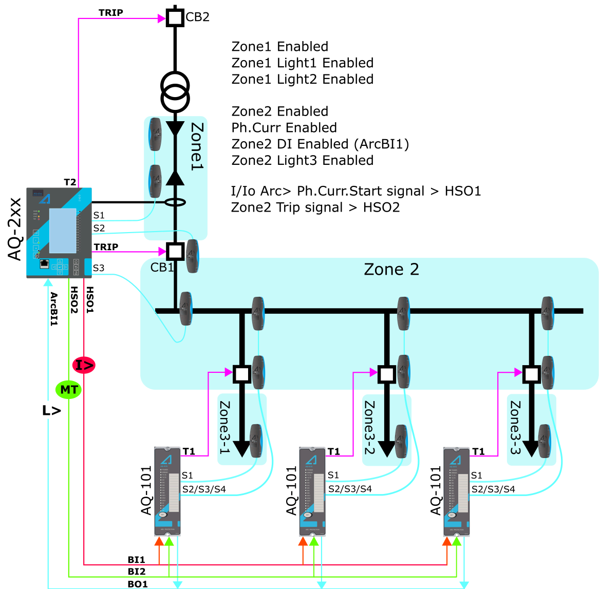
Figure. 5.4.24 - 161. Scheme with AQ-101 arc protection relays.
