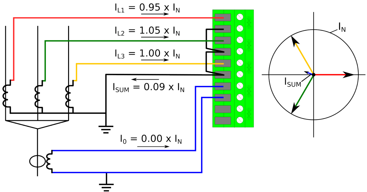
Figure. 5.4.9 - 112. Cable end differential with natural unbalance in the phase current measurement.
