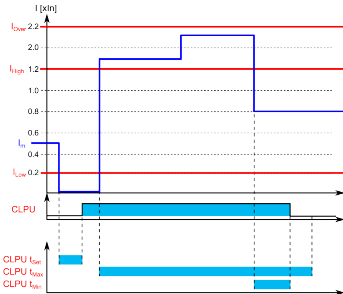
Figure. 5.5.5 - 186. Example of timers and pick-up parameters (normal CLPU situation).
