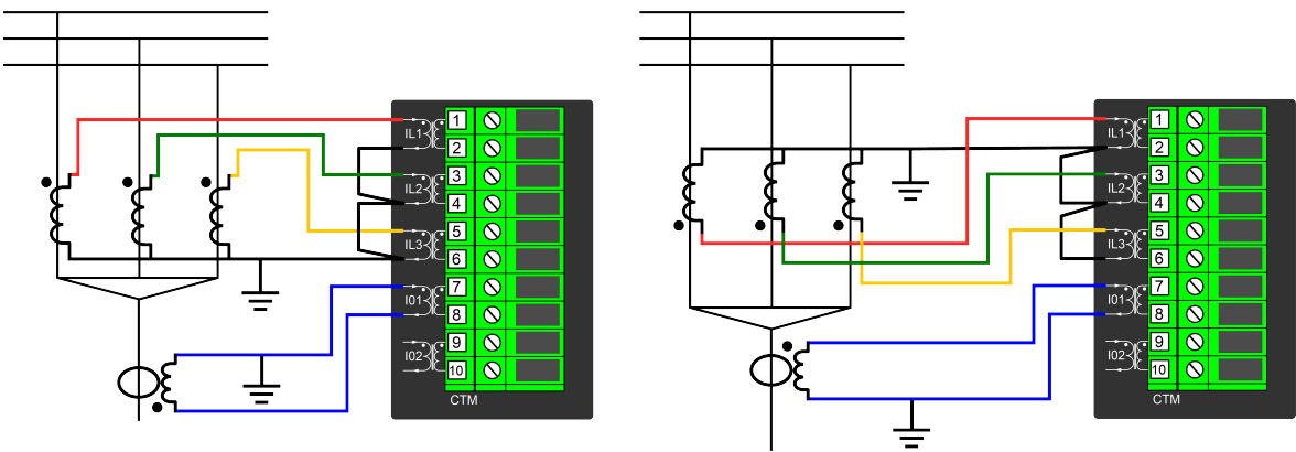
Figure. 5.4.9 - 107. "IO direction" parameter must be set to "Add" when current transformers are facing each other or away from each other.
