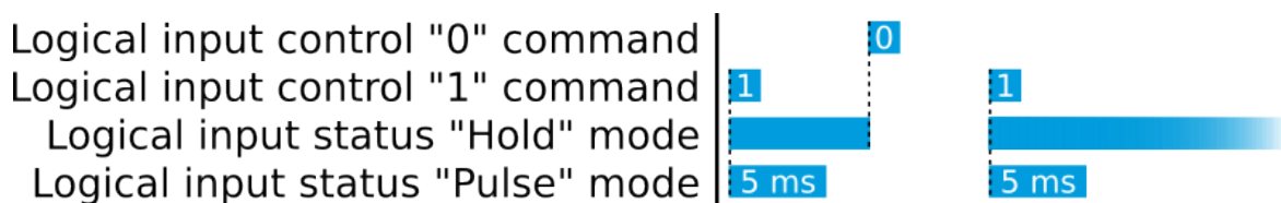
Figure. 5.5.12 - 208. Operation of logical input in "Hold" and "Pulse" modes.
