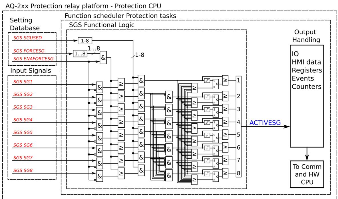
Figure. 5.5.2 - 178. Simplified function block diagram of the setting group selection function.
