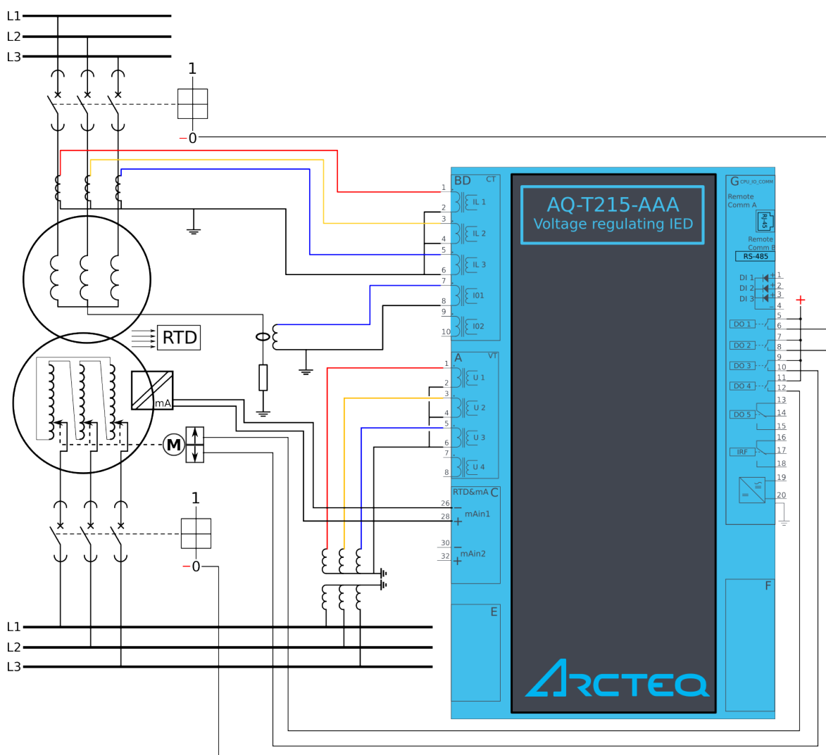
Figure. 7.2.1 - 235. Application example and its connections.
