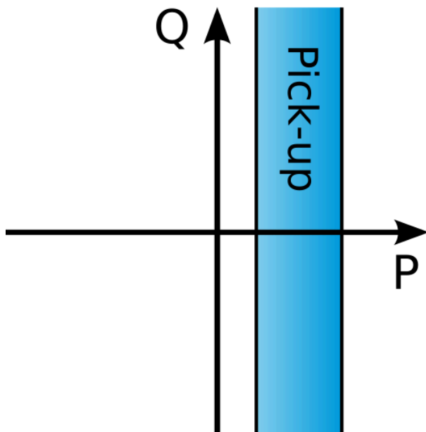
Figure. 5.4.15 - 139. Operating characteristics of underpower protection.
