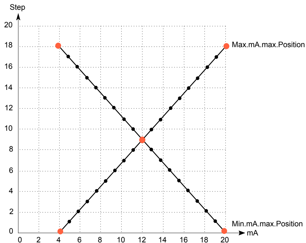
Figure. 5.5.1 - 167. Switching the tap position indication.
