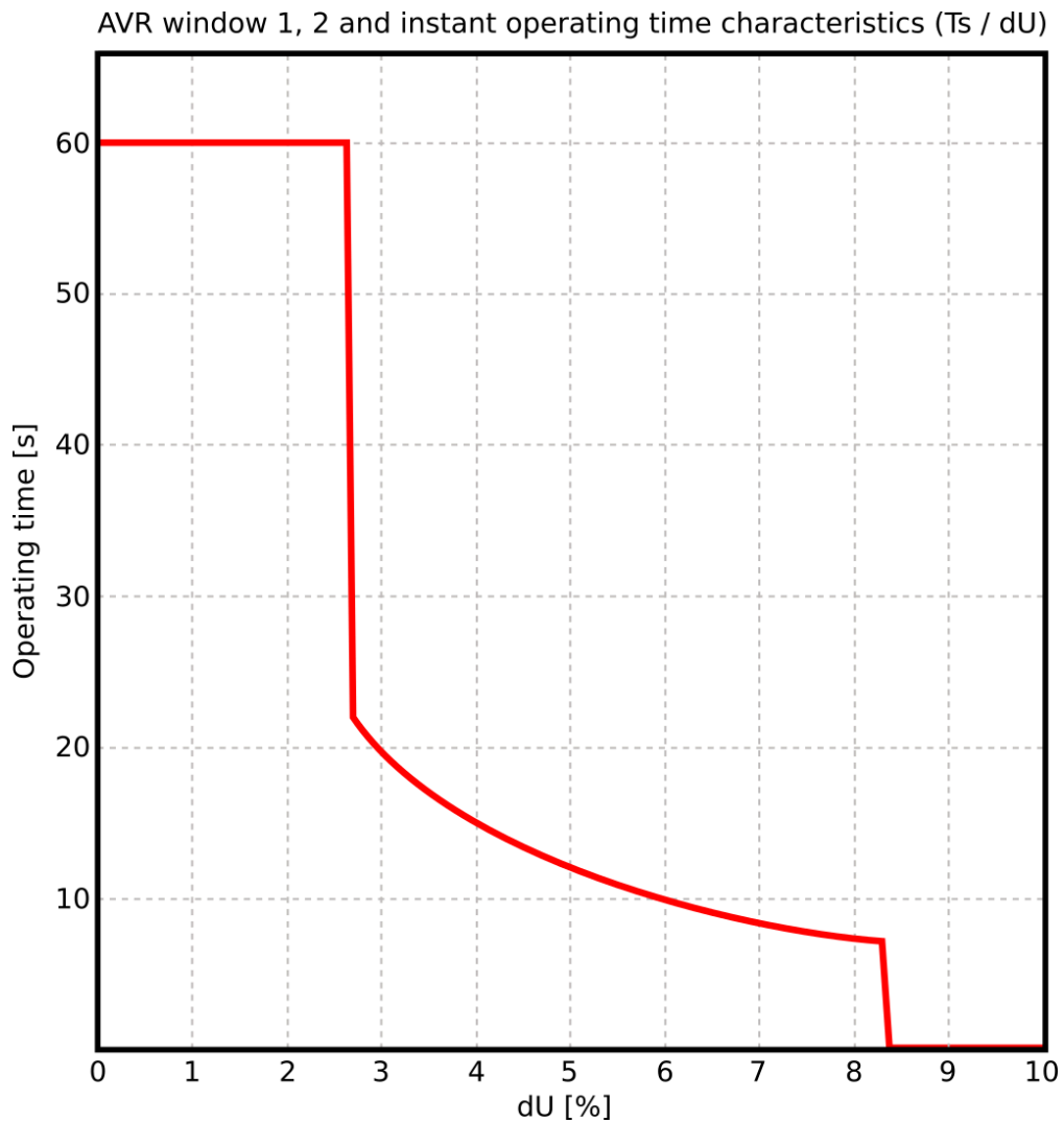
Figure. 5.5.1 - 176. Effect of the Instant low setting on time characteristics.
