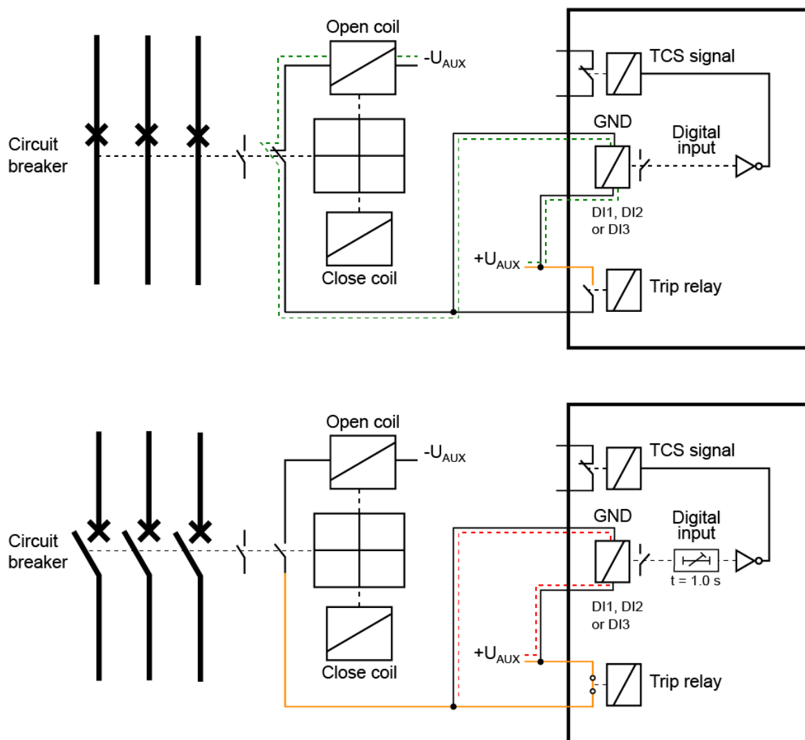
Figure. 7.2.2 - 238. Trip circuit supervision with one DI and one latched output contact.
