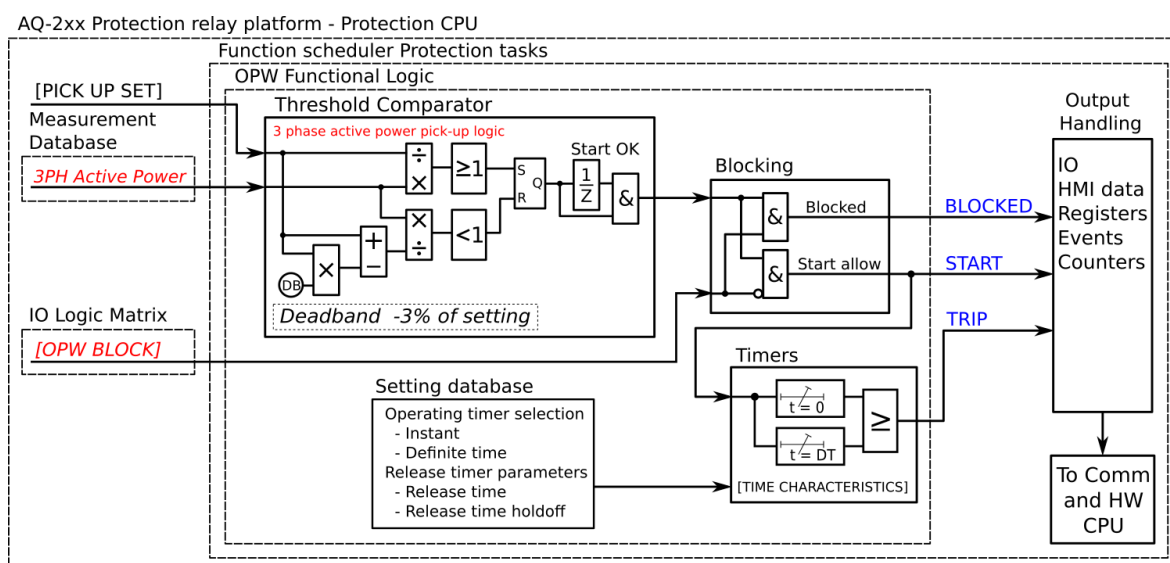
Figure. 5.4.14 - 138. Simplified function block diagram of the P&gt; function.
