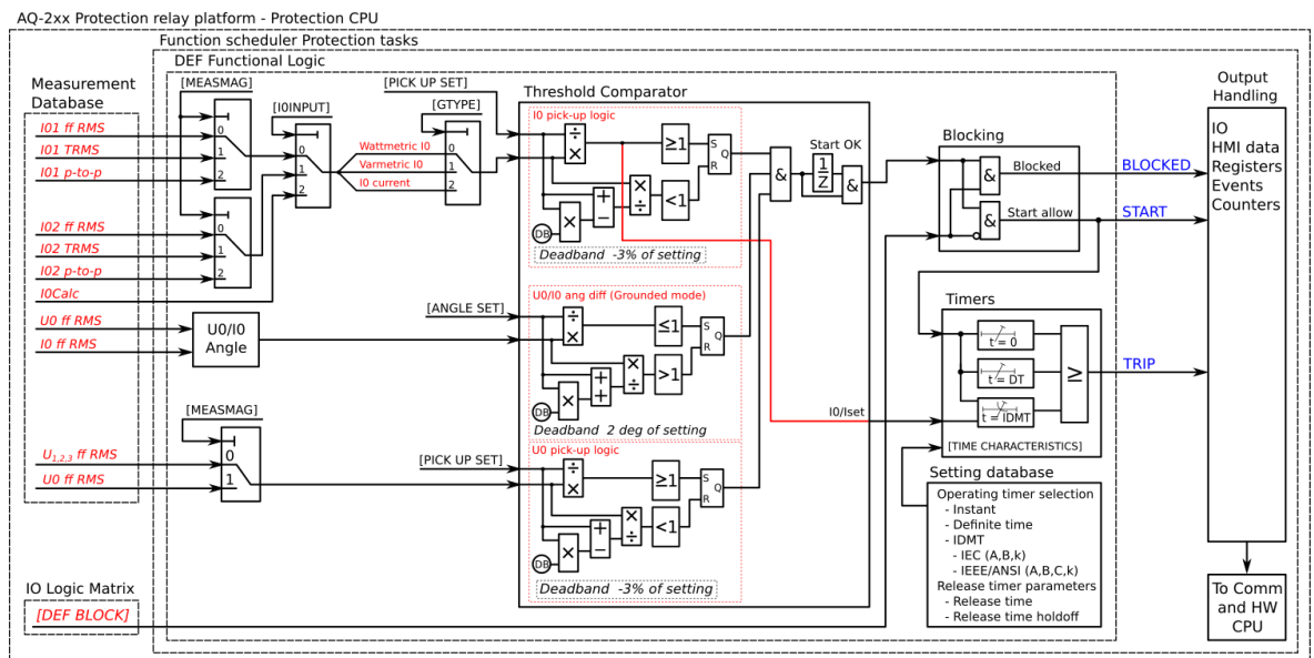
Figure. 5.4.5 - 85. Simplified function block diagram of the I0dir> function.
