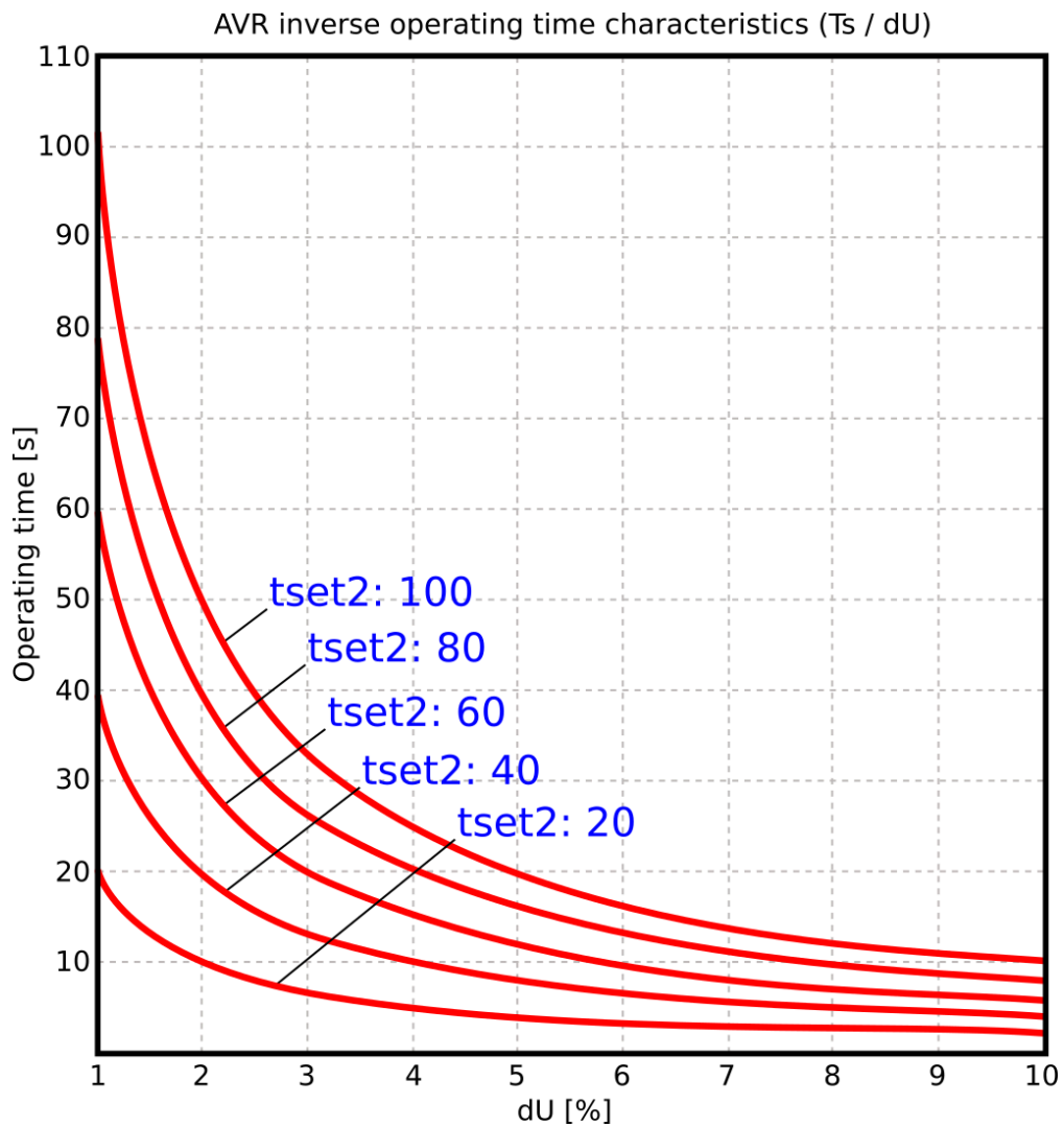
Figure. 5.5.1 - 173. Inverse operating time characteristics for the second voltage window ( U > > / < < \text{window} ).
