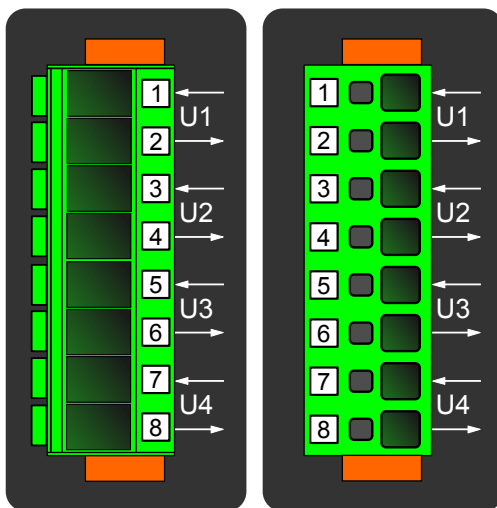
Figure. 8.4 - 244. Voltage measurement module can be equipped with standard screw terminals or spring cage terminals for connection.
