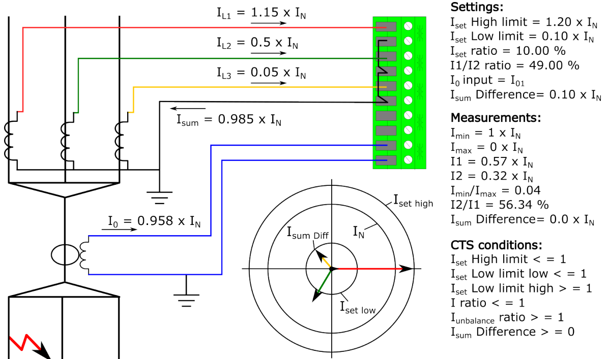
Figure. 5.6.1 - 220. Primary side high-impedance earth fault.
