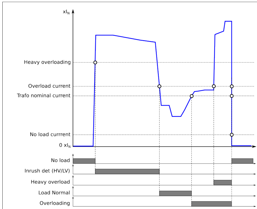
Figure. 5.4.21 - 155. Activation of the function's outputs.
