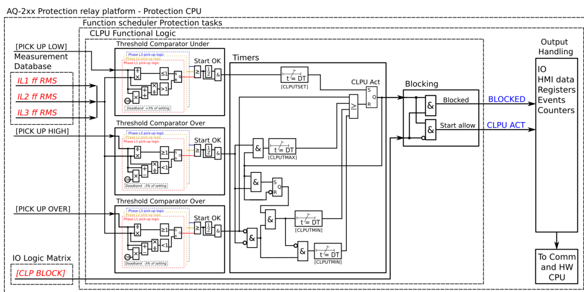
Figure. 5.5.5 - 185. Simplified function block diagram of the cold load pick-up function.
