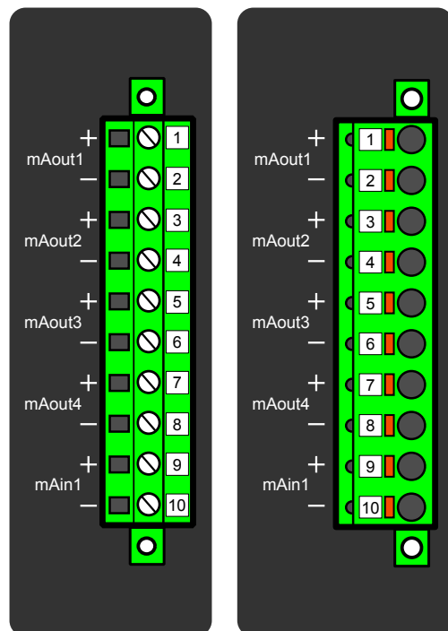
Figure. 8.5.9 - 256. Milliampere output (mA) I/O module connections. Can be equipped with standard screw terminals or spring cage terminals for connection.
