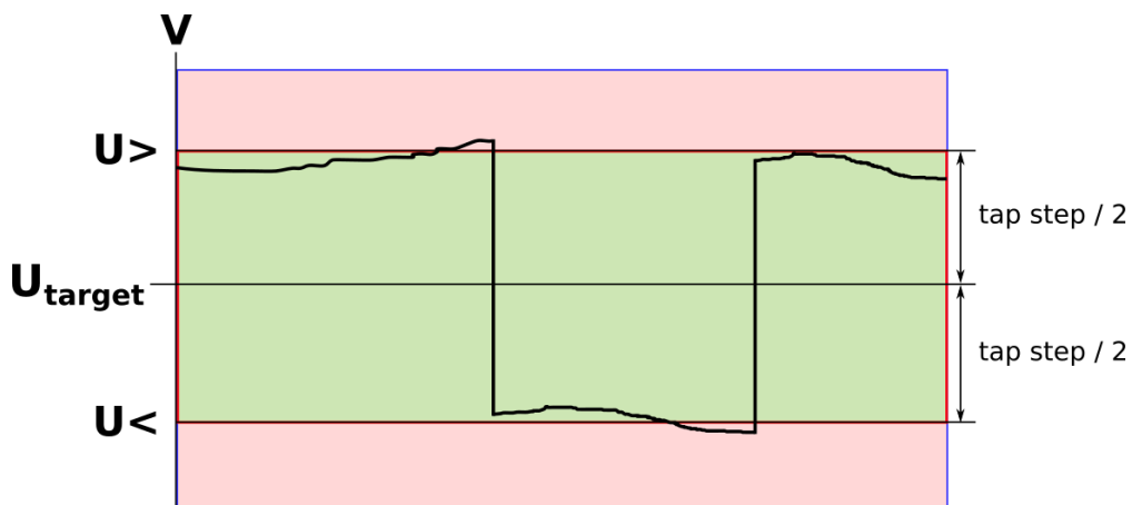
Figure. 5.5.1 - 170. Tight voltage window (window reached but voltage near the limit).
