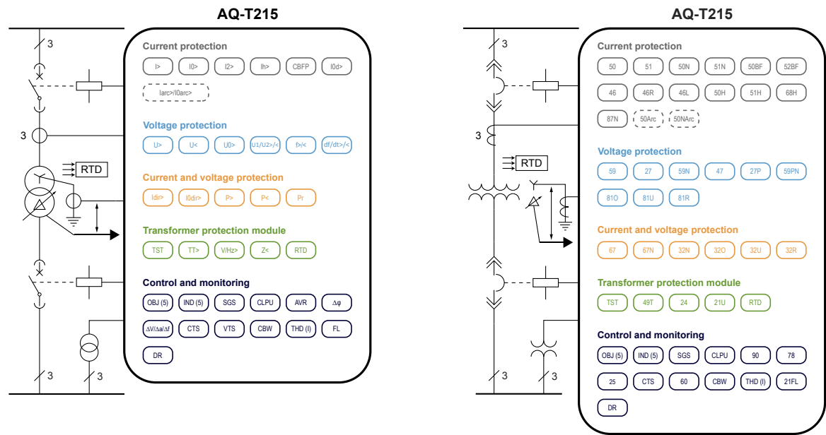
Figure. 7.1.1 - 234. AQ-T215 application example with function block diagram.
