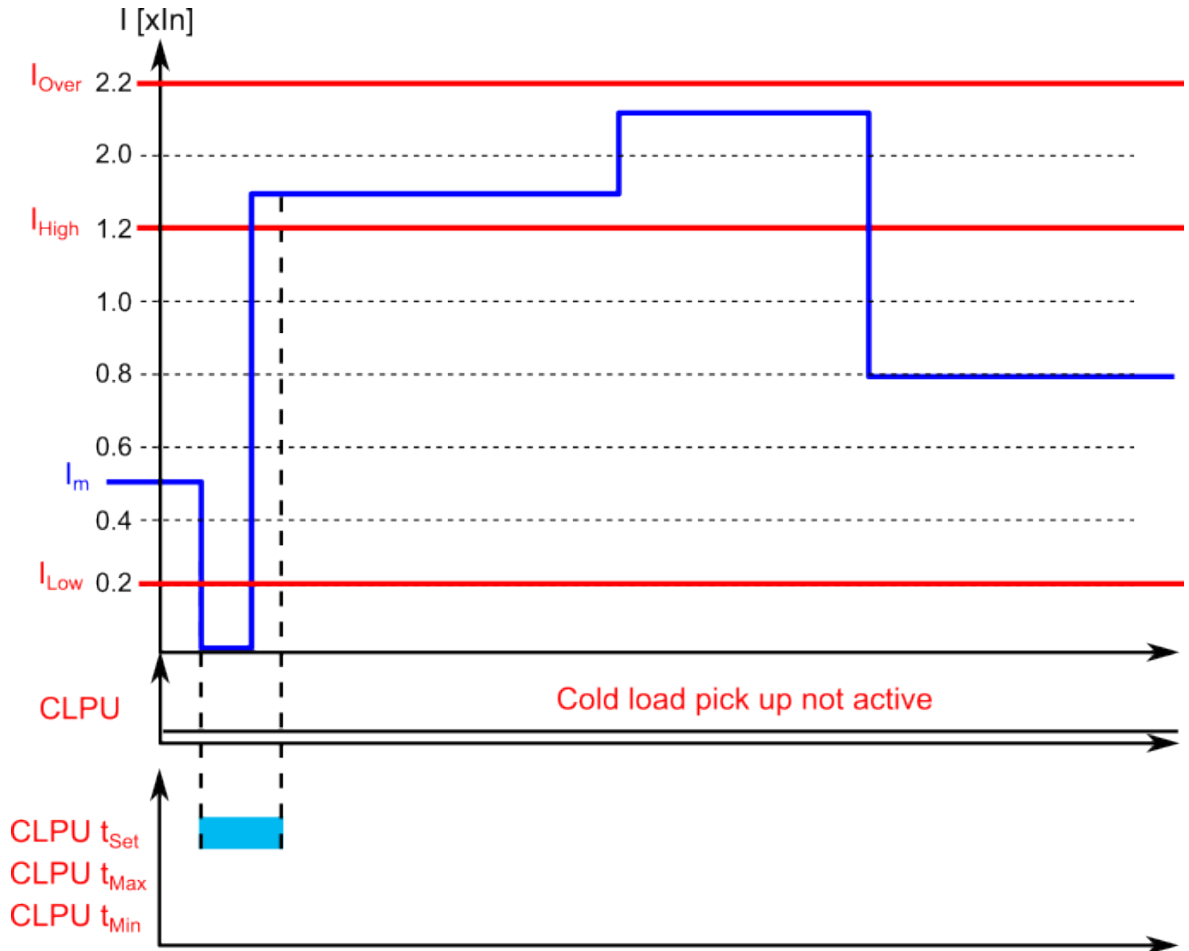
Figure. 5.5.5 - 187. Example of timers and pick-up parameters (no cold load pick-up, I_{low} too short).
