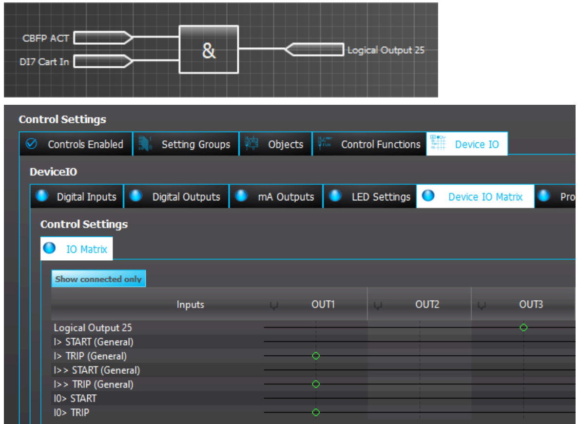
Figure. 5.5.11 - 207. Logic output example. Logical output is connected to an output relay in matrix.
