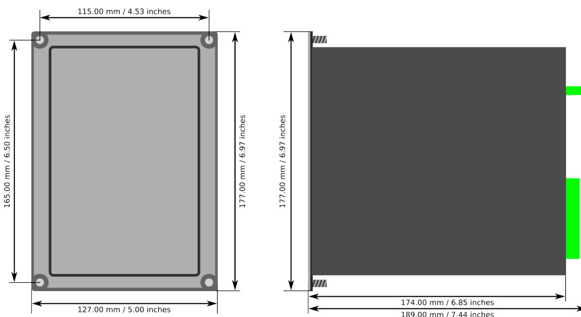
Figure. 8.6 - 257. Device dimensions.
