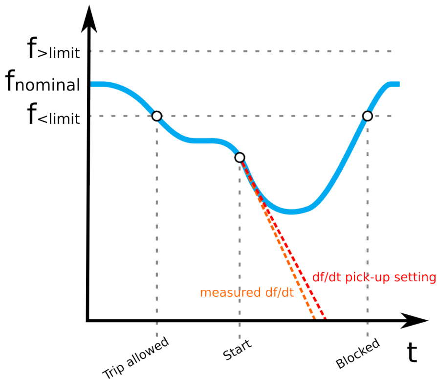
Figure. 5.4.18 - 146. Operation of the df/dt > / < function when the frequency starts but doesn't trip.
