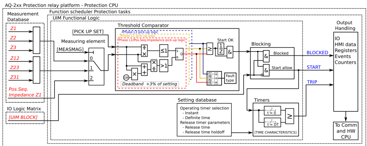
Figure. 5.4.20 - 153. Simplified function block diagram of the Z&lt; function.
