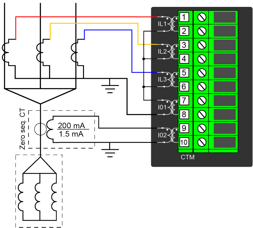
Figure. 5.2.1 - 65. Connections of ZCT scaling.
