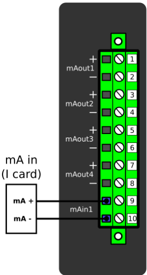
Figure. 5.5.1 - 165. Connecting mA input to option card.
