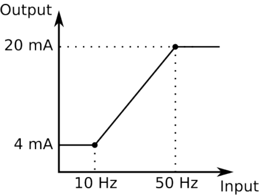
Figure. 5.5.7 - 202. Example of the effects of mA output channel settings.
