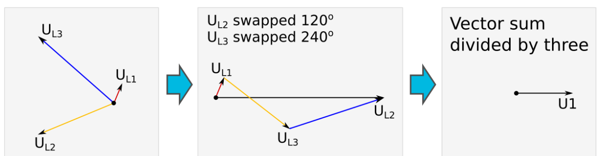
Figure. 5.4.13 - 130. Earth fault in an isolated network.
