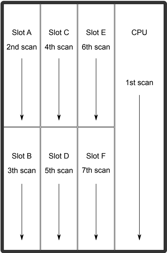
Figure. 8.1 - 241. AQ-X215 hardware scanning and I/O naming principles.
