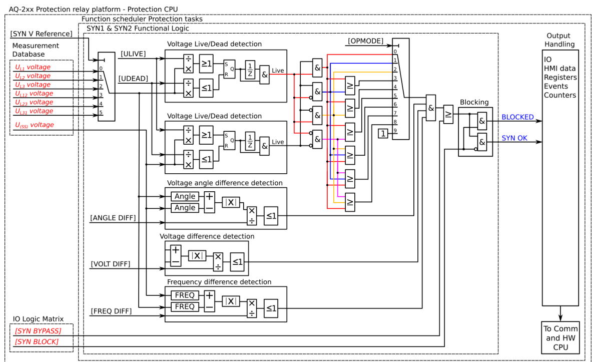
Figure. 5.5.6 - 200. Simplified function block diagram of the SYN1 and SYN2 function.
