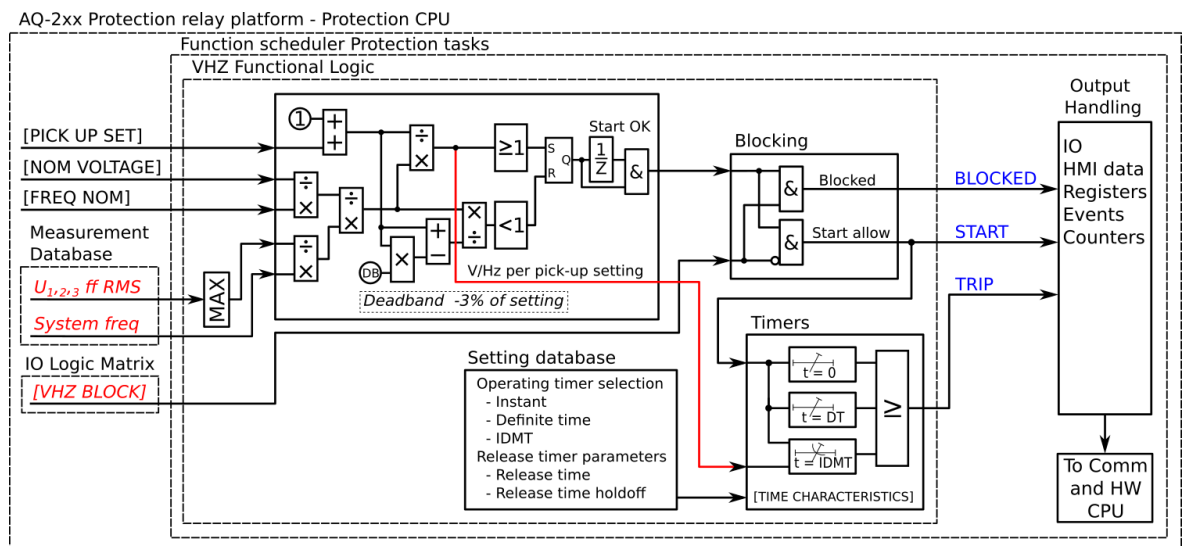
Figure. 5.4.19 - 149. Simplified function block diagram of the V/Hz> function.
