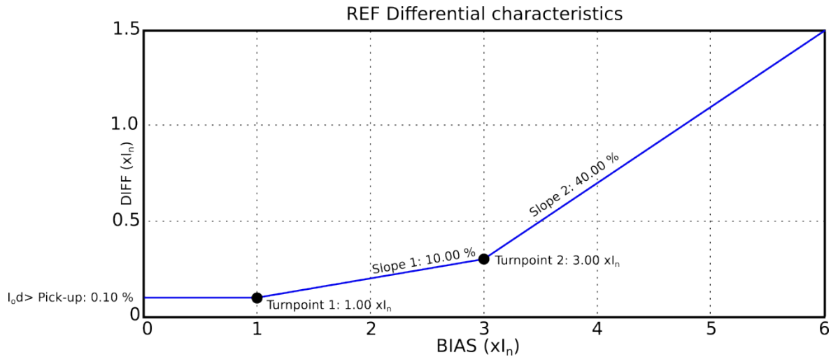
Figure. 5.4.9 - 108. Differential characteristics for the I0d&gt; function with default settings.
