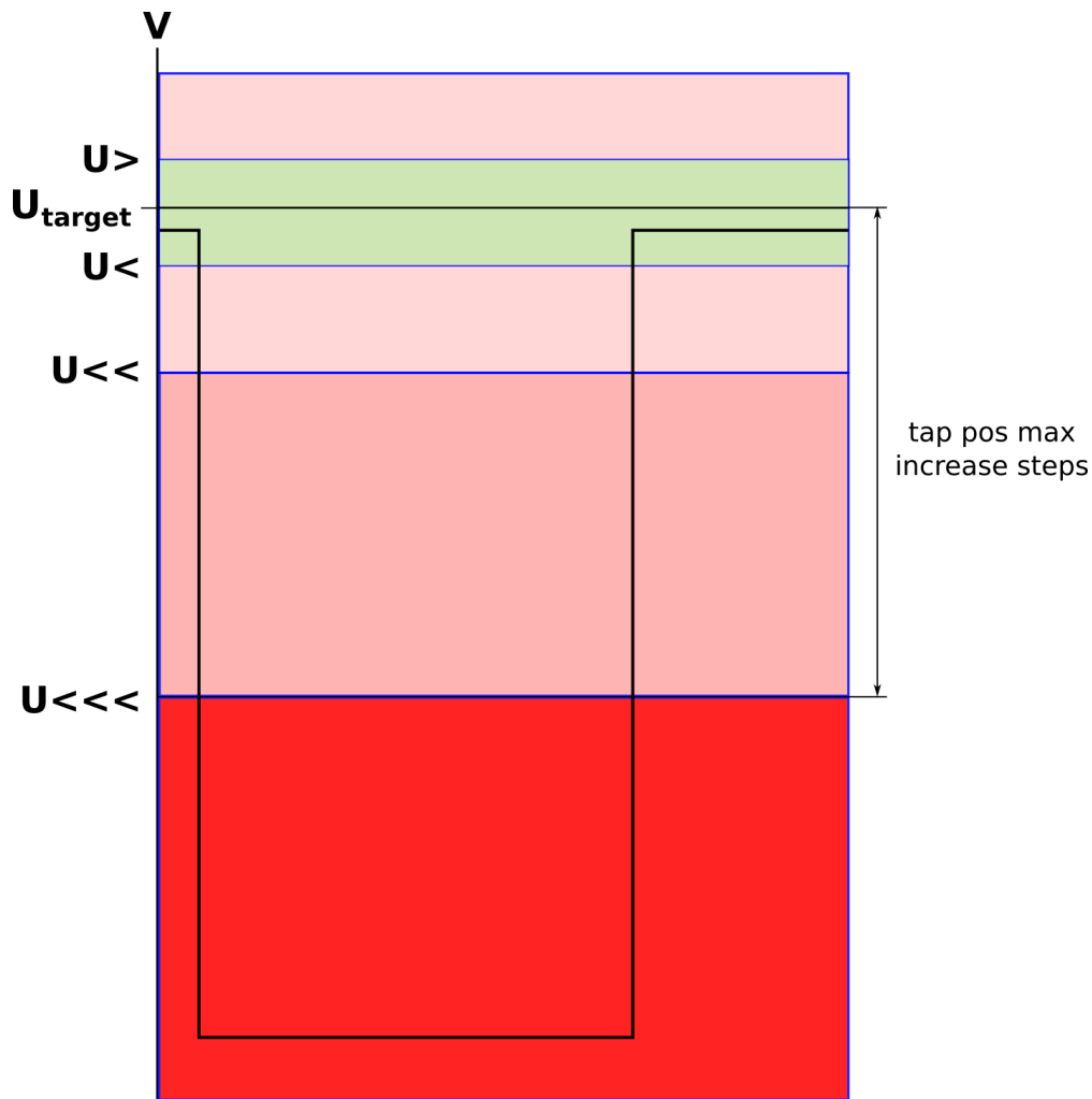
Figure. 5.5.1 - 177. Low voltage blocking.
