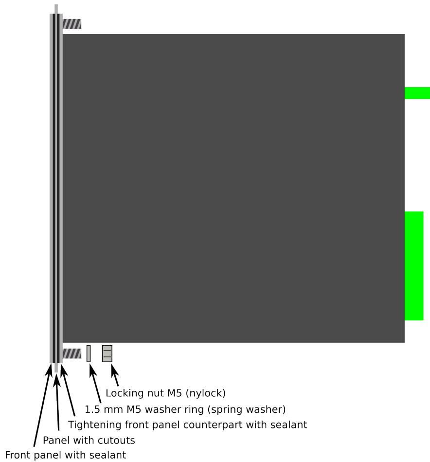
Figure. 8.6 - 258. Device installation.
