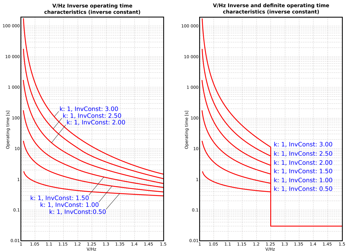
Figure. 5.4.19 - 151. Inverse (above) and inverse and DT (below) time characteristics with the inverse constant setting effect.
