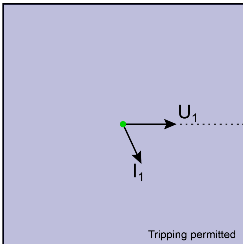
Figure. 5.4.4 - 84. When I_{dir}> function has been set to "Non-directional" the function works basically just like a traditional non-directional overcurrent protection function.
