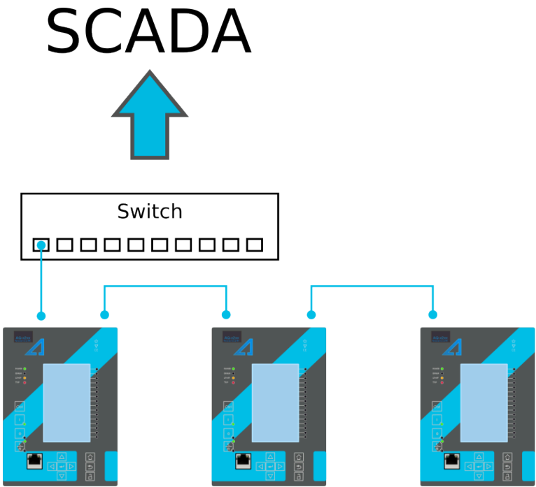
Figure. 8.5.7 - 254. Example of a multidrop configuration.
