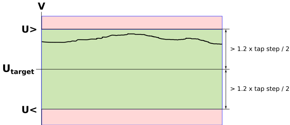
Figure. 5.5.1 - 171. Voltage window according to the recommendation.
