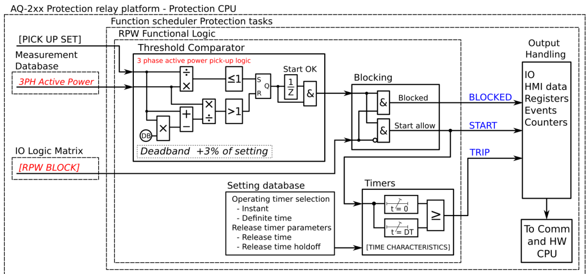
Figure. 5.4.16 - 143. Simplified function block diagram of the Pr function.
