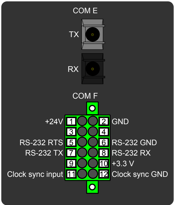
Figure. 8.5.5 - 251. Serial RS-232 module connectors.
