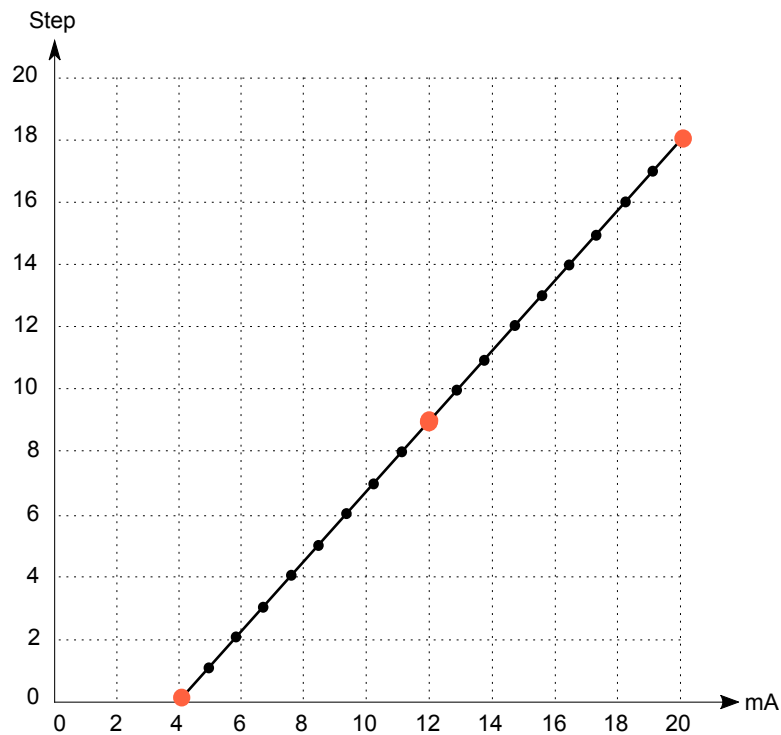
Figure. 5.5.1 - 166. Tap position indication (according to the example settings).
