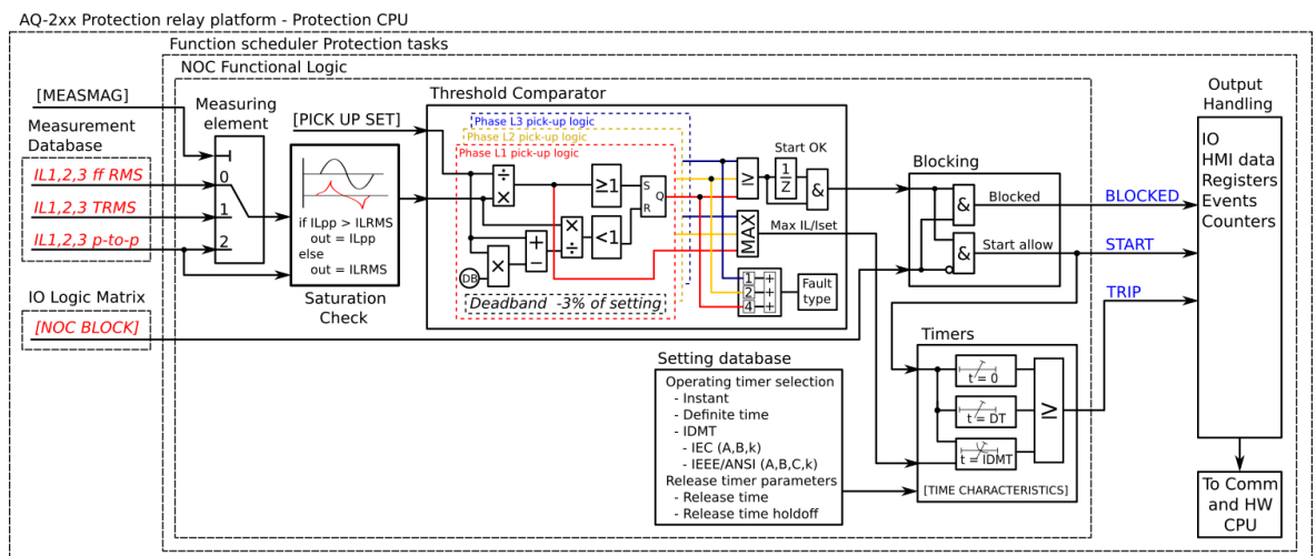
Figure. 5.4.2 - 79. Simplified function block diagram of the I > function.
