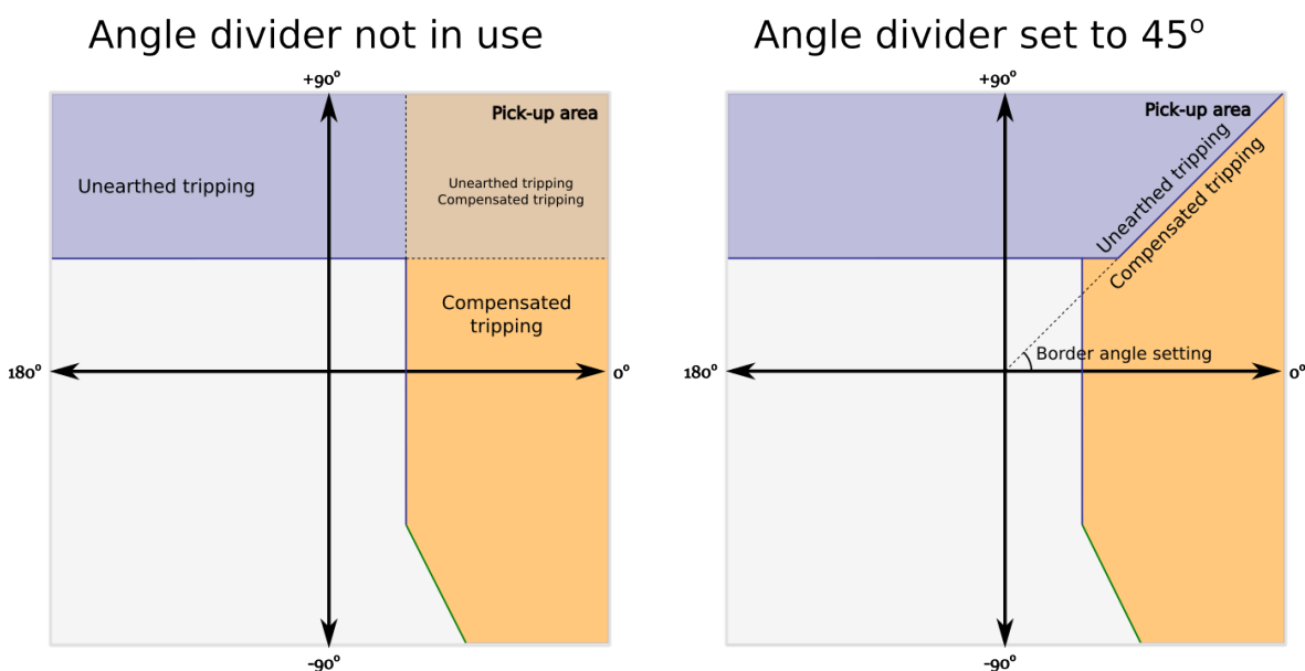
Figure. 5.4.5 - 90. Effect of angle divider when in use and when disabled.
