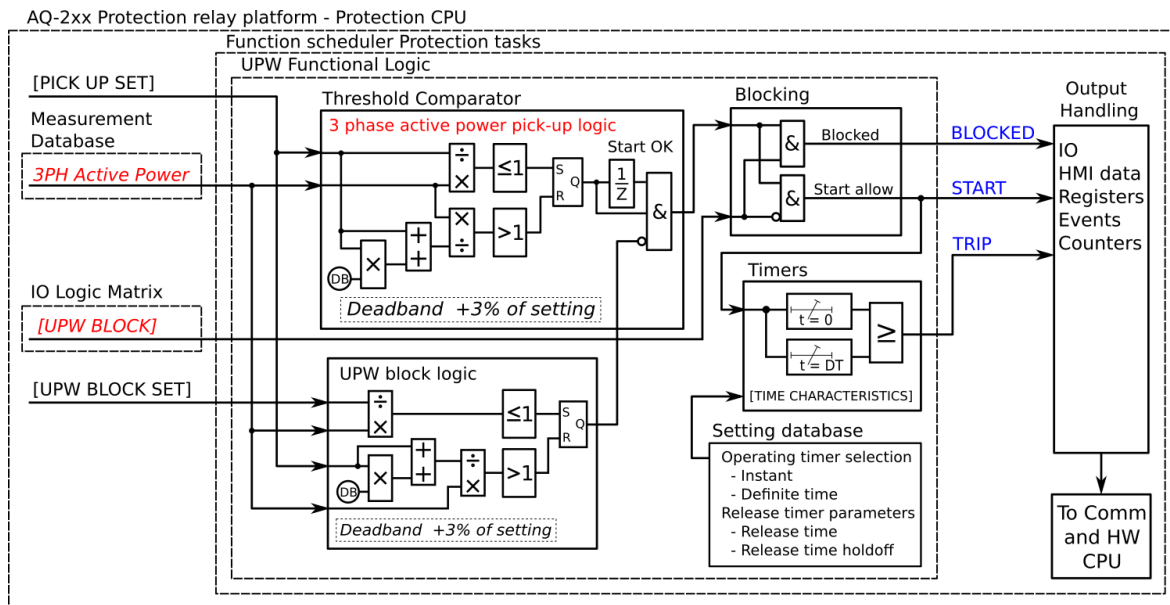
Figure. 5.4.15 - 140. Simplified function block diagram of the P< function.
