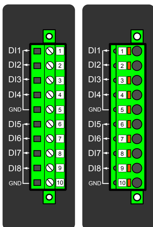
Figure. 8.5.1 - 245. Digital input module (DI8) with eight add-on digital inputs. Can be equipped with standard screw terminals or spring cage terminals for connection.
