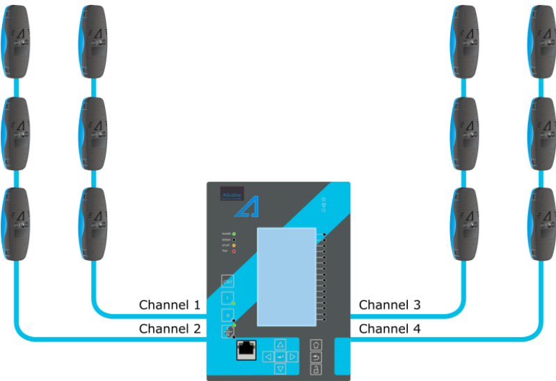
Figure. 5.4.24 - 160. Protection device equipped with arc protection.
