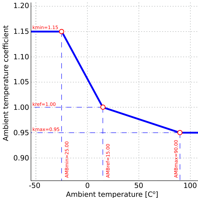
Figure. 5.4.22 - 157. Ambient temperature coefficient calculation (a three-point linear approximation and a settable correction curve).
