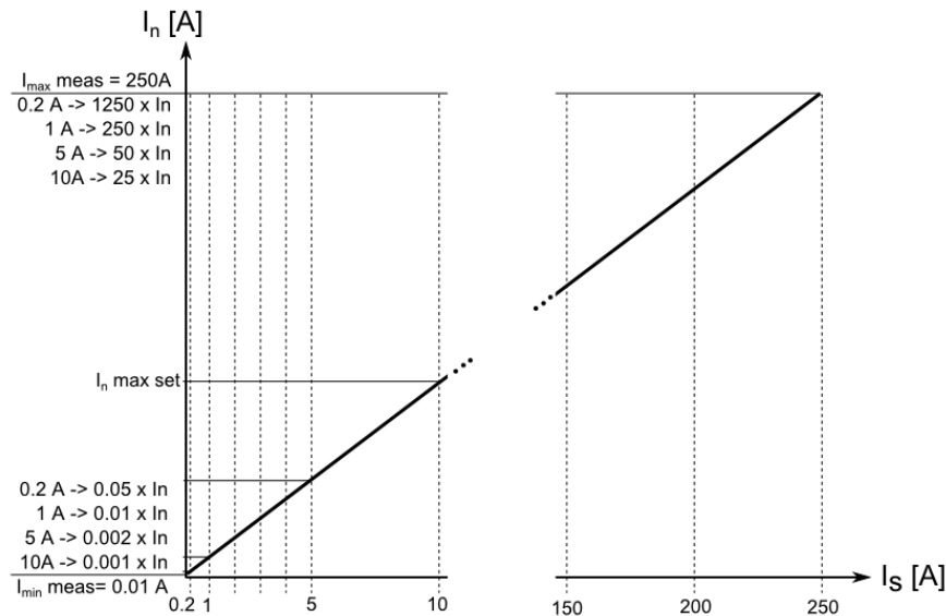
Figure. 5.4.1 - 72. Measurement range in relation to the nominal current.
