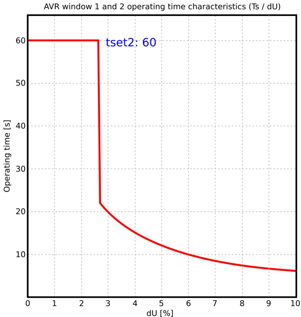
Figure. 5.5.1 - 174. Combined operating time characteristics of both voltage windows.
