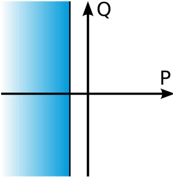
Figure. 5.4.16 - 142. Operating characteristics of reverse power protection.
