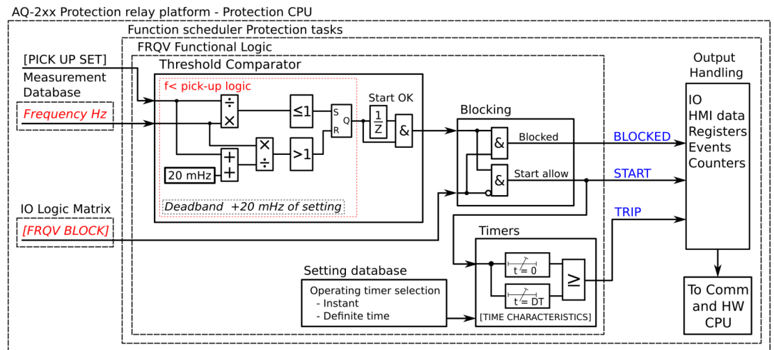
Figure. 5.4.17 - 145. Simplified function block diagram of the f< function.
