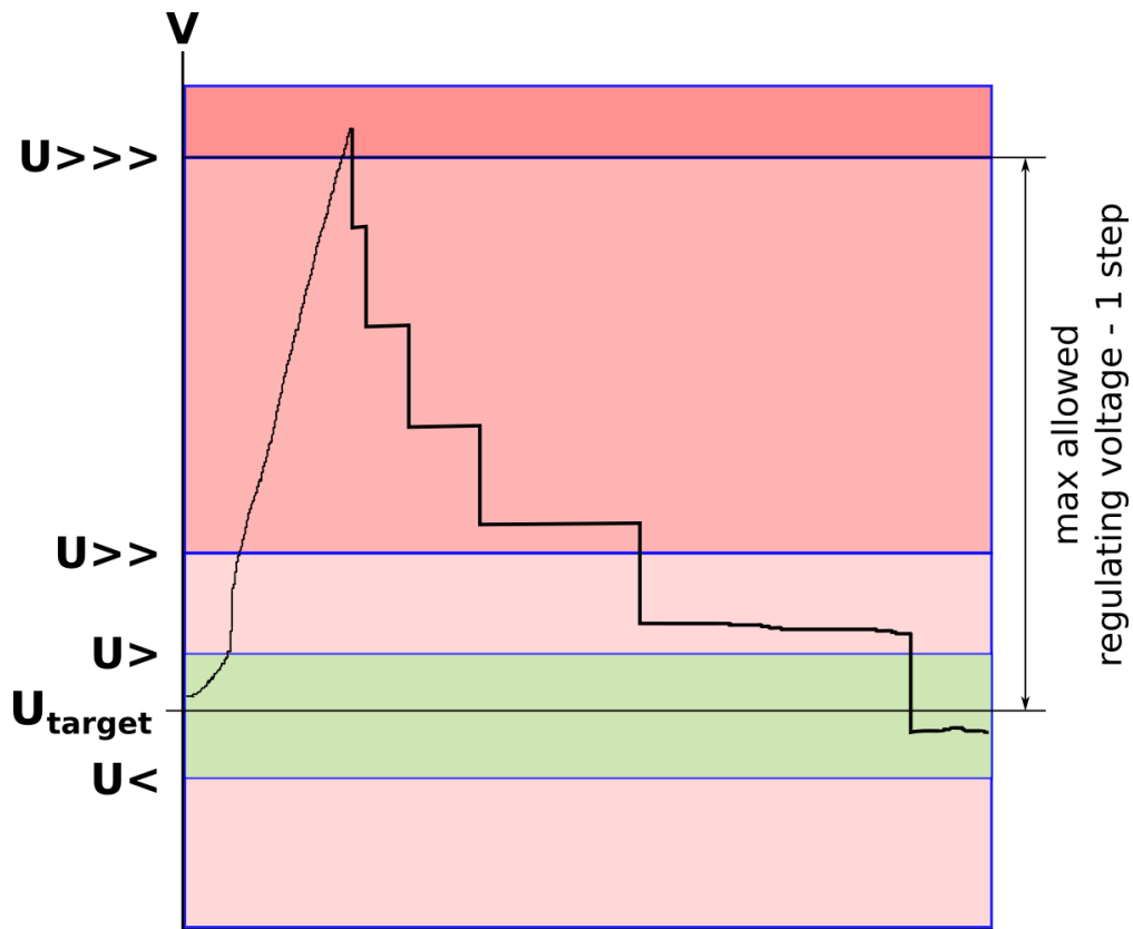
Figure. 5.5.1 - 175. Instant low command with two time-delayed windows.
