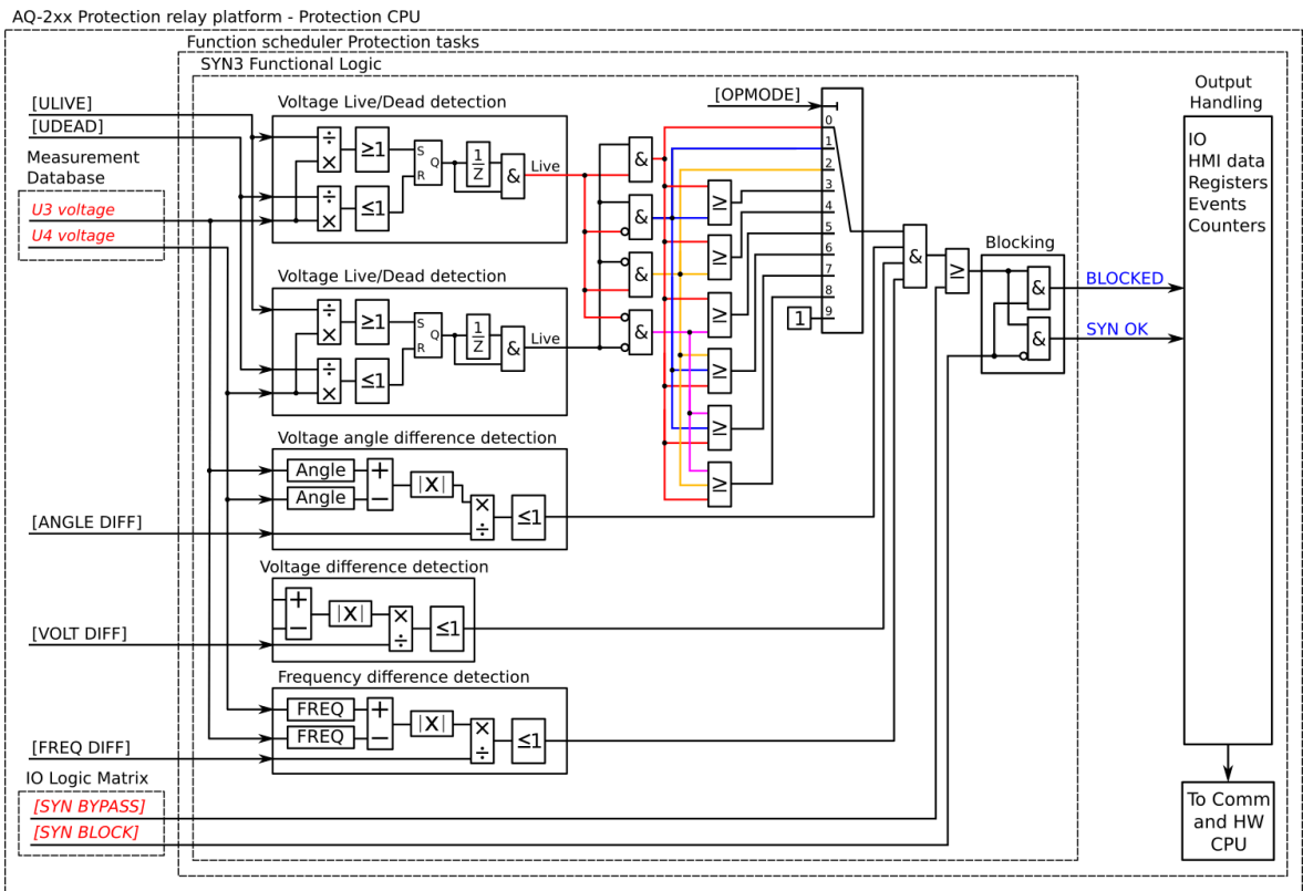
Figure. 5.5.6 - 201. Simplified function block diagram of the SYN3 function.
