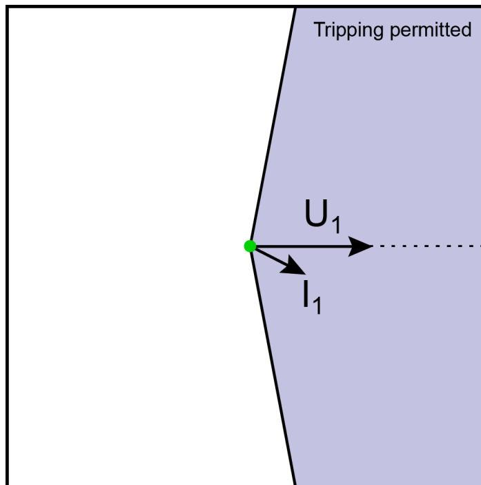
Figure. 5.4.4 - 82. Angle tracking of the I_{dir} function (3LN/3LL + U_0 mode).
