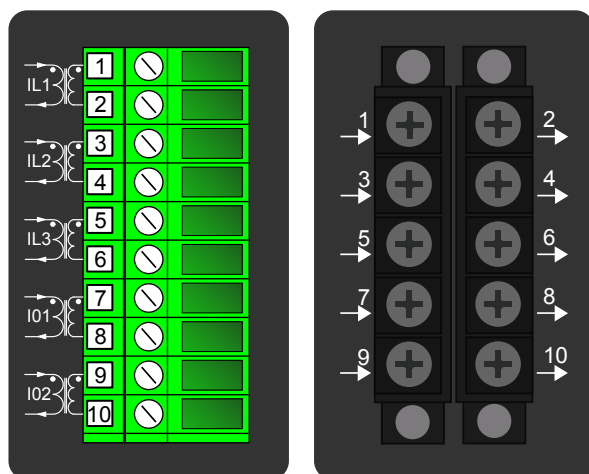
Figure. 8.3 - 243. Module connections with standard and ring lug terminals.
