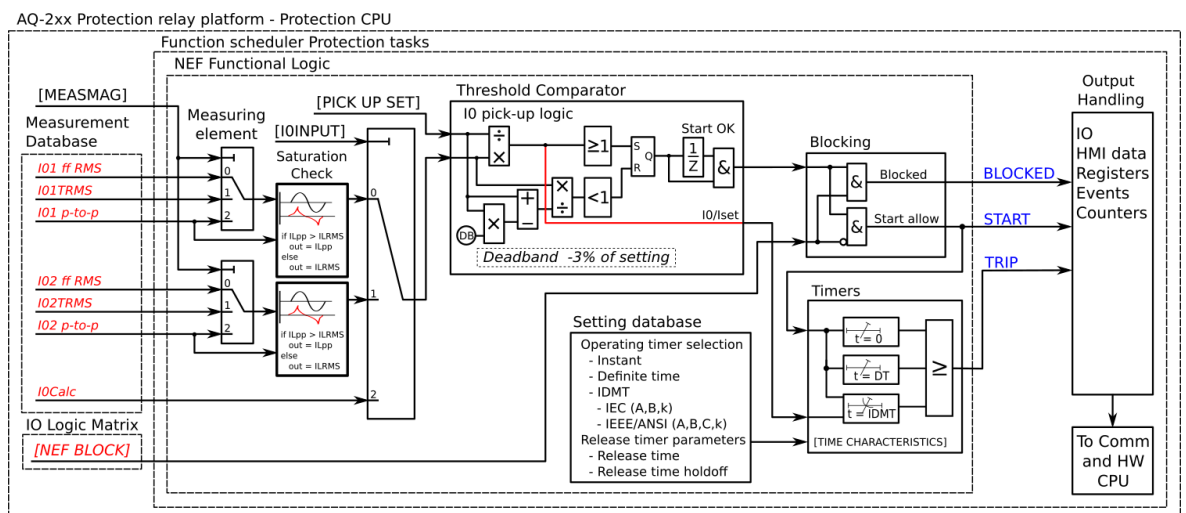
Figure. 5.4.3 - 80. Simplified function block diagram of the I_{0>} function.
