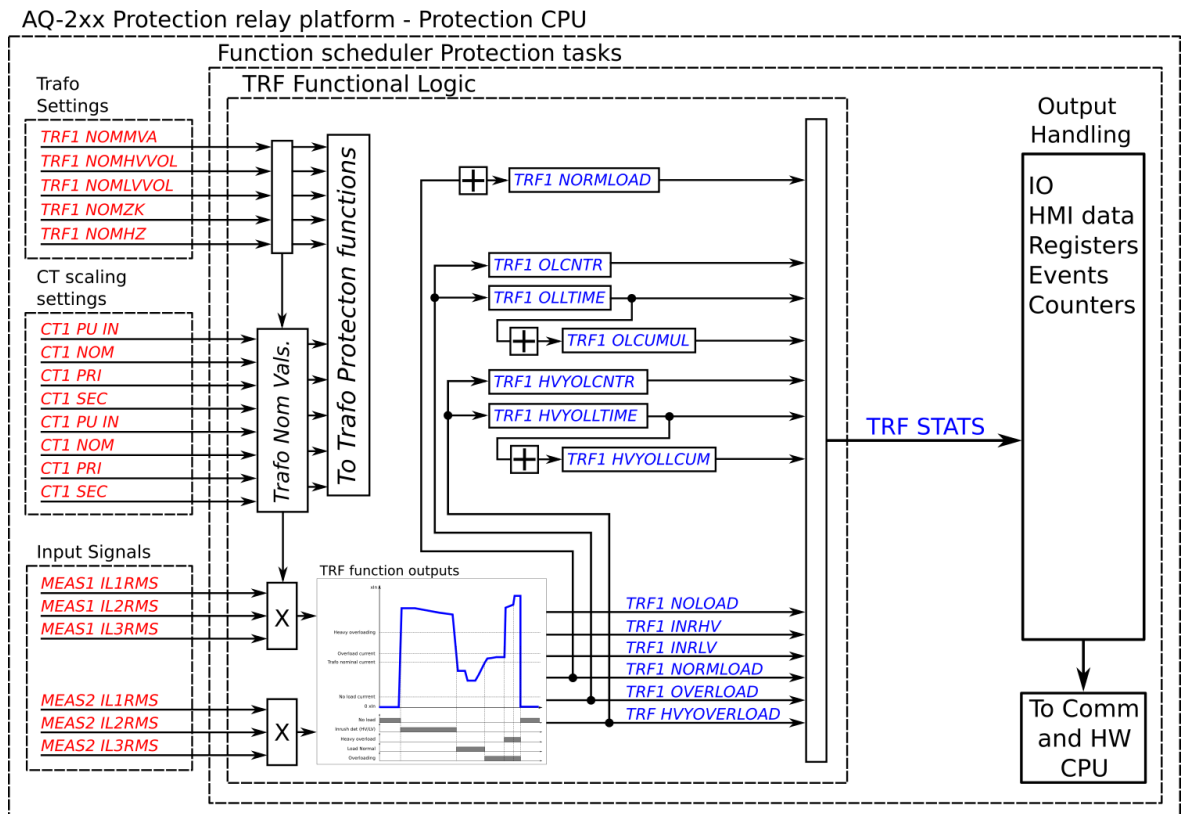
Figure. 5.4.21 - 154. Simplified function block diagram of the transformer status monitoring function.
