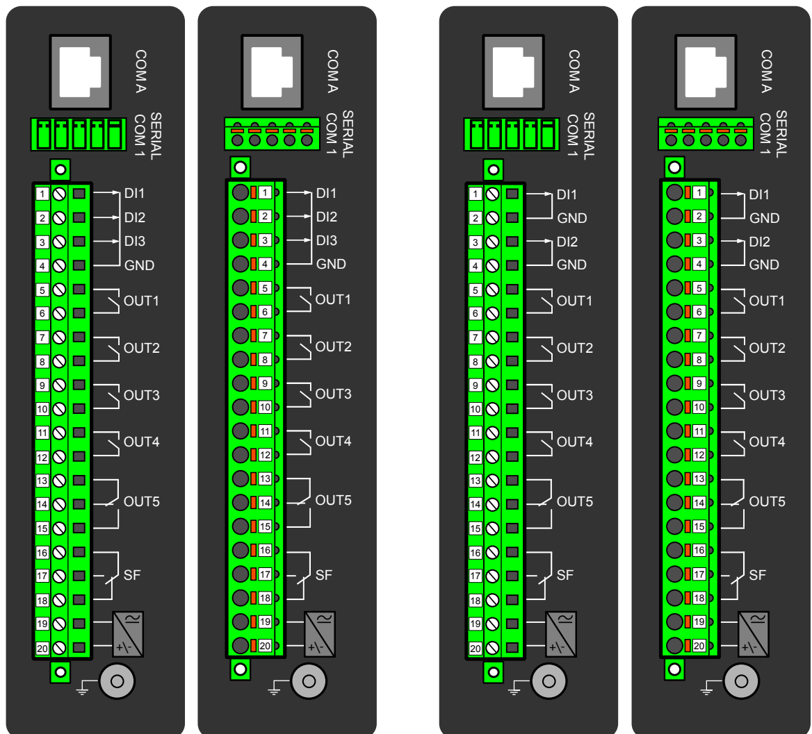
Figure. 8.2 - 242. CPU module variants are available with either two or three digital inputs, and can be equipped with standard screw terminals or spring cage terminals for connection.
