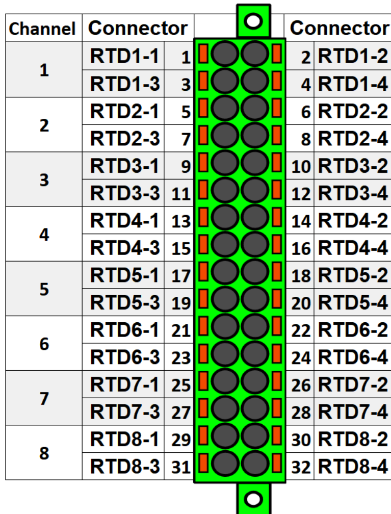
Figure. 8.5.4 - 249. RTD input module connectors.
