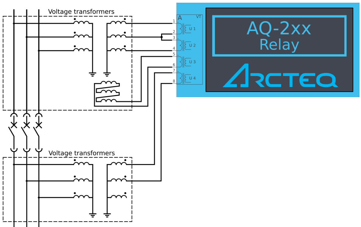
Figure. 5.5.6 - 193. Example connection of the synchrocheck function (2LL+U0+U4 mode, SYN1 in use, UL12 as reference voltage).
