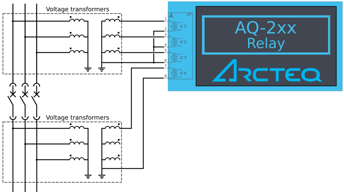
Figure. 5.5.6 - 192. Example connection of the synchrocheck function (3LN+U4 mode, SYN1 in use, UL1 as reference voltage).
