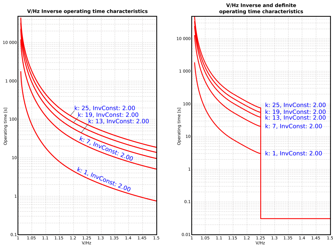
Figure. 5.4.19 - 150. Inverse (above) and inverse and DT (below) time characteristics with the TimeDial k setting effect.
