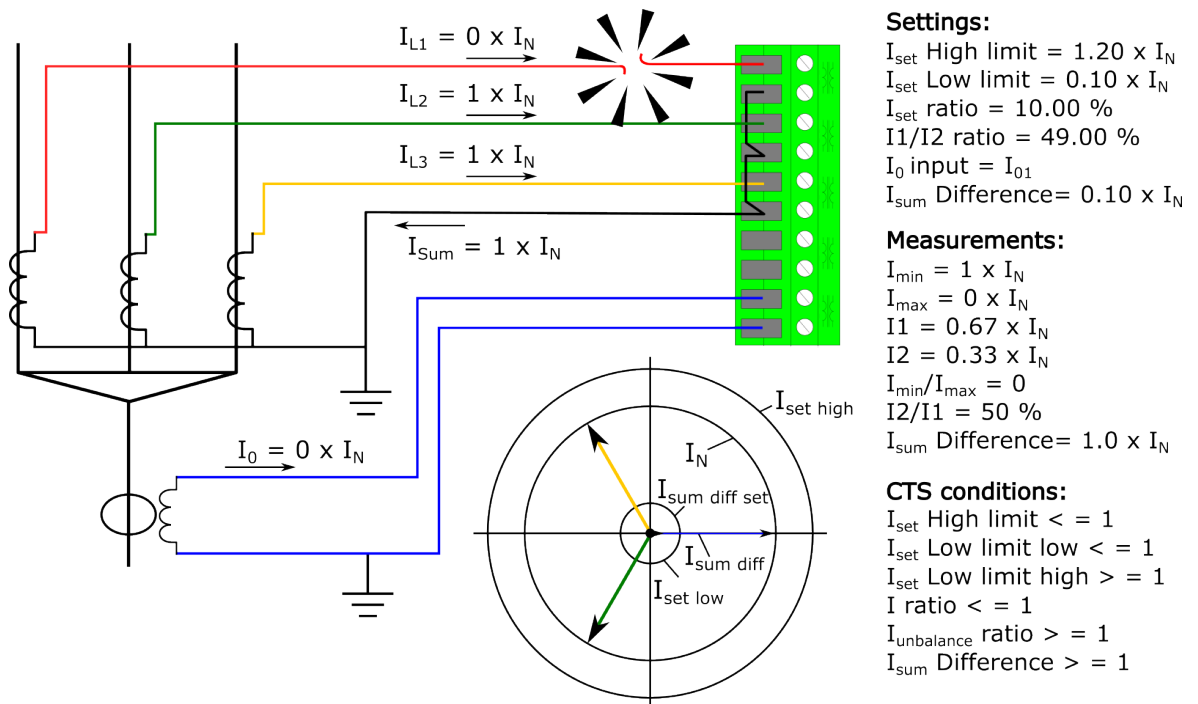
Figure. 5.6.1 - 218. Broken secondary phase current wiring.
