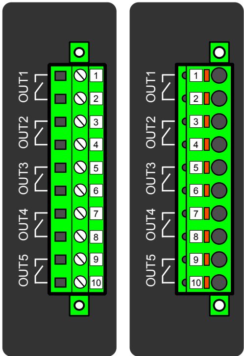
Figure. 8.5.2 - 247. Digital output module (DO5) with five add-on digital outputs. Can be equipped with standard screw terminals or spring cage terminals for connection.
