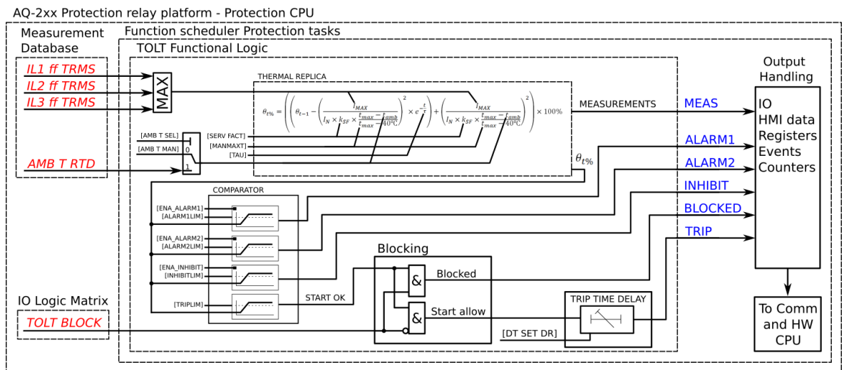
Figure. 5.4.22 - 158. Simplified function block diagram of the TT&gt; function.
