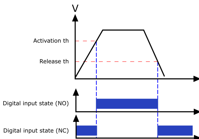
Figure. 8.5.1 - 246. Digital input state when energizing and de-energizing the digital input channels.
