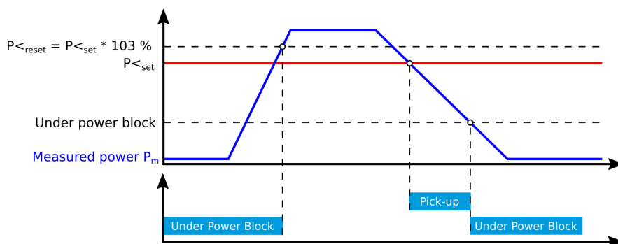
Figure. 5.4.15 - 141. Activation and deactivation characteristics of low power blocking.
