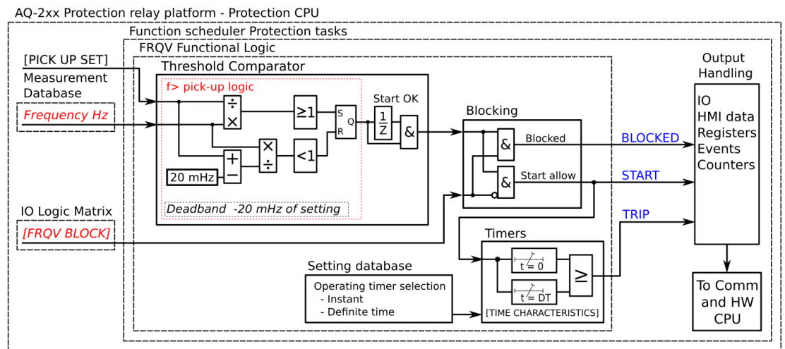
Figure. 5.4.17 - 144. Simplified function block diagram of the f> function.
