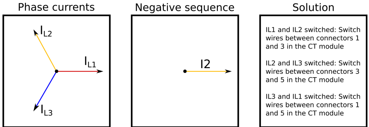
Figure. 5.2.1 - 67. Common network rotation (mixed phases) problems.
