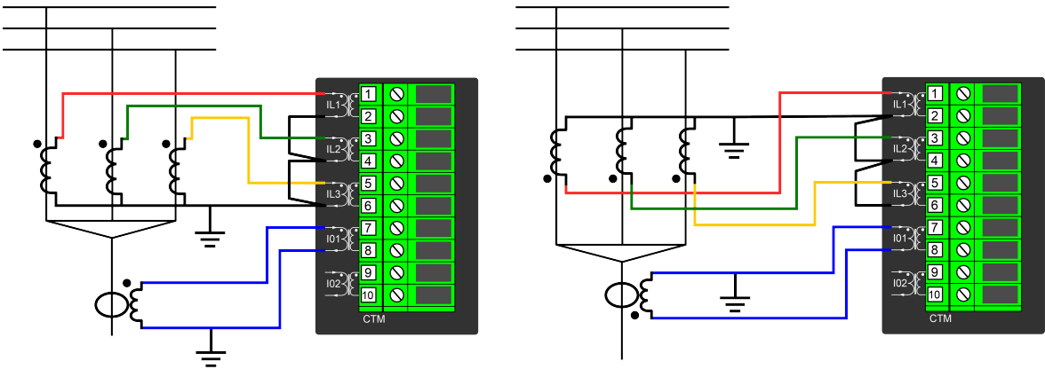
Figure. 5.4.9 - 106. "IO direction" parameter must be set to "Subtract" when current transformers are facing the same direction.
