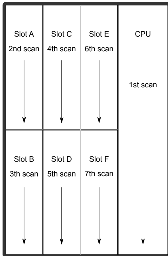
Figure. 8.1 - 184. AQ-X210 hardware scanning and I/O naming principles.
