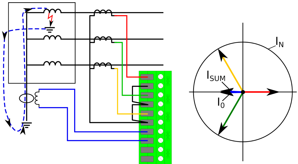
Figure. 5.4.7 - 98. Restricted earth fault inside a Y winding transformer.
