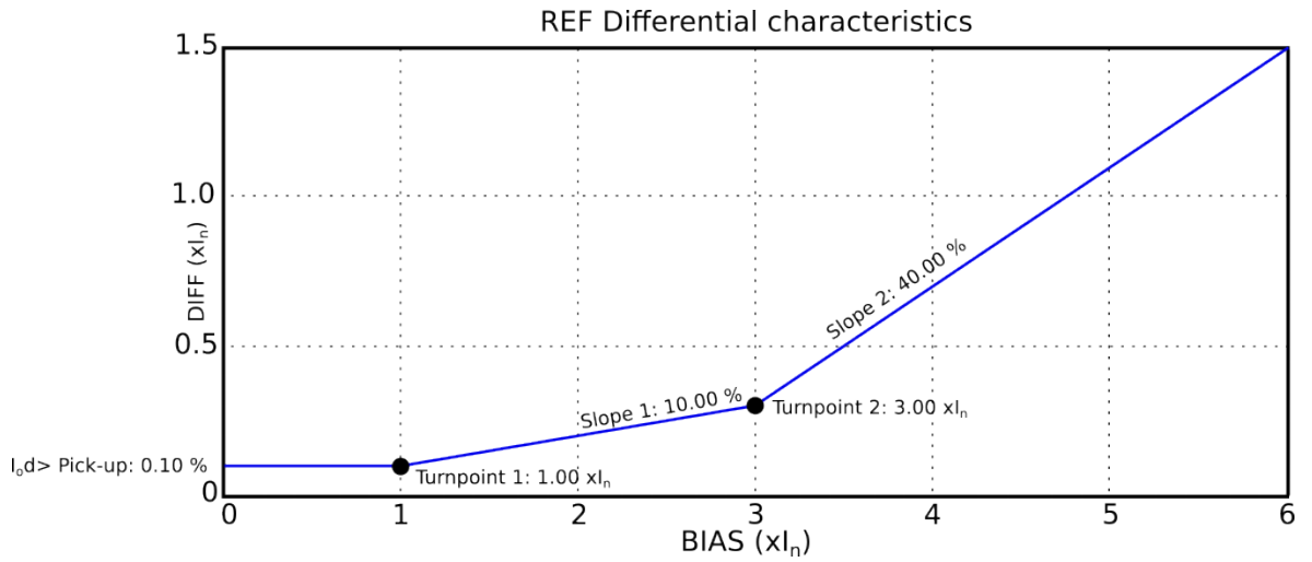
Figure. 5.4.7 - 91. Differential characteristics for the I0d&gt; function with default settings.
