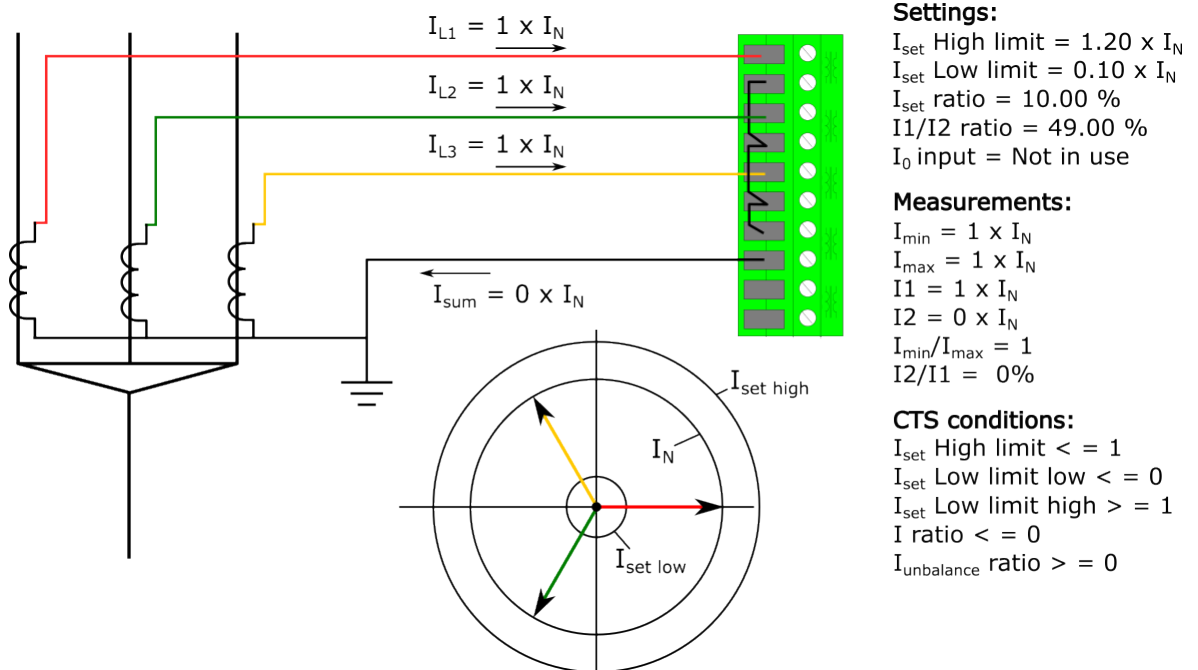
Figure. 5.6.1 - 156. All works properly, no faults.
