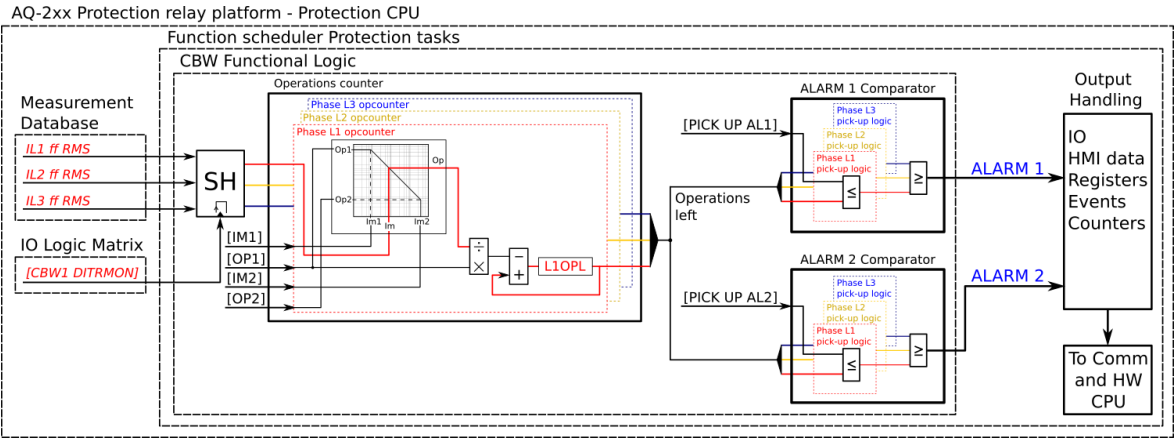
Figure. 5.6.2 - 166. Simplified function block diagram of the circuit breaker wear function.
