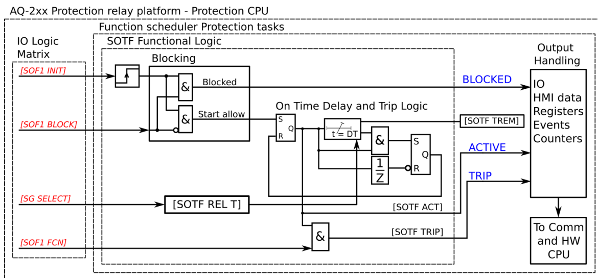
Figure. 5.5.6 - 148. Simplified function block diagram of the switch-on-to-fault function.
