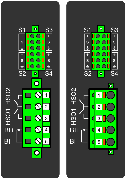
Figure. 8.4.3 - 190. Arc protection module. Can be equipped with standard screw terminals or spring cage terminals for connection.
