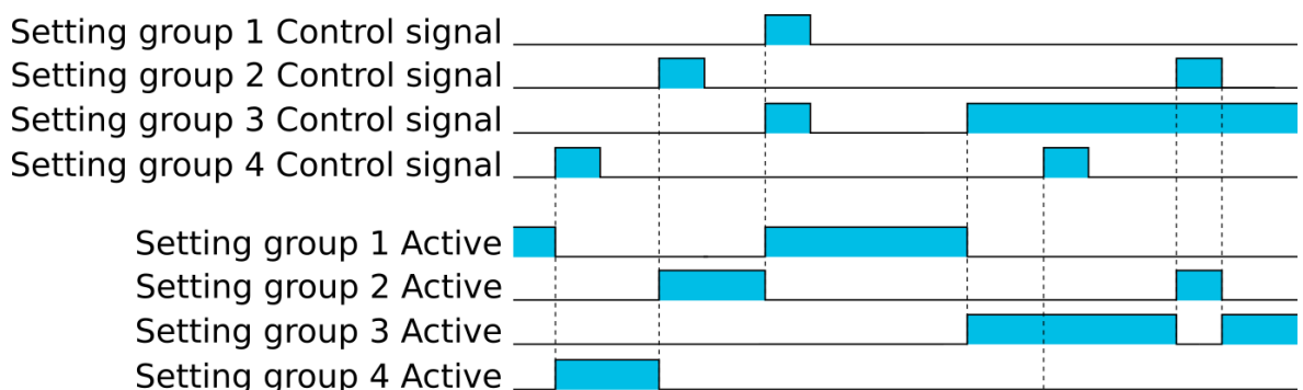
Figure. 5.5.1 - 117. Example sequences of group changing (control with pulse only, or with both pulses and static signals).
