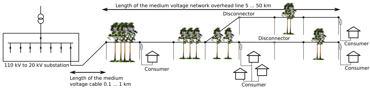
Figure. 5.5.4 - 123. Diagram of a typical radial medium-voltage network in rural areas.
