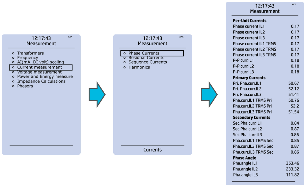
Figure. 4.8 - 46. Current measurement submenu.
