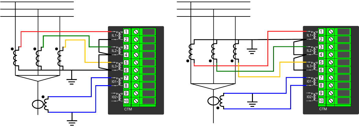
Figure. 5.4.7 - 89. "I0 direction" parameter must be set to "Subtract" when current transformers are facing the same direction.
