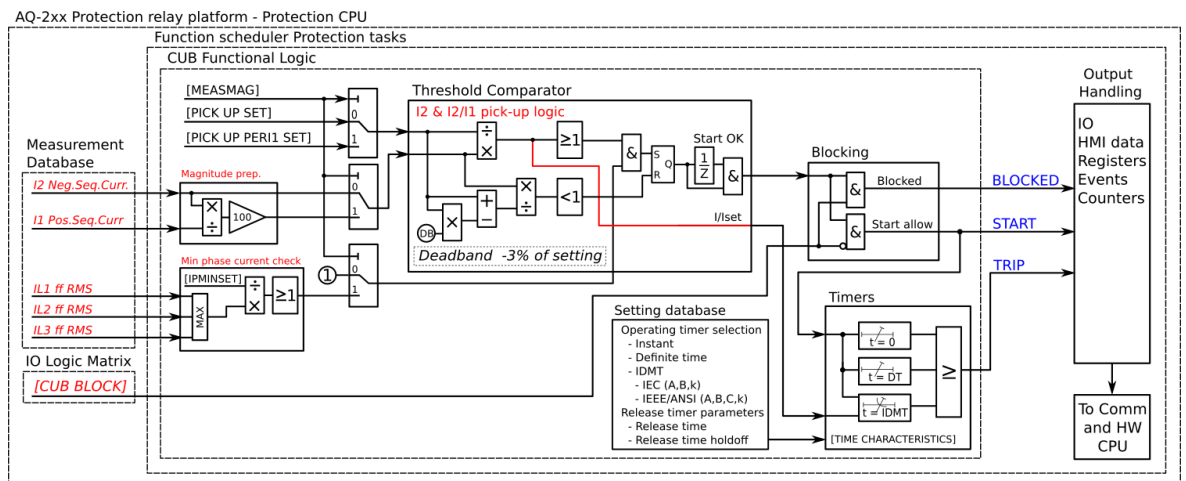
Figure. 5.4.4 - 74. Simplified function block diagram of the I2&gt; function.
