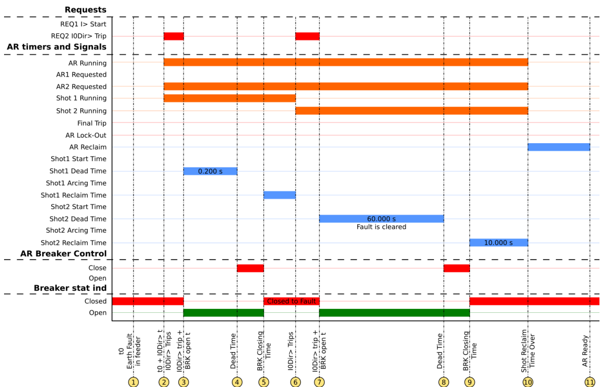
Figure. 5.5.4 - 129. Signal status graph of the semi-permanent earth fault auto-recloser cycle.
