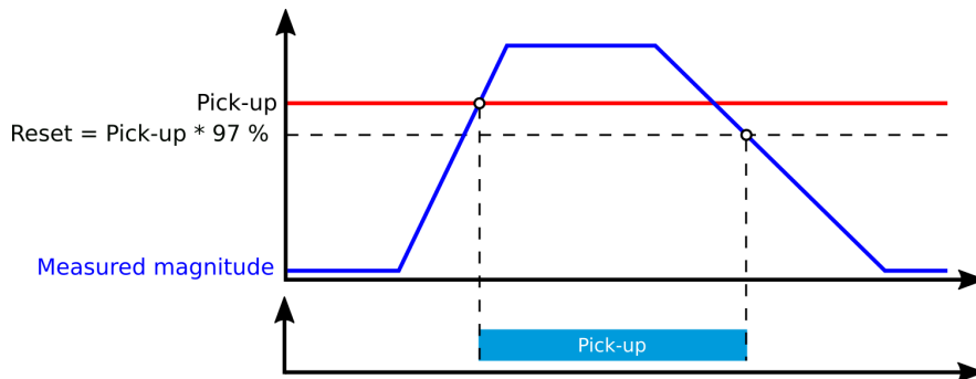
Figure. 5.4.1 - 64. Pick up and reset.
