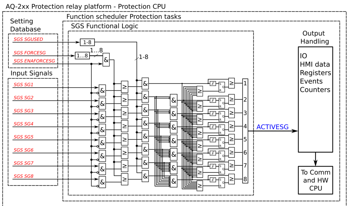
Figure. 5.5.1 - 116. Simplified function block diagram of the setting group selection function.
