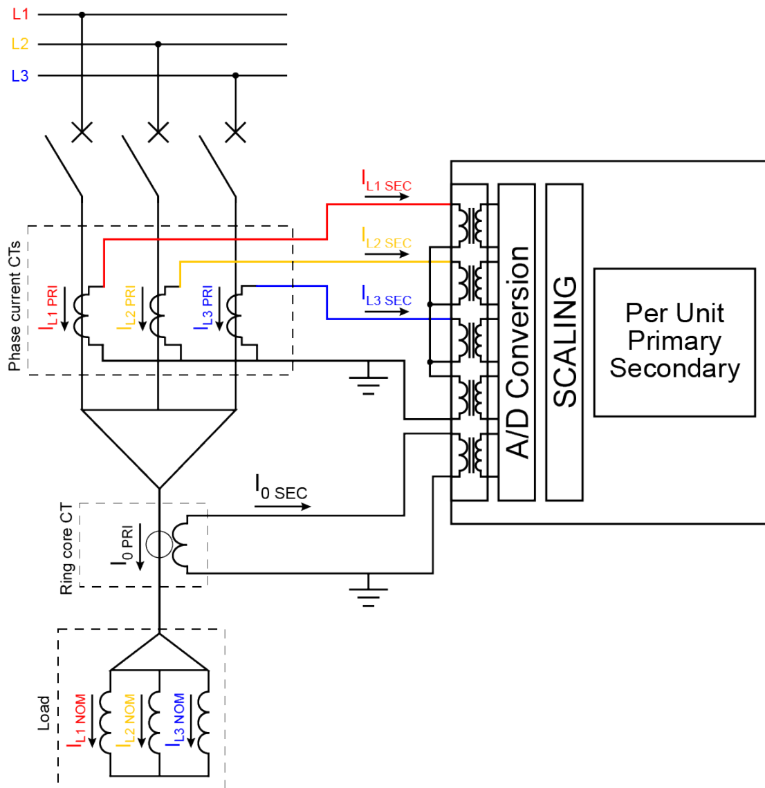
Figure. 5.2.1 - 53. Current measurement terminology.
