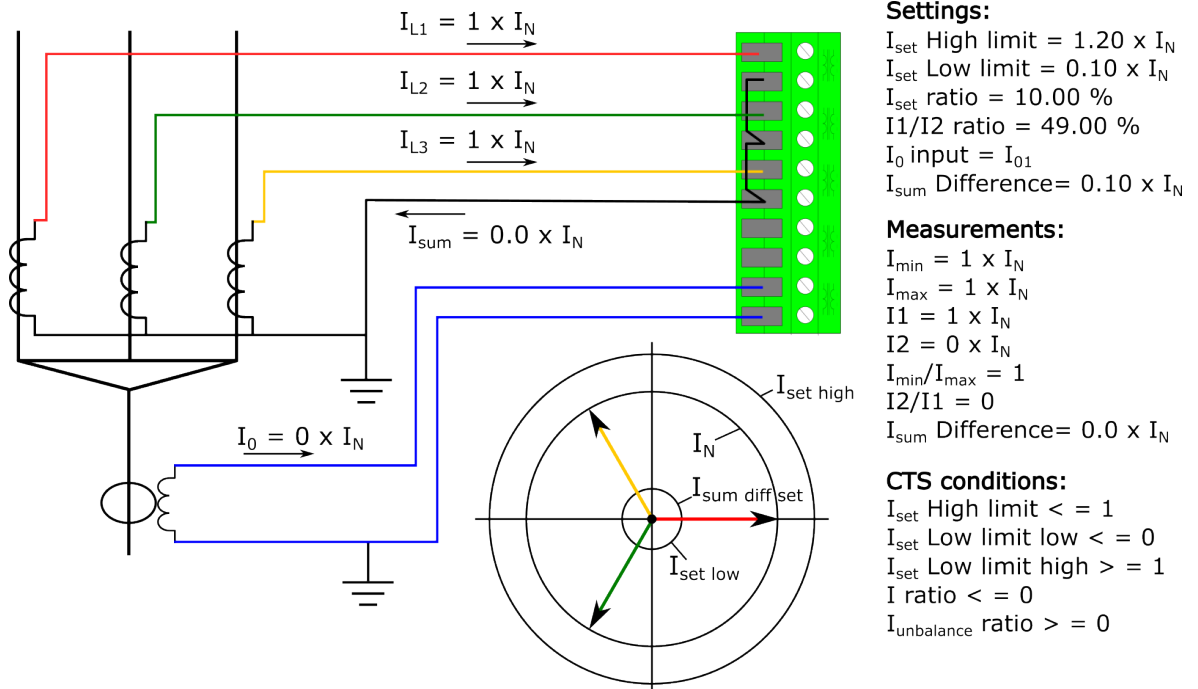
Figure. 5.6.1 - 161. Normal situation, residual current also measured.
