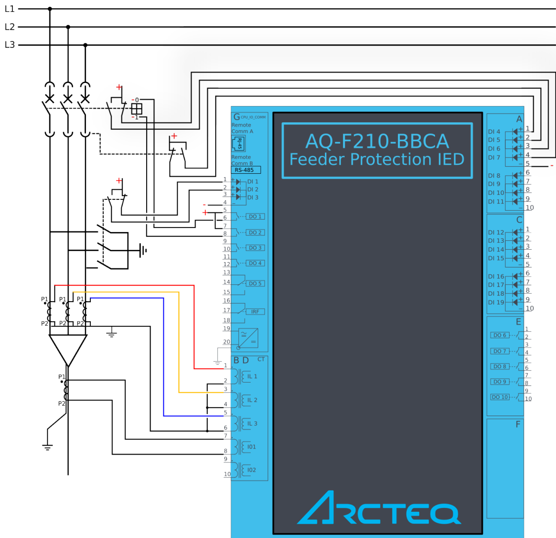
Figure. 7.2.1 - 177. Application example and its connections.
