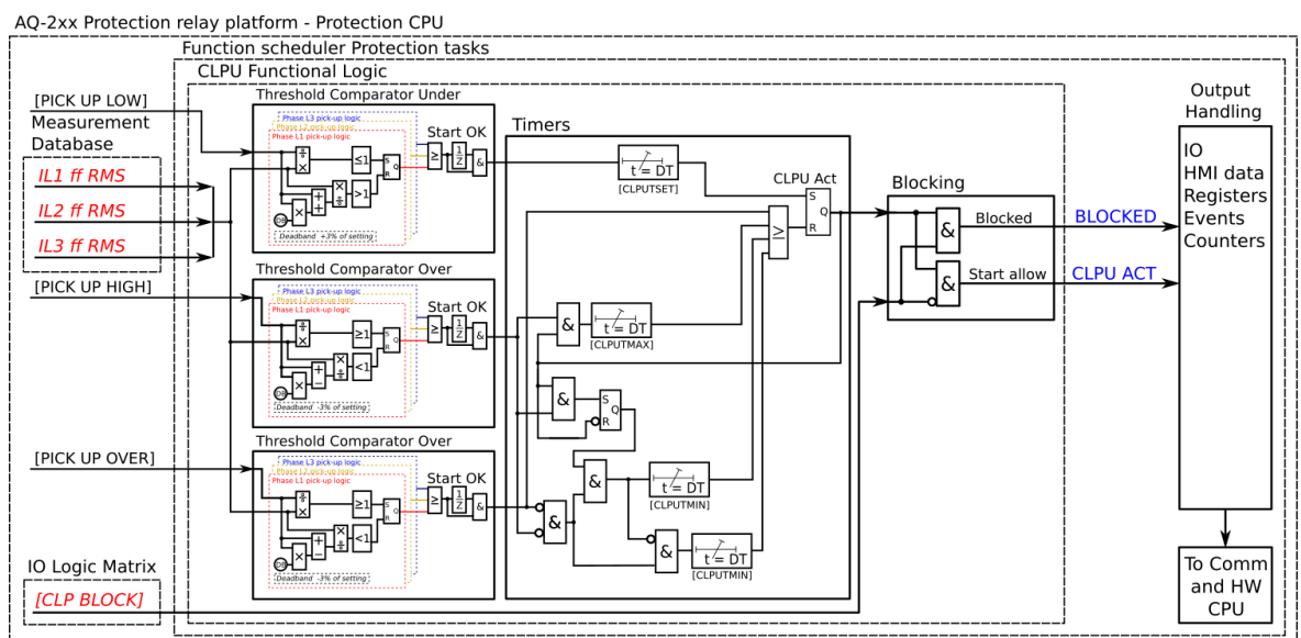
Figure. 5.5.5 - 141. Simplified function block diagram of the cold load pick-up function.
