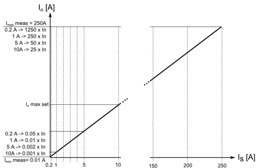
Figure. 5.4.1 - 65. Measurement range in relation to the nominal current.
