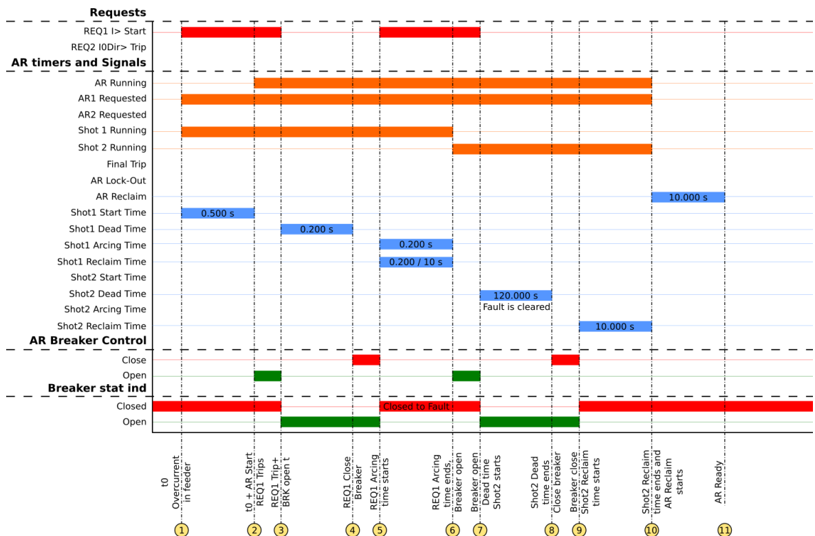
Figure. 5.5.4 - 135. Signal status graph of the semi-permanent overcurrent auto-recloser cycle.
