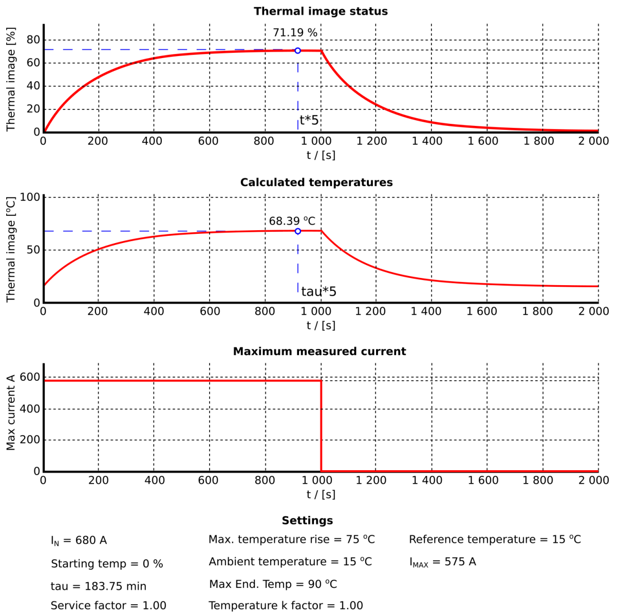
Figure. 5.4.8 - 107. Thermal image response with nominal load (installation according to presumptions).
