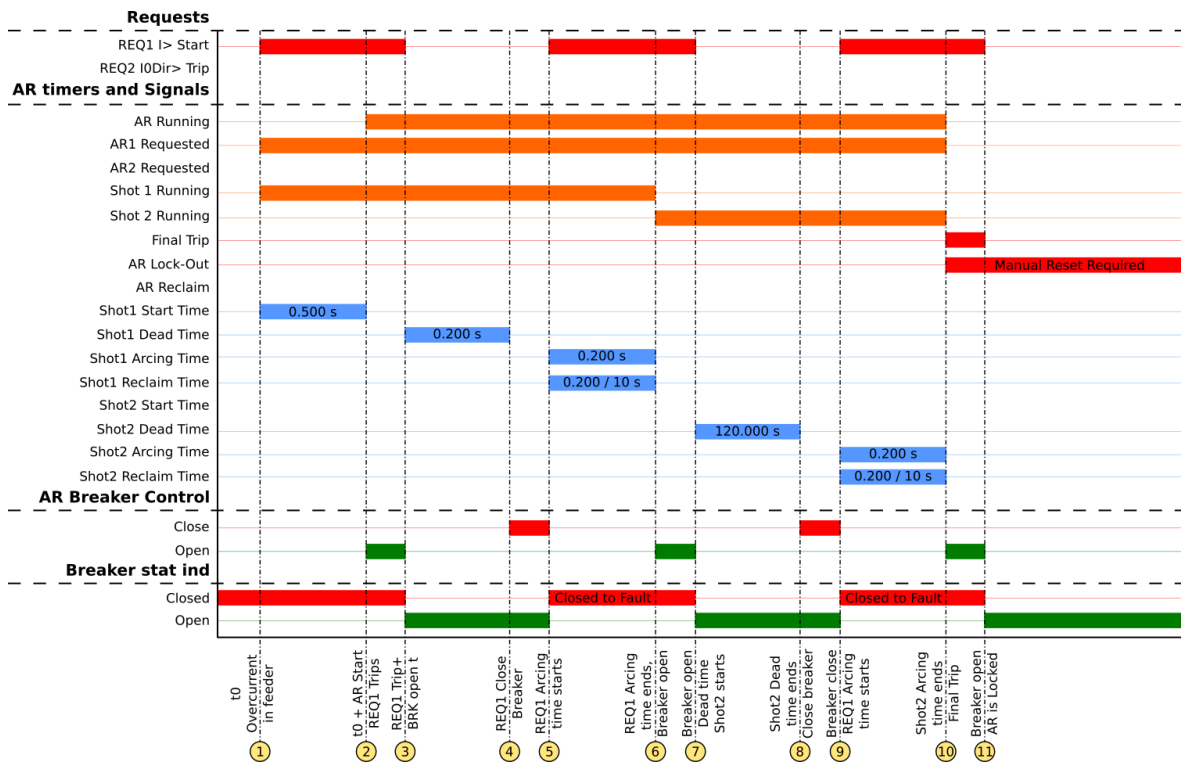
Figure. 5.5.4 - 133. Signal status graph of the permanent overcurrent auto-recloser cycle.
