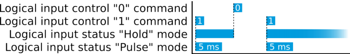
Figure. 5.5.11 - 152. Operation of logical input in "Hold" and "Pulse" modes.
