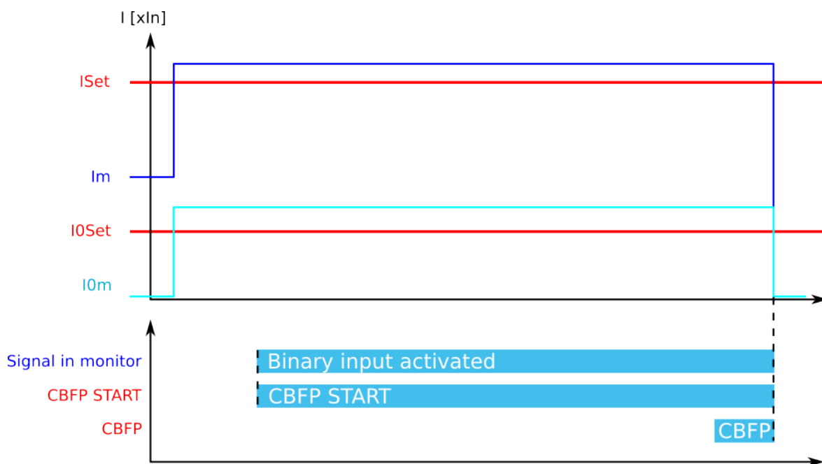
Figure. 5.4.6 - 87. Dedicated CBFP operation from digital input signal.
