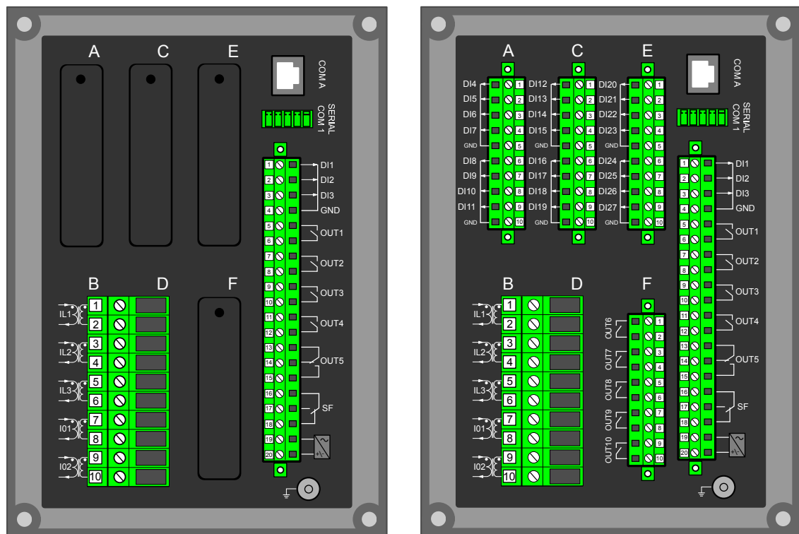
Figure. 8.1 - 183. Modular construction of AQ-X210.
