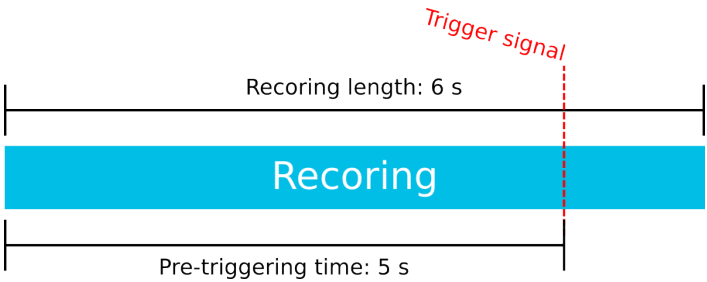
Figure. 5.6.4 - 170. Effects of recording length and pre-triggering time signals. This example is based on the settings shown above.
