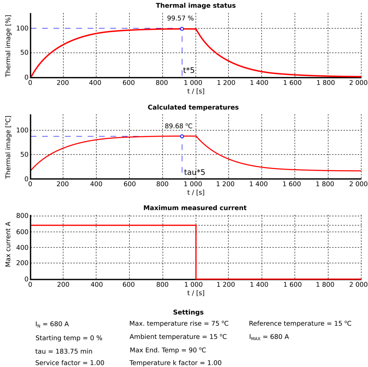
Figure. 5.4.8 - 108. Thermal image response with maximum load (installation according presumptions).
