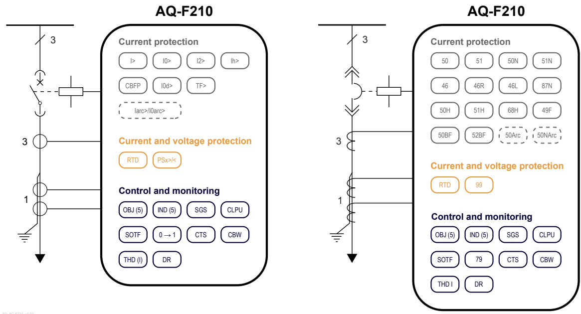
Figure. 7.1.1 - 176. AQ-F210 application example with function block diagram.
