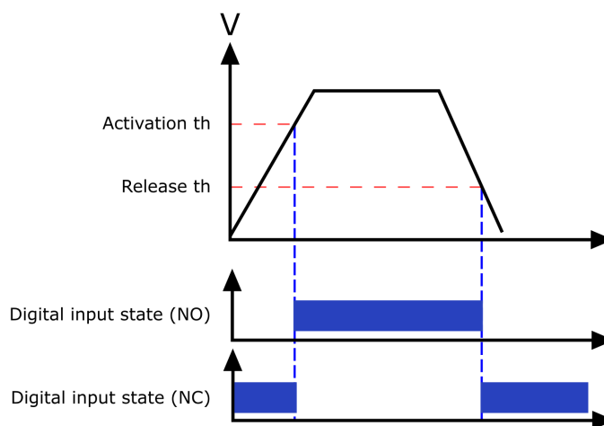
Figure. 8.4.1 - 188. Digital input state when energizing and de-energizing the digital input channels.
