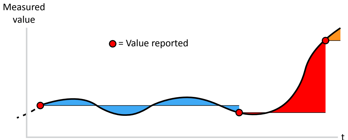
Figure. 6.3.8 - 173. Example graph showing how integration time affects measurement reporting. Small changes take longer to increase the integrated value over the deadband setting (blue area). Big changes meet the deadband criteria faster (red area).
