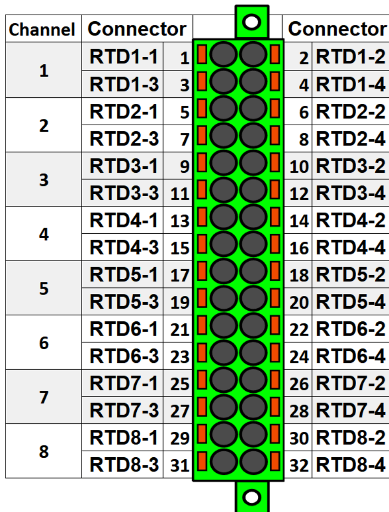
Figure. 8.4.4 - 191. RTD input module connectors.
