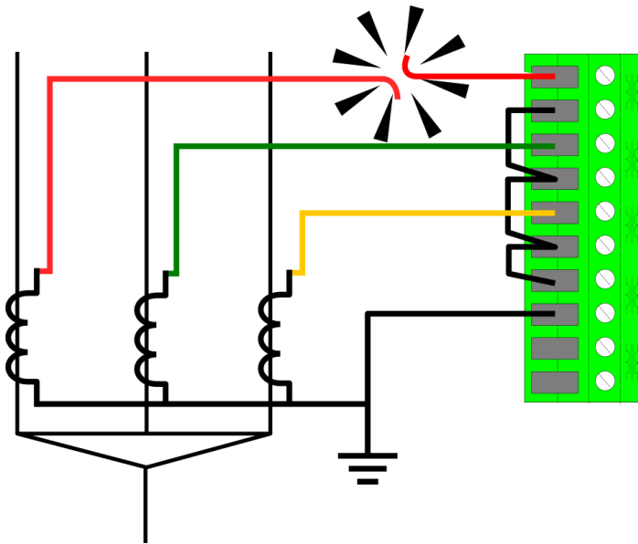
Figure. 5.6.1 - 154. Secondary circuit fault in phase L1 wiring.
