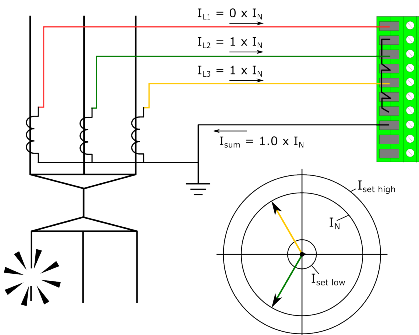
Figure. 5.6.1 - 158. Primary circuit fault in phase L1 wiring.
