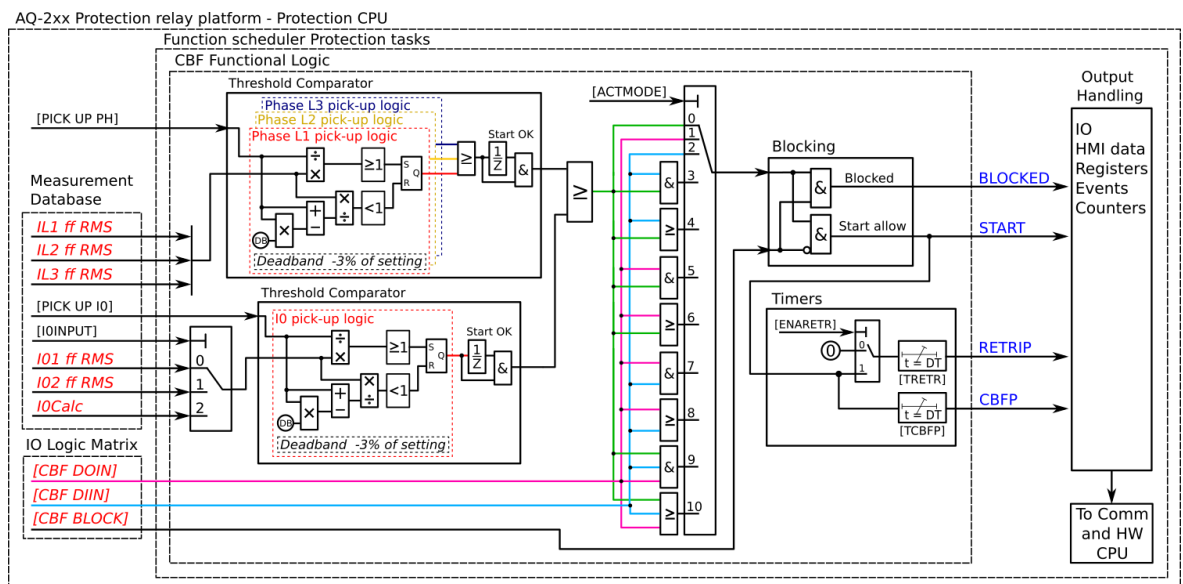
Figure. 5.4.6 - 77. Simplified function block diagram of the CBFP function.
