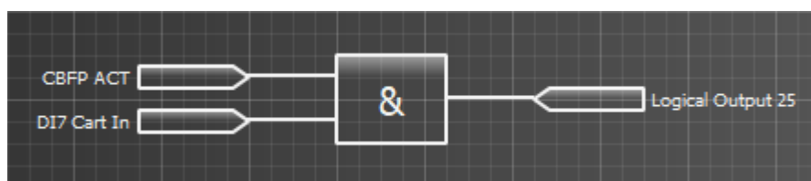
Figure. 5.5.10 - 151. Logic output example. Logical output is connected to an output relay in matrix.
