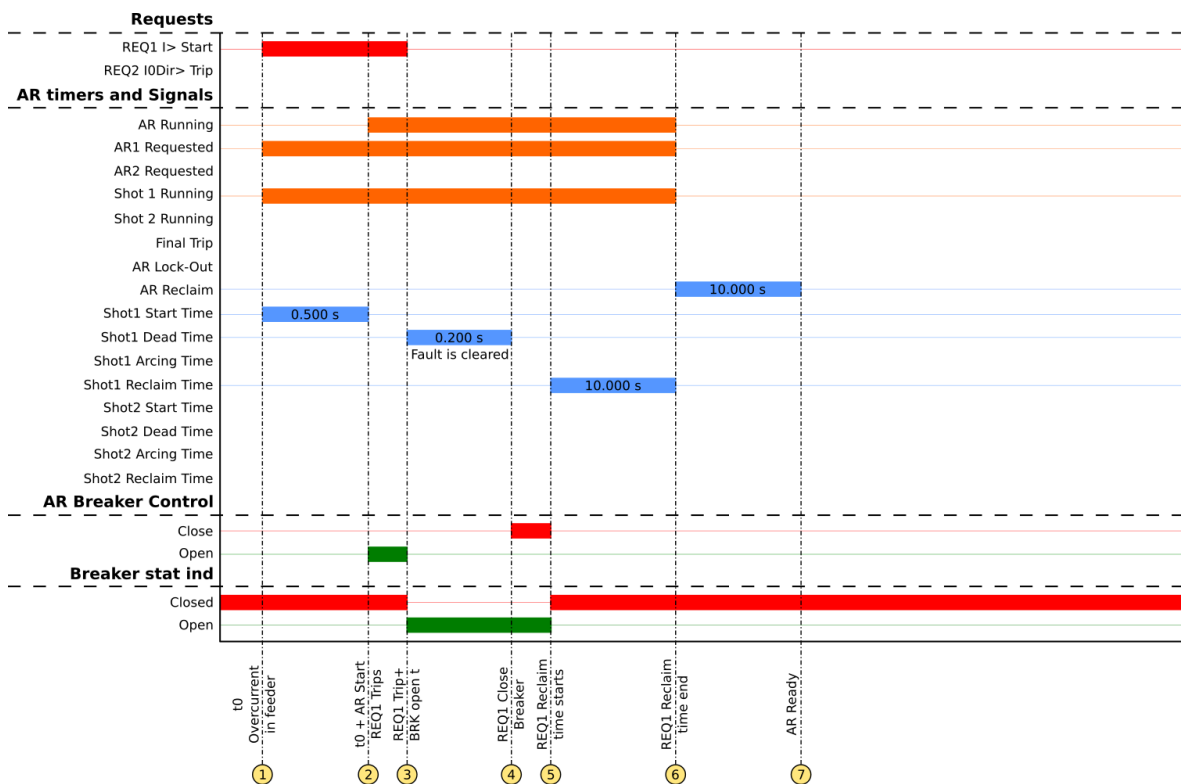
Figure. 5.5.4 - 137. Signal status graph of the transient overcurrent auto-recloser cycle.
