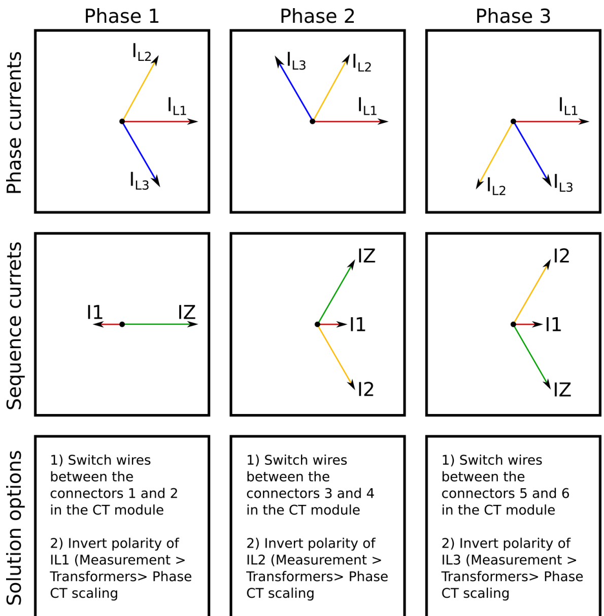
Figure. 5.2.1 - 62. Common phase polarity problems.
