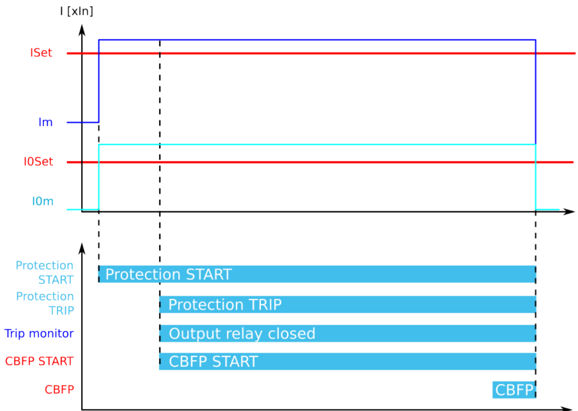
Figure. 5.4.6 - 84. CBFP when "Current and DO" is the selected criterion.
