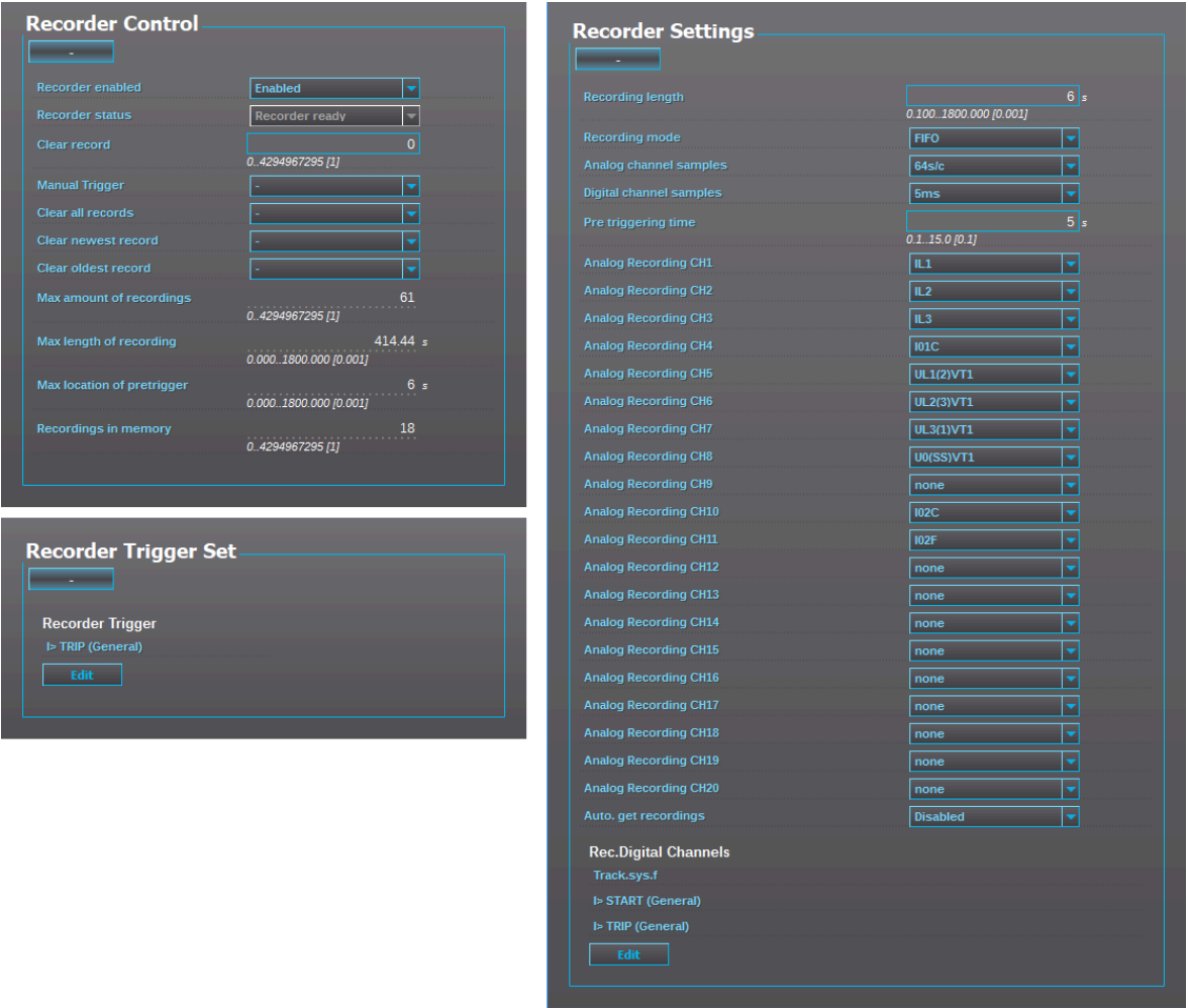
Figure. 5.6.4 - 169. Disturbance recorder settings.
