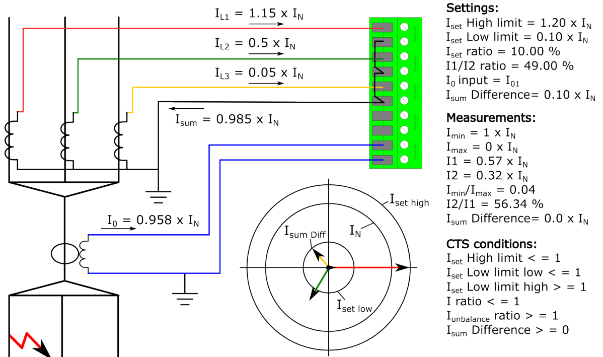
Figure. 5.6.1 - 164. Primary side high-impedance earth fault.
