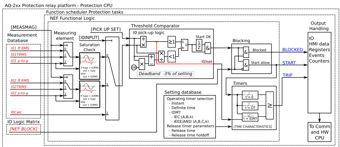
Figure. 5.4.3 - 73. Simplified function block diagram of the I_{0>} function.
