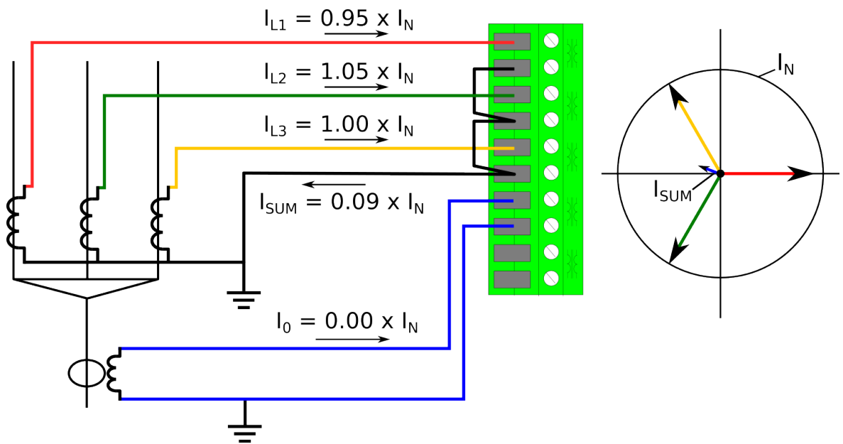
Figure. 5.4.7 - 95. Cable end differential with natural unbalance in the phase current measurement.
