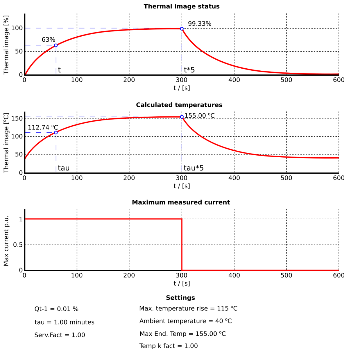
Figure. 5.4.8 - 99. Example of thermal image calculation with nominal conditions.
