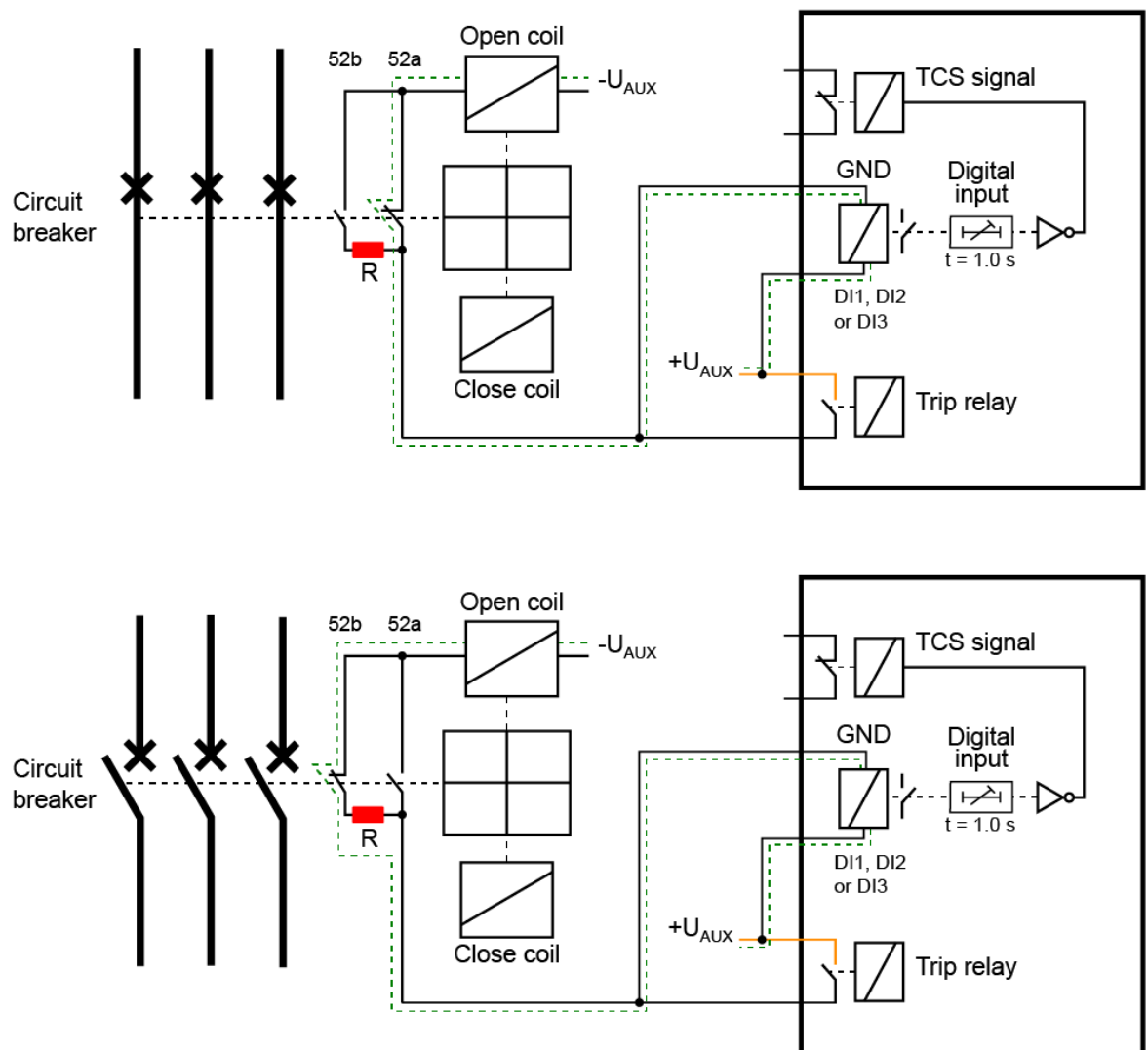
Figure. 7.2.3 - 179. Trip circuit supervision with one DI and one non-latched trip output.
