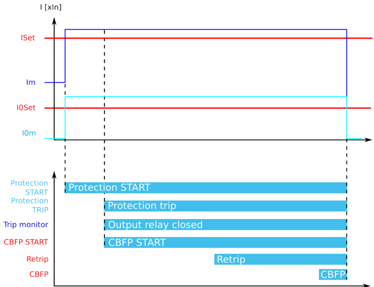
Figure. 5.4.6 - 80. Retrip and CBFP when "Current and DO" is the selected criterion.
