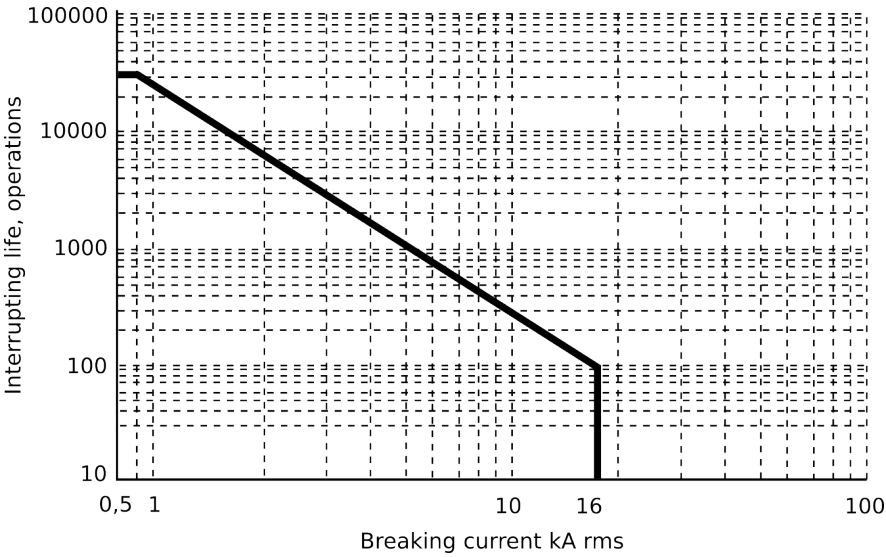
Figure. 5.6.2 - 165. Example of the circuit breaker interrupting life operations.
