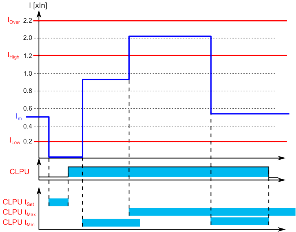
Figure. 5.5.5 - 147. Example of timers and pick-up parameters (an inrush current detected during T_{min} time).
