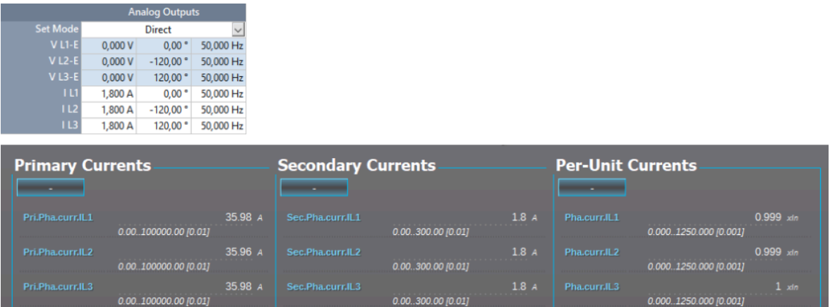
Figure. 5.2.1 - 60. Scalings display (based on the protected object's nominal current).
