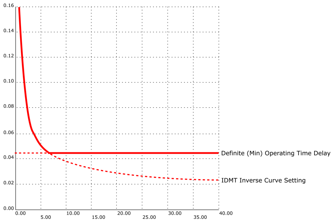
Figure. 5.4.1 - 66. Operating time delay: Definite (minimum) operating time delay and the minimum for tripping.
