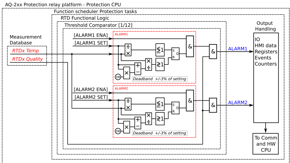
Figure. 5.4.9 - 112. Simplified function block diagram of the resistance temperature detection function.
