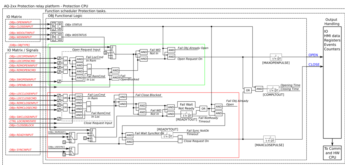
Figure. 5.5.2 - 122. Simplified function block diagram of the object control and monitoring function.
