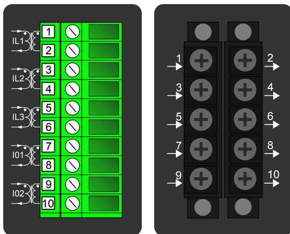
Figure. 8.3 - 186. Module connections with standard and ring lug terminals.
