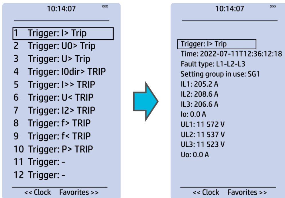
Figure. 5.6.7 - 171. 12 latest recordings can be accessed from HMI if "Fault registers" view has been enabled in "Carousel designer" tool.
