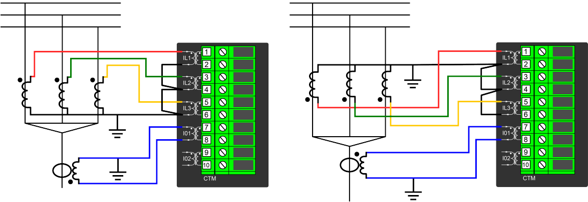
Figure. 5.4.7 - 90. "I0 direction" parameter must be set to "Add" when current transformers are facing each other or away from each other.
