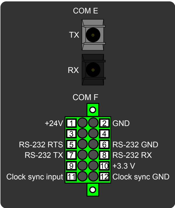
Figure. 8.4.5 - 193. Serial RS-232 module connectors.
