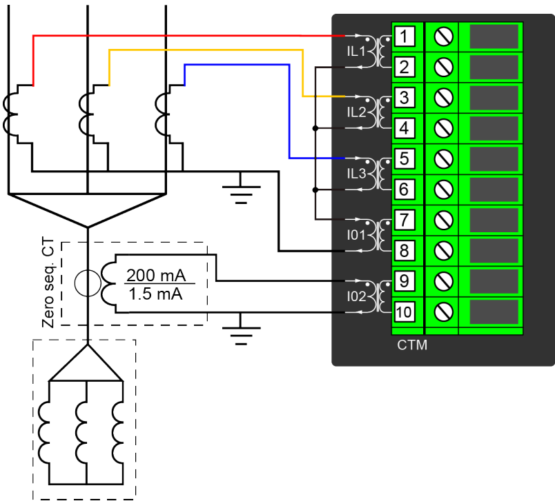
Figure. 5.2.1 - 61. Connections of ZCT scaling.
