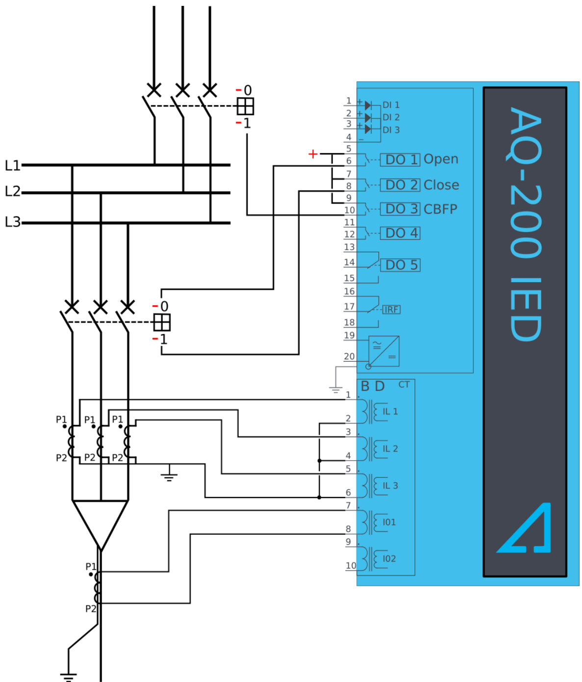
Figure. 5.4.6 - 82. Wiring diagram when Trip and CBFP are configured to the device.
