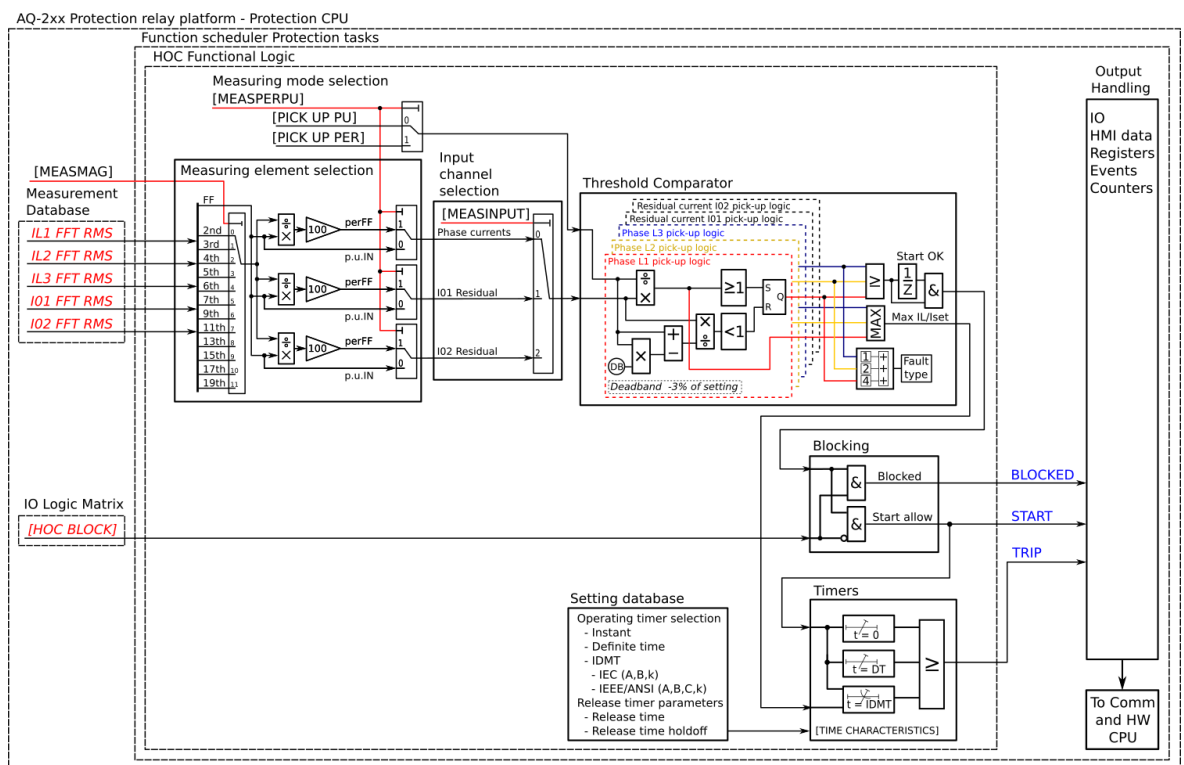
Figure. 5.4.5 - 76. Simplified function block diagram of the Ih&gt; function.
