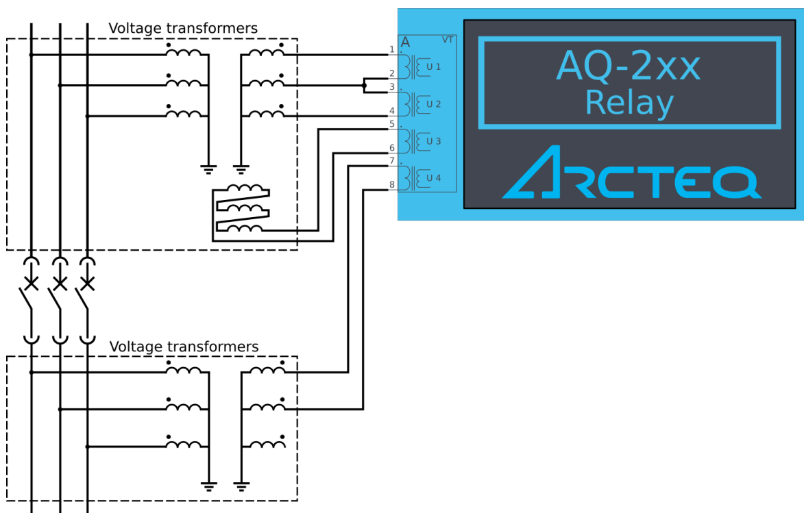
Figure. 5.5.7 - 195. Example connection of the synchrocheck function (2LL+U0+U4 mode, SYN1 in use, UL12 as reference voltage).
