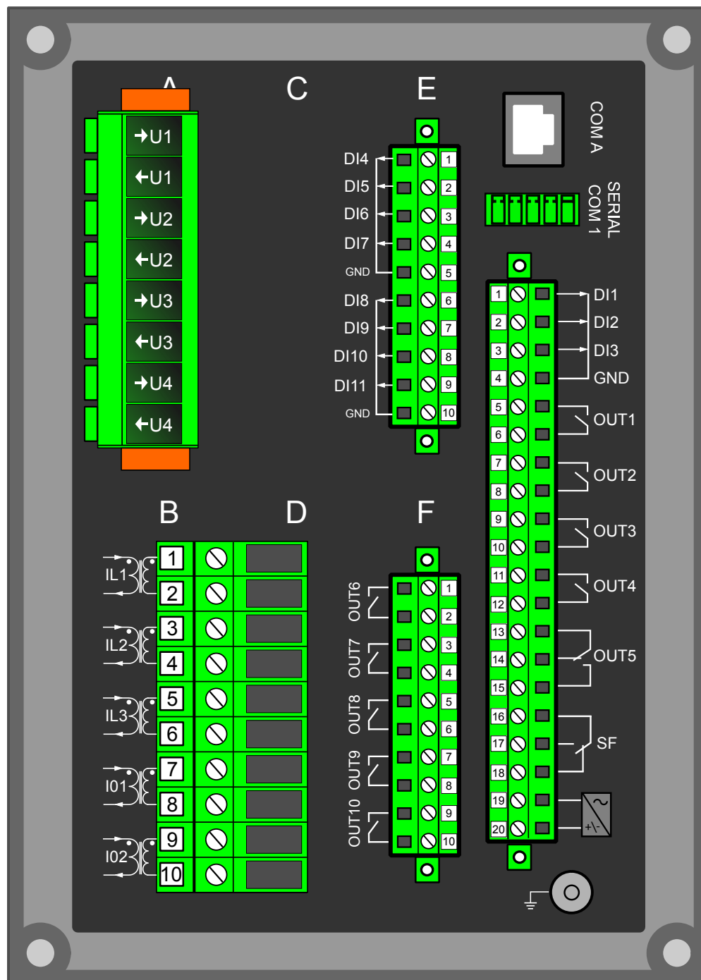
Figure. 8.1 - 239. Modular construction of AQ-F205.
