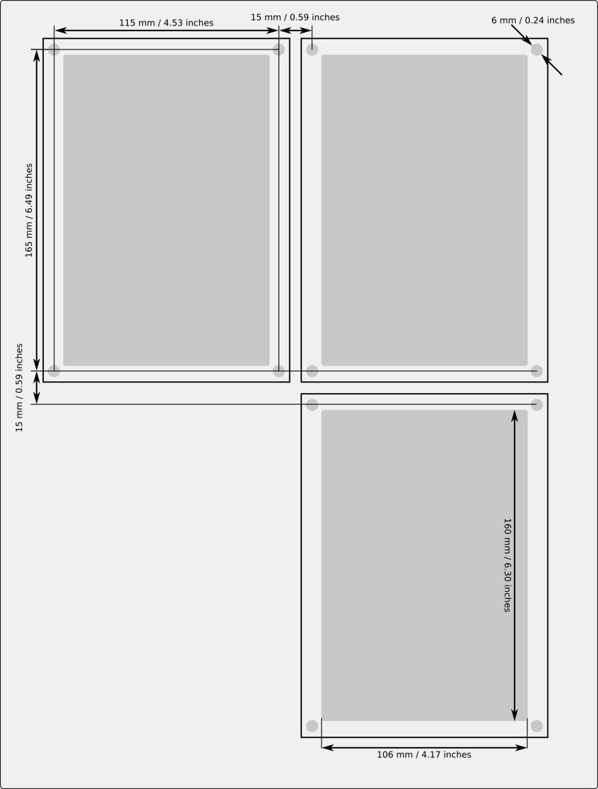
Figure. 8.4 - 244. Panel cutout dimensions and device spacing.
