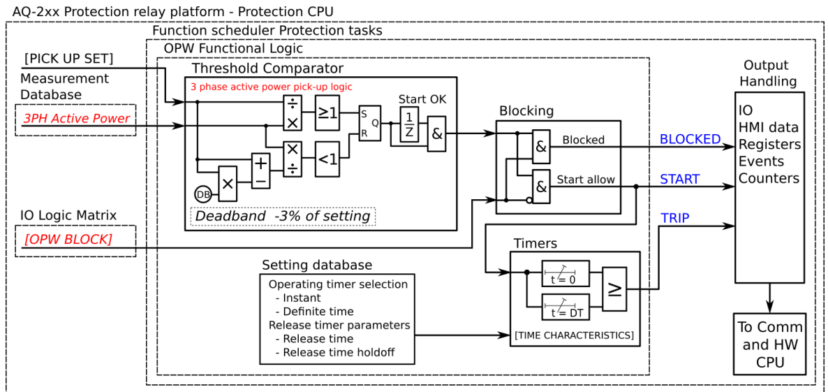
Figure. 5.4.14 - 138. Simplified function block diagram of the P> function.
