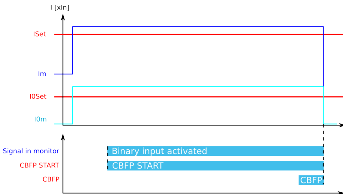
Figure. 5.4.8 - 104. Dedicated CBFP operation from digital input signal.
