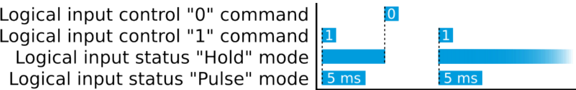
Figure. 5.5.11 - 206. Operation of logical input in "Hold" and "Pulse" modes.
