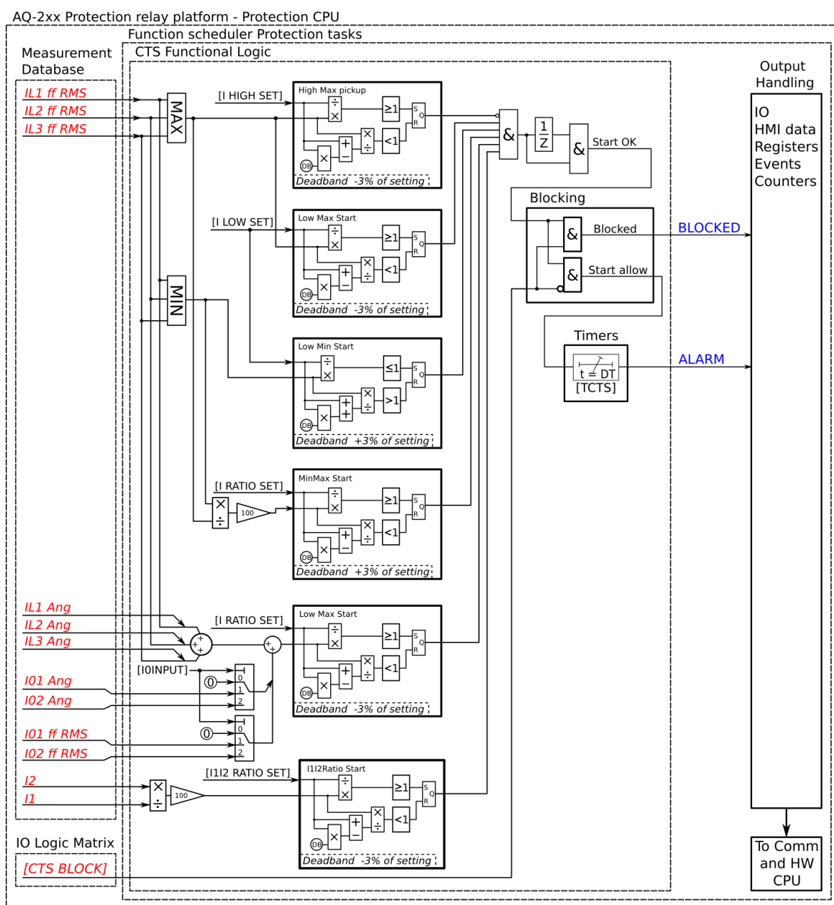
Figure. 5.6.1 - 209. Simplified function block diagram of the CTS function.
