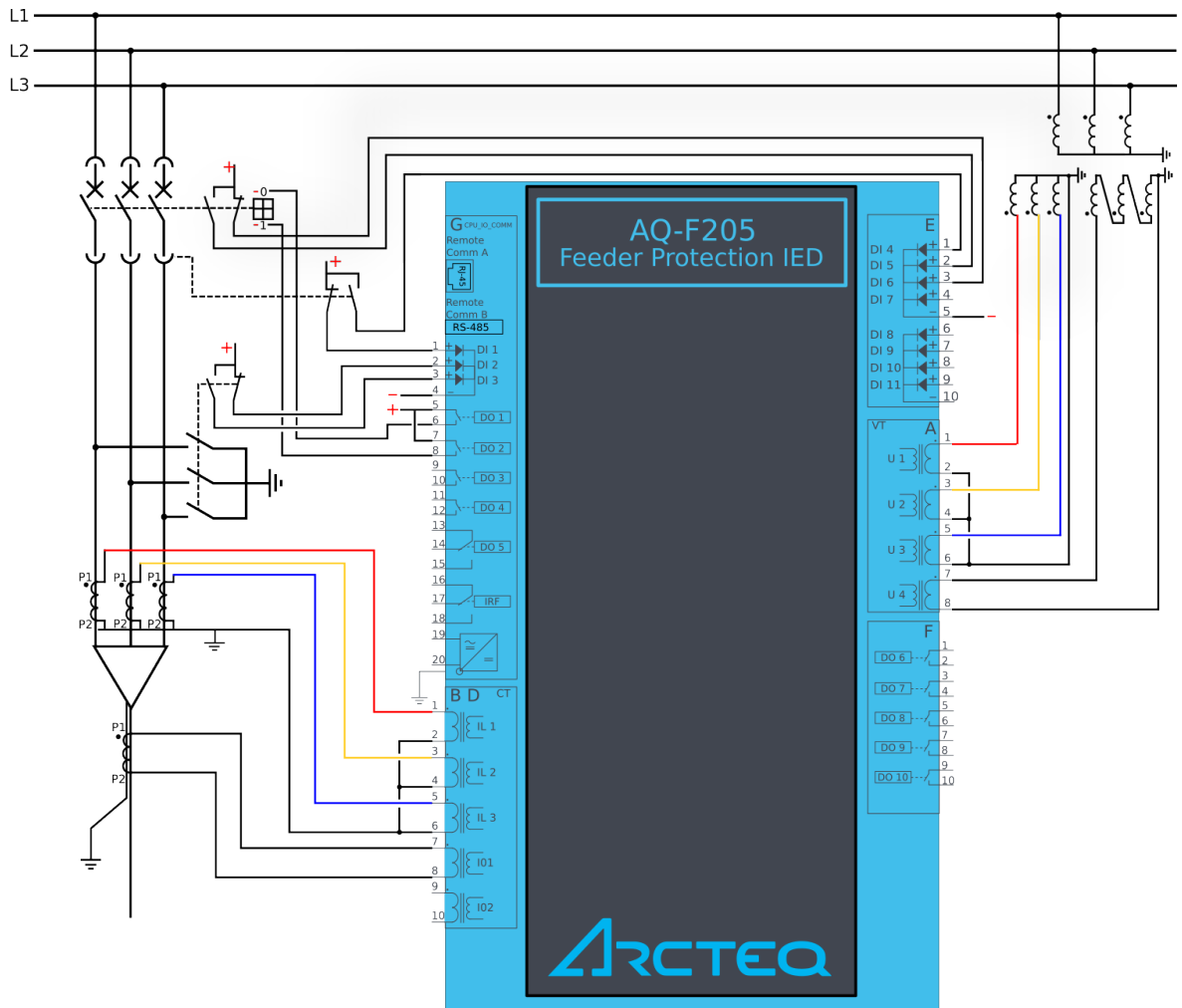
Figure. 7.2.1 - 233. Application example and its connections.
