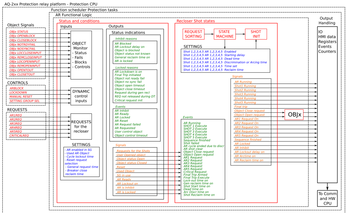
Figure. 5.5.4 - 184. Simplified function block diagram of the auto-recloser function.
