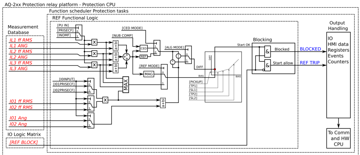
Figure. 5.4.9 - 105. Simplified function block diagram of the I0d&gt; function.
