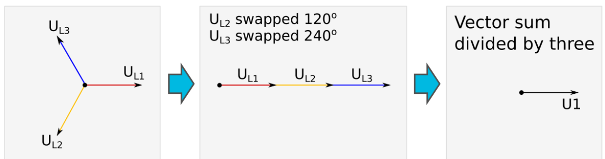
Figure. 5.4.13 - 129. Normal situation.
