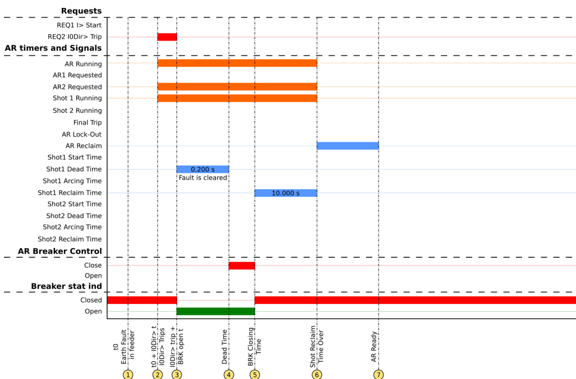
Figure. 5.5.4 - 176. Signal status graph of the transient earth fault auto-recloser cycle.
