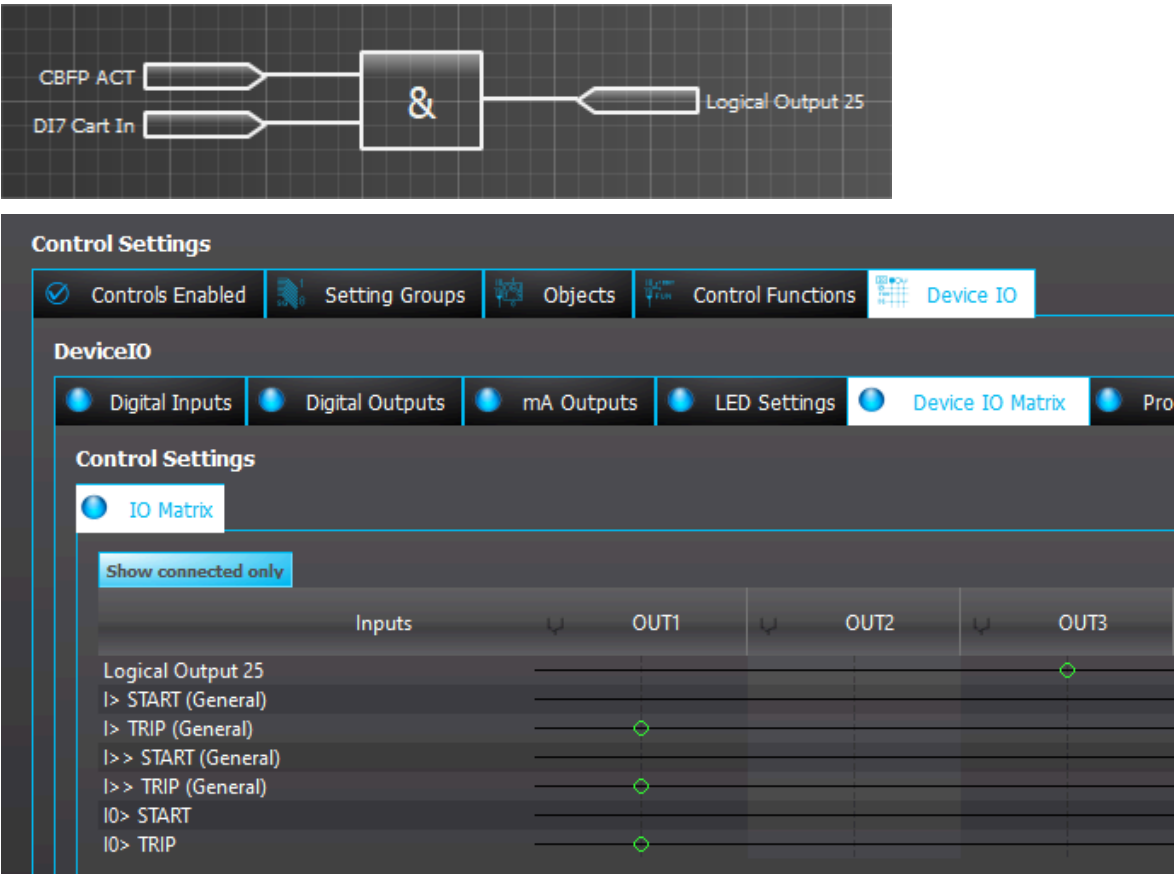
Figure. 5.5.10 - 205. Logic output example. Logical output is connected to an output relay in matrix.
