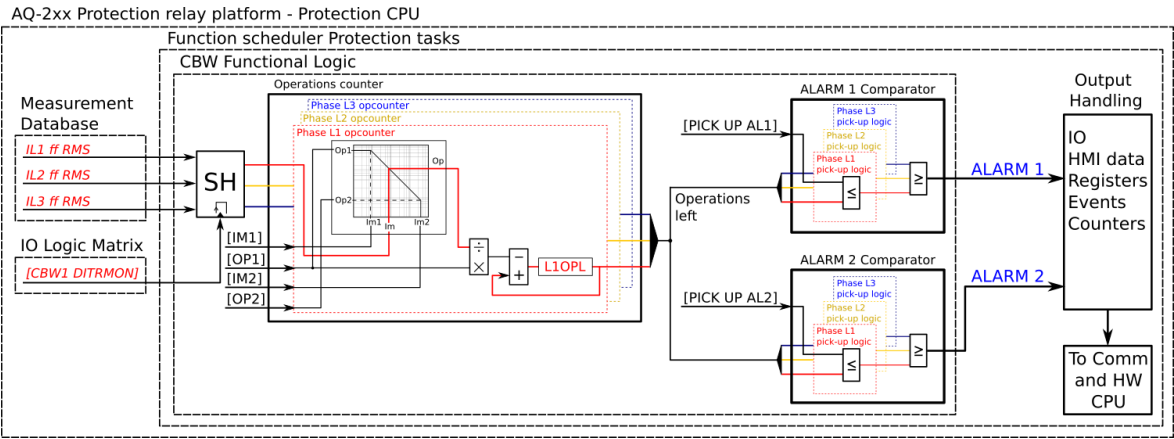
Figure. 5.6.3 - 222. Simplified function block diagram of the circuit breaker wear function.
