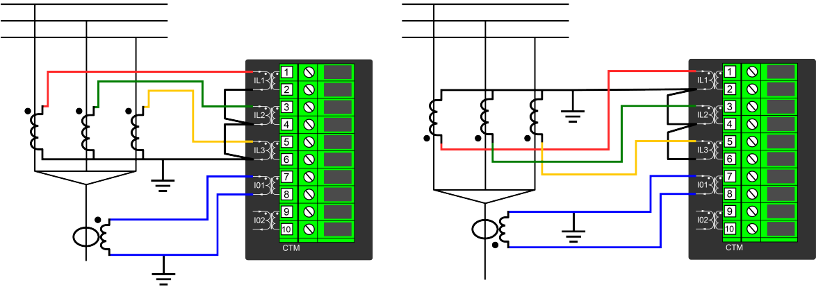
Figure. 5.4.9 - 106. "I0 direction" parameter must be set to "Subtract" when current transformers are facing the same direction.
