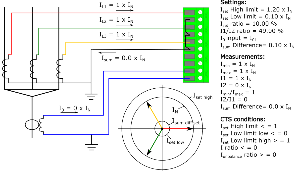
Figure. 5.6.1 - 215. Normal situation, residual current also measured.
