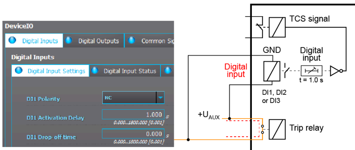
Figure. 7.2.3 - 236. Settings for a digital input used for trip circuit supervision.
