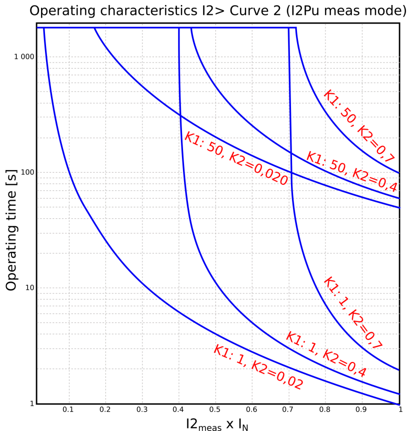
Figure. 5.4.6 - 92. Operation characteristics curve for I2> Curve2.
