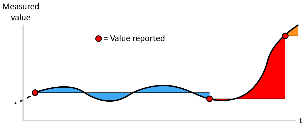
Figure. 6.3.7 - 229. Example graph showing how integration time affects measurement reporting. Small changes take longer to increase the integrated value over the deadband setting (blue area). Big changes meet the deadband criteria faster (red area).
