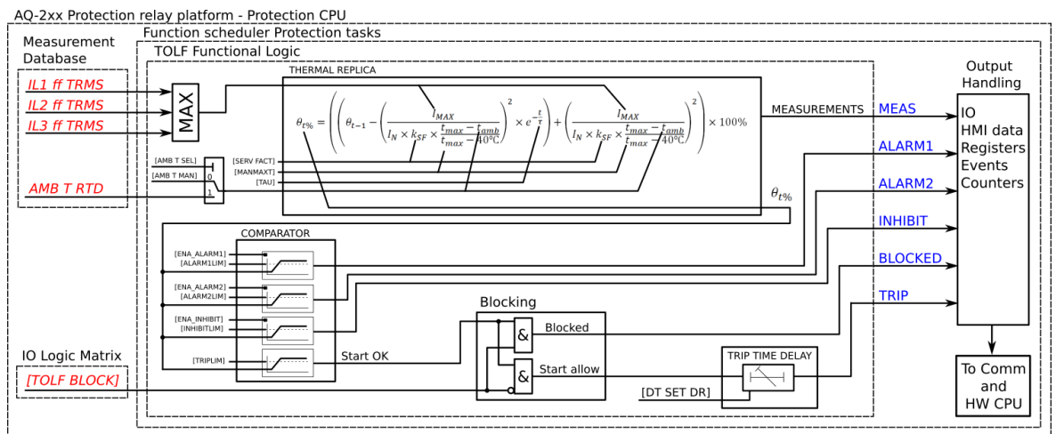
Figure. 5.4.19 - 160. Simplified function block diagram of the TF&gt; function.
