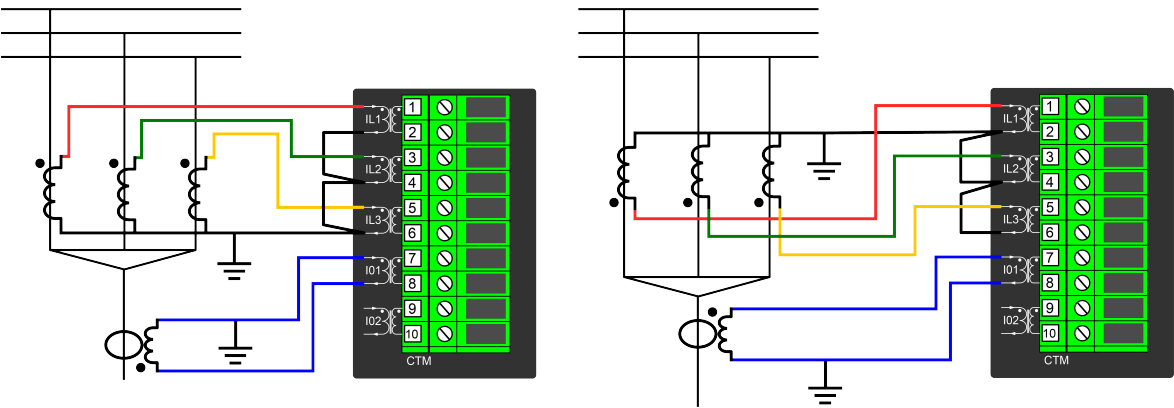
Figure. 5.4.9 - 107. "I0 direction" parameter must be set to "Add" when current transformers are facing each other or away from each other.
