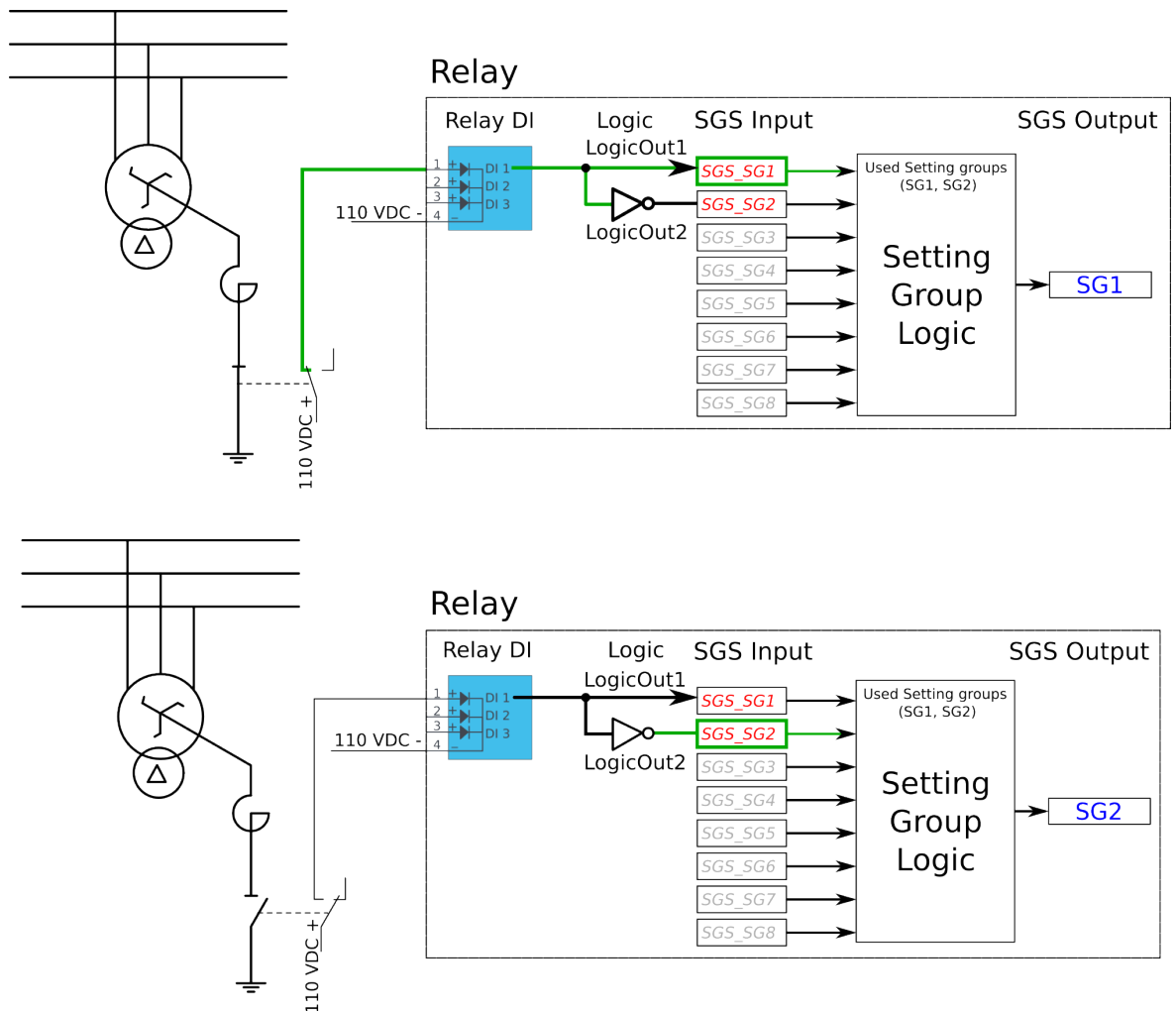
Figure. 5.5.1 - 163. Setting group control – one-wire connection from Petersen coil status.
