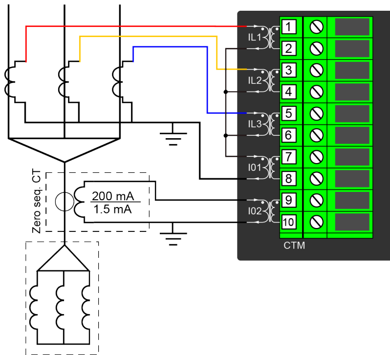
Figure. 5.2.1 - 65. Connections of ZCT scaling.
