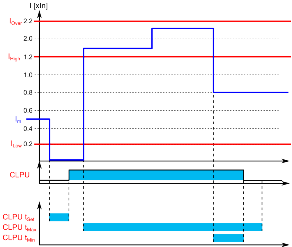
Figure. 5.5.5 - 187. Example of timers and pick-up parameters (normal CLPU situation).
