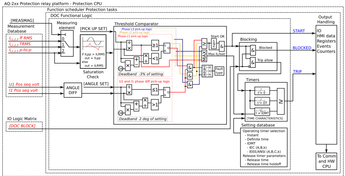
Figure. 5.4.4 - 81. Simplified function block diagram of the Idir> function.
