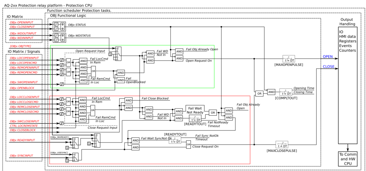
Figure. 5.5.2 - 167. Simplified function block diagram of the object control and monitoring function.
