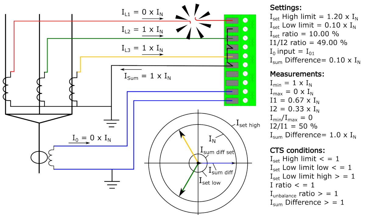
Figure. 5.6.1 - 216. Broken secondary phase current wiring.
