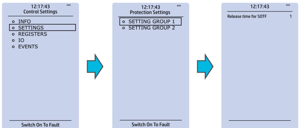
Figure. 4.6 - 27. Settings section.
