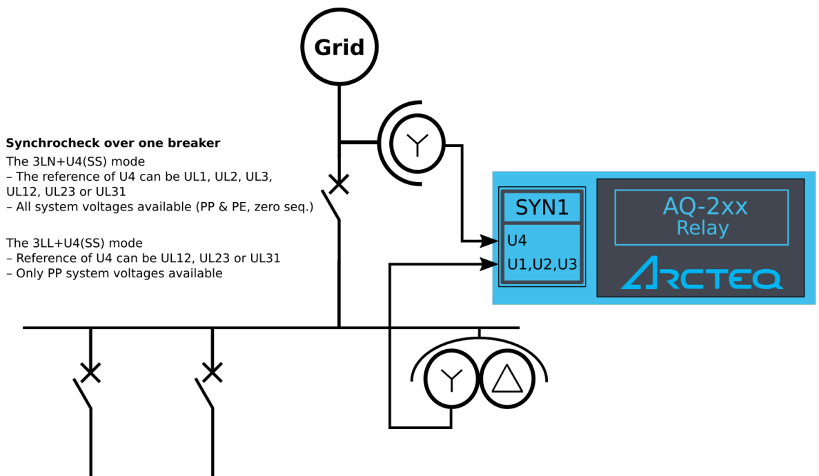
Figure. 5.5.7 - 197. Example application (synchrocheck over one breaker, with 3LL and 3LN VT connections).
