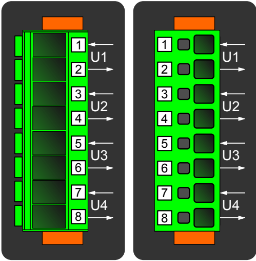
Figure. 8.3 - 241. Voltage measurement module can be equipped with standard screw terminals or spring cage terminals for connection.
