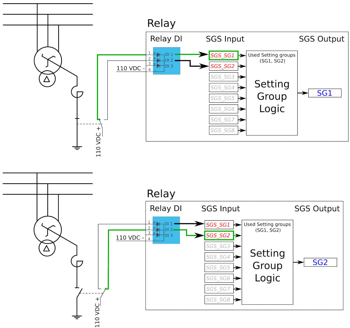
Figure. 5.5.1 - 164. Setting group control – two-wire connection from Petersen coil status.
