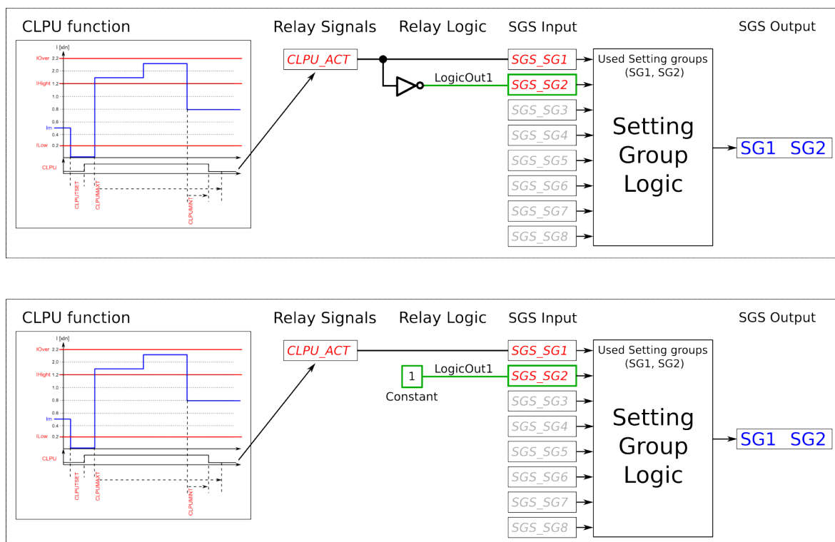
Figure. 5.5.1 - 166. Entirely application-controlled setting group change with the cold load pick-up function.
