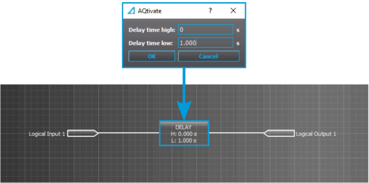
Figure. 5.5.11 - 207. Extending a logical input pulse.
