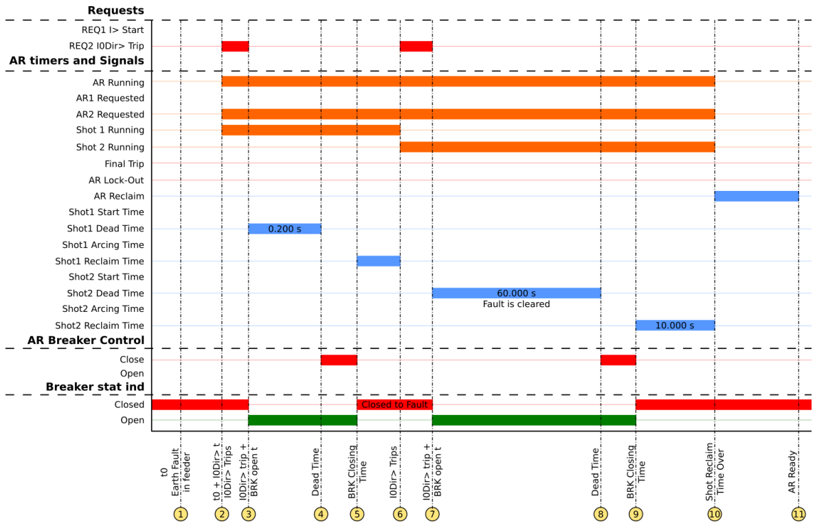
Figure. 5.5.4 - 174. Signal status graph of the semi-permanent earth fault auto-recloser cycle.
