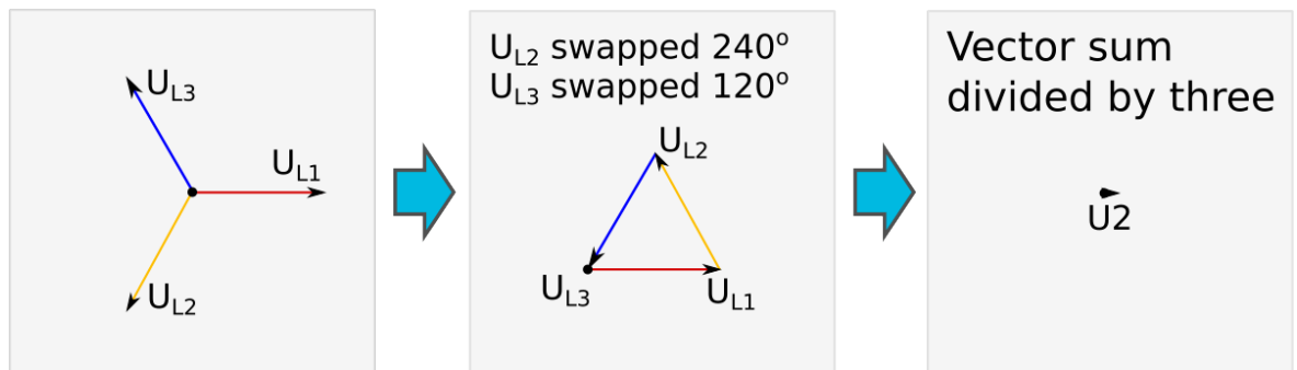
Figure. 5.4.13 - 132. Normal situation.
