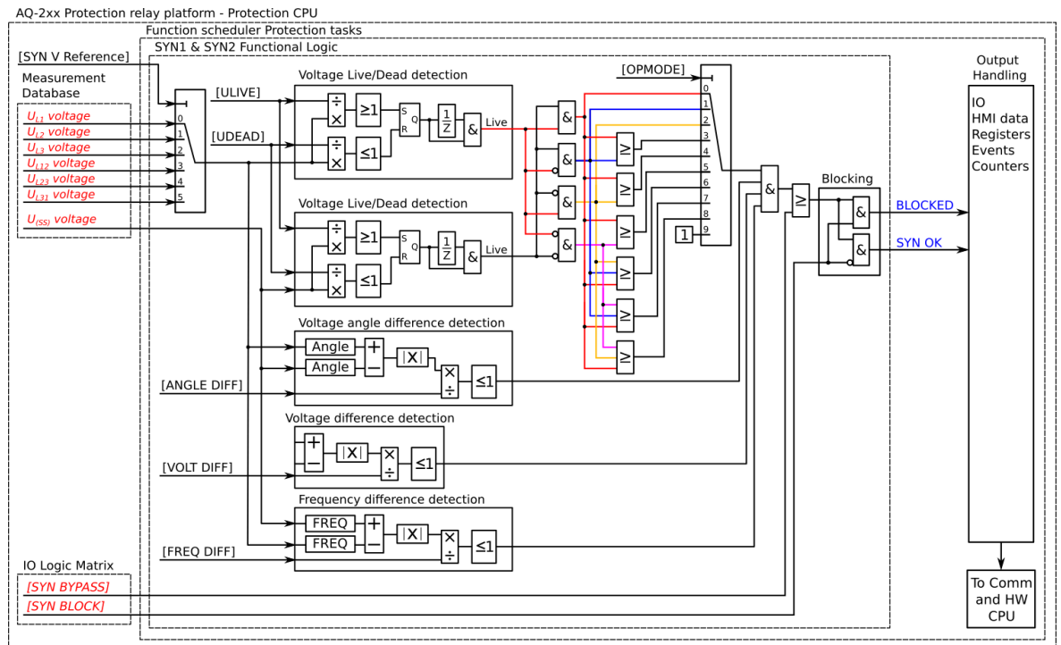
Figure. 5.5.7 - 202. Simplified function block diagram of the SYN1 and SYN2 function.
