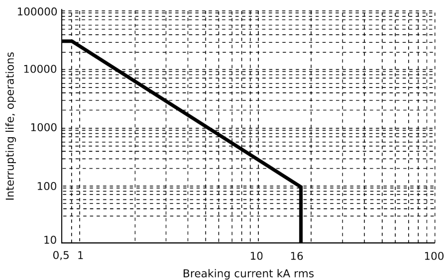
Figure. 5.6.3 - 221. Example of the circuit breaker interrupting life operations.
