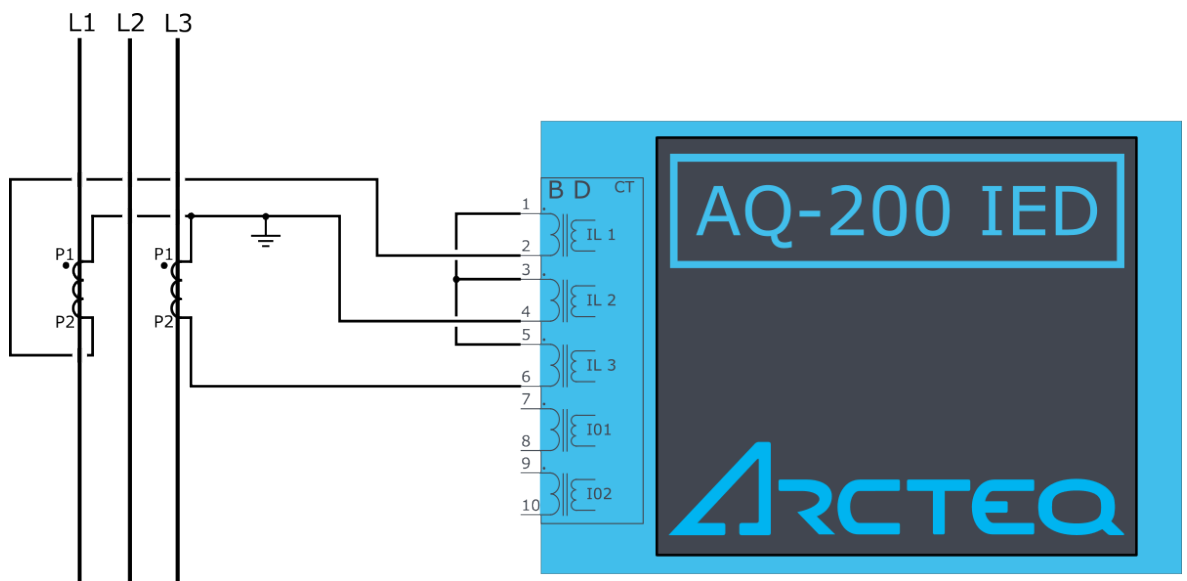
Figure. 7.2.2 - 234. ARON connection.
