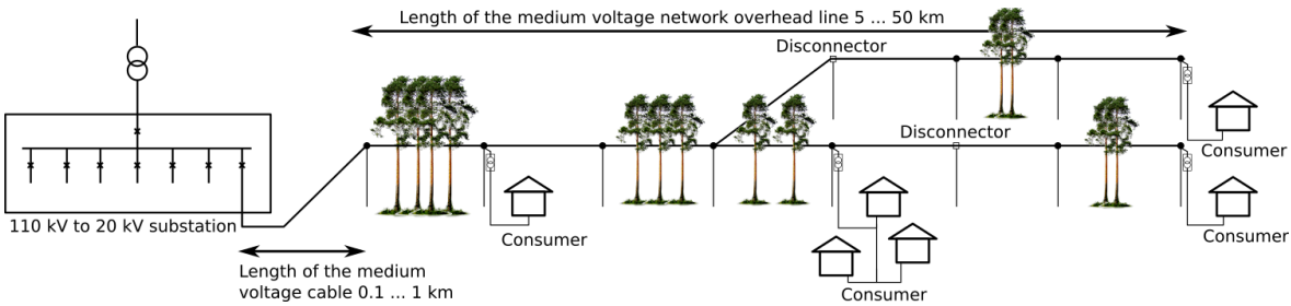
Figure. 5.5.4 - 168. Diagram of a typical radial medium-voltage network in rural areas.
