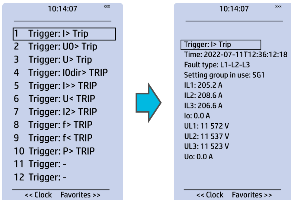
Figure. 5.6.9 - 227. 12 latest recordings can be accessed from HMI if "Fault registers" view has been enabled in "Carousel designer" tool.
