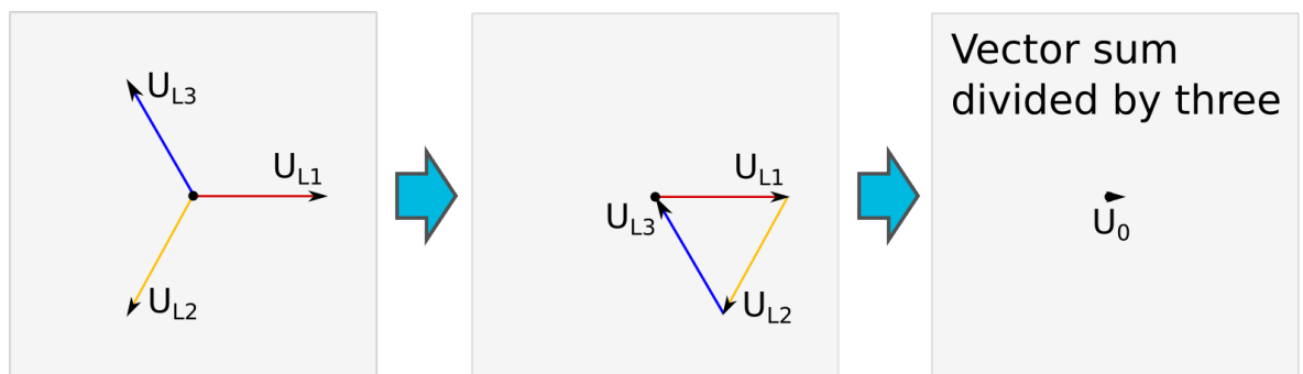
Figure. 5.4.12 - 125. Normal situation.
