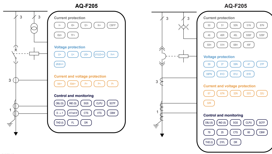
Figure. 7.1.1 - 232. AQ-F205 application example with function block diagram.
