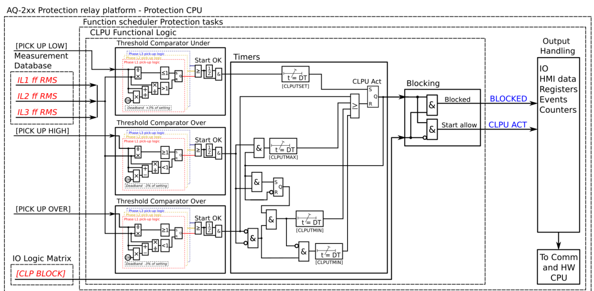
Figure. 5.5.5 - 186. Simplified function block diagram of the cold load pick-up function.
