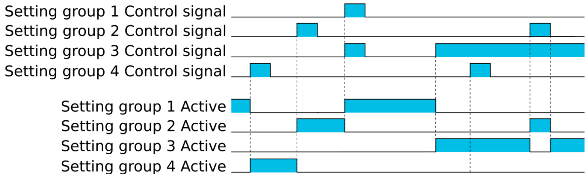
Figure. 5.5.1 - 162. Example sequences of group changing (control with pulse only, or with both pulses and static signals).
