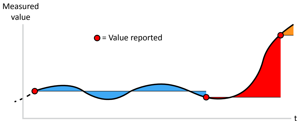
Figure. 6.3.7 - 138. Example graph showing how integration time affects measurement reporting. Small changes take longer to increase the integrated value over the deadband setting (blue area). Big changes meet the deadband criteria faster (red area).
