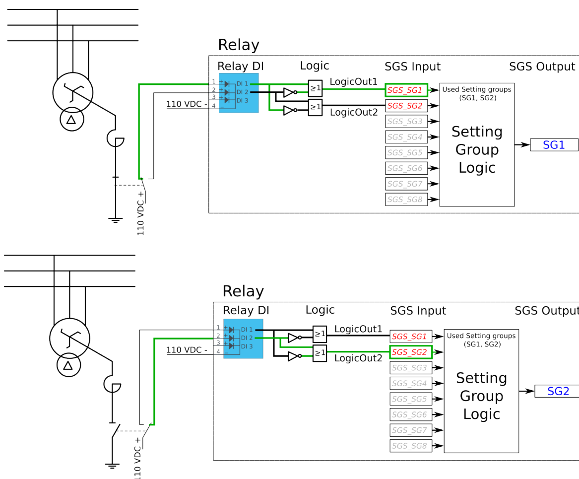
Figure. 5.5.1 - 105. Setting group control – two-wire connection from Petersen coil status with additional logic.
