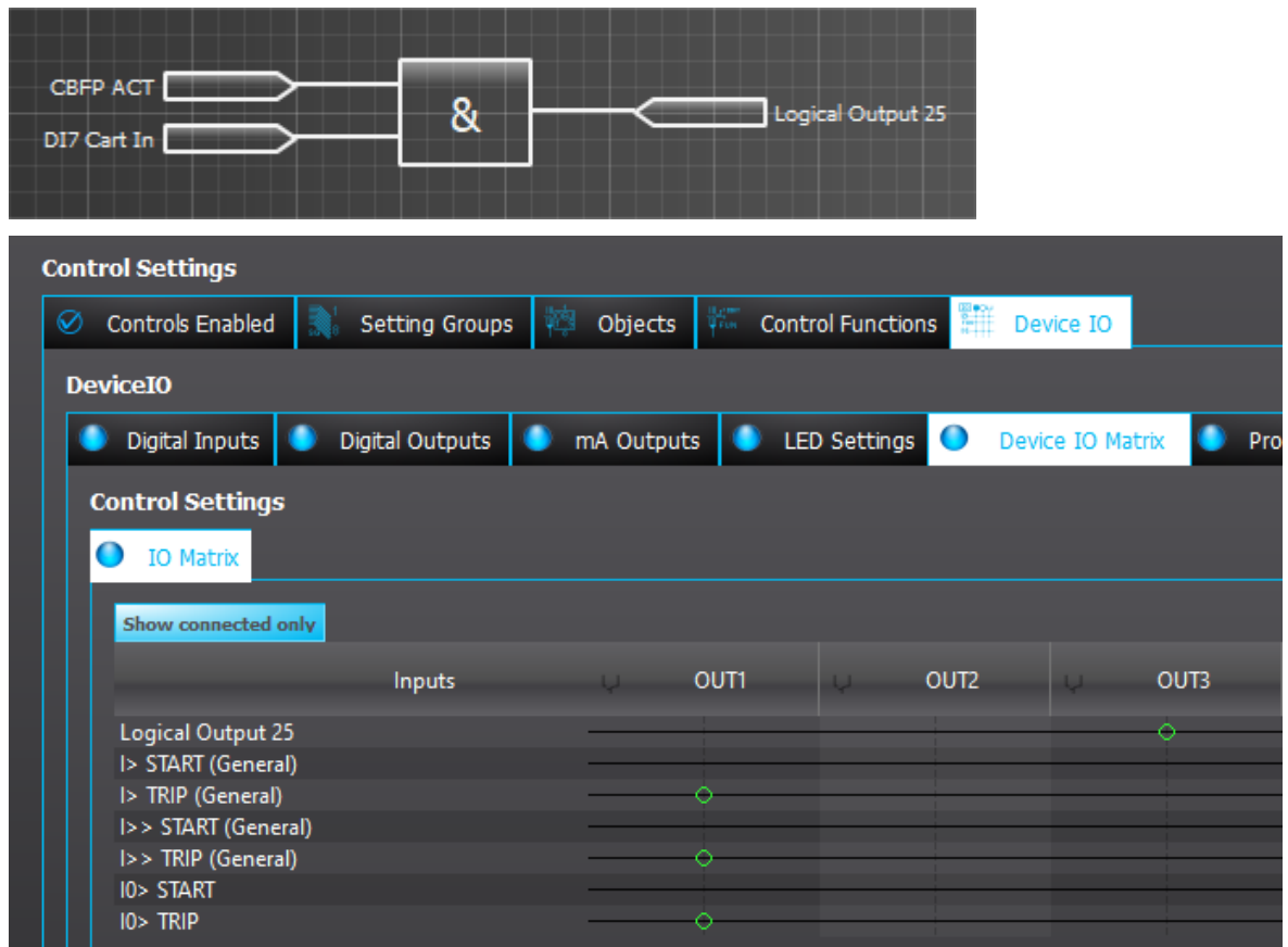
Figure. 5.5.7 - 117. Logic output example. Logical output is connected to an output relay in matrix.
