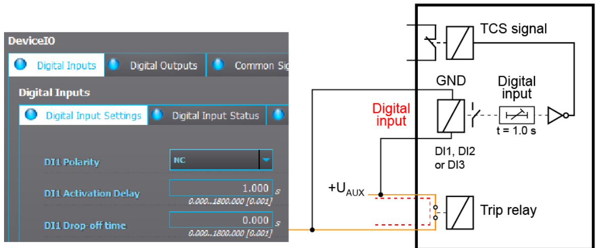
Figure. 7.2.3 - 145. Settings for a digital input used for trip circuit supervision.
