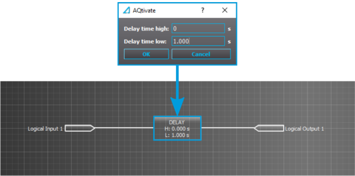
Figure. 5.5.8 - 119. Extending a logical input pulse.
