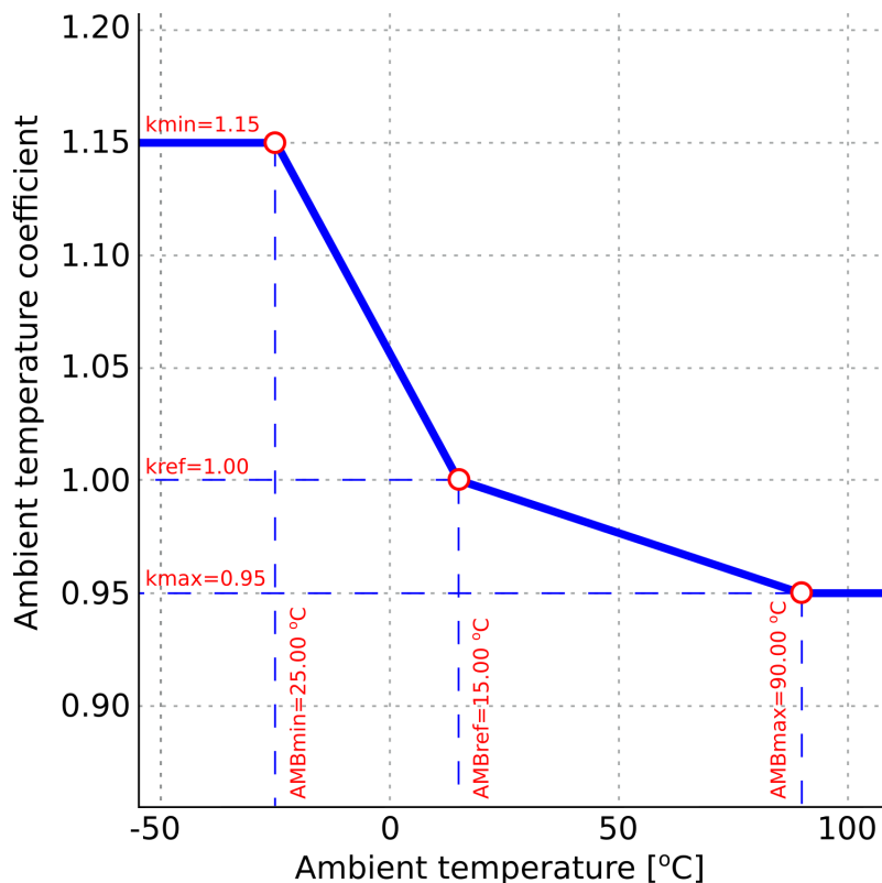
Figure. 5.4.7 - 89. Ambient temperature coefficient calculation (a three-point linear approximation and a settable correction curve).
