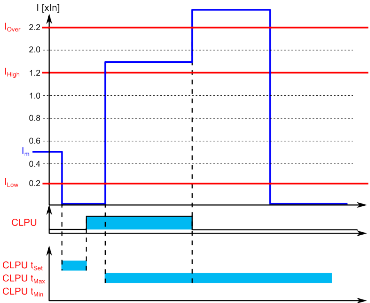
Figure. 5.5.3 - 111. Example of timers and pick-up parameters (activated pick-up and instant release due to overcurrent).
