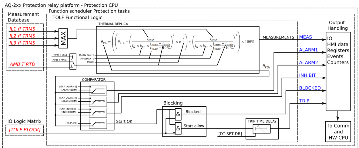
Figure. 5.4.7 - 100. Simplified function block diagram of the TF&gt; function.
