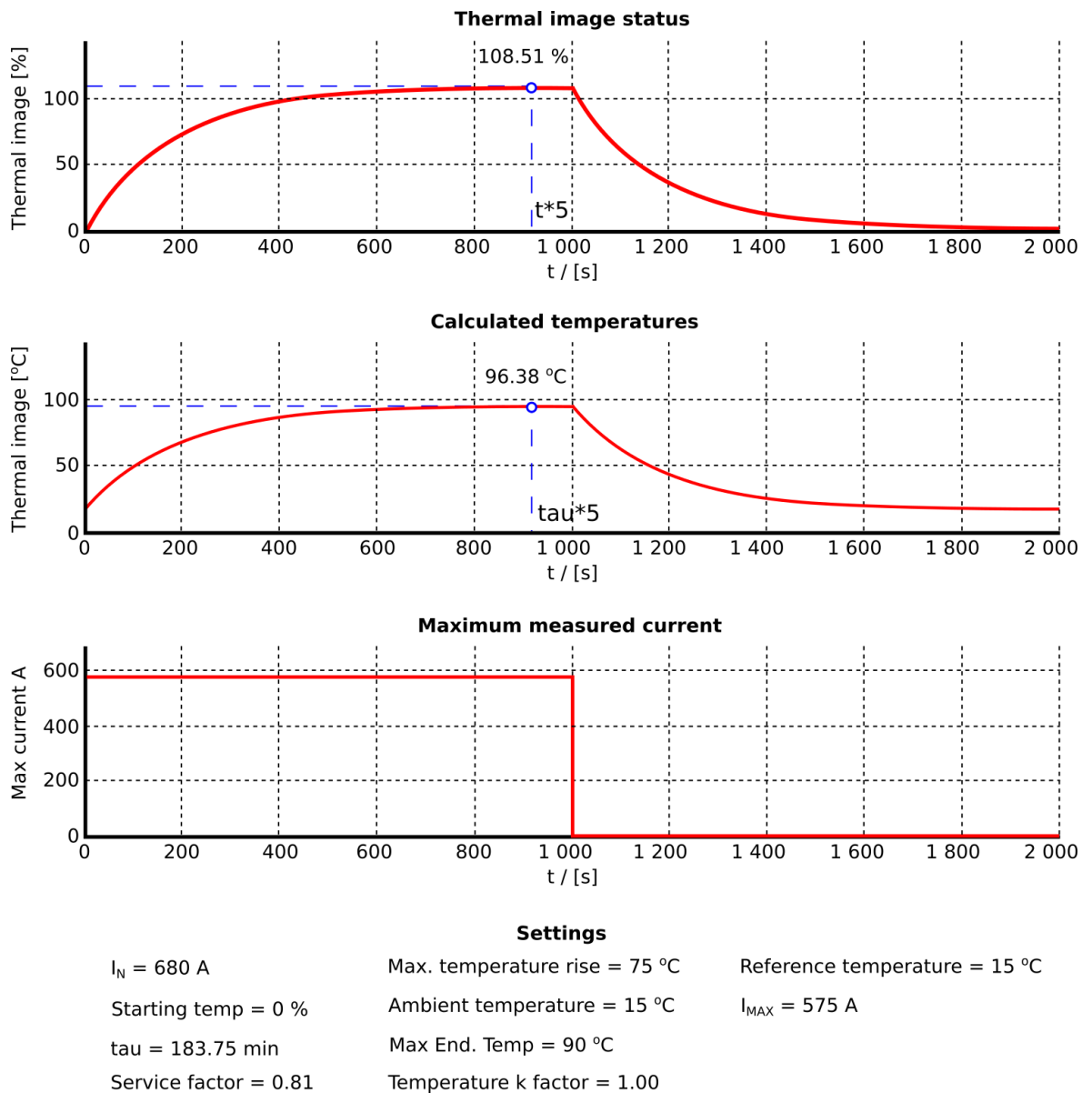
Figure. 5.4.7 - 98. Thermal image response with nominal currents and fine-tuned k_{SF} correction factor.
