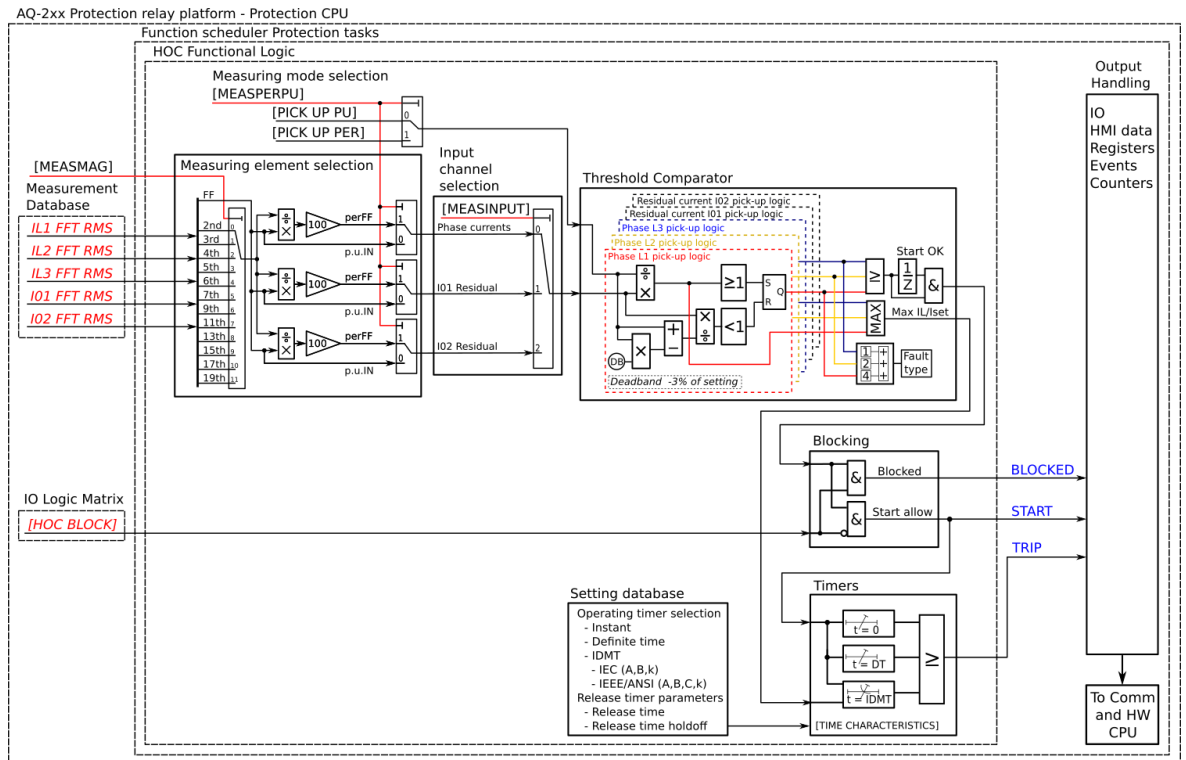
Figure. 5.4.5 - 76. Simplified function block diagram of the I_h > function.
