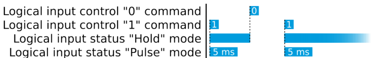
Figure. 5.5.8 - 118. Operation of logical input in "Hold" and "Pulse" modes.
