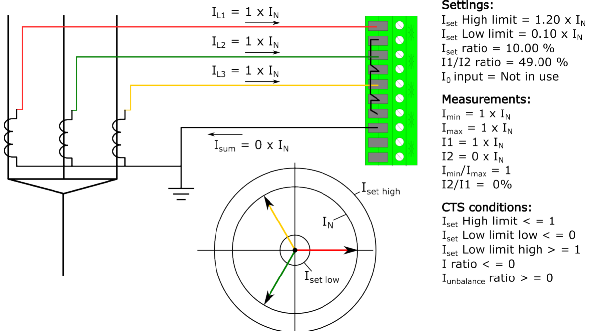
Figure. 5.6.1 - 122. All works properly, no faults.
