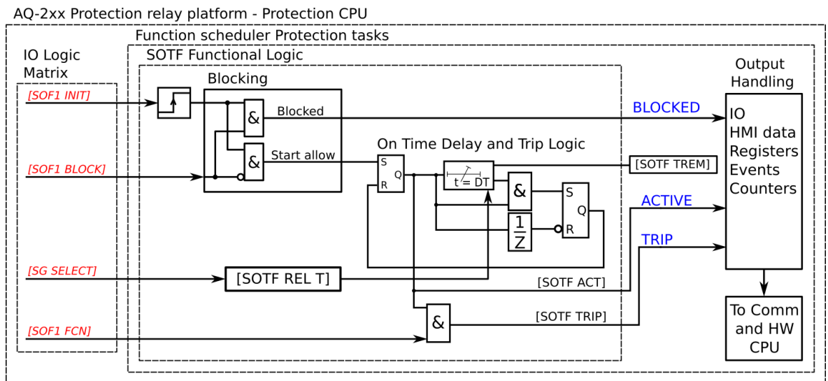
Figure. 5.5.4 - 115. Simplified function block diagram of the switch-on-to-fault function.
