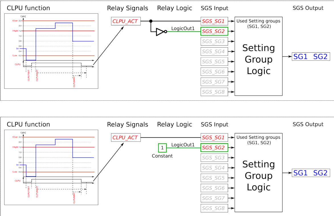
Figure. 5.5.1 - 106. Entirely application-controlled setting group change with the cold load pick-up function.
