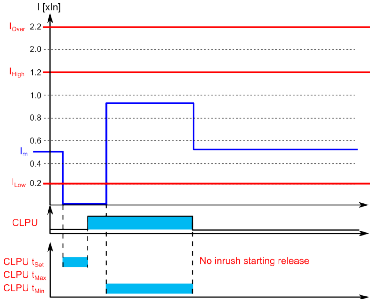
Figure. 5.5.3 - 113. Example of timers and pick-up parameters (no inrush current detected in the starting).
