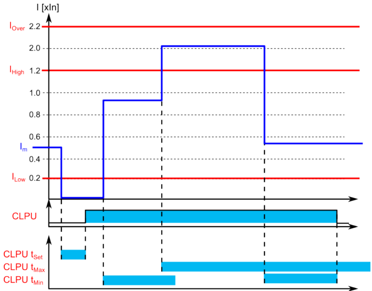
Figure. 5.5.3 - 114. Example of timers and pick-up parameters (an inrush current detected during T_{min} time).
