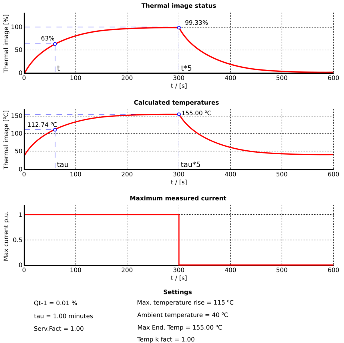
Figure. 5.4.7 - 88. Example of thermal image calculation with nominal conditions.
