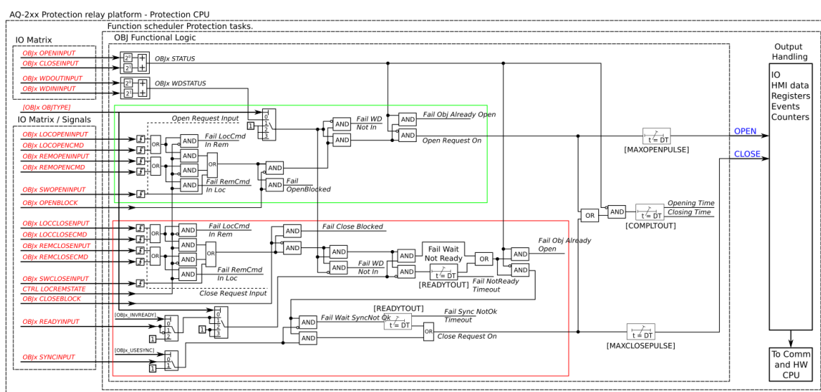
Figure. 5.5.2 - 107. Simplified function block diagram of the object control and monitoring function.
