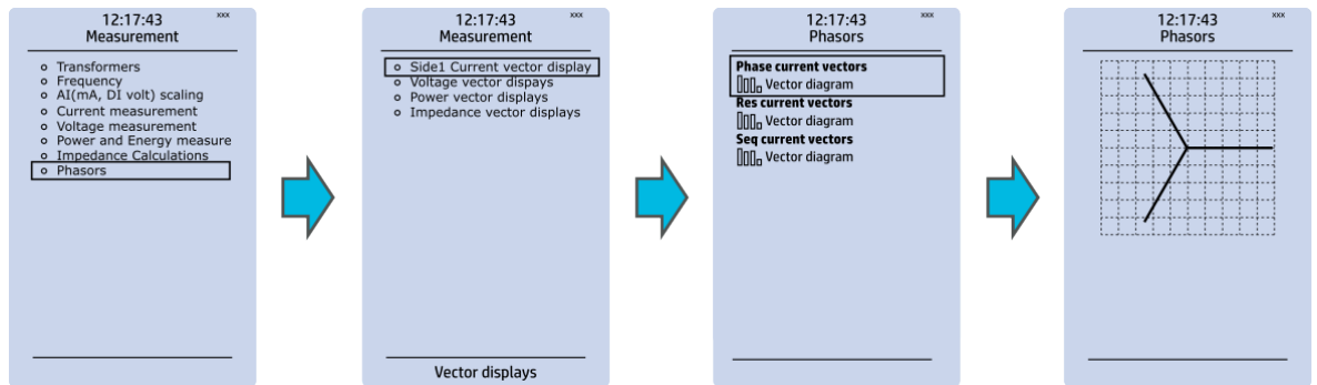
Figure. 4.8 - 47. Phasors submenu.
