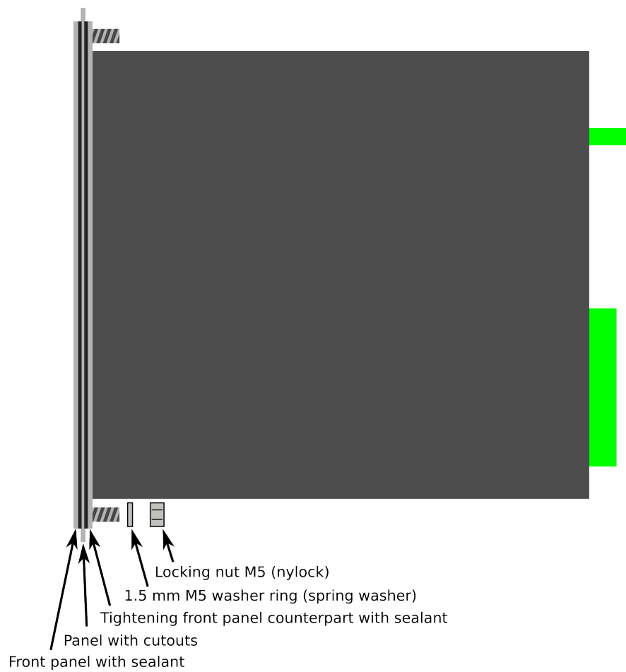
Figure. 8.4 - 152. Device installation.
