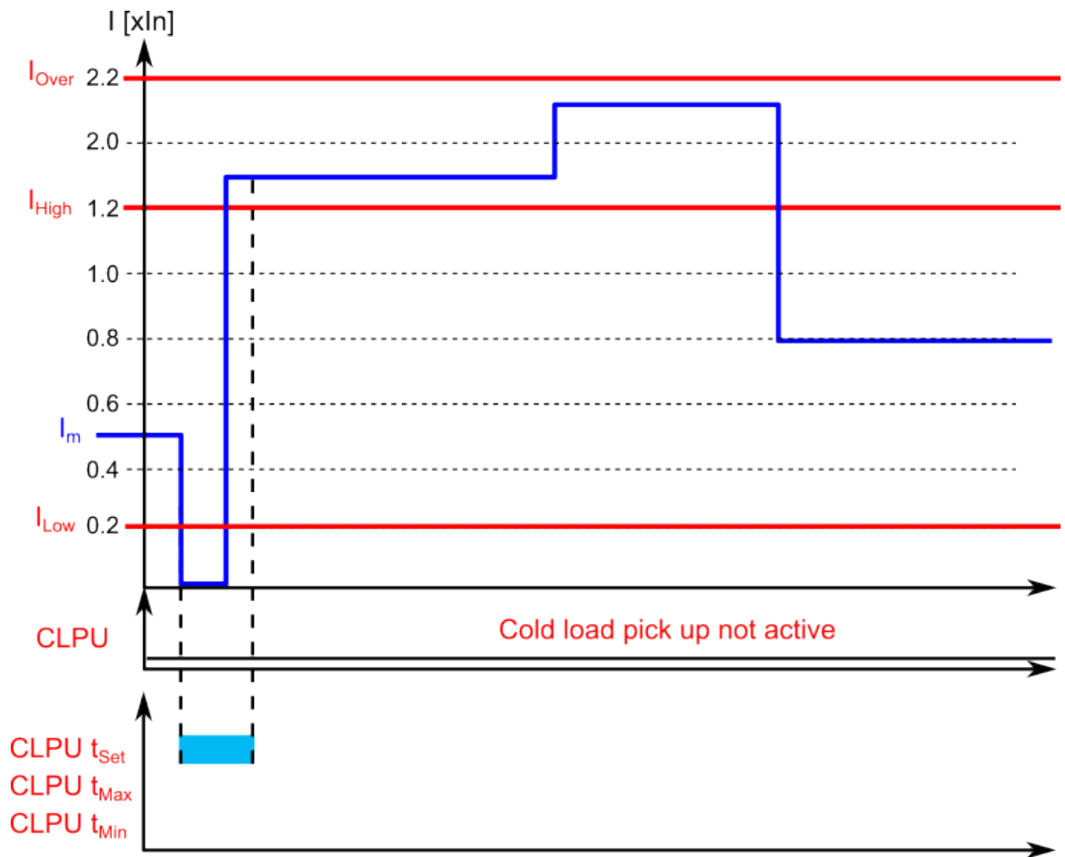
Figure. 5.5.3 - 110. Example of timers and pick-up parameters (no cold load pick-up, I_{low} too short).
