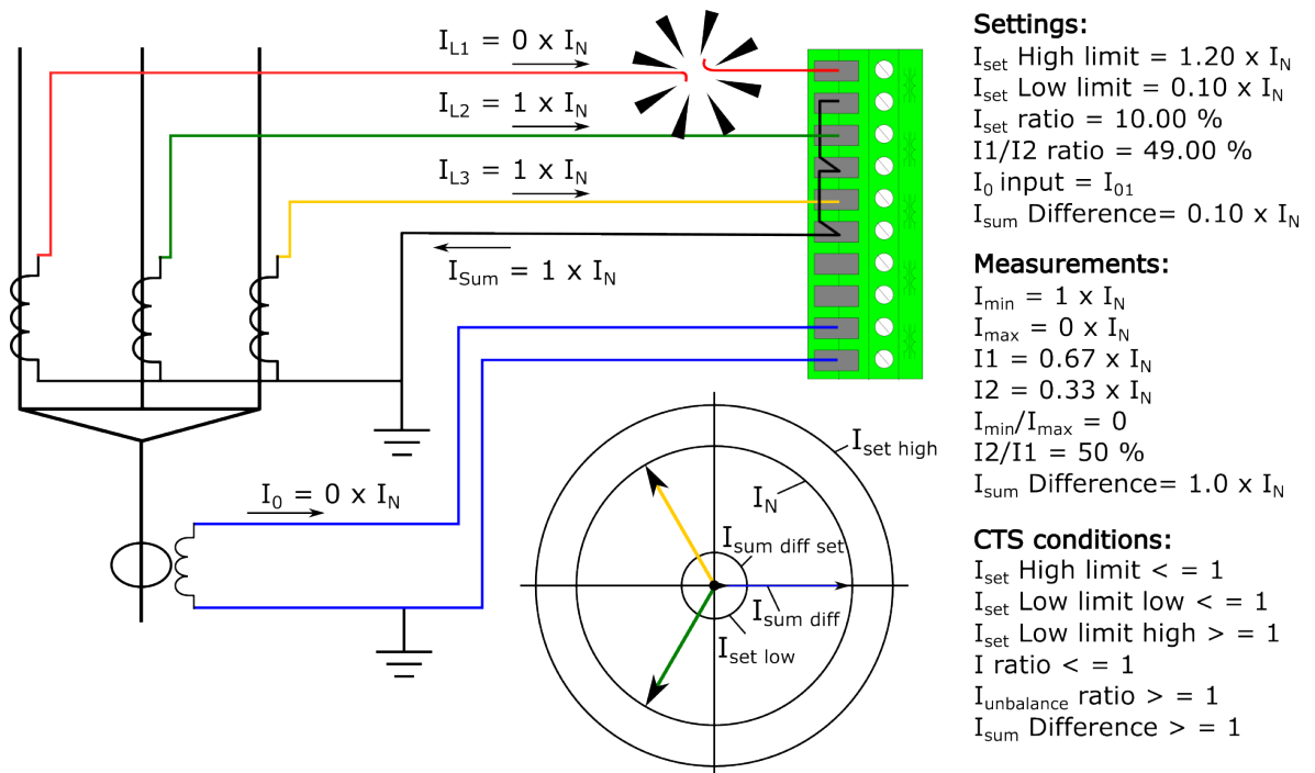
Figure. 5.6.1 - 128. Broken secondary phase current wiring.
