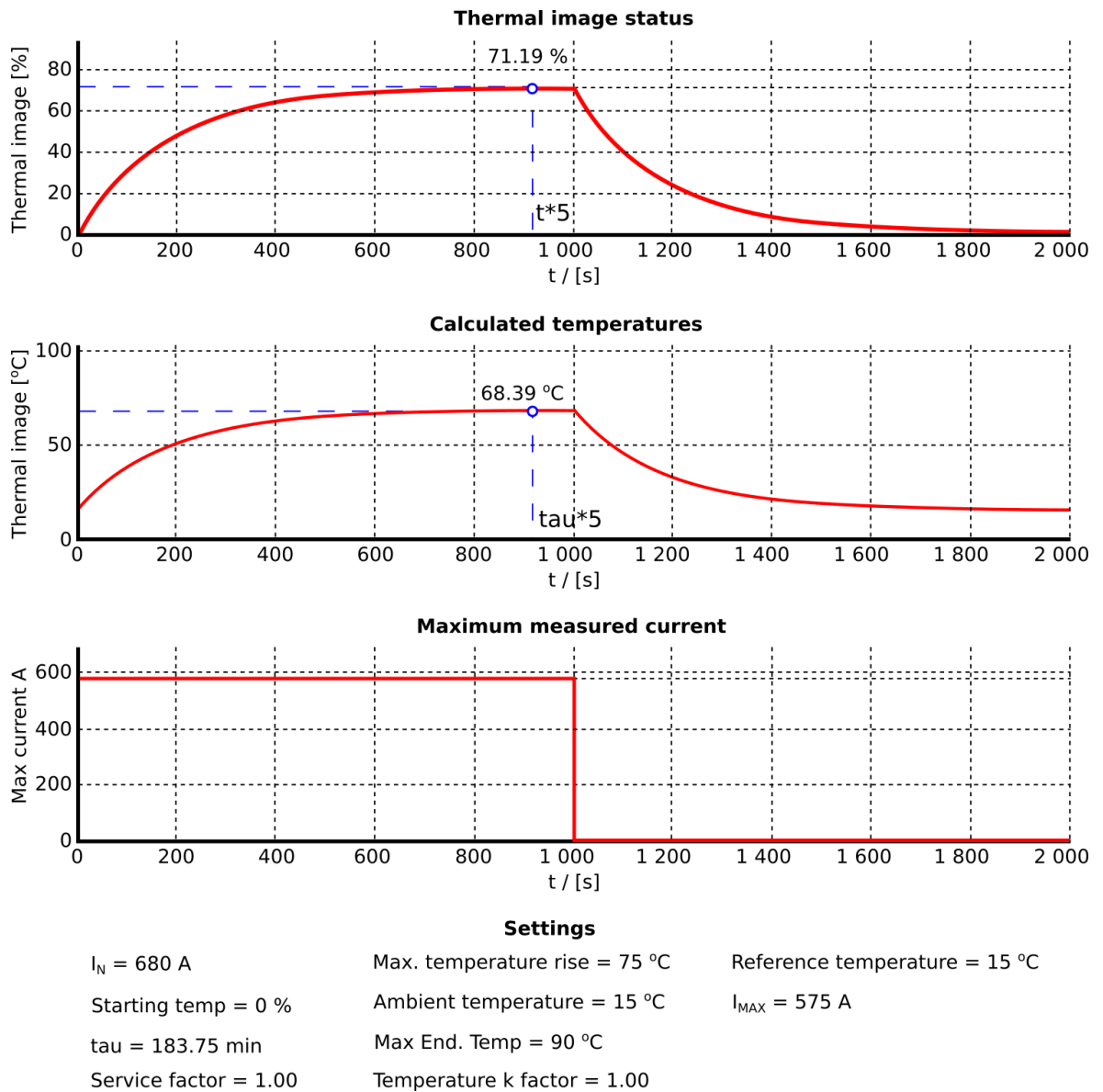
Figure. 5.4.7 - 96. Thermal image response with nominal load (installation according to presumptions).
