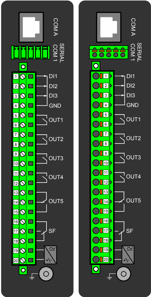
Figure. 8.2 - 149. CPU module can be equipped with standard screw terminals or spring cage terminals for connection.
