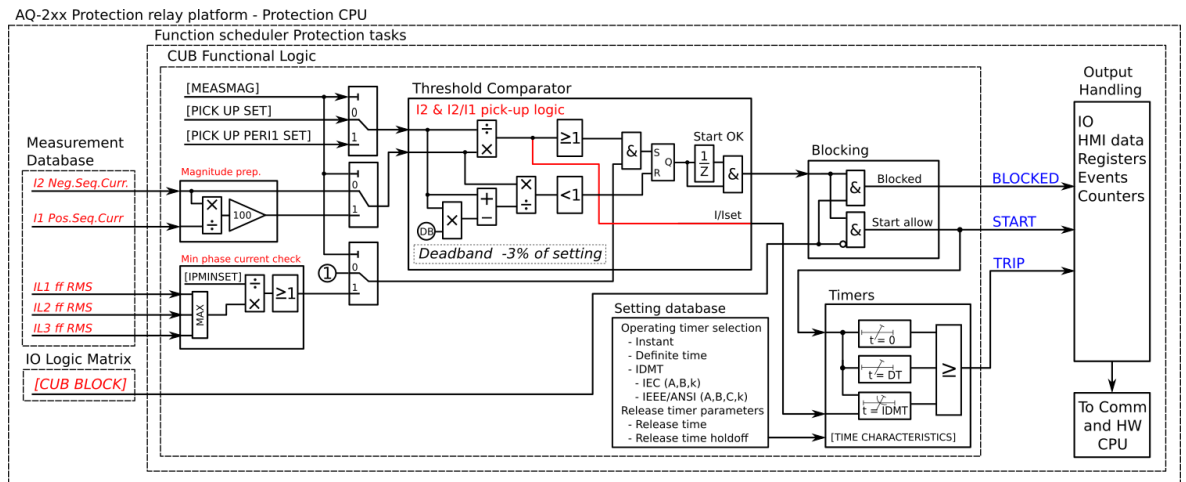
Figure. 5.4.4 - 74. Simplified function block diagram of the CUB function.
