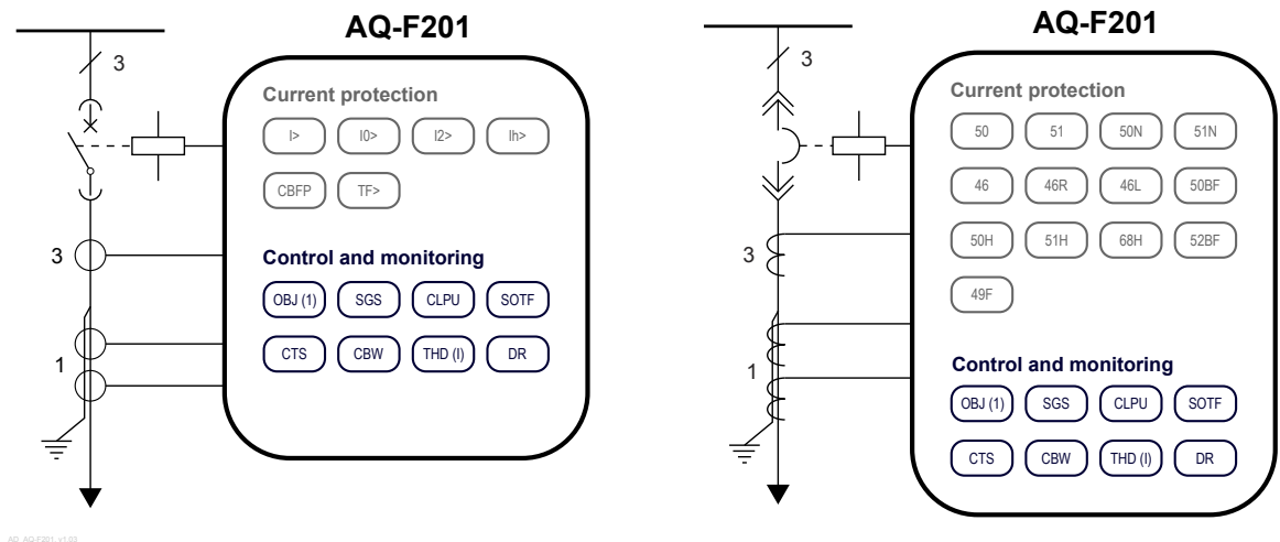
Figure. 7.1.1 - 141. AQ-F201 application example with function block diagram.
