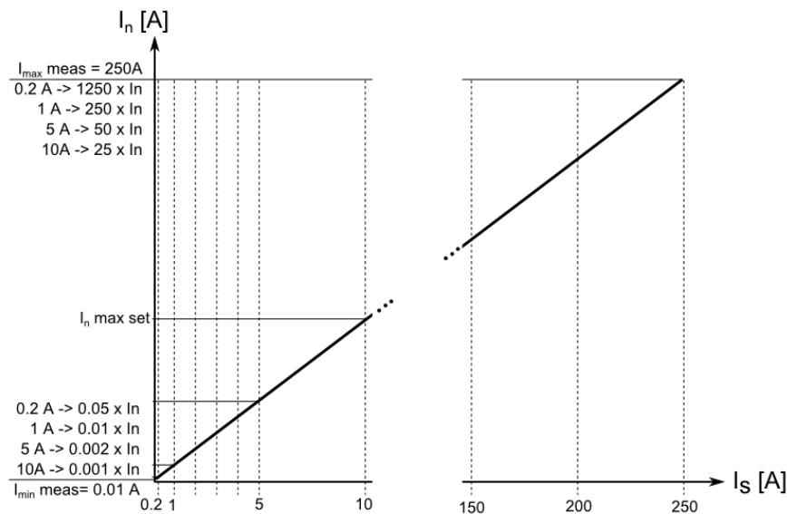
Figure. 5.4.1 - 65. Measurement range in relation to the nominal current.
