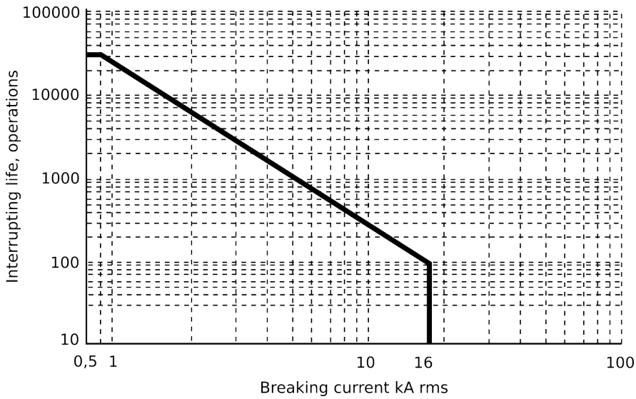
Figure. 5.6.2 - 131. Example of the circuit breaker interrupting life operations.
