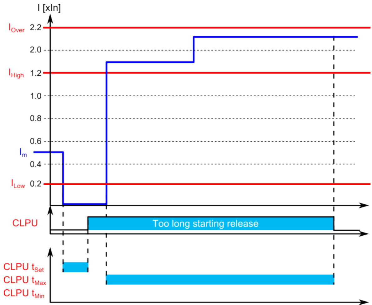
Figure. 5.5.3 - 112. Example of timers and pick-up parameters (activated pick-up and instant release due to too long starting).
