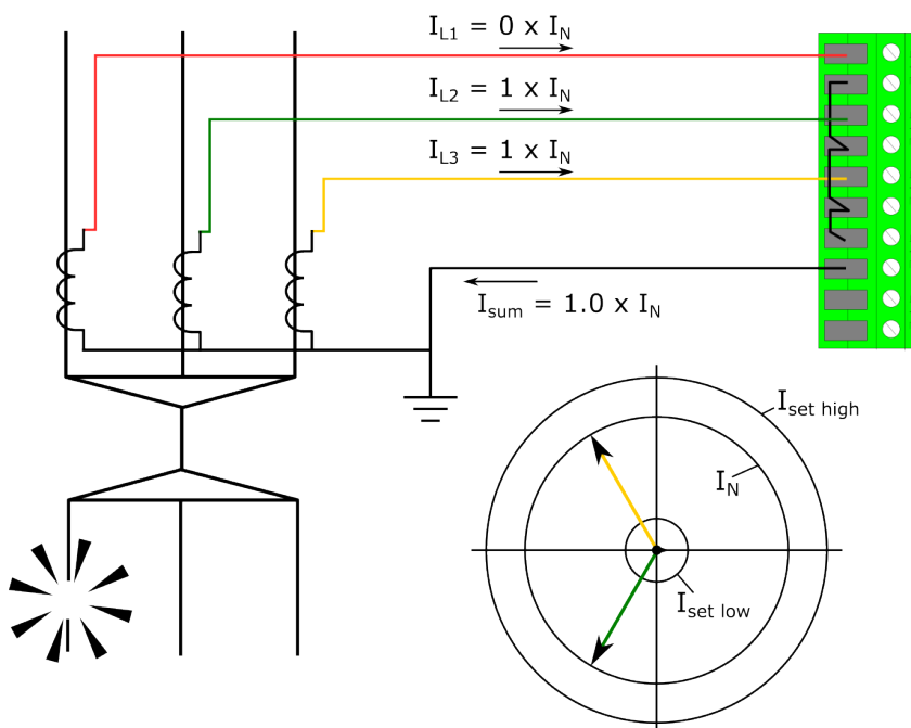
Figure. 5.6.1 - 124. Primary circuit fault in phase L1 wiring.
