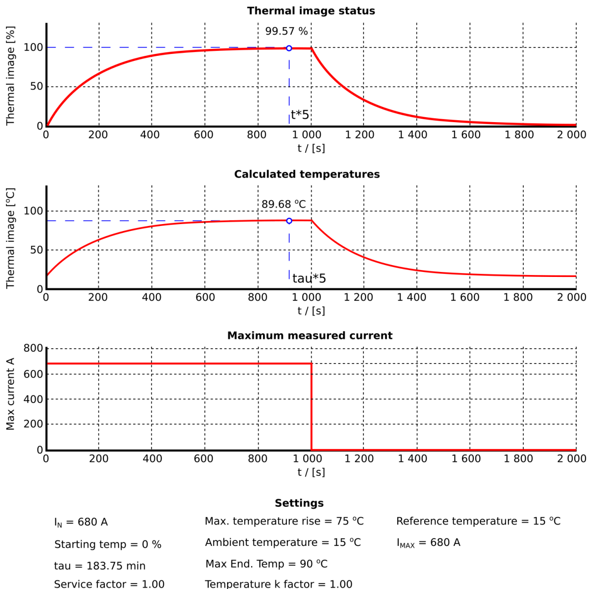
Figure. 5.4.7 - 97. Thermal image response with maximum load (installation according presumptions).
