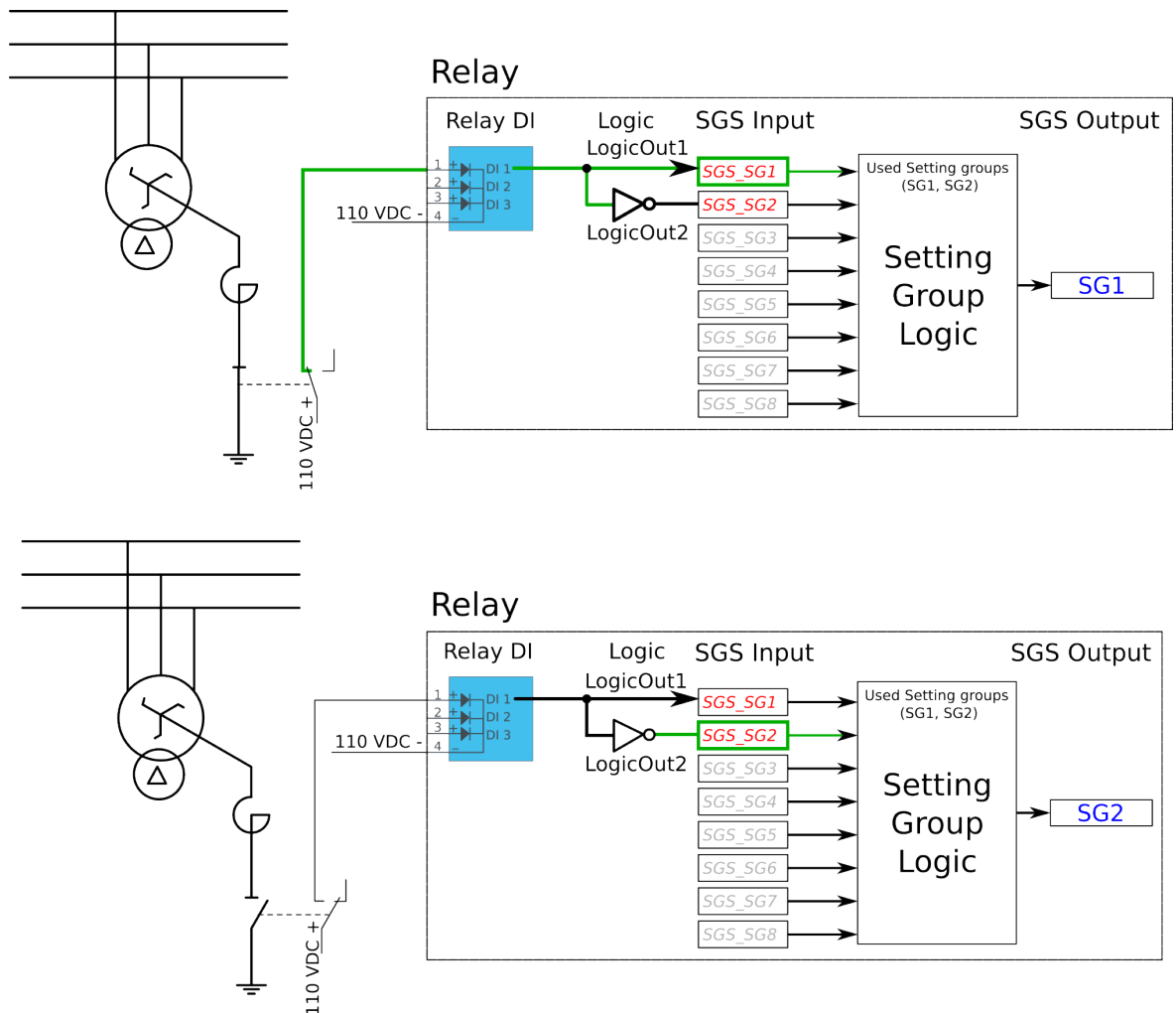
Figure. 5.5.1 - 103. Setting group control – one-wire connection from Petersen coil status.
