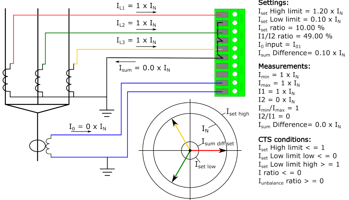
Figure. 5.6.1 - 127. Normal situation, residual current also measured.
