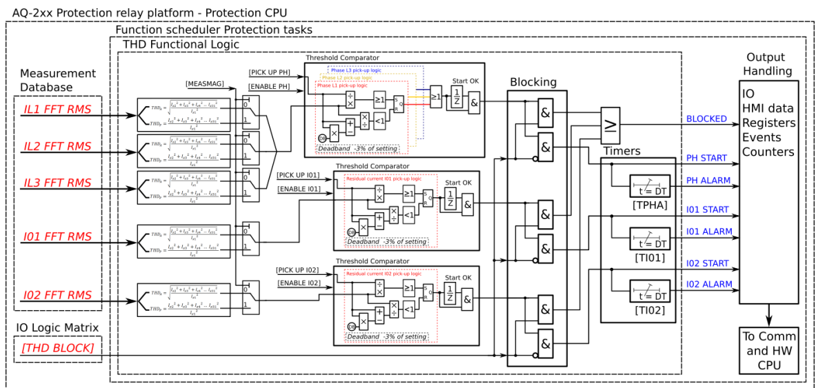
Figure. 5.6.3 - 134. Simplified function block diagram of the total harmonic distortion monitor function.
