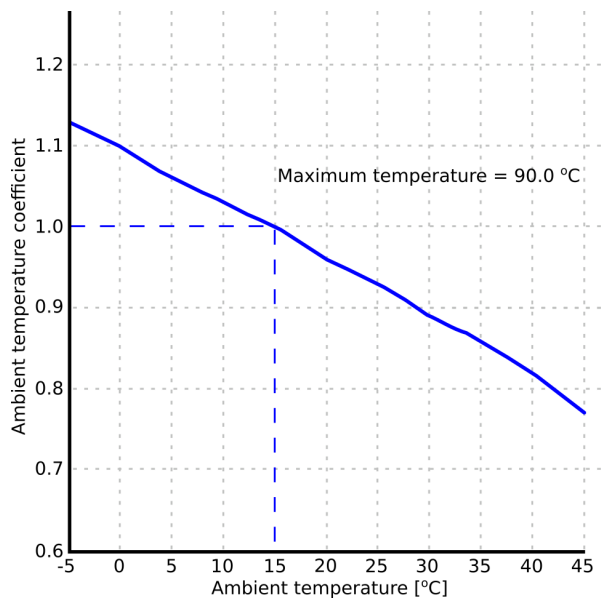
Figure. 5.4.7 - 92. Set correction curve for ambient temperature.
