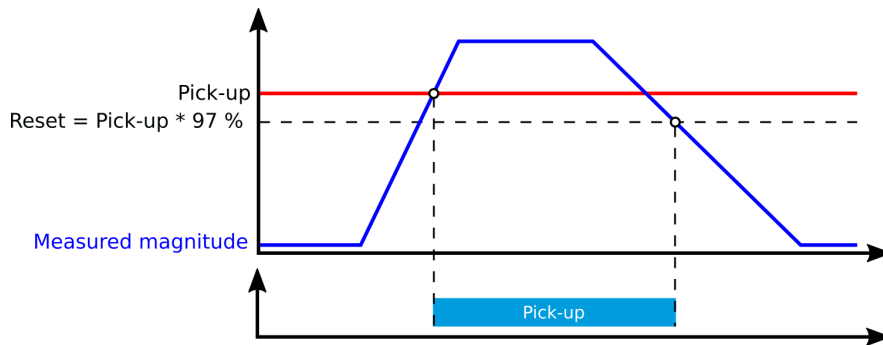
Figure. 5.4.1 - 64. Pick up and reset.
