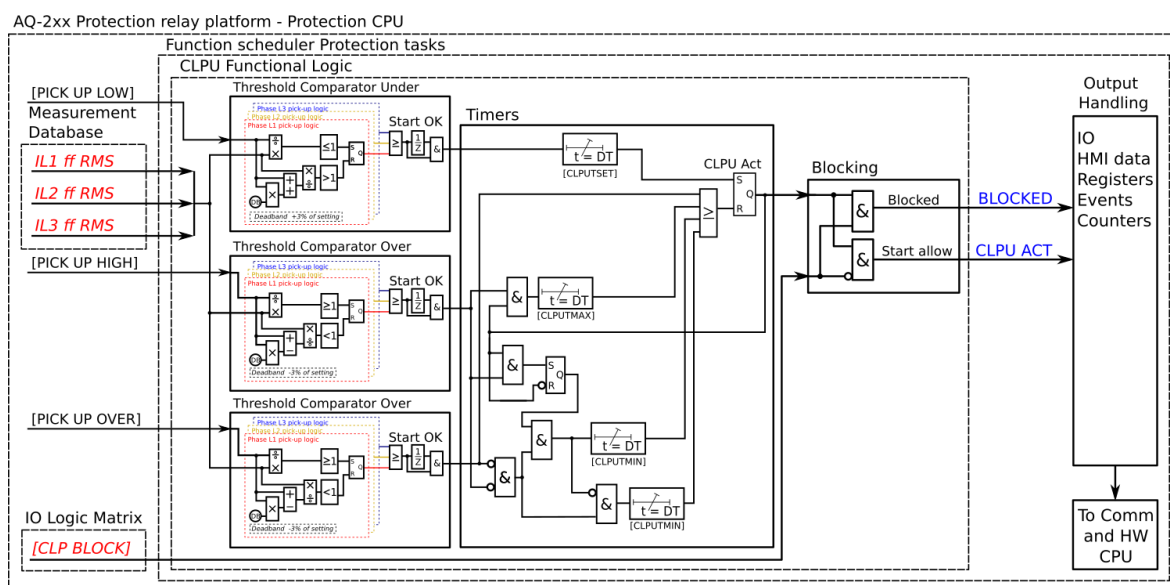
Figure. 5.5.3 - 108. Simplified function block diagram of the cold load pick-up function.
