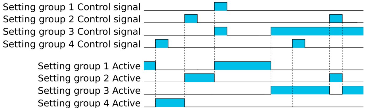
Figure. 5.5.1 - 102. Example sequences of group changing (control with pulse only, or with both pulses and static signals).
