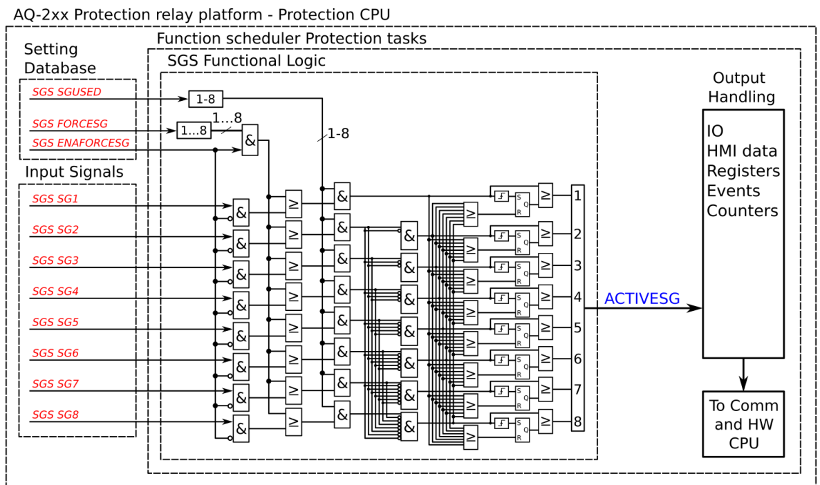
Figure. 5.5.1 - 101. Simplified function block diagram of the setting group selection function.
