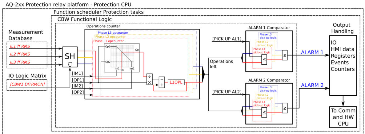
Figure. 5.6.2 - 132. Simplified function block diagram of the circuit breaker wear function.
