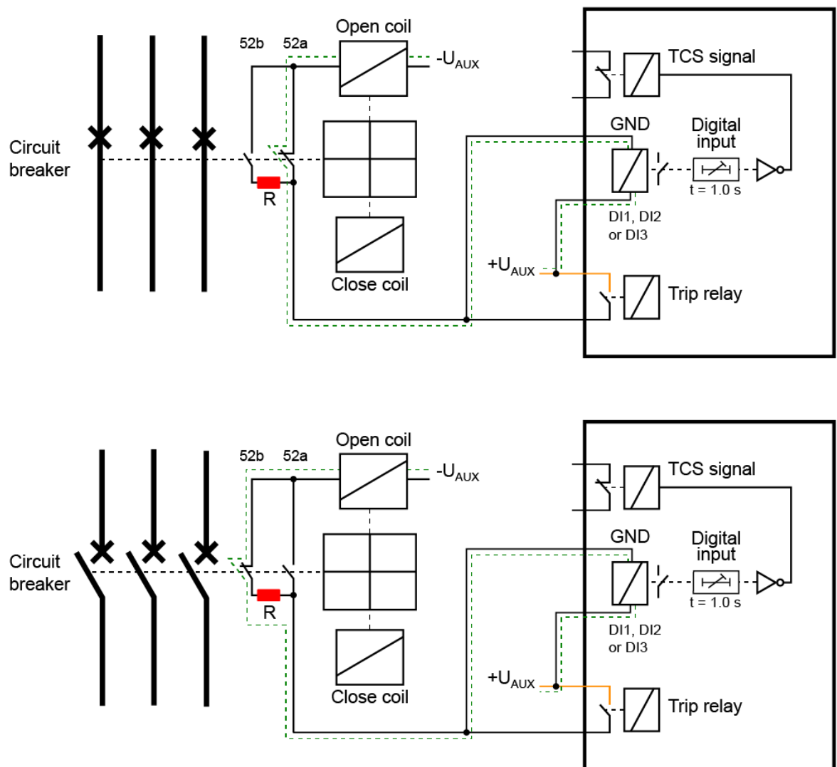
Figure. 7.2.3 - 144. Trip circuit supervision with one DI and one non-latched trip output.
