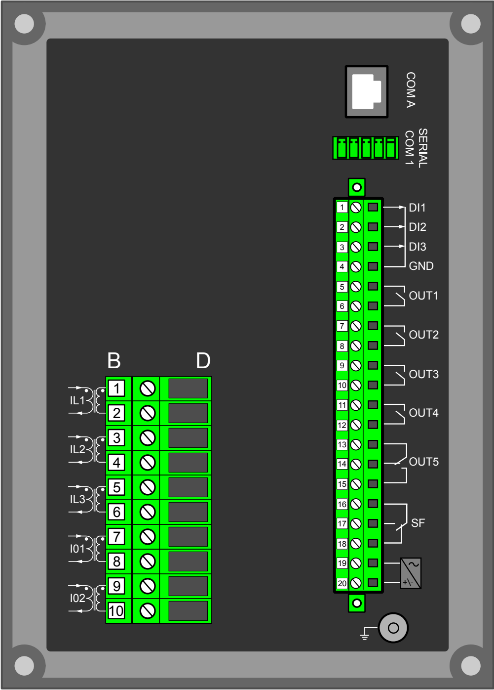
Figure. 8.1 - 148. Connections and modules in AQ-F201.
