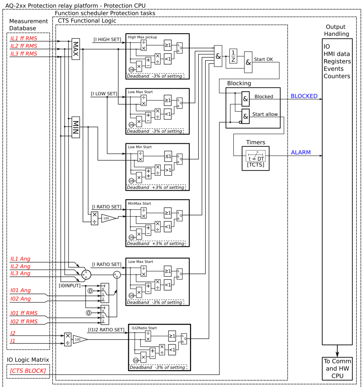
Figure. 5.6.1 - 121. Simplified function block diagram of the CTS function.
