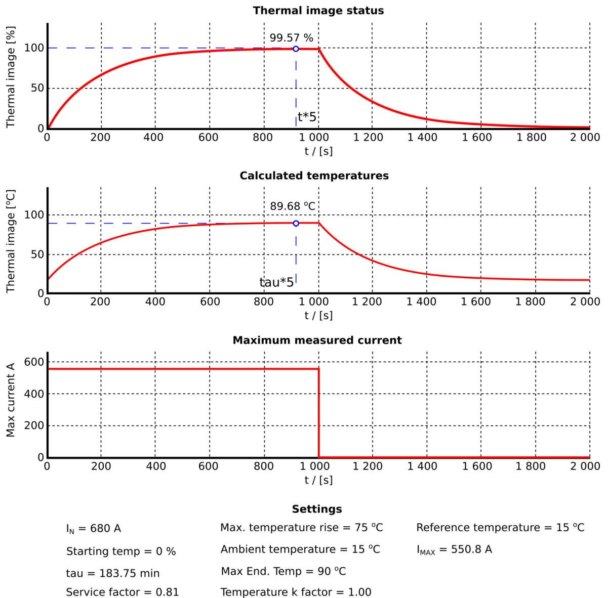
Figure. 5.4.7 - 99. Thermal response with k sf factor correctly set.
