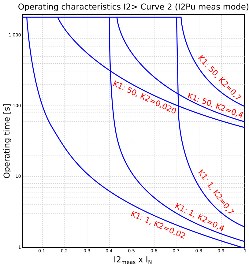
Figure. 5.4.4 - 75. Operation characteristics curve for I_2 > \text{Curve2} .
