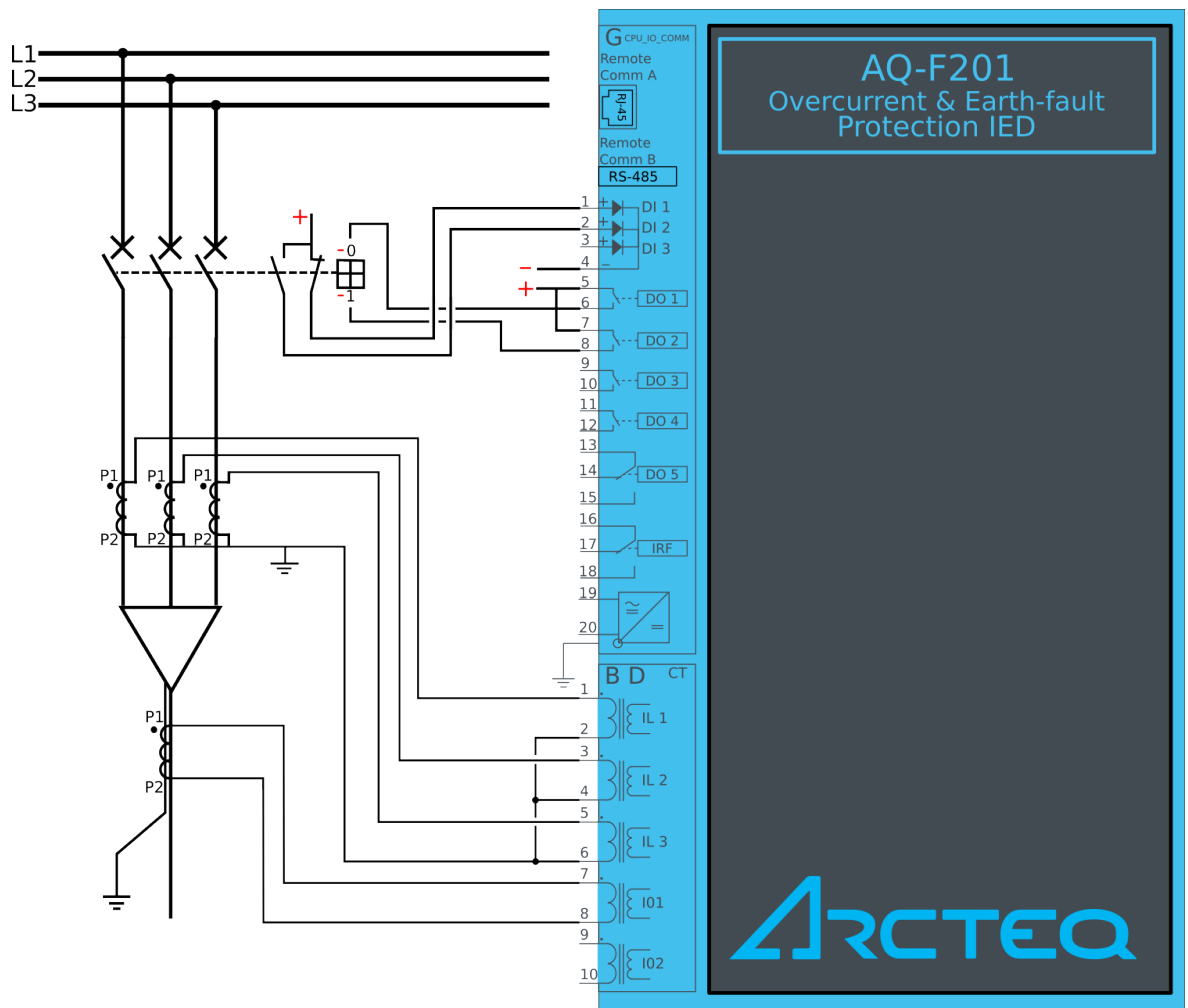
Figure. 7.2.1 - 142. Application example and its connections.
