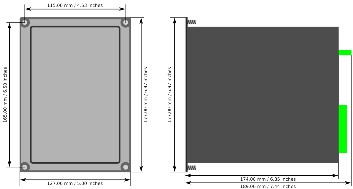
Figure. 8.4 - 151. Device dimensions.
