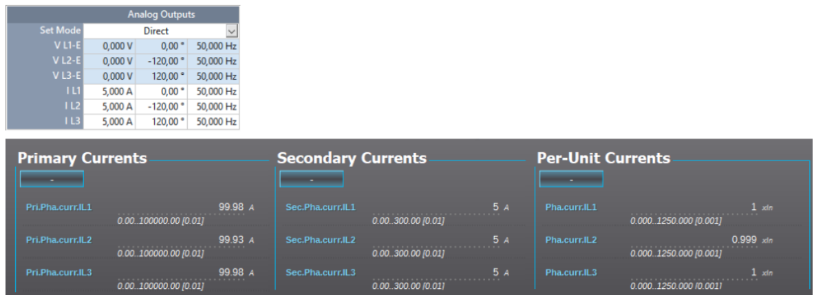
Figure. 5.2.1 - 59. Scalings display (based on the CT nominal).
