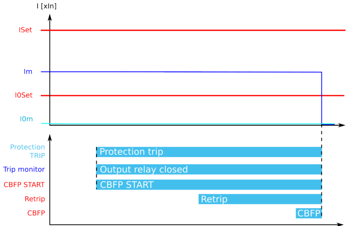
Figure. 5.4.6 - 88. Retrip and CBFP when "Current or DO" is the selected criterion.
