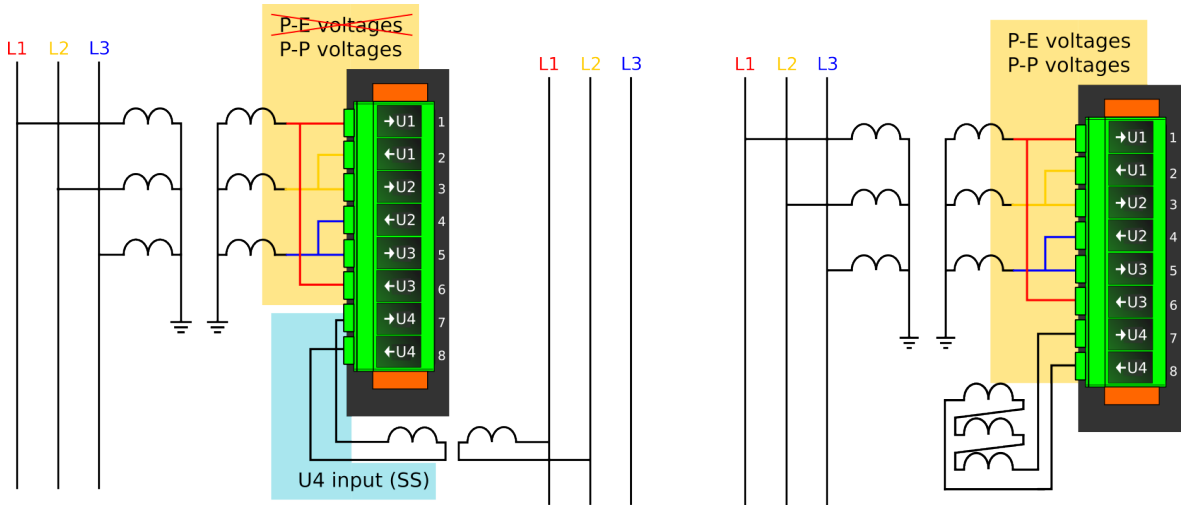
Figure. 5.4.8 - 101. Selectable measurement magnitudes with 3LL+U4 VT connection (P-E voltages not available without residual voltage).
