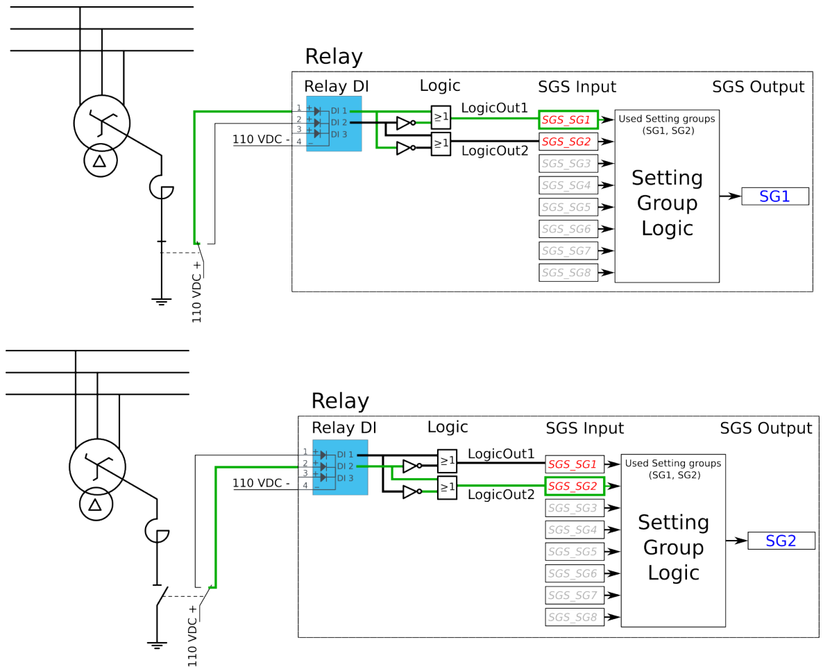
Figure. 5.5.1 - 137. Setting group control – two-wire connection from Petersen coil status with additional logic.
