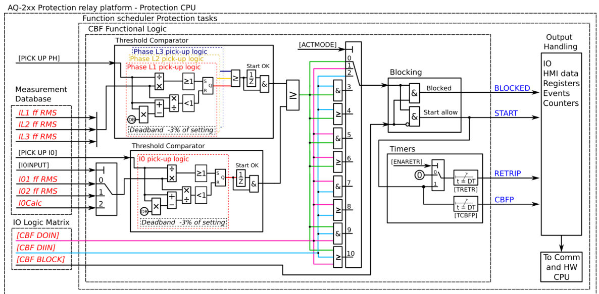
Figure. 5.4.6 - 84. Simplified function block diagram of the CBFP function.
