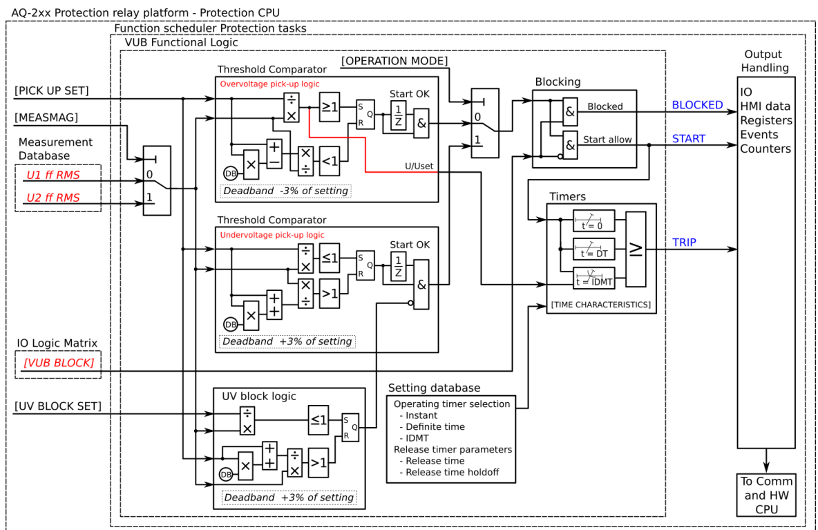
Figure. 5.4.10 - 114. Simplified function block diagram of the U1/U2&gt;/&lt; function.
