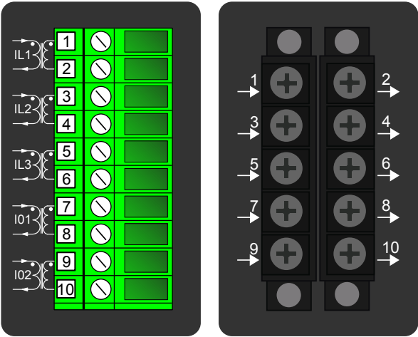
Figure. 8.3 - 181. Module connections with standard and ring lug terminals.
