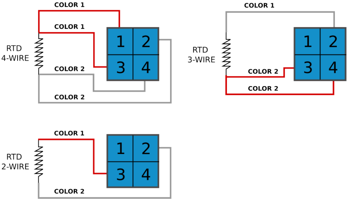
Figure. 8.5.4 - 188. RTD sensor connection types.
