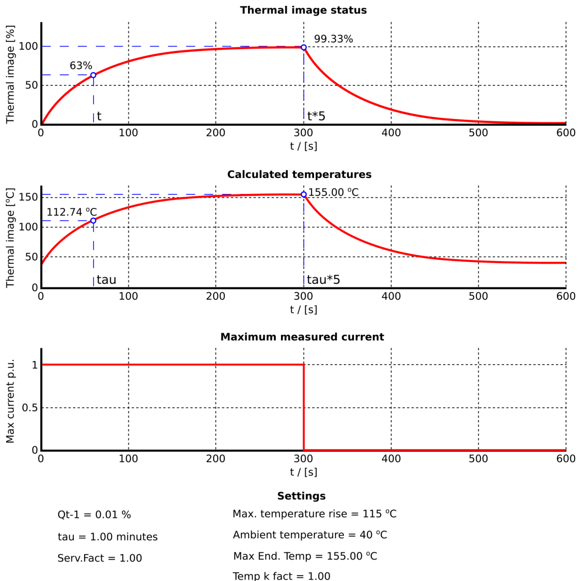
Figure. 5.4.11 - 116. Example of thermal image calculation with nominal conditions.
