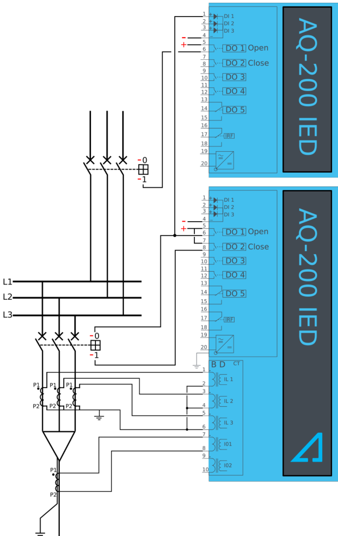
Figure. 5.4.6 - 93. Wiring diagram when the device is configured as a dedicated CBFP unit.
