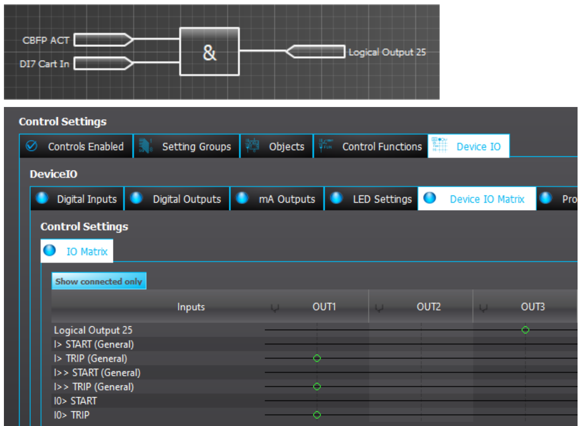
Figure. 5.5.8 - 143. Logic output example. Logical output is connected to an output relay in matrix.
