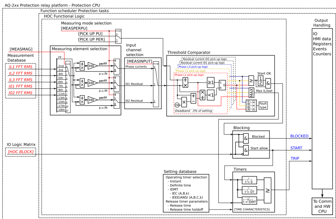
Figure. 5.4.5 - 83. Simplified function block diagram of the Ih&gt; function.
