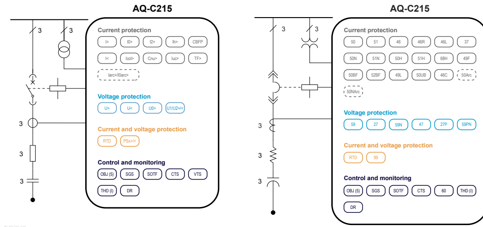
Figure. 7.1.1 - 170. AQ-C215 application example with function block diagram.
