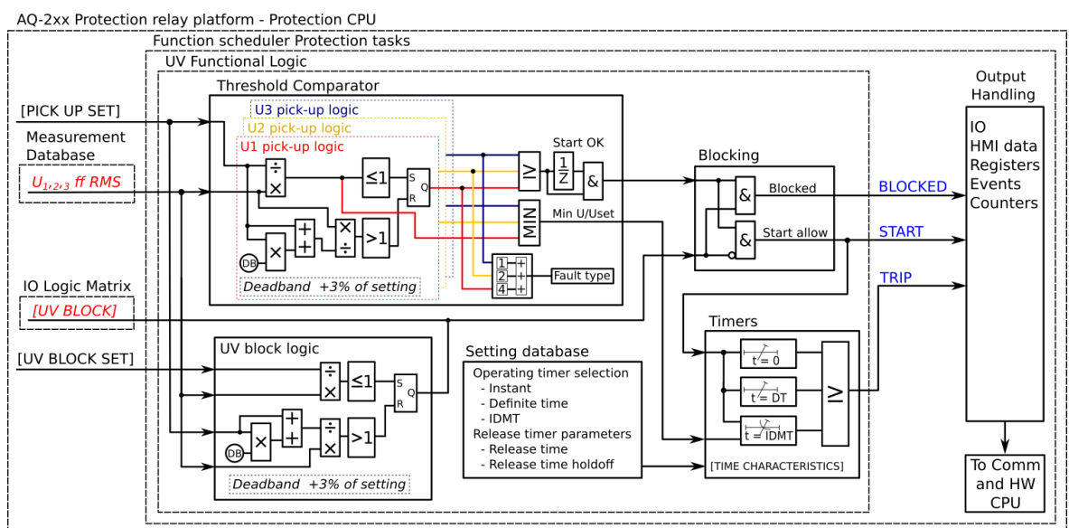
Figure. 5.4.8 - 99. Simplified function block diagram of the U < function.
