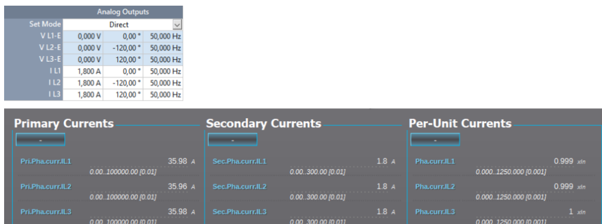
Figure. 5.2.1 - 64. Scalings display (based on the protected object's nominal current).
