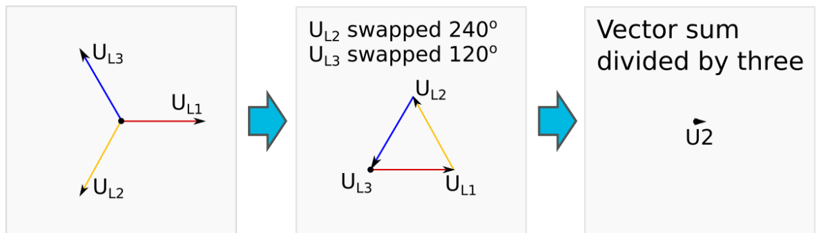
Figure. 5.4.10 - 111. Normal situation.
