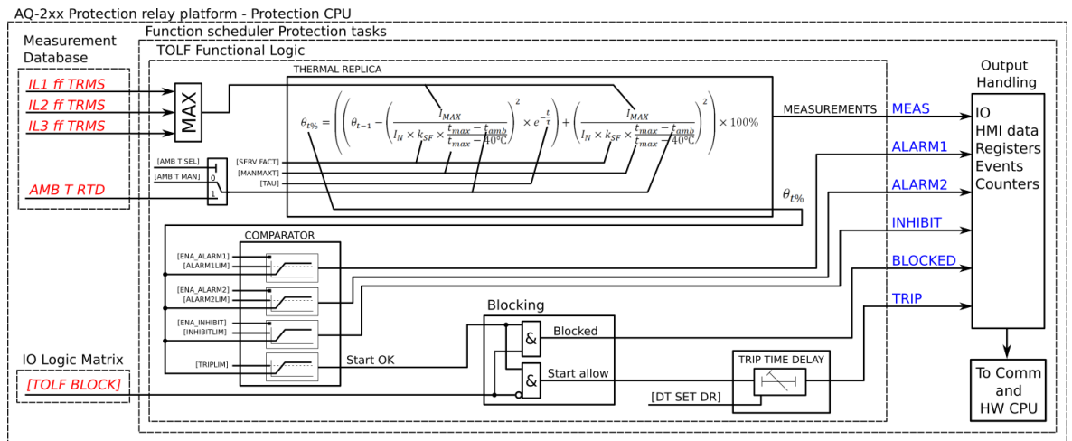
Figure. 5.4.11 - 128. Simplified function block diagram of the TF> function.
