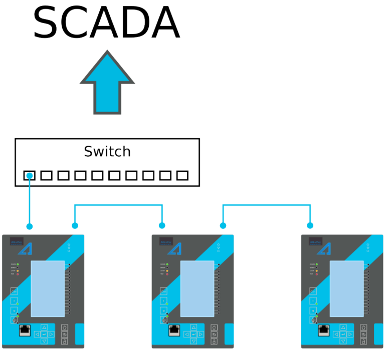
Figure. 8.5.7 - 192. Example of a multidrop configuration.
