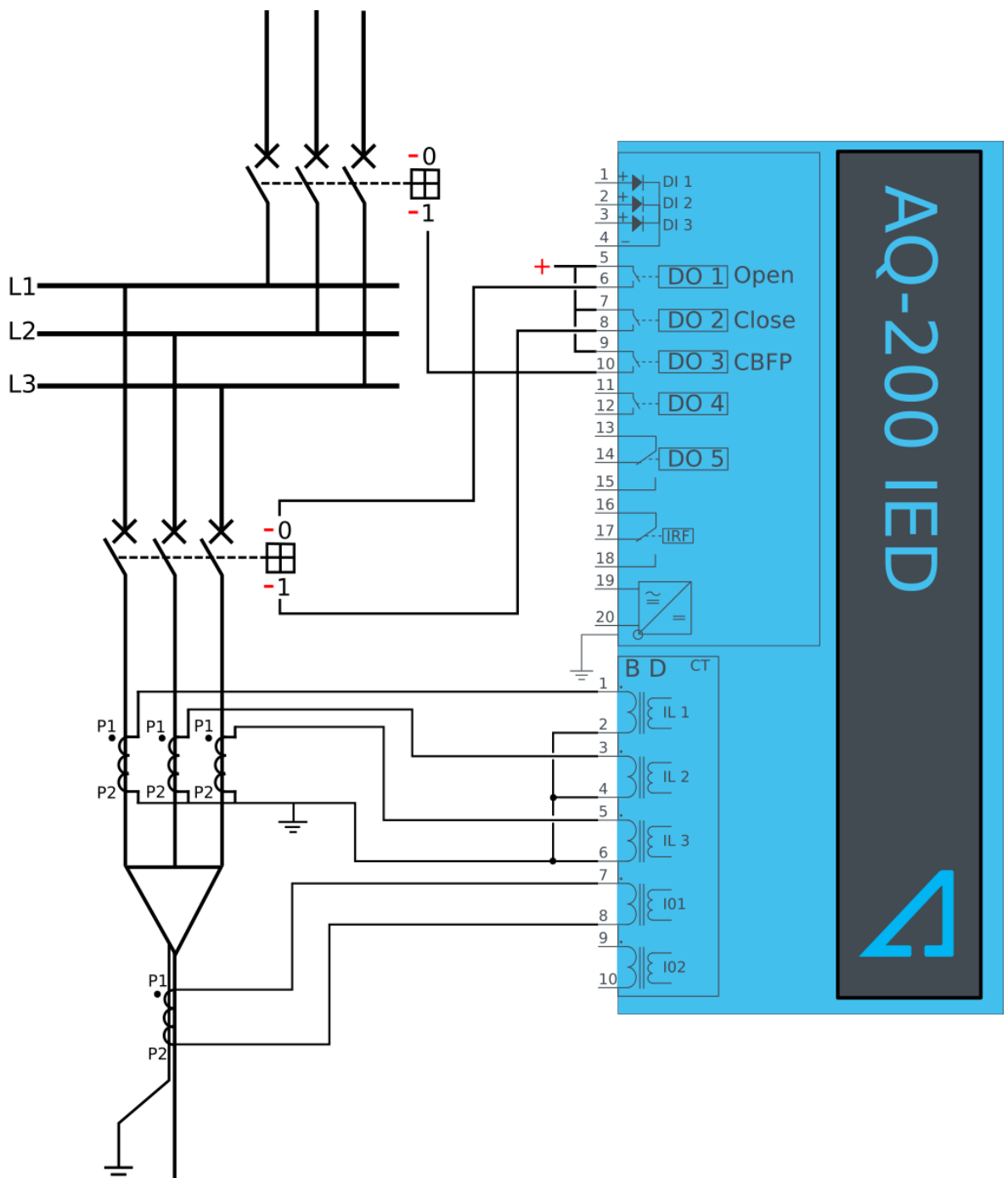
Figure. 5.4.6 - 89. Wiring diagram when Trip and CBFP are configured to the device.
