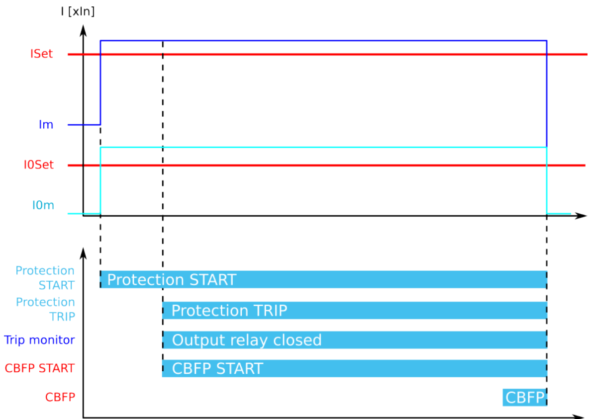
Figure. 5.4.6 - 91. CBFP when "Current and DO" is the selected criterion.
