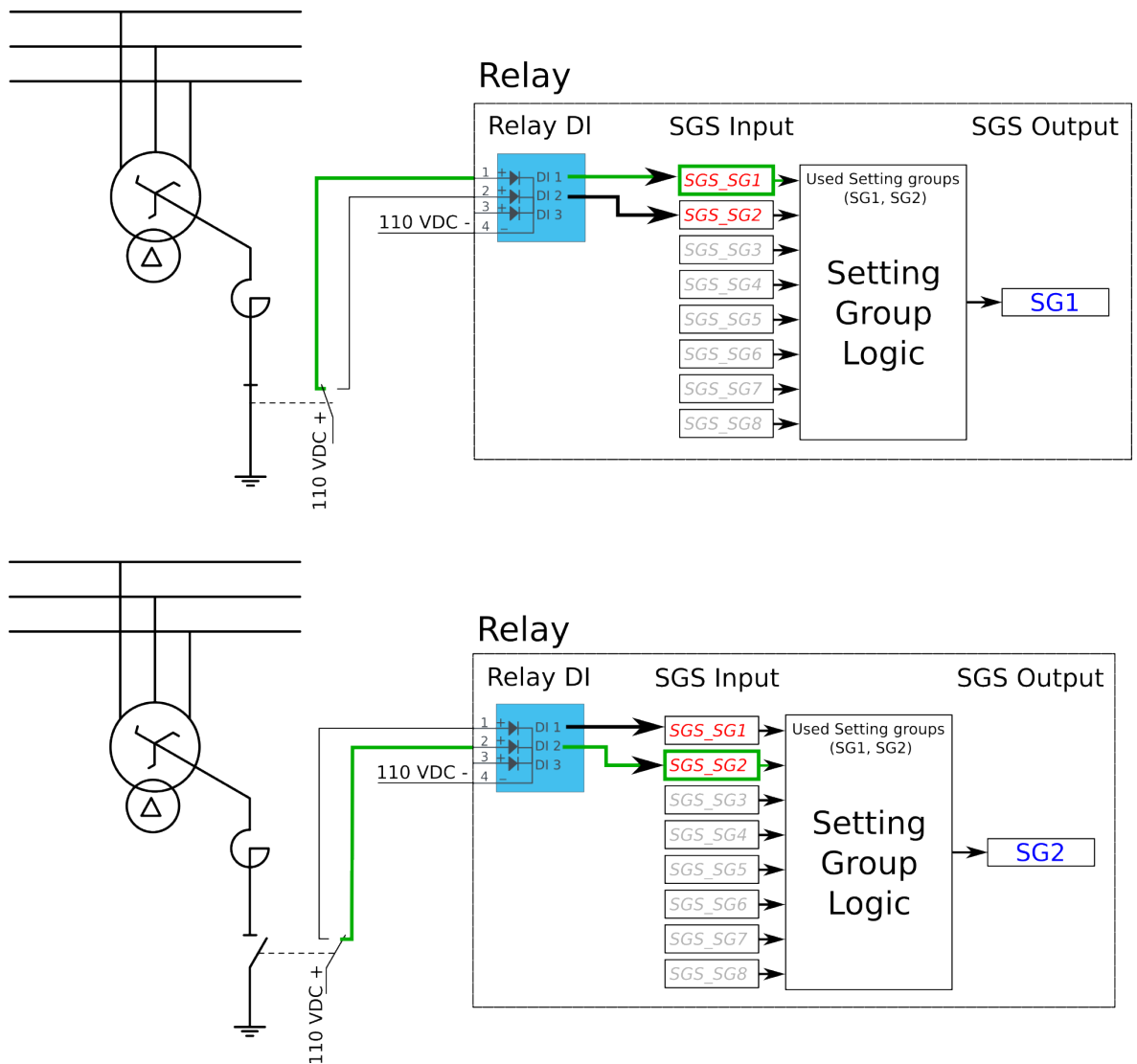
Figure. 5.5.1 - 136. Setting group control – two-wire connection from Petersen coil status.
