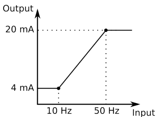
Figure. 5.5.5 - 141. Example of the effects of mA output channel settings.
