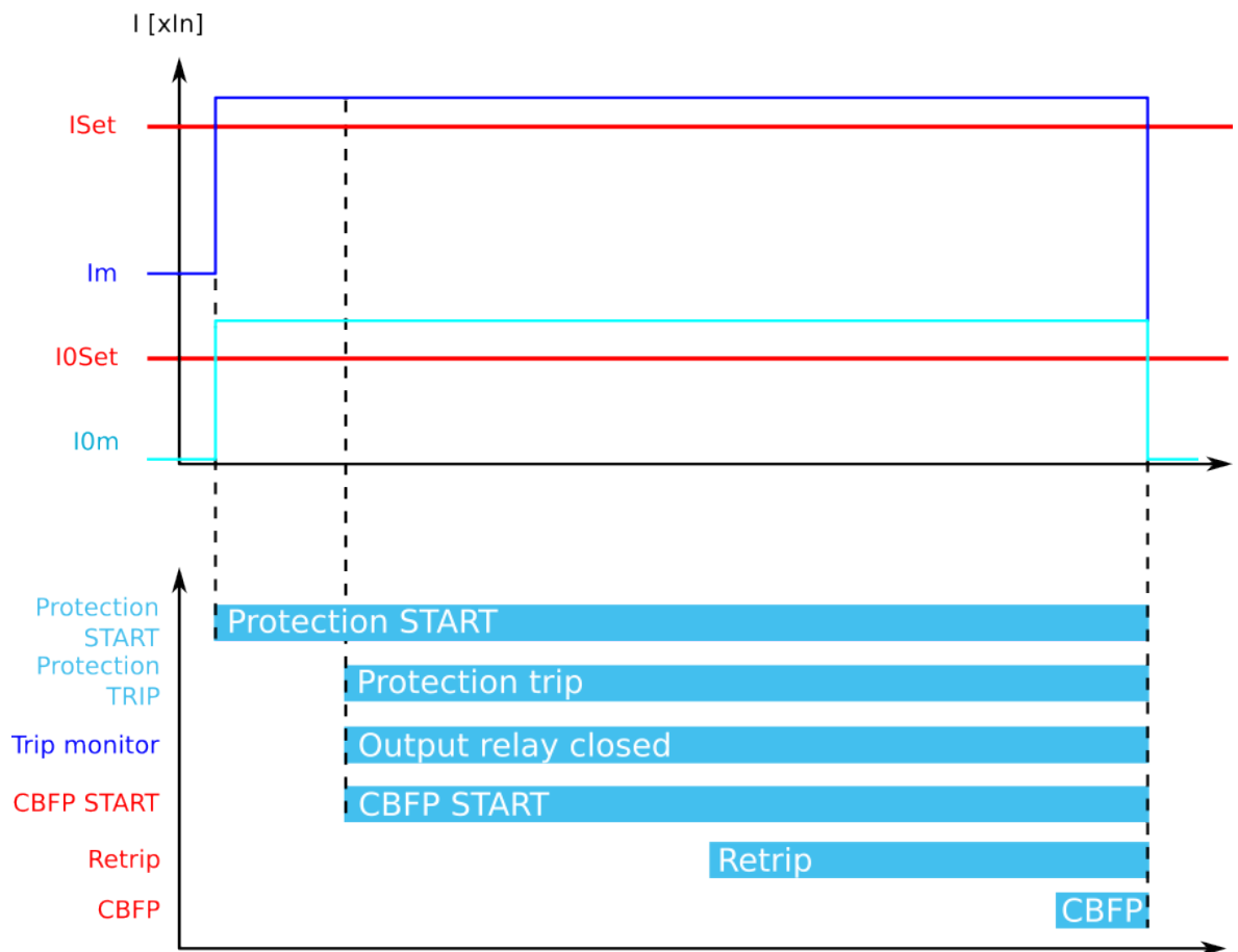
Figure. 5.4.6 - 87. Retrip and CBFP when "Current and DO" is the selected criterion.
