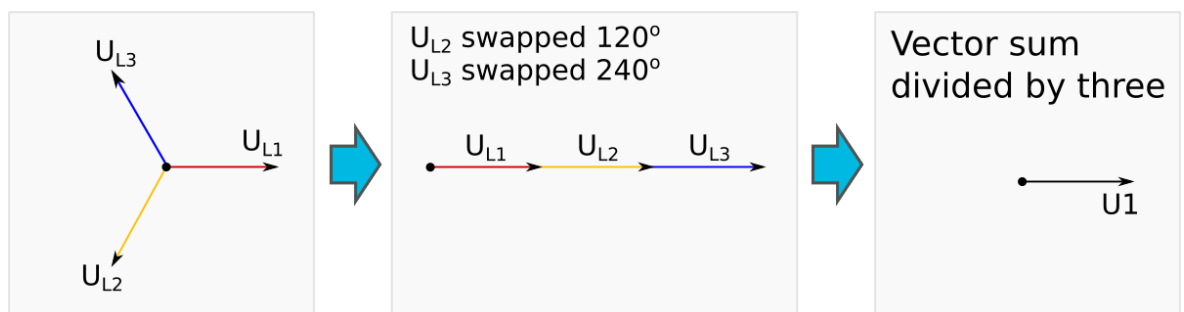
Figure. 5.4.10 - 108. Normal situation.
