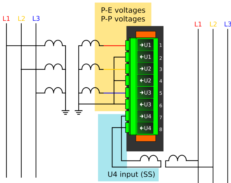
Figure. 5.4.7 - 96. Selectable measurement magnitudes with 3LN+U4 VT connection.
