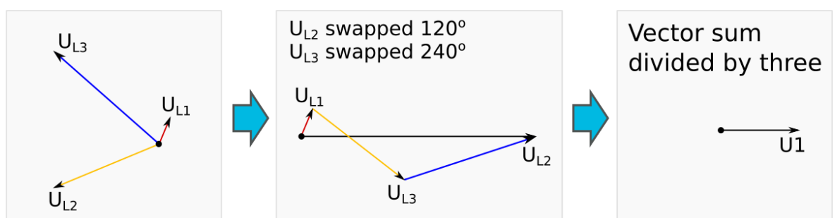
Figure. 5.4.10 - 109. Earth fault in an isolated network.
