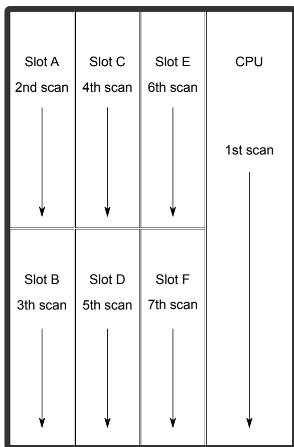
Figure. 8.1 - 179. AQ-X215 hardware scanning and I/O naming principles.
