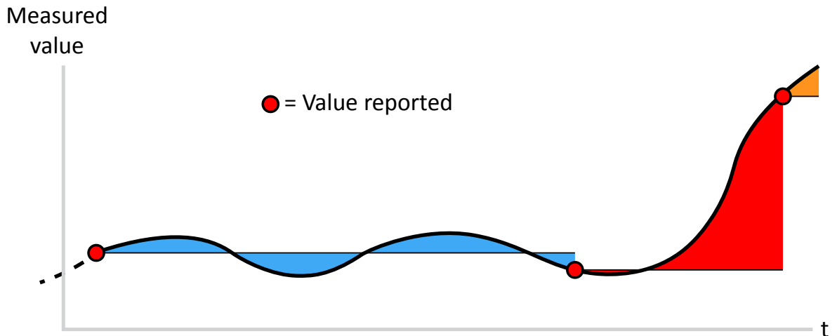
Figure. 6.3.8 - 167. Example graph showing how integration time affects measurement reporting. Small changes take longer to increase the integrated value over the deadband setting (blue area). Big changes meet the deadband criteria faster (red area).
