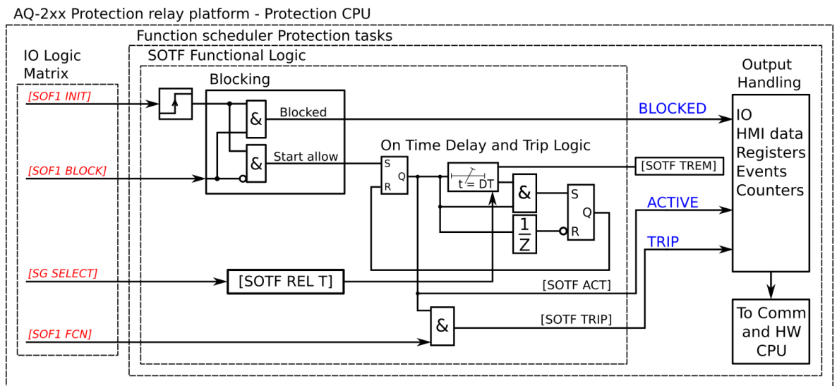
Figure. 5.5.4 - 140. Simplified function block diagram of the switch-on-to-fault function.
