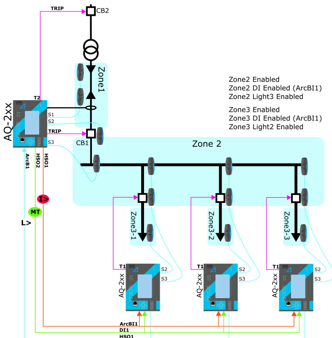
Figure. 5.4.13 - 132. Scheme with AQ-200 protection devices.
