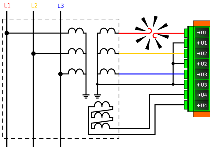
Figure. 5.6.2 - 157. Secondary circuit fault in phase L1 wiring.
