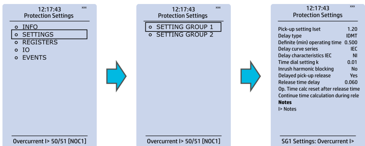
Figure. 4.5 - 12. Settings.
