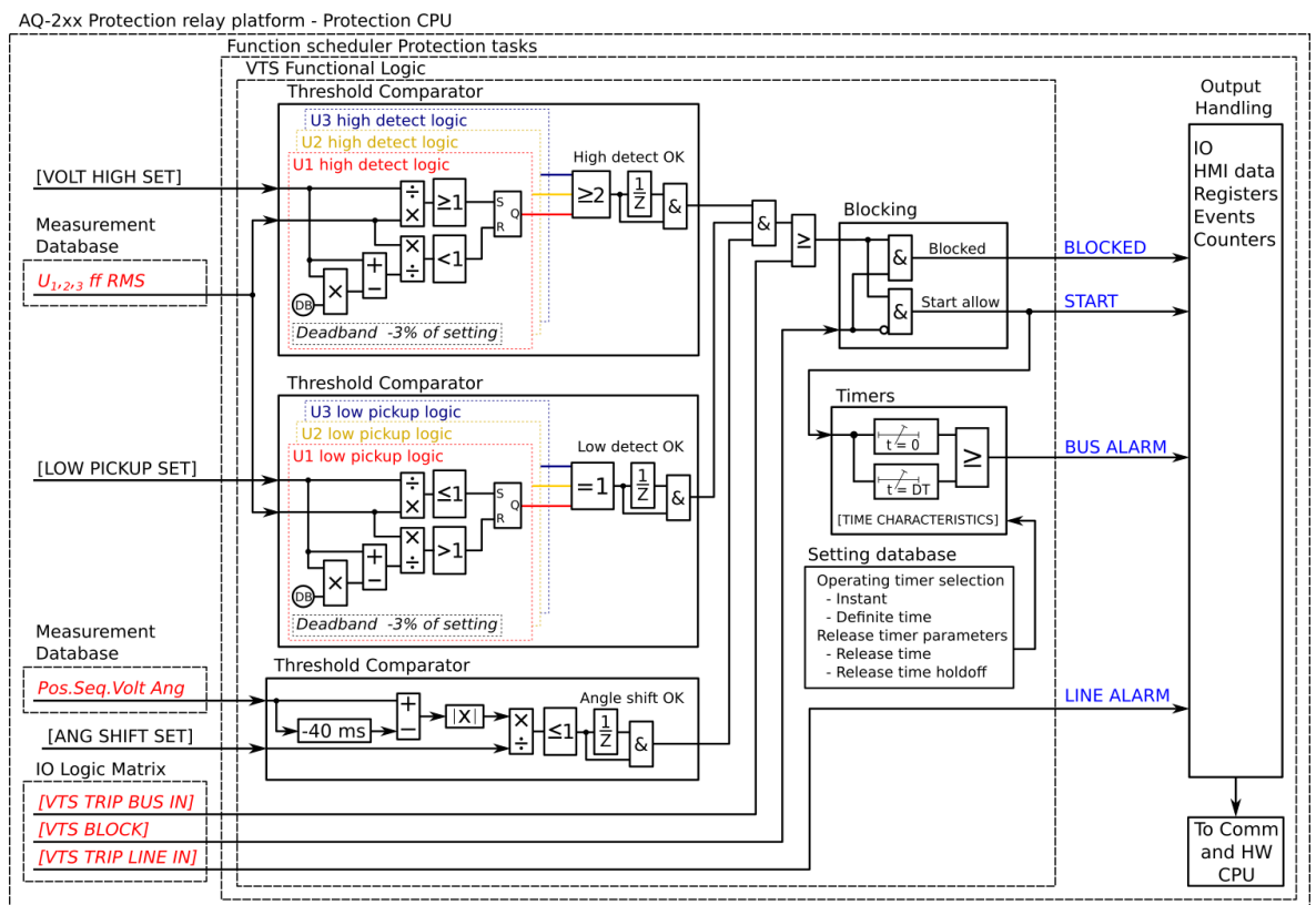
Figure. 5.6.2 - 158. Simplified function block diagram of the VTS function.
