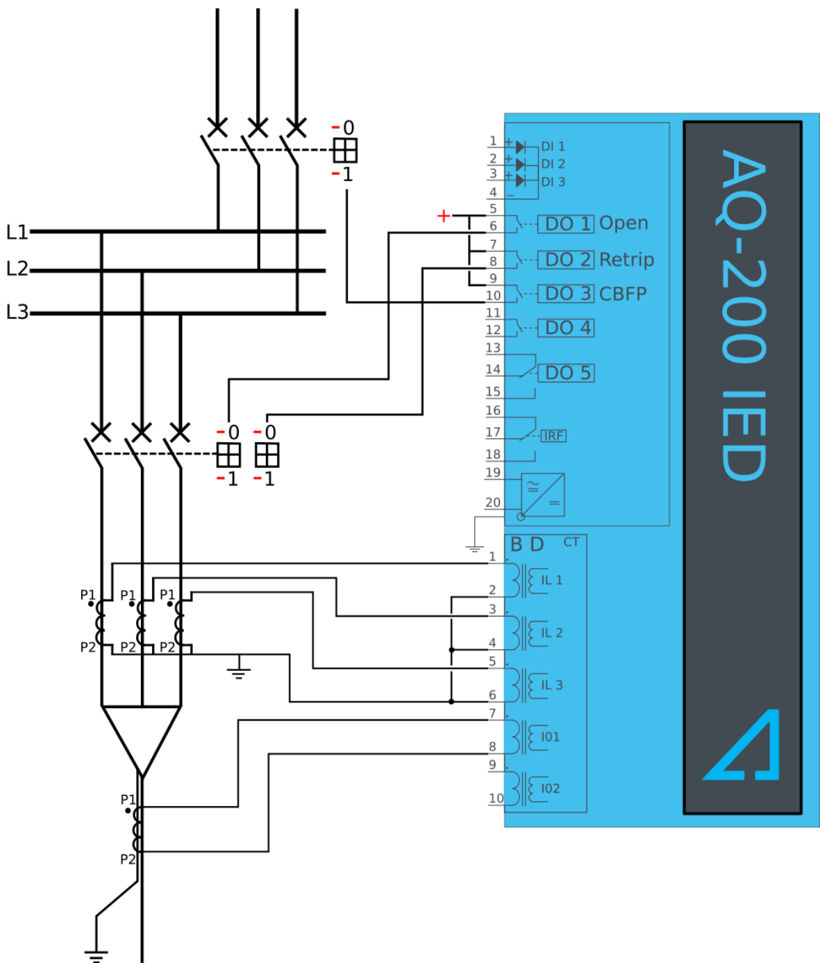
Figure. 5.4.6 - 85. Wiring diagram when Trip, Retrip and CBFP are configured to the device.
