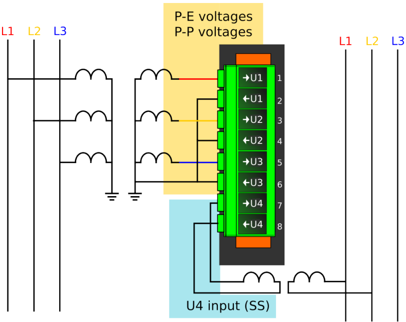
Figure. 5.4.8 - 100. Selectable measurement magnitudes with 3LN+U4 VT connection.
