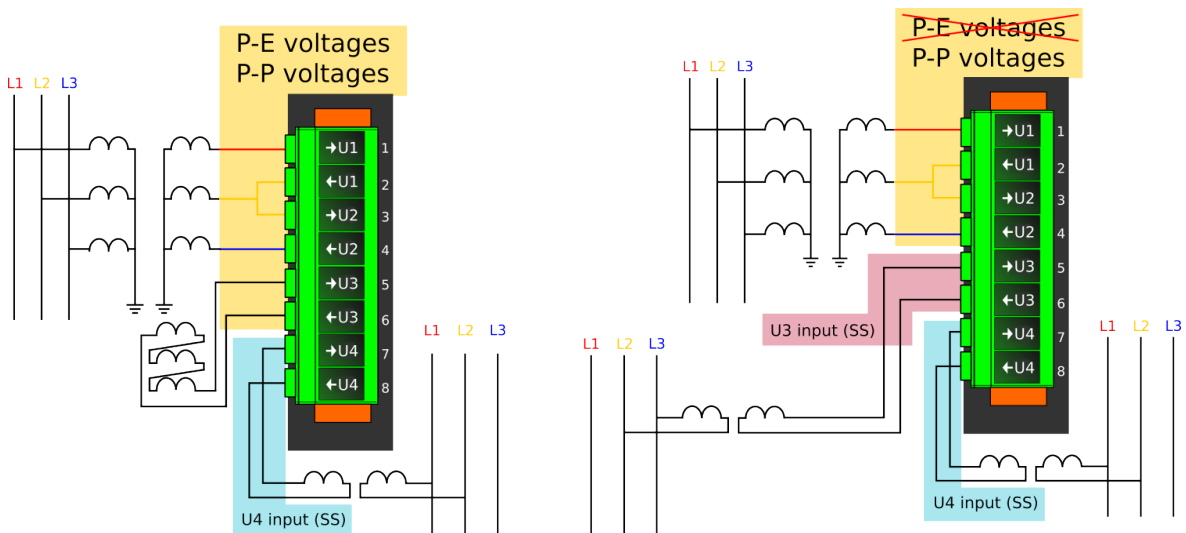
Figure. 5.4.8 - 102. Selectable measurement magnitudes with 2LL+U4 VT connection (P-E voltages not available without residual voltage).
