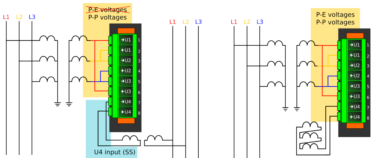
Figure. 5.4.7 - 97. Selectable measurement magnitudes with 3LL+U4 VT connection (P-E voltages not available without residual voltage).
