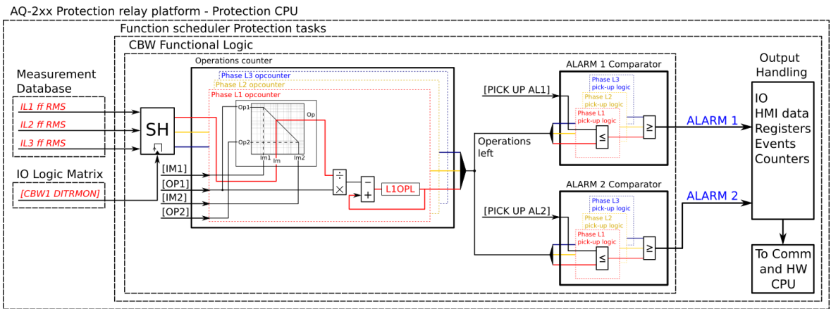
Figure. 5.6.3 - 160. Simplified function block diagram of the circuit breaker wear function.
