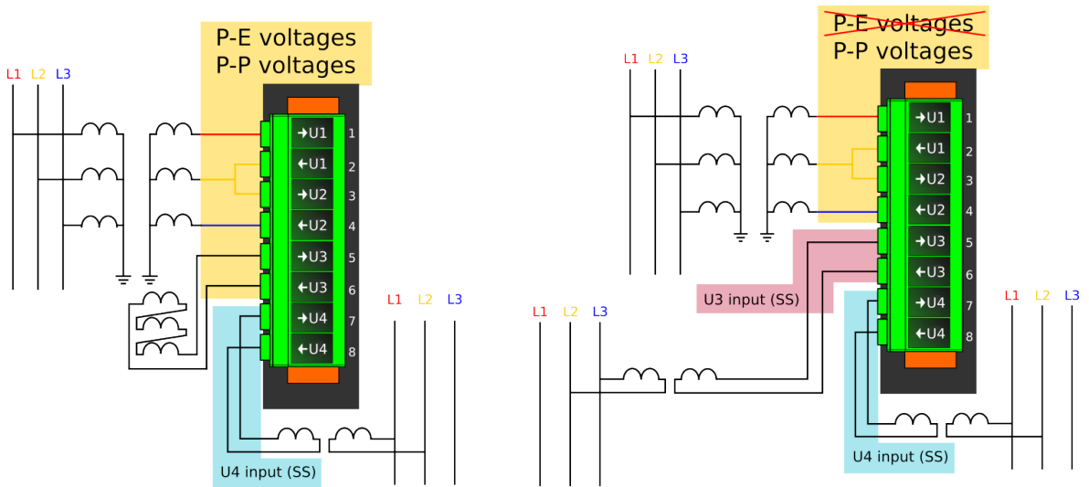
Figure. 5.4.7 - 98. Selectable measurement magnitudes with 2LL+U3+U4 VT connection (P-E voltages not available without residual voltage).
