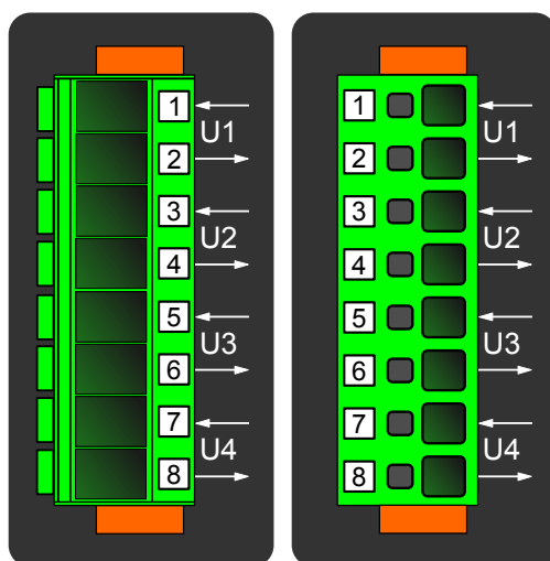
Figure. 8.4 - 182. Voltage measurement module can be equipped with standard screw terminals or spring cage terminals for connection.
