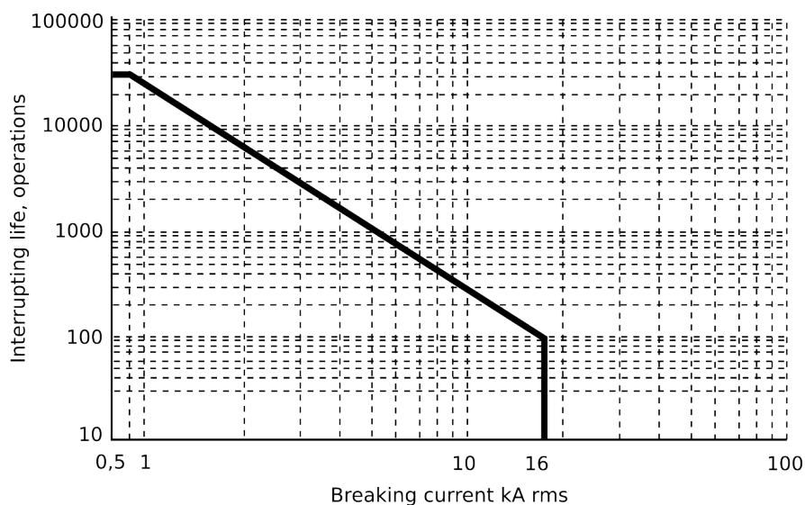
Figure. 5.6.3 - 159. Example of the circuit breaker interrupting life operations.
