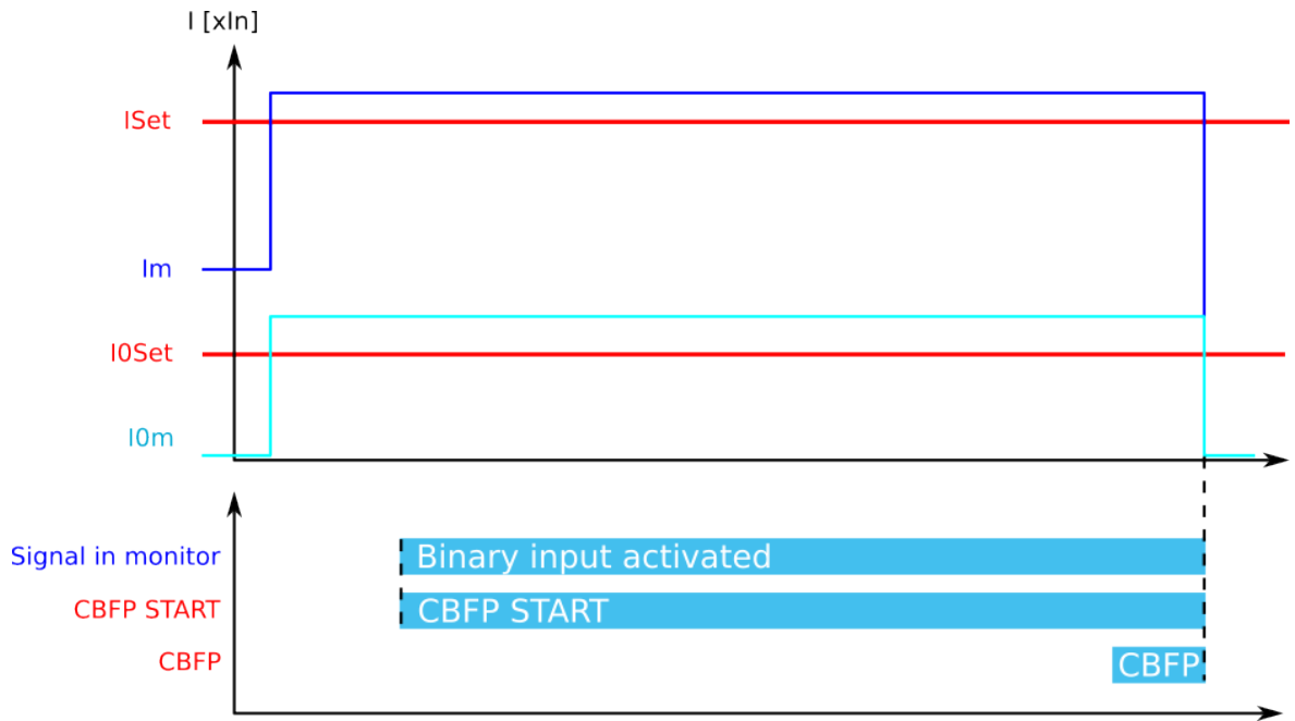
Figure. 5.4.6 - 94. Dedicated CBFP operation from digital input signal.
