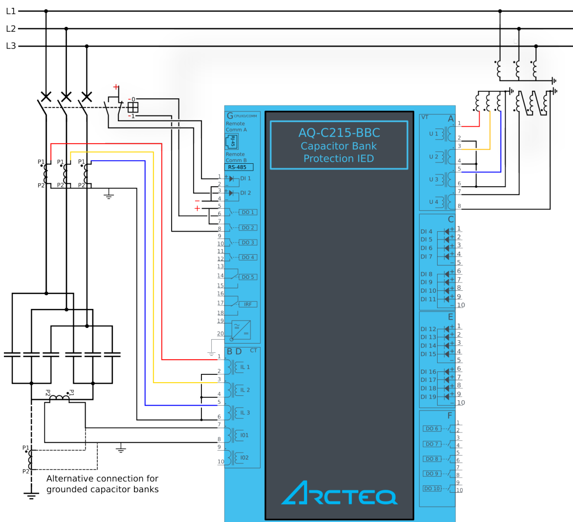
Figure. 7.2.1 - 172. Application example and its connections in double wye bank.
