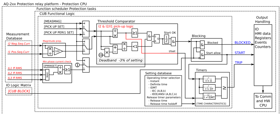
Figure. 5.4.4 - 81. Simplified function block diagram of the I2> function.
