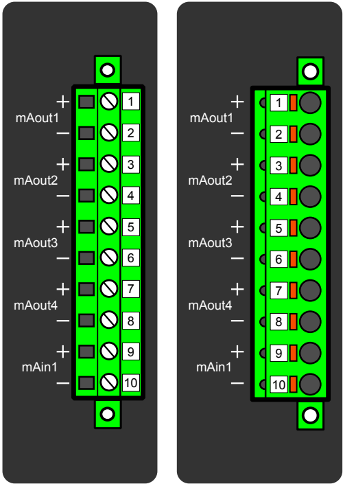
Figure. 8.5.9 - 194. Milliampere output (mA) I/O module connections. Can be equipped with standard screw terminals or spring cage terminals for connection.
