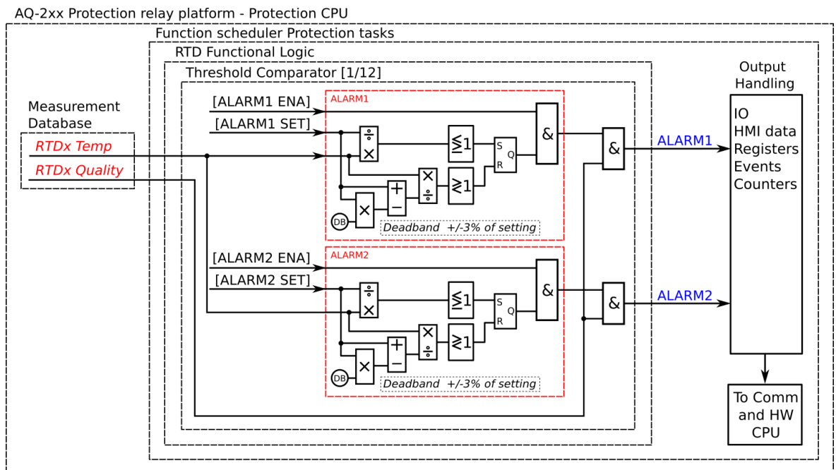
Figure. 5.4.12 - 129. Simplified function block diagram of the resistance temperature detection function.
