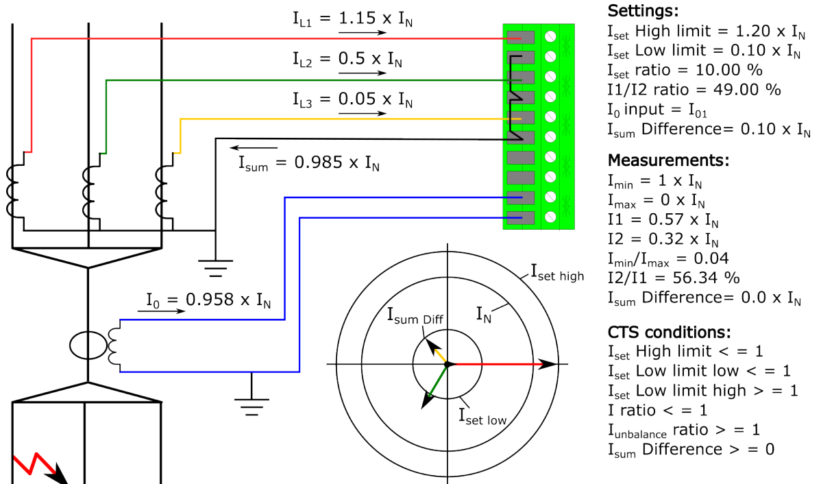
Figure. 5.6.1 - 156. Primary side high-impedance earth fault.
