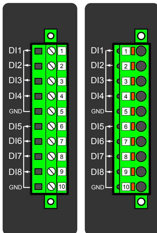
Figure. 8.5.1 - 183. Digital input module (DI8) with eight add-on digital inputs. Can be equipped with standard screw terminals or spring cage terminals for connection.
