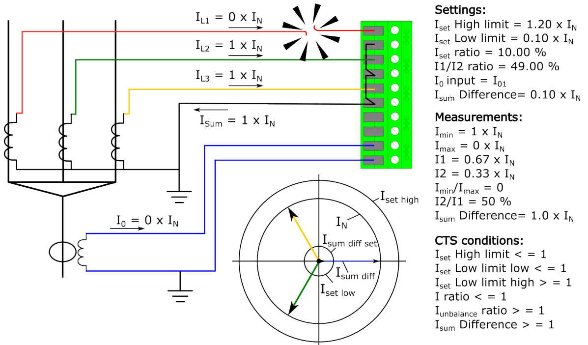
Figure. 5.6.1 - 154. Broken secondary phase current wiring.
