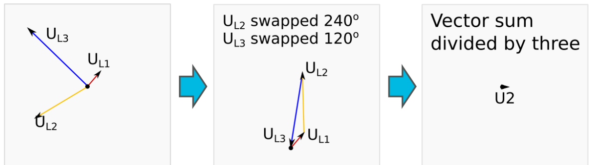
Figure. 5.4.10 - 112. Earth fault in isolated network.
