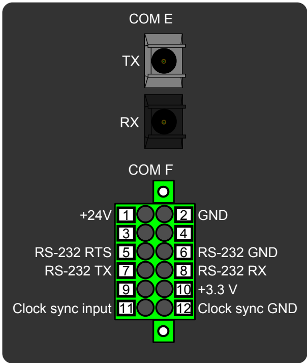
Figure. 8.5.5 - 189. Serial RS-232 module connectors.
