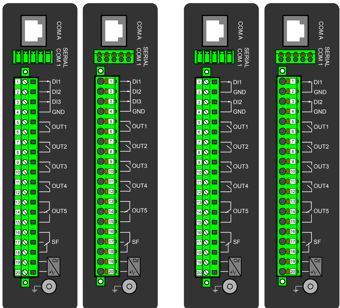
Figure. 8.2 - 180. CPU module variants are available with either two or three digital inputs, and can be equipped with standard screw terminals or spring cage terminals for connection.
