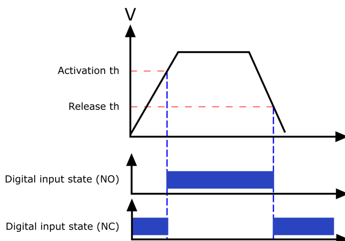
Figure. 8.5.1 - 184. Digital input state when energizing and de-energizing the digital input channels.
