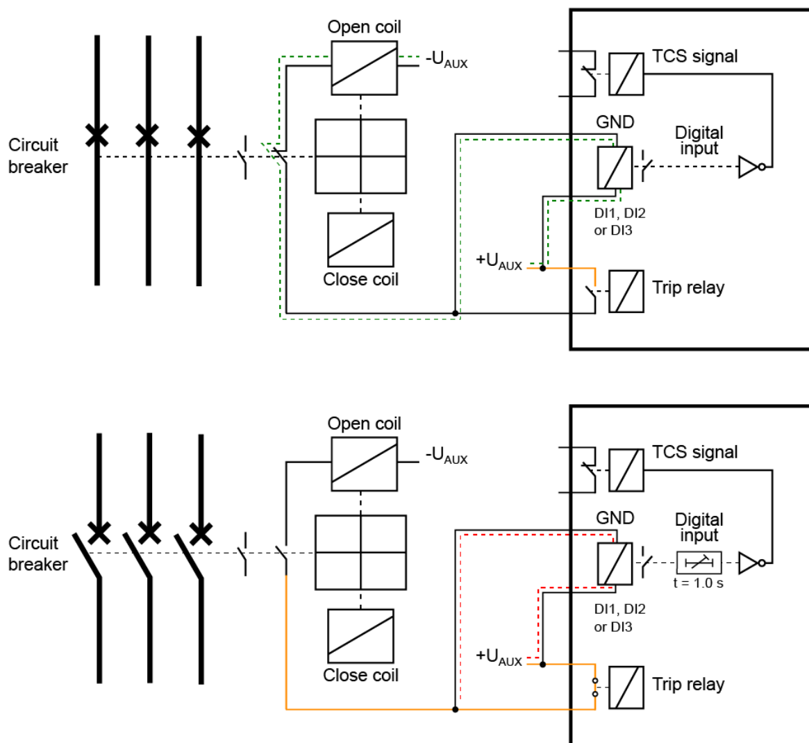
Figure. 7.2.3 - 176. Trip circuit supervision with one DI and one latched output contact.
