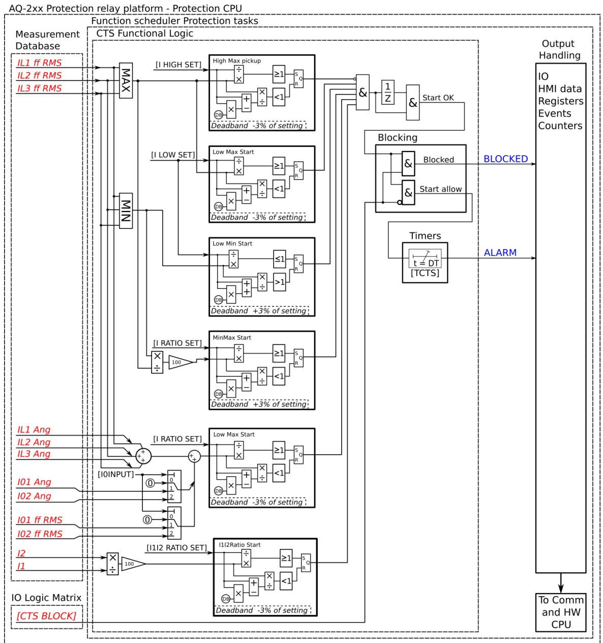
Figure. 5.6.1 - 147. Simplified function block diagram of the CTS function.
