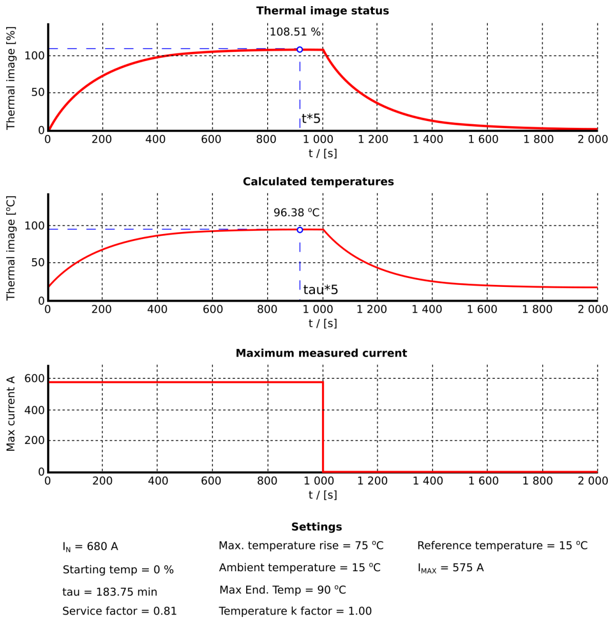
Figure. 5.4.11 - 126. Thermal image response with nominal currents and fine-tuned k_{SF} correction factor.
