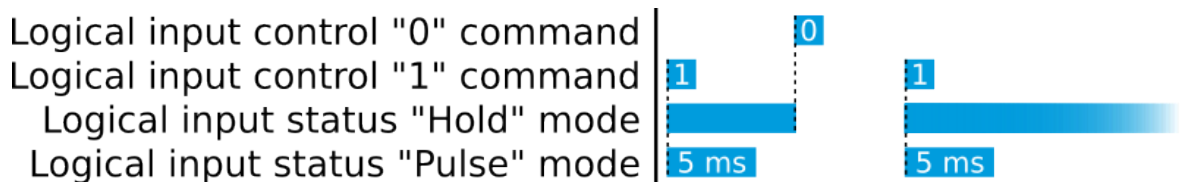
Figure. 5.5.9 - 144. Operation of logical input in "Hold" and "Pulse" modes.
