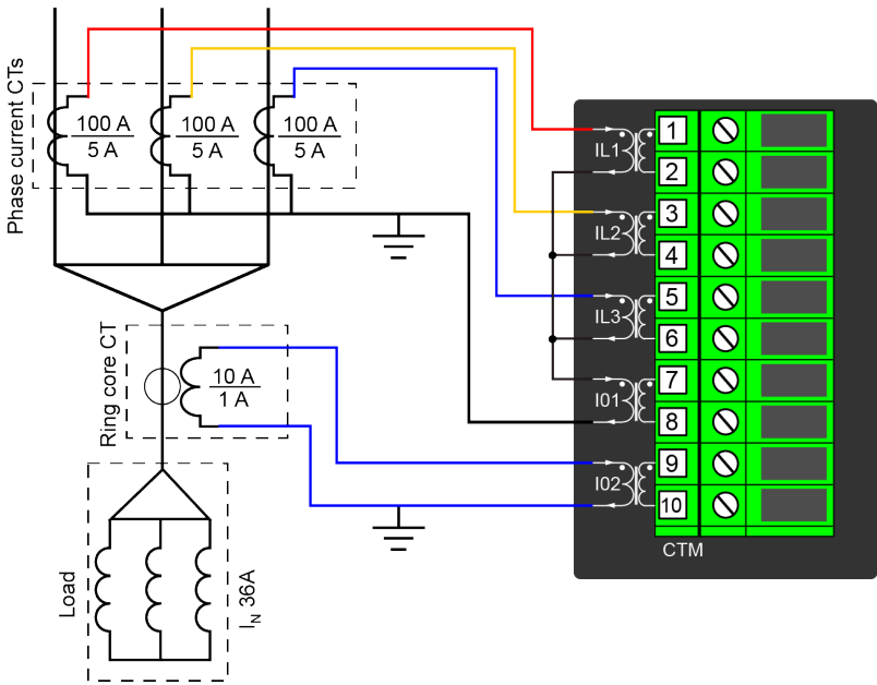
Figure. 5.2.1 - 58. Connections.
