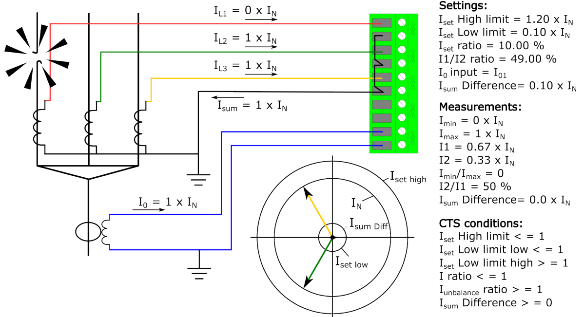
Figure. 5.6.1 - 155. Broken primary phase current wiring.
