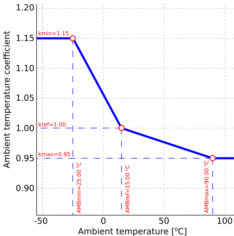
Figure. 5.4.11 - 117. Ambient temperature coefficient calculation (a three-point linear approximation and a settable correction curve).
