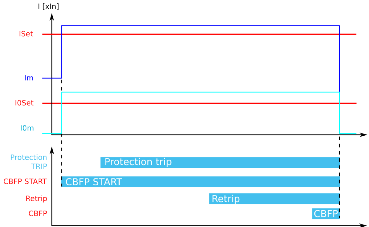
Figure. 5.4.6 - 86. Retrip and CBFP when "Current" is the selected criterion.
