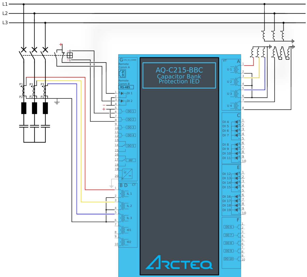
Figure. 7.2.1 - 171. Application example and its connections.
