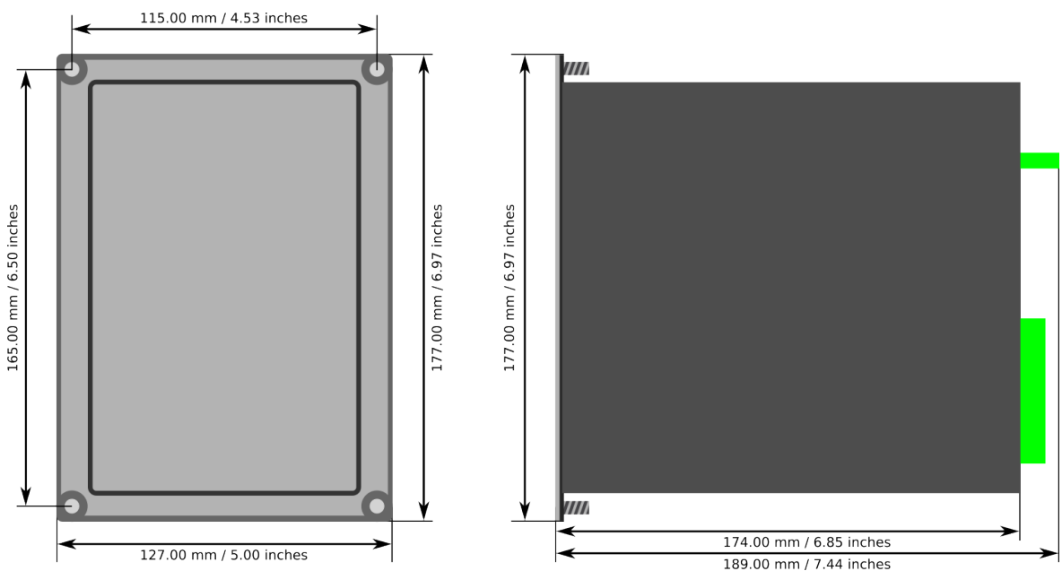
Figure. 8.6 - 195. Device dimensions.
