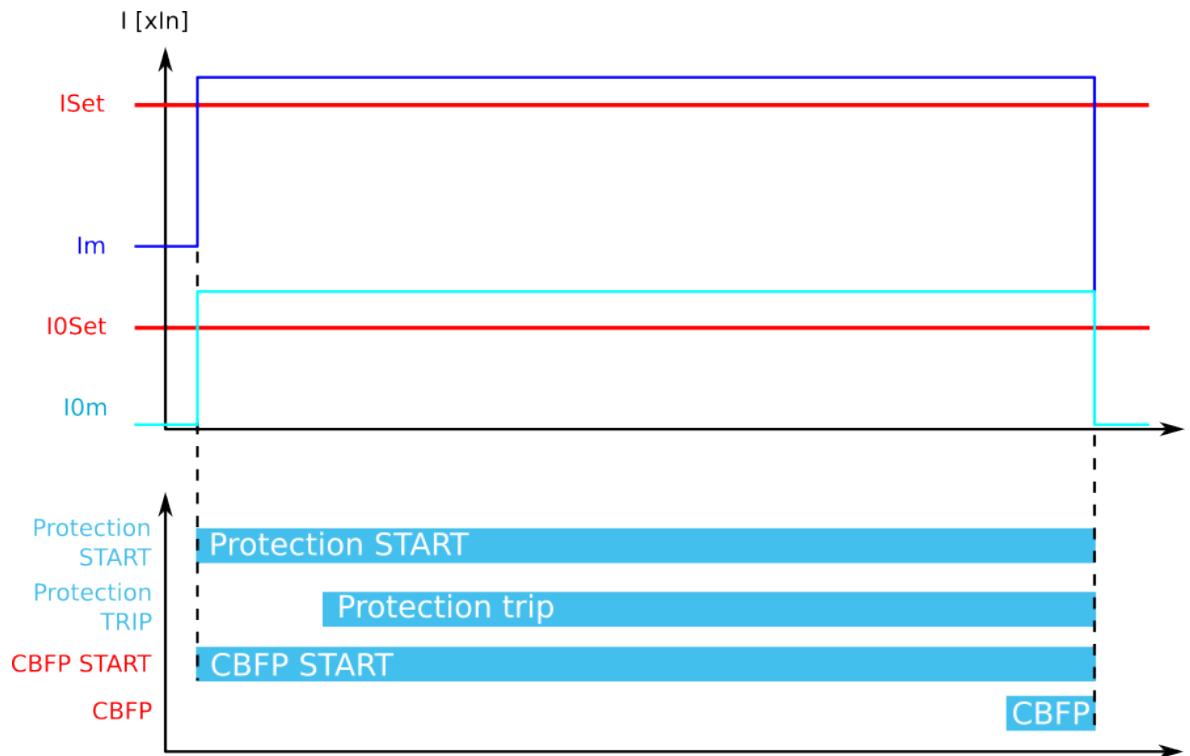
Figure. 5.4.6 - 90. CBFP when "Current" is the selected criterion.
