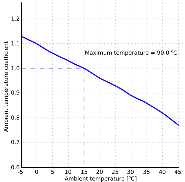
Figure. 5.4.11 - 120. Set correction curve for ambient temperature.
