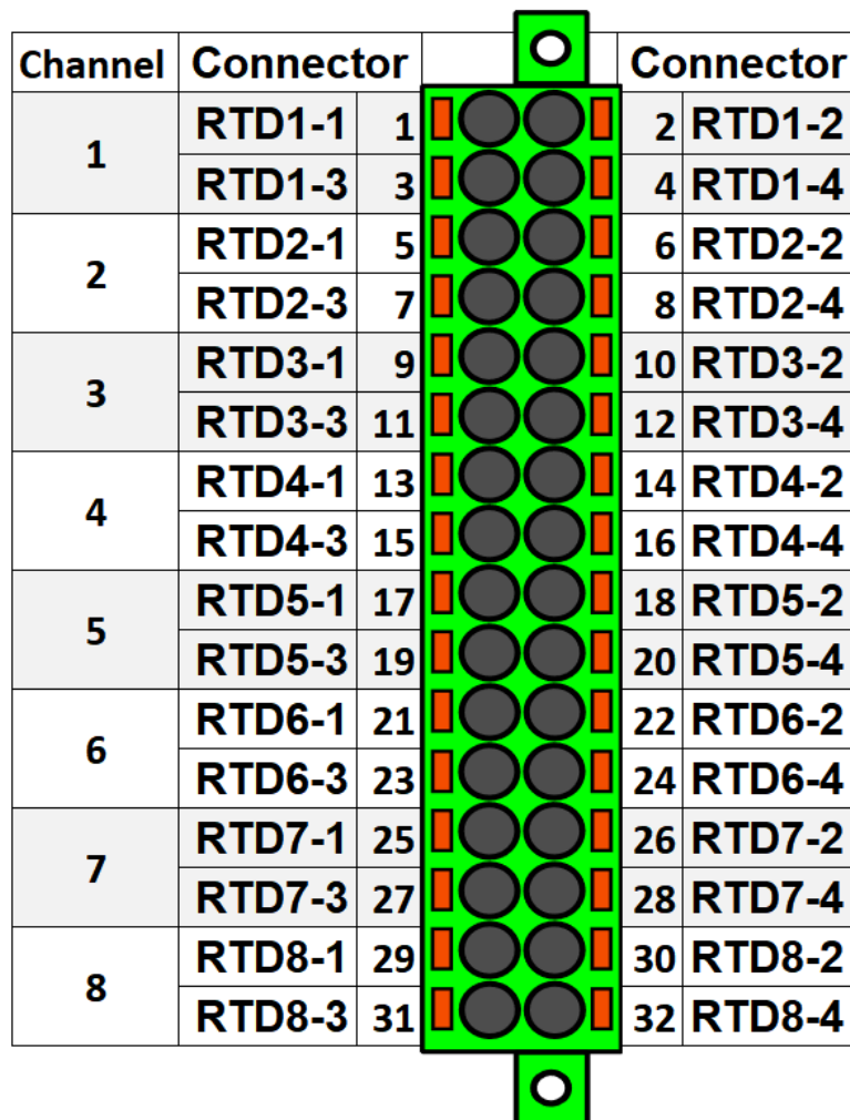
Figure. 8.5.4 - 187. RTD input module connectors.
