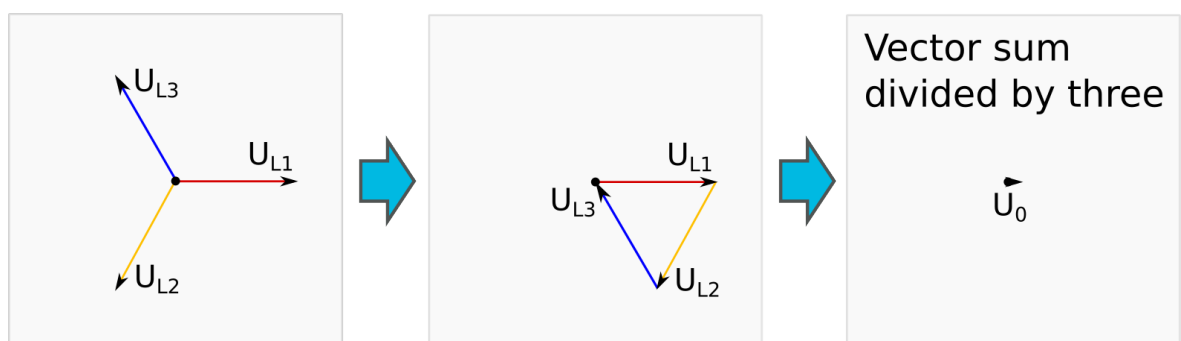
Figure. 5.4.9 - 104. Normal situation.
