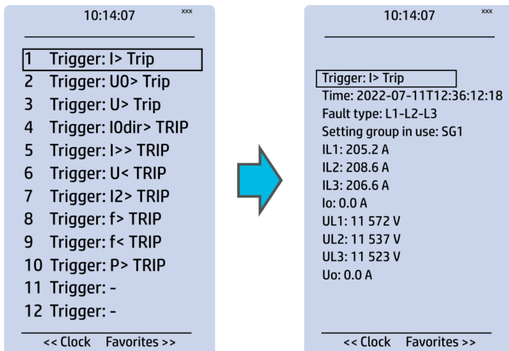
Figure. 5.6.8 - 165. 12 latest recordings can be accessed from HMI if "Fault registers" view has been enabled in "Carousel designer" tool.
