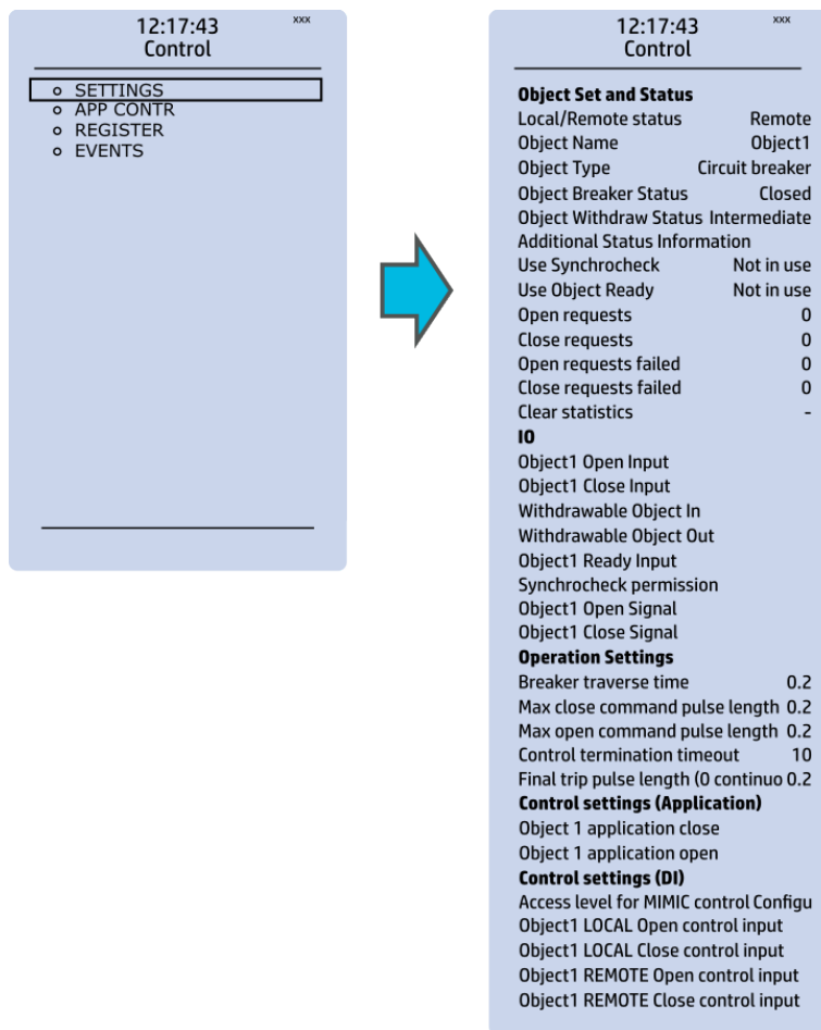
Figure. 4.6 - 21. Settings section.
