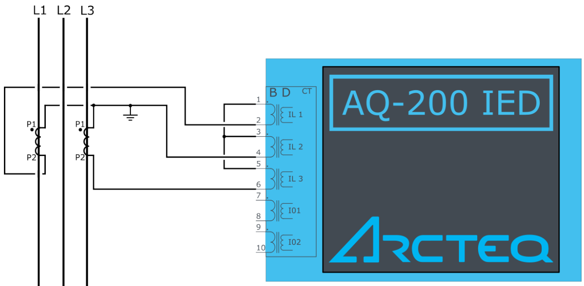
Figure. 7.2.2 - 173. ARON connection.
