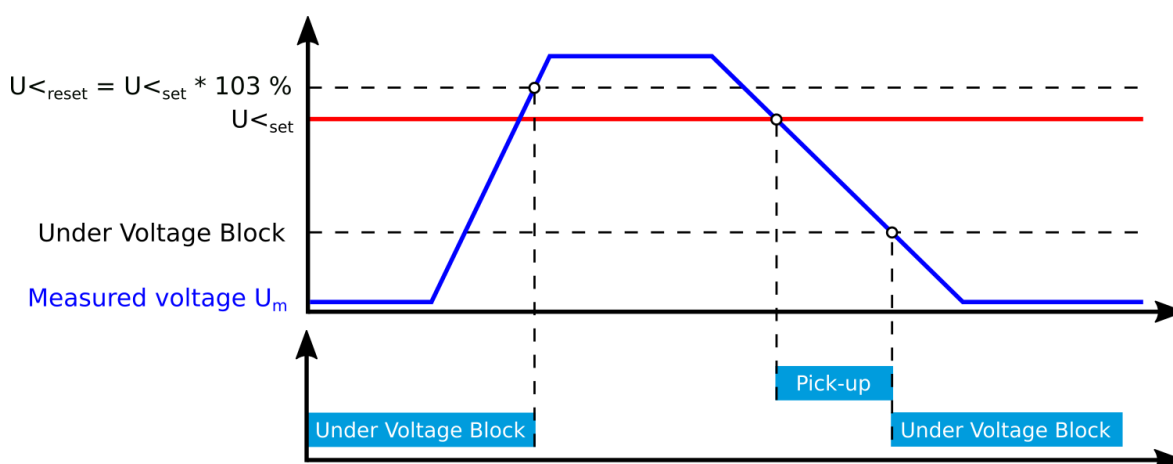
Figure. 5.4.10 - 115. Example of the block setting operation.
