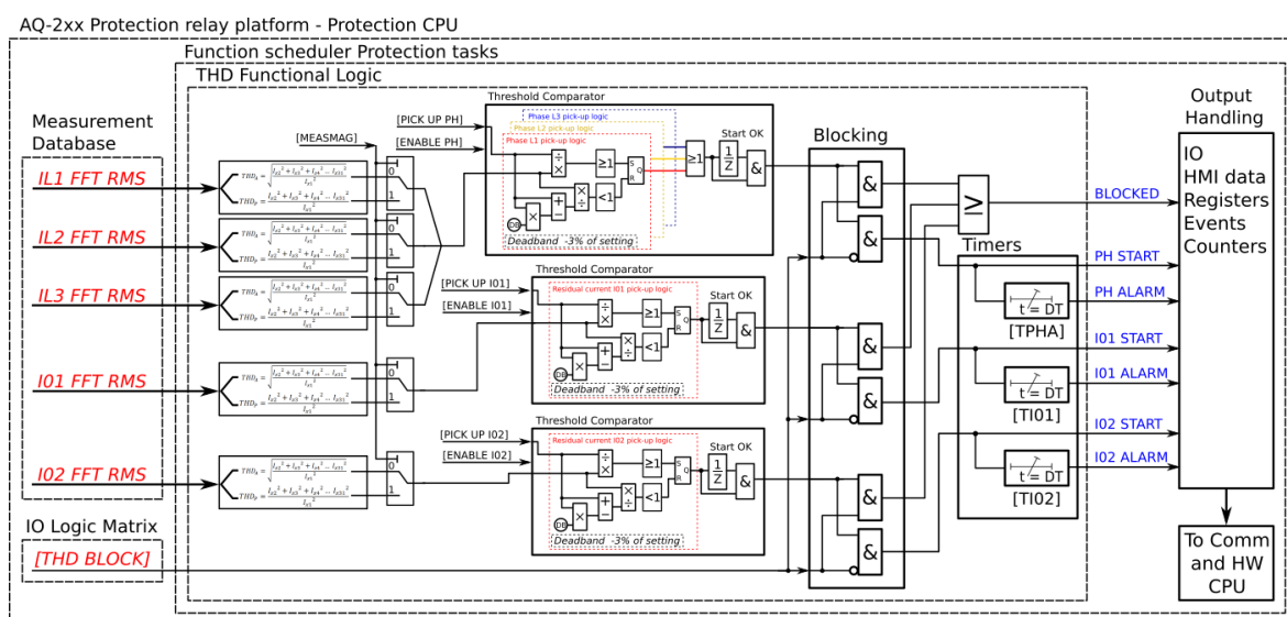
Figure. 5.6.4 - 162. Simplified function block diagram of the total harmonic distortion monitor function.
