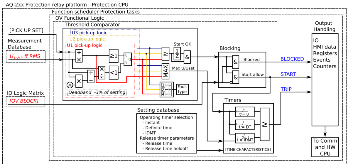
Figure. 5.4.7 - 95. Simplified function block diagram of the U> function.
