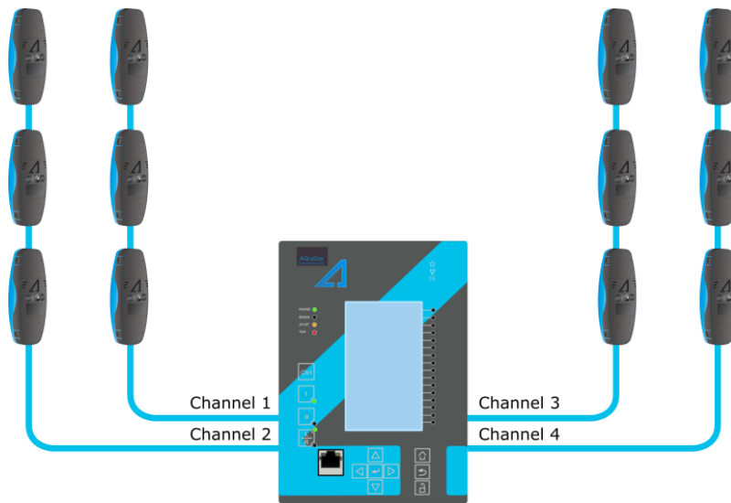
Figure. 5.4.13 - 130. Protection device equipped with arc protection.
