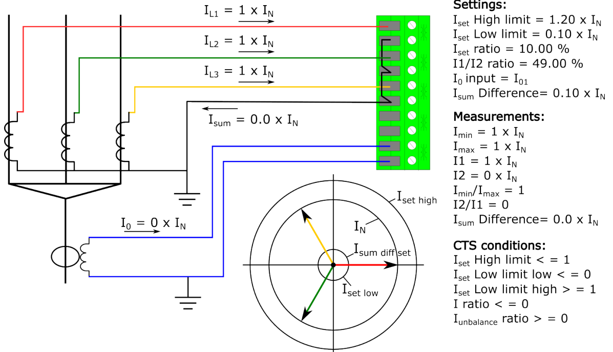
Figure. 5.6.1 - 153. Normal situation, residual current also measured.
