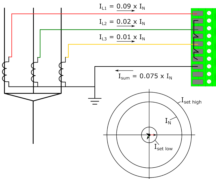
Figure. 5.6.1 - 152. Low current and heavy unbalance.
