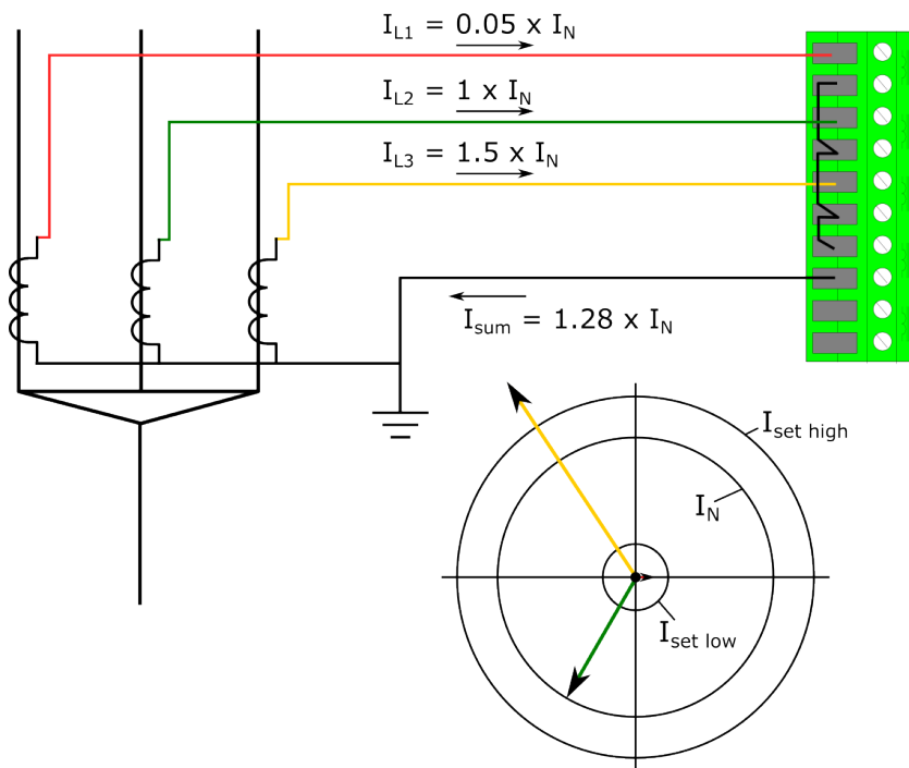
Figure. 5.6.1 - 151. No wiring fault but heavy unbalance.
