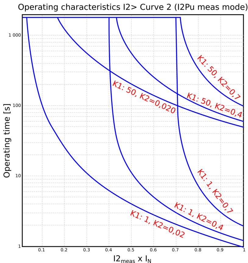
Figure. 5.4.4 - 82. Operation characteristics curve for I2&gt; Curve2.
