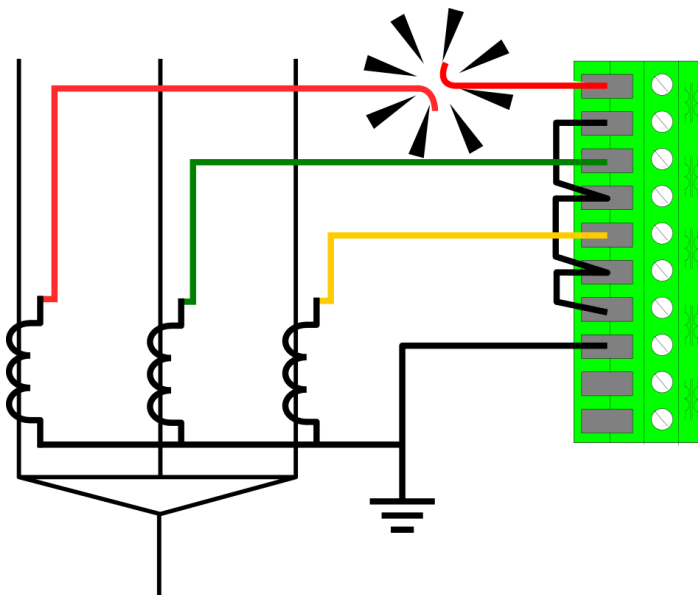
Figure. 5.6.1 - 146. Secondary circuit fault in phase L1 wiring.
