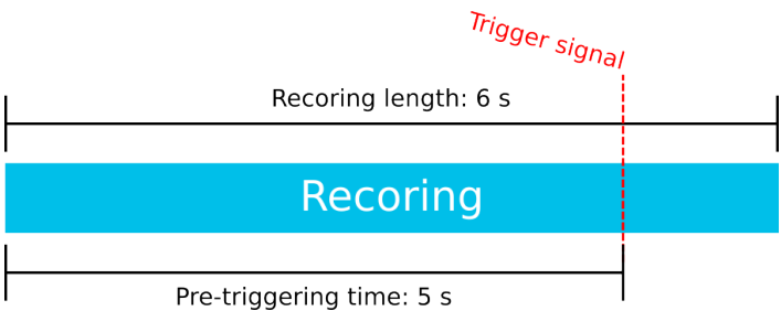
Figure. 5.6.5 - 164. Effects of recording length and pre-triggering time signals. This example is based on the settings shown above.
