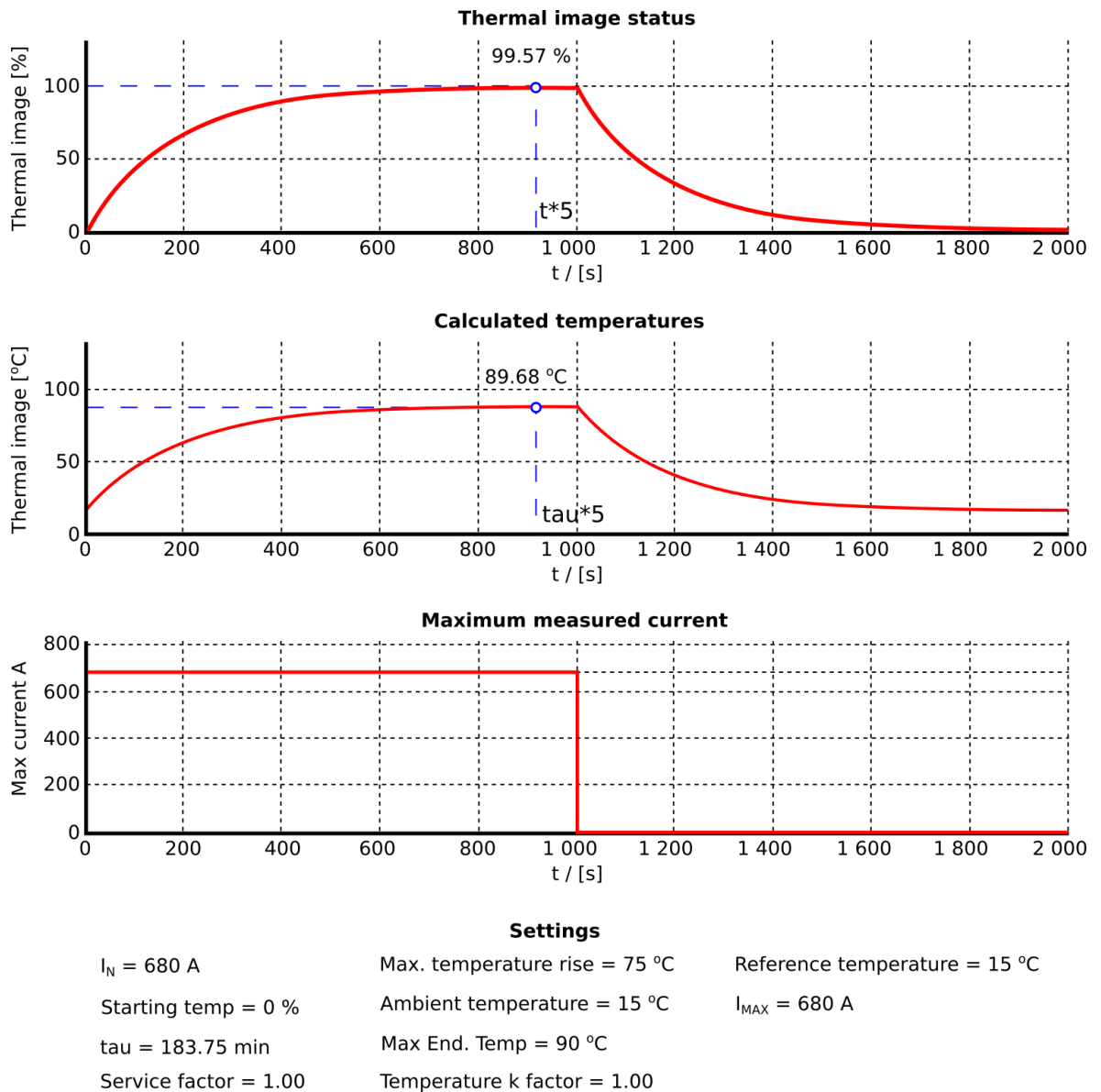
Figure. 5.4.11 - 125. Thermal image response with maximum load (installation according to presumptions).
