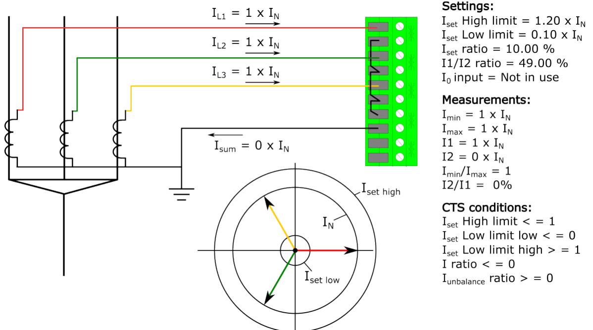
Figure. 5.6.1 - 148. All works properly, no faults.
