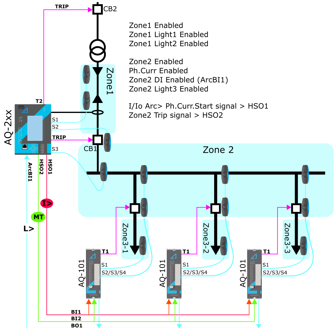
Figure. 5.4.13 - 131. Scheme with AQ-101 arc protection relays.
