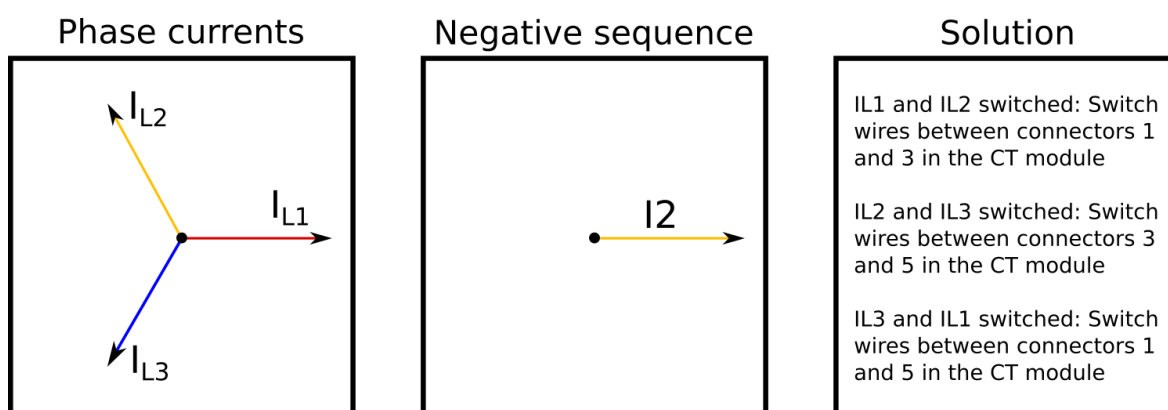
Figure. 5.2.1 - 67. Common network rotation (mixed phases) problems.
