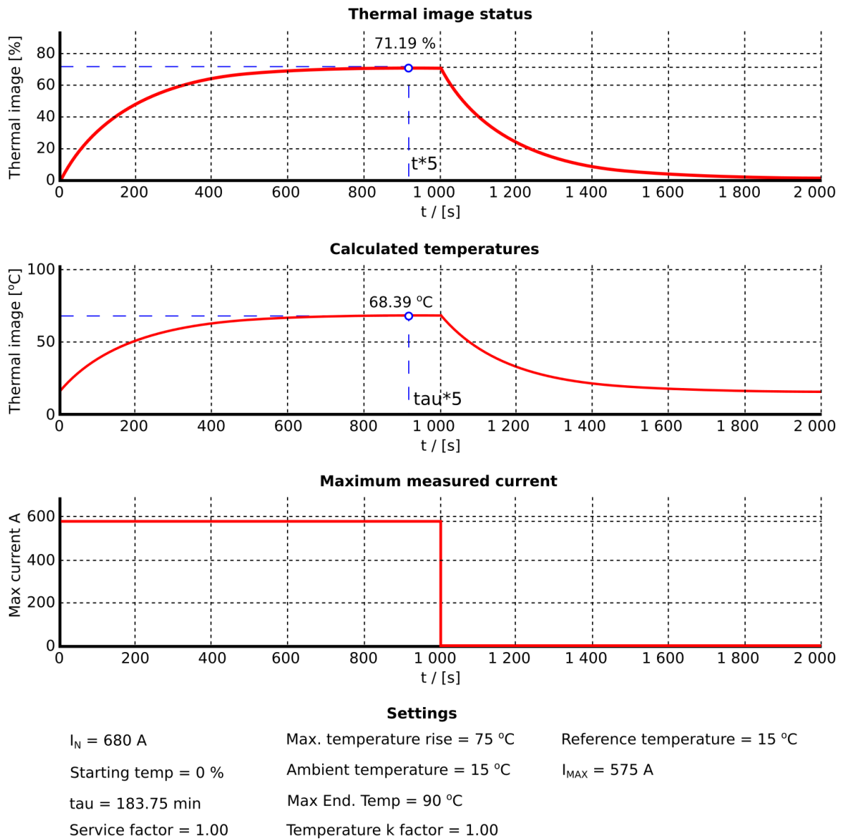
Figure. 5.4.11 - 124. Thermal image response with nominal load (installation according to presumptions).
