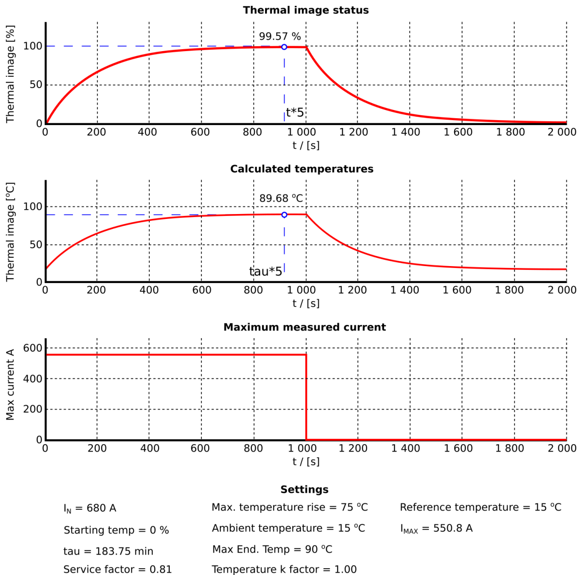
Figure. 5.4.11 - 127. Thermal response with k sf factor correctly set.
