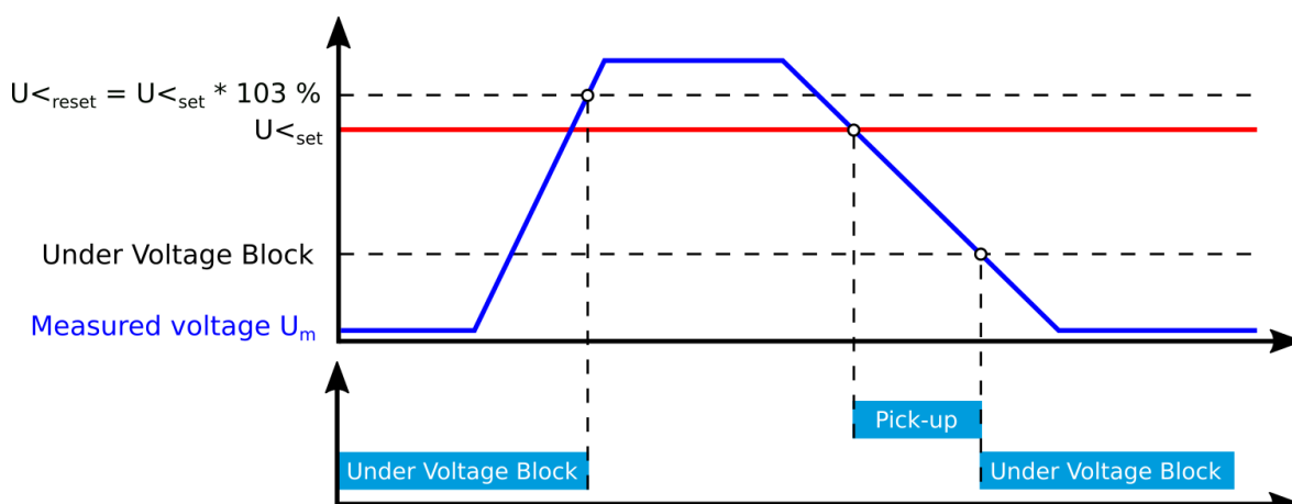
Figure. 5.4.8 - 103. Example of the block setting operation.
