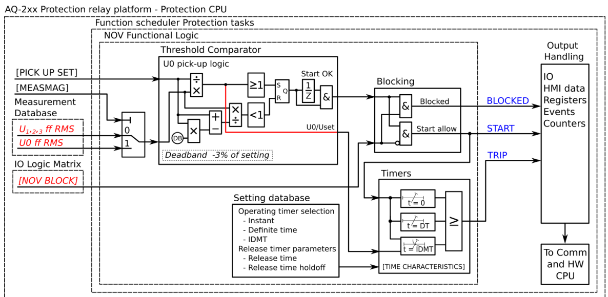
Figure. 5.4.9 - 107. Simplified function block diagram of the U0> function.
