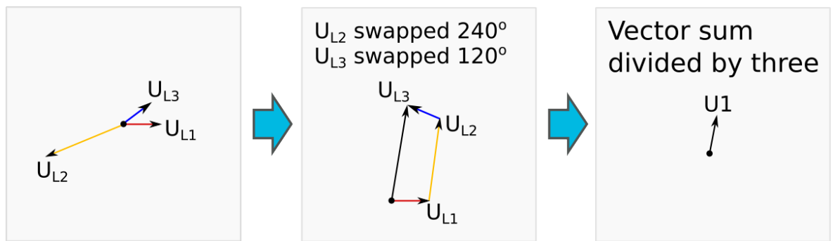
Figure. 5.4.10 - 113. Close-distance short-circuit between phases 1 and 3.
