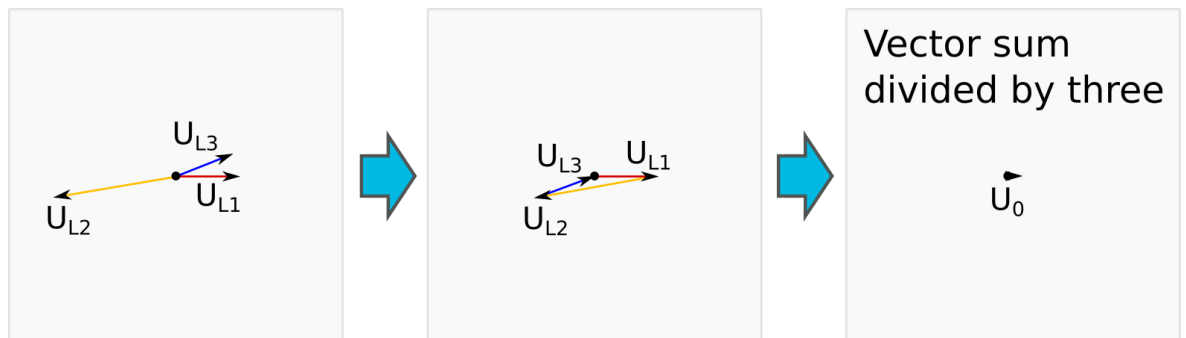
Figure. 5.4.9 - 106. Close-distance short-circuit between phases 1 and 3.
