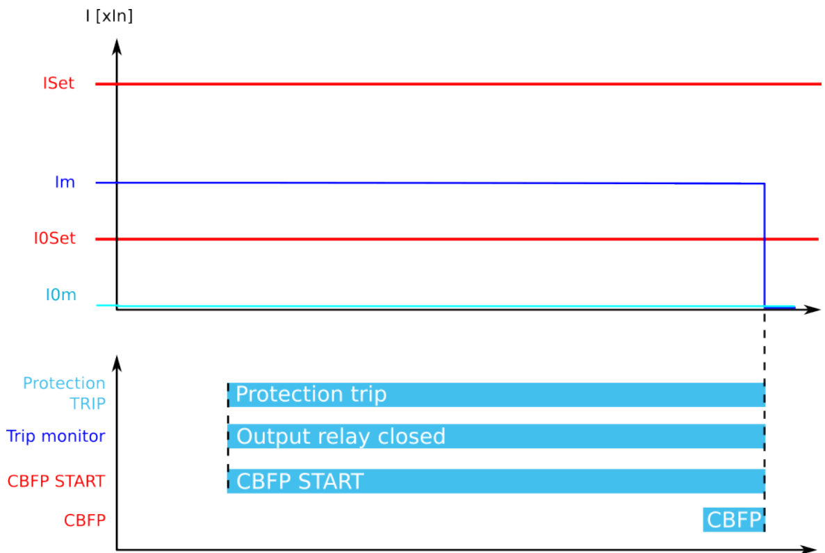
Figure. 5.4.6 - 92. CBFP when "Current or DO" is the selected criterion.
