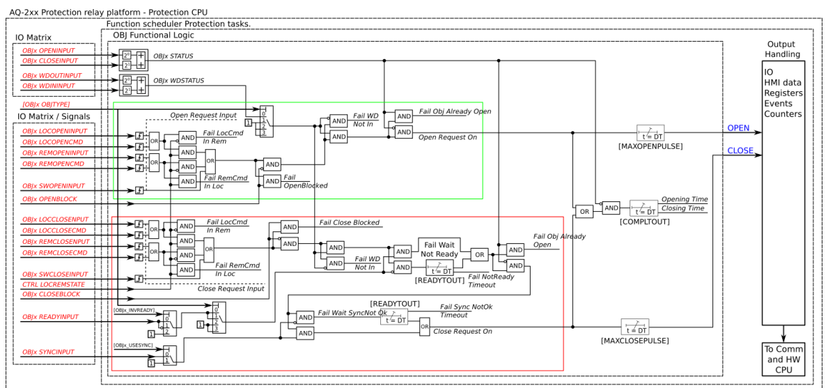
Figure. 5.5.2 - 139. Simplified function block diagram of the object control and monitoring function.
