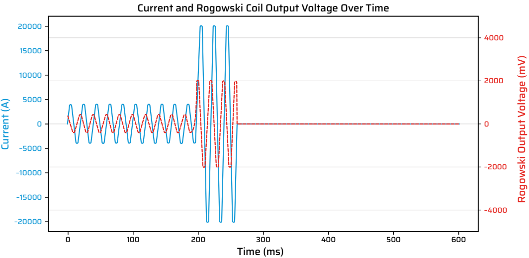
Simulated oscillograph of Rogowski sensor's current-to-voltage ratio from pre-fault state and through the fault to the main incomer trip. The graph shows that Rogowski sensor performs accurately in all conditions as it does not saturate.
