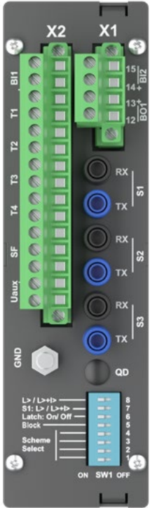
AQ-102LV rear view
