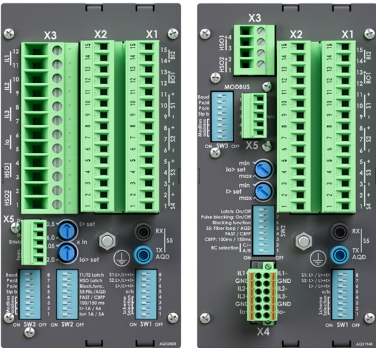
Rear of AQ-110PLV with CT inputs and Modbus connector.
