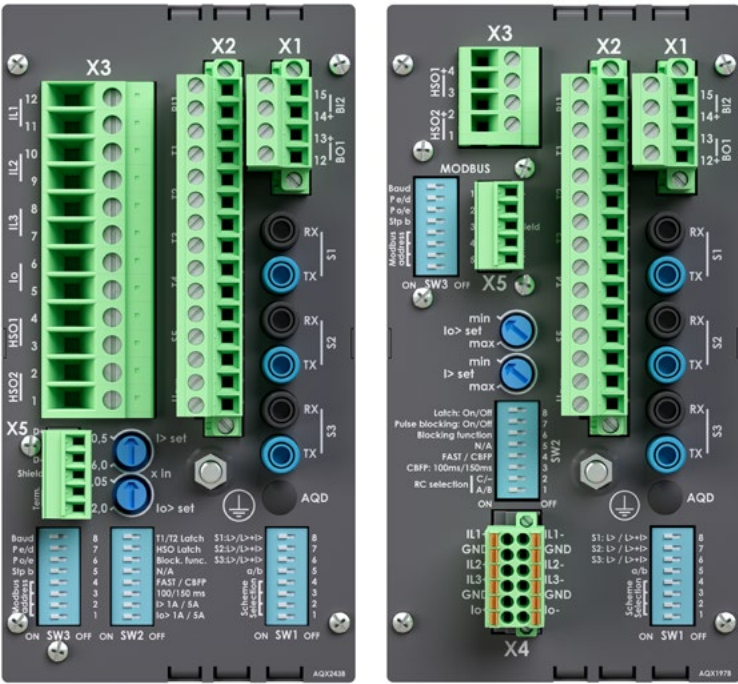
Rear of AQ-110FLV with CT inputs and Modbus connector.
