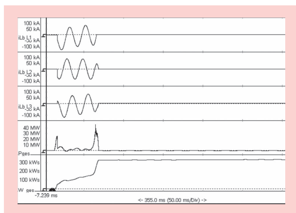
FIGURE 7. A 65-kA arc test with AQD engaged followed by the CB opening (refer to Figure 11).
