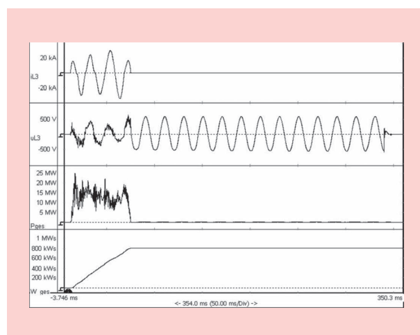
FIGURE 9. A 20-kA arc test with arc flash detection and CB opening approximately three cycles (refer to Figure 11).
