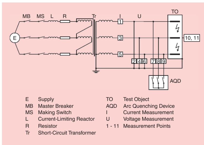
FIGURE 11. The AQD system test configuration.
