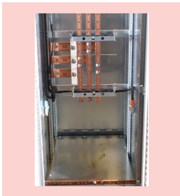
FIGURE 12. The cabinet after the 63 kA test after AQD engaged.
