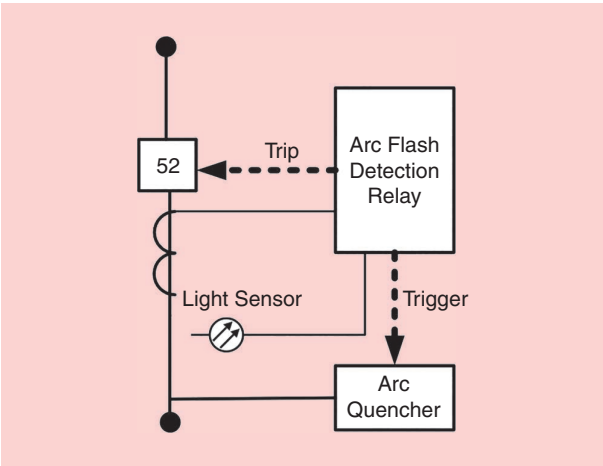
FIGURE 2. The arc detection relay with a light and current-based quenching system.
