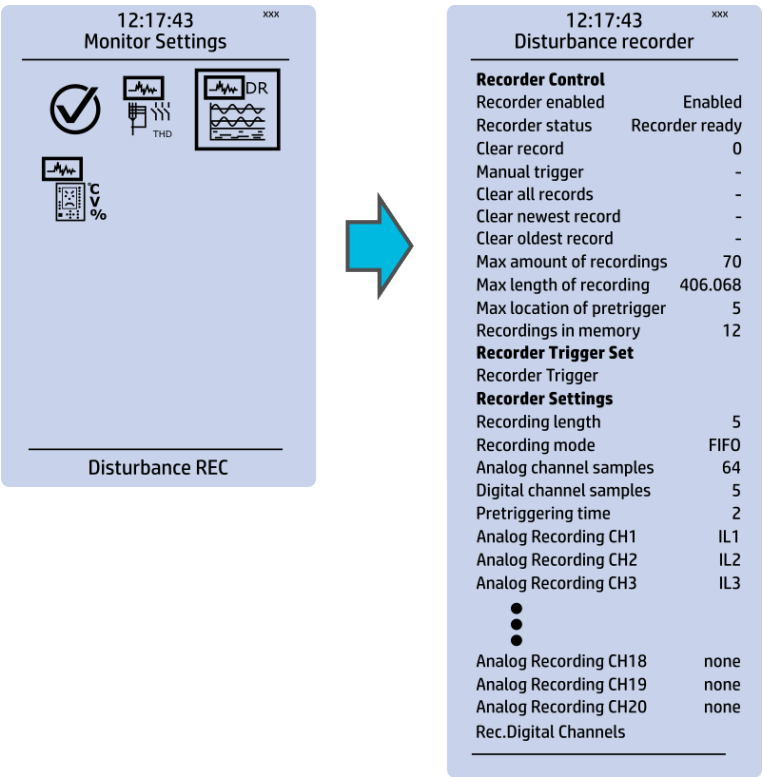
Figure. 3.6 - 36. Disturbance recorder settings.
