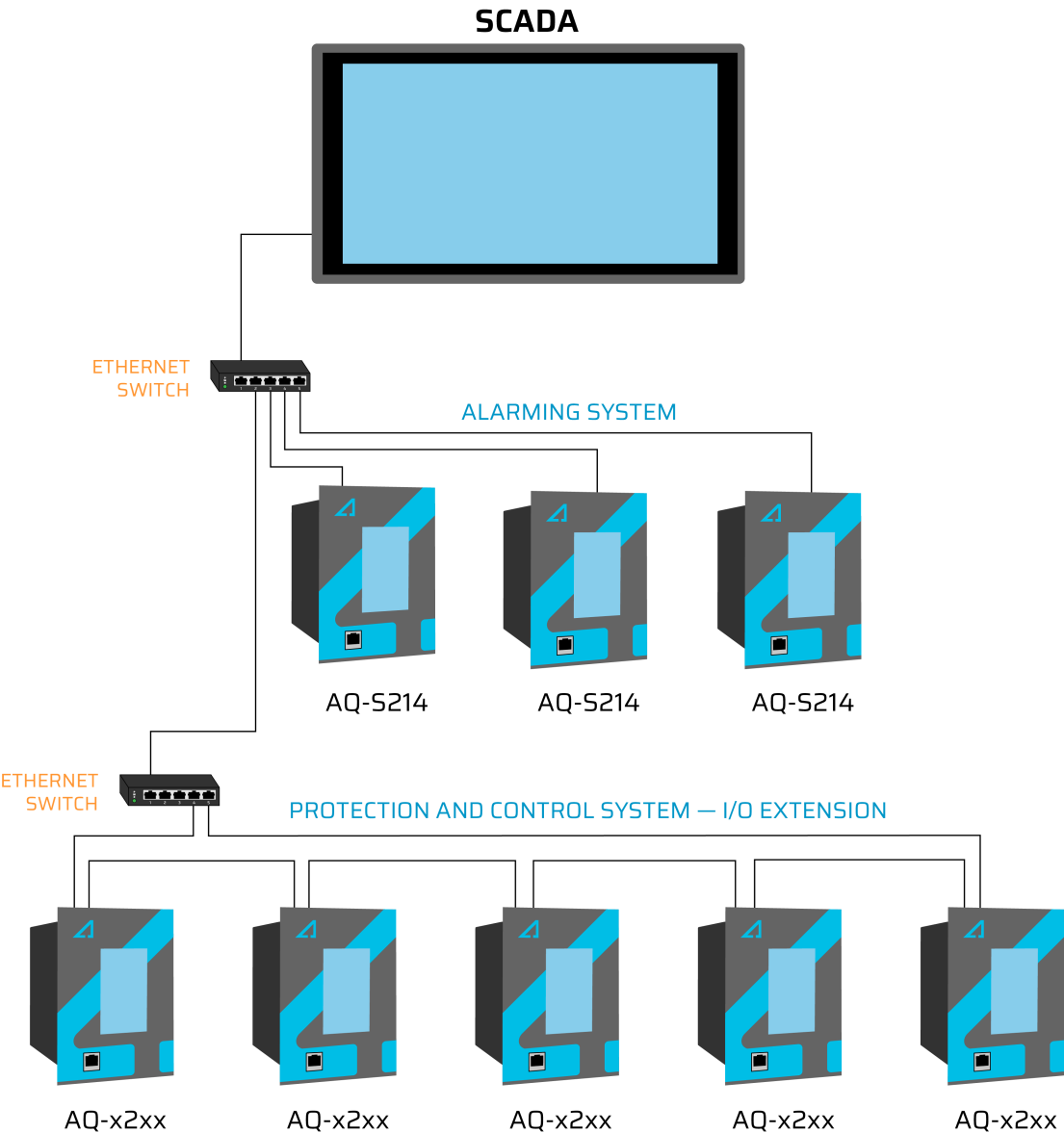
Figure. 6.1 - 60. AQ-S214 application example.
