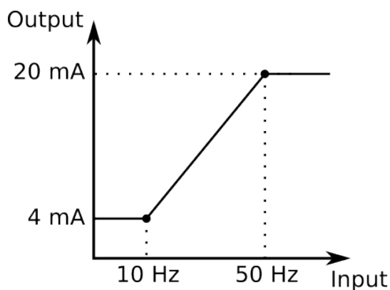
Figure. 4.4.4 - 50. Example of the effects of mA output channel settings.
