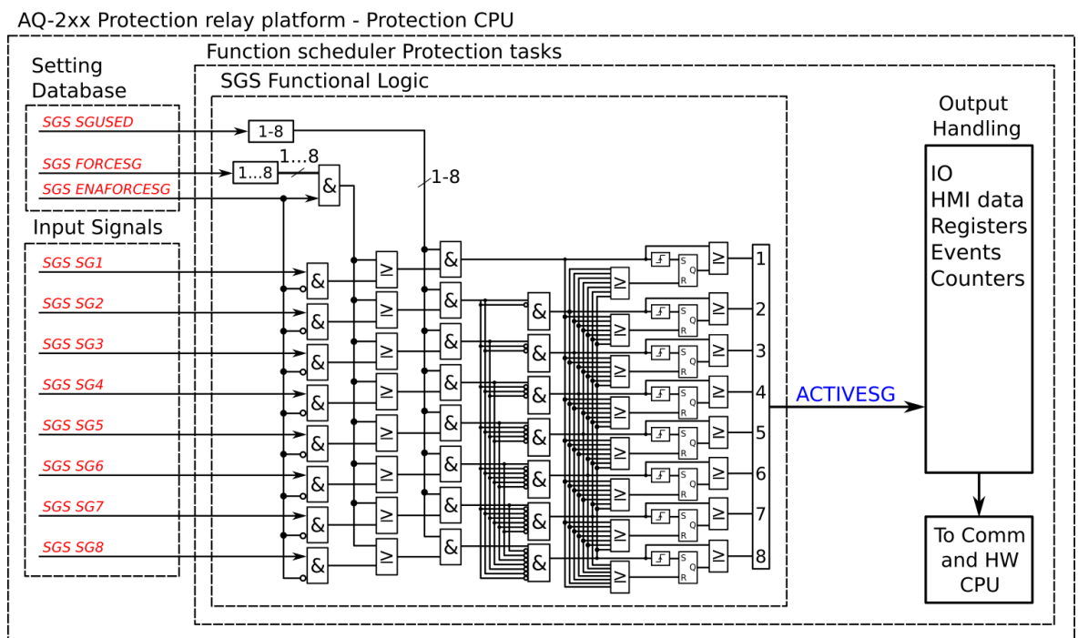
Figure. 4.4.1 - 43. Simplified function block diagram of the setting group selection function.
