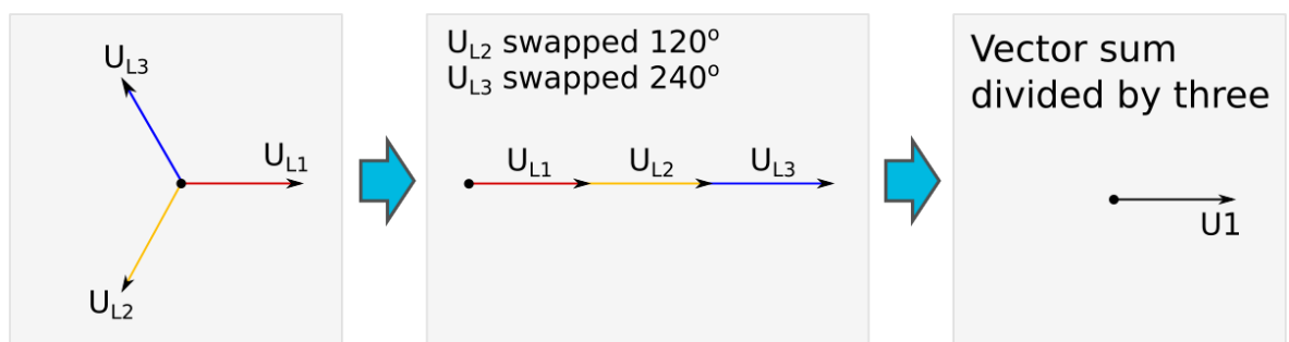
Figure. 4.4.14 - 142. Normal situation.
