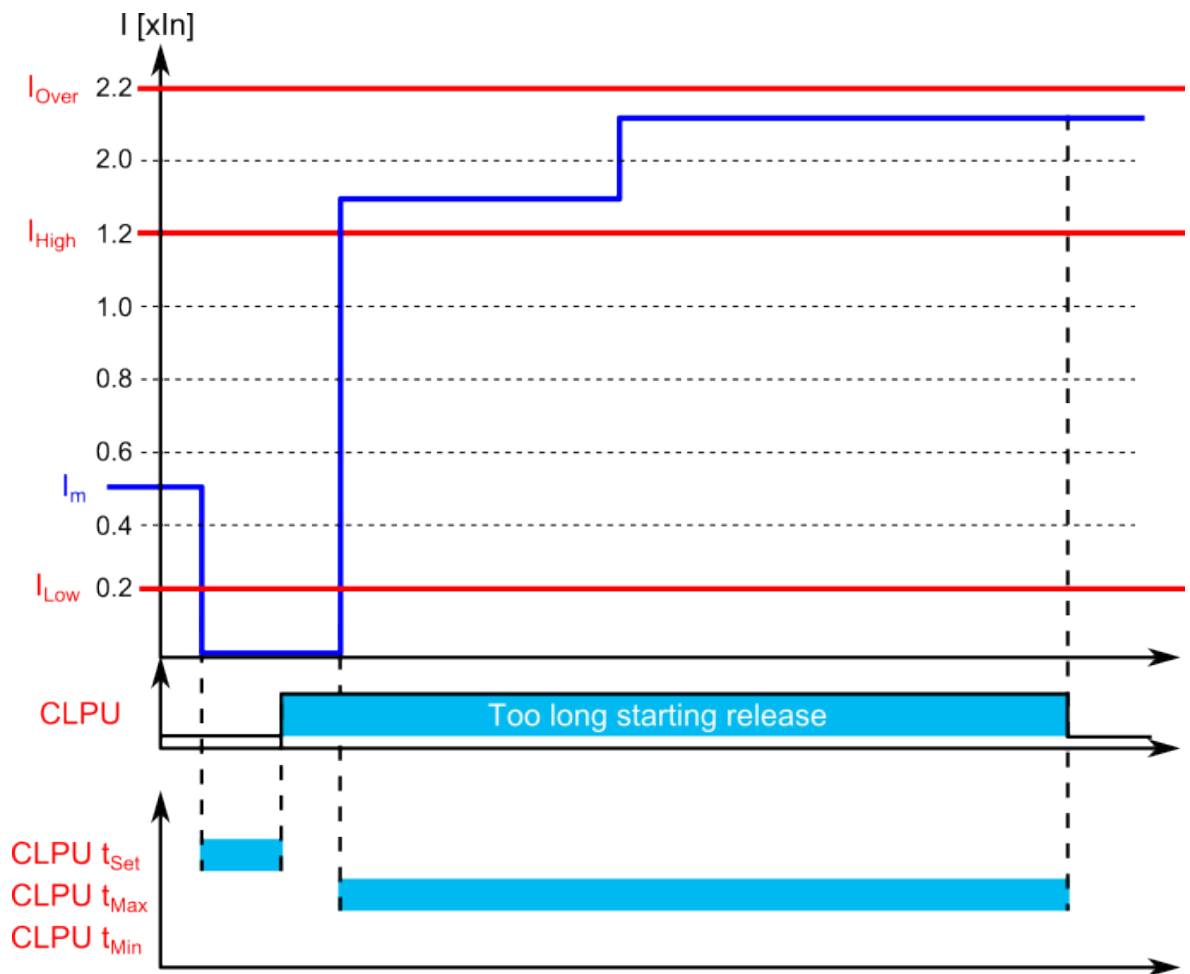
Figure. 4.5.5 - 191. Example of timers and pick-up parameters (activated pick-up and instant release due to too long starting).
