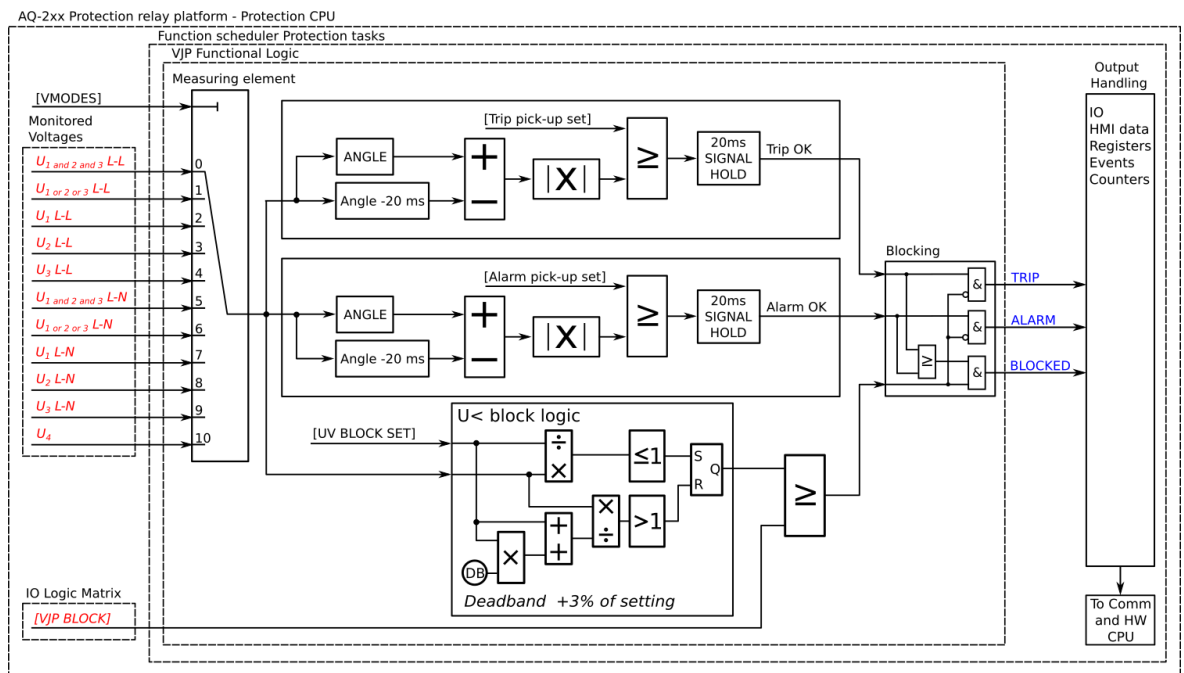
Figure. 4.5.9 - 214. Simplified function block diagram of the \Delta\phi function.
