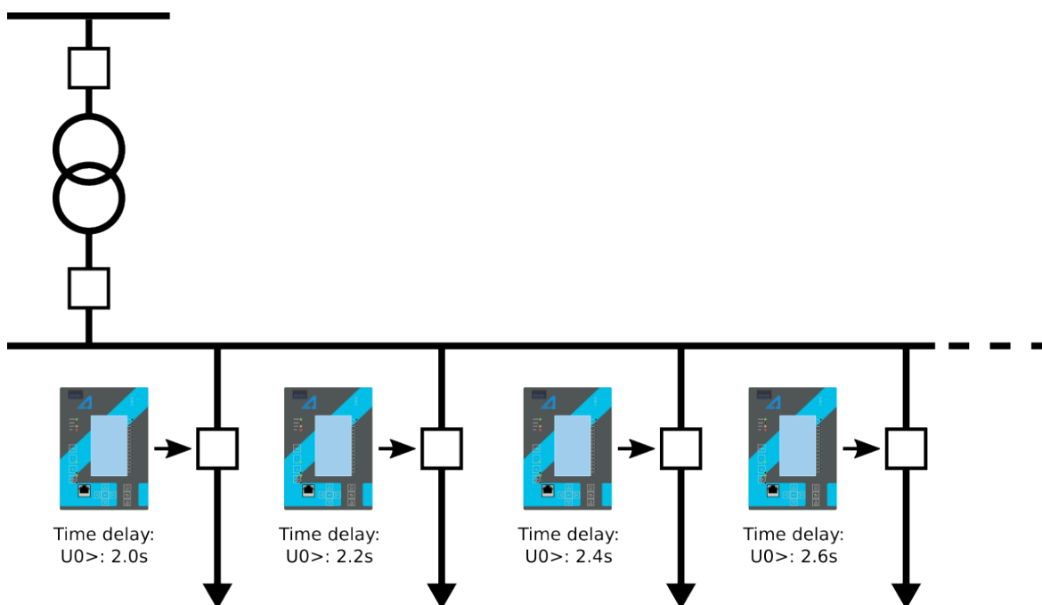
Figure. 4.5.8 - 213. Example application of zero sequence recloser. Each feeder has slightly longer operation time delay than the previous one.
