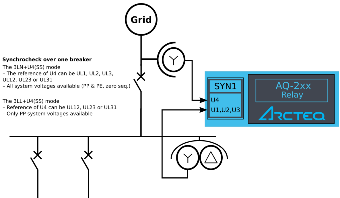
Figure. 4.5.10 - 220. Example application (synchrocheck over one breaker, with 3LL and 3LN VT connections).
