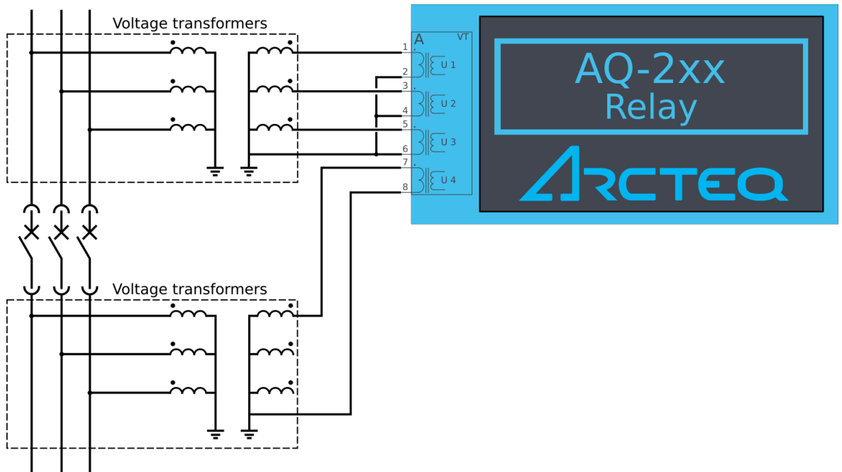
Figure. 4.5.10 - 217. Example connection of the synchrocheck function (3LN+U4 mode, SYN1 in use, UL1 as reference voltage).
