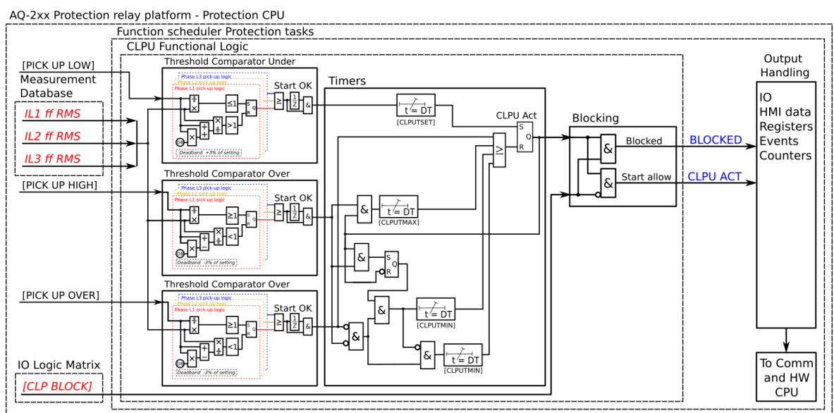
Figure. 4.5.5 - 187. Simplified function block diagram of the cold load pick-up function.
