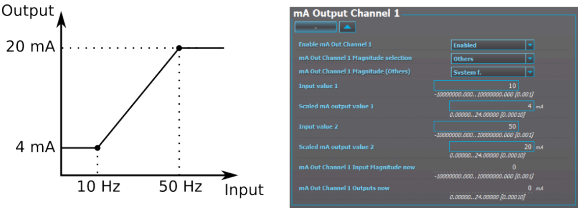
Figure. 4.5.11 - 227. Example of the effects of mA output channel settings.
