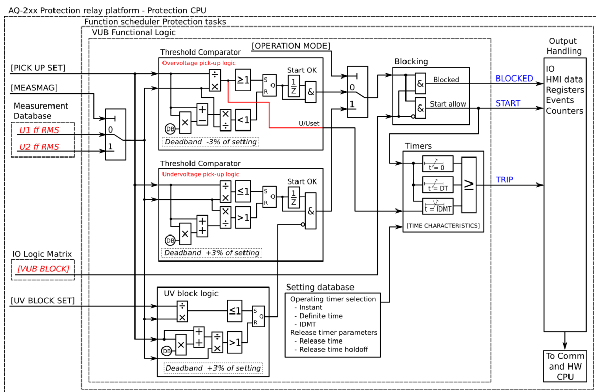
Figure. 4.4.14 - 148. Simplified function block diagram of the U1/U2&gt;/&lt; function.
