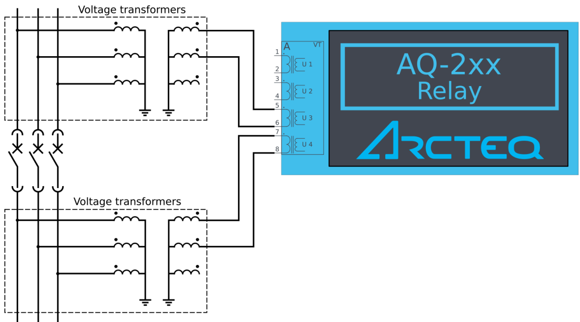
Figure. 4.5.10 - 219. Example connection of the synchrocheck function (2LL+U3+U4 mode, SYN3 in use, UL12 as reference voltage).
