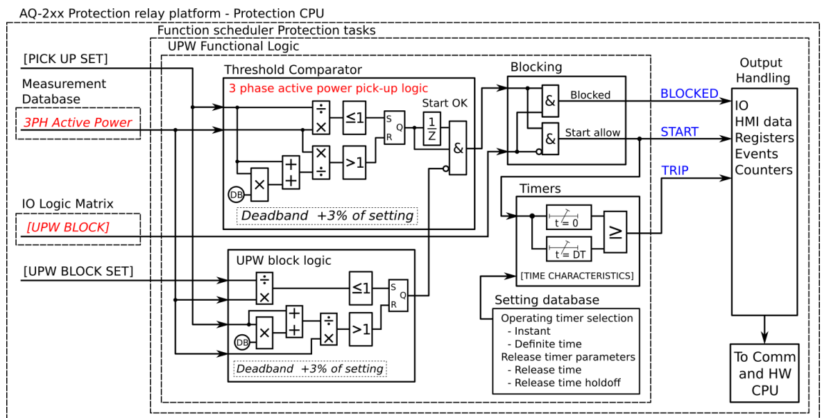
Figure. 4.4.18 - 157. Simplified function block diagram of the P < function.
