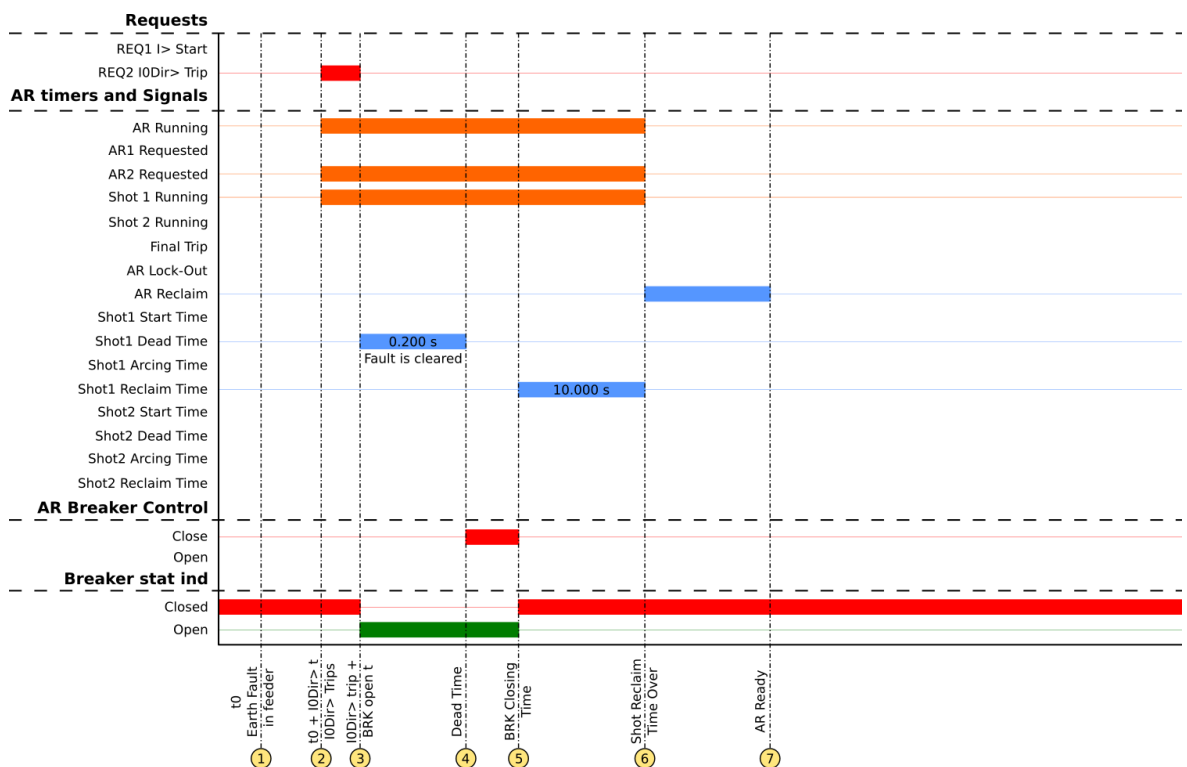
Figure. 4.5.7 - 203. Signal status graph of the transient earth fault auto-recloser cycle.
