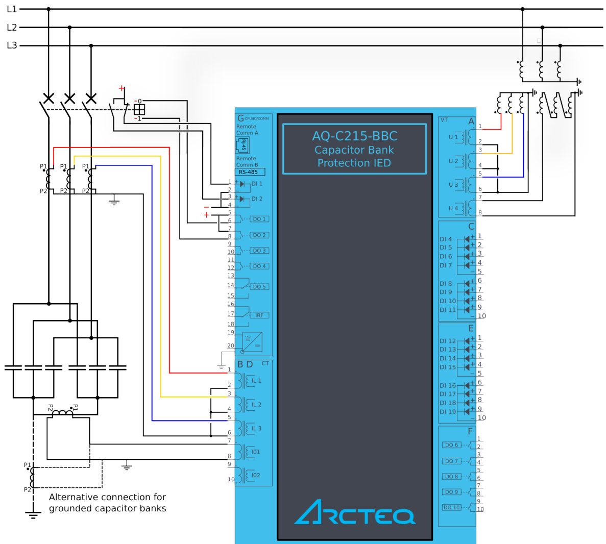
Figure. 6.2 - 180. Application example and its connections in double wye bank.
