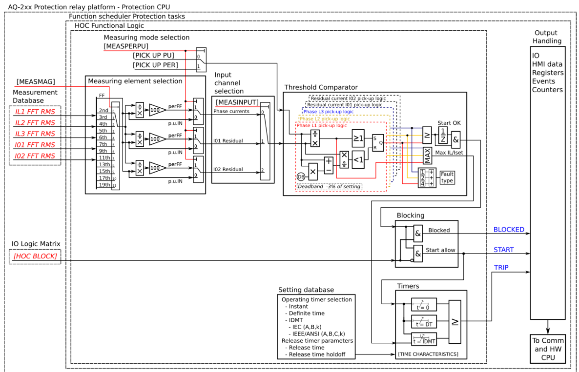
Figure. 4.4.7 - 94. Simplified function block diagram of the Ih&gt; function.
