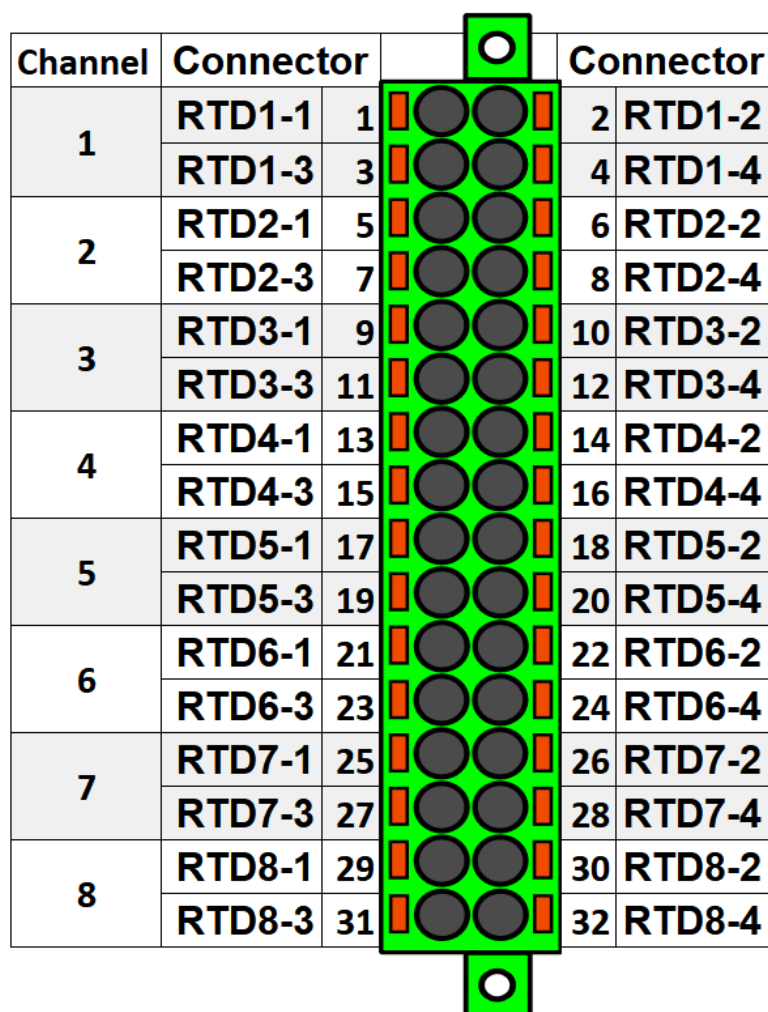
Figure. 7.5.5 - 196. RTD input module connectors.
