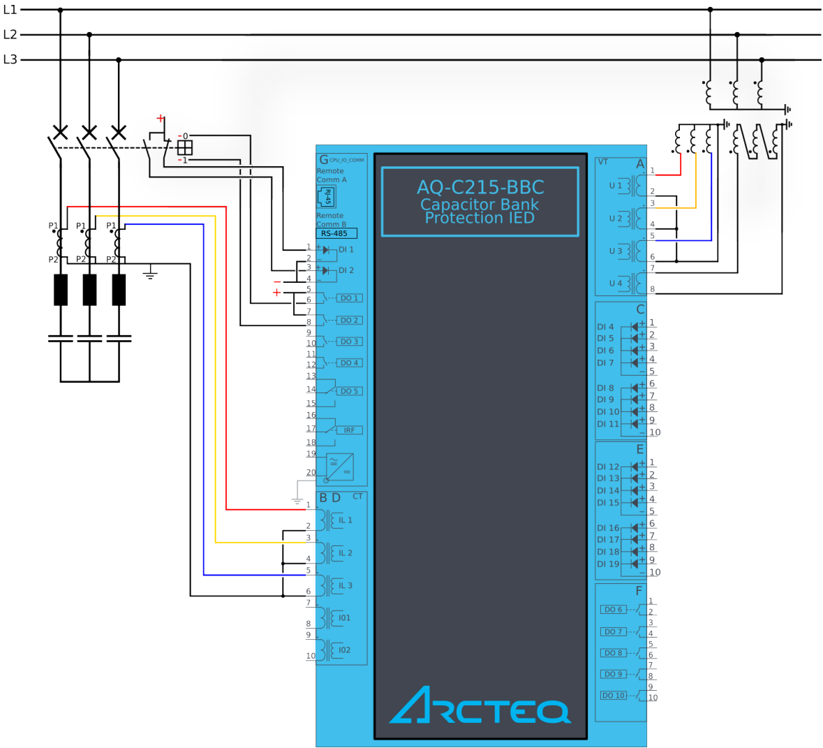
Figure. 6.2 - 179. Application example and its connections.
