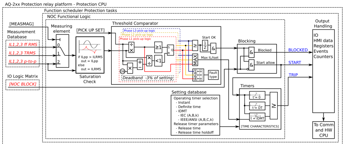
Figure. 4.4.4 - 90. Simplified function block diagram of the I&gt; function.
