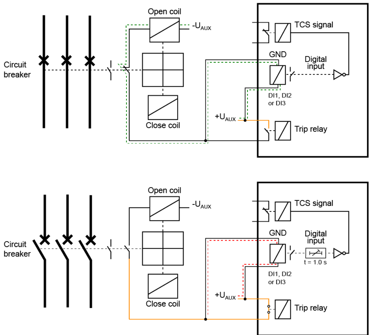
Figure. 6.4 - 184. Trip circuit supervision with one DI and one latched output contact.
