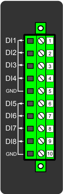
Figure. 7.5.1 - 191. Digital input module (DI8) with eight add-on digital inputs.
