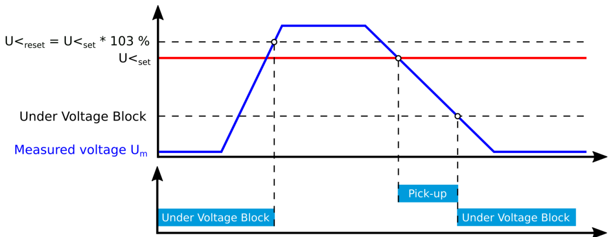
Figure. 4.4.10 - 114. Example of the block setting operation.
