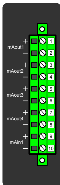
Figure. 7.5.3 - 194. Milliampere output (mA) I/O module connections.
