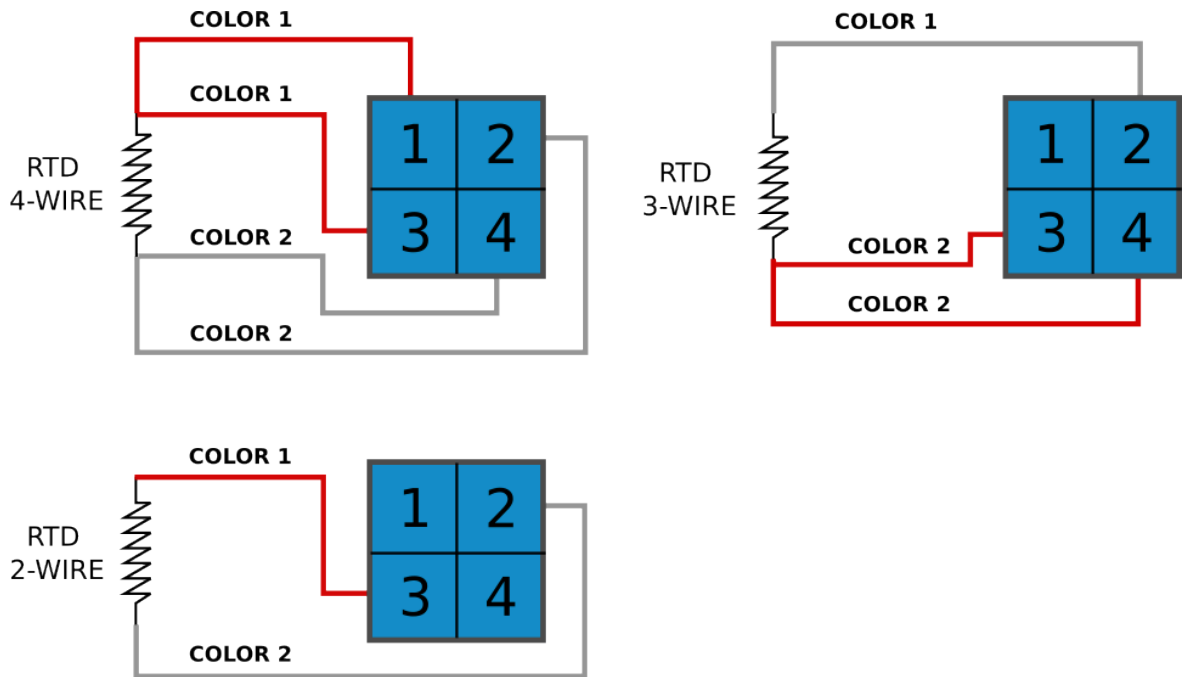
Figure. 7.5.5 - 197. RTD sensor connection types.
