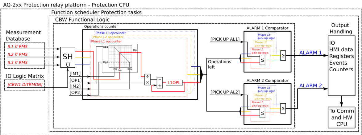
Figure. 4.6.3 - 171. Simplified function block diagram of the circuit breaker wear function.
