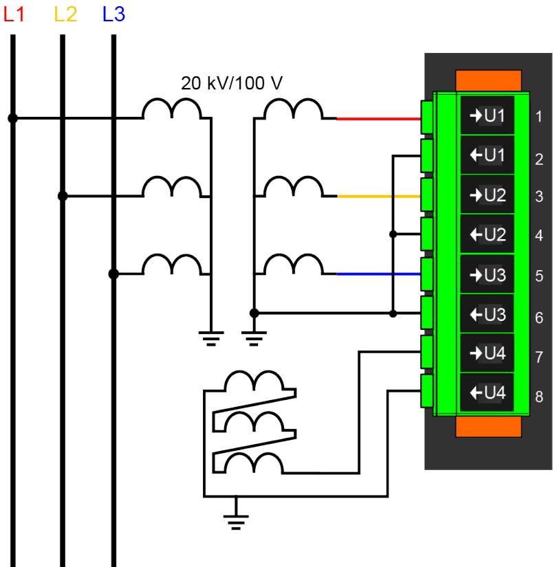
Figure. 4.2.2 - 69. Connections.
