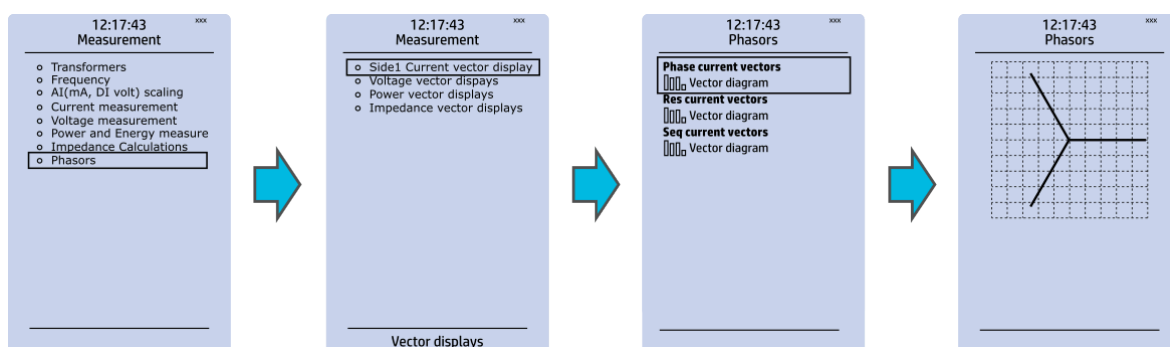
Figure. 3.7 - 51. Phasors submenu.
