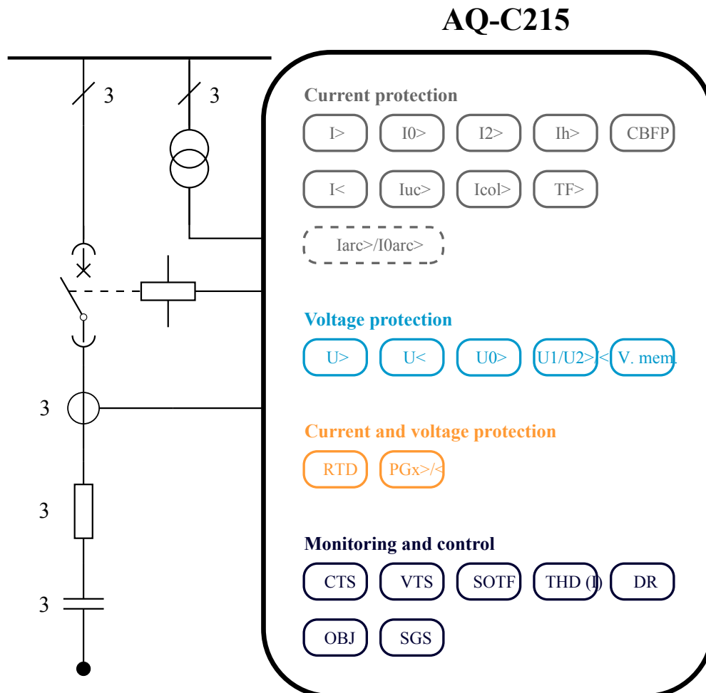
Figure. 6.1 - 178. AQ-C215 application example with function block diagram.
