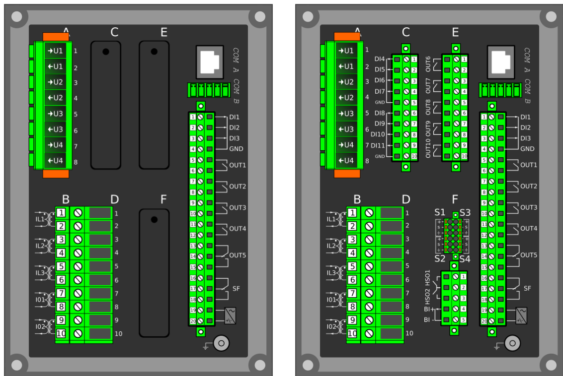
Figure. 7.1 - 186. Modular construction of AQ-X215.
