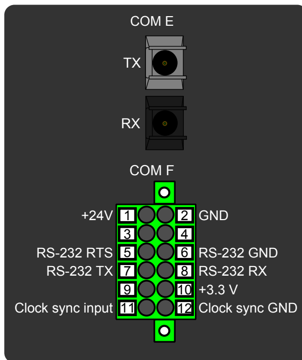
Figure. 7.5.10 - 203. Serial RS-232 module connectors.
