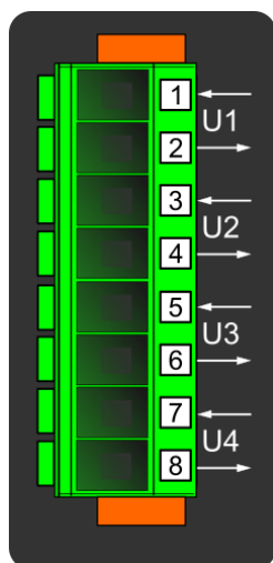
Figure. 7.4 - 190. Voltage measurement module.
