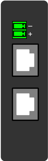
Figure. 7.5.7 - 199. Double RJ-45 10/100 Mbps Ethernet communication module.
