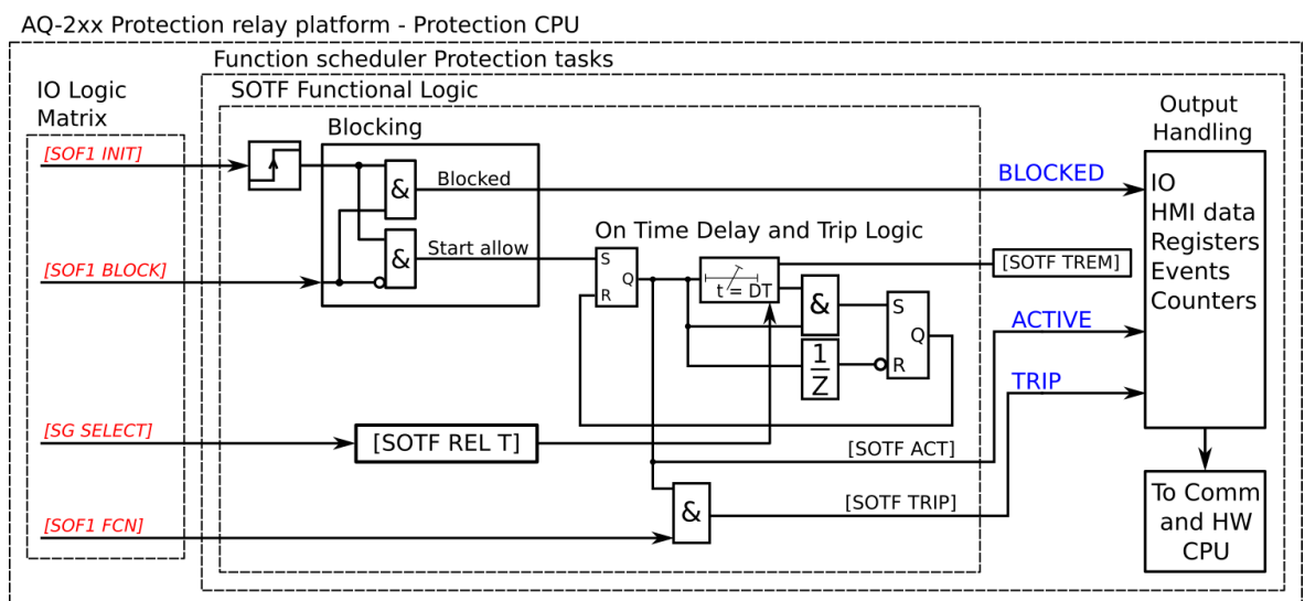
Figure. 4.5.5 - 151. Simplified function block diagram of the switch-on-to-fault function.
