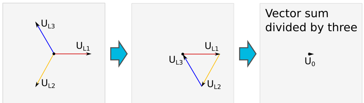
Figure. 4.4.11 - 115. Normal situation.
