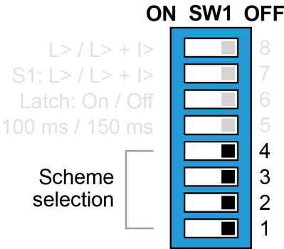
Figure. 8.2 - 10. DIP switches used for selecting the logic scheme.
