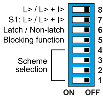
Figure. 8.1 - 9. DIP switch diagram.
