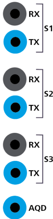
Figure. 6.1.1 - 3. Arc fiber loop sensor and arc quenching device connections.
