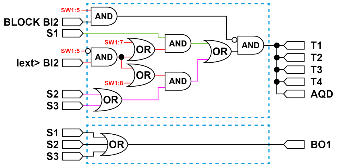
Figure. 8.2.3 - 19. Simplified logic diagram of SS:2.
