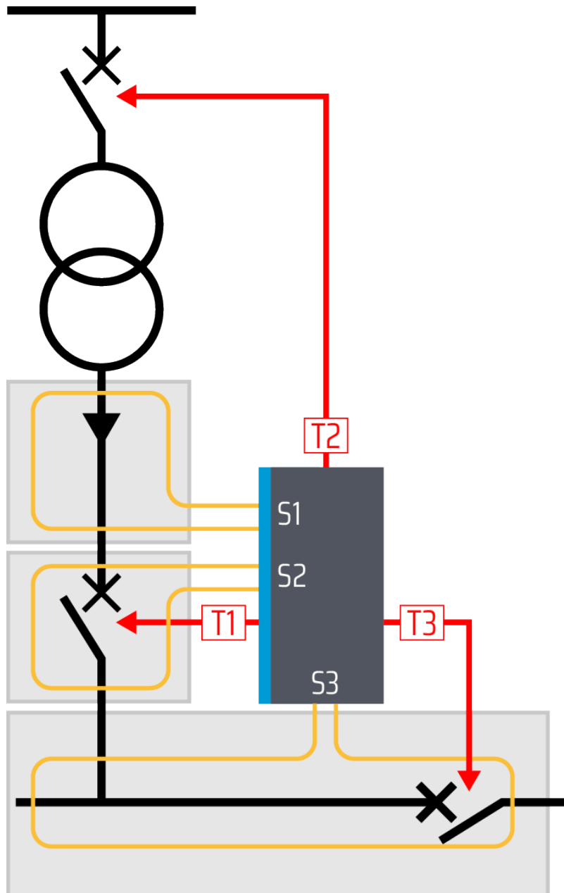
Figure. 8.2.2 - 14. SS:1 example application.
