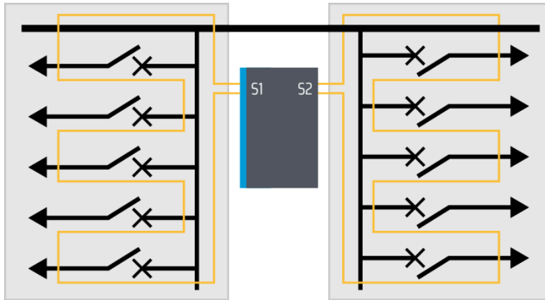
Figure. 8.2.1 - 11. SS:0 example application.
