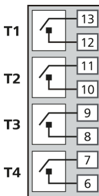
Figure. 6.2.2 - 6. Trip relay connections
