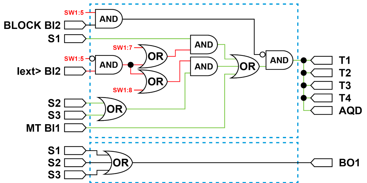
Figure. 8.2.1 - 13. Simplified logic diagram of SS:0.
