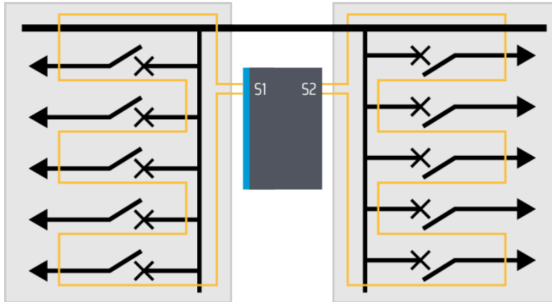
Figure. 8.2.3 - 17. SS:2 example application.
