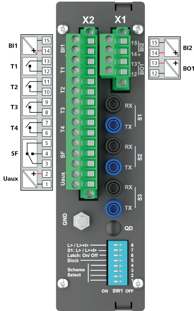
Figure. 6 - 2. Rear terminals of AQ-102LV.
