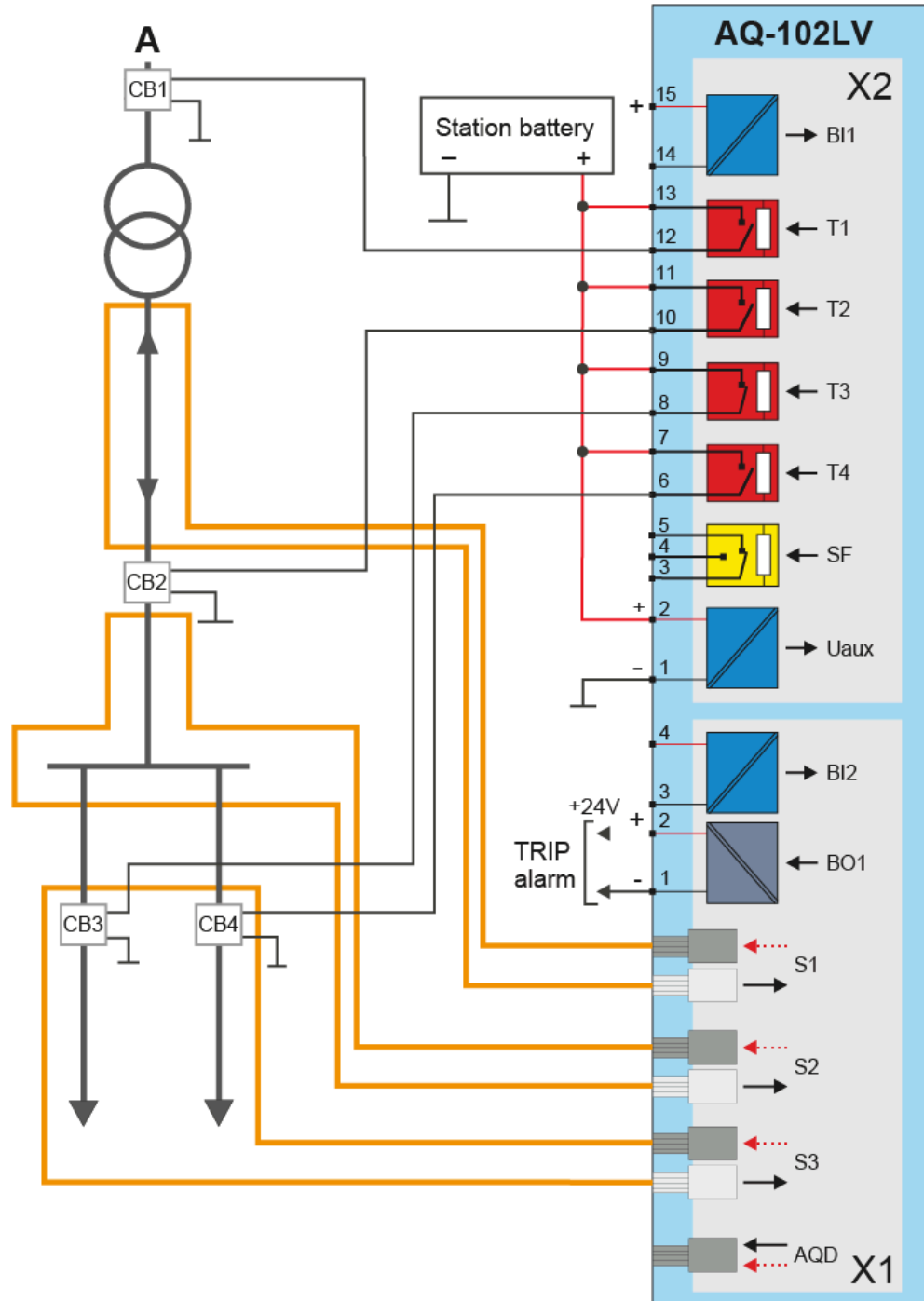
Figure. 10 - 25. Example wiring diagram for AQ-102LV.
