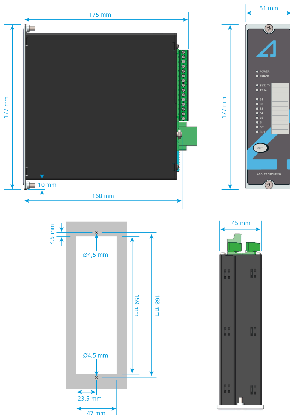
Figure. 11 - 26. Dimensions of the device and its cut-out panel.
