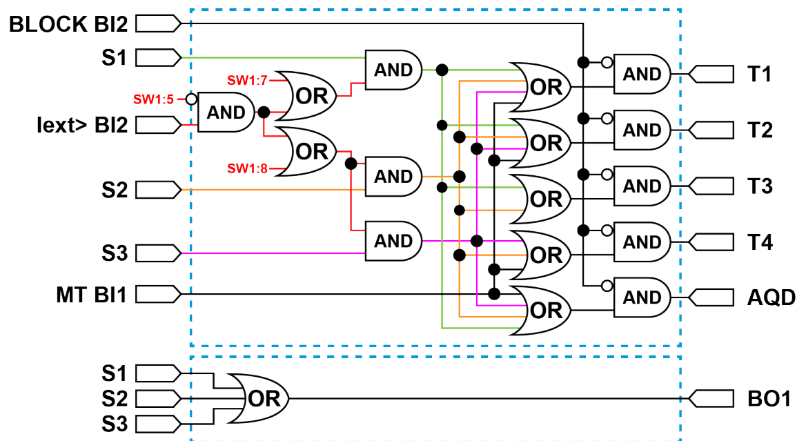
Figure. 8.2.4 - 21. Simplified logic diagram of SS:3.
