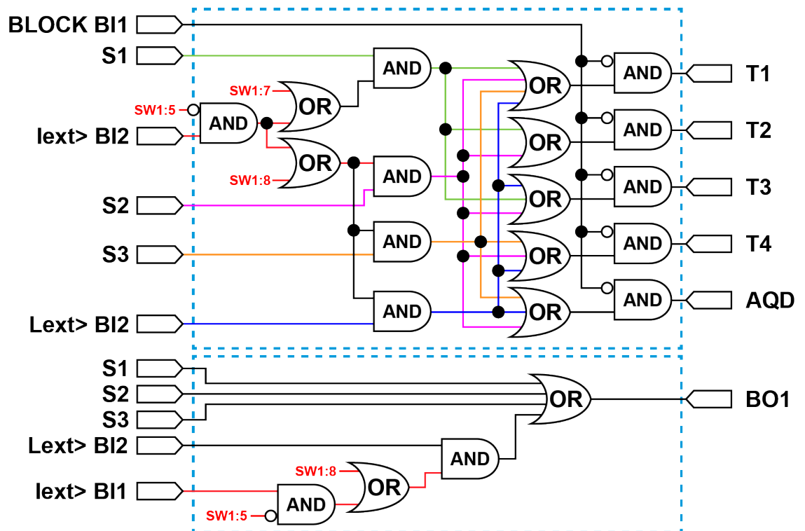
Figure. 8.2.5 - 23. Simplified logic diagram of SS:4.
