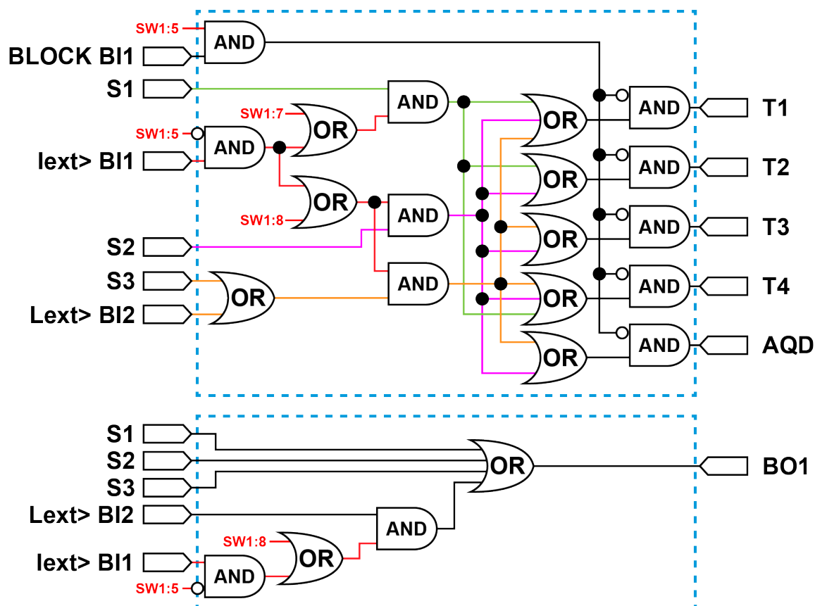
Figure. 8.2.2 - 16. Simplified logic diagram of SS:1.
