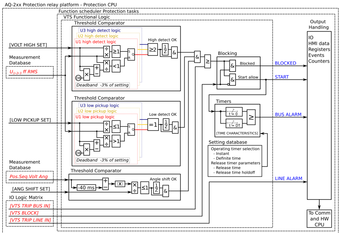
Figure. 4.6.2 - 233. Simplified function block diagram of the VTS function.
