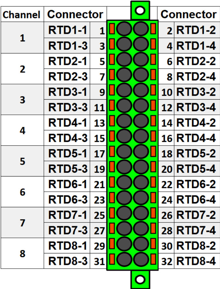
Figure. 7.5.4 - 258. RTD input module connectors.
