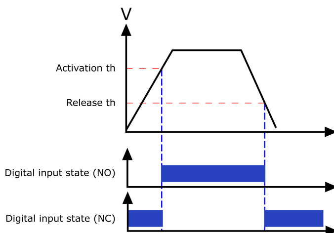
Figure. 7.5.1 - 255. Digital input state when energizing and de-energizing the digital input channels.
