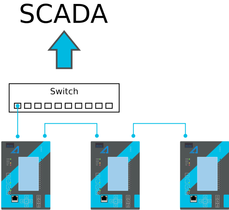
Figure. 7.5.8 - 265. Example of a multidrop configuration.
