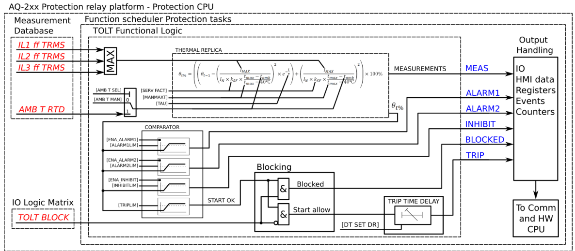
Figure. 4.4.22 - 167. Simplified function block diagram of the TT> function.
