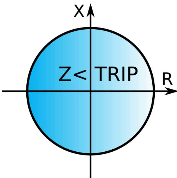
Figure. 4.4.20 - 161. Operating characteristics of underimpedance protection.
