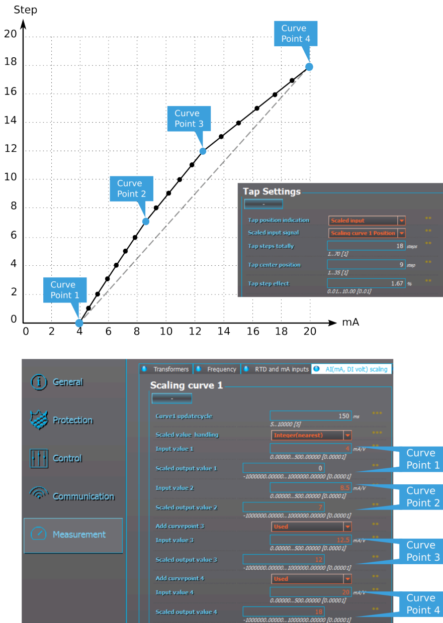
Figure. 4.5.2 - 177. Example of Scaled input setting.
