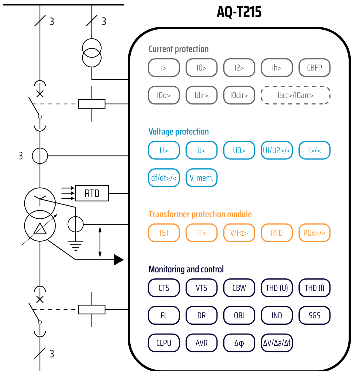
Figure. 6.1 - 242. AQ-T215 application example with function block diagram.
