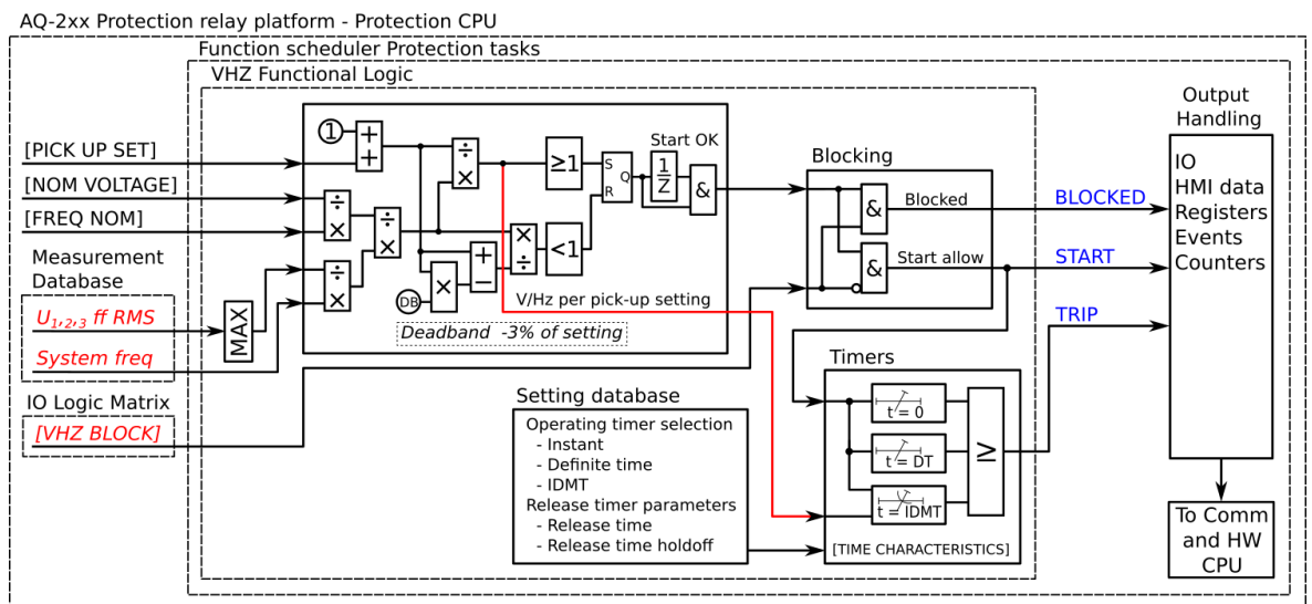
Figure. 4.4.19 - 158. Simplified function block diagram of the V/Hz&gt; function.
