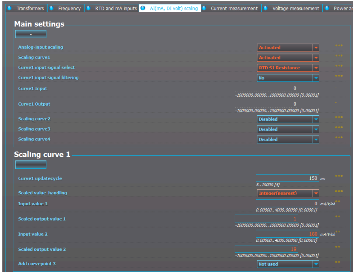
Figure. 4.5.2 - 178. Example scaling for tap position indication with RTD measurement.
