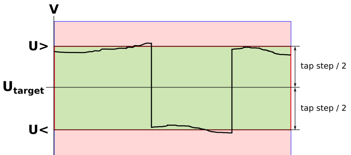
Figure. 4.5.2 - 181. Tight voltage window (window reached but voltage near the limit).
