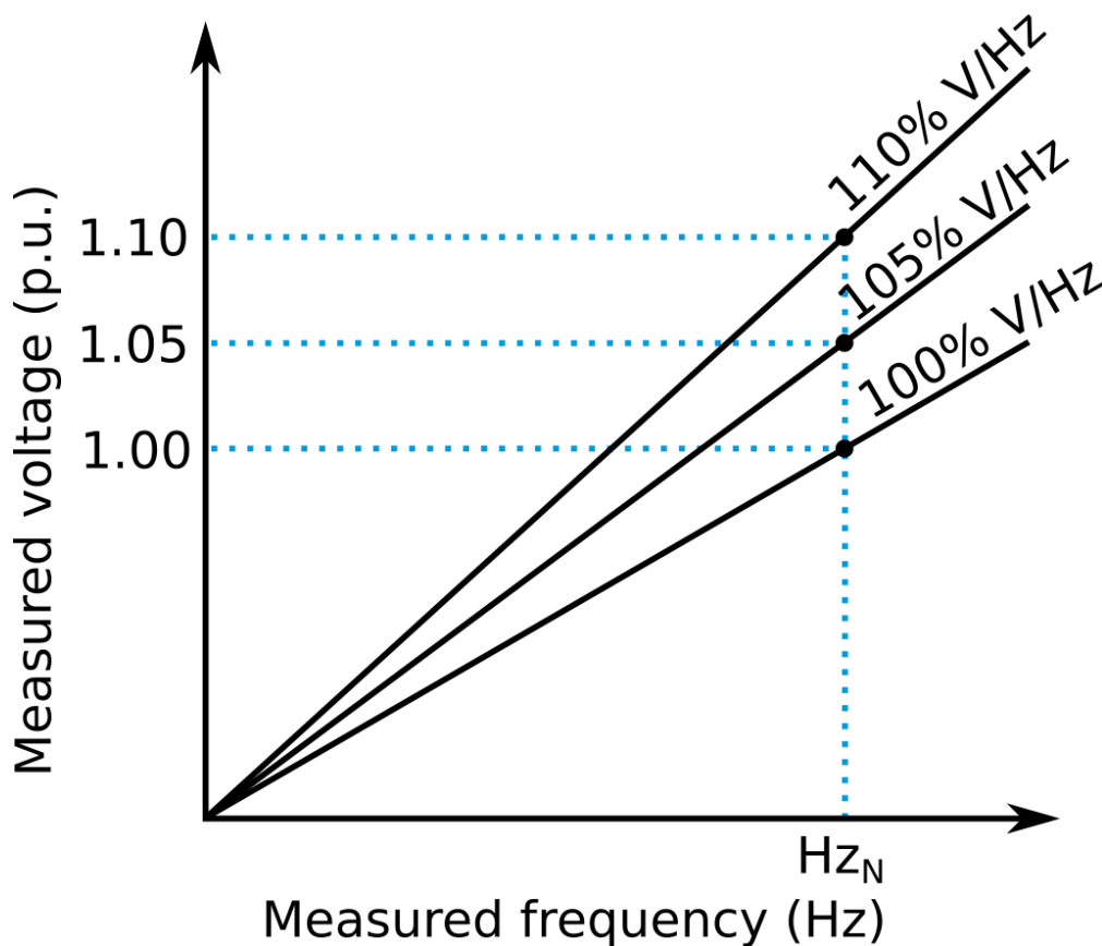
Figure. 4.4.19 - 157. Effect of pick-up settings and the measured frequency to the overvoltage function's pick-up level.
