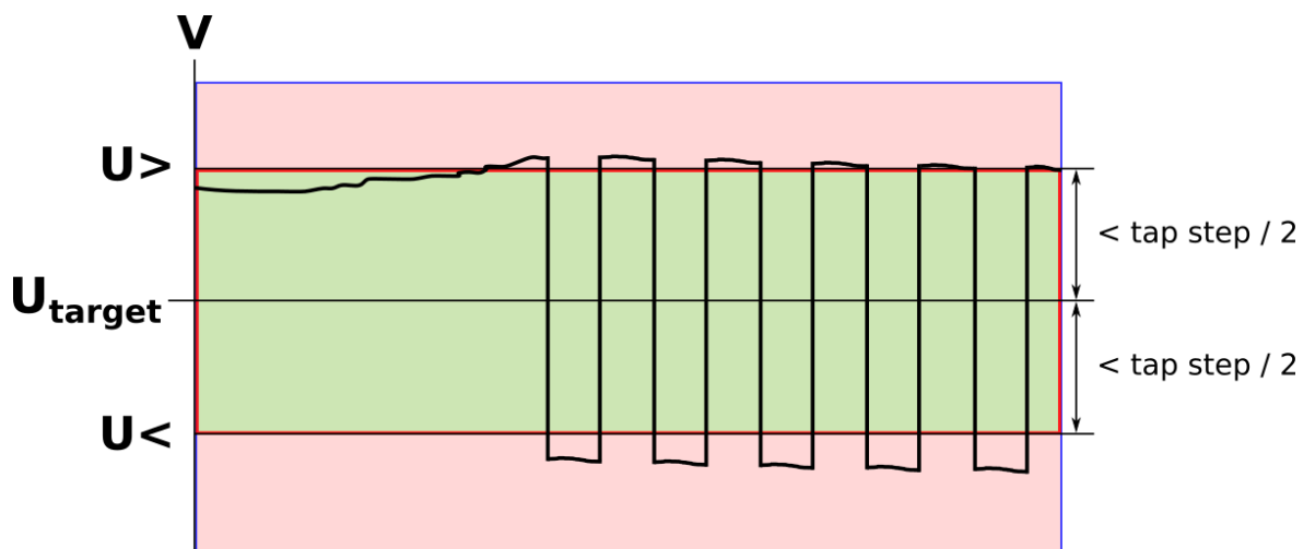
Figure. 4.5.2 - 180. Tight voltage window (window not reached).
