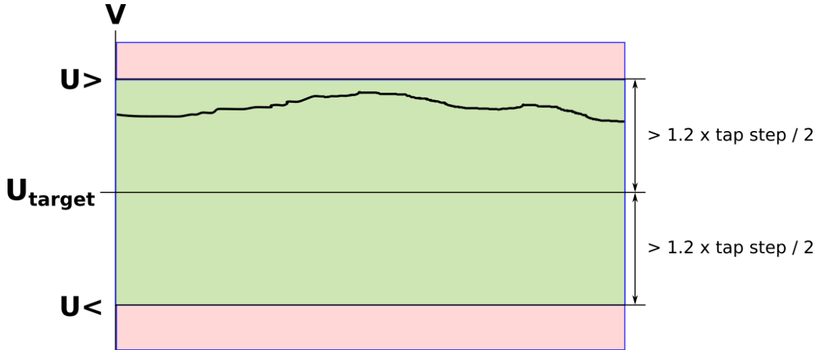
Figure. 4.5.2 - 182. Voltage window according to the recommendation.
