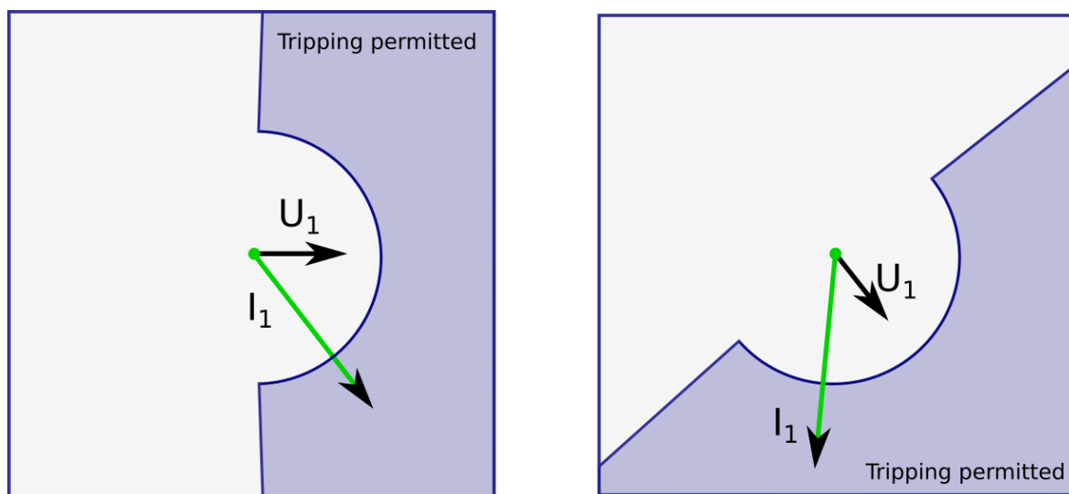
Figure. 4.4.4 - 91. Angle tracking of the I_{dir}> function (3LN/3LL + U_0 mode).
