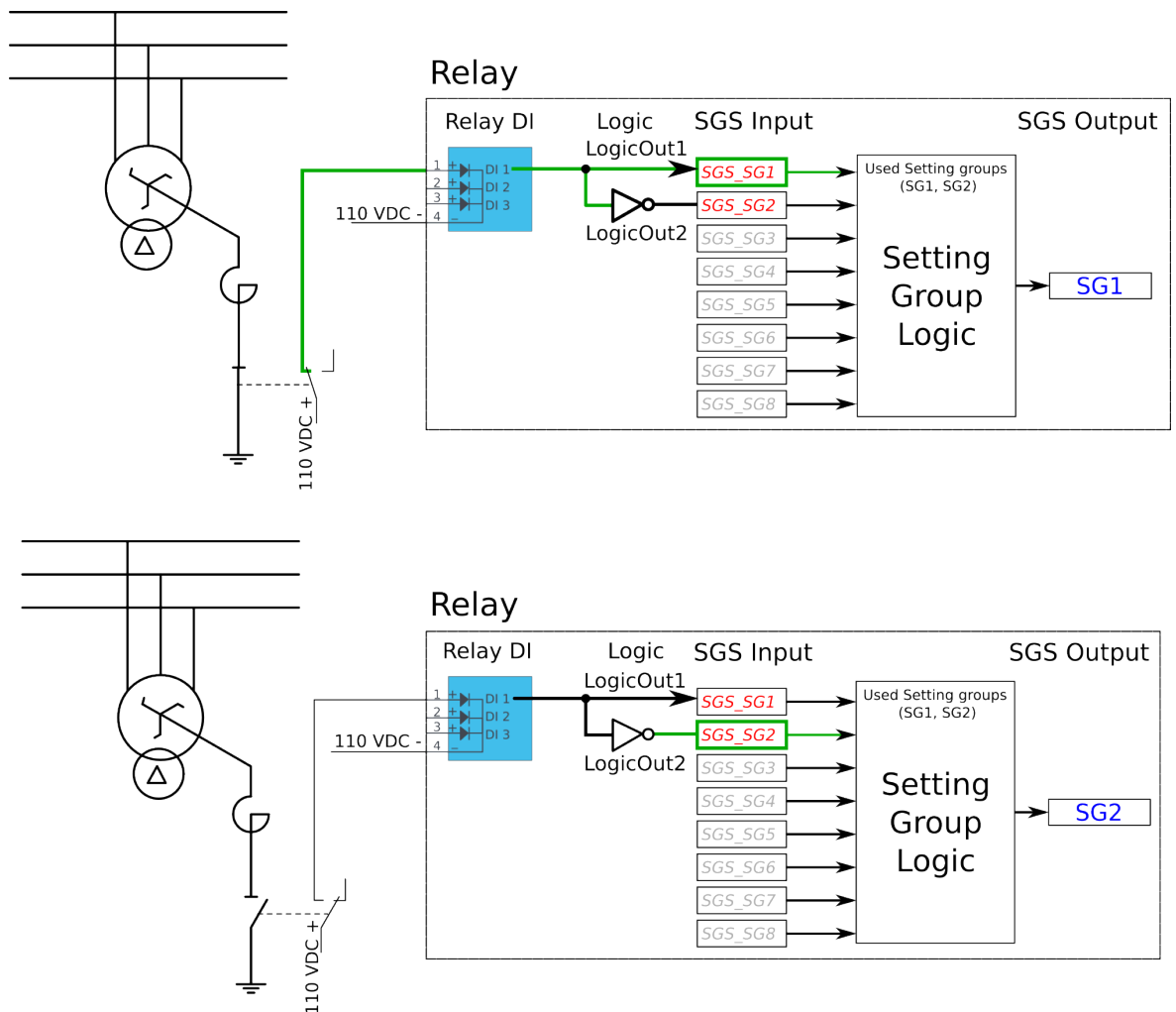
Figure. 4.5.3 - 191. Setting group control – one-wire connection from Petersen coil status.
