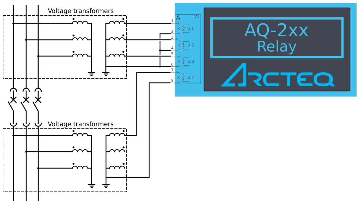
Figure. 4.5.7 - 204. Example connection of the synchrocheck function (3LN+U4 mode, SYN1 in use, UL1 as reference voltage).
