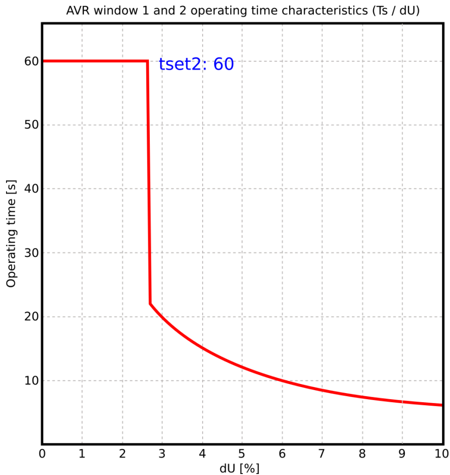
Figure. 4.5.2 - 185. Combined operating time characteristics of both voltage windows.
