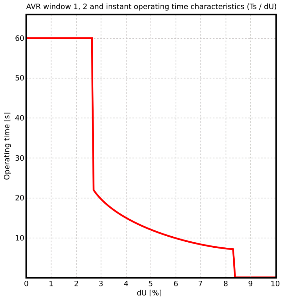
Figure. 4.5.2 - 187. Effect of the Instant low setting on time characteristics.
