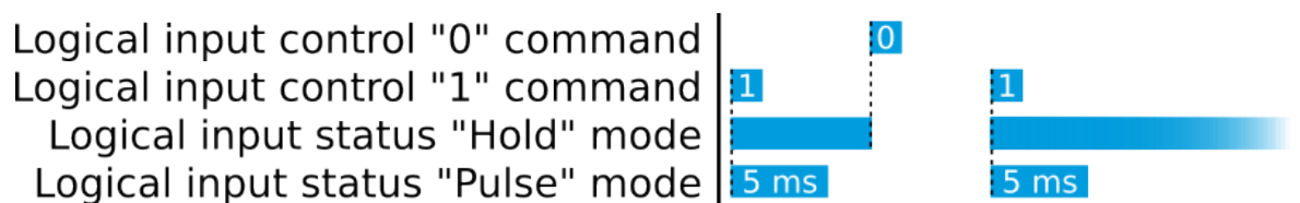
Figure. 4.5.13 - 219. Operation of logical input in "Hold" and "Pulse" modes.
