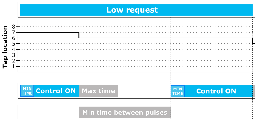
Figure. 4.5.2 - 173. Control pulse timing settings.
