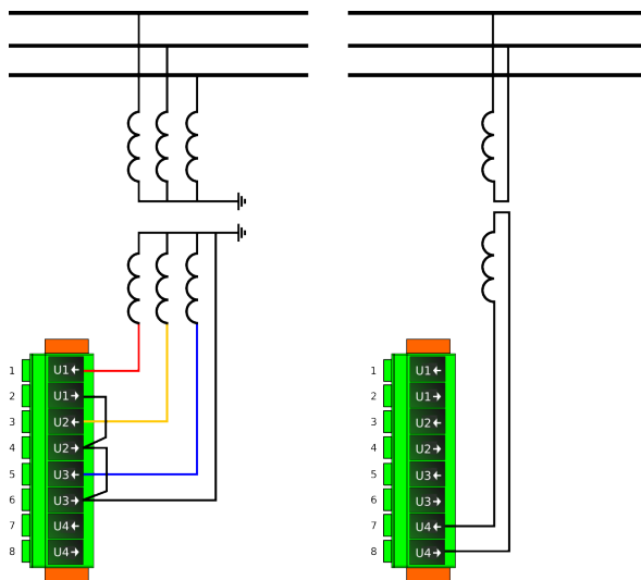
Figure. 4.5.2 - 172. Two connection options for voltage measurement.
