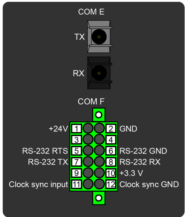
Figure. 7.5.5 - 260. Serial RS-232 module connectors.
