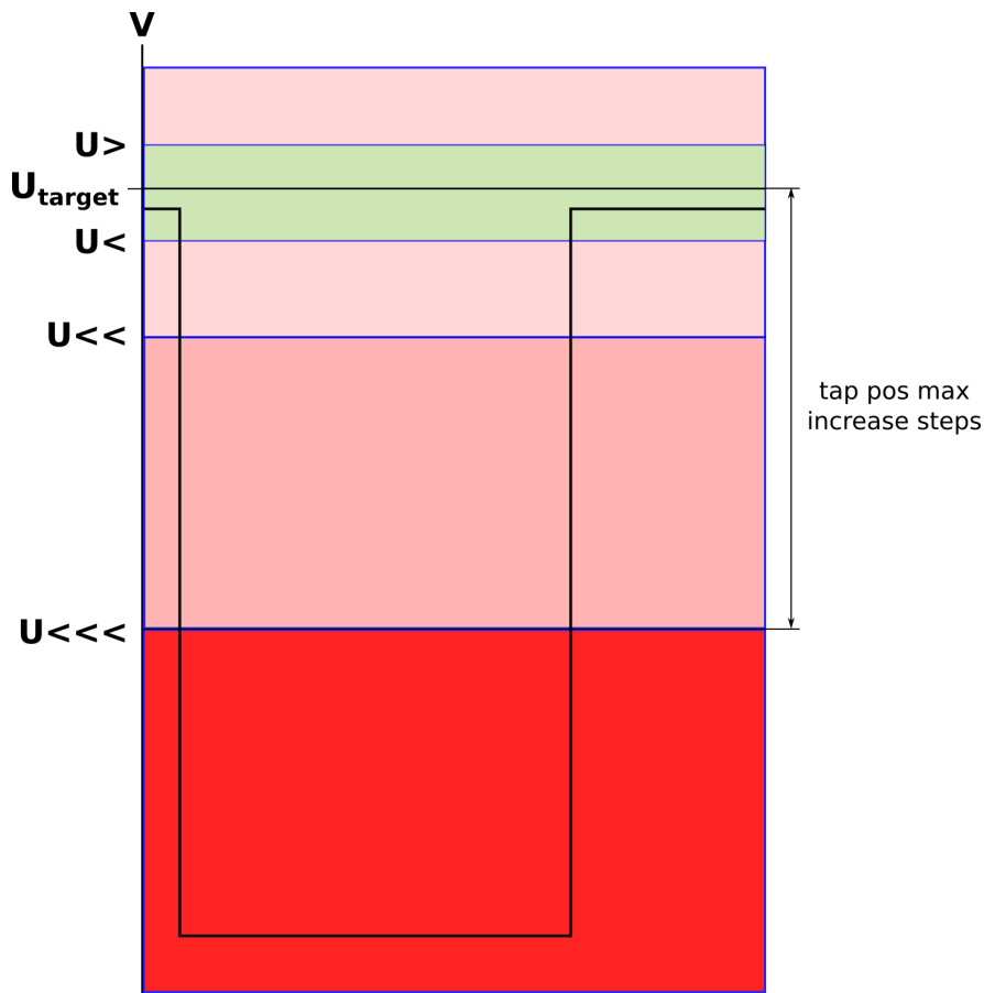
Figure. 4.5.2 - 188. Low voltage blocking.
