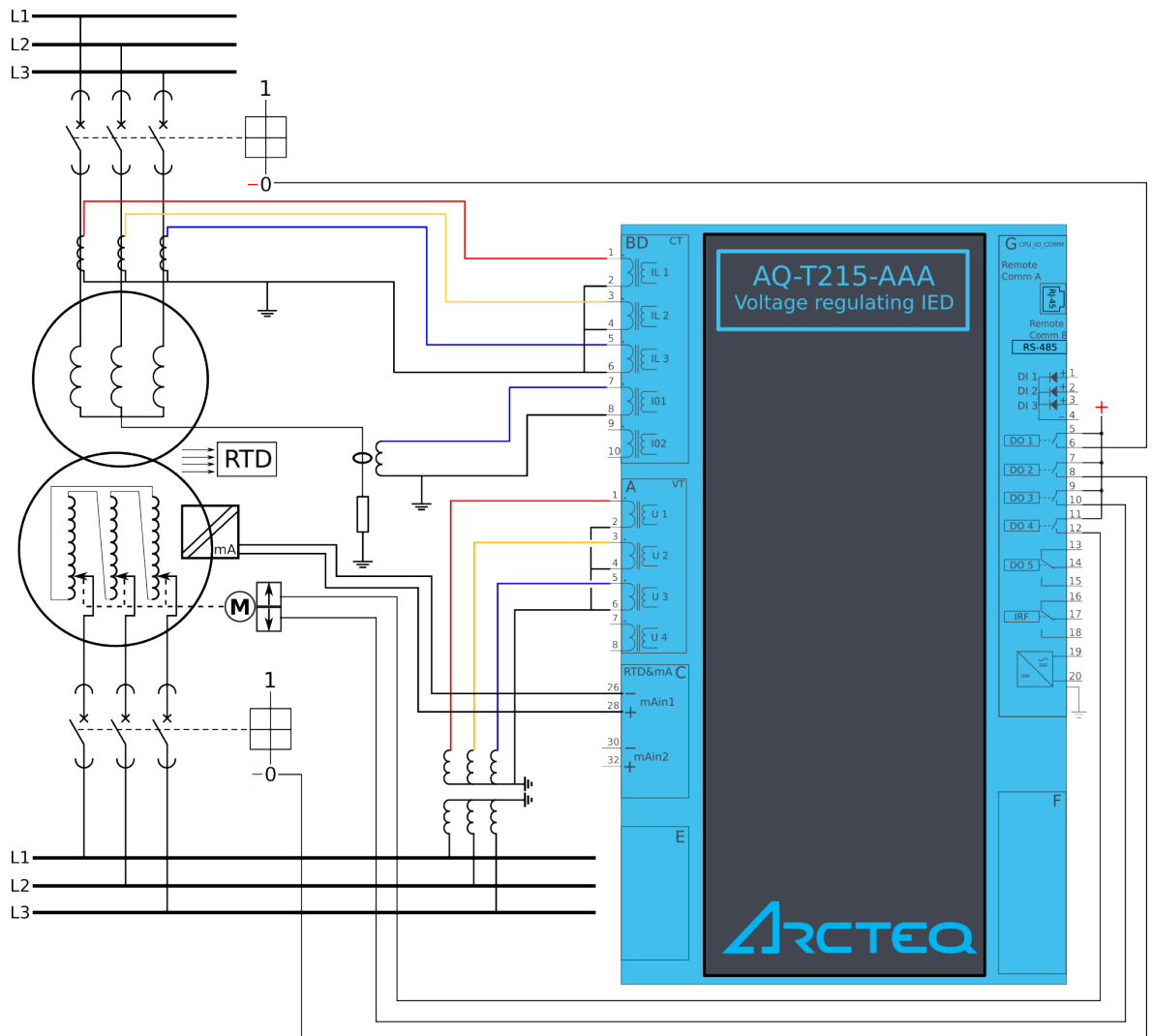
Figure. 6.2 - 243. Application example and its connections.
