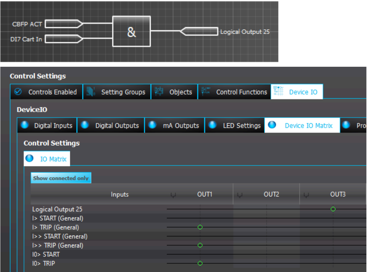
Figure. 4.5.12 - 218. Logic output example. Logical output is connected to an output relay in matrix.
