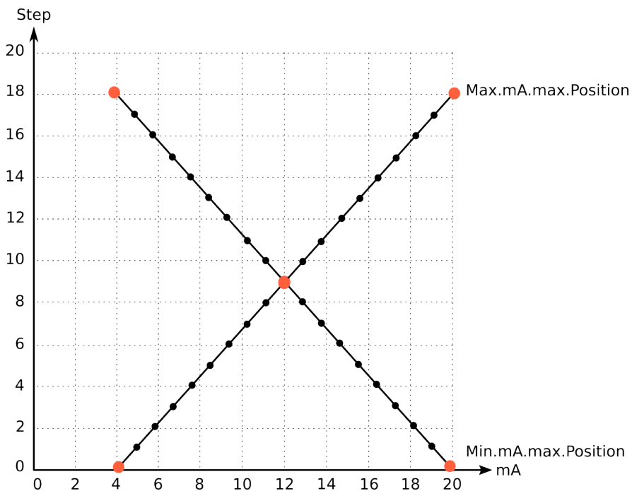
Figure. 4.5.2 - 176. Switching the tap position indication.
