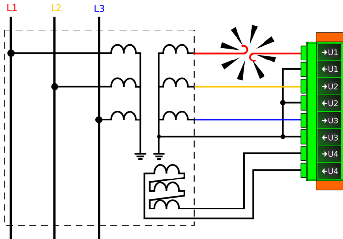
Figure. 4.6.2 - 232. Secondary circuit fault in phase L1 wiring.
