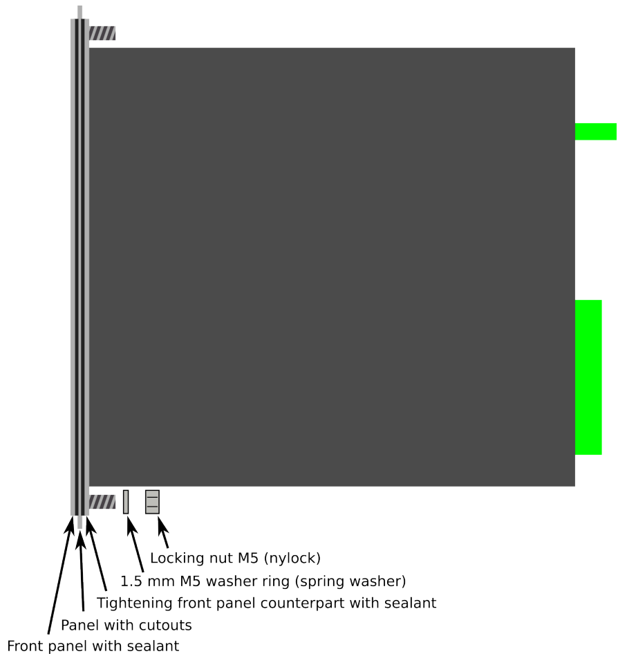
Figure. 7.6 - 268. Device installation.
