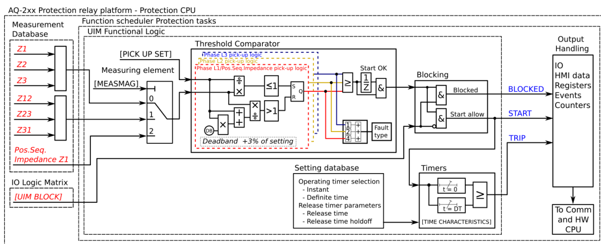
Figure. 4.4.20 - 162. Simplified function block diagram of the Z&lt; function.
