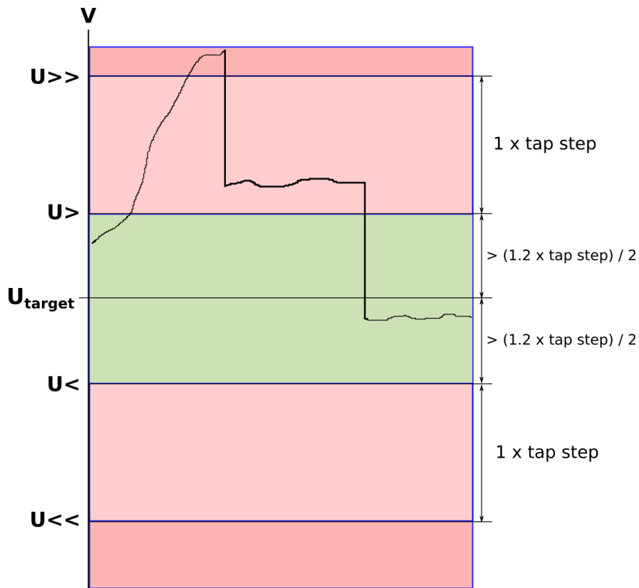
Figure. 4.5.2 - 183. Second voltage window two tap steps from the first voltage window.
