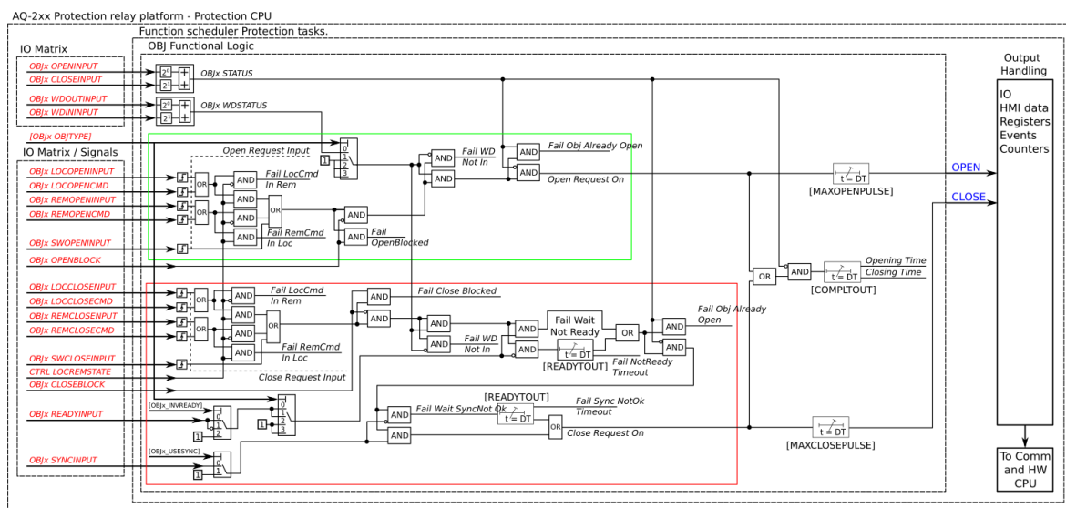
Figure. 4.5.4 - 195. Simplified function block diagram of the object control and monitoring function.
