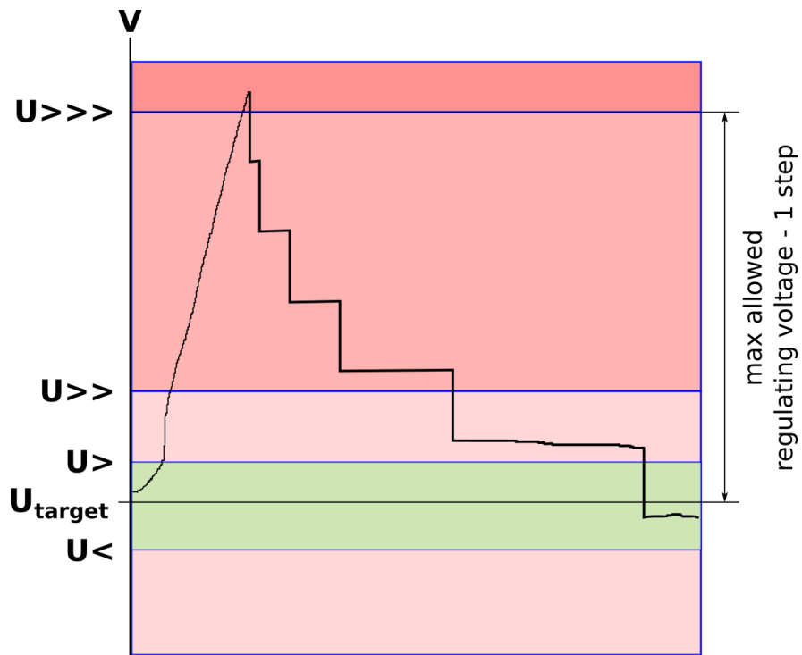
Figure. 4.5.2 - 186. Instant low command with two time-delayed windows.
