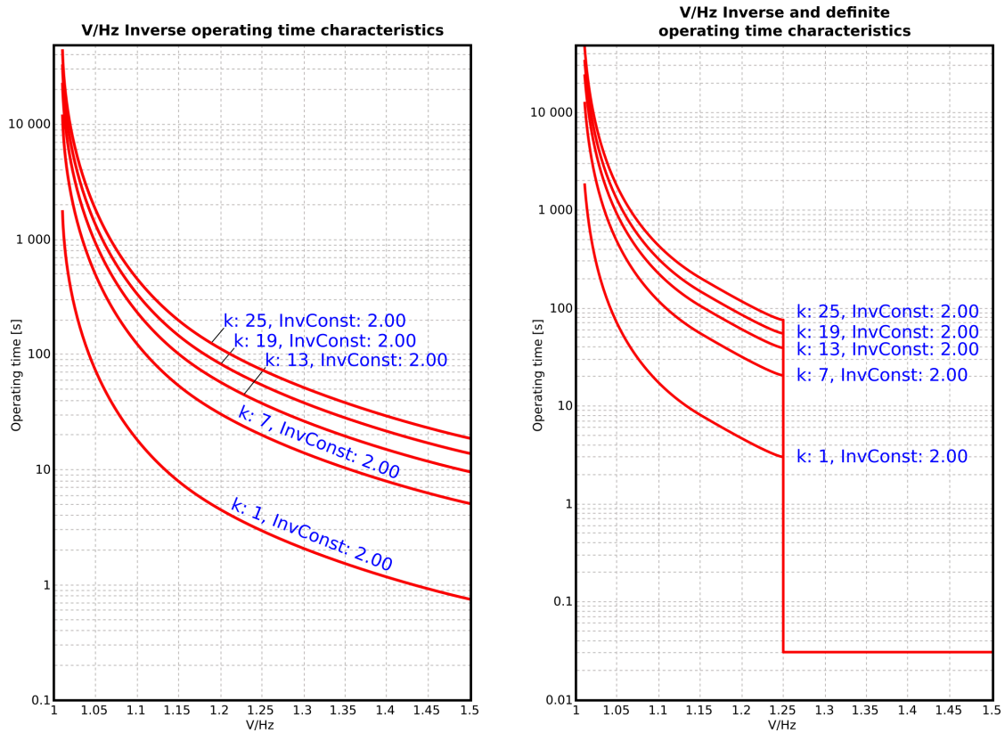
Figure. 4.4.19 - 159. Inverse (above) and inverse and DT (below) time characteristics with the TimeDial k setting effect.
