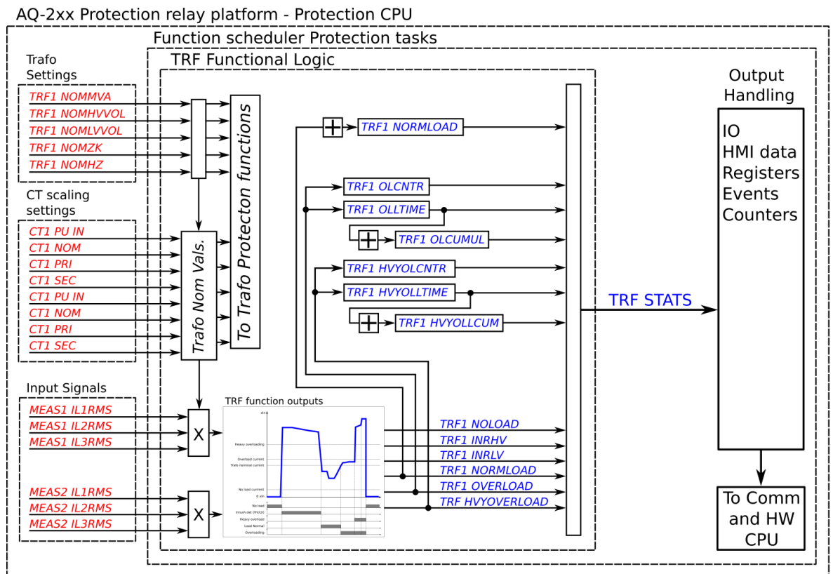
Figure. 4.4.21 - 163. Simplified function block diagram of the transformer status monitoring function.
