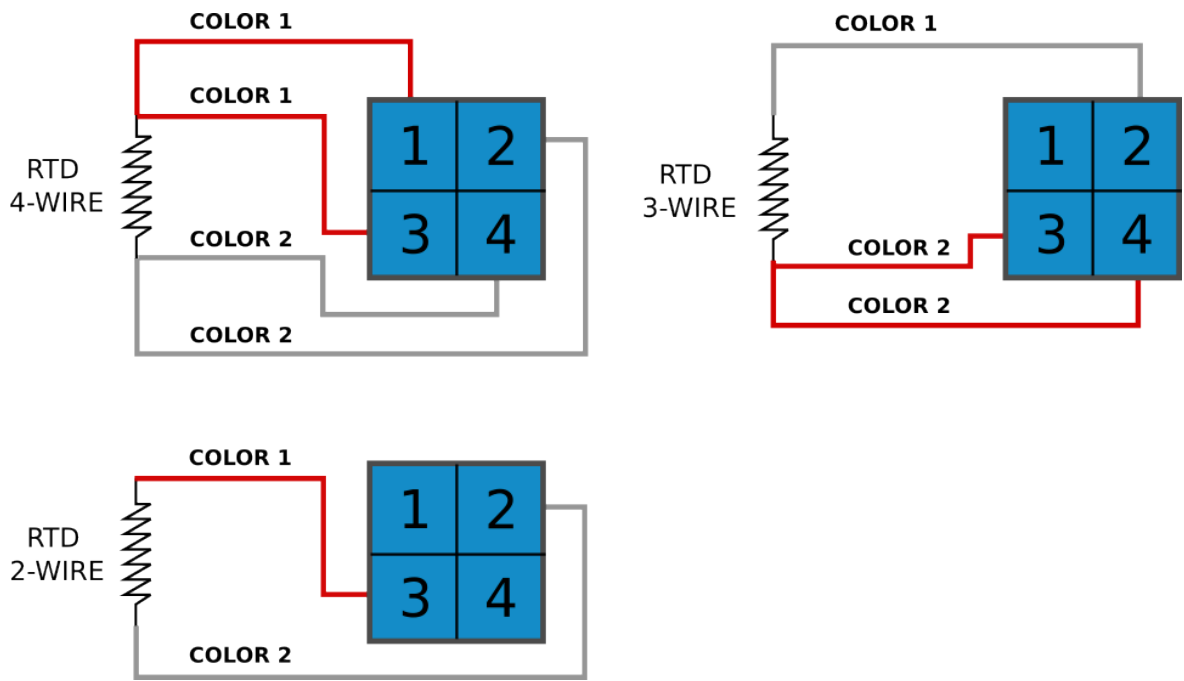
Figure. 7.5.4 - 259. RTD sensor connection types.
