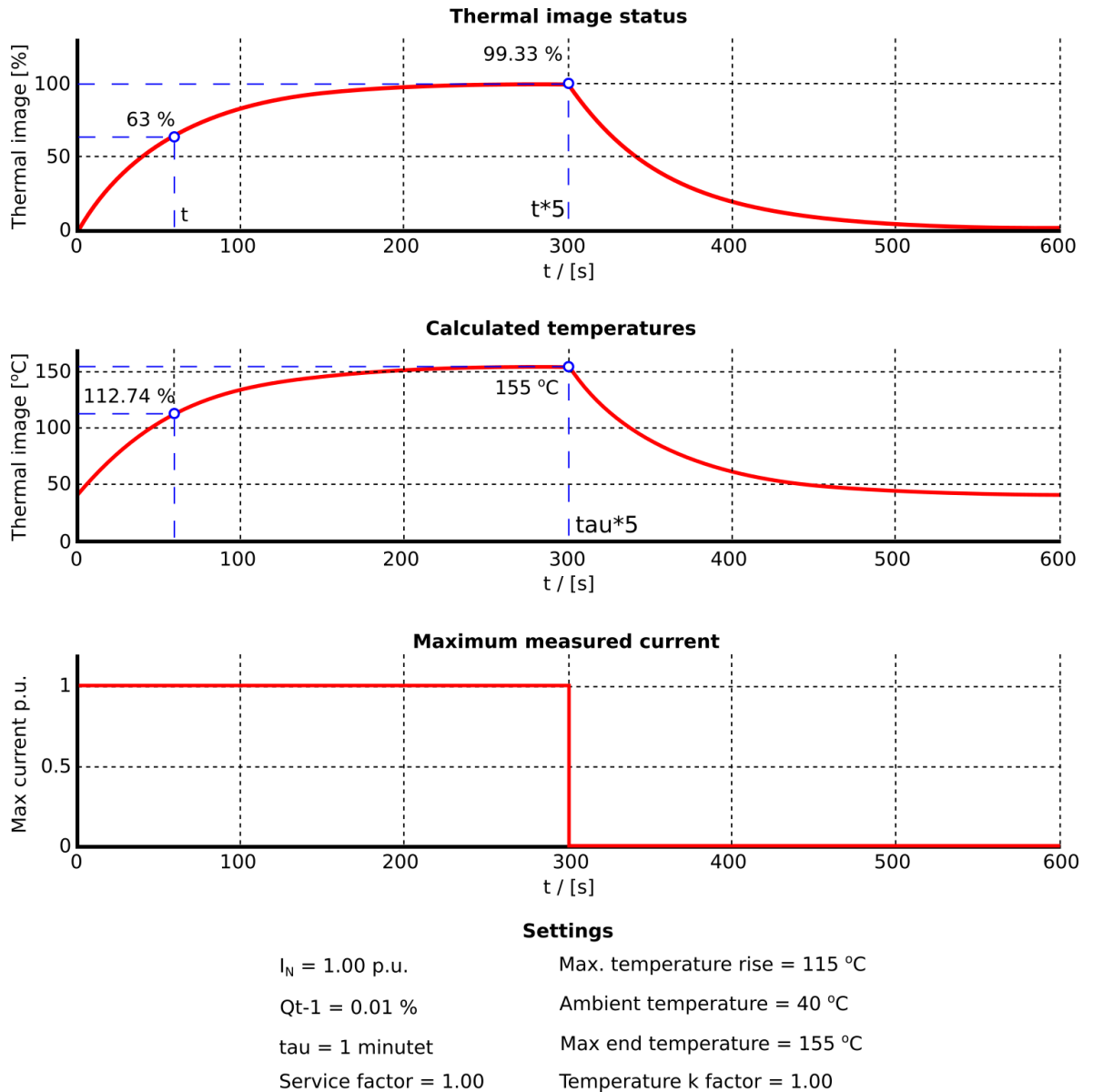
Figure. 4.4.22 - 165. Example of thermal image calculation with nominal conditions.
