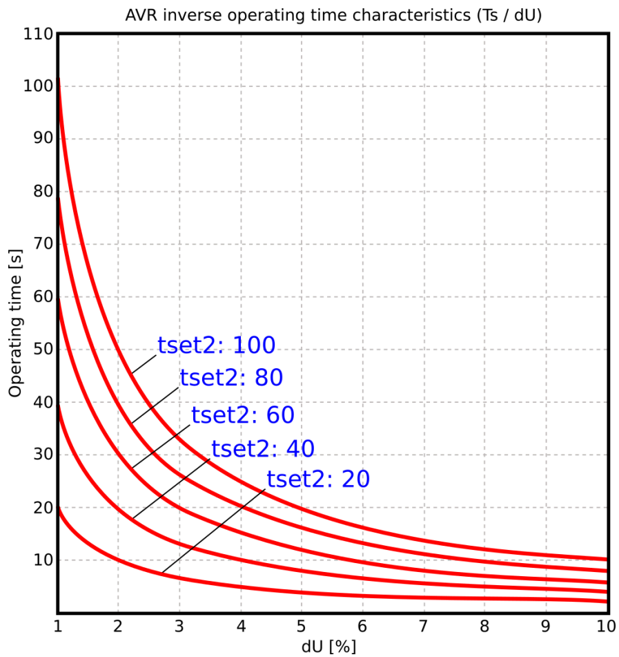
Figure. 4.5.2 - 184. Inverse operating time characteristics for the second voltage window ( U > / < U_{window} ).
