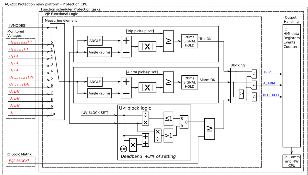
Figure. 4.5.9 - 215. Simplified function block diagram of the \Delta\phi function.
