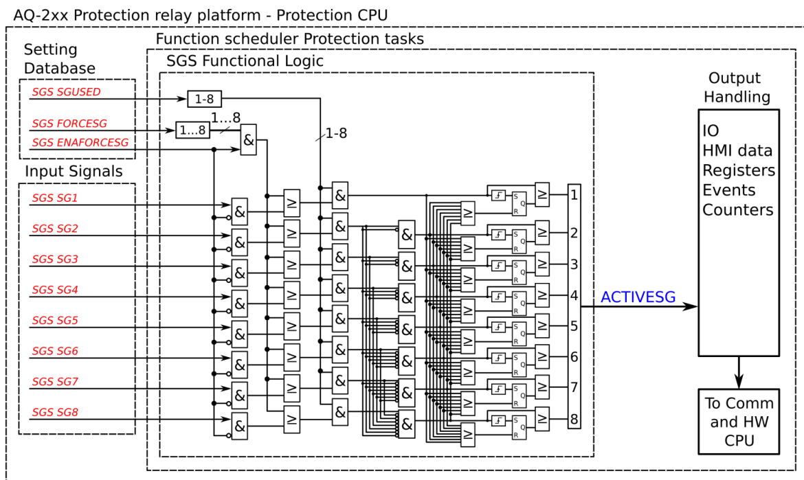
Figure. 4.5.3 - 189. Simplified function block diagram of the setting group selection function.
