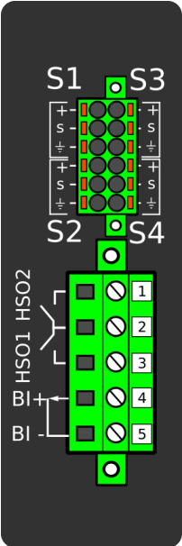
Figure. 7.5.3 - 257. Arc protection module.
