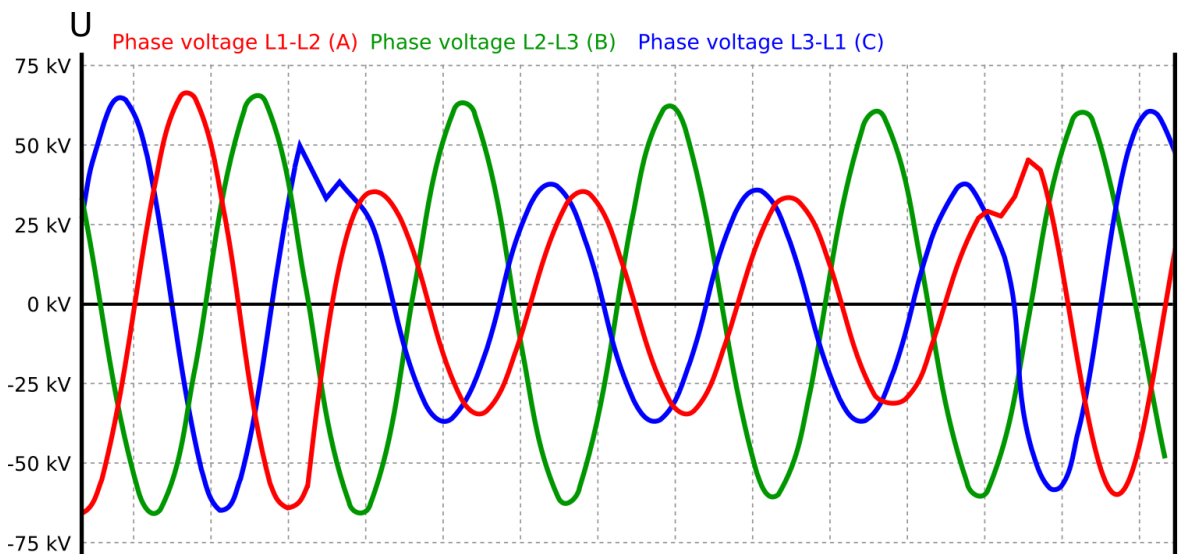
Figure. 4.5.9 - 216. Generator islanding.
