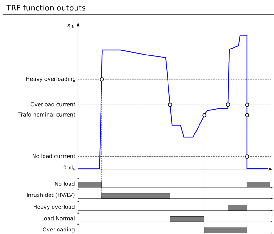
Figure. 4.4.21 - 164. Activation of the function's outputs.
