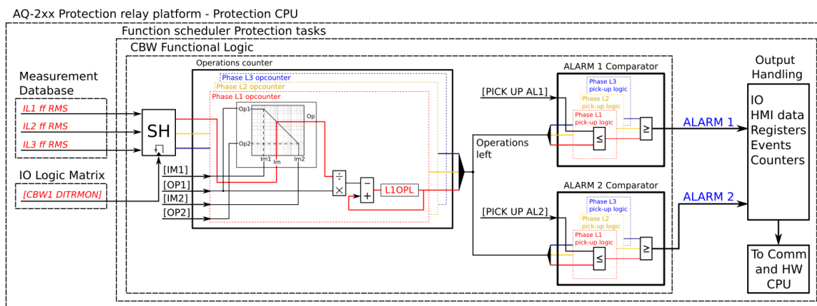
Figure. 4.6.3 - 235. Simplified function block diagram of the circuit breaker wear function.
