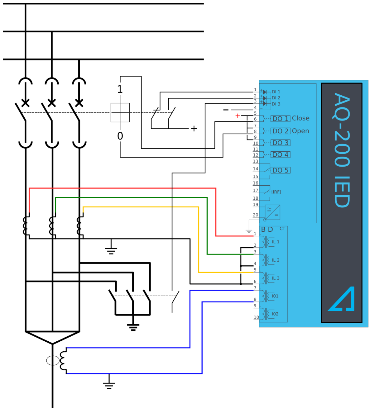
Figure. 4.5.4 - 196. Example of an interlock application.
