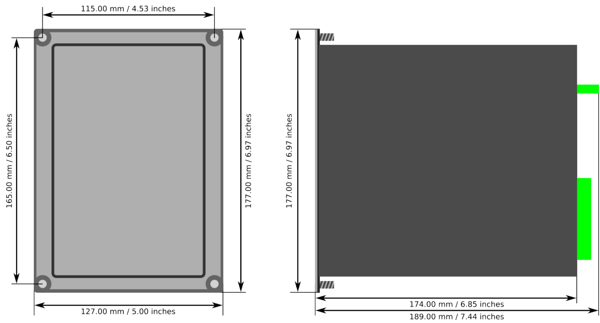
Figure. 7.6 - 267. Device dimensions.
