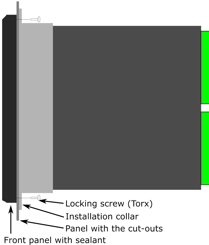
Figure. 7.4 - 45. Device installation.
