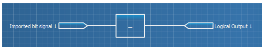
Figure. 5.5 - 25. To report imported bit signals to SCADA the signals must be connected to a logical output.
