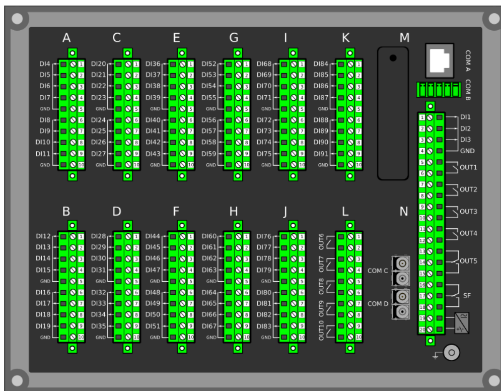
Figure. 7.1 - 30. Modular construction of AQ-X254-XXXXXX-BBBBBBBBBBBBCAJ
