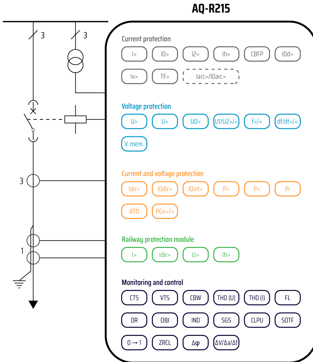
Figure. 6.1 - 254. AQ-R215 application example with function block diagram.
