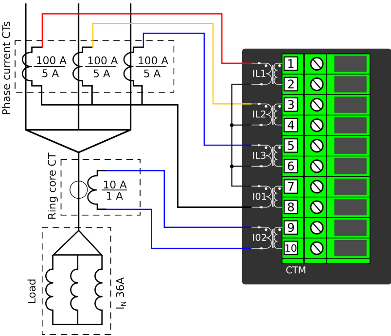
Figure. 4.2.1 - 58. Connections.
