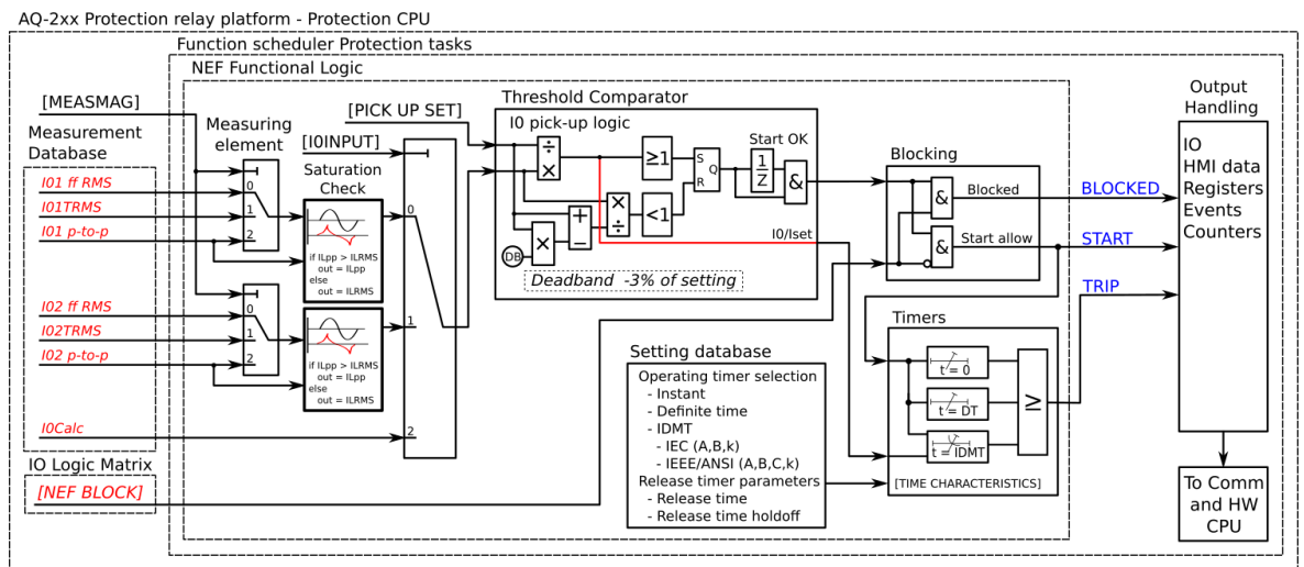
Figure. 4.4.4 - 93. Simplified function block diagram of the I0&gt; function.
