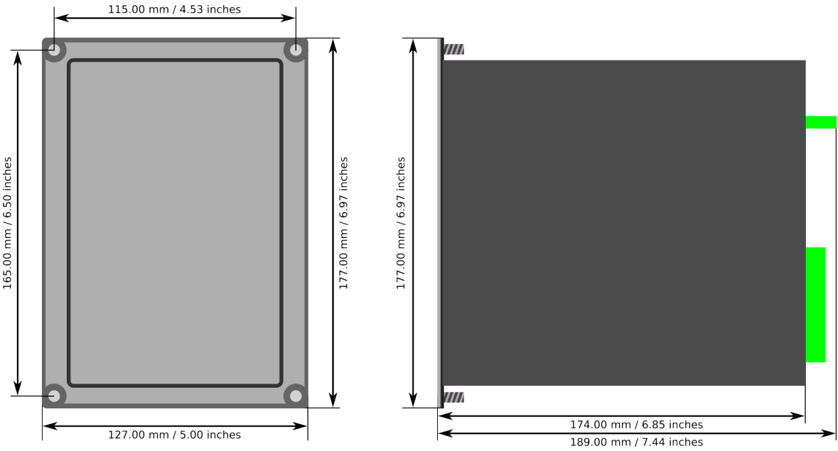
Figure. 7.6 - 279. Device dimensions.
