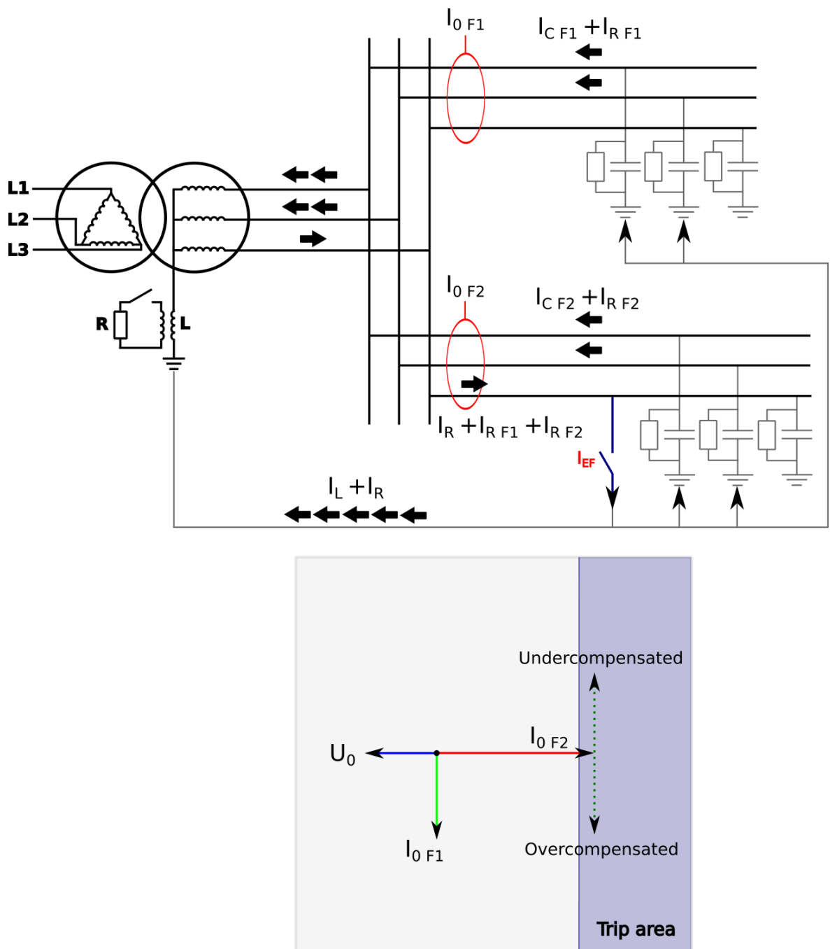
Figure. 4.4.6 - 100. Angle tracking of I_{0dir} function (Petersen coil earthed network model).
