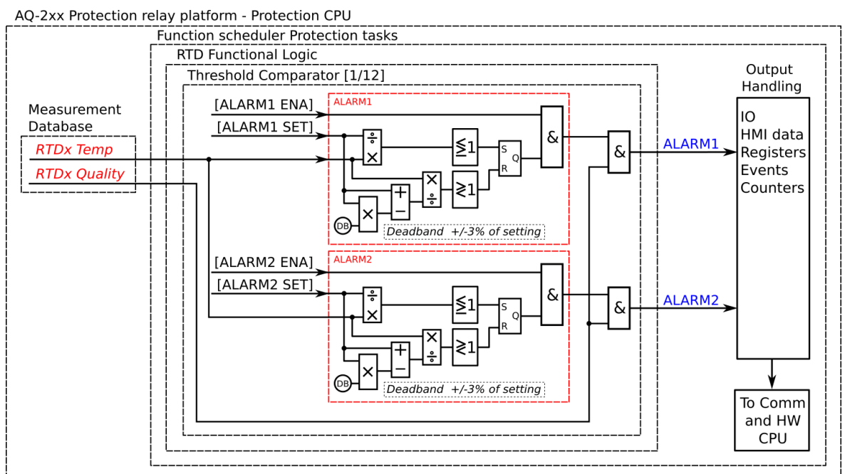
Figure. 4.4.22 - 178. Simplified function block diagram of the resistance temperature detection function.
