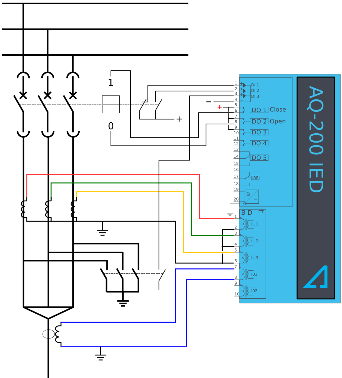
Figure. 4.5.3 - 189. Example of an interlock application.
