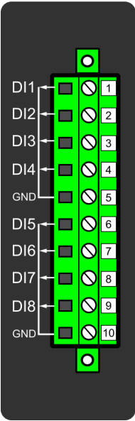
Figure. 7.5.1 - 266. Digital input module (DI8) with eight add-on digital inputs.
