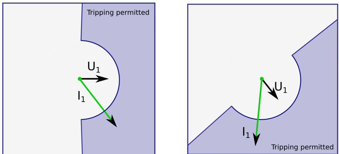
Figure. 4.4.5 - 95. Angle tracking of the I_{dir}> function (3LN/3LL + U_0 mode).
