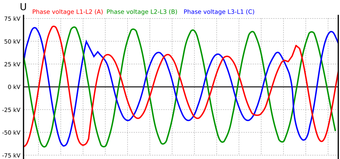
Figure. 4.5.10 - 228. Generator islanding.
