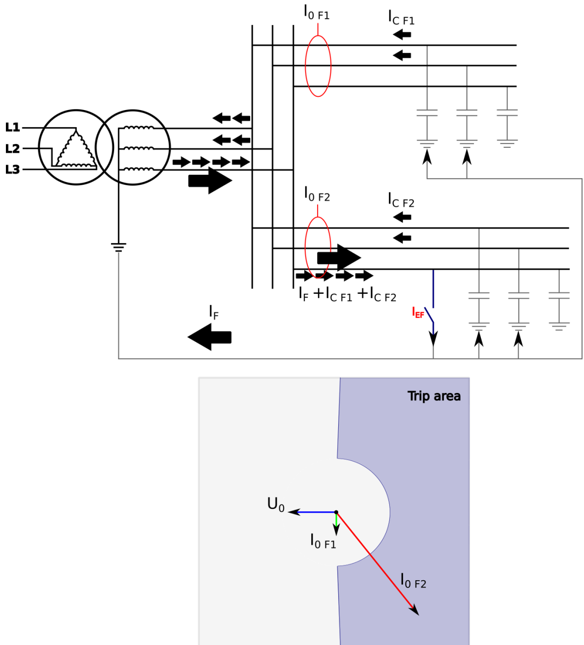
Figure. 4.4.6 - 101. Angle tracking of I_{0dir} function (directly earthed or small impedance network).
