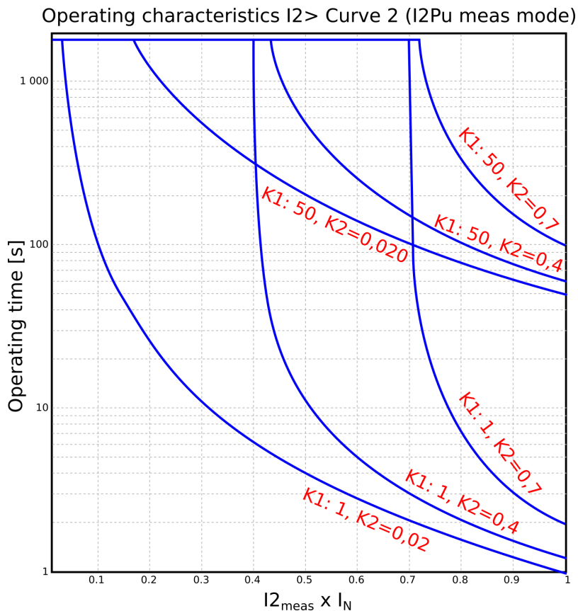
Figure. 4.4.8 - 109. Operation characteristics curve for I2> Curve2.
