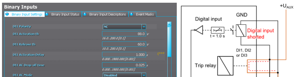
Figure. 6.3 - 257. Settings for a digital input used for trip circuit supervision.
