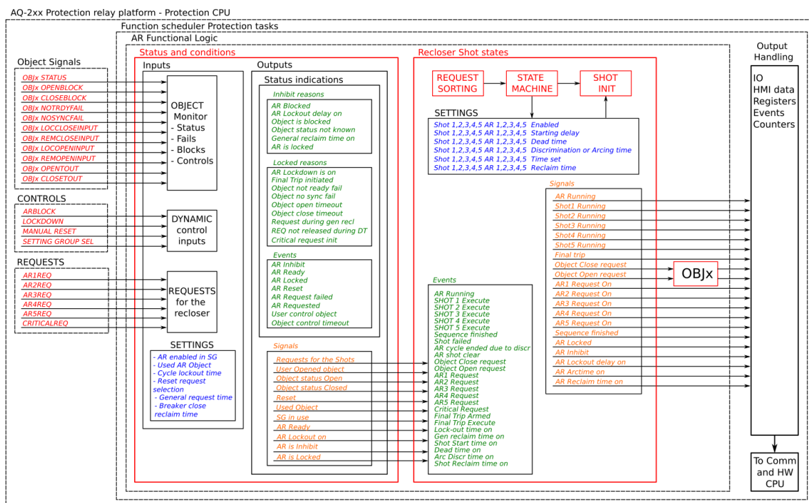
Figure. 4.5.5 - 206. Simplified function block diagram of the auto-recloser function.
