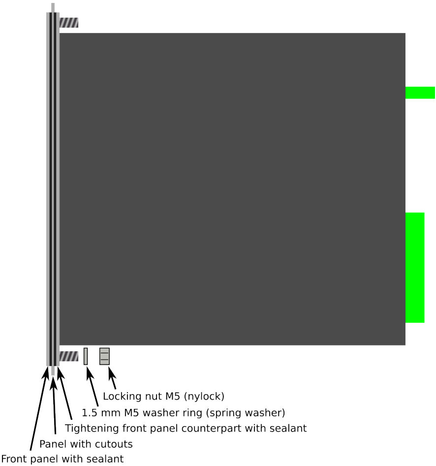
Figure. 7.6 - 280. Device installation.
