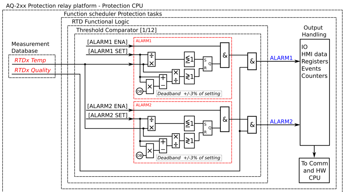
Figure. 4.4.15 - 139. Simplified function block diagram of the resistance temperature detection function.
