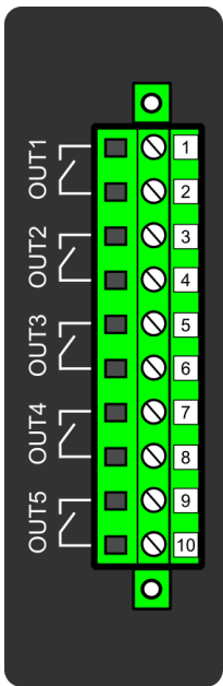
Figure. 7.4.2 - 195. Digital output module (DO5) with five add-on digital outputs.
