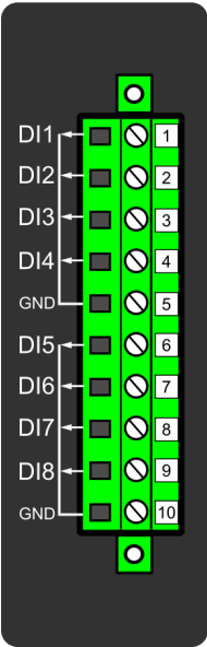
Figure. 7.4.1 - 193. Digital input module (DI8) with eight add-on digital inputs.
