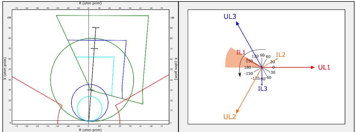
Figure. 4.2.2 - 74. Distance protection characteristics and directional overcurrent.
