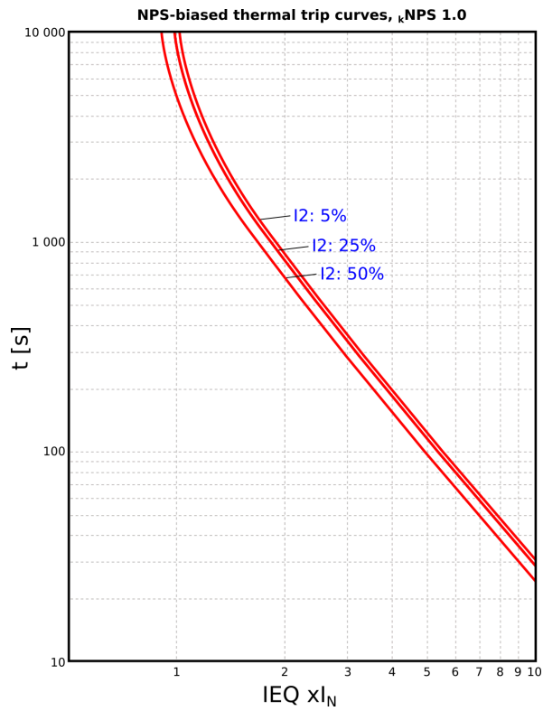
Figure. 4.4.17 - 163. NPS-biased thermal trip curves with k_{NPS} value of 1.
