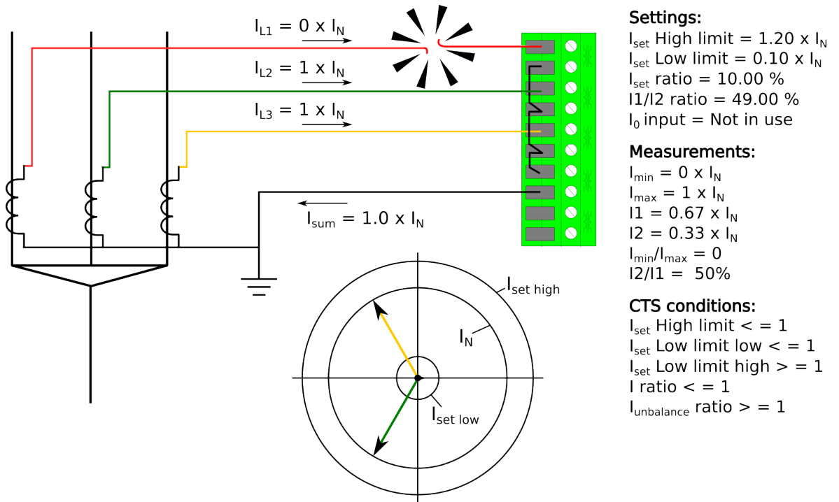
Figure. 4.6.1 - 212. Secondary circuit fault in phase L1 wiring.
