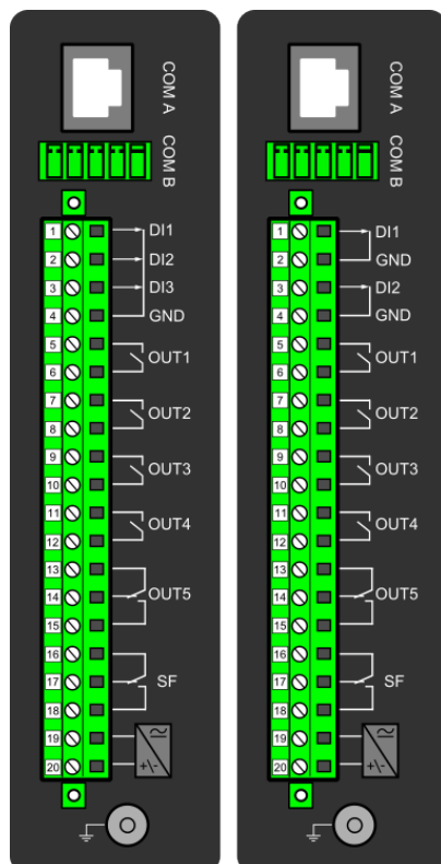
Figure. 7.2 - 240. CPU module.
