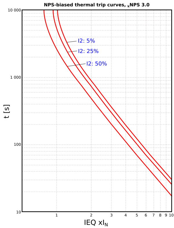
Figure. 4.4.17 - 164. NPS-biased thermal trip curves with k_{NPS} value of 3.
