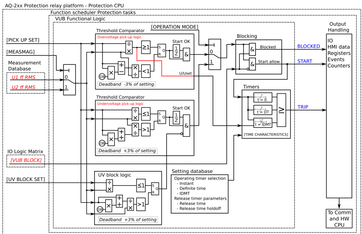
Figure. 4.4.14 - 148. Simplified function block diagram of the U1/U2&gt;/&lt; function.
