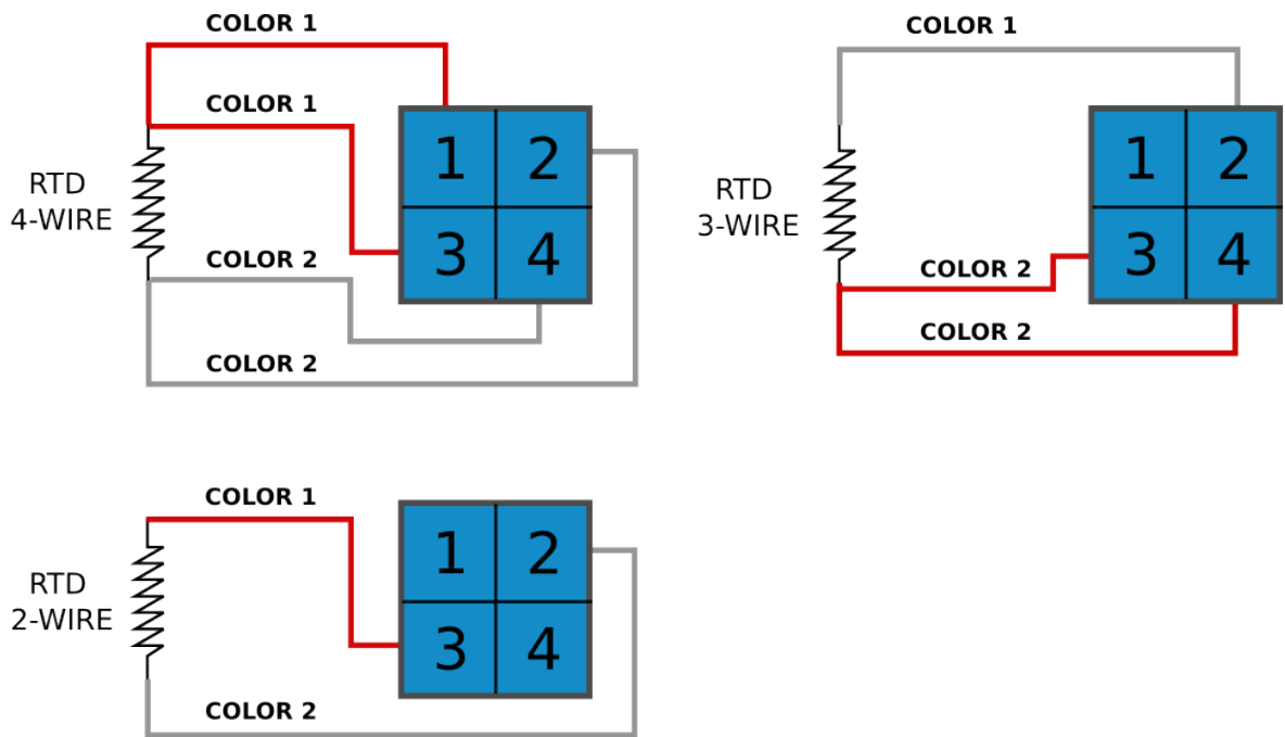
Figure. 7.5.4 - 271. RTD sensor connection types.
