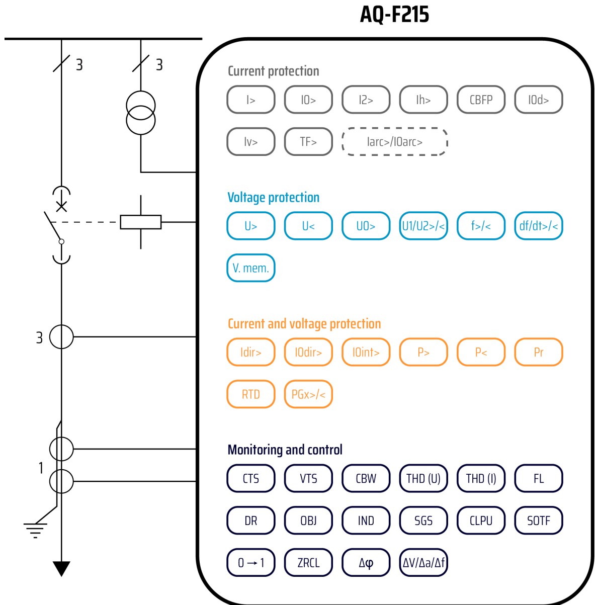
Figure. 6.1 - 253. AQ-F215 application example with function block diagram.
