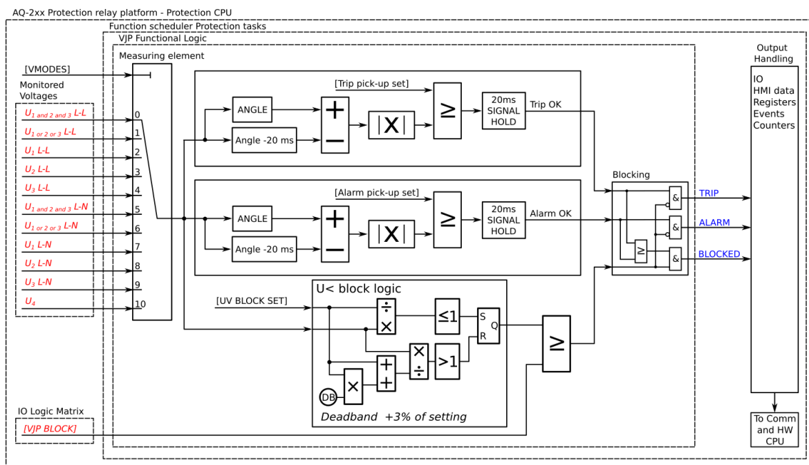
Figure. 4.5.11 - 226. Simplified function block diagram of the \Delta\phi function.
