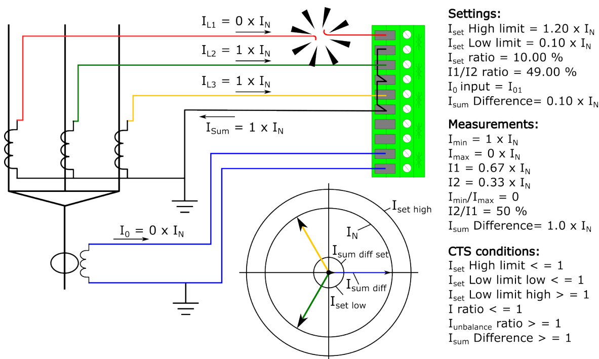
Figure. 4.6.1 - 240. Broken secondary phase current wiring.
