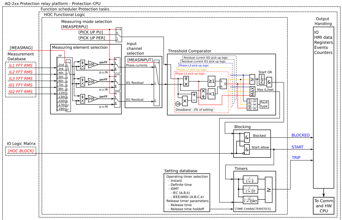
Figure. 4.4.8 - 106. Simplified function block diagram of the Ih> function.
