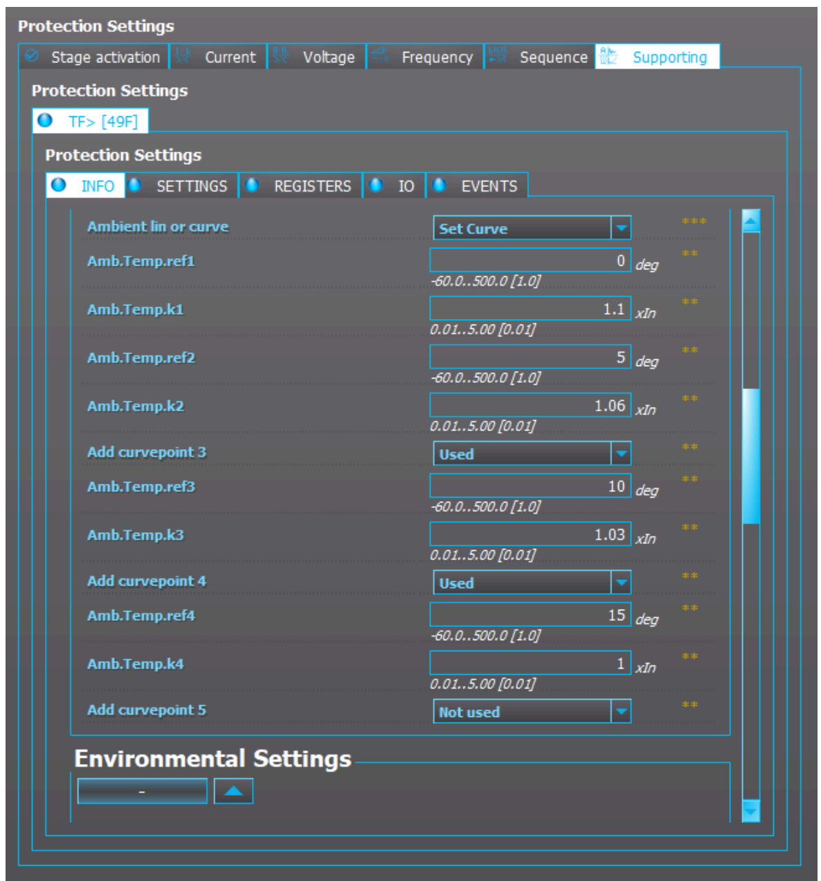
Figure. 4.4.21 - 166. Settings of the function's ambient temperature coefficient curve.
