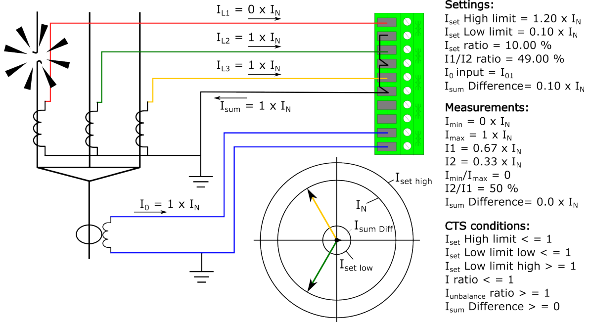
Figure. 4.6.1 - 241. Broken primary phase current wiring.
