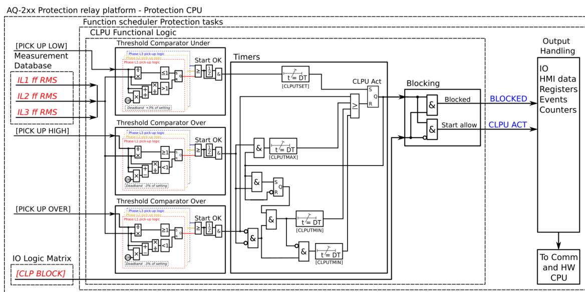
Figure. 4.5.7 - 207. Simplified function block diagram of the cold load pick-up function.
