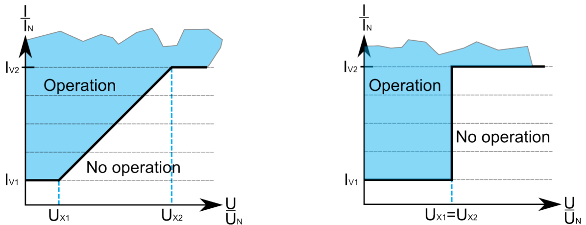
Figure. 4.4.20 - 161. Pick-up levels in the two modes.
