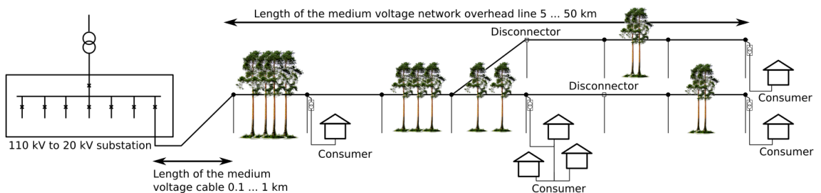
Figure. 4.5.5 - 188. Diagram of a typical radial medium-voltage network in rural areas.
