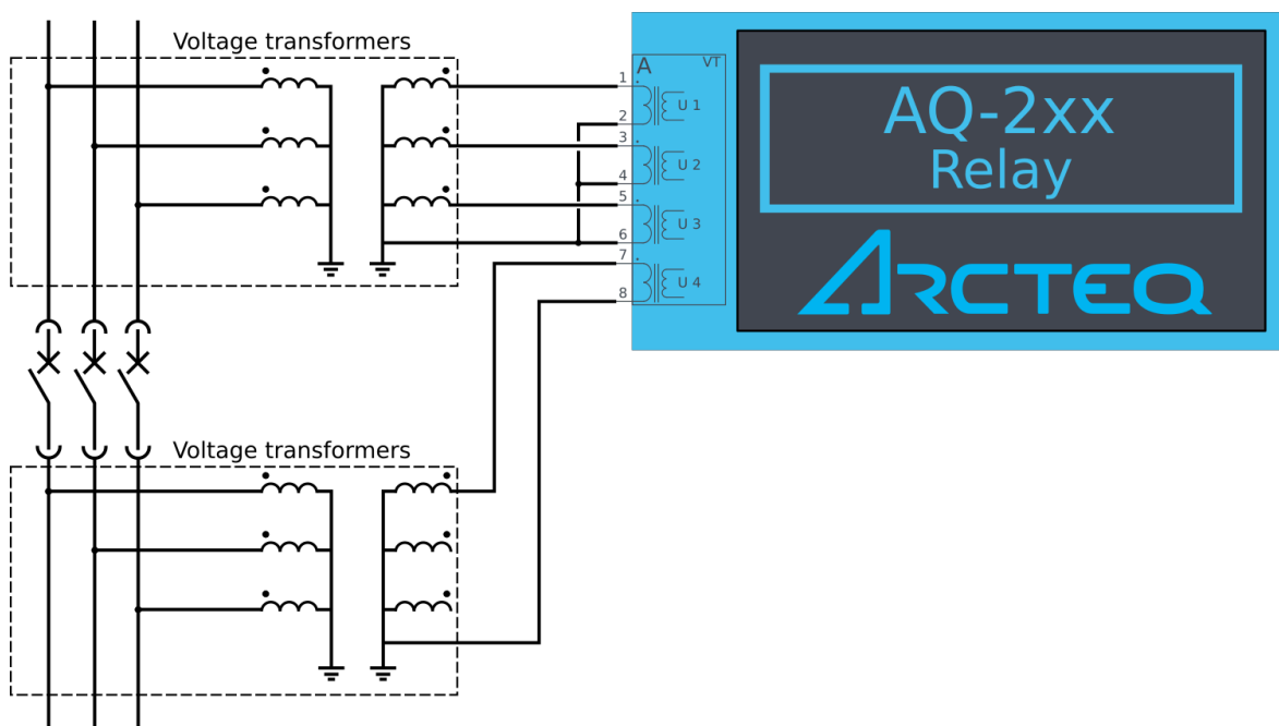
Figure. 4.5.9 - 215. Example connection of the synchrocheck function (3LN+U4 mode, SYN1 in use, UL1 as reference voltage).
