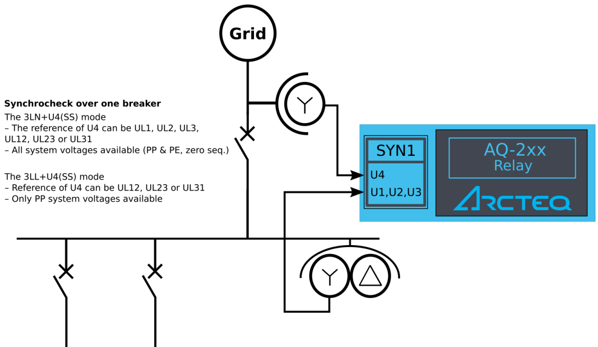
Figure. 4.5.9 - 218. Example application (synchrocheck over one breaker, with 3LL and 3LN VT connections).
