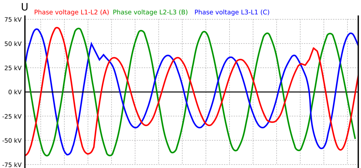
Figure. 4.5.11 - 227. Generator islanding.
