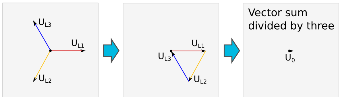
Figure. 4.4.13 - 138. Normal situation.
