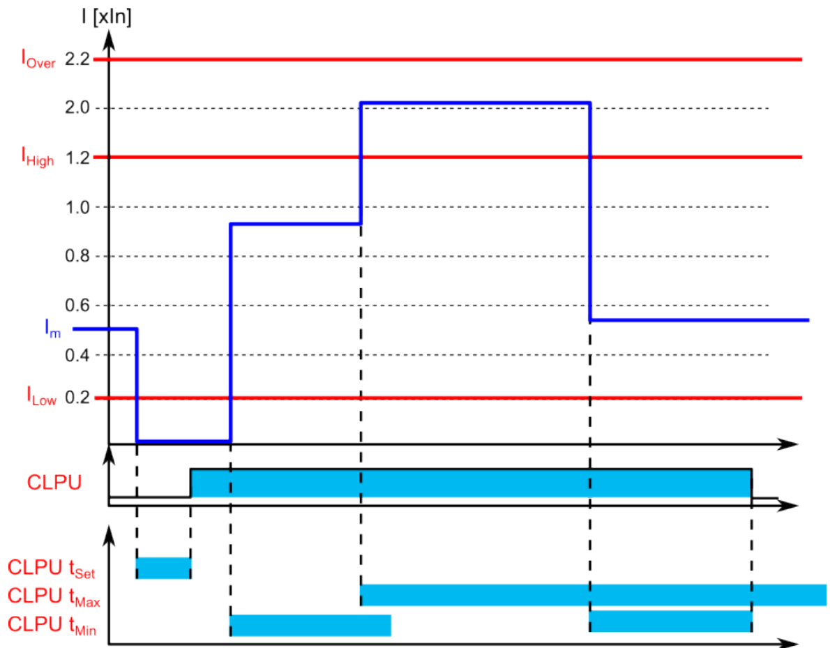
Figure. 4.5.7 - 213. Example of timers and pick-up parameters (an inrush current detected during T_{min} time).
