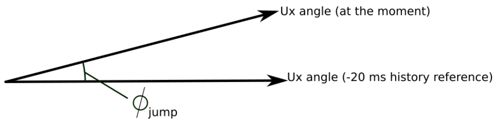
Figure. 4.5.11 - 228. Vector jump from the function's point of view.
