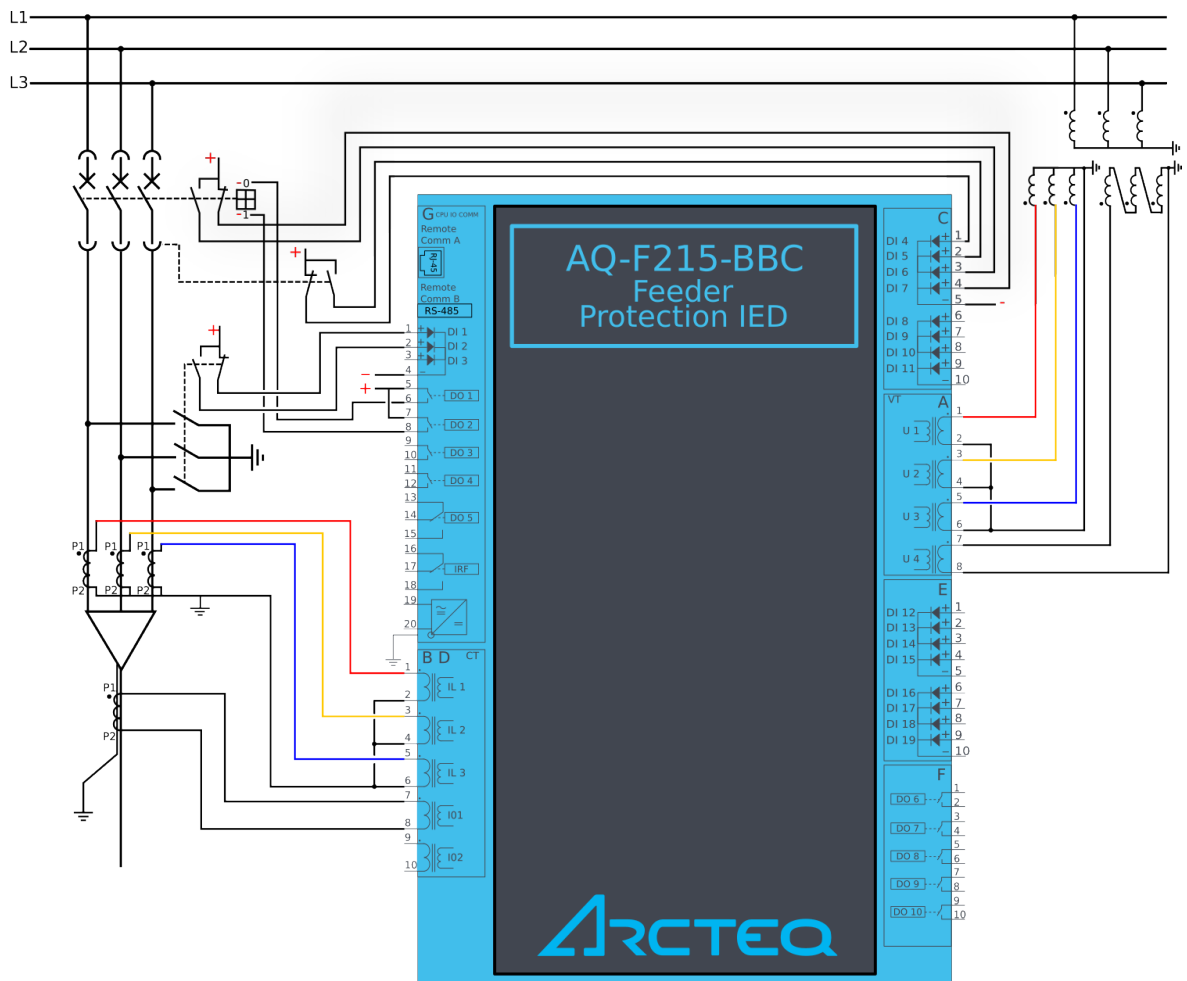
Figure. 6.2 - 254. Application example and its connections.
