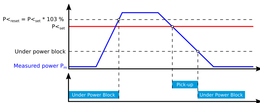
Figure. 4.4.18 - 158. Activation and deactivation characteristics of low power blocking.
