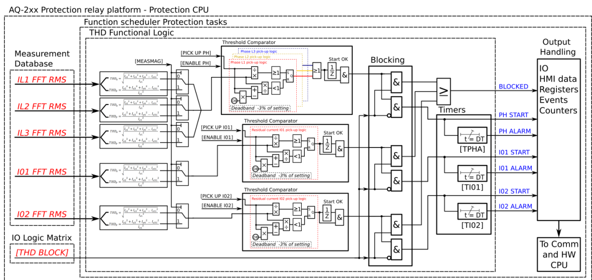
Figure. 4.6.4 - 248. Simplified function block diagram of the total harmonic distortion monitor function.
