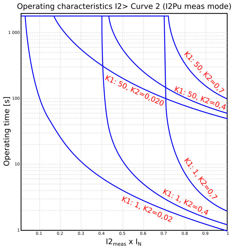
Figure. 4.4.7 - 105. Operation characteristics curve for I2> Curve2.
