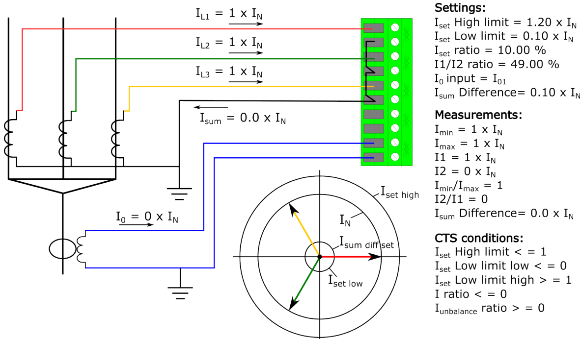
Figure. 4.6.1 - 239. Normal situation, residual current also measured.
