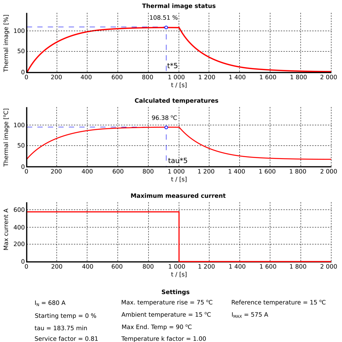
Figure. 4.4.21 - 173. Thermal image response with nominal currents and fine-tuned k_{SF} correction factor.
