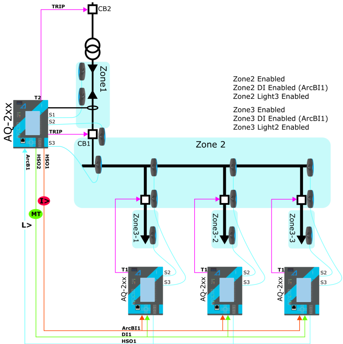
Figure. 4.4.24 - 179. Scheme with AQ-200 protection devices.
