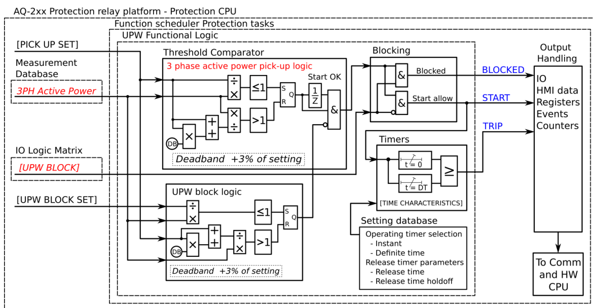
Figure. 4.4.18 - 157. Simplified function block diagram of the P&lt; function.
