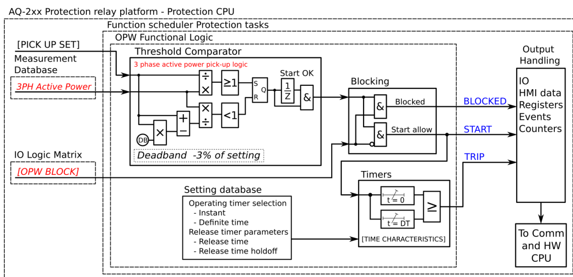
Figure. 4.4.17 - 155. Simplified function block diagram of the P> function.
