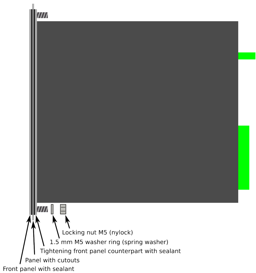
Figure. 7.5 - 200. Device installation.
