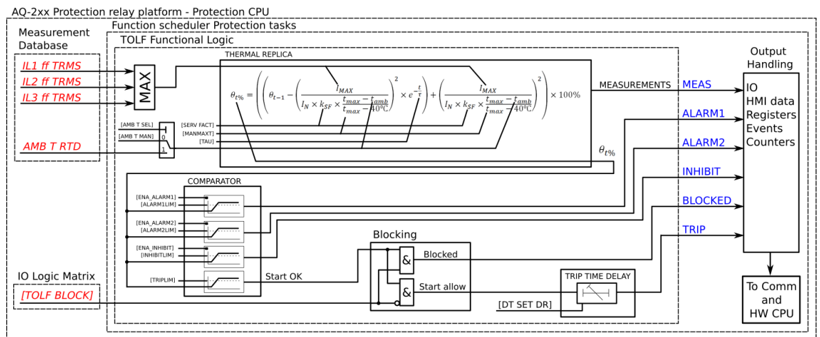
Figure. 4.4.8 - 112. Simplified function block diagram of the TF> function.
