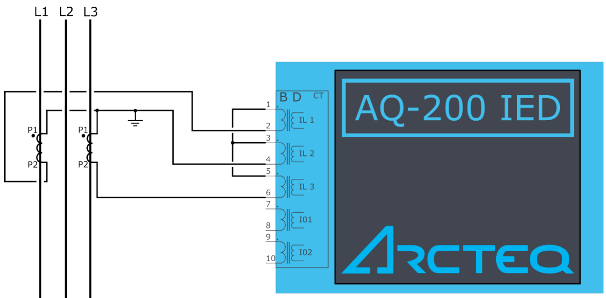
Figure. 6.3 - 176. ARON connection.
