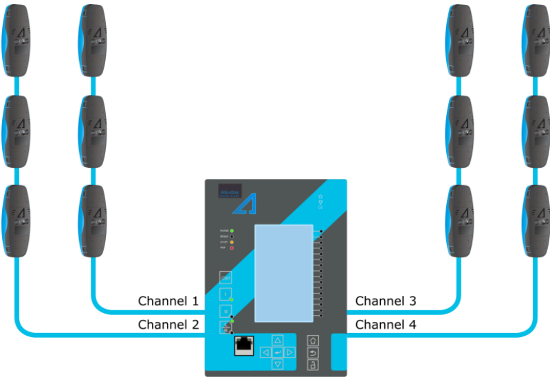
Figure. 4.4.11 - 114. Protection device equipped with arc protection.
