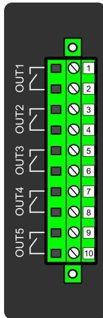
Figure. 7.5.2 - 192. Digital output module (DO5) with five add-on digital outputs.
