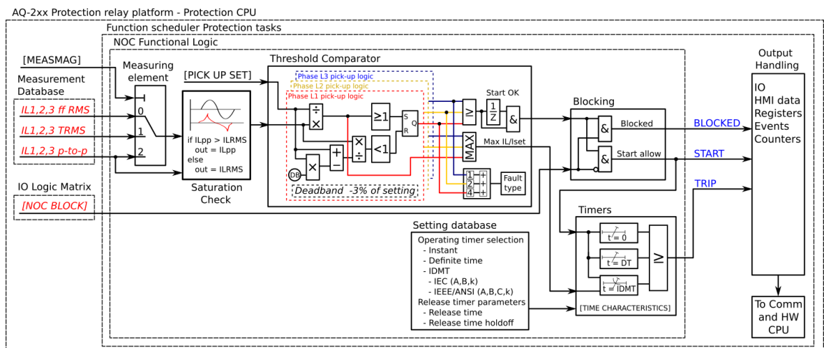
Figure. 4.4.4 - 90. Simplified function block diagram of the I > function.
