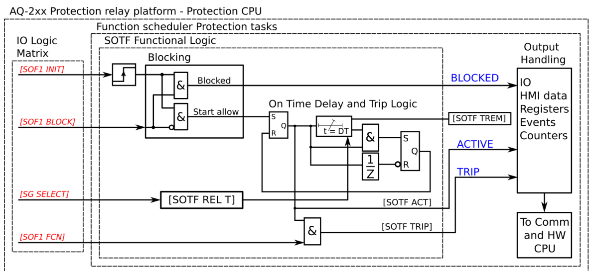
Figure. 4.5.5 - 152. Simplified function block diagram of the switch-on-to-fault function.
