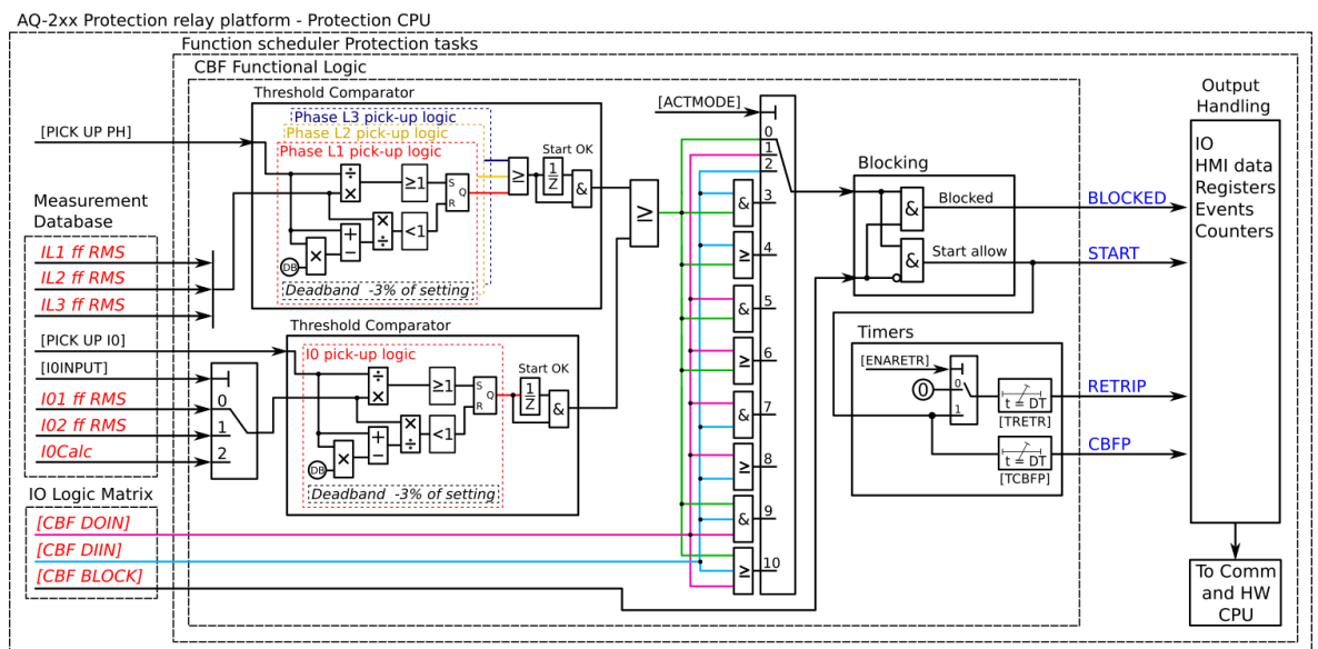
Figure. 4.4.8 - 95. Simplified function block diagram of the CBFP function.
