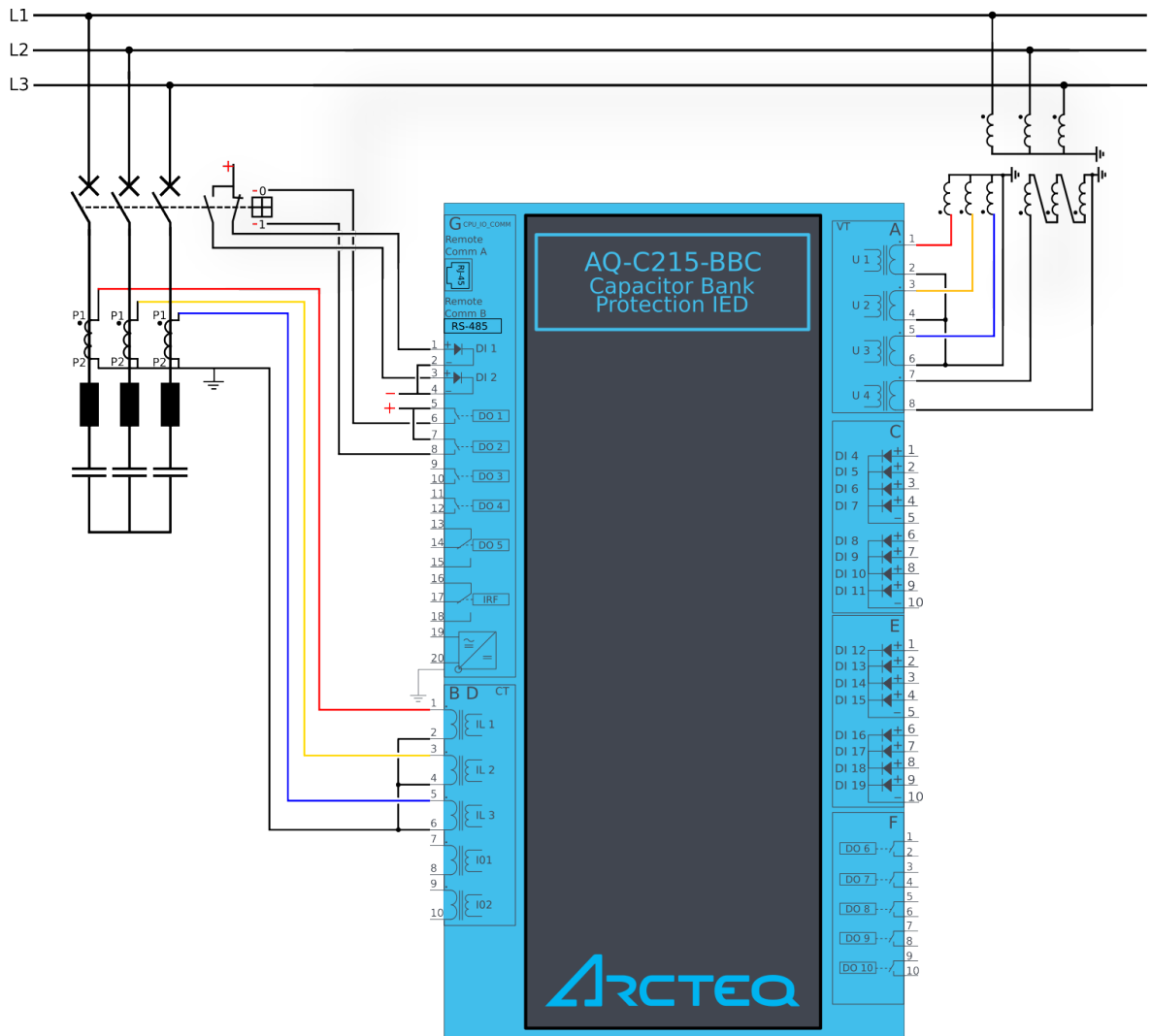
Figure. 6.2 - 177. Application example and its connections.
