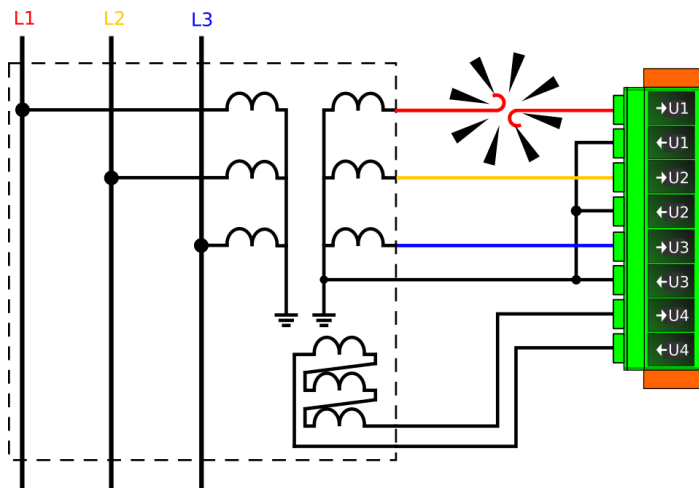
Figure. 4.6.2 - 168. Secondary circuit fault in phase L1 wiring.
