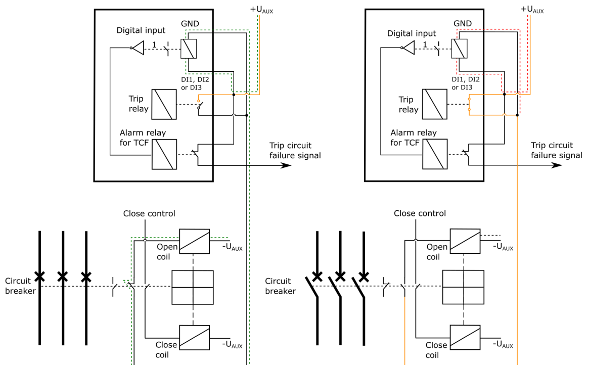
Figure. 6.4 - 183. Trip circuit supervision with one DI and one latched output contact.
