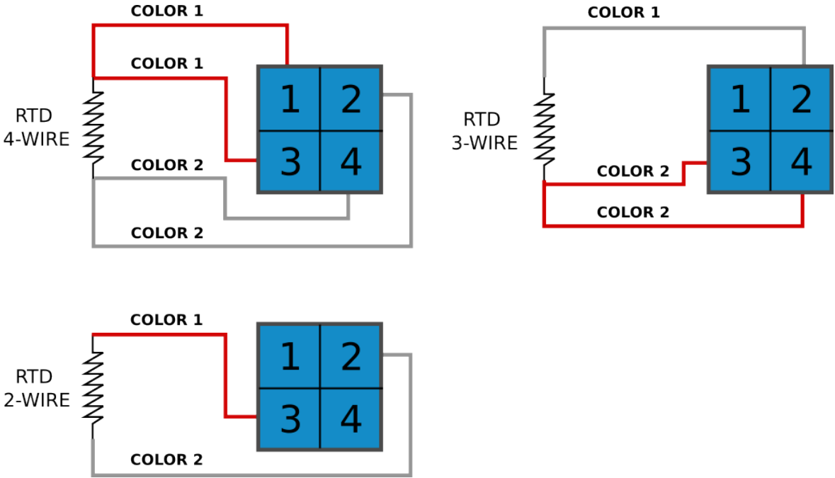
Figure. 7.5.4 - 195. RTD sensor connection types.
