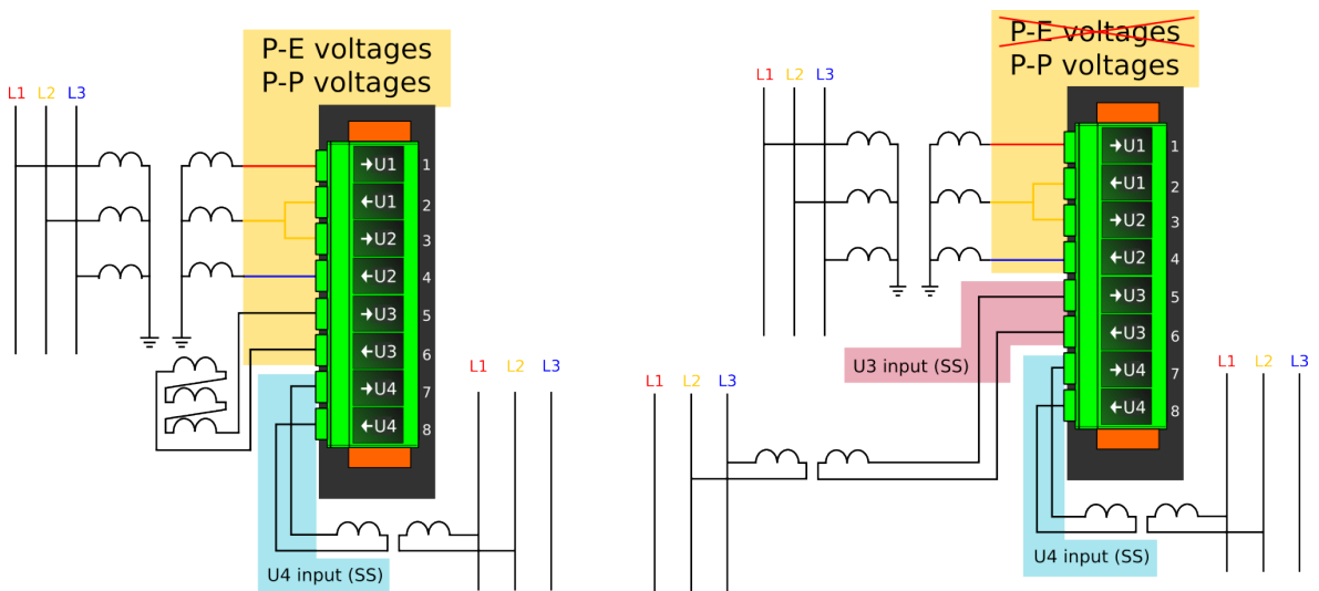
Figure. 4.4.10 - 113. Selectable measurement magnitudes with 2LL+U4 VT connection (P-E voltages not available without residual voltage).
