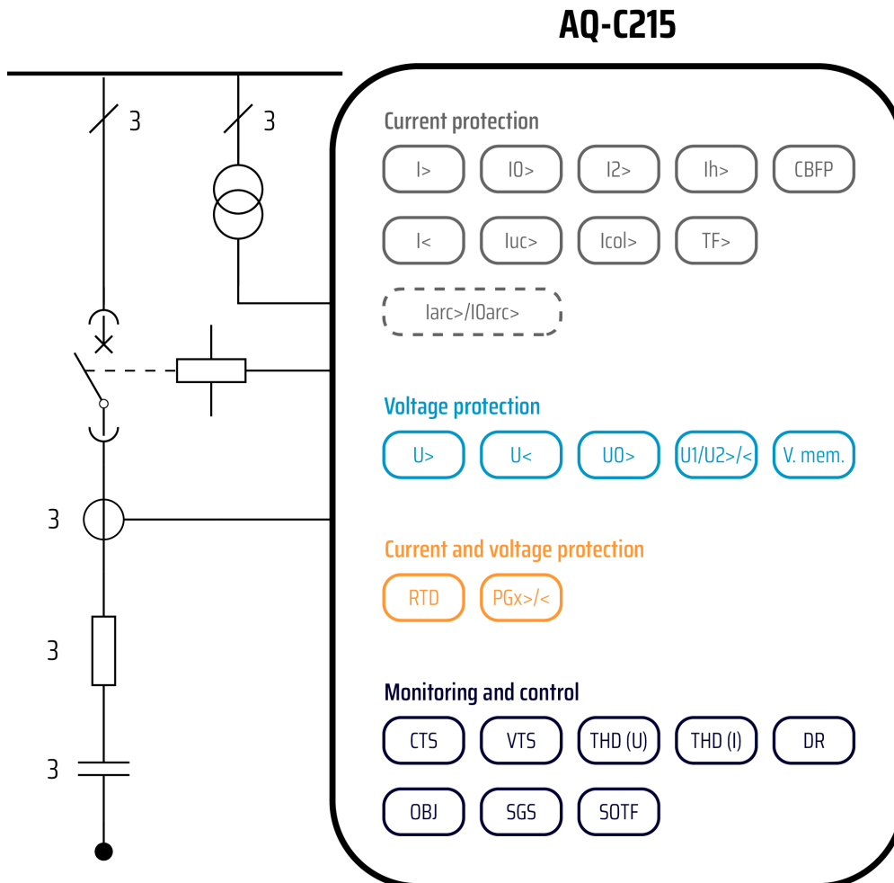
Figure. 6.1 - 176. AQ-C215 application example with function block diagram.
