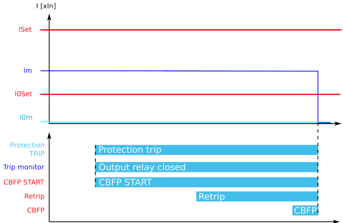
Figure. 4.4.8 - 99. Retrip and CBFP when "Current or DO" is the selected criterion.
