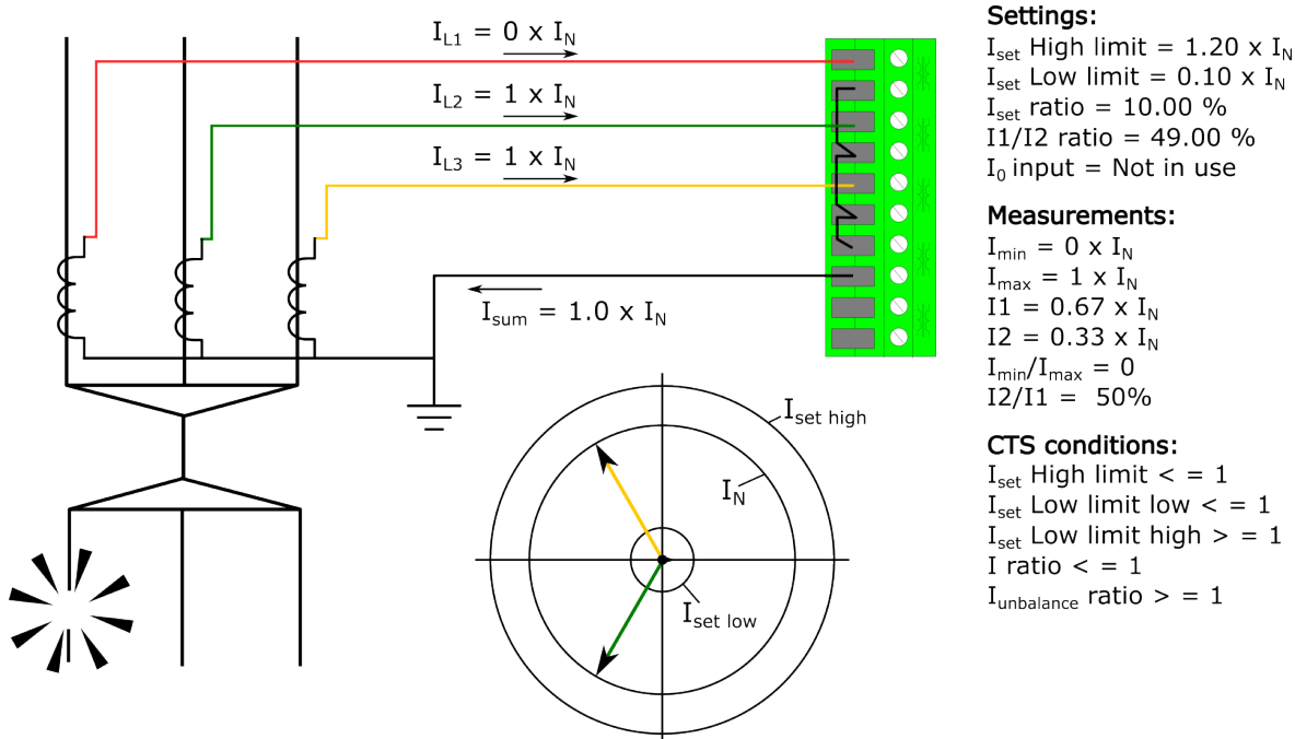
Figure. 4.6.1 - 161. Primary circuit fault in phase L1 wiring.
