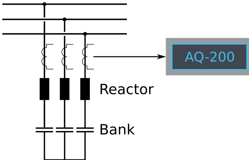
Figure. 4.4.3 - 89. Measurement connection of the luc&gt; function.
