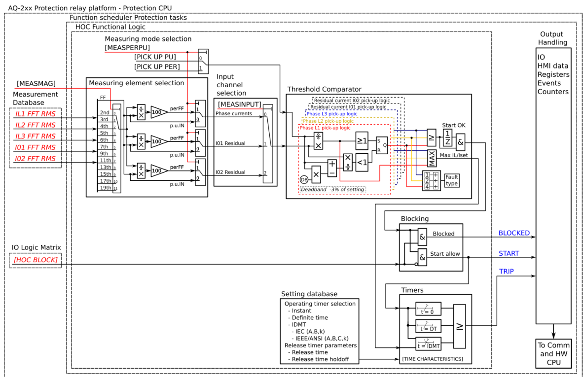
Figure. 4.4.7 - 94. Simplified function block diagram of the lh> function.
