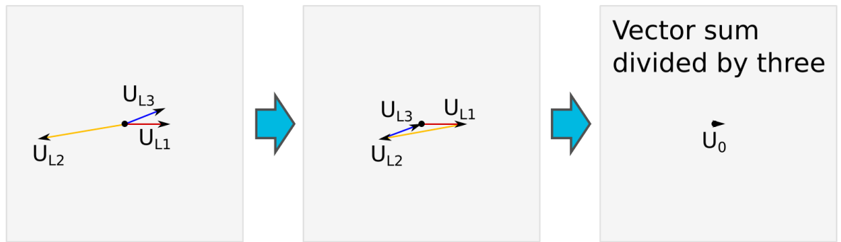
Figure. 4.4.11 - 117. Close-distance short-circuit between phases 1 and 3.
