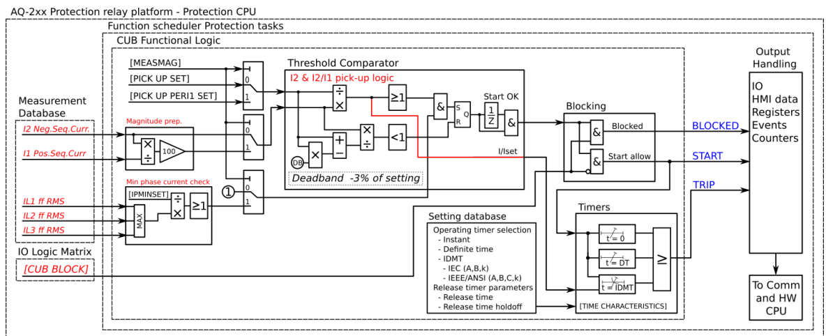
Figure. 4.4.6 - 92. Simplified function block diagram of the I_{2>} function.
