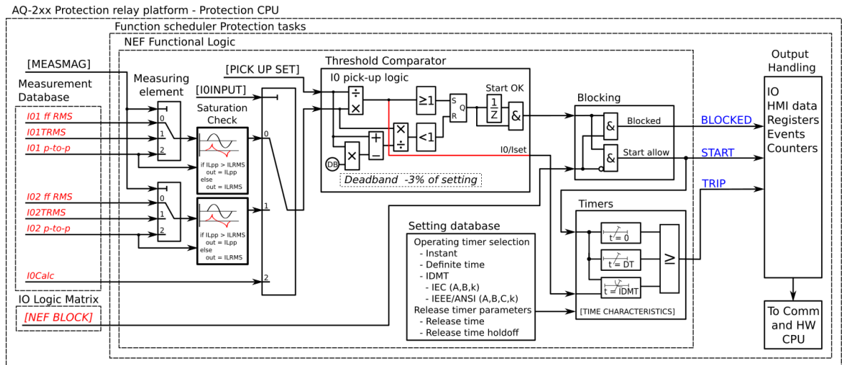
Figure. 4.4.5 - 91. Simplified function block diagram of the I_{0>} function.
