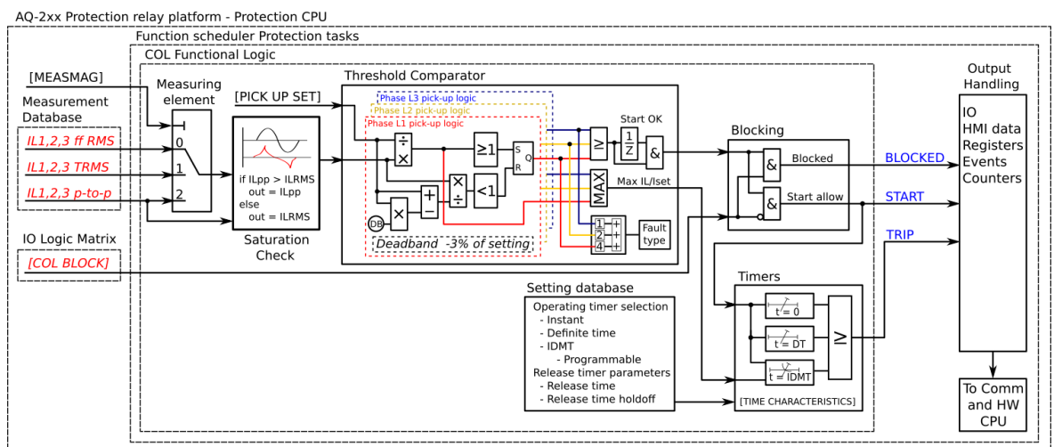
Figure. 4.4.2 - 88. Simplified function block diagram of the Icol> function.
