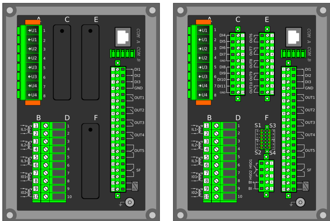
Figure. 7.1 - 185. Modular construction of AQ-X215.
