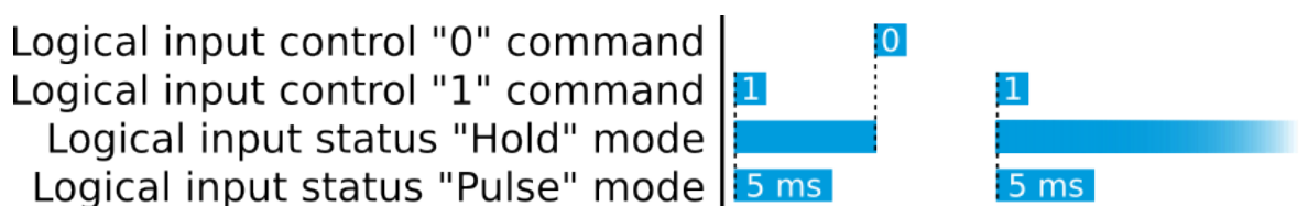
Figure. 4.5.10 - 155. Operation of logical input in "Hold" and "Pulse" modes.
