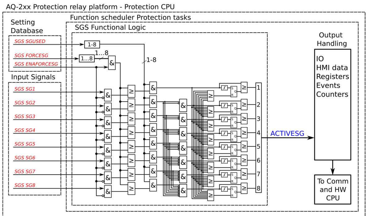
Figure. 4.5.2 - 144. Simplified function block diagram of the setting group selection function.
