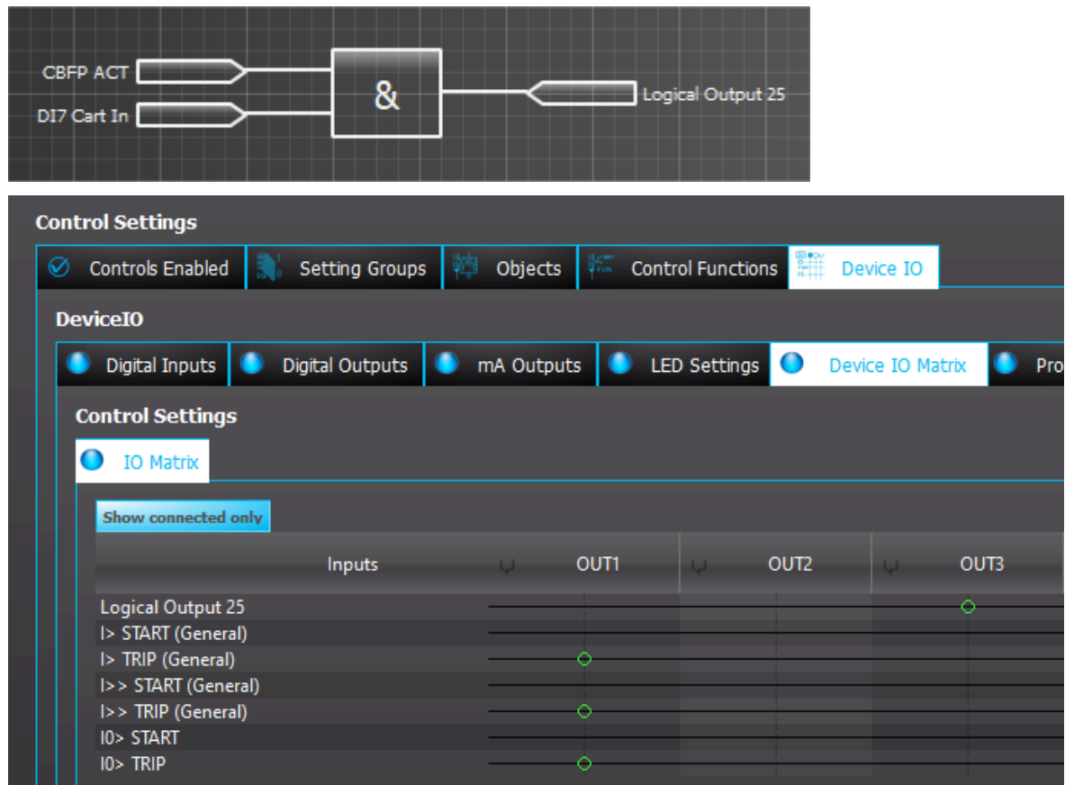
Figure. 4.5.9 - 154. Logic output example. Logical output is connected to an output relay in matrix.
