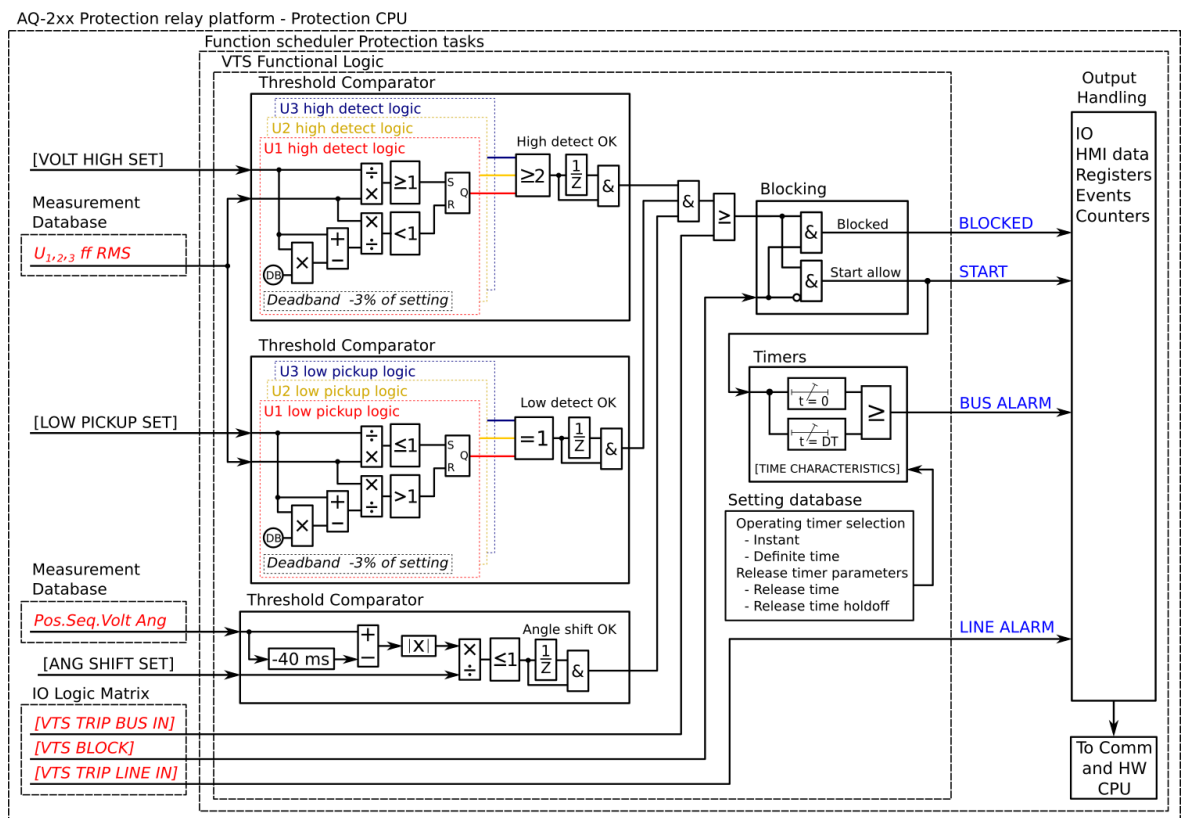
Figure. 4.6.2 - 169. Simplified function block diagram of the VTS function.
