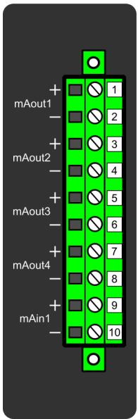
Figure. 7.5.9 - 202. Milliampere output (mA) I/O module connections.
