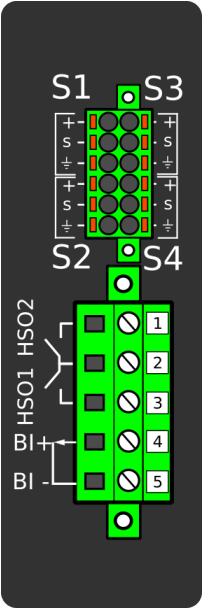
Figure. 7.5.3 - 193. Arc protection module.
