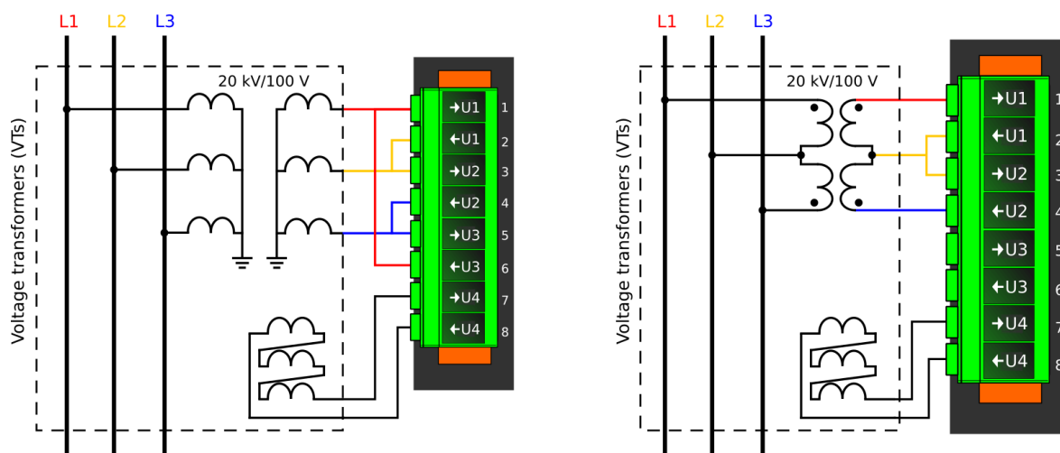
Figure. 4.2.2 - 70. Example connections for voltage line-to-line measurement.
