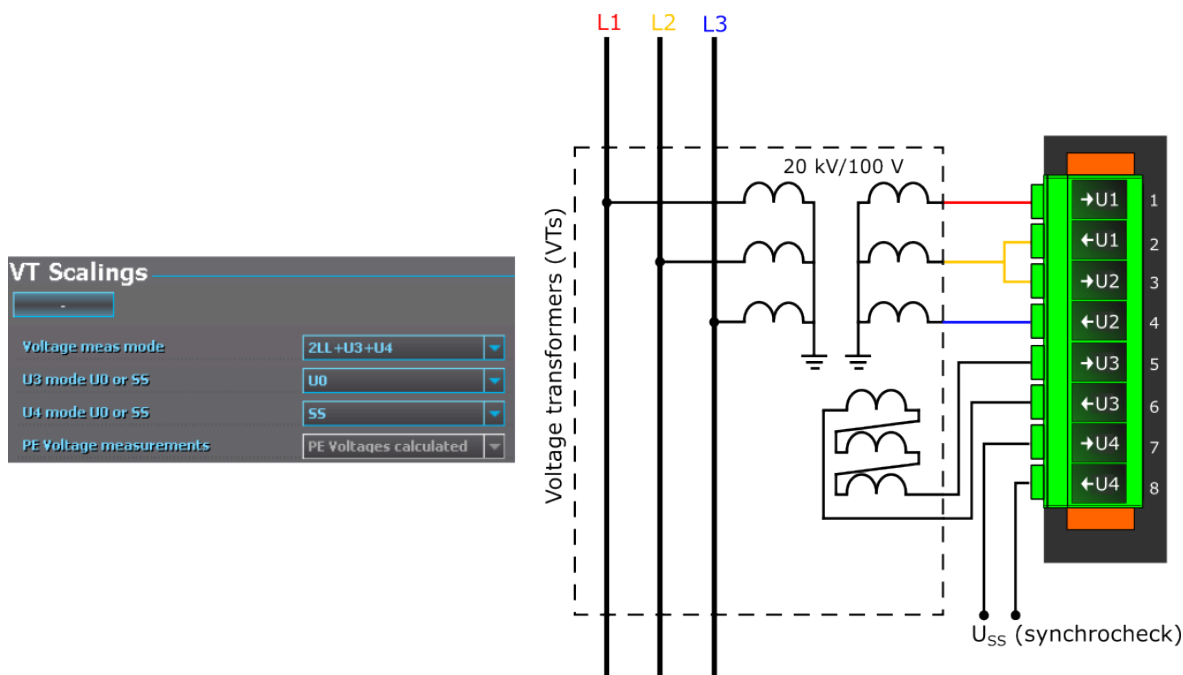
Figure. 4.2.2 - 71. 2LL+U_0+SS settings and connections.
