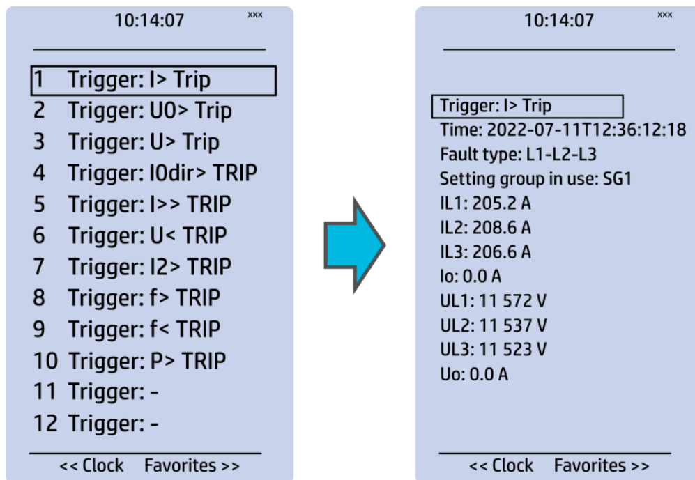
Figure. 4.6.7 - 175. 12 latest recordings can be accessed from HMI if "Fault registers" view has been enabled in "Carousel designer" tool.
