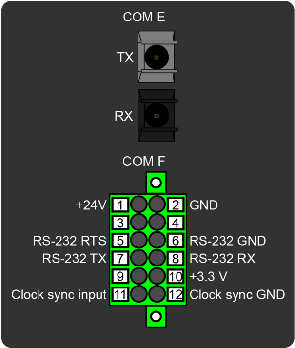
Figure. 7.5.5 - 196. Serial RS-232 module connectors.
