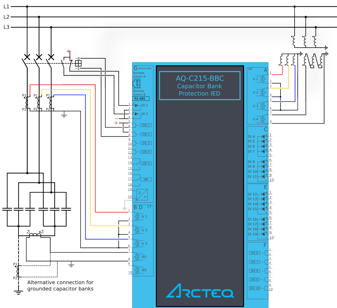
Figure. 6.2 - 178. Application example and its connections in double wye bank.
