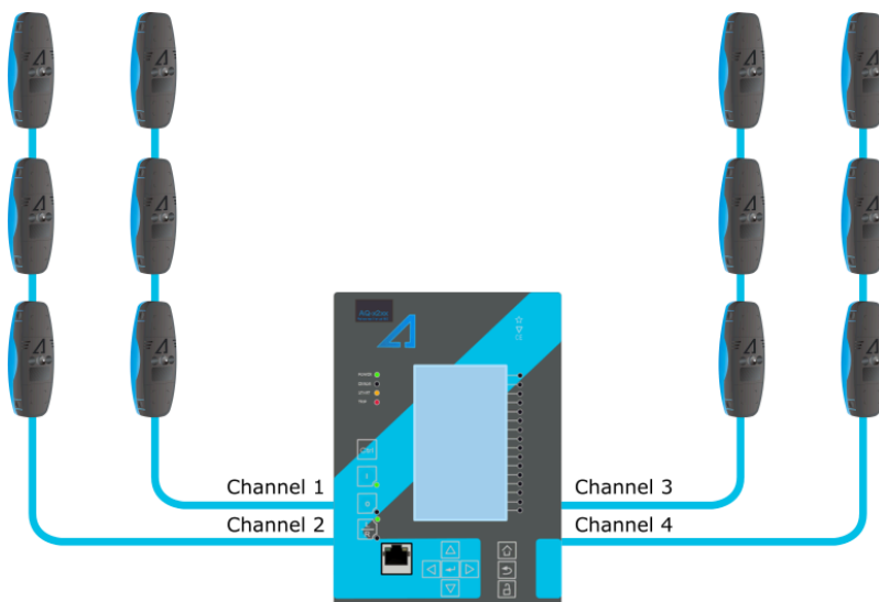
Figure. 4.4.16 - 141. Protection device equipped with arc protection.
