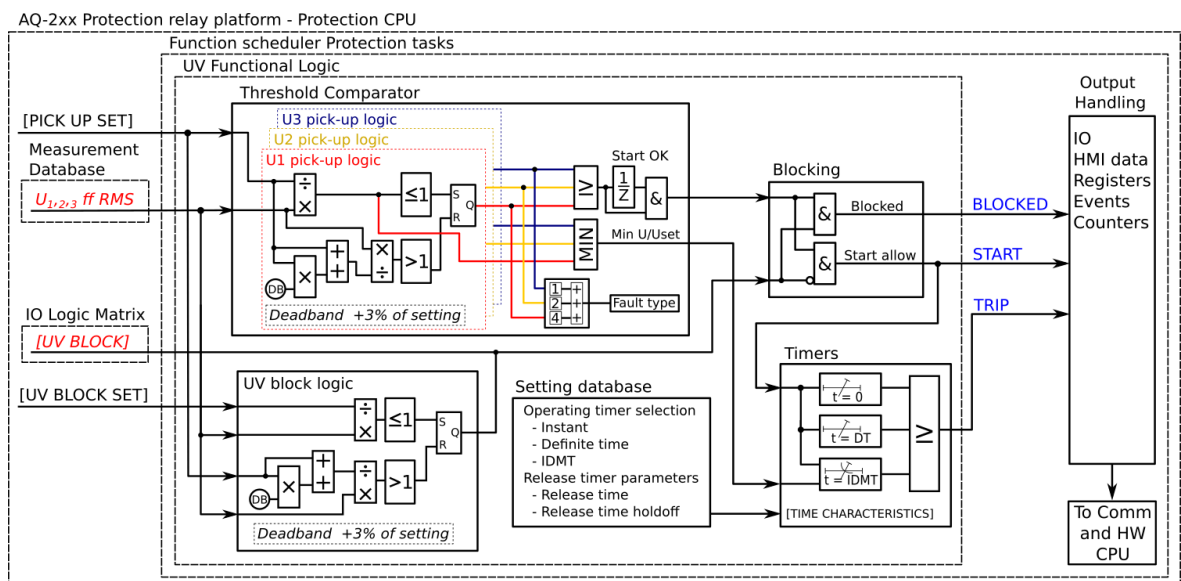
Figure. 4.4.10 - 110. Simplified function block diagram of the U< function.
