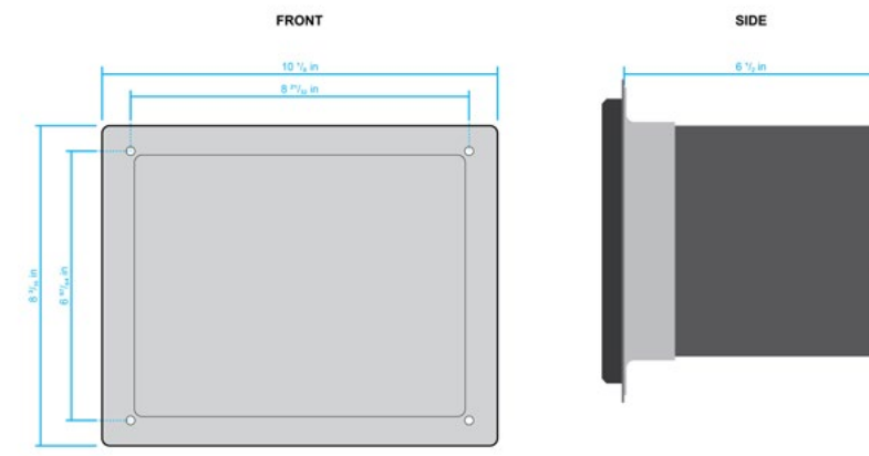
Dimensions of the AQ-25x device.
