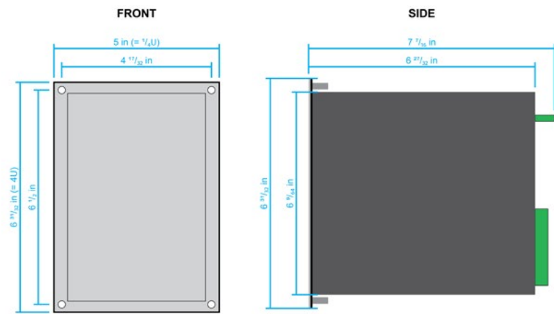
Dimensions of the AQ-21x device.
