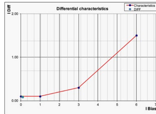
The images above show cable-end differential protection without natural unbalance compensation. The phase current CT errors cause a significant differential current. Compensation is essential to have a sensitive protection setting.
