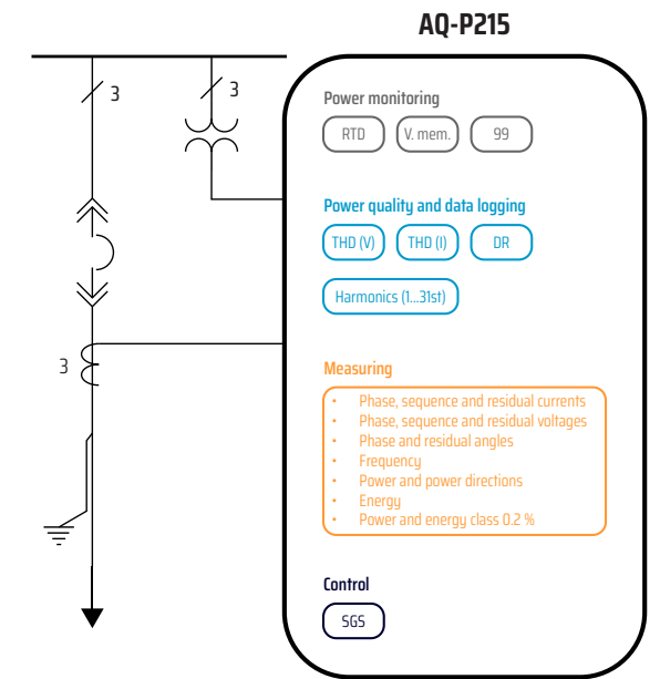
AQ-P215 Power monitoring device
