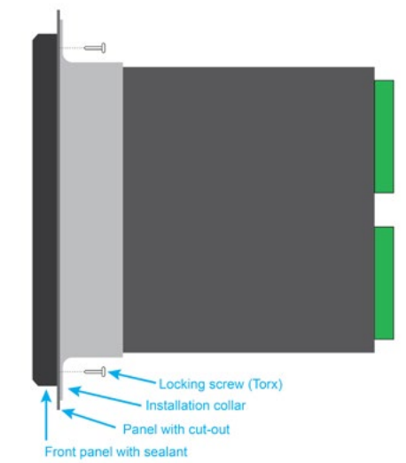
Installation of the AQ-25x device.
