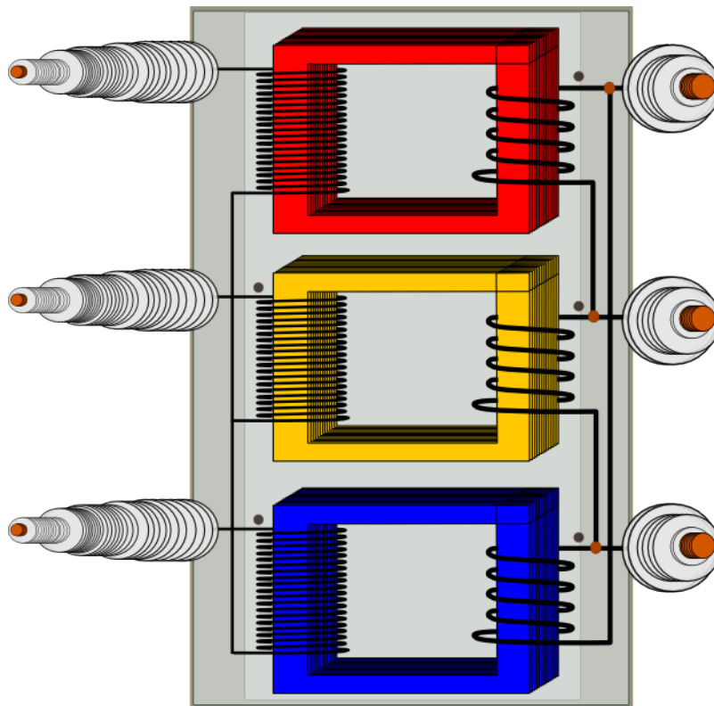
Figure. 4.4.9 - 45. Yd1 transformer's internal connection (in theory).
