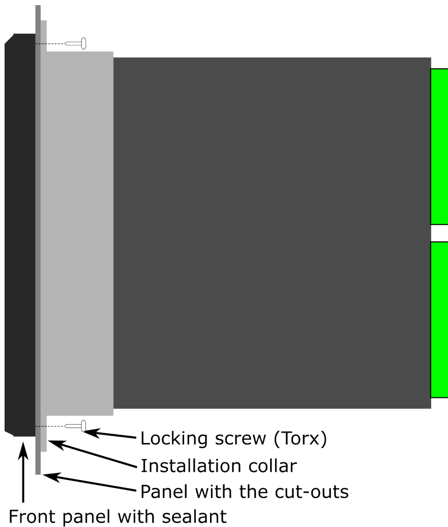
Figure. 7.5 - 139. Device installation.
