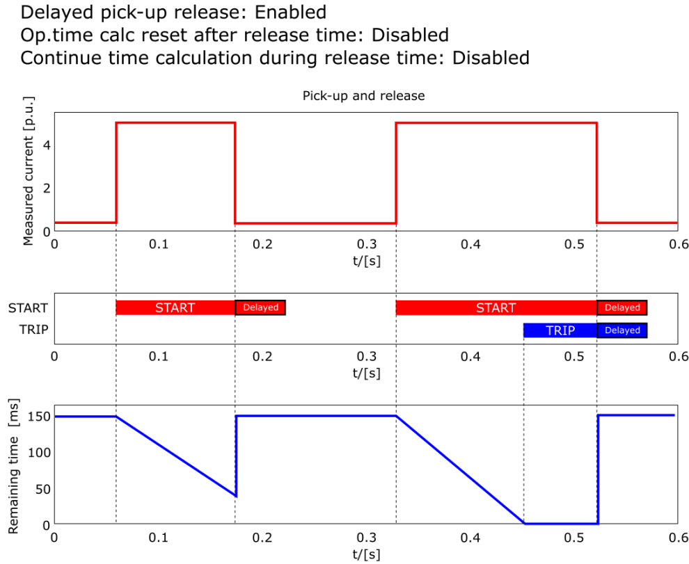
Figure. 4.4.1 - 15. Delayed pick-up release, delay counter is reset at signal drop-off.
