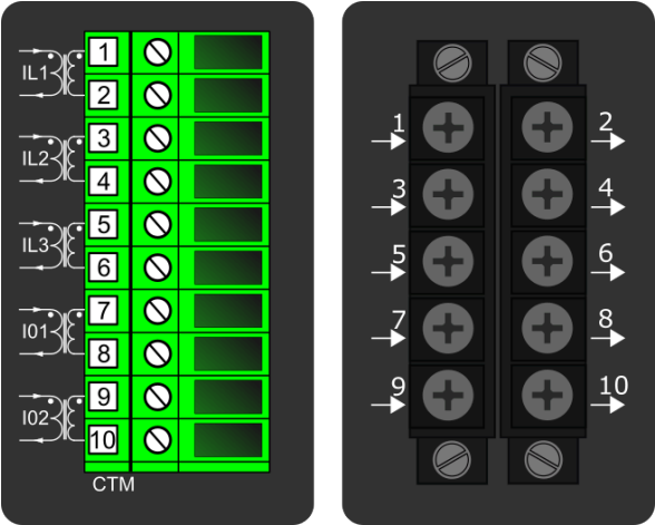
Figure. 7.3 - 124. Module connections with standard and ring lug terminals.
