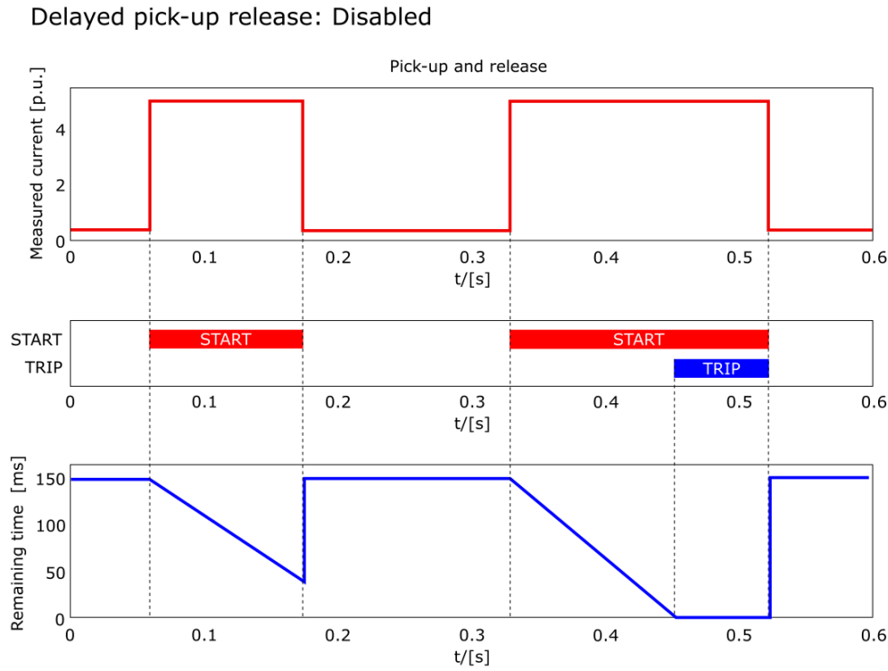
Figure. 4.4.1 - 15. Delayed pick-up release, delay counter is reset at signal drop-off.
