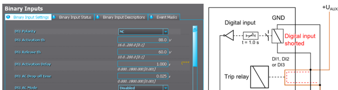
Figure. 6.3 - 245. Settings for a digital input used for trip circuit supervision.
