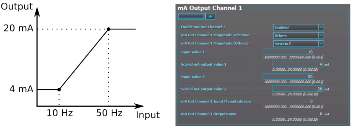
Figure. 4.5.8 - 214. Example of the effects of mA output channel settings.
