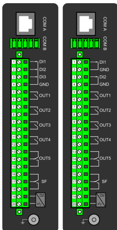
Figure. 7.2 - 251. CPU module.
