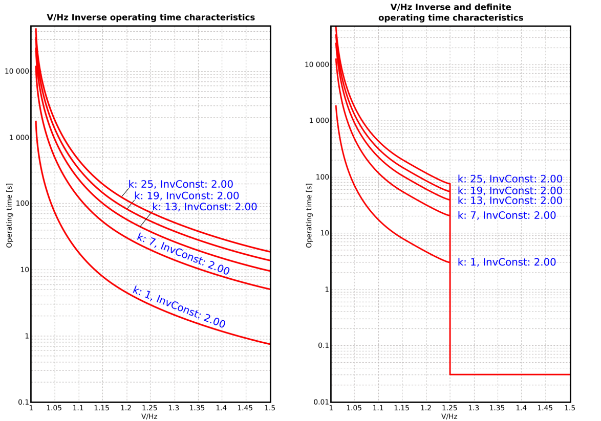
Figure. 4.4.19 - 159. Inverse (above) and inverse and DT (below) time characteristics with the TimeDial k setting effect.
