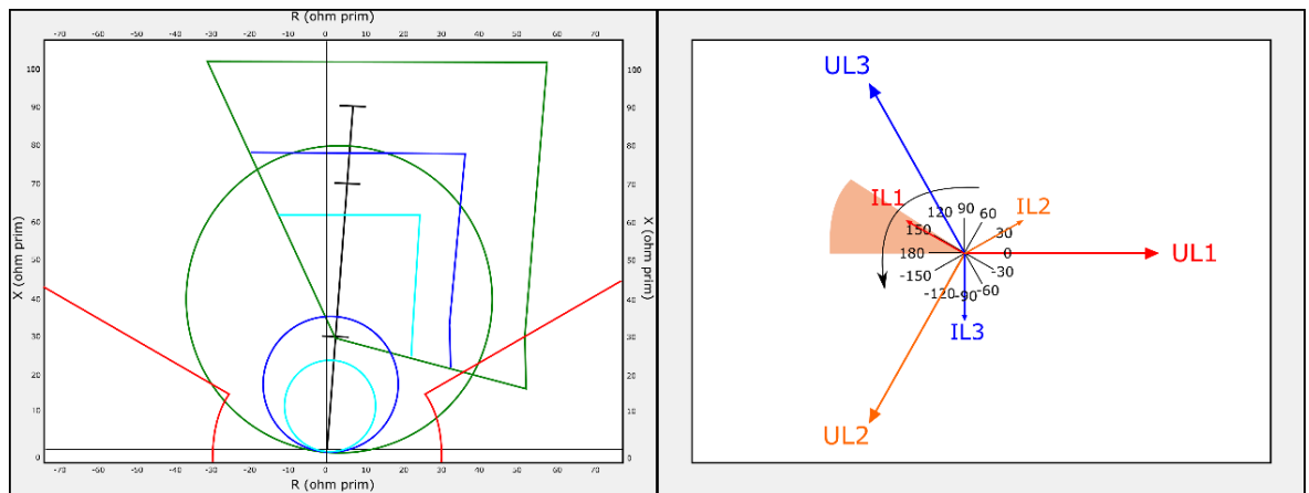
Figure. 4.2.2 - 72. Distance protection characteristics and directional overcurrent.
