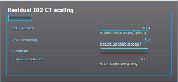
Figure. 4.2.1 - 60. Residual I02 CT scaling (sensitive).
