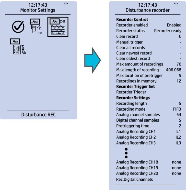
Figure. 3.8 - 53. Disturbance recorder settings.
