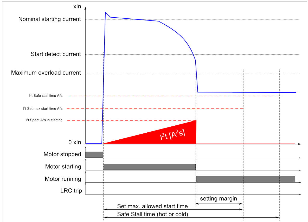
Figure. 4.4.22 - 160. Outputs in normal motor start, no speed switch.
