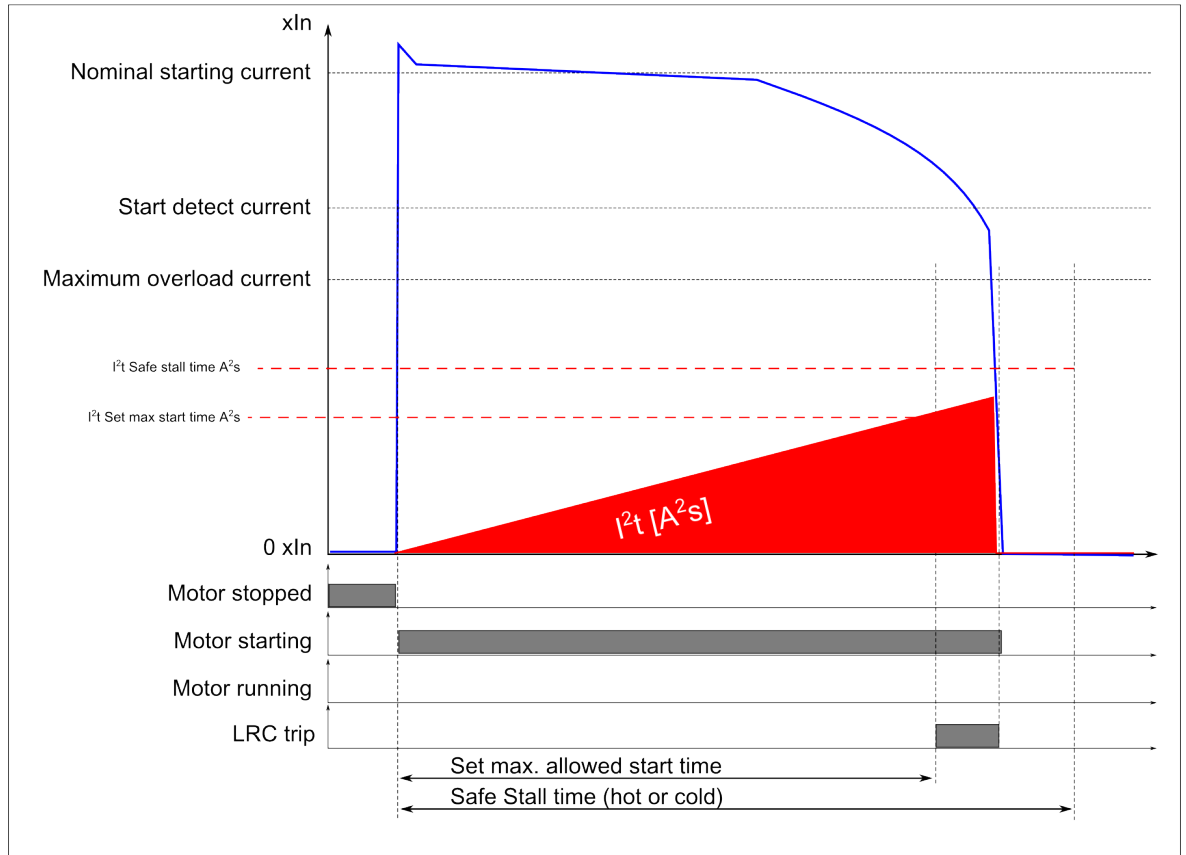
Figure. 4.4.22 - 161. Outputs when motor starting takes too long, no speed switch.
