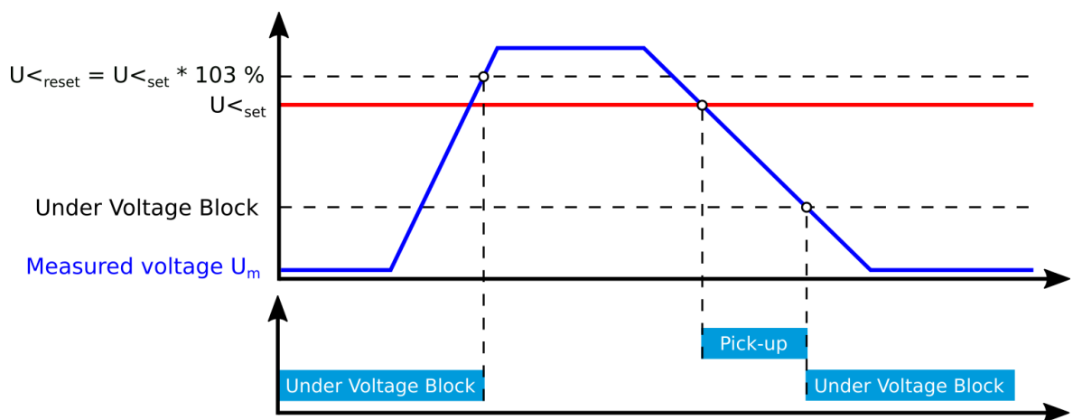
Figure. 4.4.12 - 132. Example of the block setting operation.
