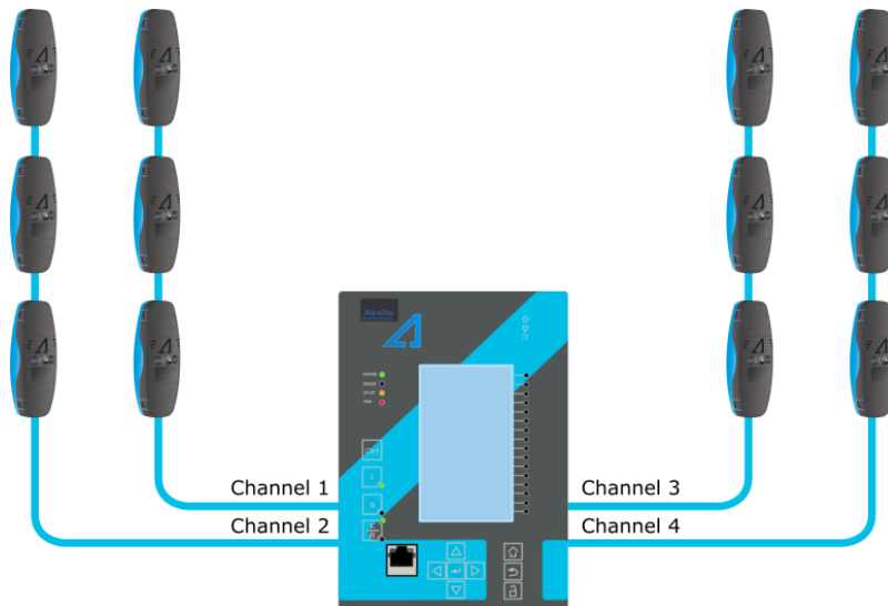
Figure. 4.4.30 - 198. Protection device equipped with arc protection.
