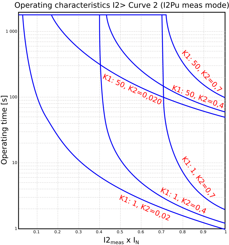
Figure. 4.4.7 - 100. Operation characteristics curve for I2> Curve2.
