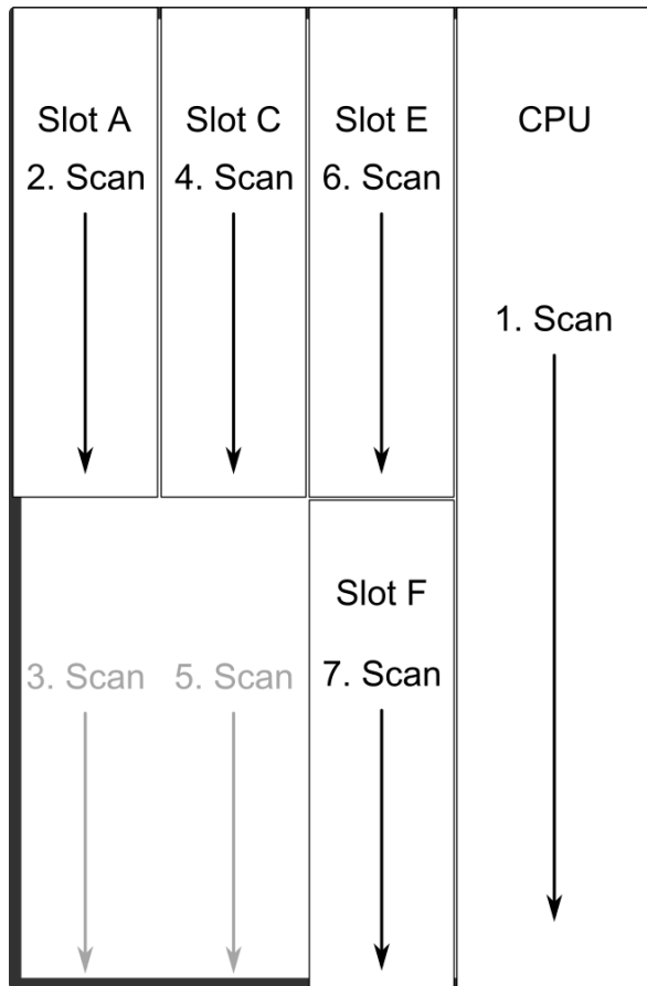
Figure. 7.1 - 190. AQ-X210 hardware scanning and I/O naming principles.
