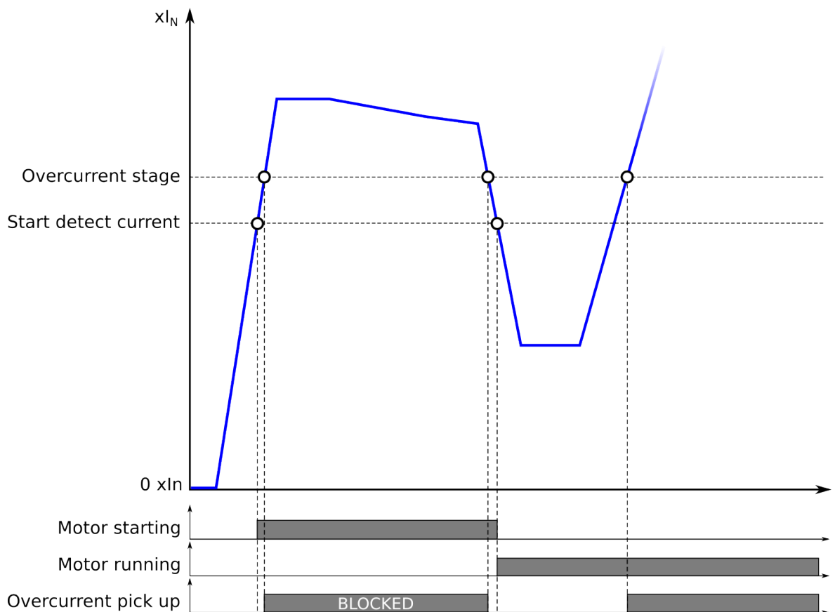
Figure. 4.4.9 - 102. Example of application: motor starting scheme and using motor status signals.
