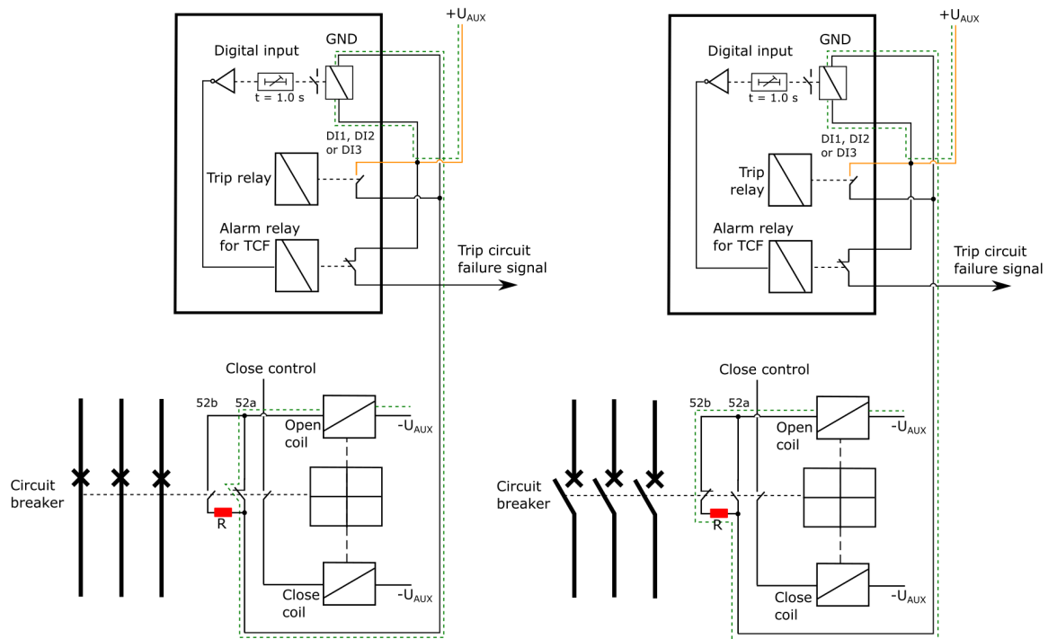
Figure. 6.4 - 184. Trip circuit supervision with one DI and one non-latched trip output.
