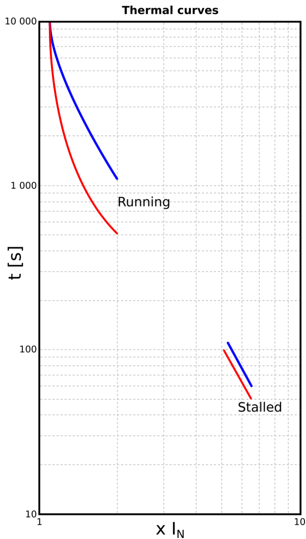
Figure. 4.4.14 - 124. Example of thermal limit curves in a motor.
