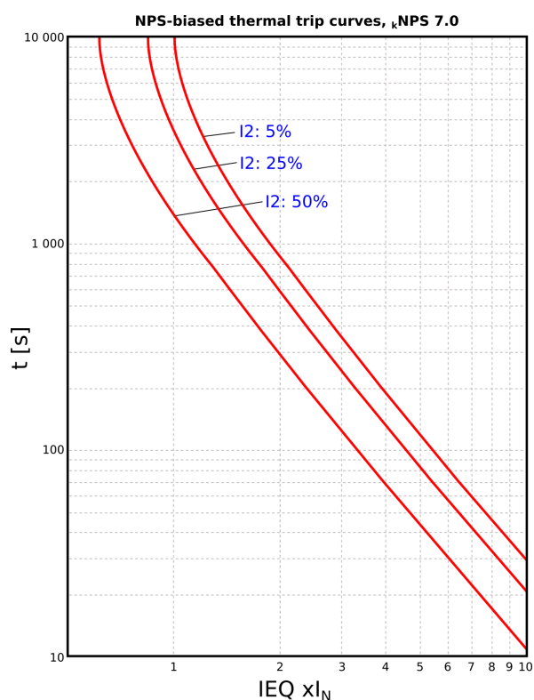
Figure. 4.4.14 - 136. NPS-biased thermal trip curves with k_{NPS} value of 7.
