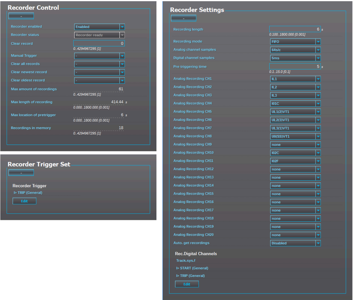
Figure. 4.6.4 - 177. Disturbance recorder settings.
