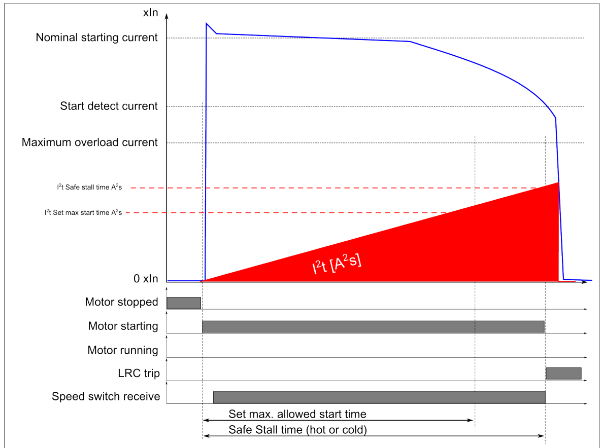
Figure. 4.4.10 - 107. Outputs when motor starting takes too long, with a speed switch.
