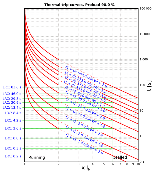
Figure. 4.4.14 - 128. Thermal tripping curves with single time constant, pre-load 90% (hot).
