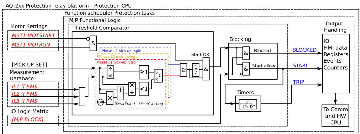
Figure. 4.4.13 - 113. Simplified function block diagram of the I_{m>} function.
