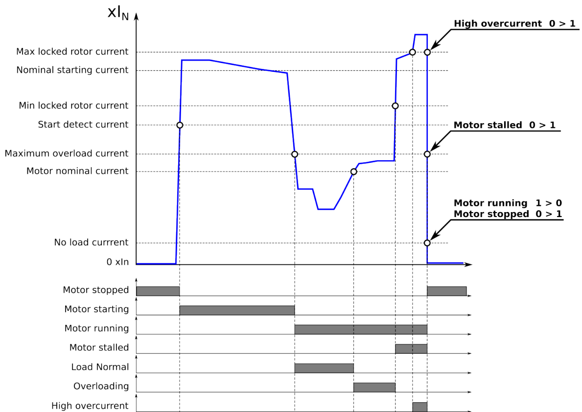
Figure. 4.4.9 - 101. Activation of the function's outputs.
