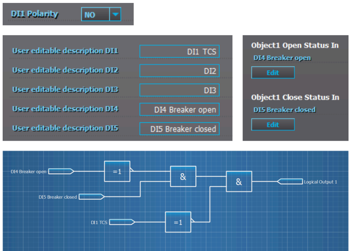
Figure. 6.4 - 188. Example block scheme.
