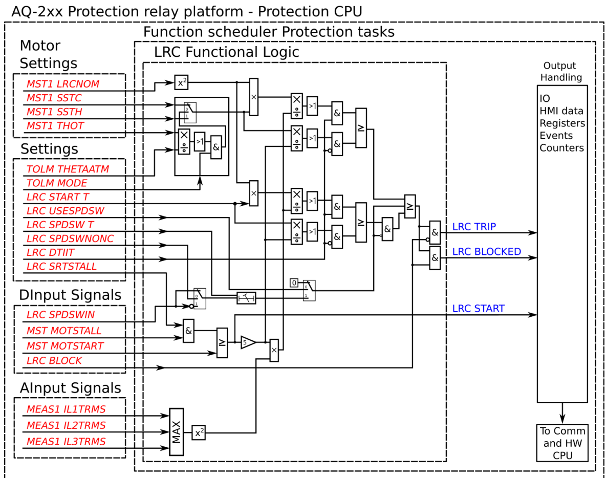
Figure. 4.4.10 - 103. Simplified function block diagram of the motor start/ locked rotor monitoring function.
