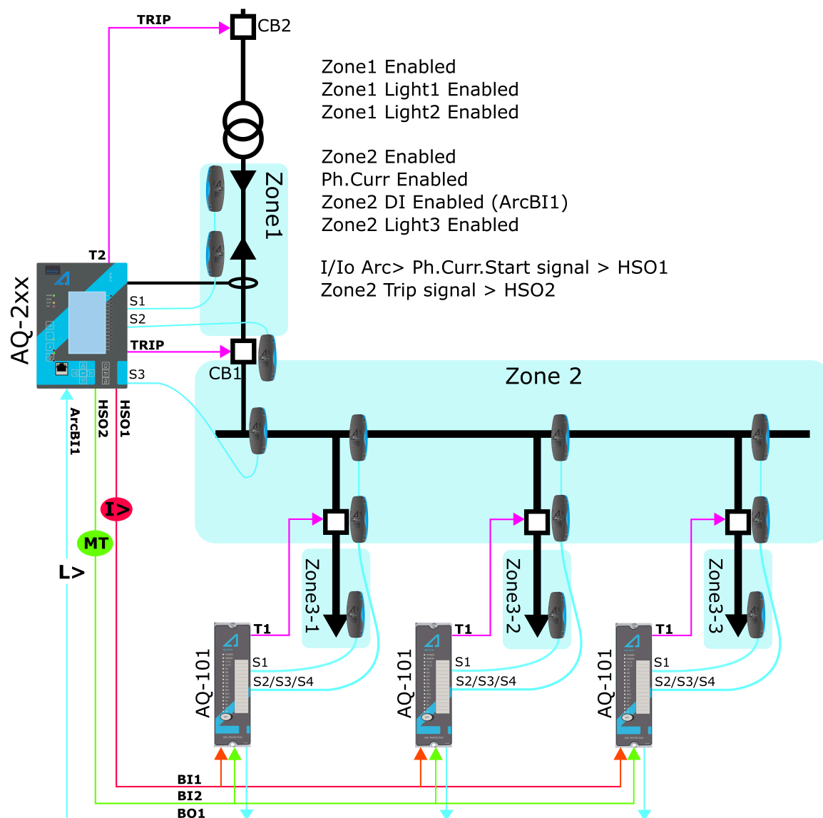
Figure. 4.4.17 - 141. Scheme with AQ-101 arc protection relays.
