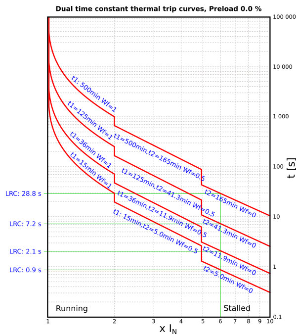
Figure. 4.4.14 - 130. Thermal tripping curves with dual dynamic time constants and correction factor, pre-load 90% (hot).
