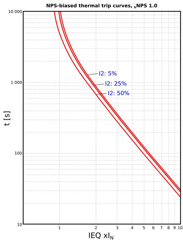
Figure. 4.4.14 - 134. NPS-biased thermal trip curves with k_{NPS} value of 1.
