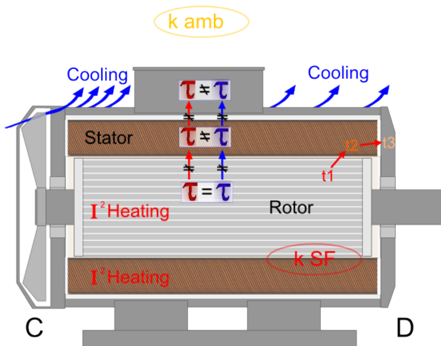
Figure. 4.4.14 - 120. Simplified motor construction and time constants.
