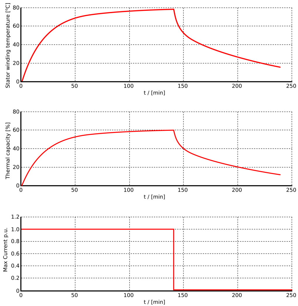
Figure. 4.4.14 - 122. Measured motor temperature in heating/cooling test.
