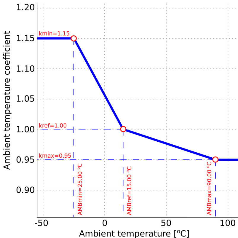
Figure. 4.4.14 - 117. Ambient temperature coefficient calculation (linear approximation, three points).
