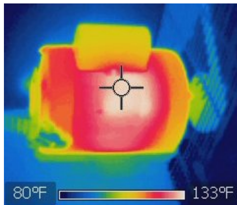
Figure. 4.4.14 - 121. Running motor's temperature with thermal image camera.
