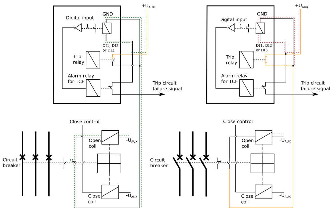
Figure. 6.4 - 187. Trip circuit supervision with one DI and one latched output contact.
