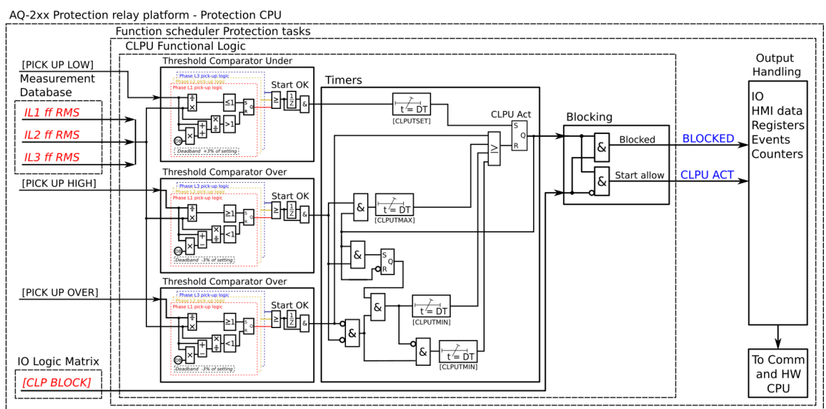
Figure. 4.5.5 - 151. Simplified function block diagram of the cold load pick-up function.
