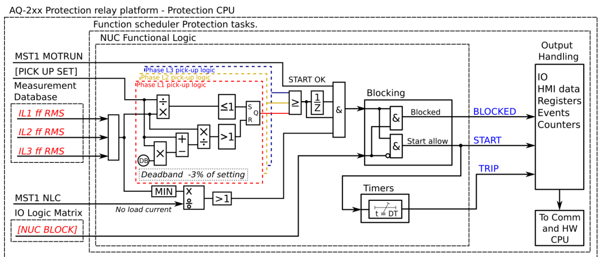
Figure. 4.4.12 - 112. Simplified function block diagram of the I< function.
