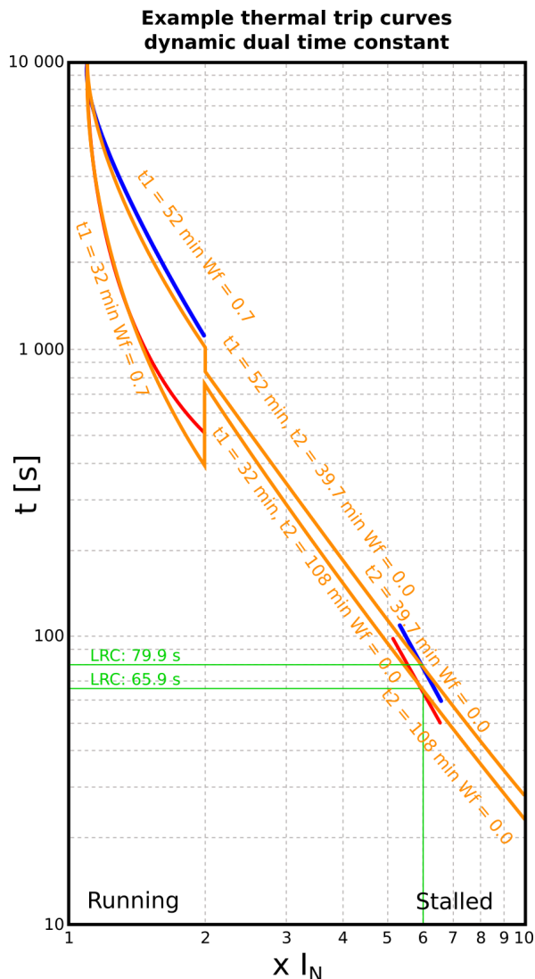
Figure. 4.4.14 - 126. Comparing dual time constant thermal replica tripping curves to given motor thermal characteristics.
