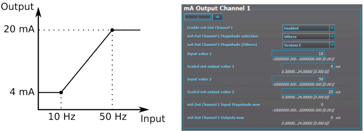
Figure. 4.5.6 - 158. Example of the effects of mA output channel settings.
