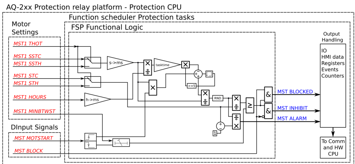
Figure. 4.4.11 - 109. Simplified function block diagram of the N> function.
