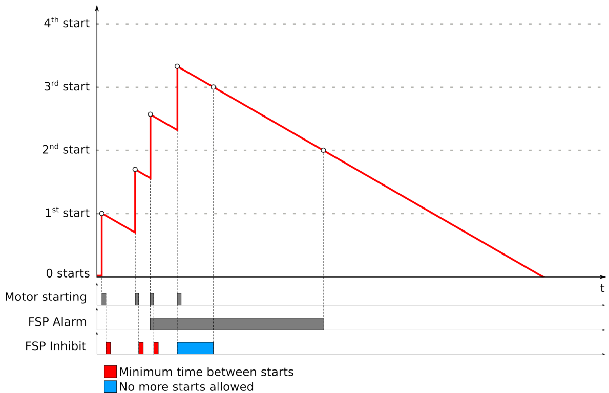
Figure. 4.4.11 - 110. Updating the function's start counter (image not to scale with regard to time).
