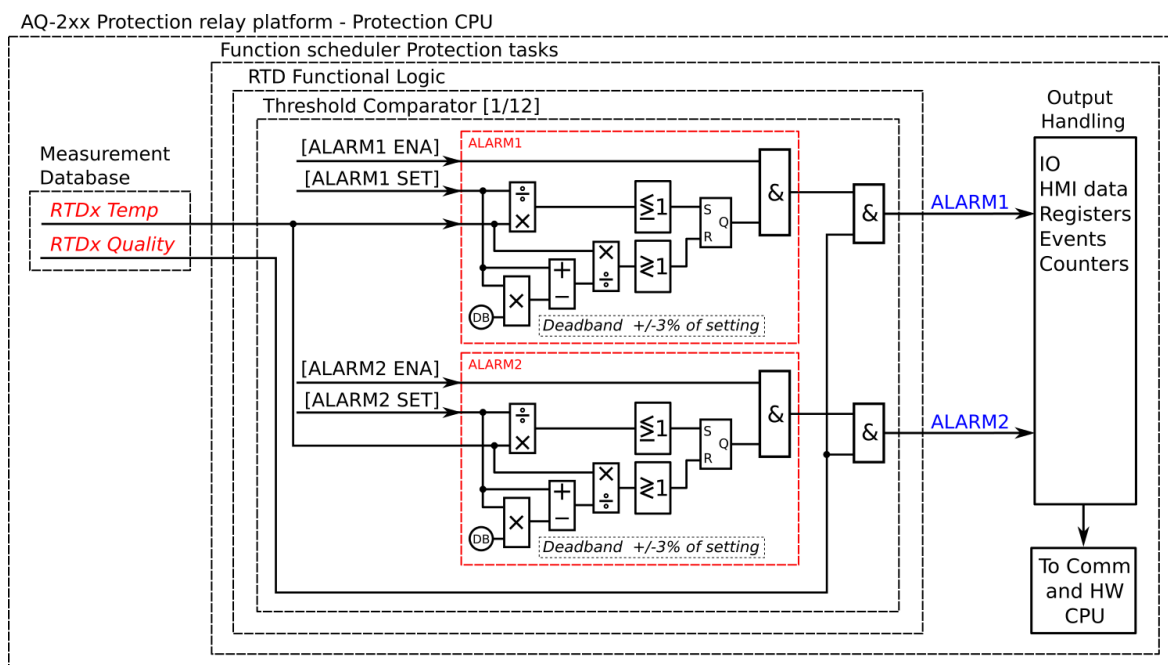
Figure. 4.4.15 - 139. Simplified function block diagram of the resistance temperature detection function.
