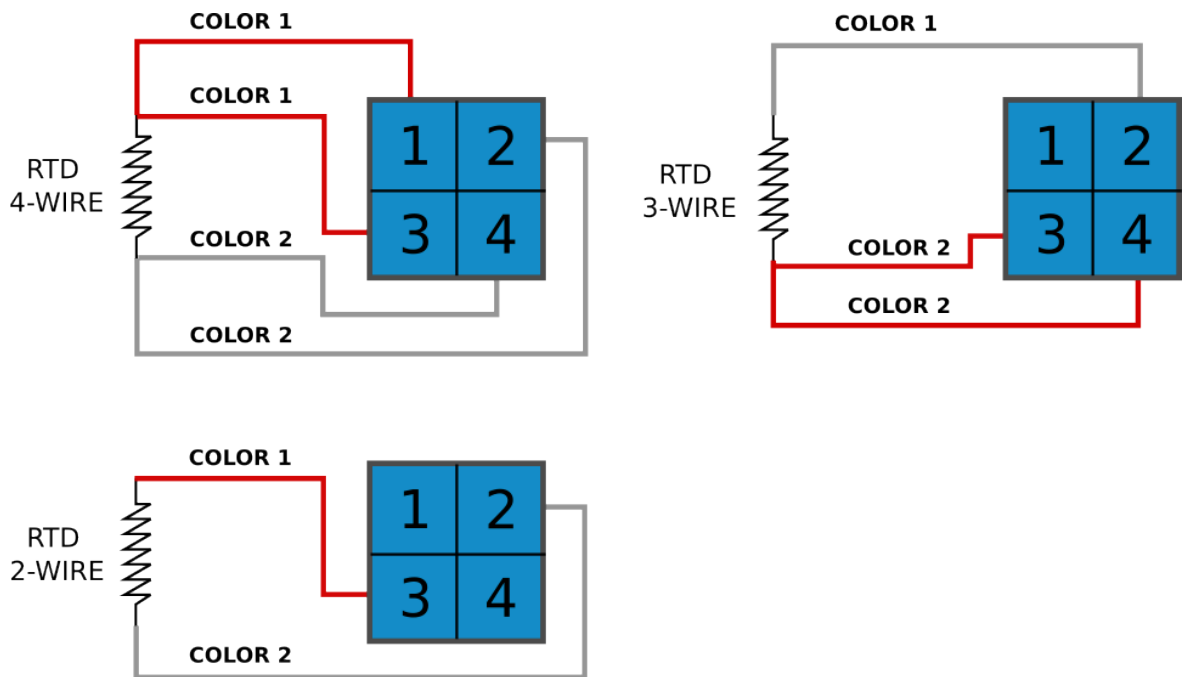
Figure. 7.4.4 - 198. RTD sensor connection types.
