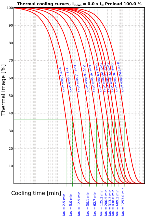
Figure. 4.4.14 - 131. Thermal cooling curves, single cooling time constant.
