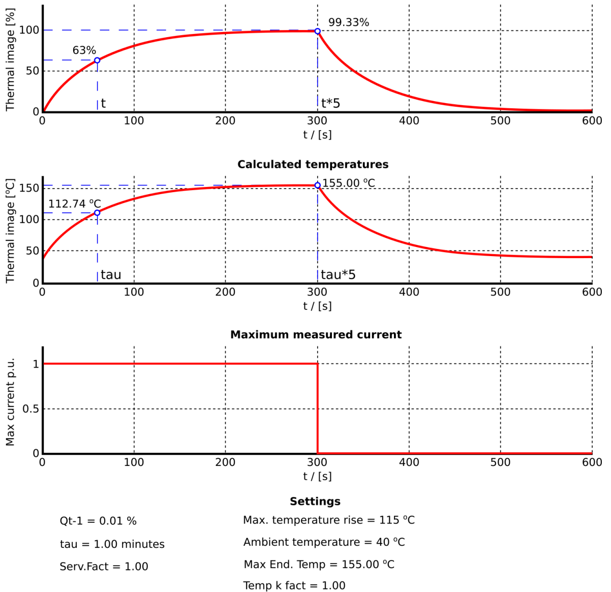
Figure. 4.4.14 - 116. Thermal image calculation with nominal conditions: single time constant thermal replica.
