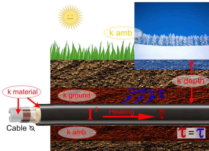
Figure. 4.4.14 - 119. Factors affecting the cooling and current-carrying capacity of a cable.
