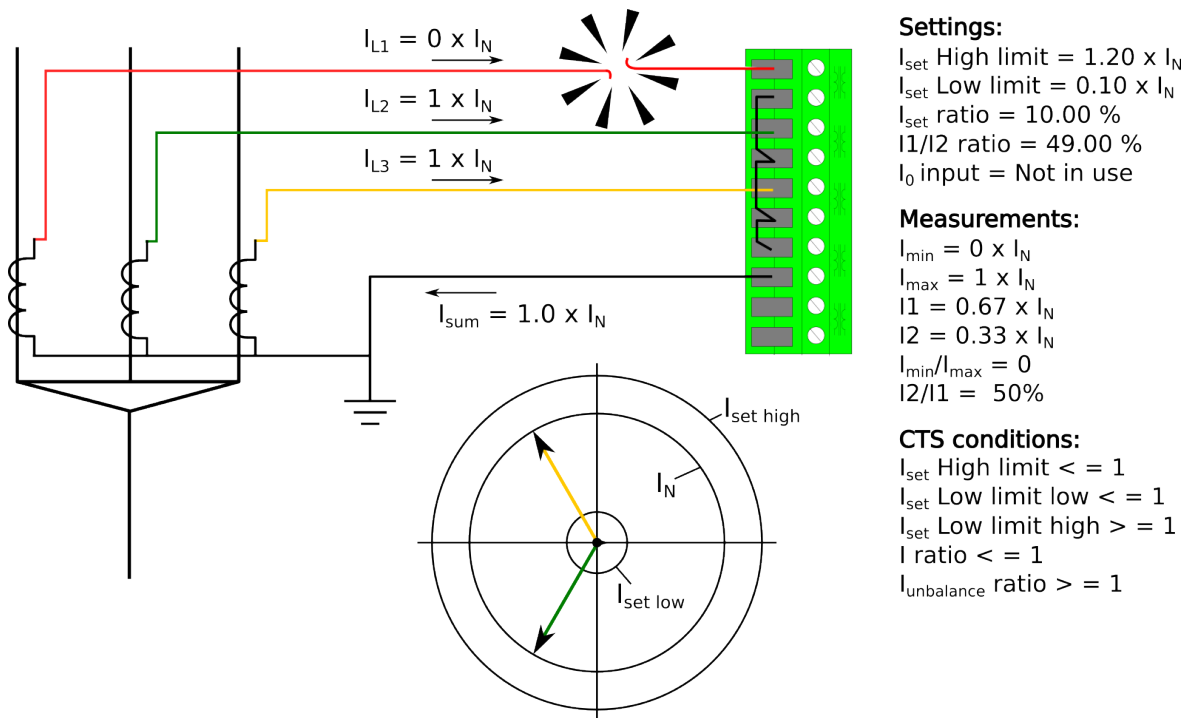
Figure. 4.6.1 - 165. Secondary circuit fault in phase L1 wiring.
