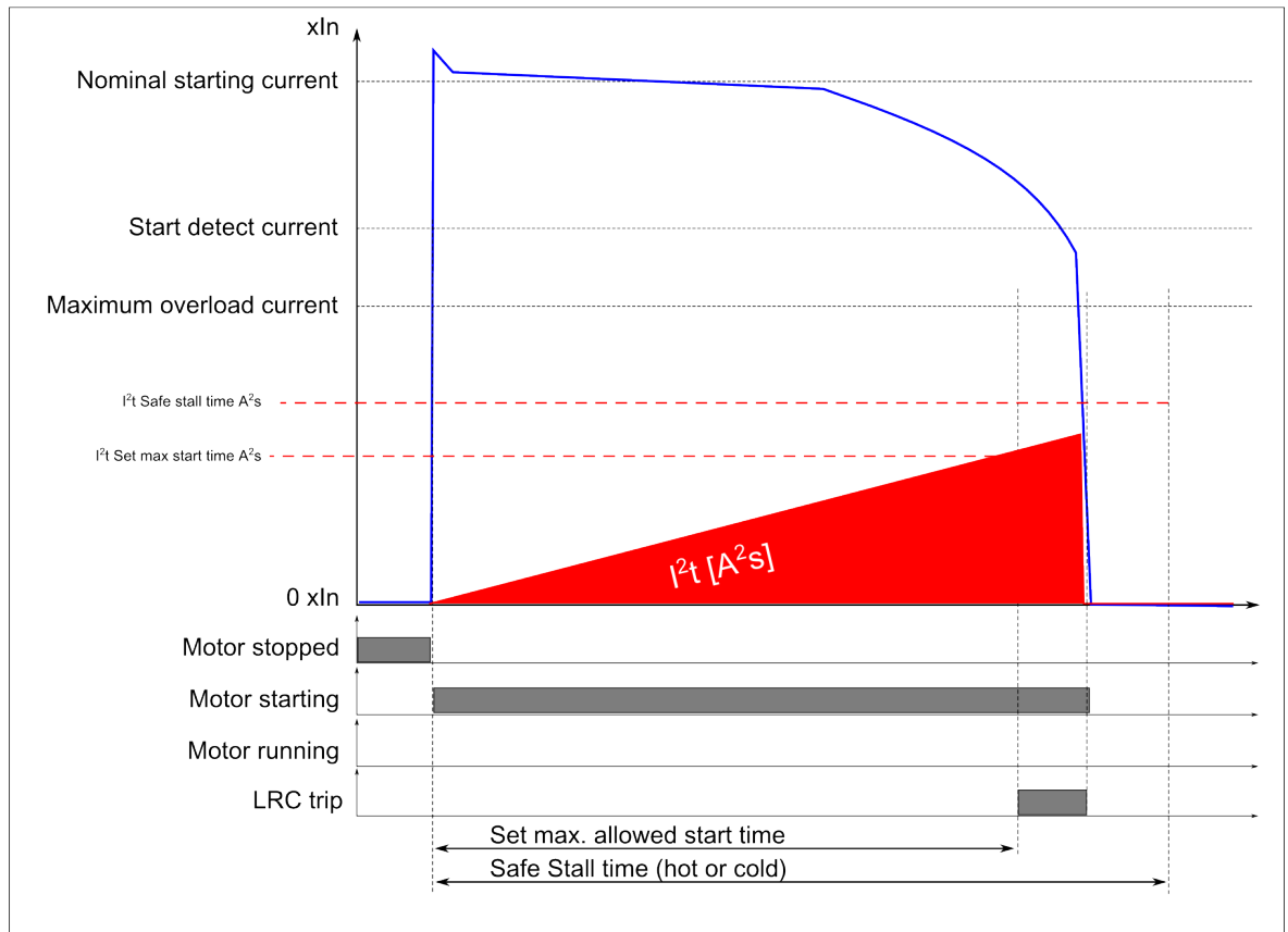
Figure. 4.4.10 - 105. Outputs when motor starting takes too long, no speed switch.
