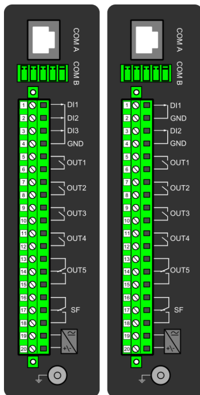
Figure. 7.2 - 191. CPU module.
