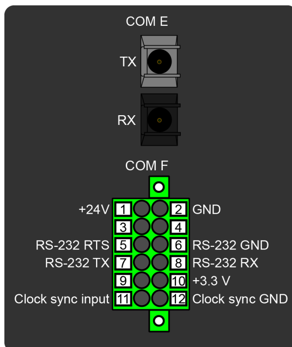
Figure. 7.4.5 - 199. Serial RS-232 module connectors.
