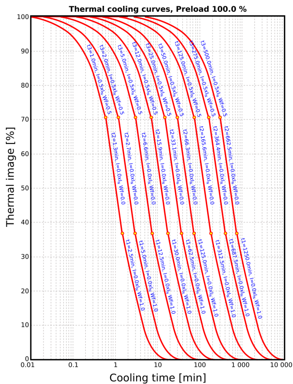
Figure. 4.4.14 - 133. Thermal cooling curves, dynamic triple time constant (motor is running without load in the first part with dedicated time constant).
