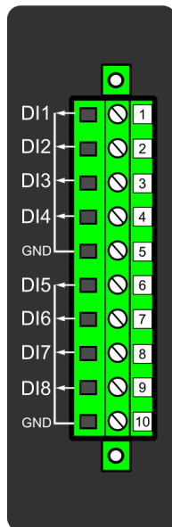
Figure. 7.4.1 - 193. Digital input module (DI8) with eight add-on digital inputs.
