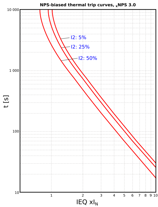
Figure. 4.4.14 - 135. NPS-biased thermal trip curves with k_{NPS} value of 3.
