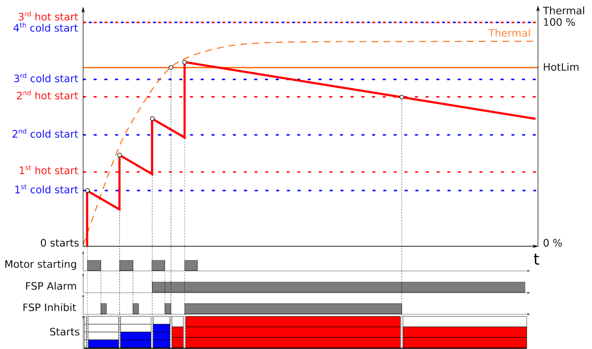
Figure. 4.4.11 - 111. Updating the starts counter when thermal hot and cold status taken into consideration.
