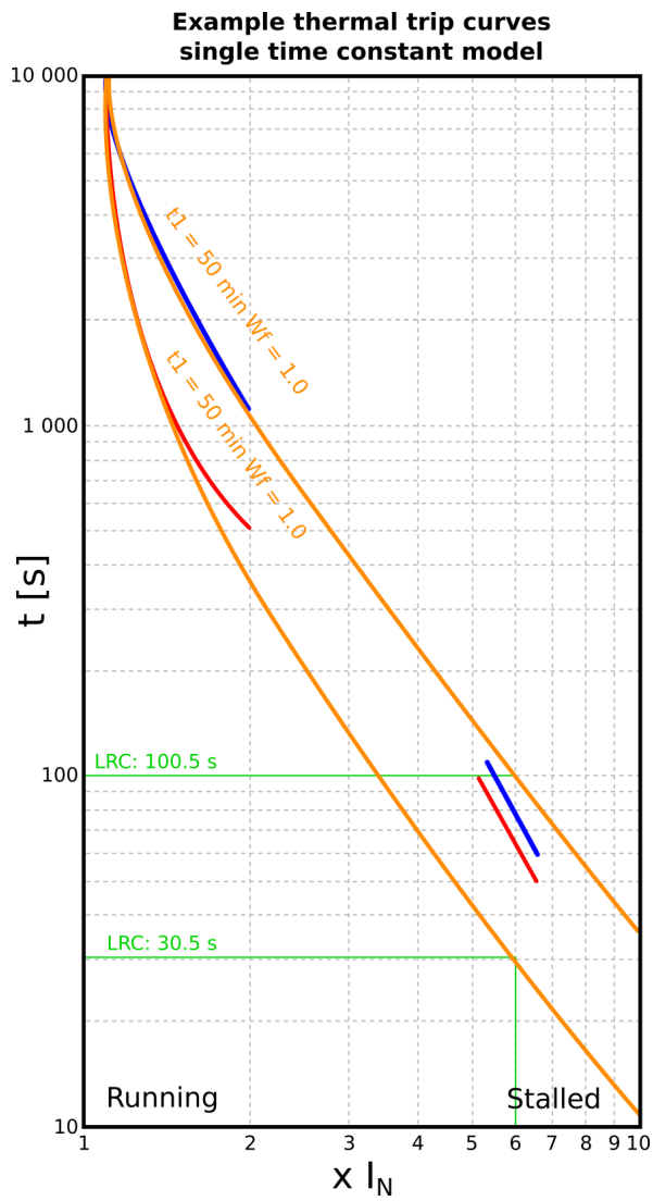
Figure. 4.4.14 - 125. Comparing single time constant thermal replica tripping curves to given motor thermal characteristics.
