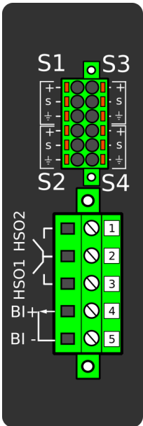
Figure. 7.5.3 - 250. Arc protection module.
