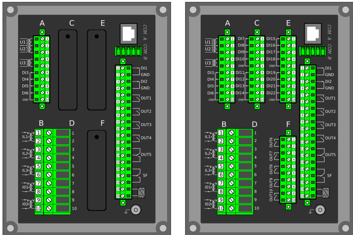
Figure. 7.1 - 242. Modular construction of AQ-X213.
