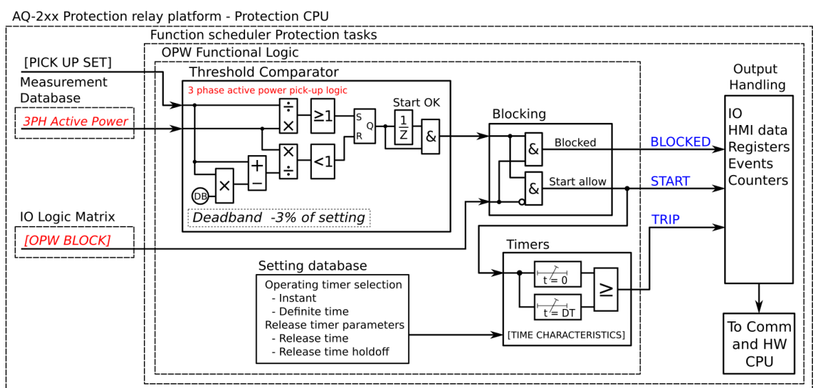
Figure. 4.4.16 - 145. Simplified function block diagram of the P> function.
