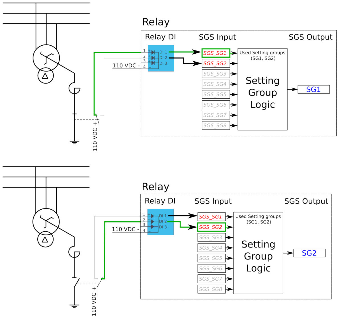
Figure. 4.5.2 - 171. Setting group control – two-wire connection from Petersen coil status.
