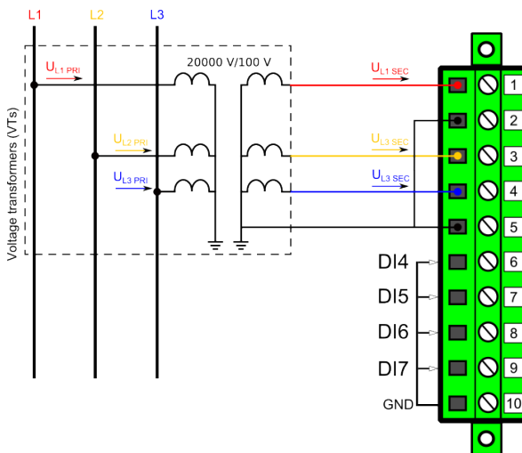
Figure. 4.2.2 - 67. Voltage measurement terminology
