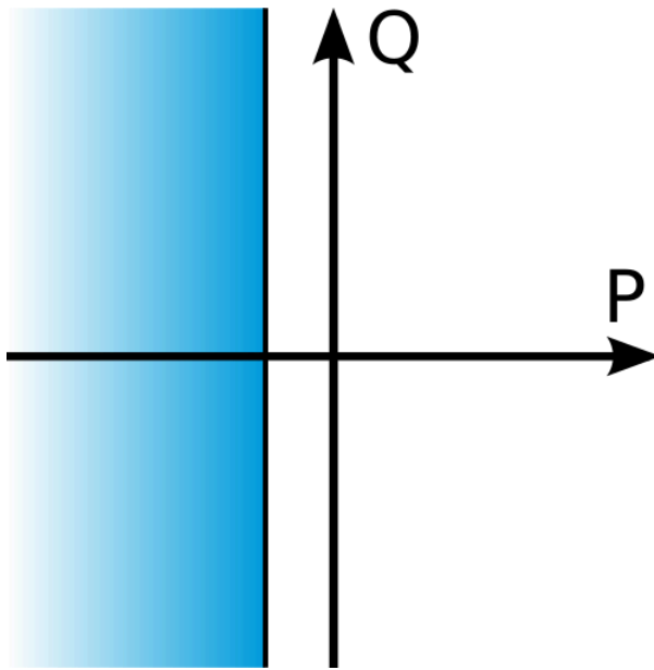
Figure. 4.4.18 - 149. Operating characteristics of reverse power protection.
