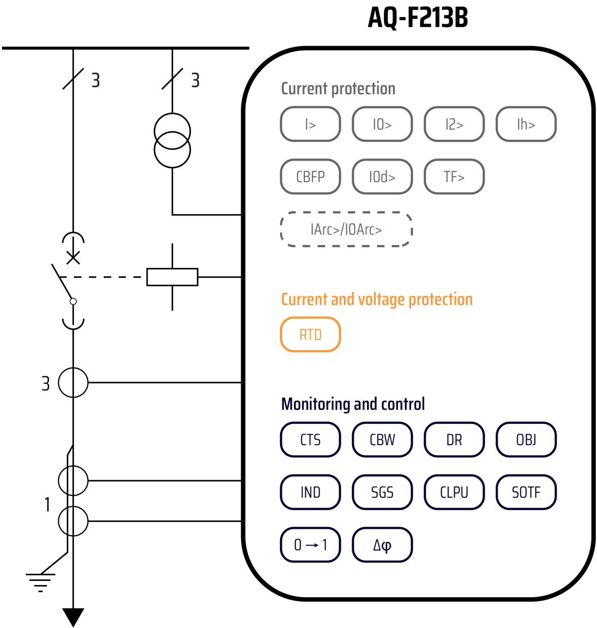
Figure. 6.1 - 231. AQ-F213B application example with function block diagram.
