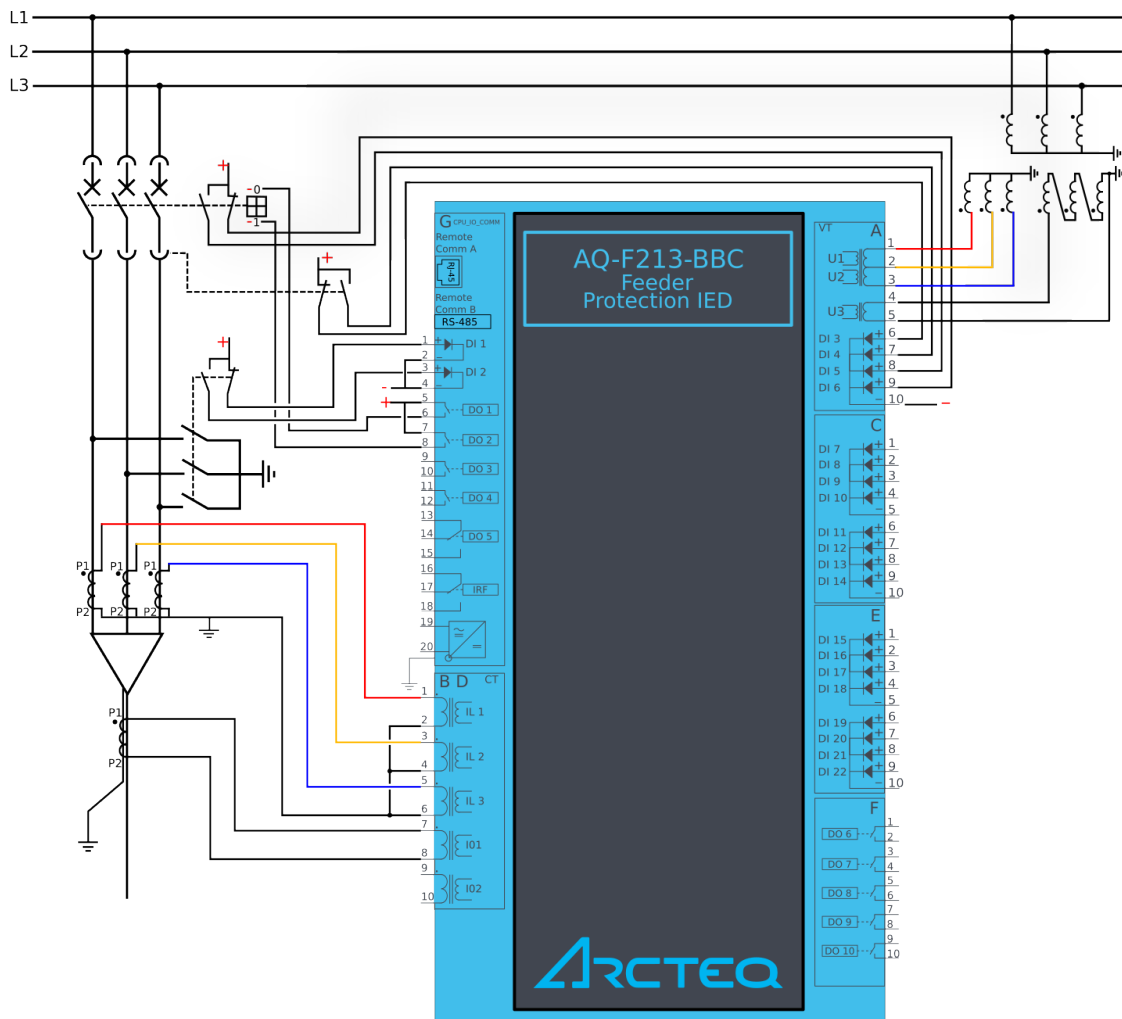
Figure. 6.2 - 235. Application example and its connections.
