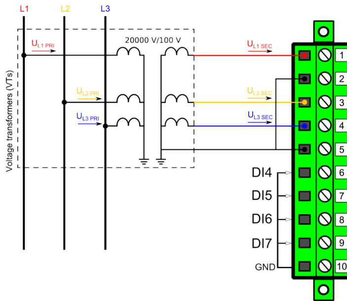
Figure. 4.2.2 - 69. Example connections for 3LN voltage measurement.
