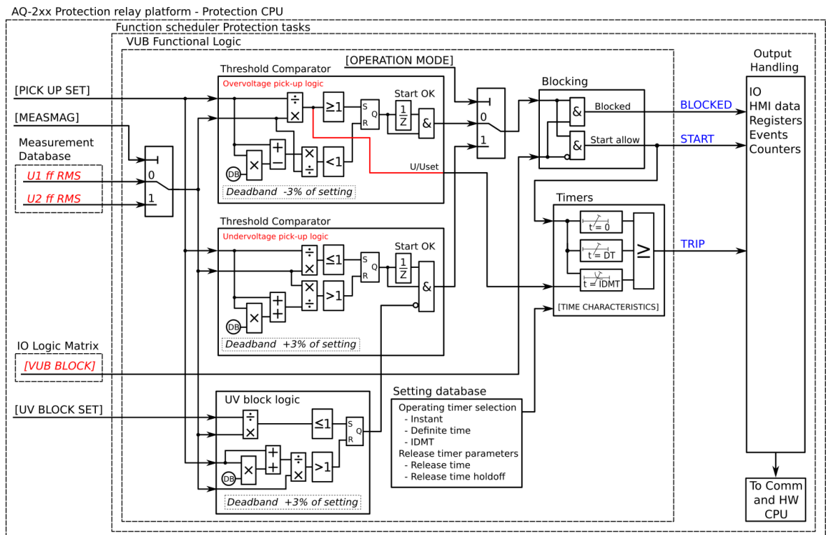
Figure. 4.4.13 - 138. Simplified function block diagram of the U1/U2&gt;/&lt; function.
