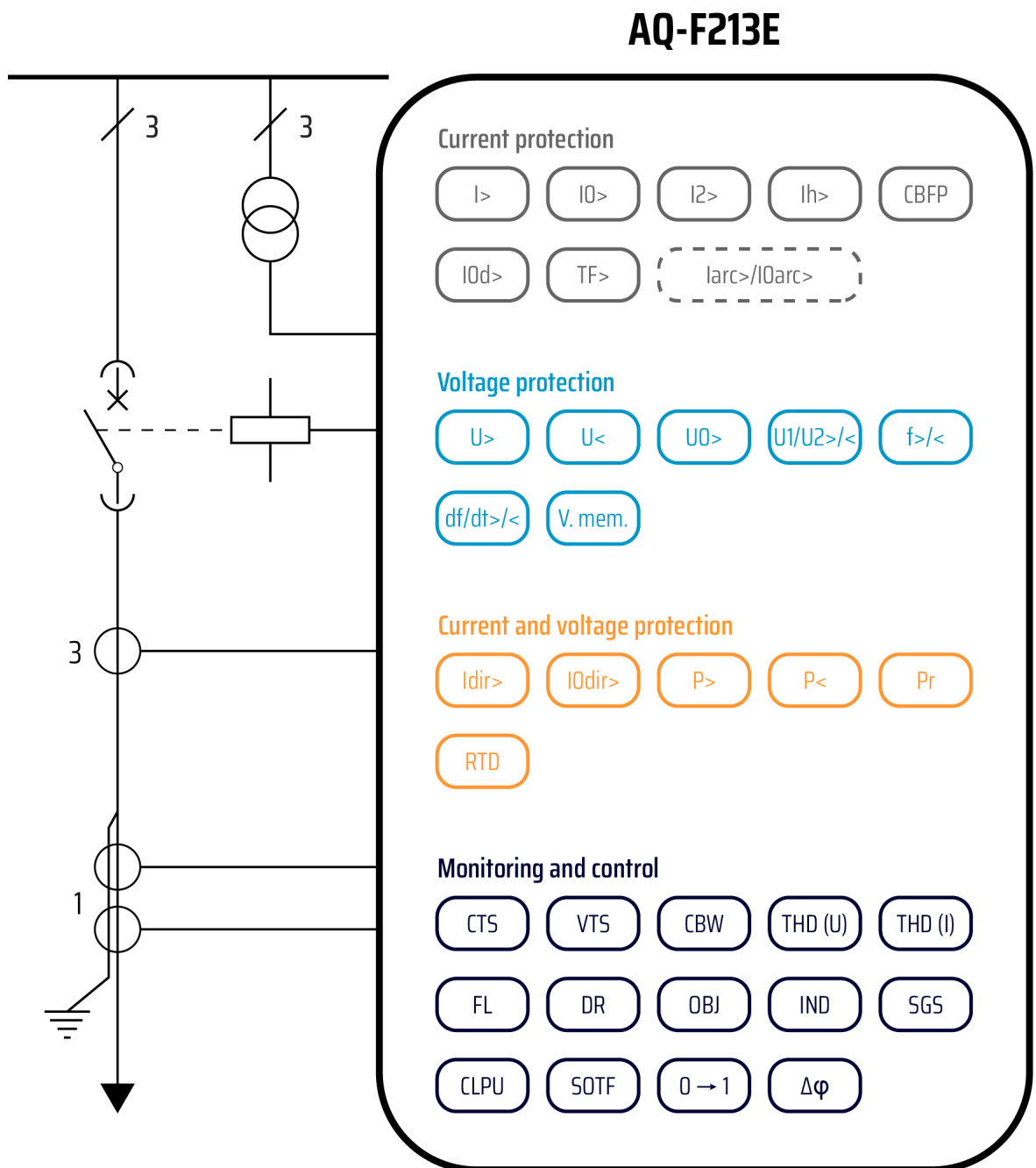
Figure. 6.1 - 234. AQ-F213B application example with function block diagram.
