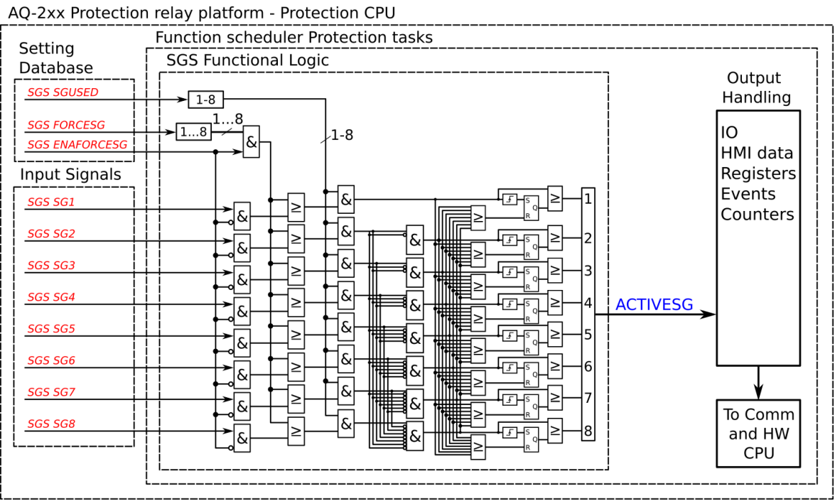
Figure. 4.5.2 - 168. Simplified function block diagram of the setting group selection function.
