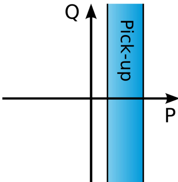
Figure. 4.4.17 - 146. Operating characteristics of underpower protection.
