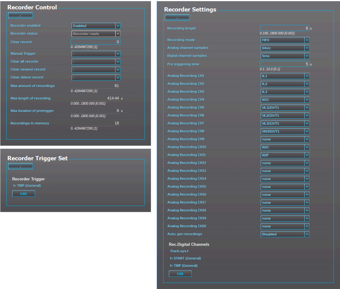
Figure. 4.6.6 - 226. Disturbance recorder settings.
