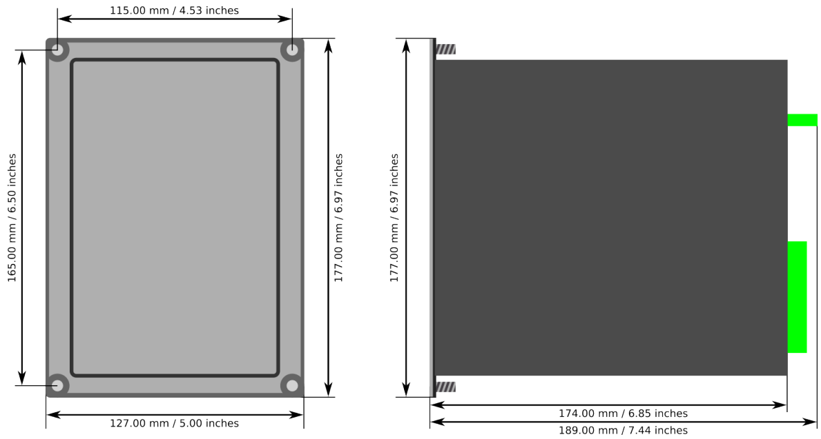
Figure. 7.6 - 260. Device dimensions.
