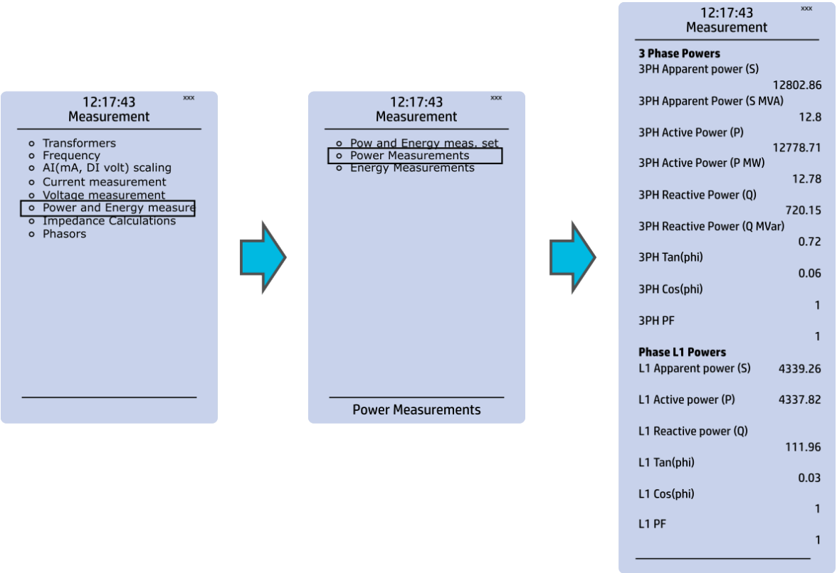
Figure. 3.7 - 48. Power and Energy measurement submenu.
