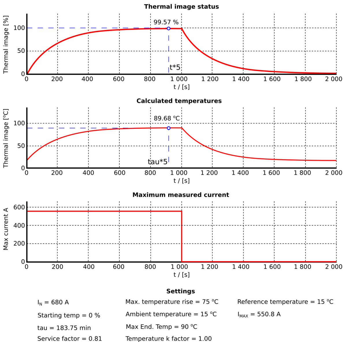
Figure. 4.4.19 - 162. Thermal response with k sf factor correctly set.
