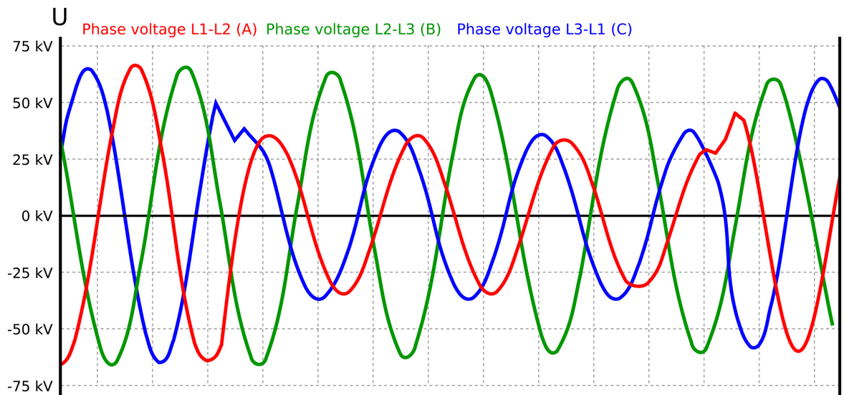
Figure. 4.5.9 - 204. Generator islanding.
