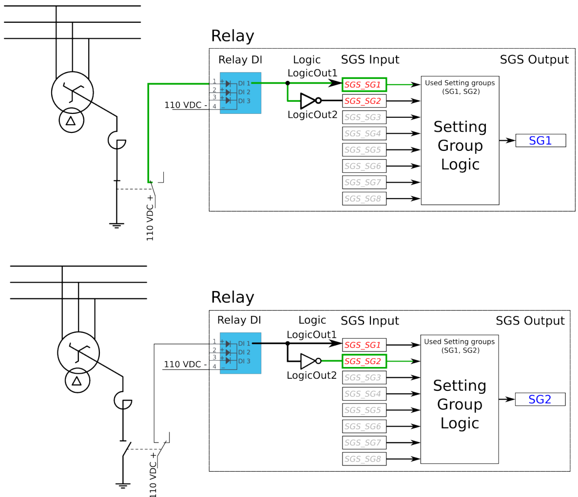
Figure. 4.5.2 - 170. Setting group control – one-wire connection from Petersen coil status.
