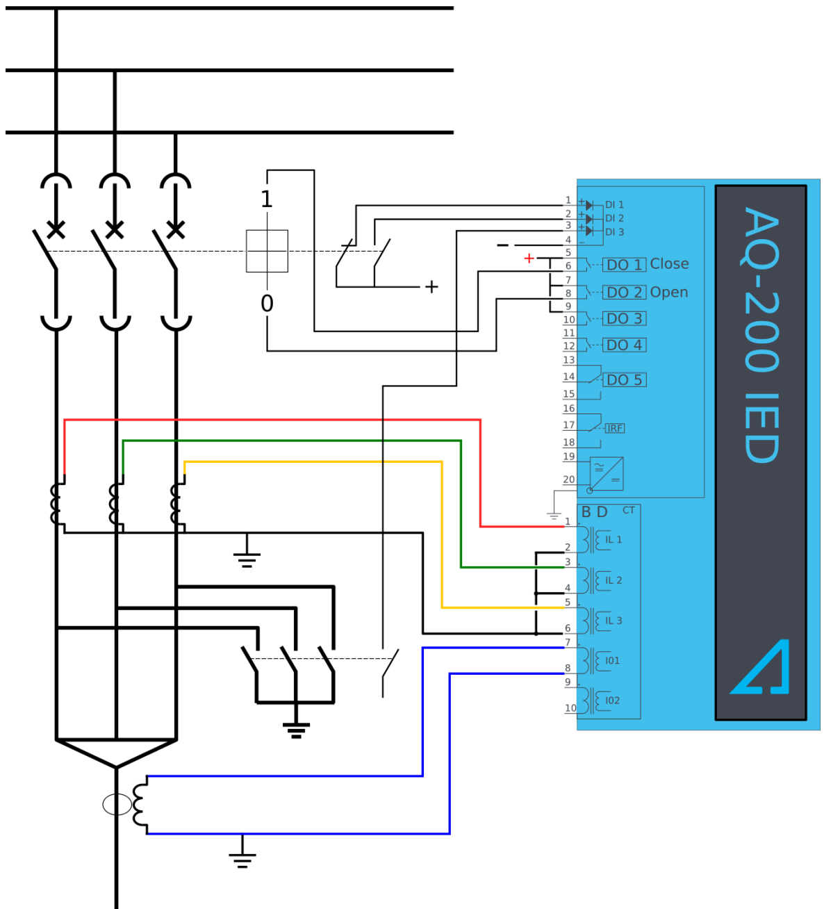
Figure. 4.5.3 - 175. Example of an interlock application.
