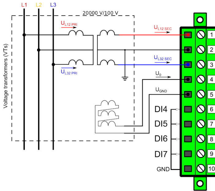
Figure. 4.2.2 - 71. Example connections for 2LL+U0 (open delta 2LL) voltage measurement.
