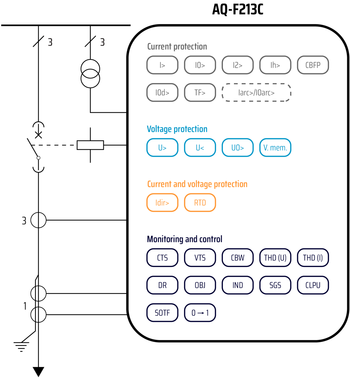
Figure. 6.1 - 232. AQ-F213C application example with function block diagram.
