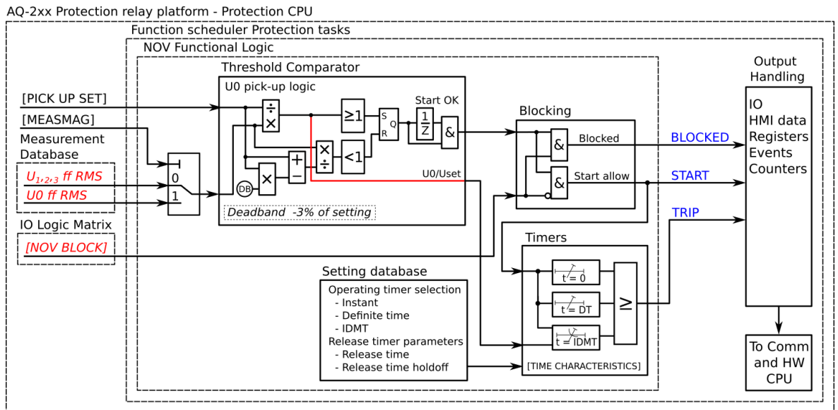
Figure. 4.4.12 - 131. Simplified function block diagram of the U0> function.
