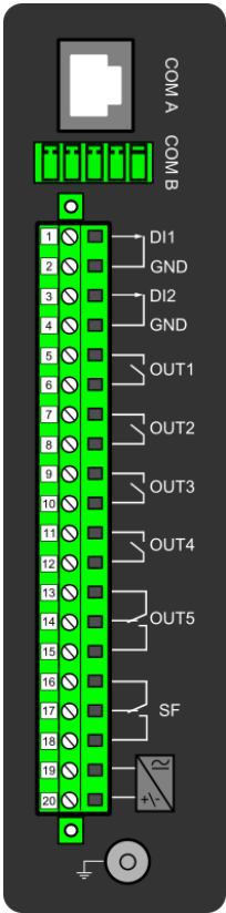
Figure. 7.2 - 244. CPU module.
