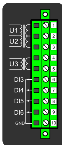
Figure. 7.4 - 246. Voltage measurement module.
