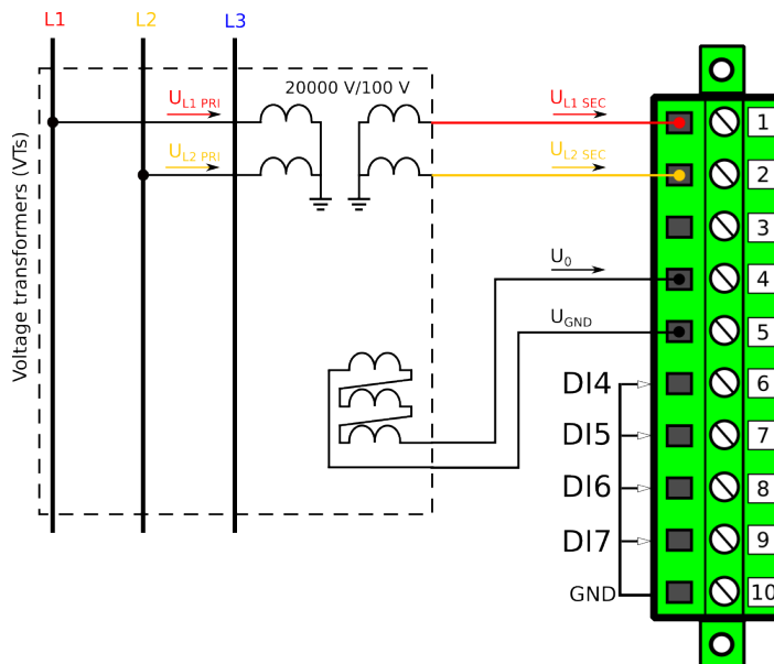
Figure. 4.2.2 - 72. Example connections for 1LL+U0 voltage measurement.
