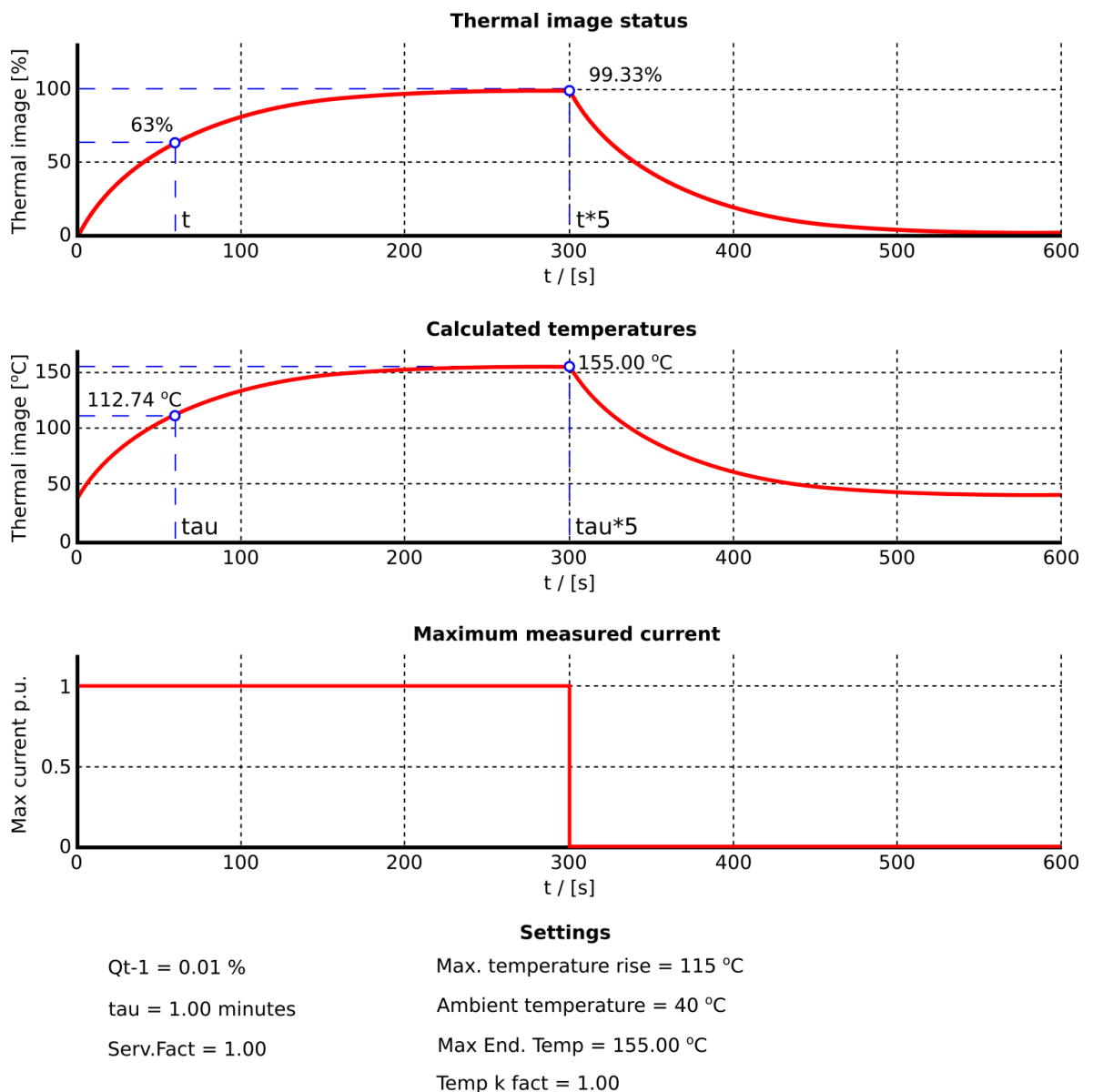
Figure. 4.4.19 - 151. Example of thermal image calculation with nominal conditions.
