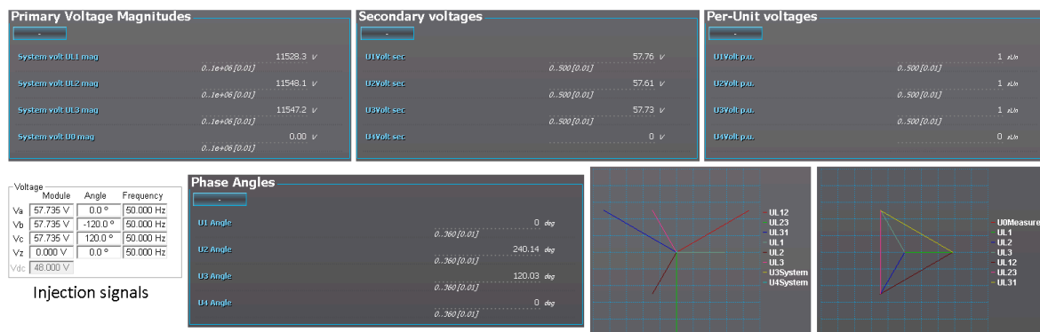
Figure. 4.2.2 - 73. Measurement behavior when nominal voltage injected during LN voltage measurements.
