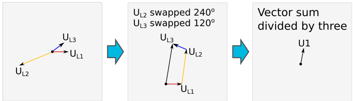
Figure. 4.4.13 - 137. Close-distance short-circuit between phases 1 and 3.
