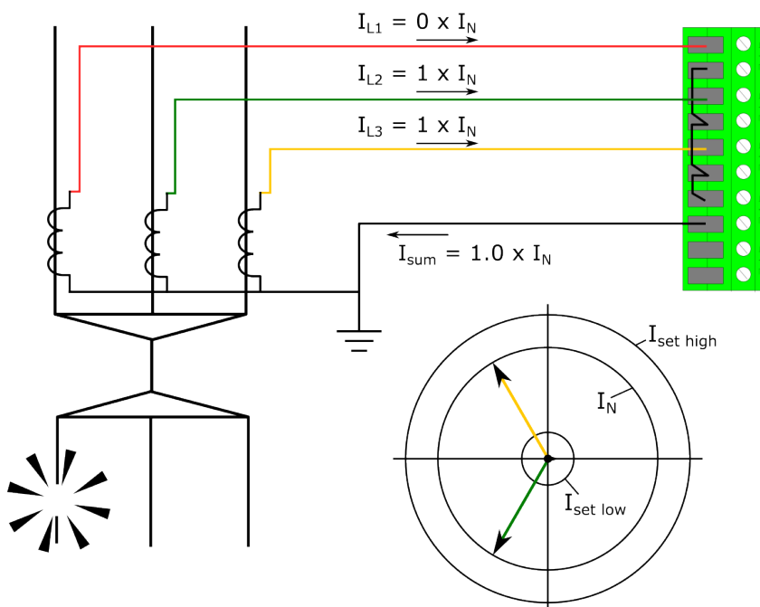
Figure. 4.6.1 - 213. Primary circuit fault in phase L1 wiring.
