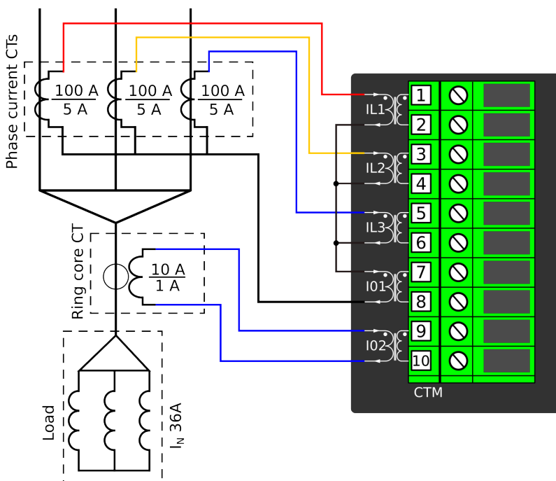
Figure. 4.2.1 - 57. Connections.
