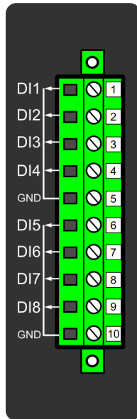
Figure. 7.5.1 - 247. Digital input module (DI8) with eight add-on digital inputs.
