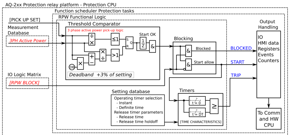
Figure. 4.4.18 - 150. Simplified function block diagram of the Pr function.
