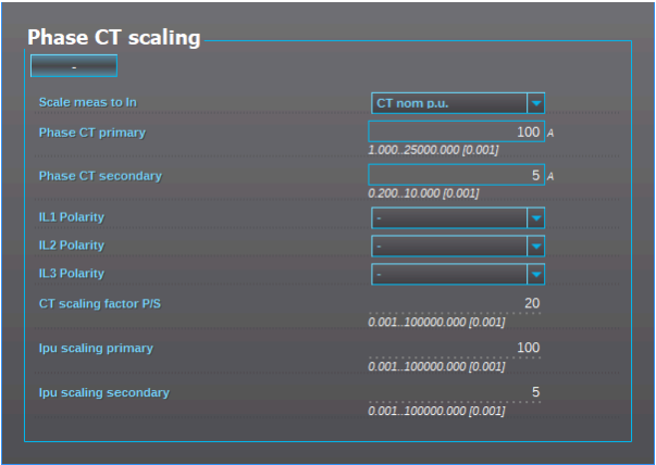
Figure. 4.2.1 - 58. Setting the phase current transformer scalings to CT nominal.
