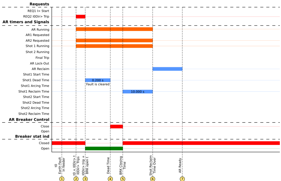
Figure. 4.5.5 - 184. Signal status graph of the transient earth fault auto-recloser cycle.
