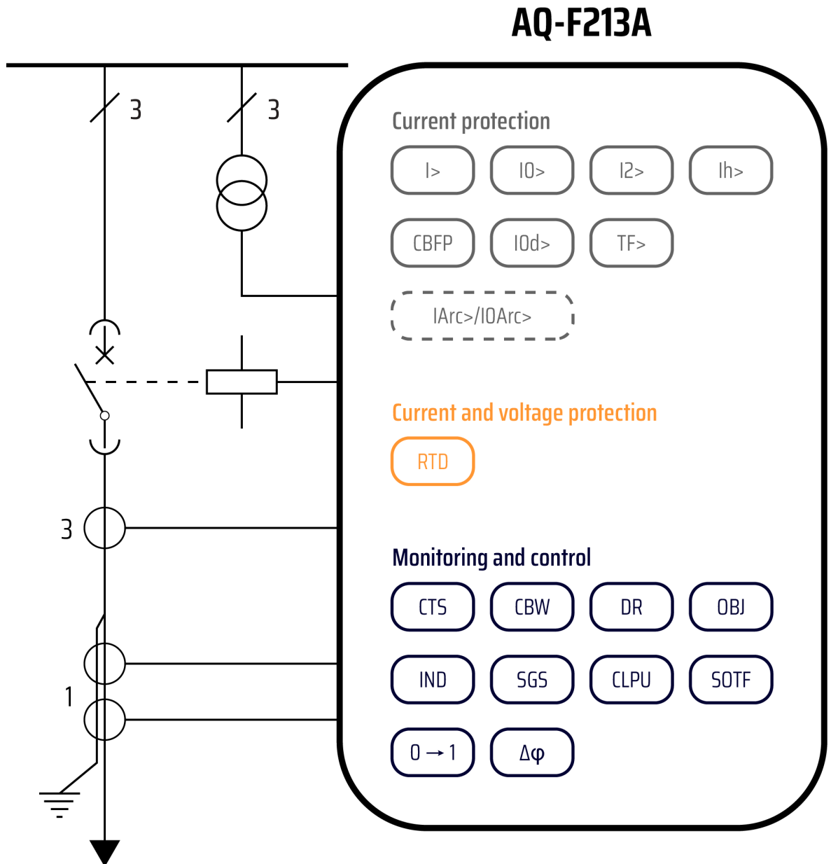
Figure. 6.1 - 230. AQ-F213A application example with function block diagram.
