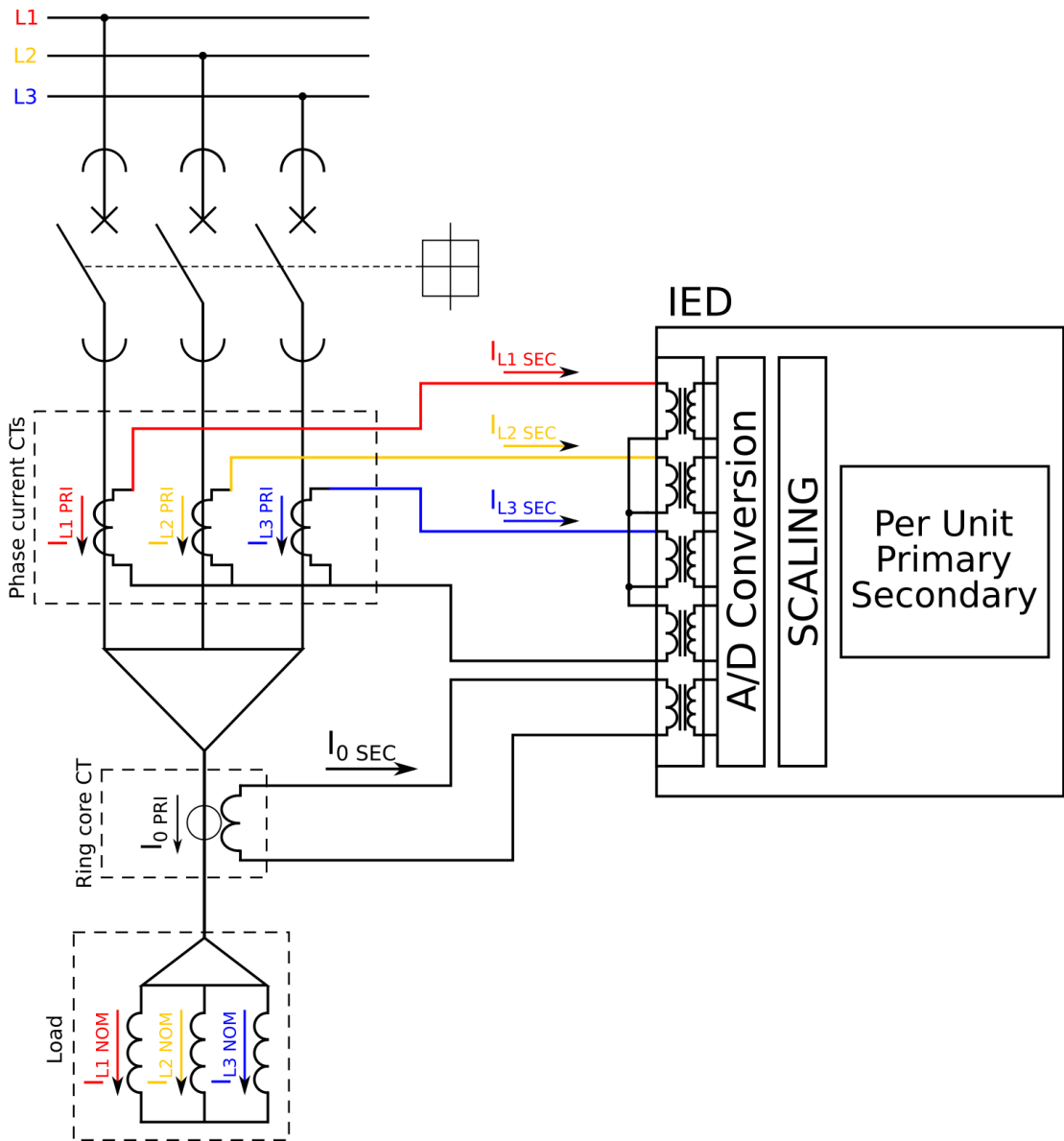
Figure. 4.2.1 - 56. Current measurement terminology.
