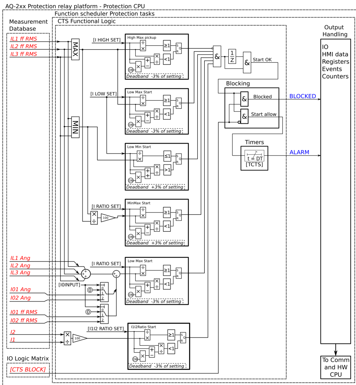
Figure. 4.6.1 - 210. Simplified function block diagram of the CTS function.
