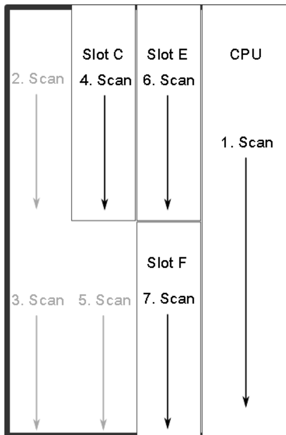
Figure. 7.1 - 243. AQ-X213 hardware scanning and I/O naming principles.
