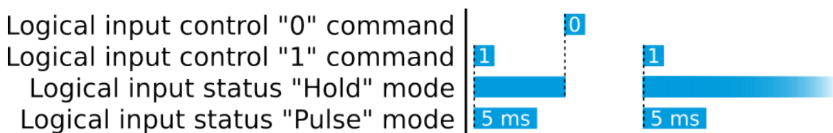
Figure. 4.5.13 - 207. Operation of logical input in "Hold" and "Pulse" modes.
