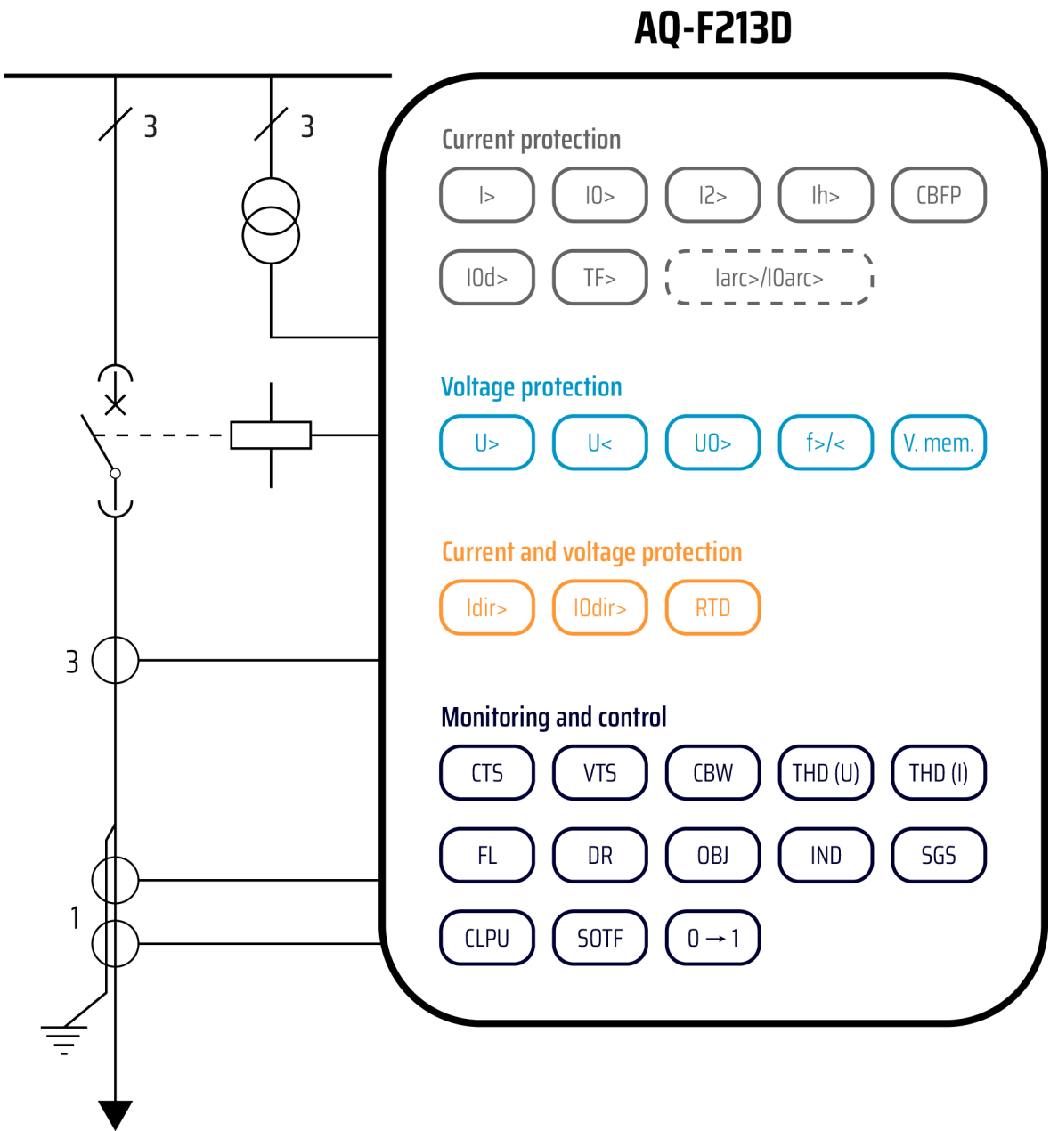
Figure. 6.1 - 233. AQ-F213D application example with function block diagram.
