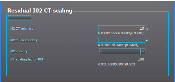
Figure. 4.2.1 - 61. Residual I02 CT scaling (sensitive).
