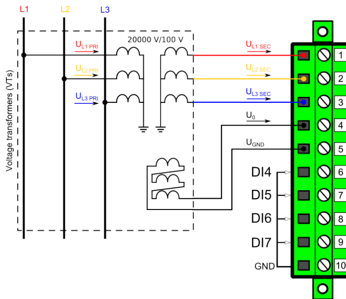
Figure. 4.2.2 - 70. Example connections for 2LL+U0 voltage measurement.
