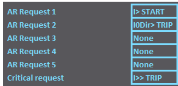
Figure. 4.5.5 - 177. Example of assigning request signals.
