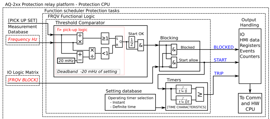
Figure. 4.4.14 - 140. Simplified function block diagram of the f> function.
