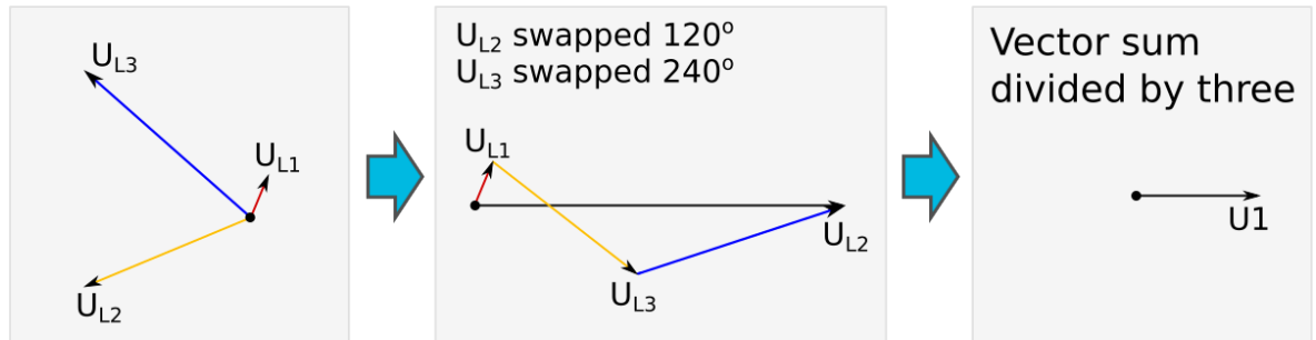
Figure. 4.4.13 - 133. Earth fault in an isolated network.
