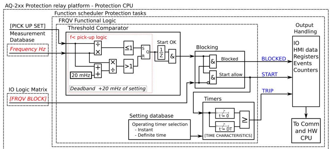
Figure. 4.4.14 - 141. Simplified function block diagram of the f< function.
