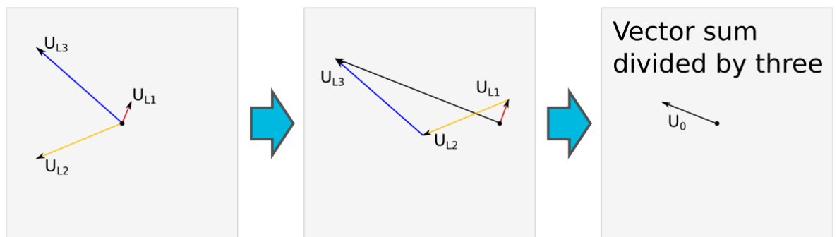
Figure. 4.4.12 - 129. Earth fault in isolated network.
