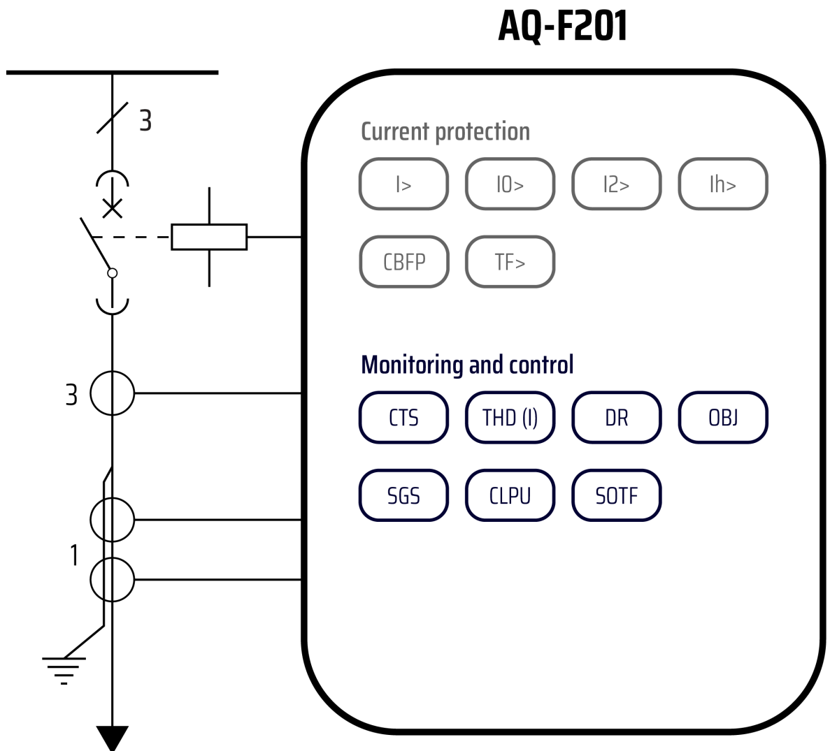
Figure. 6.1 - 140. AQ-F201 application example with function block diagram.
