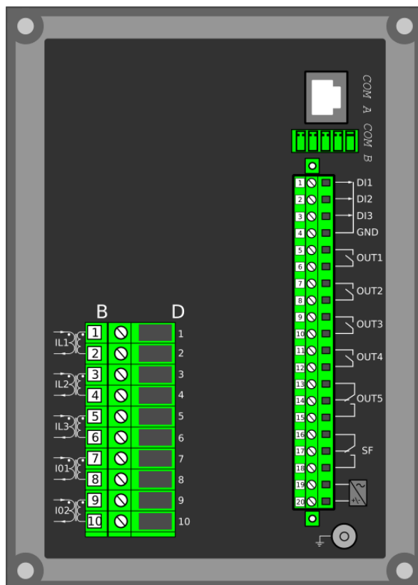
Figure. 7.1 - 148. Connections and modules in AQ-F201.
