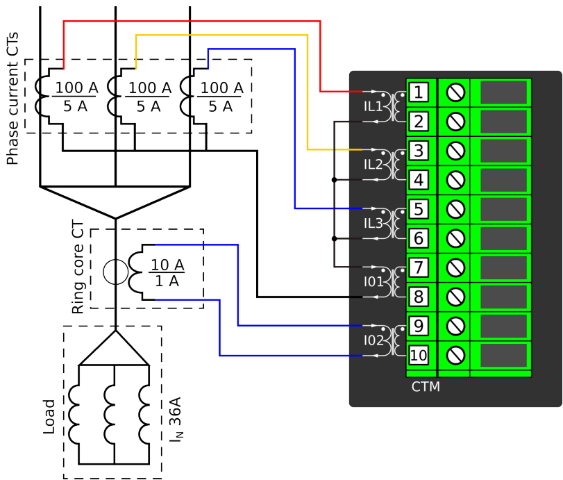
Figure. 4.2.1 - 54. Connections.
