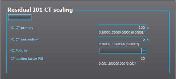
Figure. 4.2.1 - 57. Residual I01 CT scaling (coarse).
