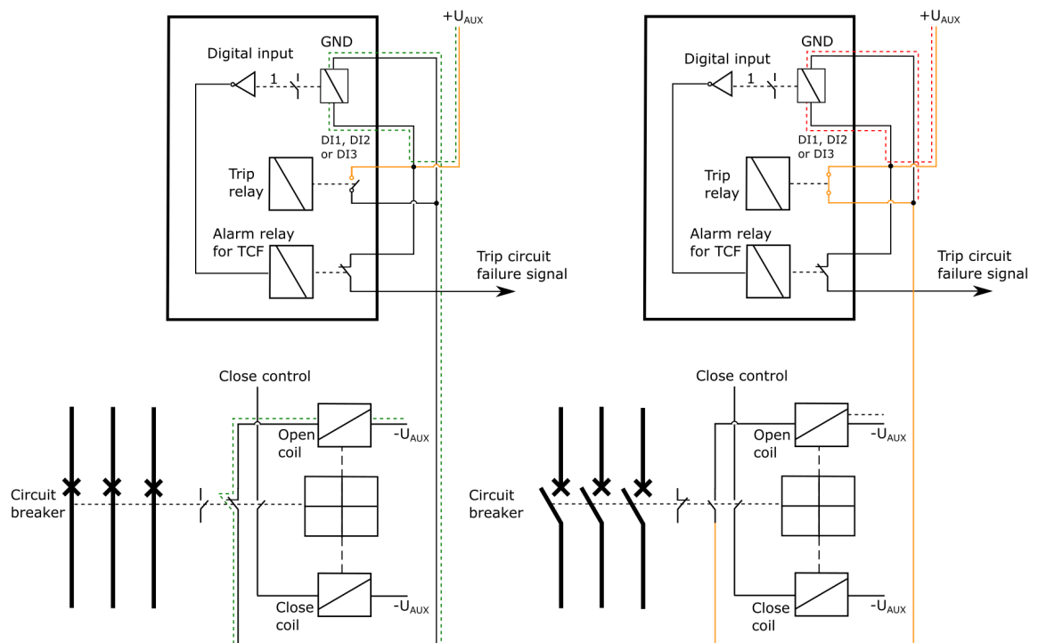
Figure. 6.4 - 146. Trip circuit supervision with one DI and one latched output contact.
