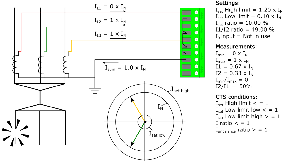
Figure. 4.6.1 - 125. Primary circuit fault in phase L1 wiring.
