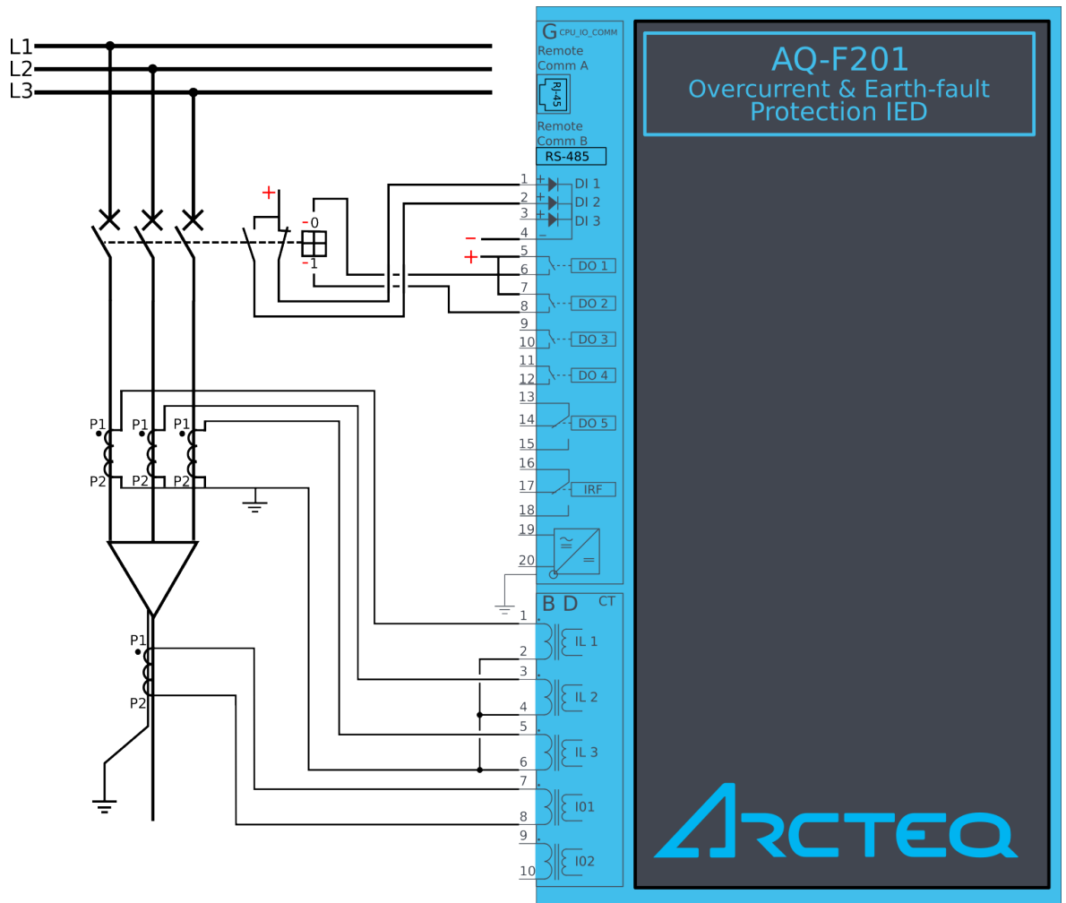
Figure. 6.2 - 141. Application example and its connections.
