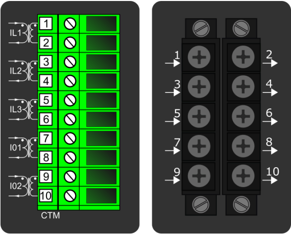
Figure. 7.3 - 150. Module connections with standard and ring lug terminals.
