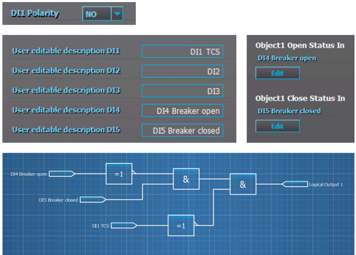
Figure. 6.4 - 147. Example block scheme.
