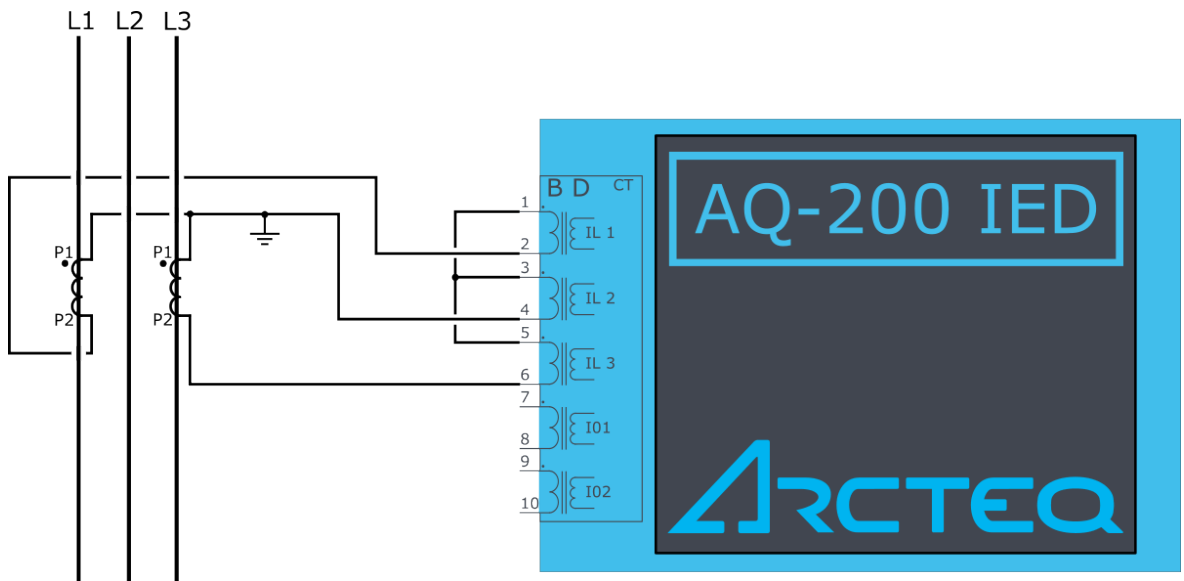
Figure. 6.3 - 142. ARON connection.
