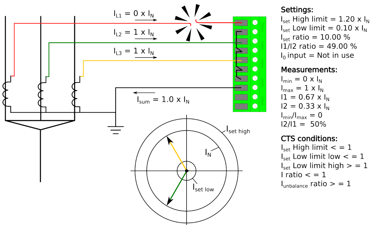
Figure. 4.6.1 - 124. Secondary circuit fault in phase L1 wiring.
