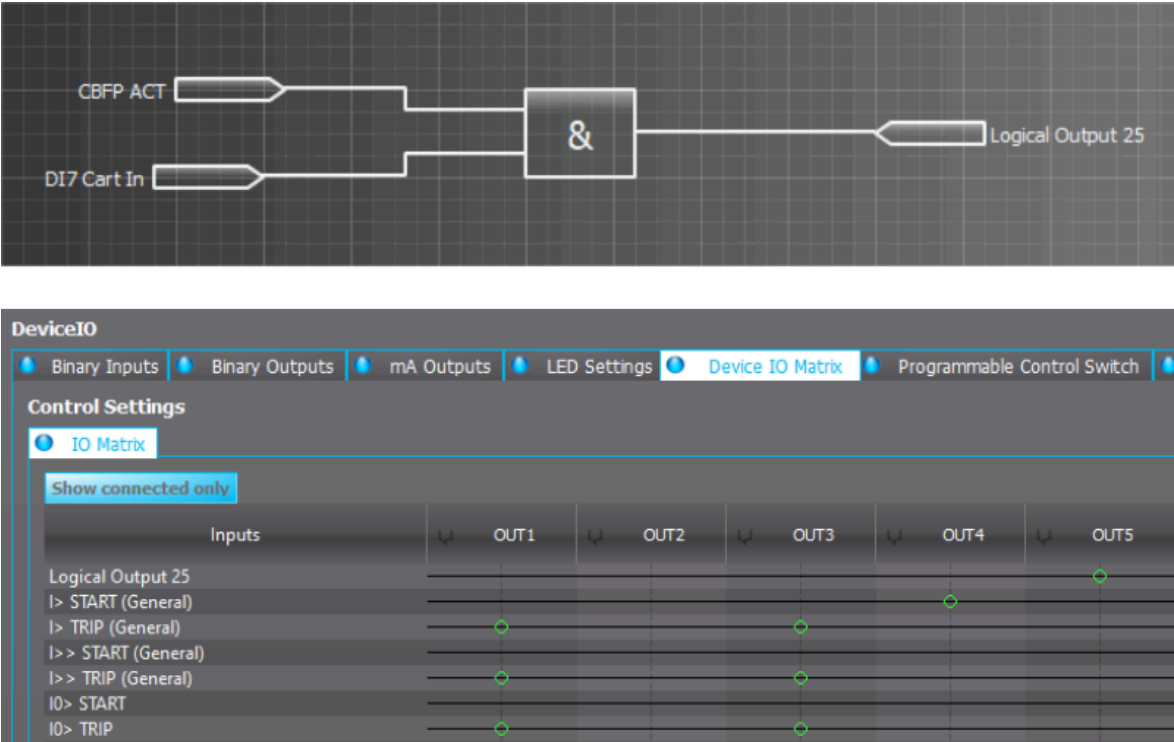
Figure. 4.5.7 - 118. Logic output example. Logical output is connected to an output relay in matrix.
