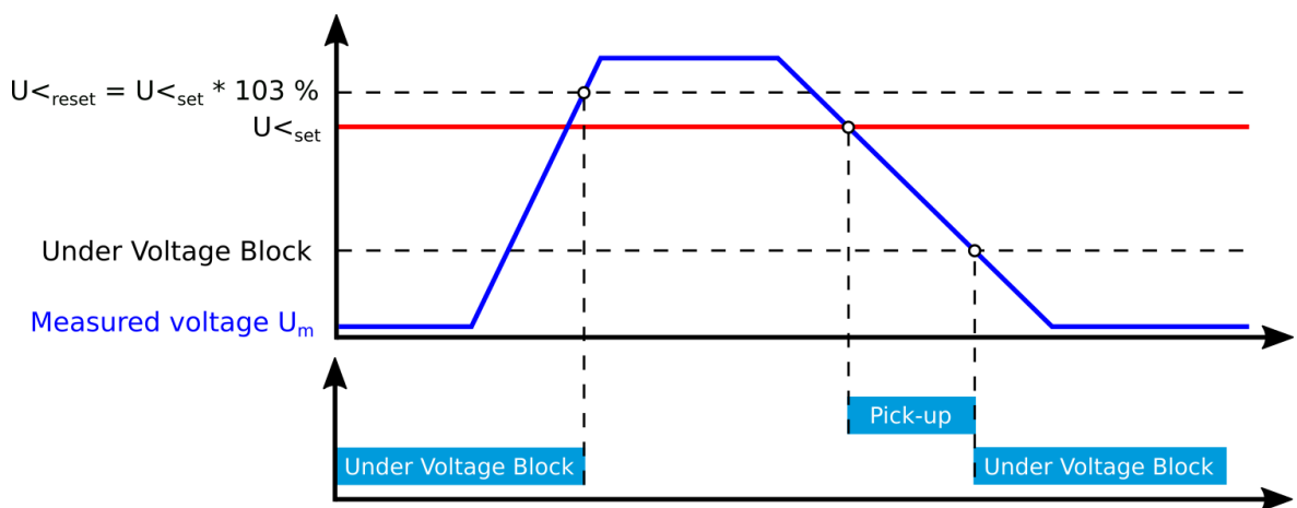
Figure. 4.4.10 - 114. Example of the block setting operation.
