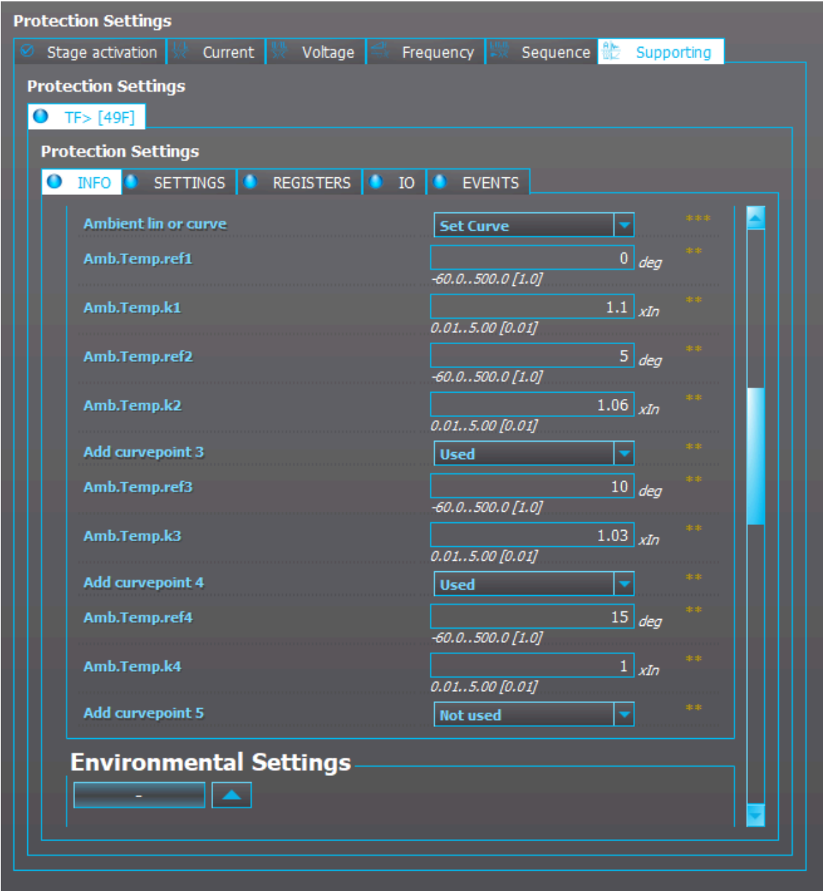
Figure. 4.4.13 - 130. Settings of the function's ambient temperature coefficient curve.
