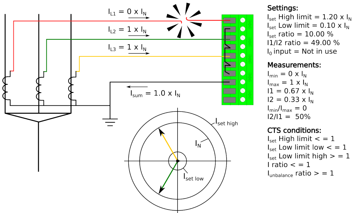
Figure. 4.6.1 - 160. Secondary circuit fault in phase L1 wiring.
