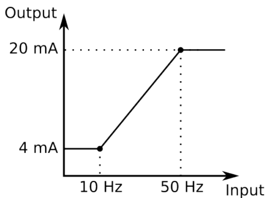
Figure. 4.5.6 - 153. Example of the effects of mA output channel settings.
