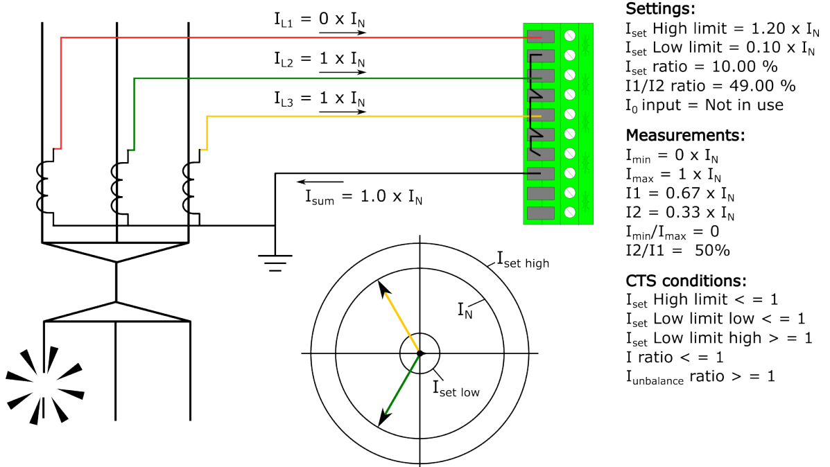
Figure. 4.6.1 - 161. Primary circuit fault in phase L1 wiring.
