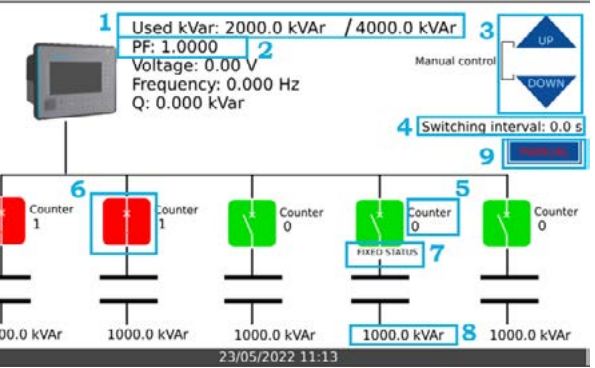
The AQ C255 Power Factor Controller
