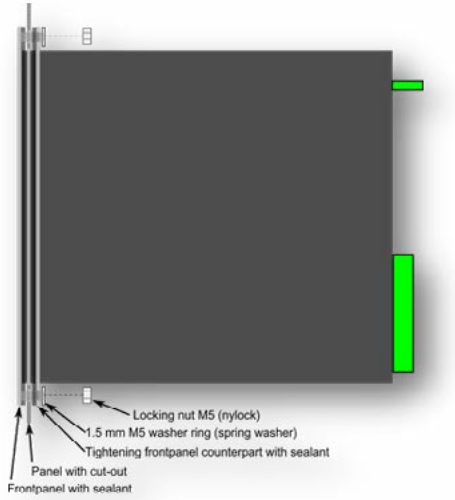
Installation of the AQ-21x device.
