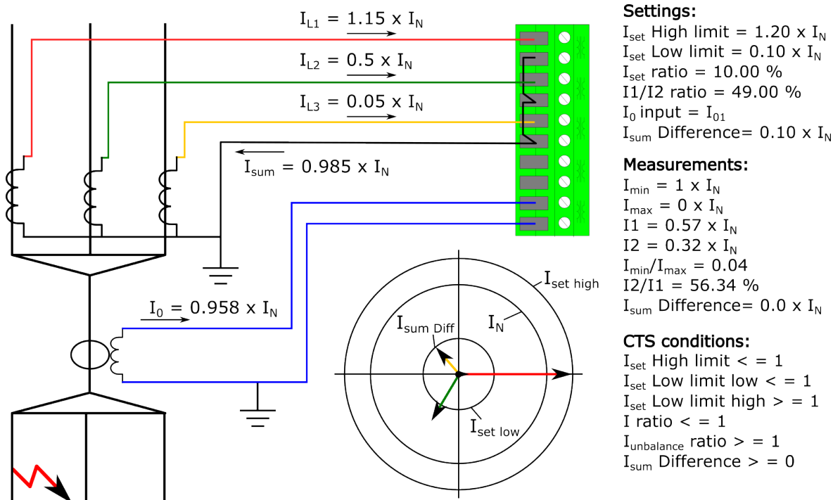
Figure. 4.6.1 - 227. Primary side high-impedance earth fault.
