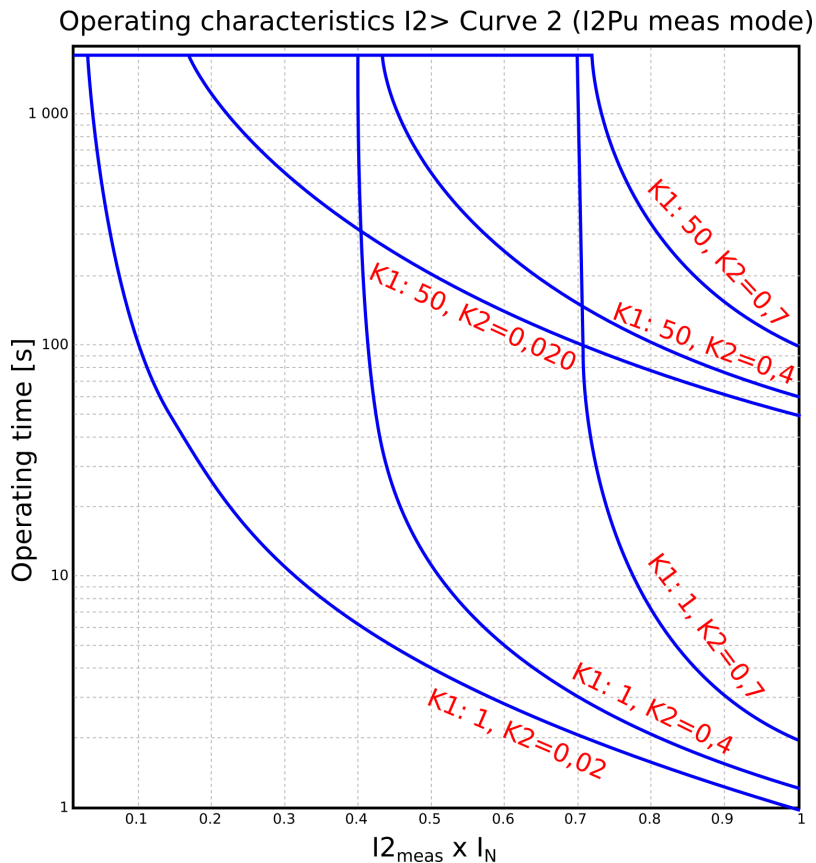
Figure. 4.4.7 - 103. Operation characteristics curve for I2> Curve2.
