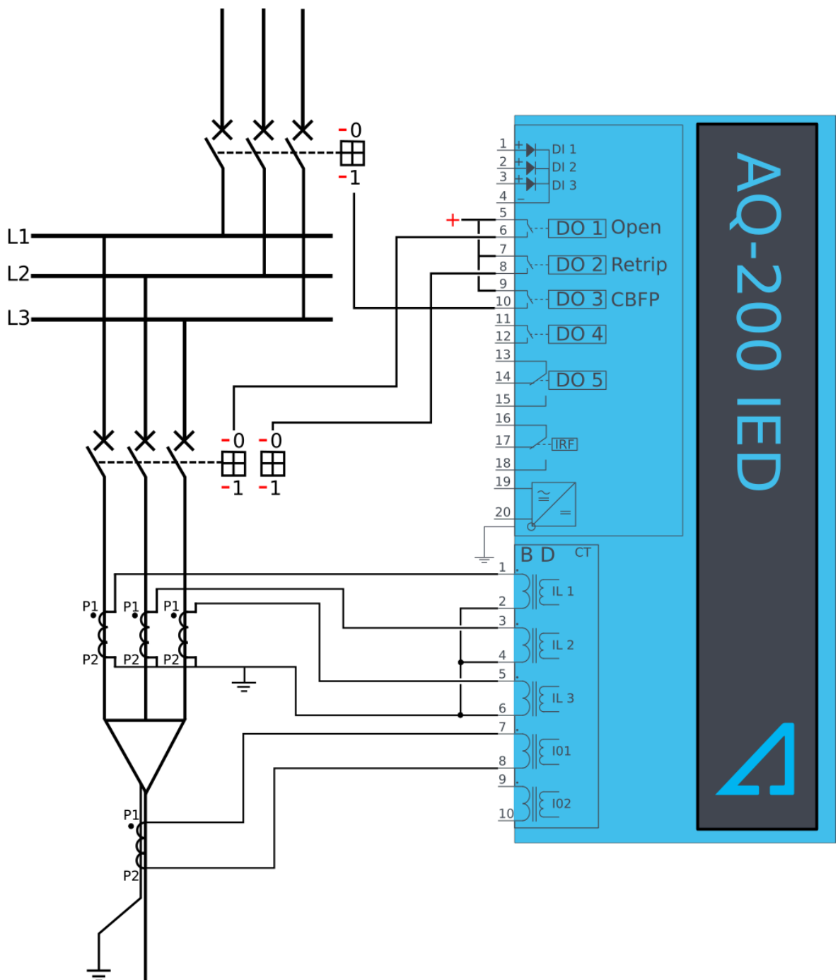
Figure. 4.4.9 - 106. Wiring diagram when Trip, Retrip and CBFP are configured to the device.
