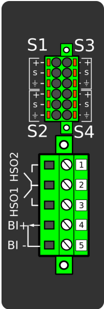
Figure. 7.5.3 - 256. Arc protection module.
