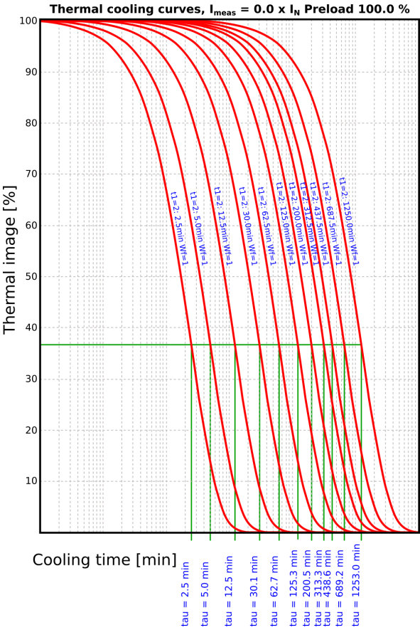
Figure. 4.4.26 - 194. Thermal cooling curves, single cooling time constant.
