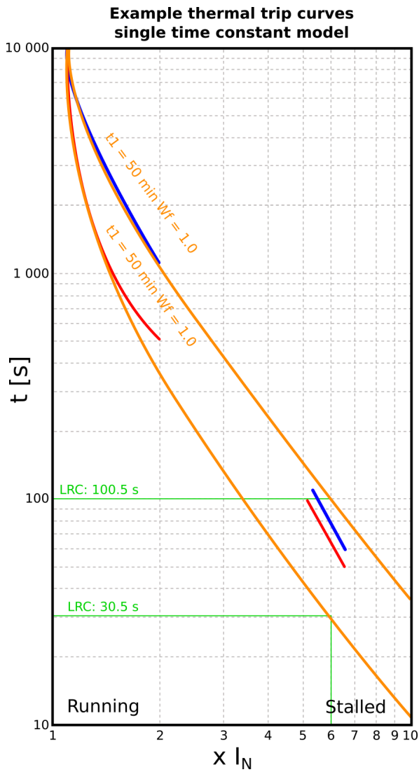
Figure. 4.4.26 - 188. Comparing single time constant thermal replica tripping curves to given motor thermal characteristics.
