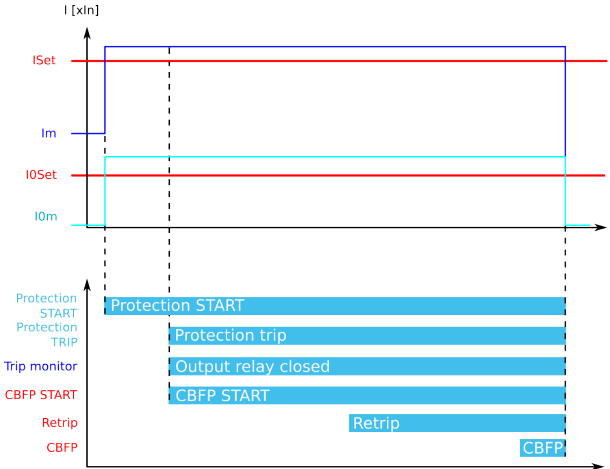
Figure. 4.4.9 - 108. Retrip and CBFP when "Current and DO" is the selected criterion.
