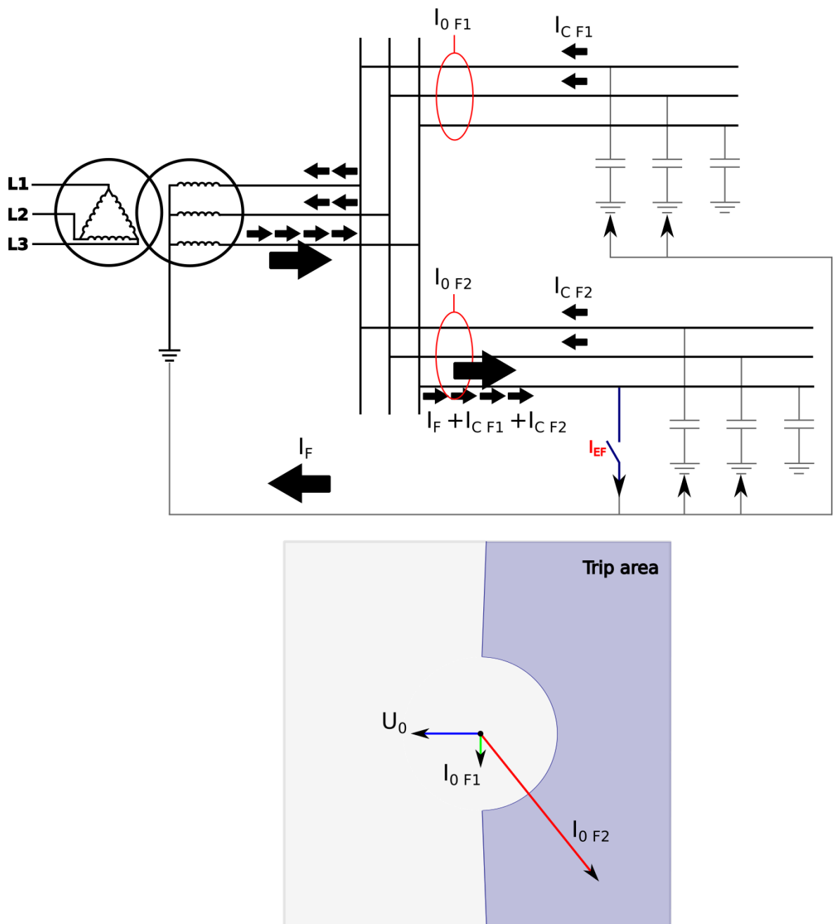
Figure. 4.4.5 - 95. Angle tracking of I_{0dir} function (directly earthed or small impedance network).
