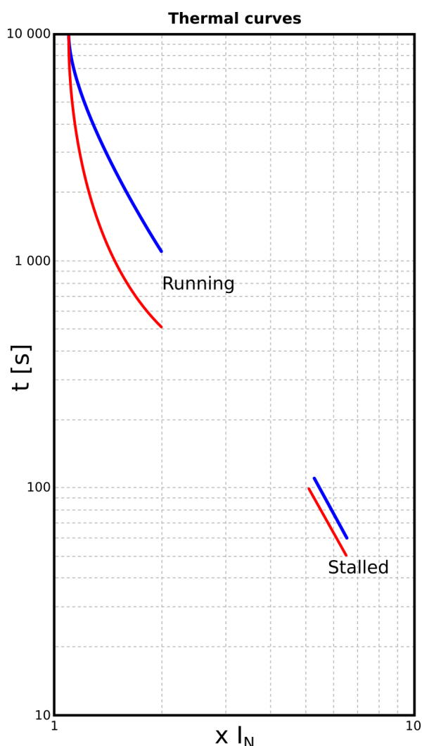
Figure. 4.4.26 - 187. Example of thermal limit curves in a motor.
