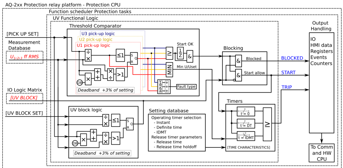
Figure. 4.4.12 - 131. Simplified function block diagram of the U< function.
