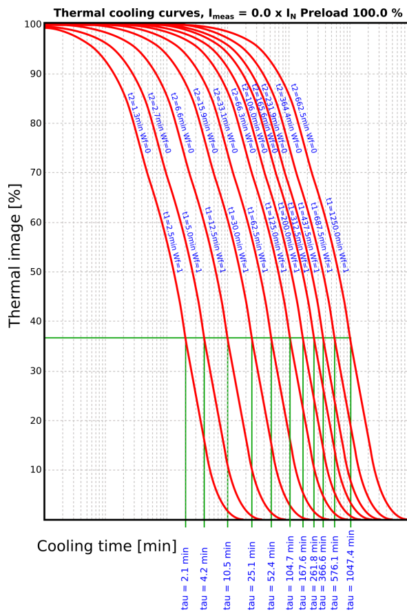
Figure. 4.4.26 - 195. Thermal cooling curves, dynamic dual time constant.
