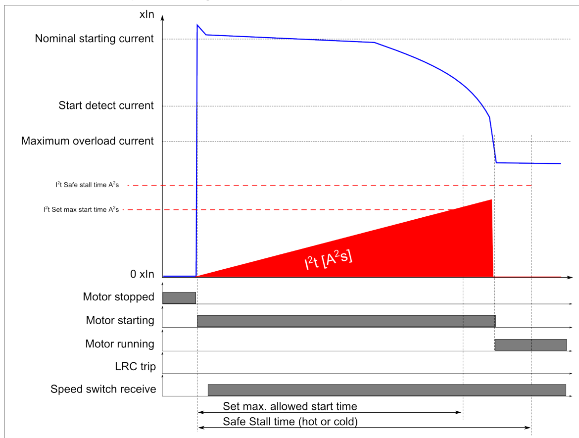
Figure. 4.4.21 - 167. Outputs in long motor starting, with a speed switch.
