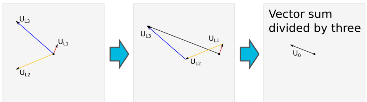
Figure. 4.4.13 - 137. Earth fault in isolated network.
