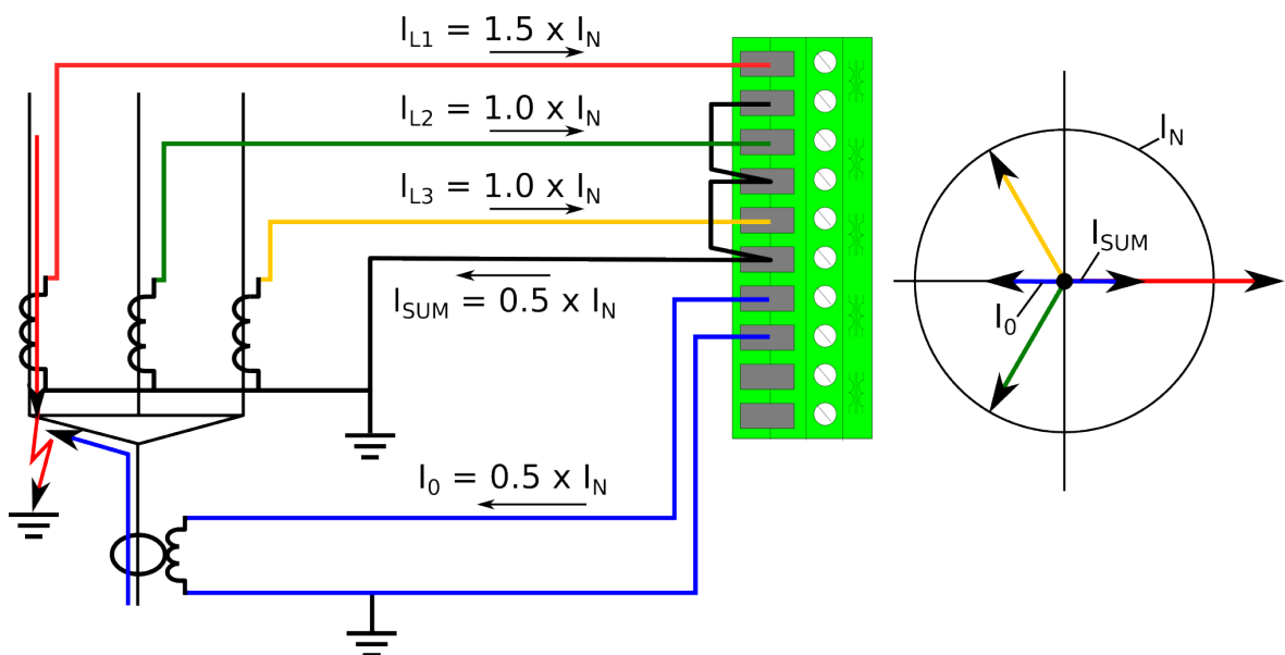
Figure. 4.4.10 - 124. Cable end differential when a fault occurs.
