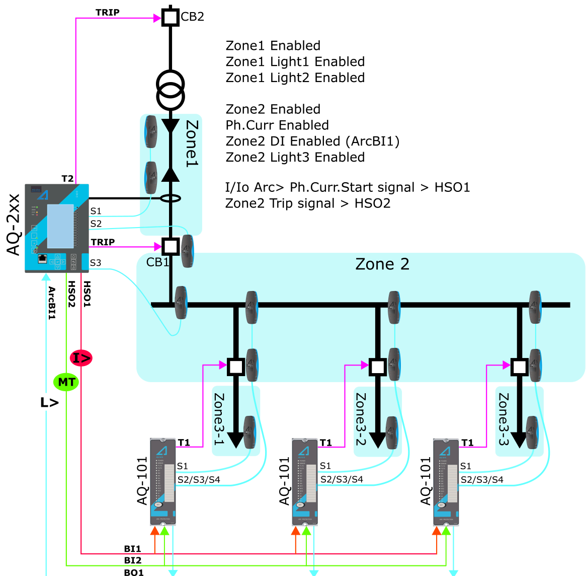
Figure. 4.4.29 - 203. Scheme IA1 (with AQ-101 arc protection relays).
