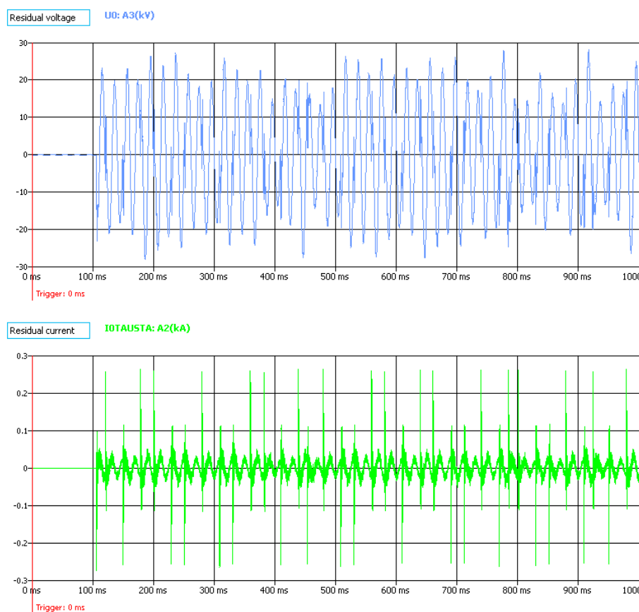
Figure. 4.4.6 - 101. Undercompensated medium size network intermittent earth fault seen by healthy feeder relay.
