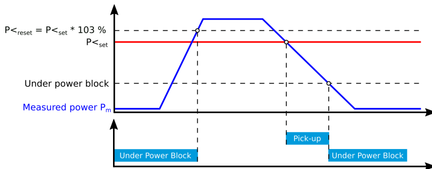
Figure. 4.4.18 - 156. Activation and deactivation characteristics of low power blocking.
