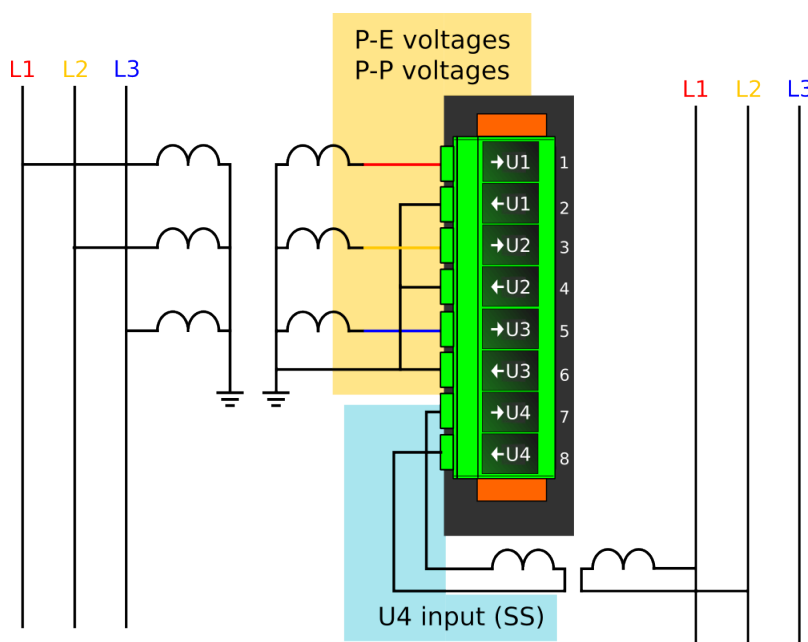
Figure. 4.4.12 - 132. Selectable measurement magnitudes with 3LN+U4 VT connection.
