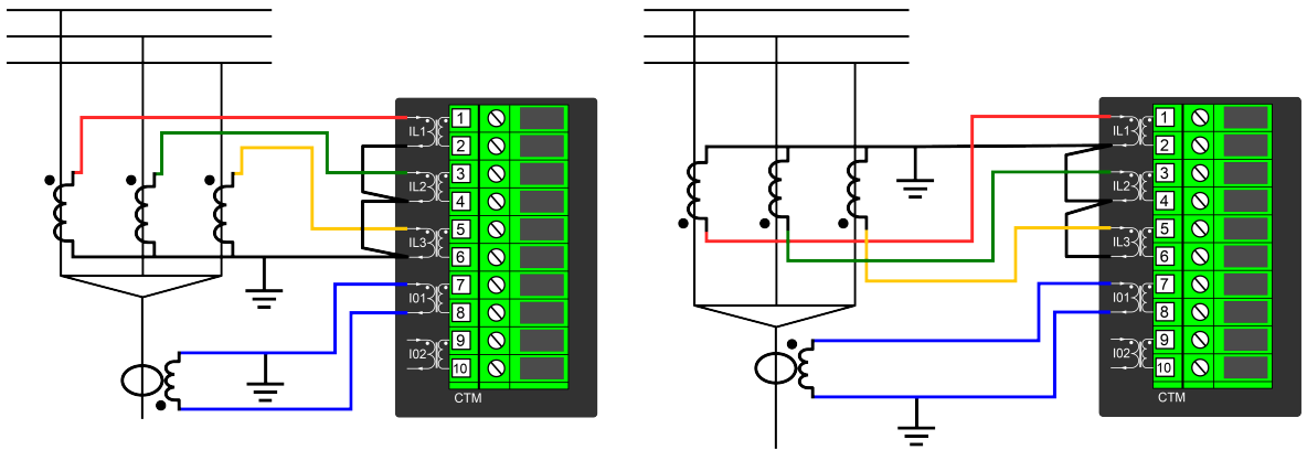
Figure. 4.4.10 - 118. "I0 direction" parameter must be set to "Add" when current transformers are facing each other or away from each other.
