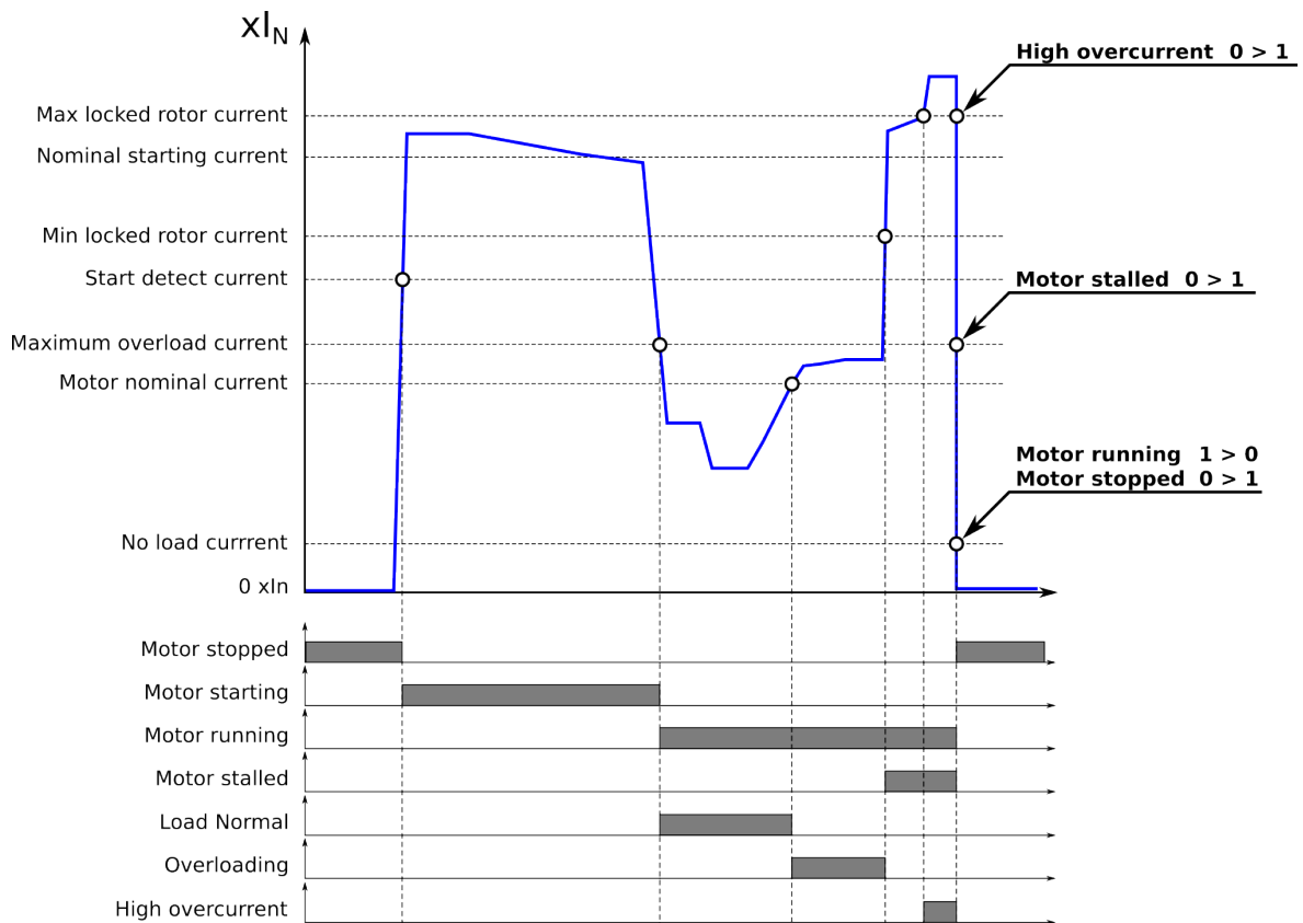
Figure. 4.4.20 - 160. Activation of the function's outputs.
