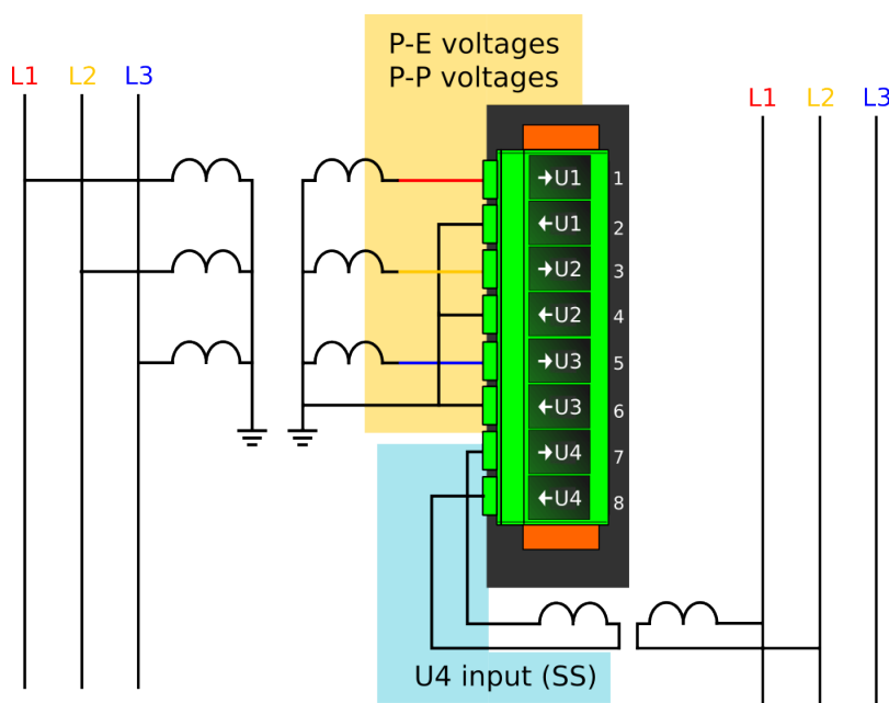
Figure. 4.4.11 - 128. Selectable measurement magnitudes with 3LN+U4 VT connection.
