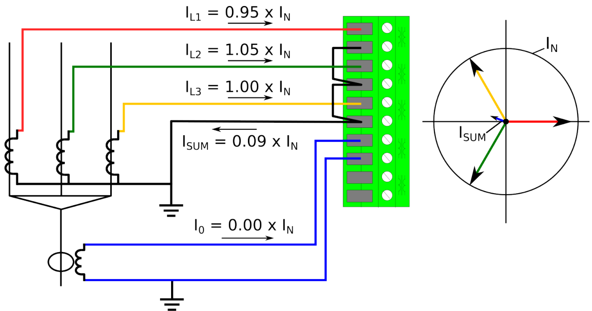
Figure. 4.4.10 - 123. Cable end differential with natural unbalance in the phase current measurement.
