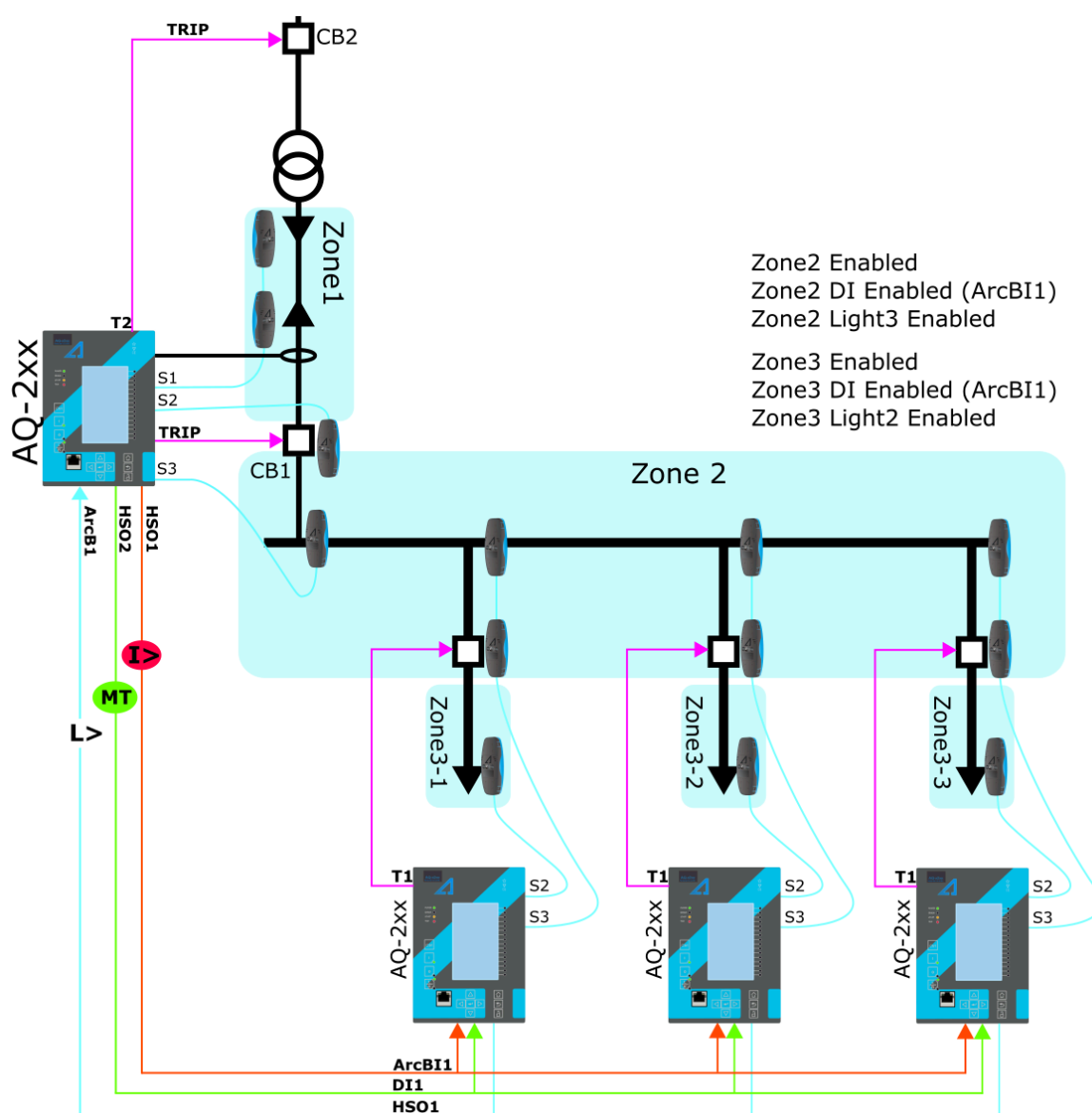
Figure. 4.4.29 - 204. Scheme IA1 (with AQ-200 protection relays).
