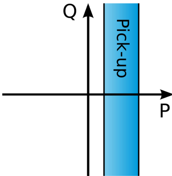
Figure. 4.4.18 - 154. Operating characteristics of underpower protection.
