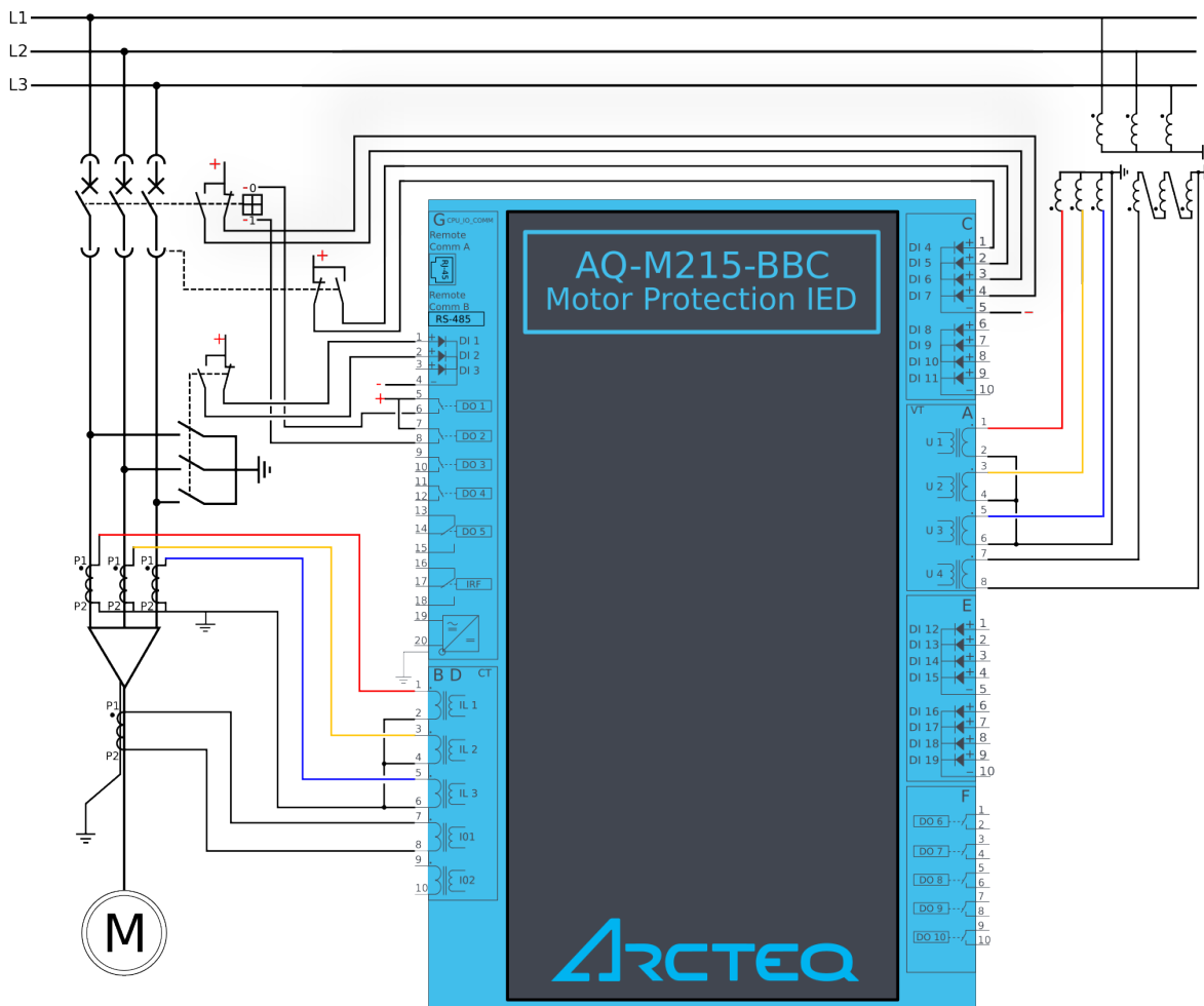
Figure. 6.2 - 241. Application example and its connections.
