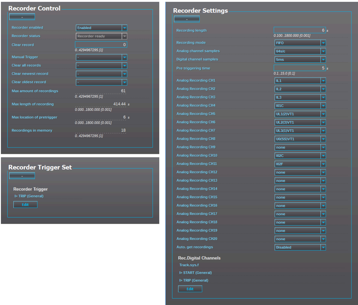
Figure. 4.6.5 - 234. Disturbance recorder settings.
