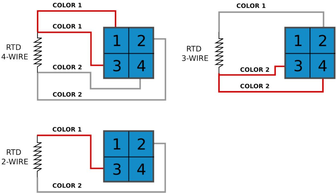
Figure. 7.5.4 - 258. RTD sensor connection types.
