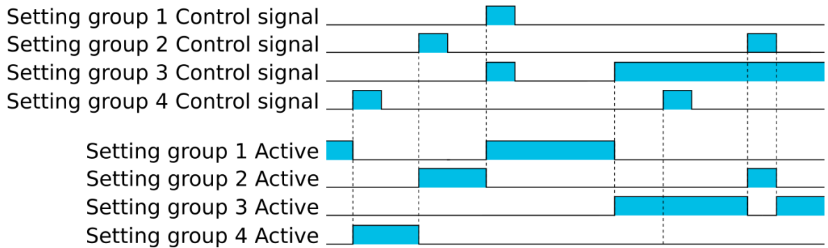
Figure. 4.5.2 - 206. Example sequences of group changing (control with pulse only, or with both pulses and static signals).
