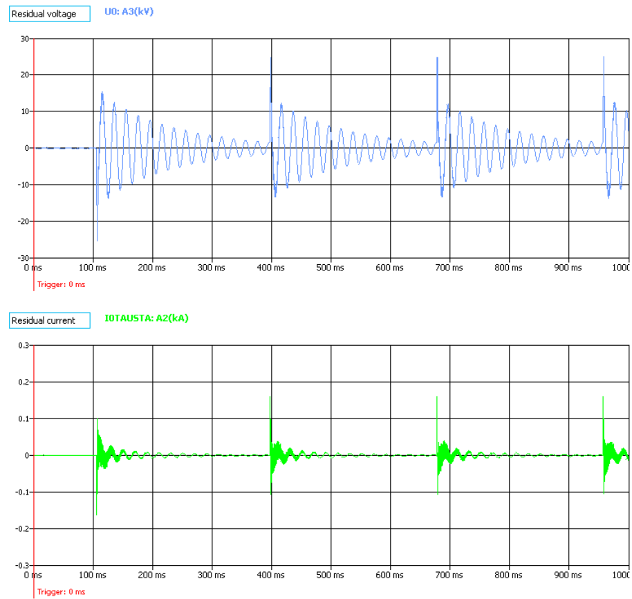
Figure. 4.4.6 - 99. An intermittent earth fault in a network tuned close to resonance, as seen by a healthy feeder relay.
