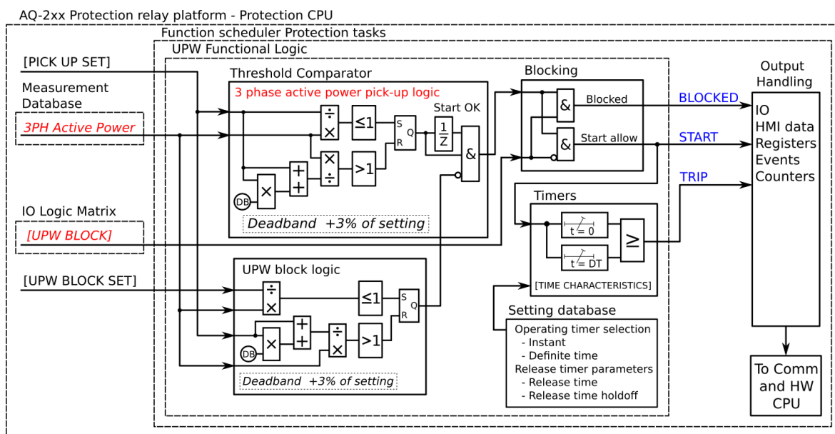
Figure. 4.4.18 - 155. Simplified function block diagram of the P < function.
