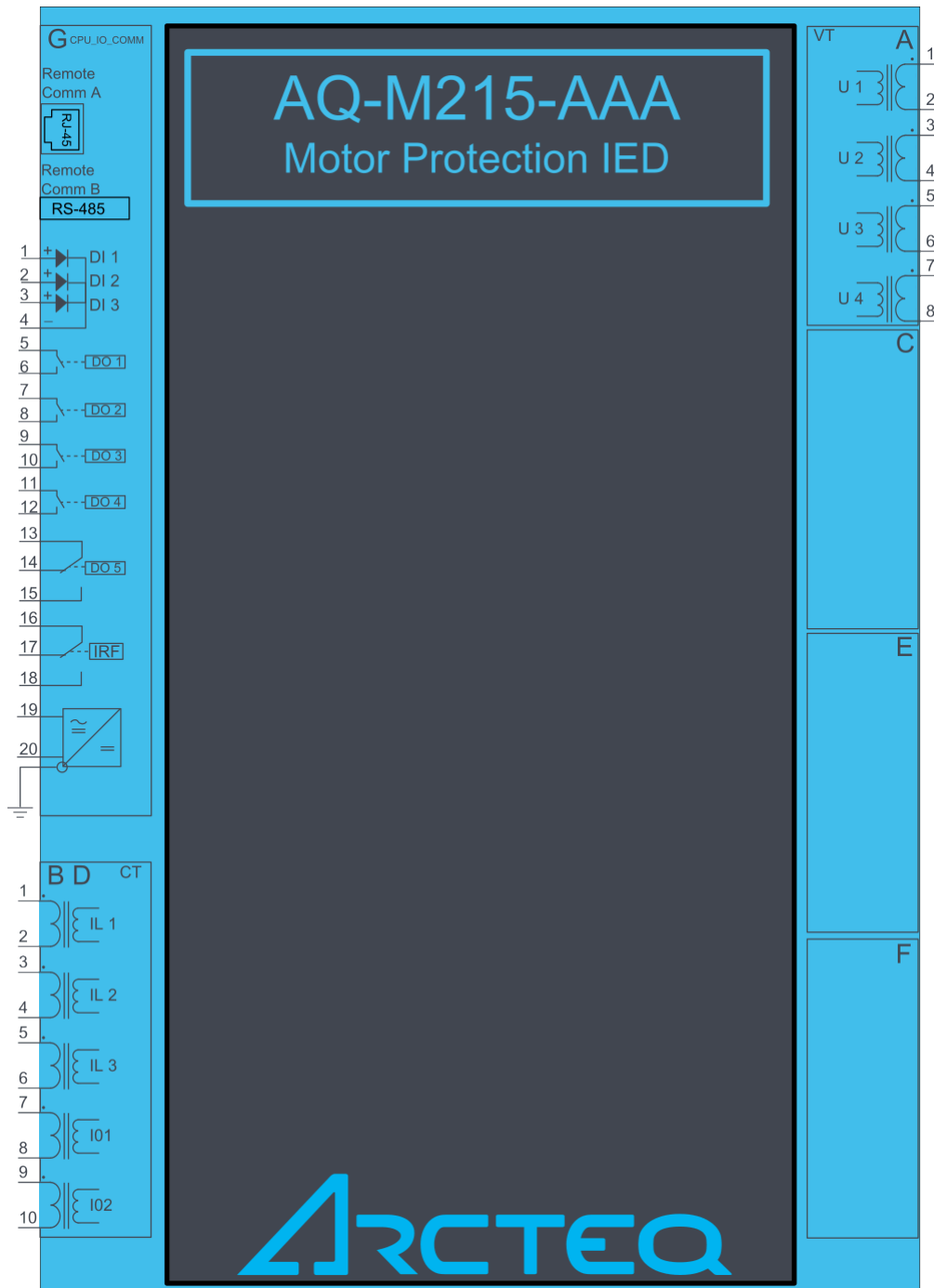
Figure. 6.1 - 238. AQ-M215 variant without add-on modules.
