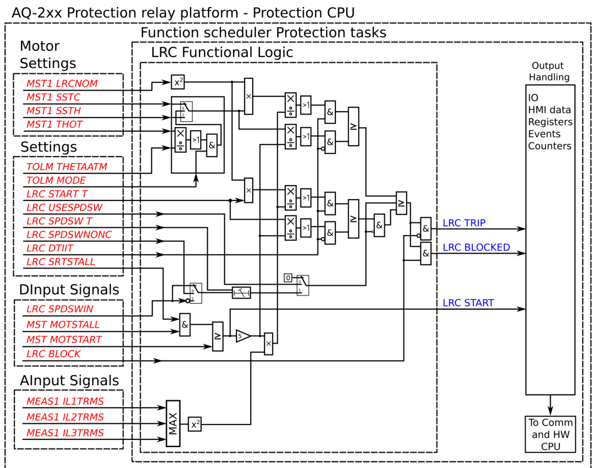
Figure. 4.4.21 - 164. Simplified function block diagram of the motor start/ locked rotor monitoring function.
