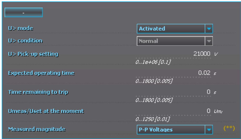
Figure. 4.2.2 - 68. Selecting the measured magnitude.
