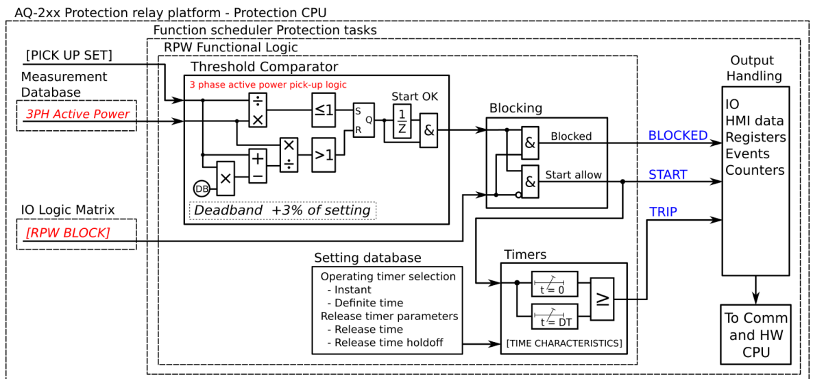
Figure. 4.4.19 - 158. Simplified function block diagram of the Pr function.
