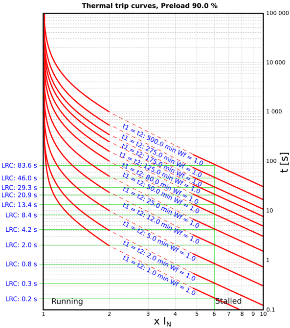
Figure. 4.4.26 - 191. Thermal tripping curves with single time constant, pre-load 90% (hot).
