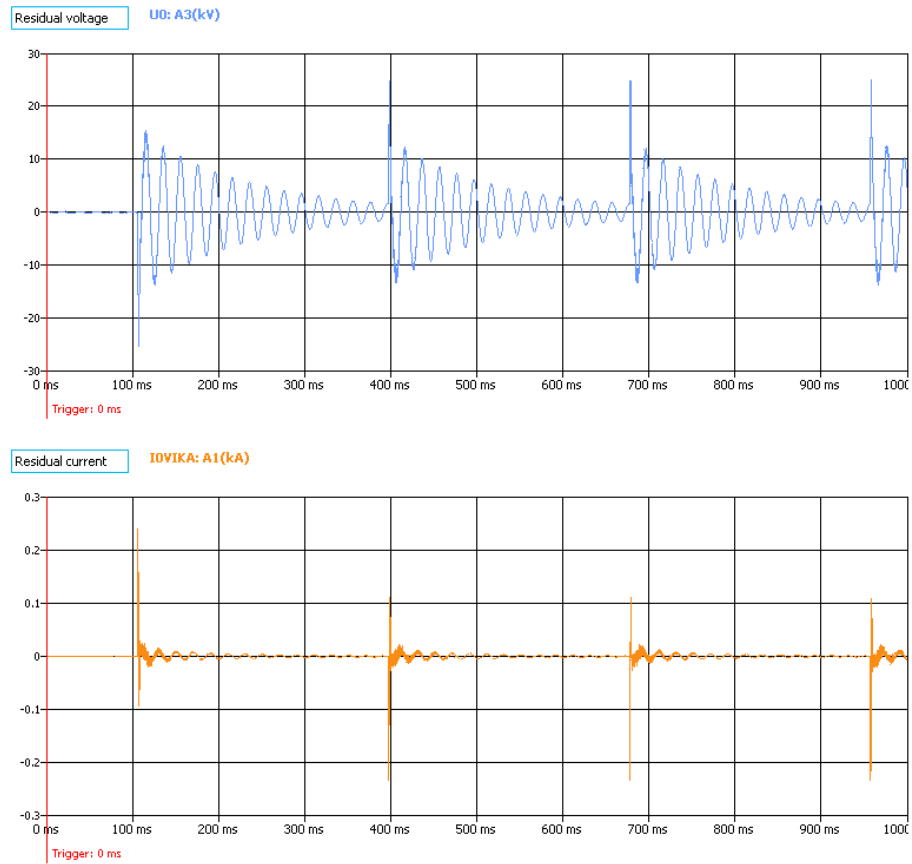
Figure. 4.4.6 - 98. An intermittent earth fault in a medium size network tuned close to resonance, as seen by a faulty feeder relay.
