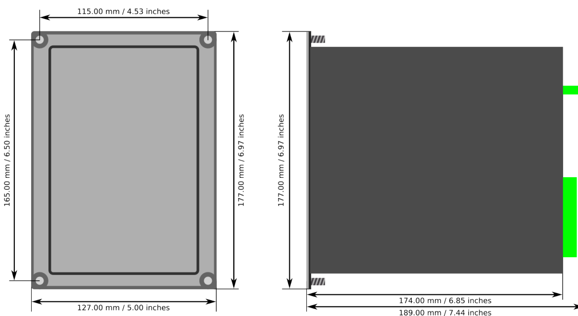
Figure. 7.6 - 267. Device dimensions.
