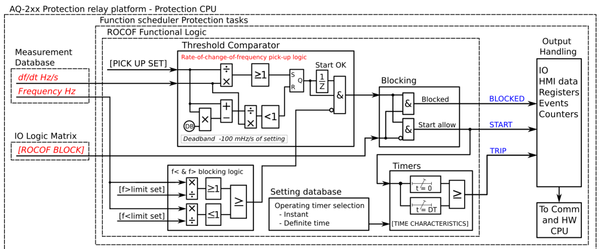
Figure. 4.4.16 - 151. Simplified function block diagram of the df/dt > / < function.
