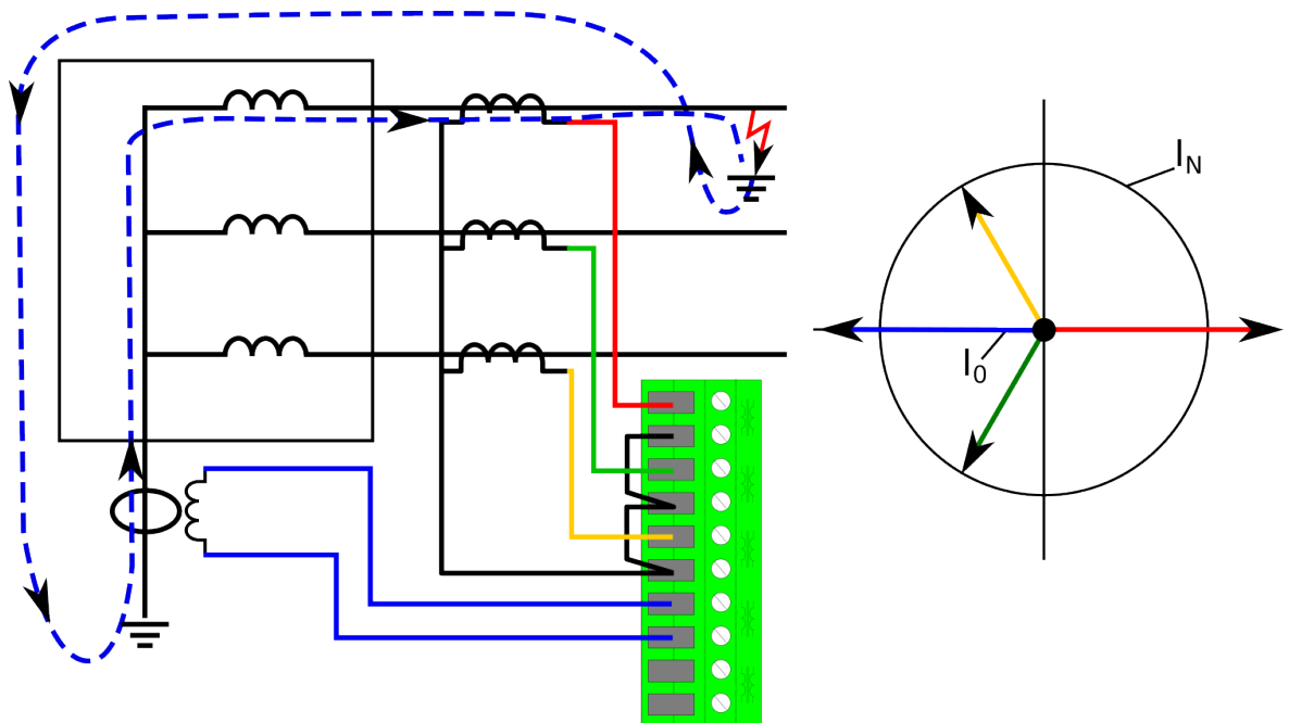
Figure. 4.4.10 - 125. Restricted earth fault outside a Y winding transformer.
