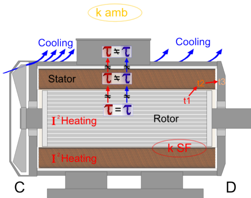
Figure. 4.4.26 - 183. Simplified motor construction and time constants.
