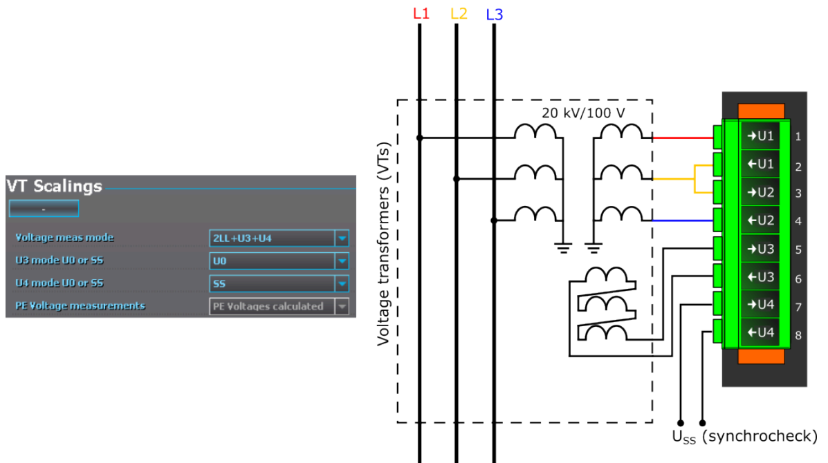
Figure. 4.2.2 - 71. 2LL+U_0+SS settings and connections.
