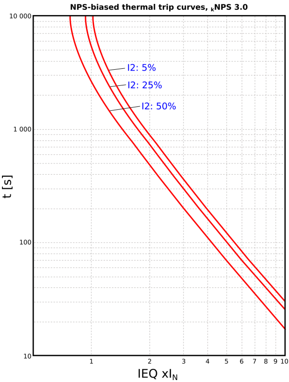
Figure. 4.4.26 - 198. NPS-biased thermal trip curves with k_{NPS} value of 3.
