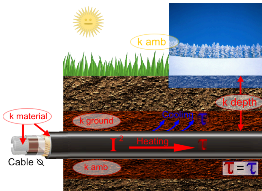
Figure. 4.4.26 - 182. Factors affecting the cooling and current-carrying capacity of a cable.
