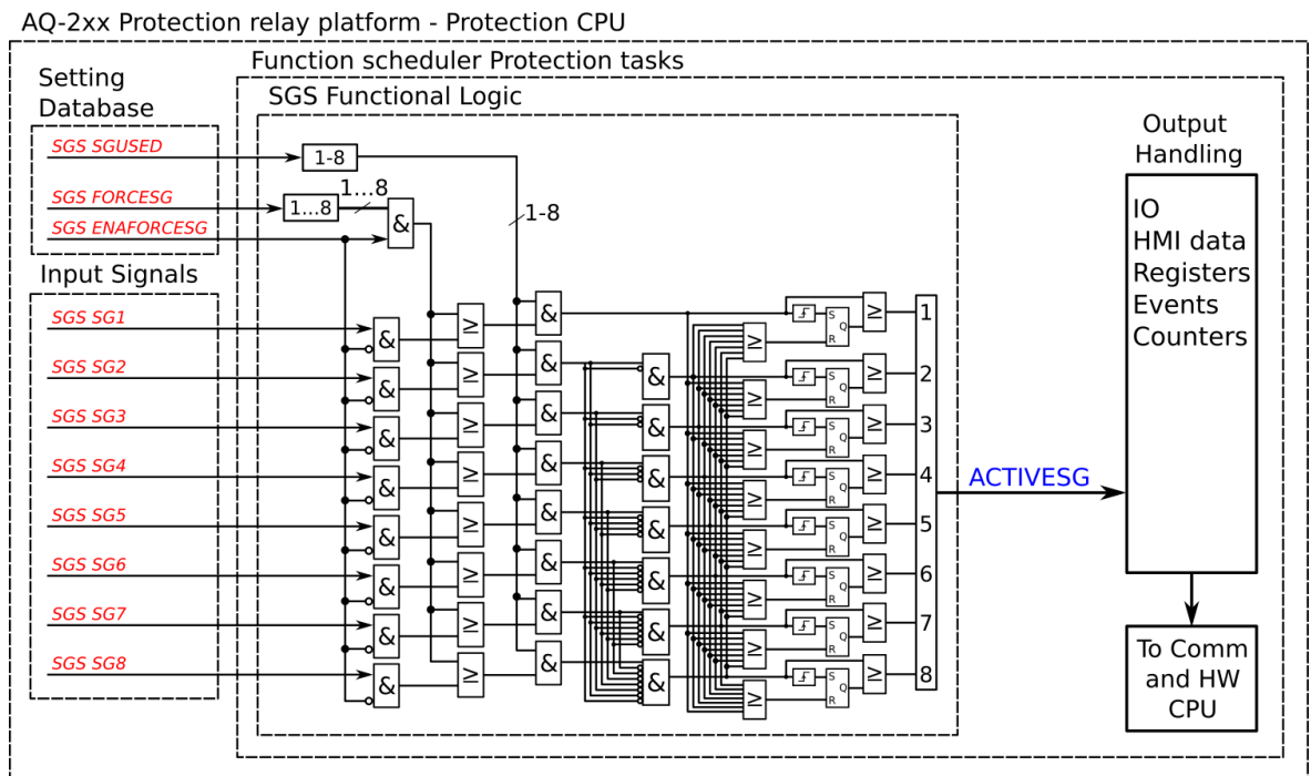
Figure. 4.5.2 - 205. Simplified function block diagram of the setting group selection function.
