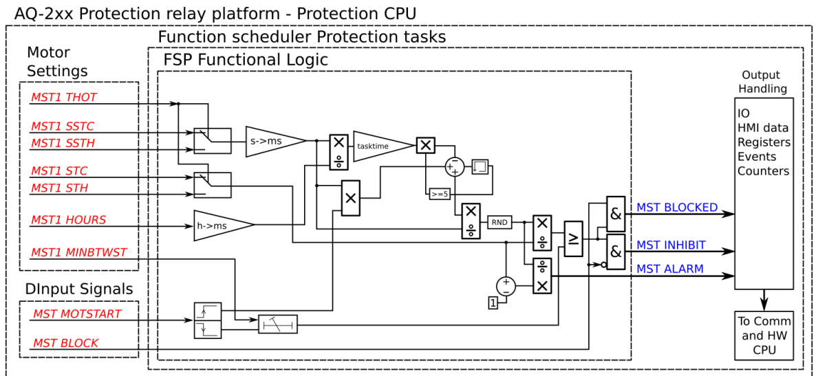
Figure. 4.4.22 - 170. Simplified function block diagram of the N> function.
