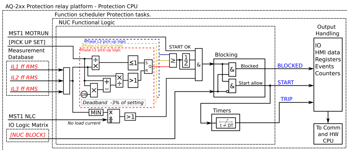
Figure. 4.4.23 - 173. Simplified function block diagram of the I< function.
