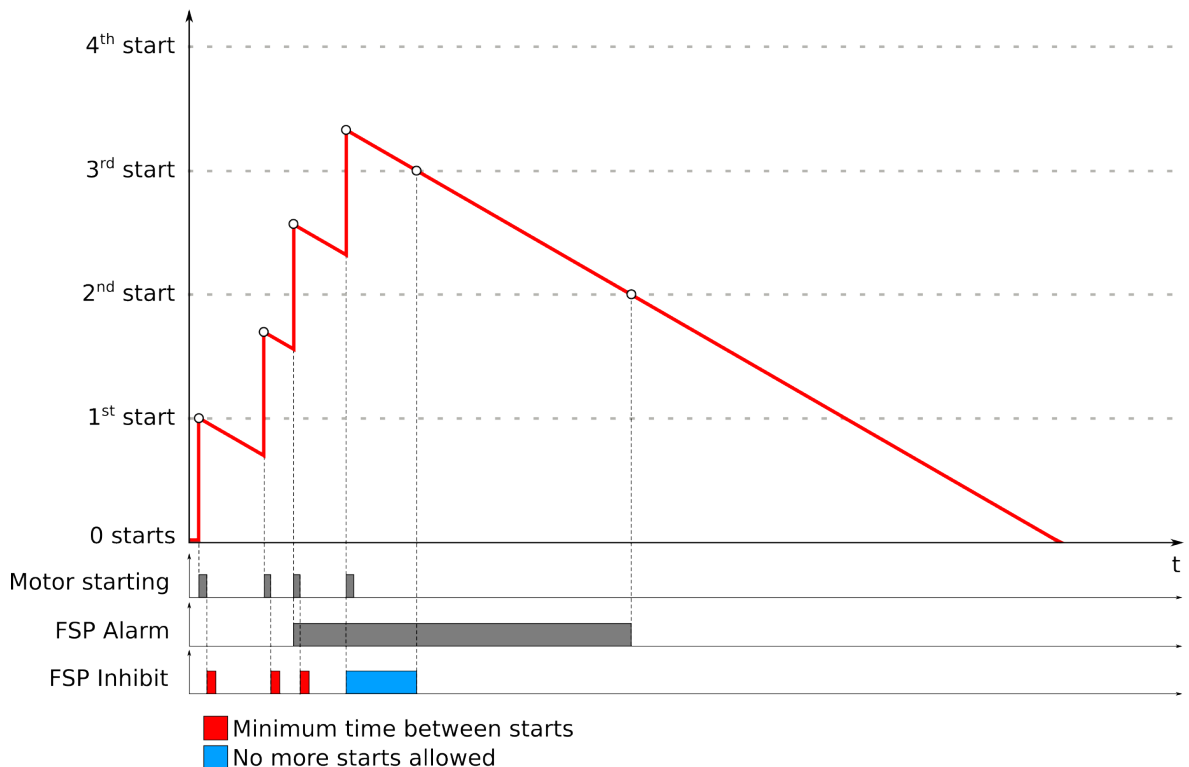
Figure. 4.4.22 - 171. Updating the function's start counter (image not to scale with regard to time).
