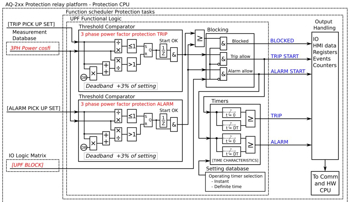
Figure. 4.4.25 - 176. Simplified function block diagram of the PF> function.
