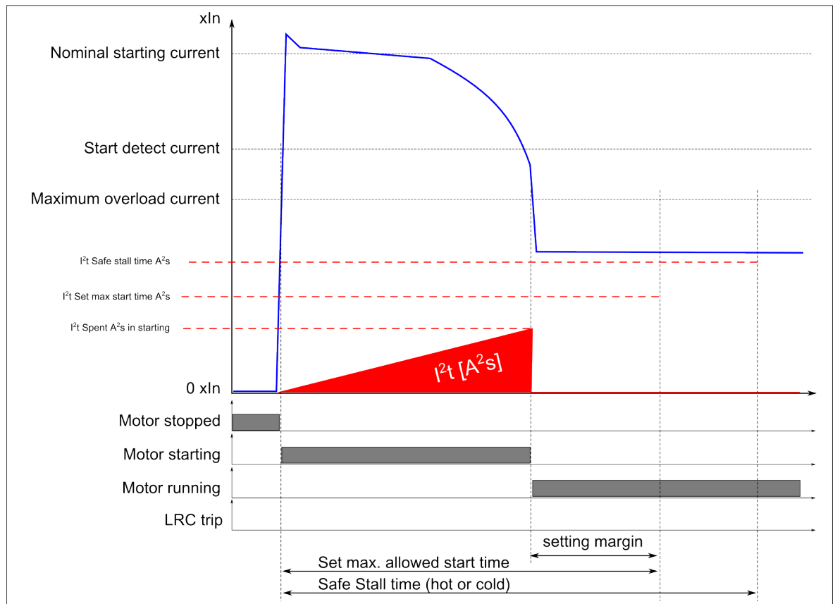
Figure. 4.4.21 - 165. Outputs in normal motor start, no speed switch.
