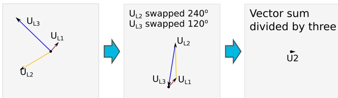
Figure. 4.4.14 - 144. Earth fault in isolated network.
