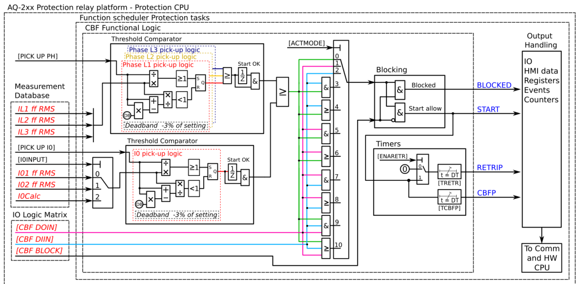
Figure. 4.4.9 - 105. Simplified function block diagram of the CBFP function.
