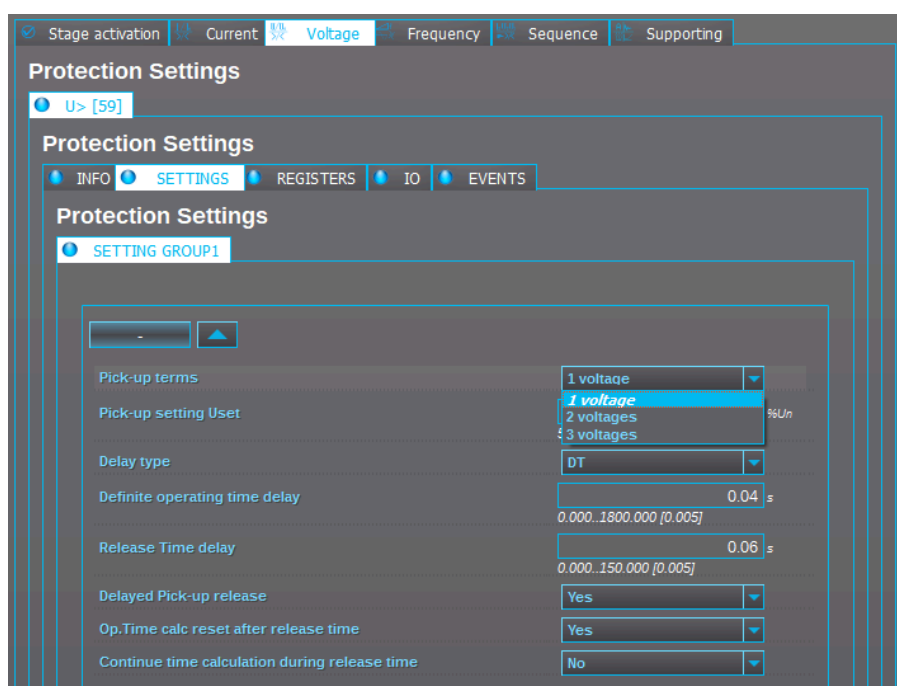
Figure. 4.2.2 - 69. Selecting the operating mode.
