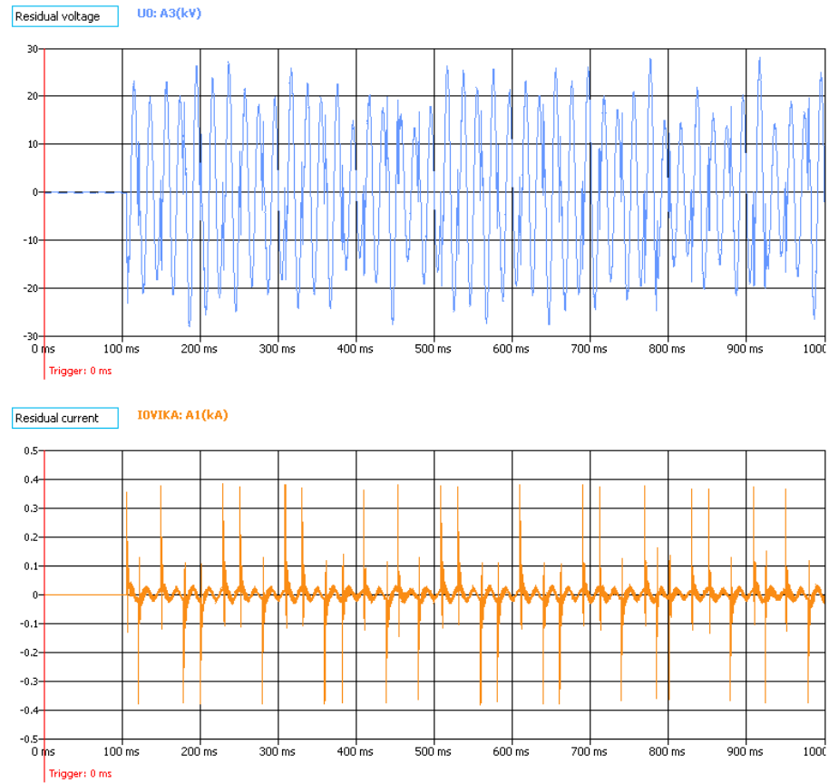
Figure. 4.4.6 - 100. An intermittent earth fault in an undercompensated medium size network, as seen by a faulty feeder relay.
