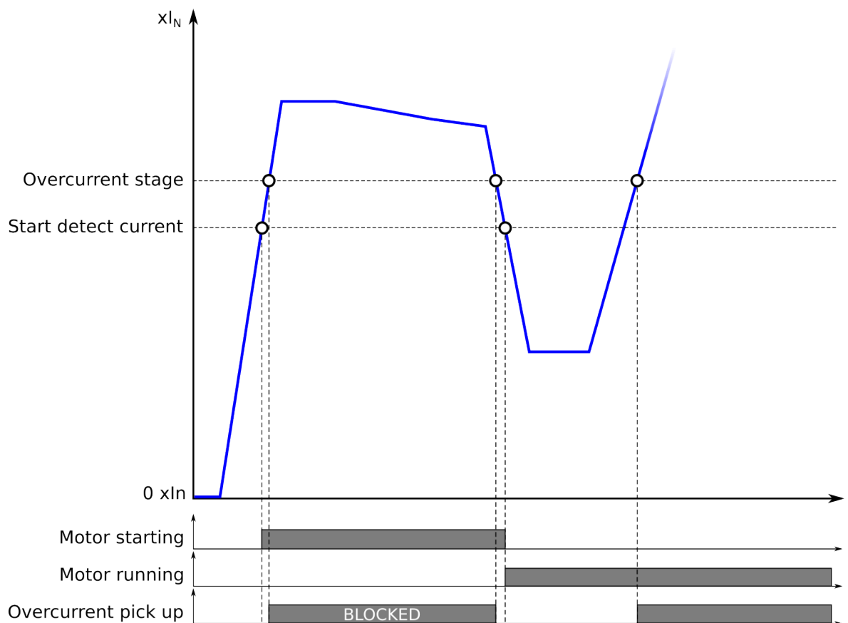
Figure. 4.4.20 - 161. Example of application: motor starting scheme and using motor status signals.
