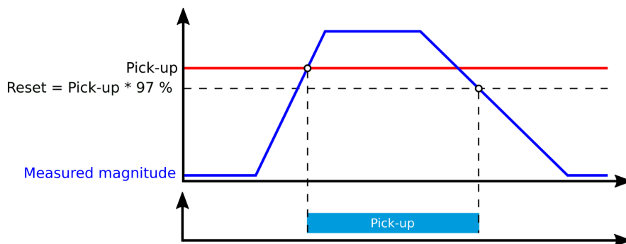
Figure. 4.4.1 - 78. Pick up and reset.
