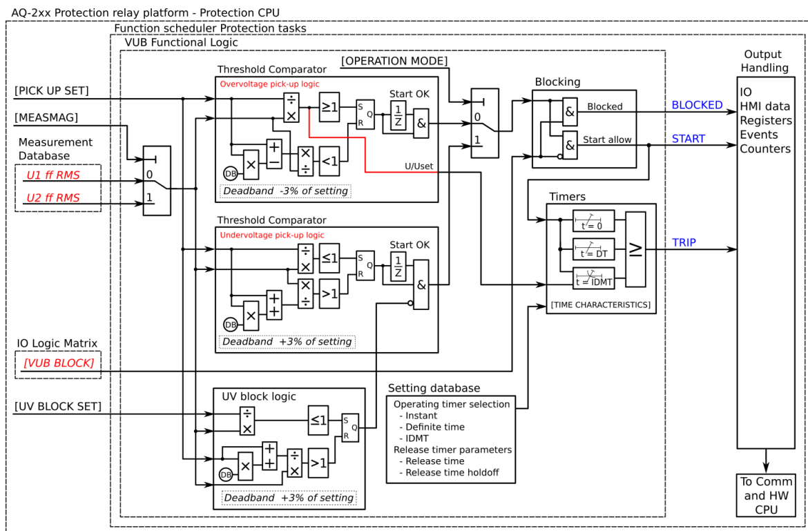
Figure. 4.4.14 - 146. Simplified function block diagram of the U1/U2>/< function.
