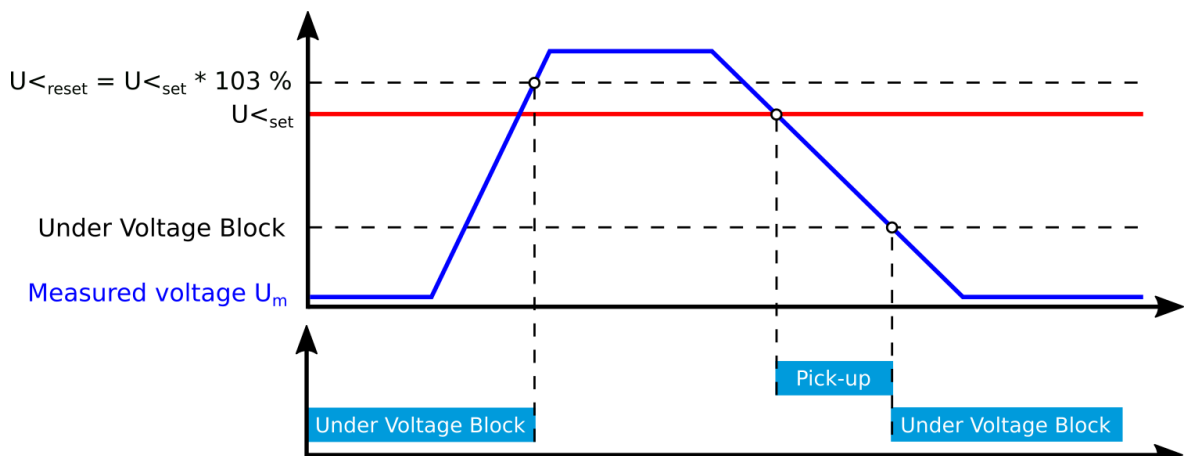
Figure. 4.4.12 - 135. Example of the block setting operation.
