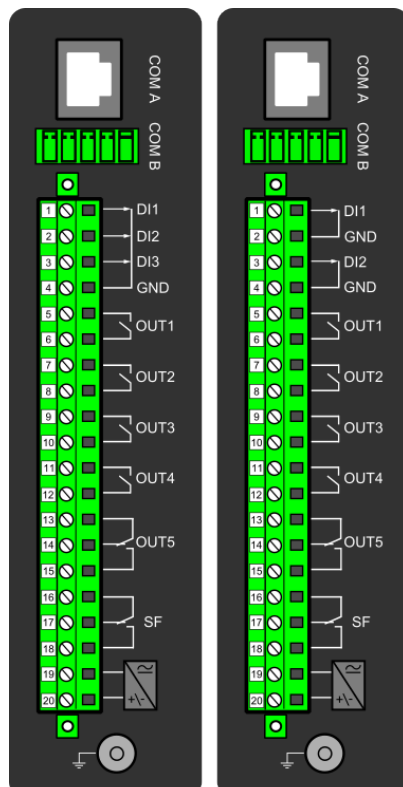
Figure. 7.2 - 250. CPU module.
