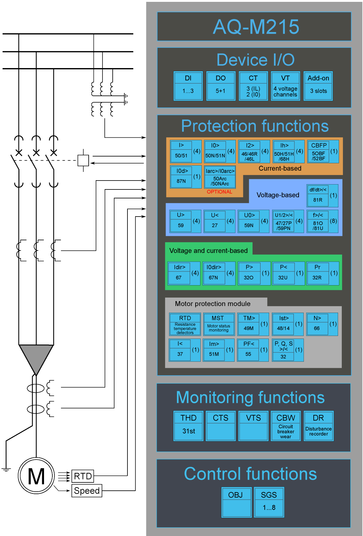
Figure. 6.1 - 240. AQ-M215 application example with function block diagram.
