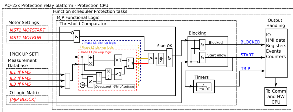
Figure. 4.4.24 - 174. Simplified function block diagram of the I_{m>} function.
