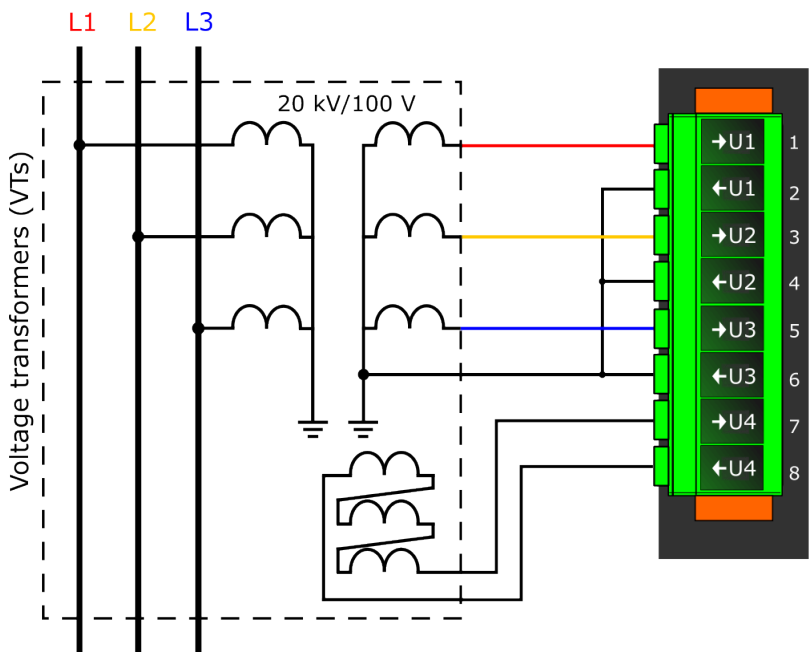
Figure. 4.2.2 - 67. Connections.
