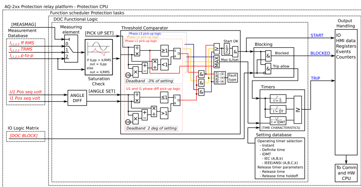
Figure. 4.4.4 - 88. Simplified function block diagram of the Idir> function.
