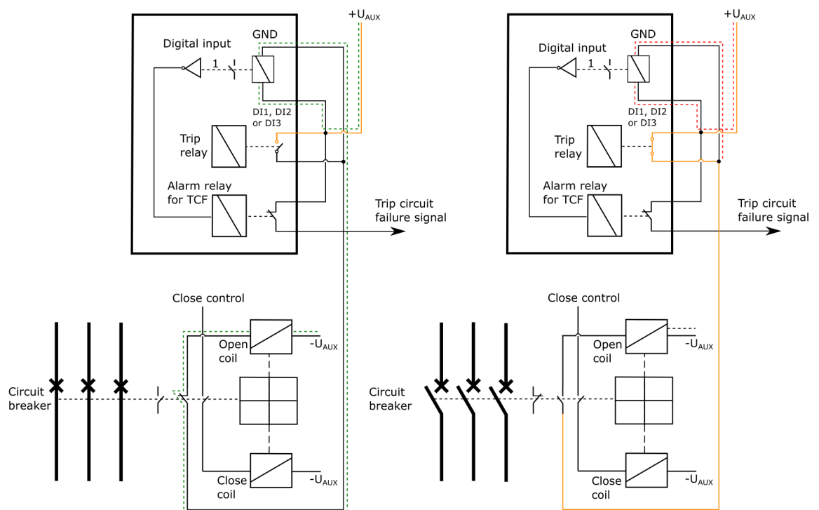
Figure. 6.4 - 246. Trip circuit supervision with one DI and one latched output contact.
