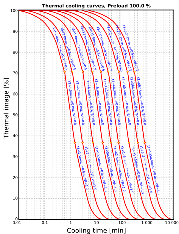
Figure. 4.4.26 - 196. Thermal cooling curves, dynamic triple time constant (motor is running without load in the first part with dedicated time constant).
