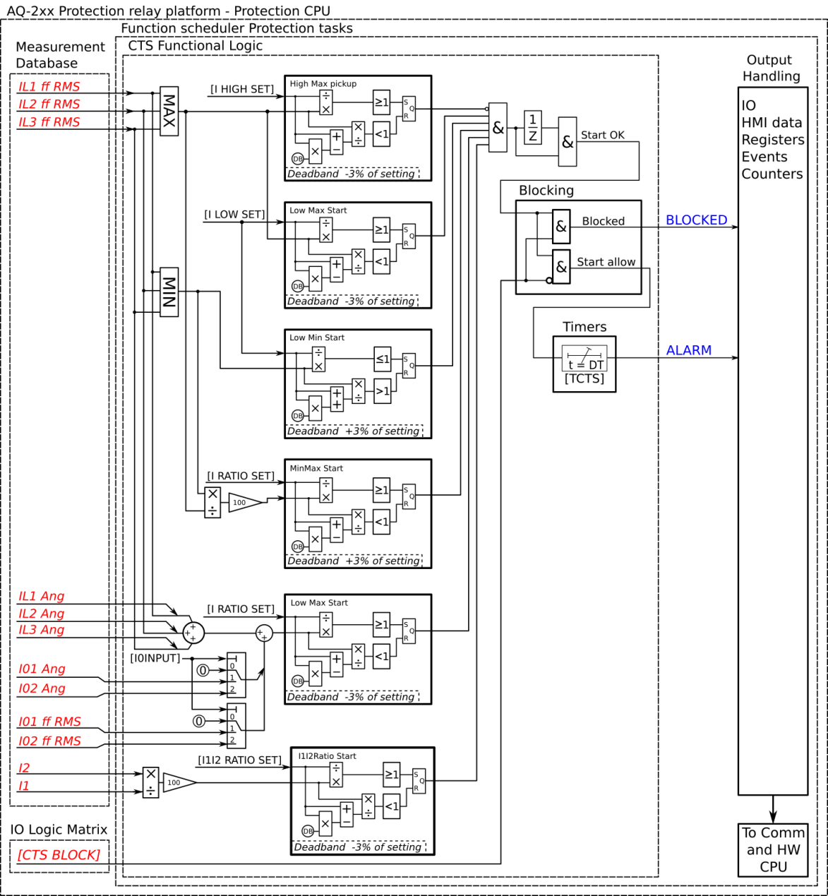
Figure. 4.6.1 - 218. Simplified function block diagram of the CTS function.
