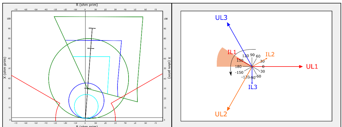
Figure. 4.2.3 - 74. Distance protection characteristics and directional overcurrent.
