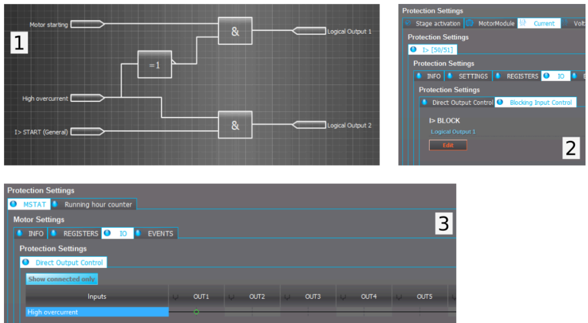
Figure. 4.4.20 - 163. Motor start up overcurrent control logic.
