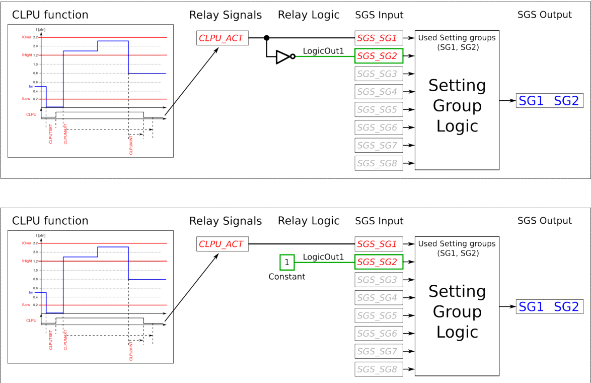
Figure. 4.5.2 - 210. Entirely application-controlled setting group change with the cold load pick-up function.
