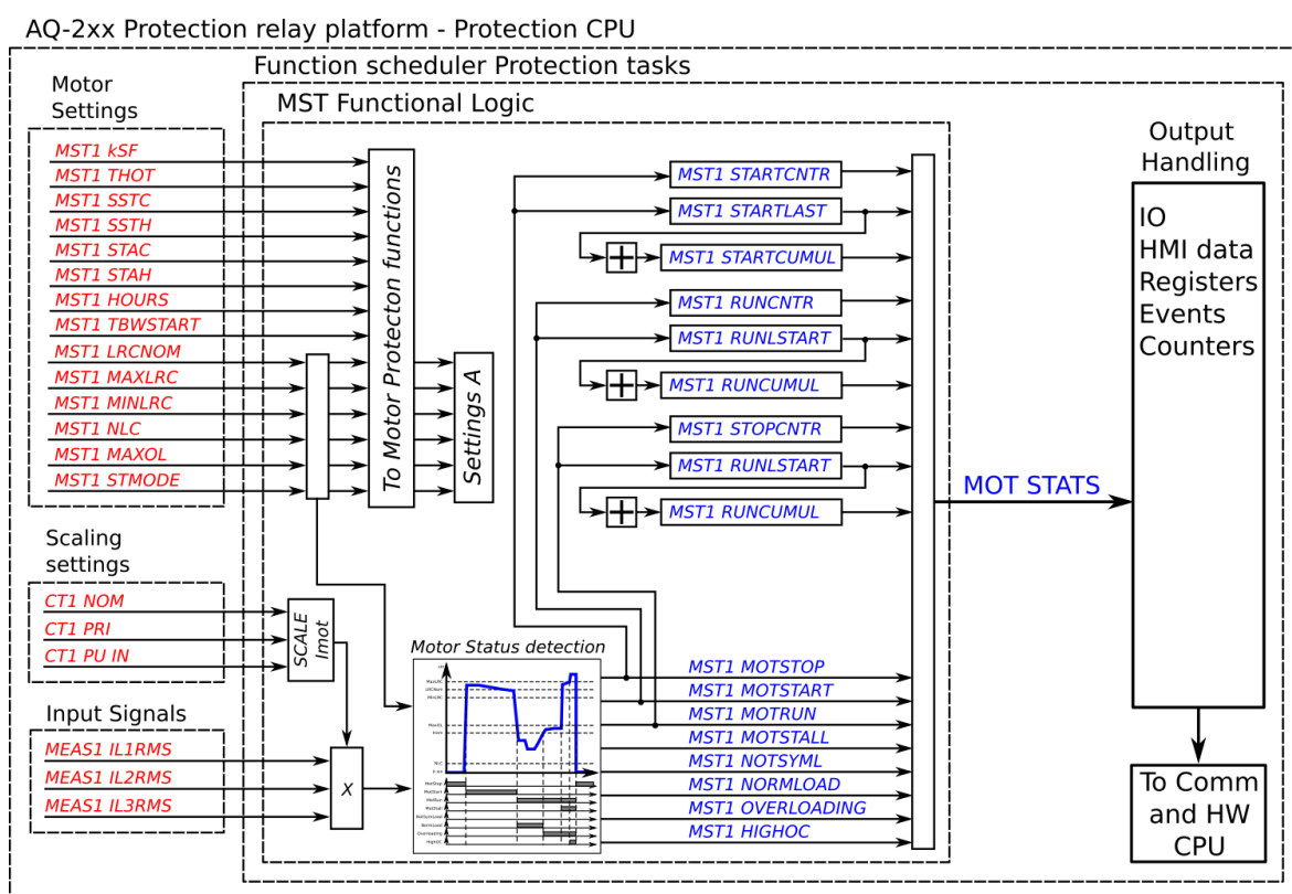
Figure. 4.4.20 - 159. Simplified function block diagram of the motor status monitoring function.
