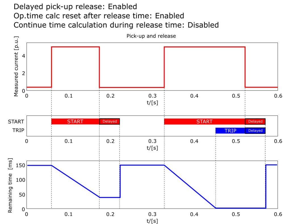
Figure. 4.4.1 - 84. Delayed pick-up release, delay counter value is held during the release time.
