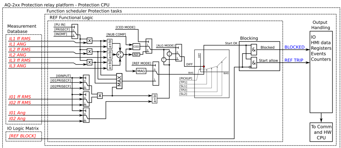
Figure. 4.4.10 - 116. Simplified function block diagram of the I0d> function.
