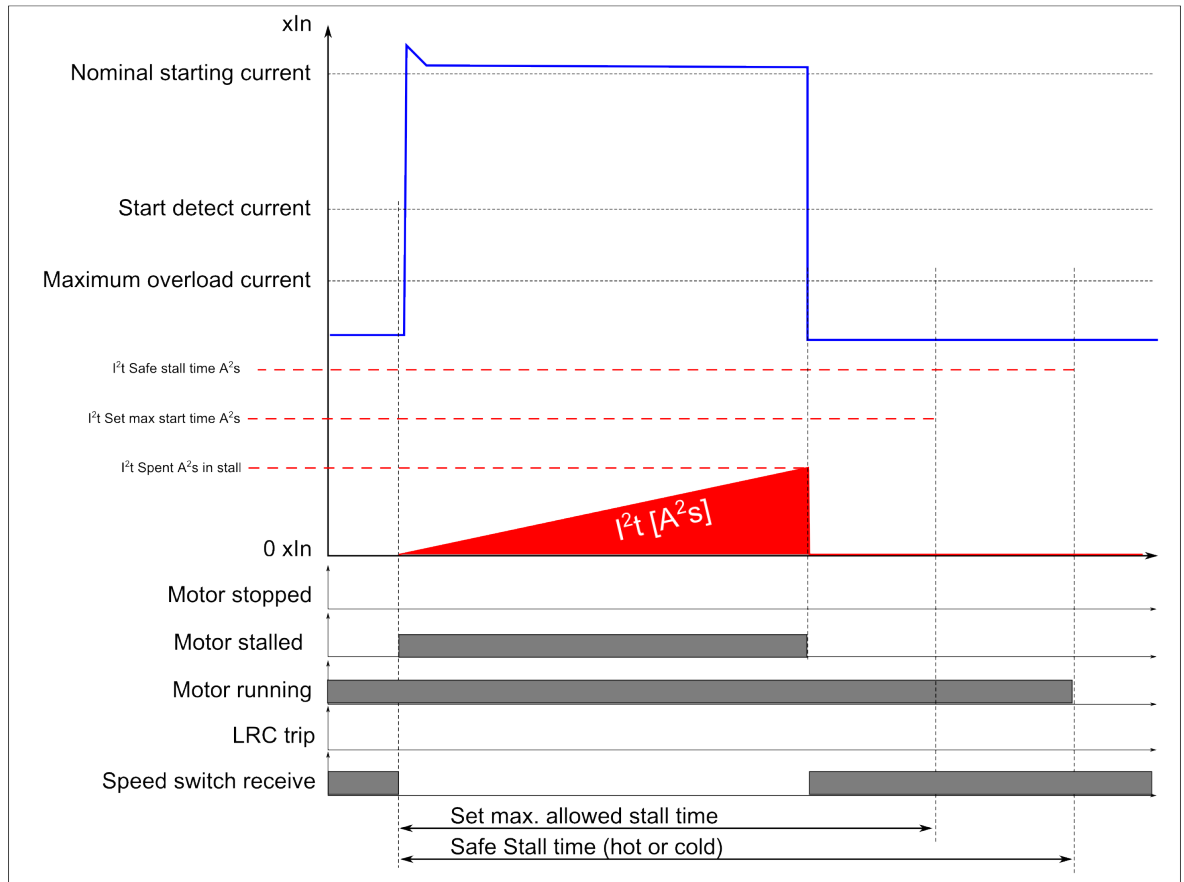
Figure. 4.4.21 - 169. Motor stall monitoring.
