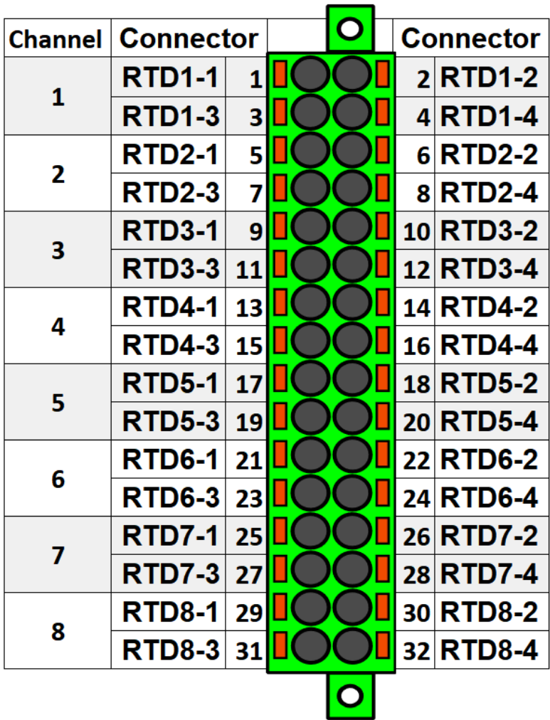
Figure. 7.5.4 - 257. RTD input module connectors.
