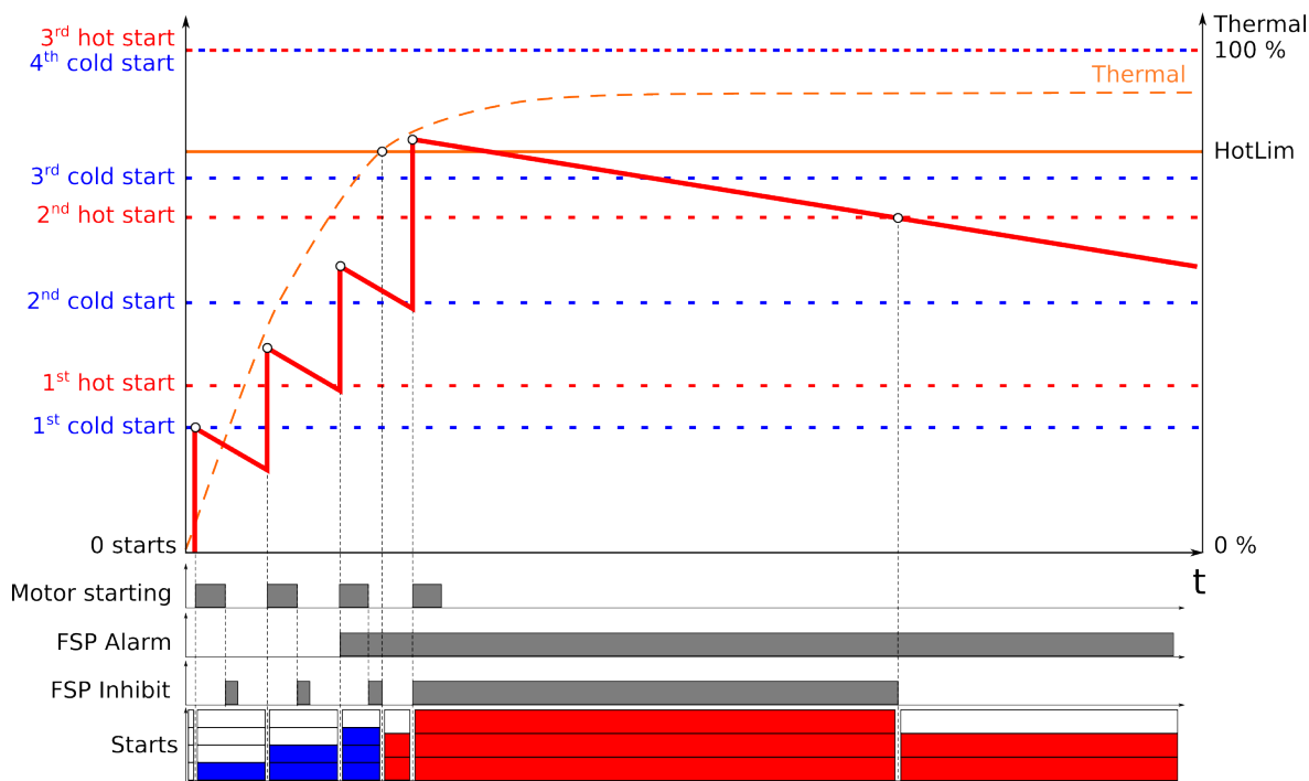
Figure. 4.4.22 - 172. Updating the starts counter when thermal hot and cold status taken into consideration.
