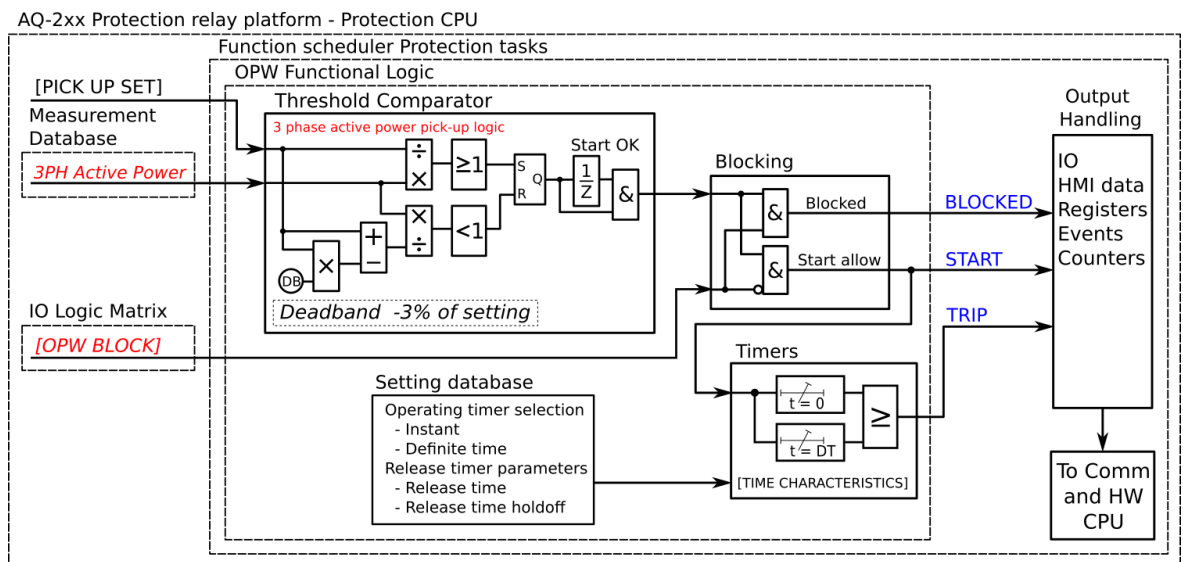
Figure. 4.4.17 - 153. Simplified function block diagram of the P> function.
