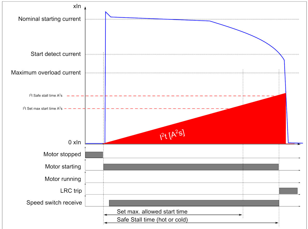
Figure. 4.4.21 - 168. Outputs when motor starting takes too long, with a speed switch.
