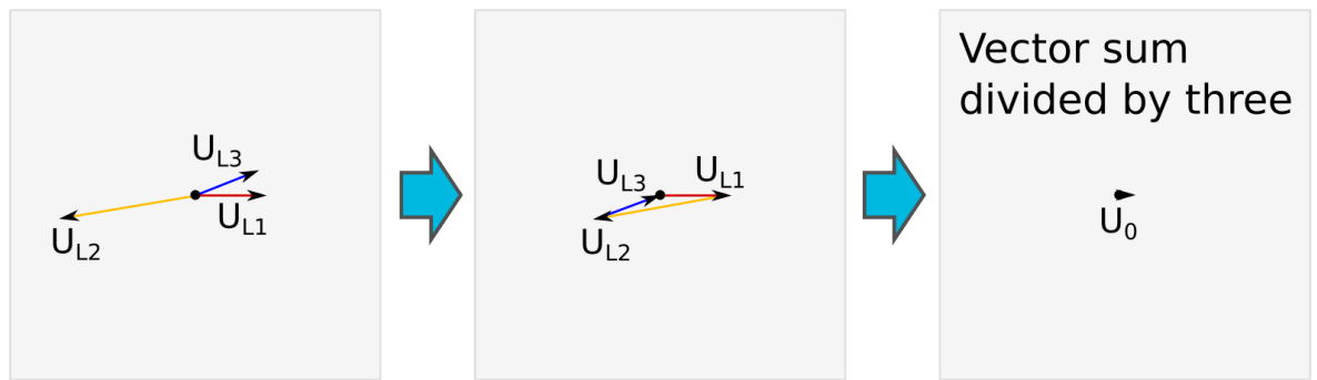
Figure. 4.4.13 - 138. Close-distance short-circuit between phases 1 and 3.
