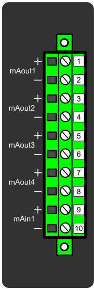
Figure. 7.5.9 - 266. Milliampere (mA) I/O module connections.
