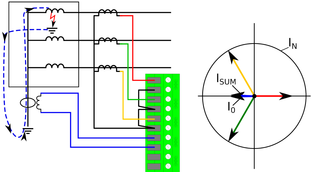
Figure. 4.4.10 - 126. Restricted earth fault inside a Y winding transformer.
