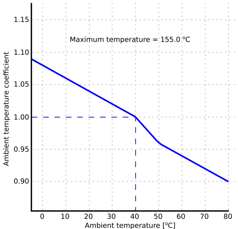
Figure. 4.4.26 - 181. Ambient temperature coefficient calculation (linear approximation, indefinite points).
