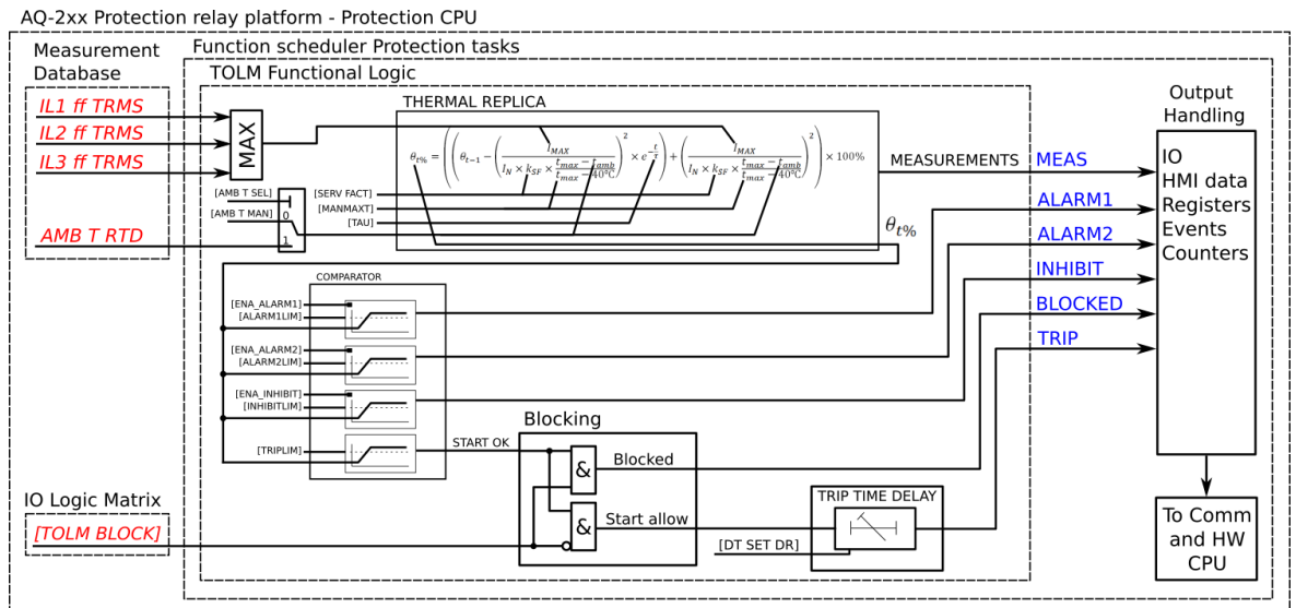
Figure. 4.4.26 - 201. Simplified function block diagram of the TM> function.
