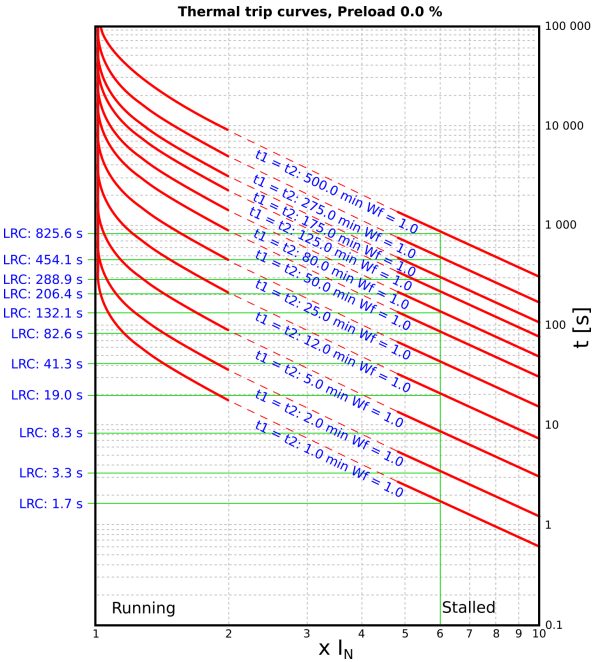
Figure. 4.4.26 - 190. Thermal tripping curves with single time constant, pre-load 0% (cold).
