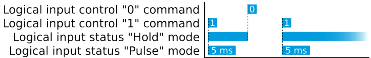
Figure. 4.5.9 - 215. Operation of logical input in "Hold" and "Pulse" modes.
