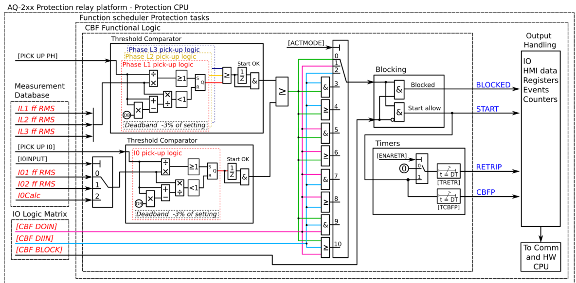
Figure. 4.4.8 - 106. Simplified function block diagram of the CBFP function.
