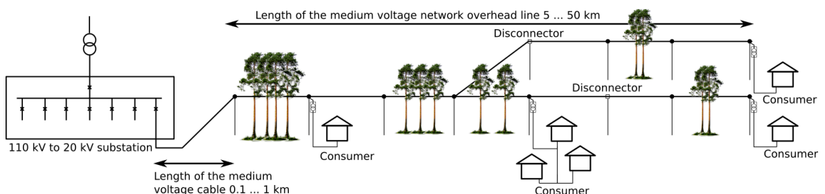
Figure. 4.5.5 - 178. Diagram of a typical radial medium-voltage network in rural areas.
