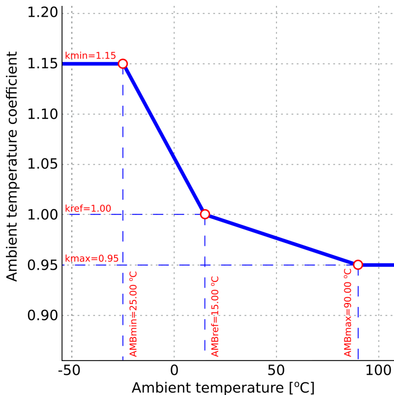
Figure. 4.4.19 - 155. Ambient temperature coefficient calculation (a three-point linear approximation and a settable correction curve).
