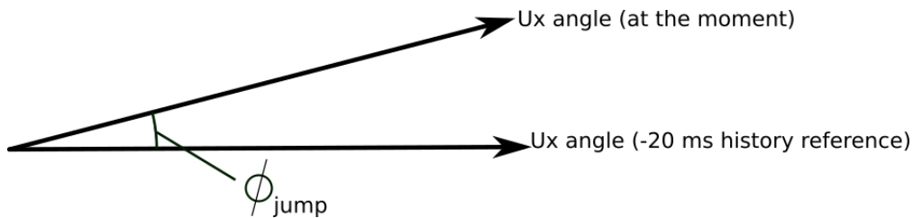
Figure. 4.5.9 - 207. Vector jump from the relay's point of view.
