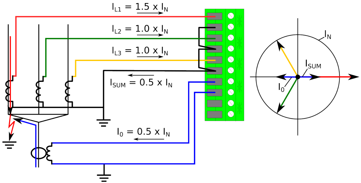
Figure. 4.4.9 - 125. Cable end differential when a fault occurs.
