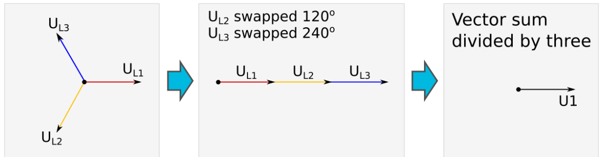
Figure. 4.4.13 - 135. Normal situation.
