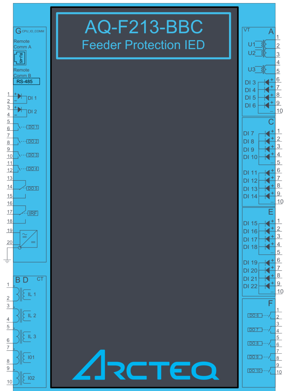
Figure. 6.1 - 233. AQ-F213 variant with digital input and output modules.
