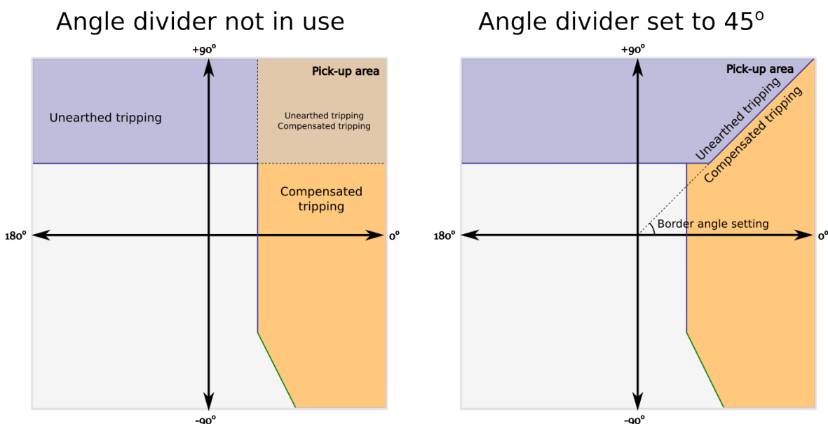
Figure. 4.4.5 - 102. Effect of angle divider when in use and when disabled.
