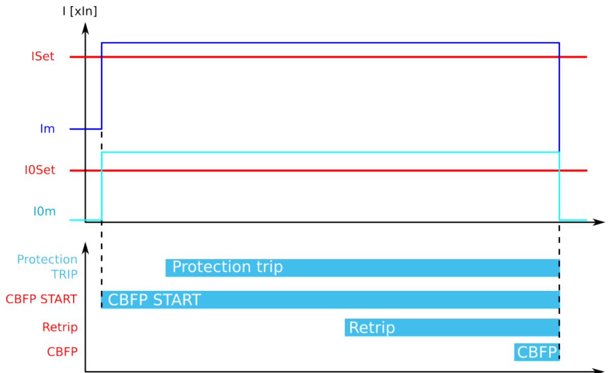
Figure. 4.4.8 - 108. Retrip and CBFP when "Current" is the selected criterion.
