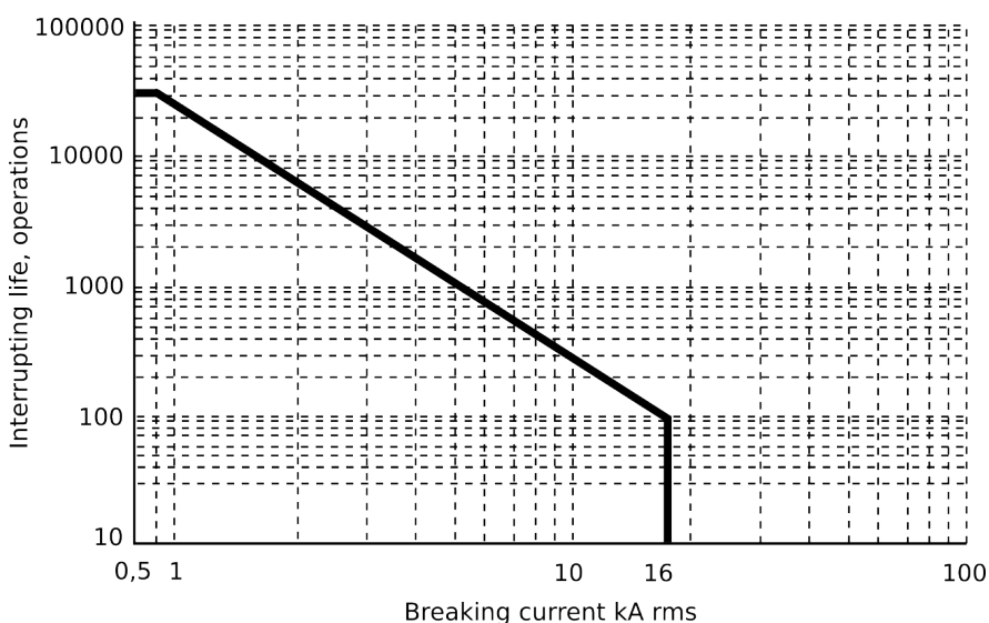
Figure. 4.6.3 - 224. Example of the circuit breaker interrupting life operations.
