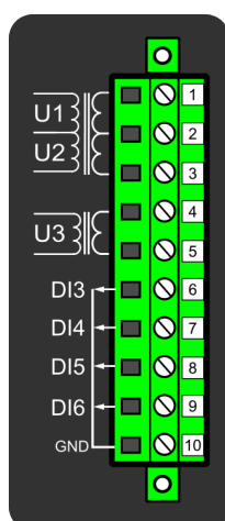
Figure. 7.4 - 246. Voltage measurement module.
