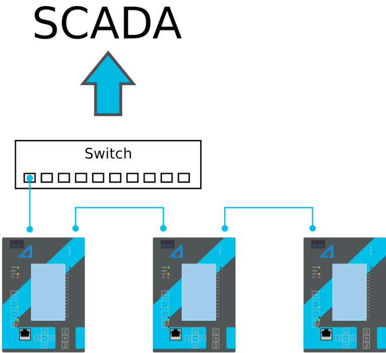
Figure. 7.5.8 - 259. Example of a multidrop configuration.
