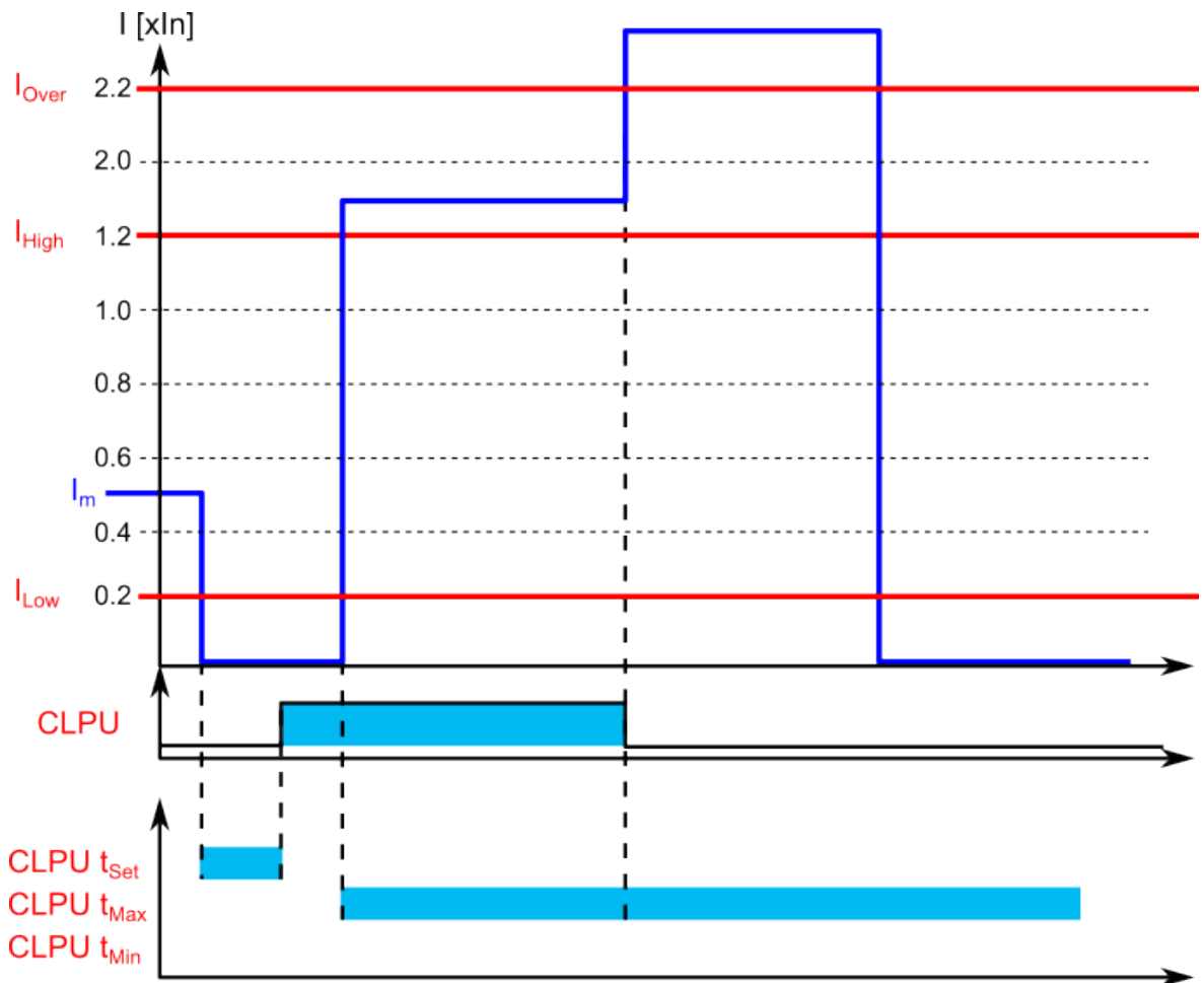
Figure. 4.5.6 - 199. Example of timers and pick-up parameters (activated pick-up and instant release due to overcurrent).
