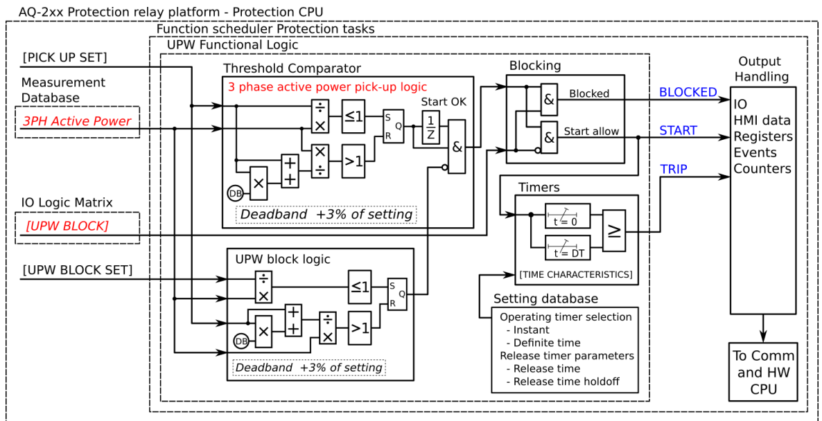
Figure. 4.4.17 - 150. Simplified function block diagram of the P< function.
