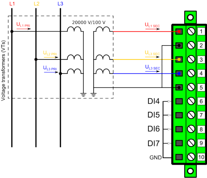
Figure. 4.2.2 - 71. Example connections for 3LN voltage measurement.
