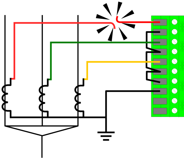
Figure. 4.6.1 - 211. Secondary circuit fault in phase L1 wiring.
