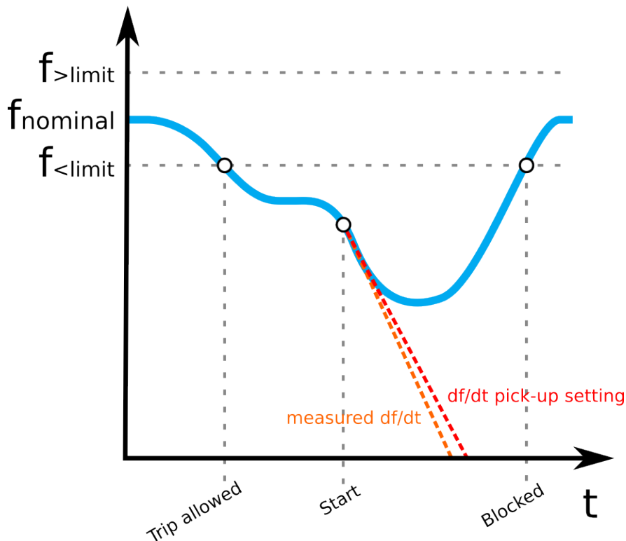
Figure. 4.4.15 - 145. Operation of the df/dt > / < function when the frequency starts but doesn't trip.
