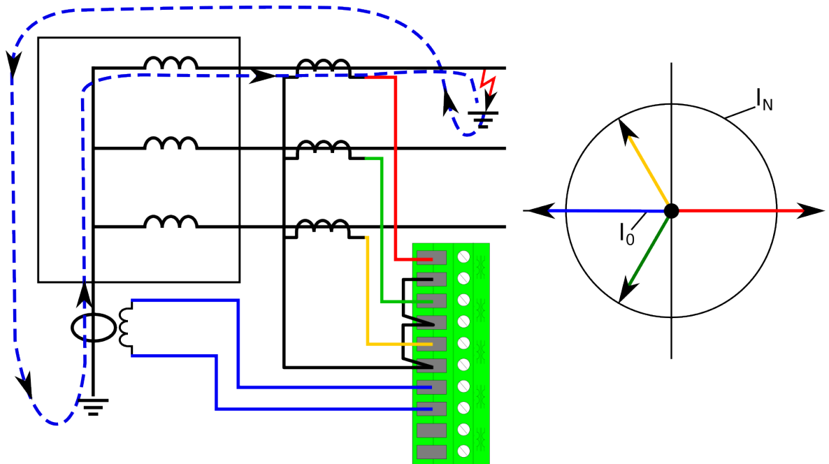
Figure. 4.4.9 - 126. Restricted earth fault outside a Y winding transformer.
