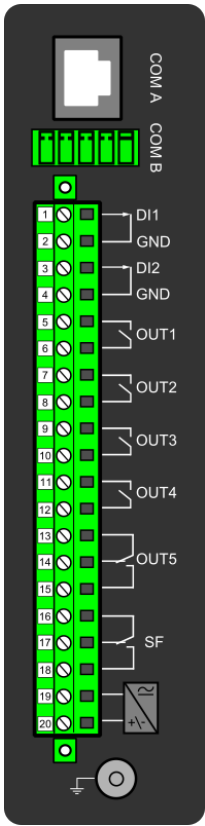
Figure. 7.2 - 244. CPU module.
