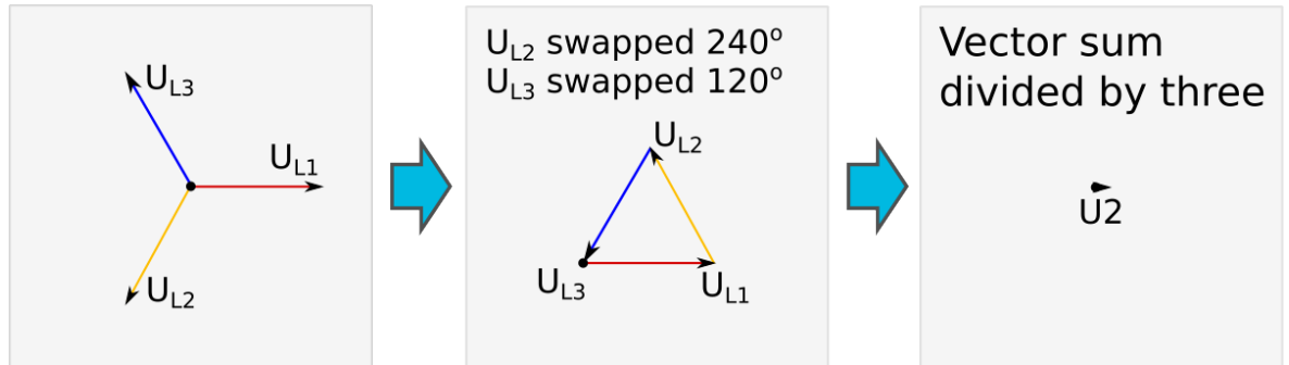
Figure. 4.4.13 - 138. Normal situation.
