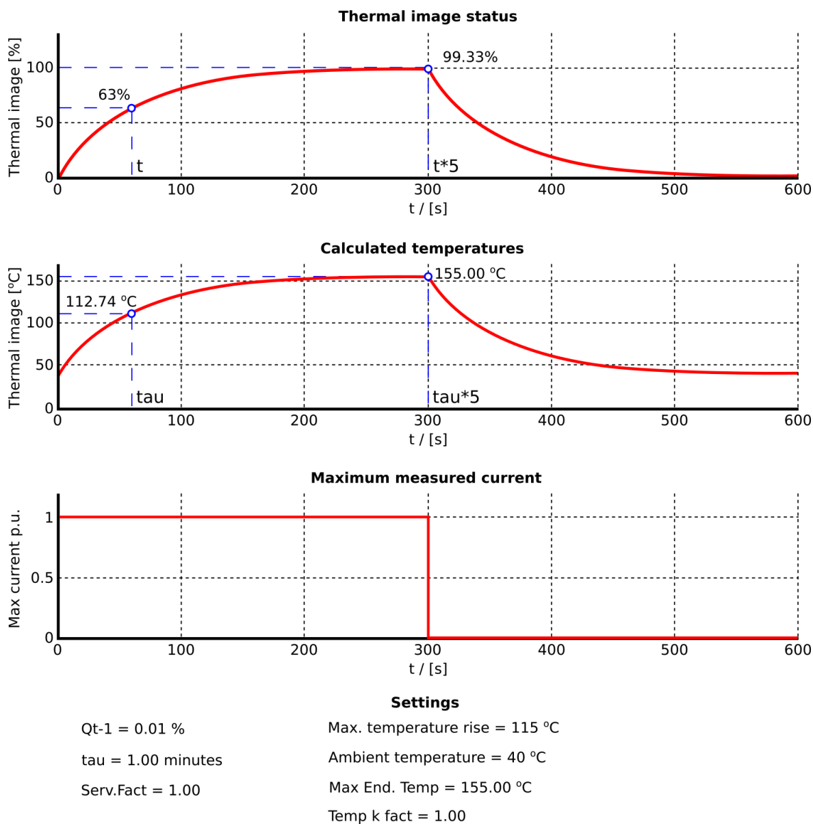
Figure. 4.4.19 - 154. Example of thermal image calculation with nominal conditions.
