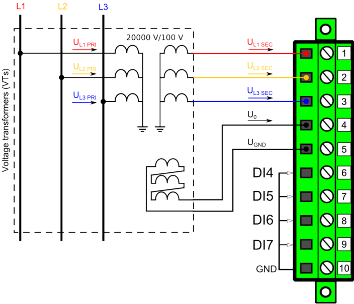
Figure. 4.2.2 - 72. Example connections for 2LL+U0 voltage measurement.
