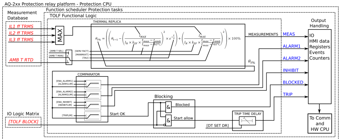
Figure. 4.4.19 - 166. Simplified function block diagram of the TF> function.
