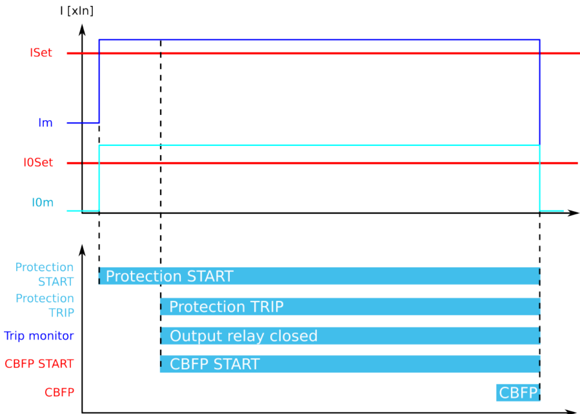
Figure. 4.4.8 - 113. CBFP when "Current and DO" is the selected criterion.
