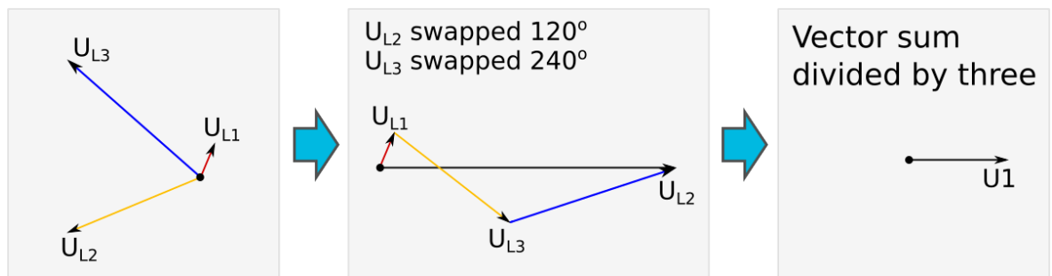
Figure. 4.4.13 - 136. Earth fault in an isolated network.
