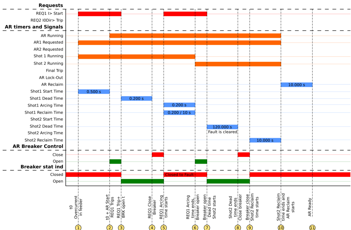
Figure. 4.5.5 - 190. Signal status graph of the semi-permanent overcurrent auto-recloser cycle.
