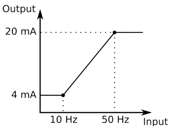
Figure. 4.5.8 - 204. Example of the effects of mA output channel settings.
