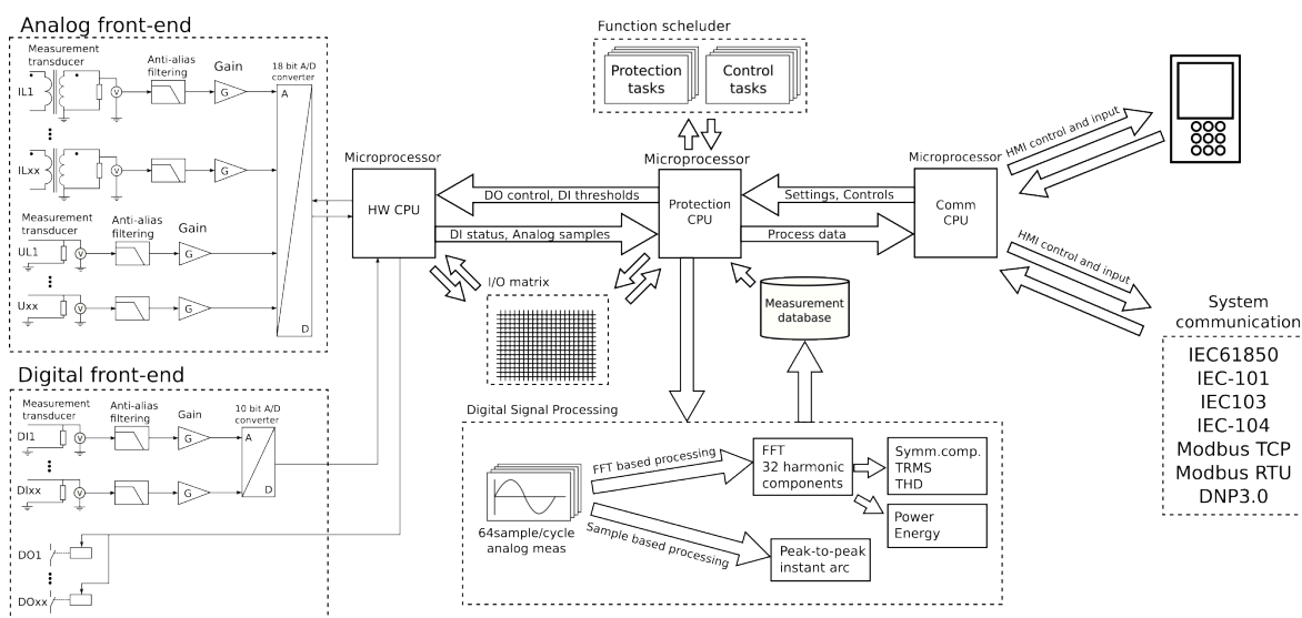
Figure. 4.4.1 - 82. Principle diagram of the protection relay platform.
