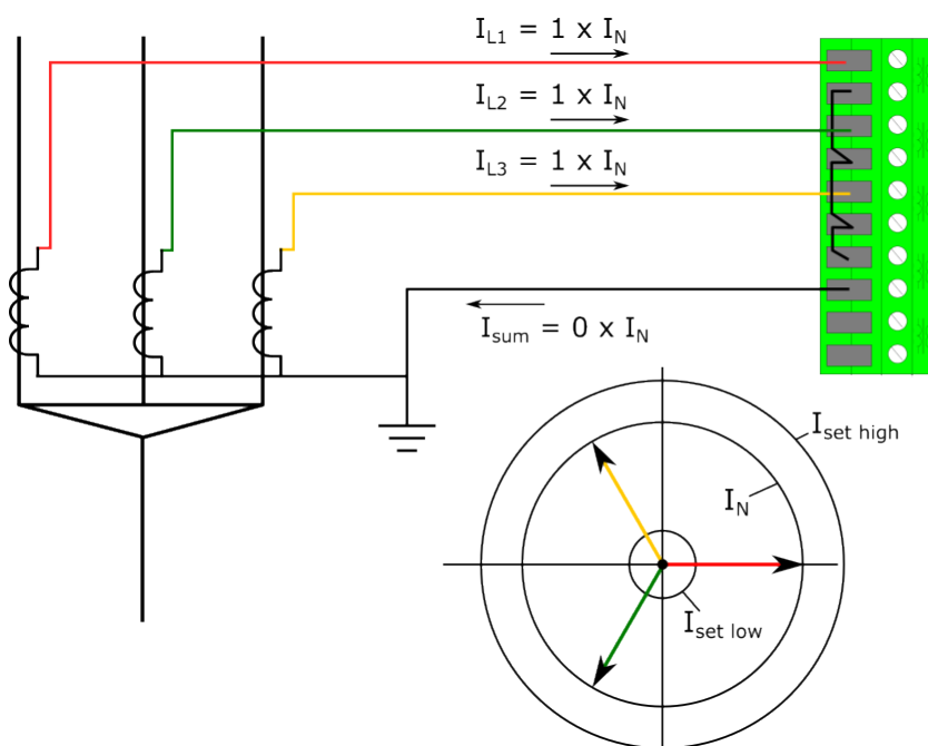
Figure. 4.6.1 - 213. All works properly, no faults.
