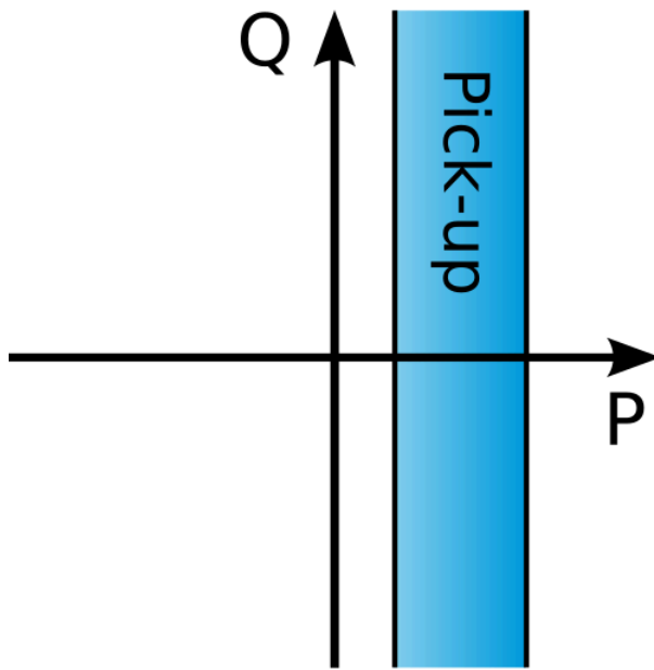
Figure. 4.4.17 - 149. Operating characteristics of underpower protection.
