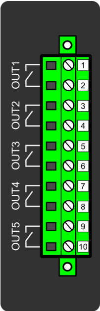
Figure. 7.5.2 - 249. Digital output module (DO5) with five add-on digital outputs.
