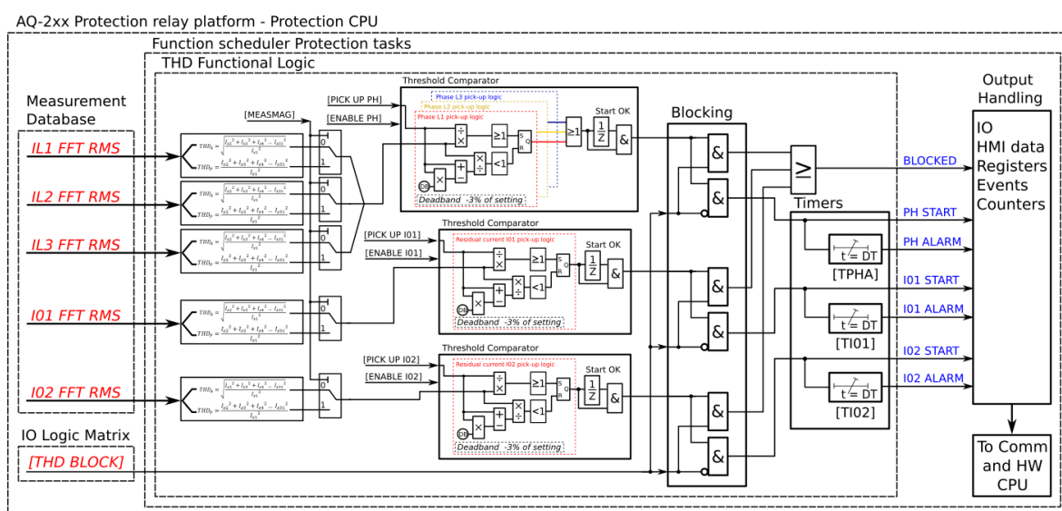
Figure. 4.6.4 - 227. Simplified function block diagram of the total harmonic distortion monitor function.
