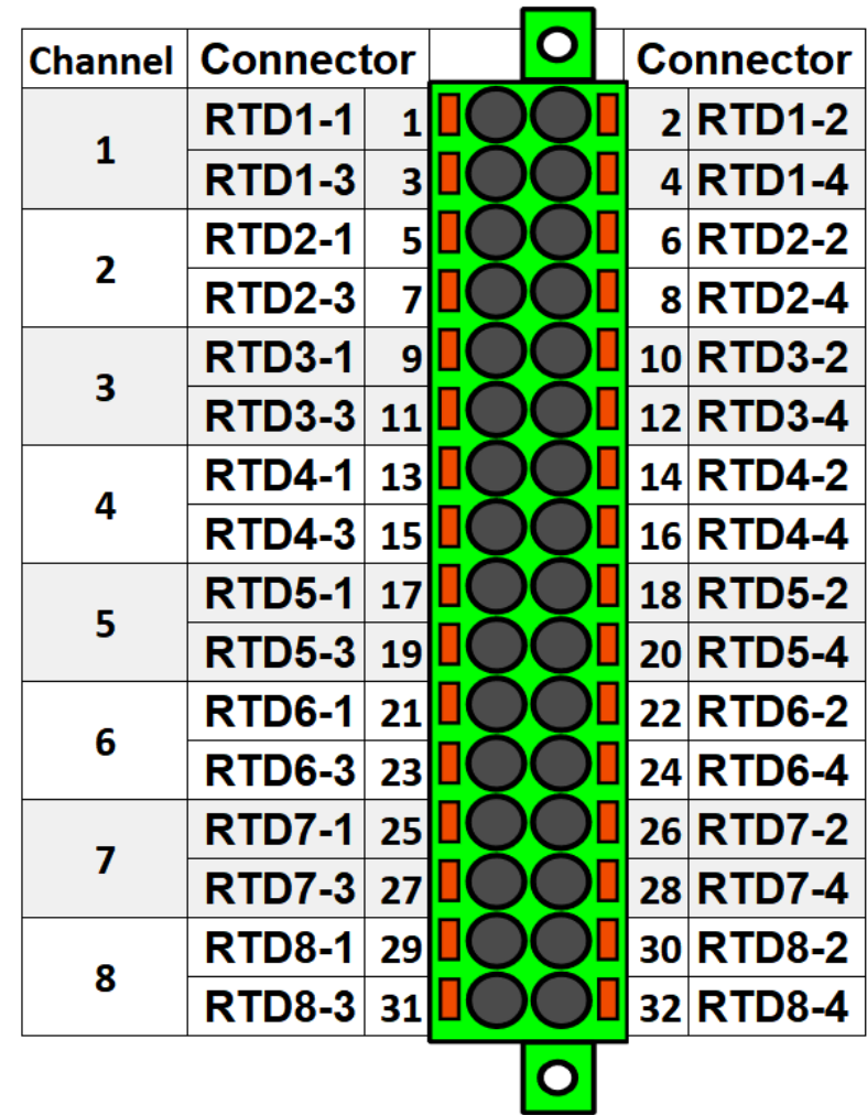
Figure. 7.5.4 - 251. RTD input module connectors.
