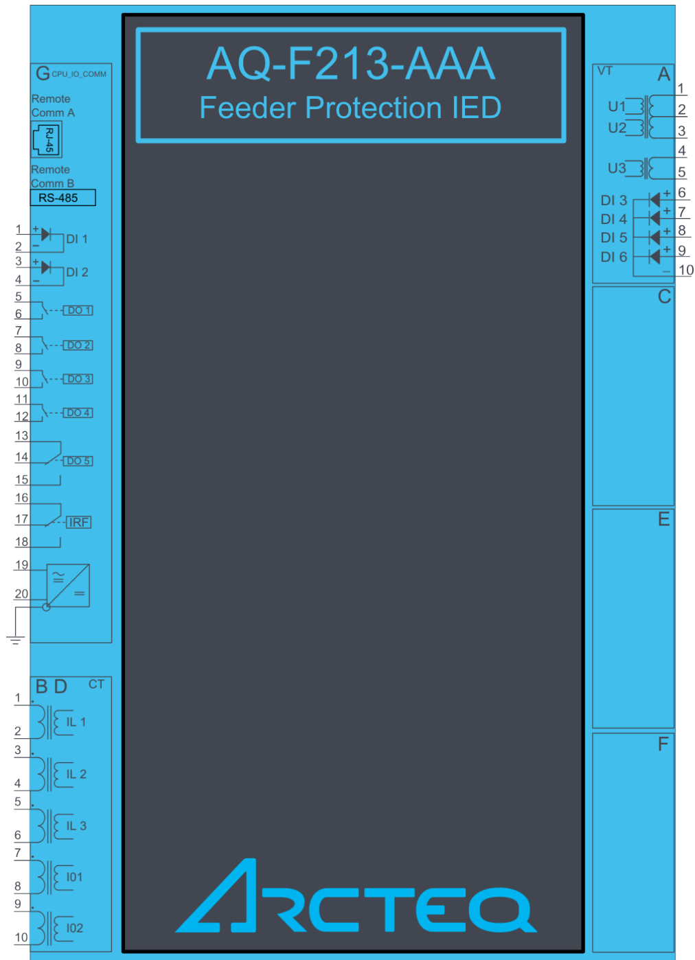
Figure. 6.1 - 232. AQ-F213 variant without add-on modules.
