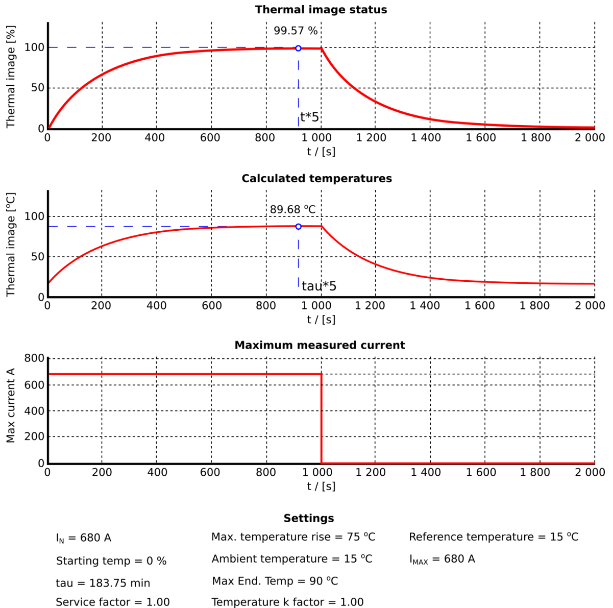
Figure. 4.4.19 - 163. Thermal image response with maximum load (installation according to presumptions).
