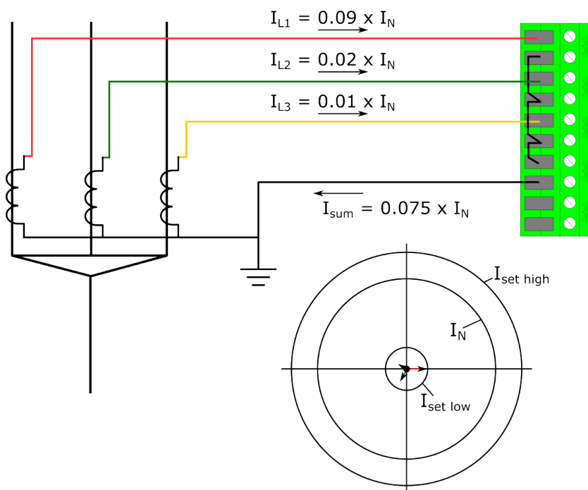
Figure. 4.6.1 - 217. Low current and heavy unbalance.
