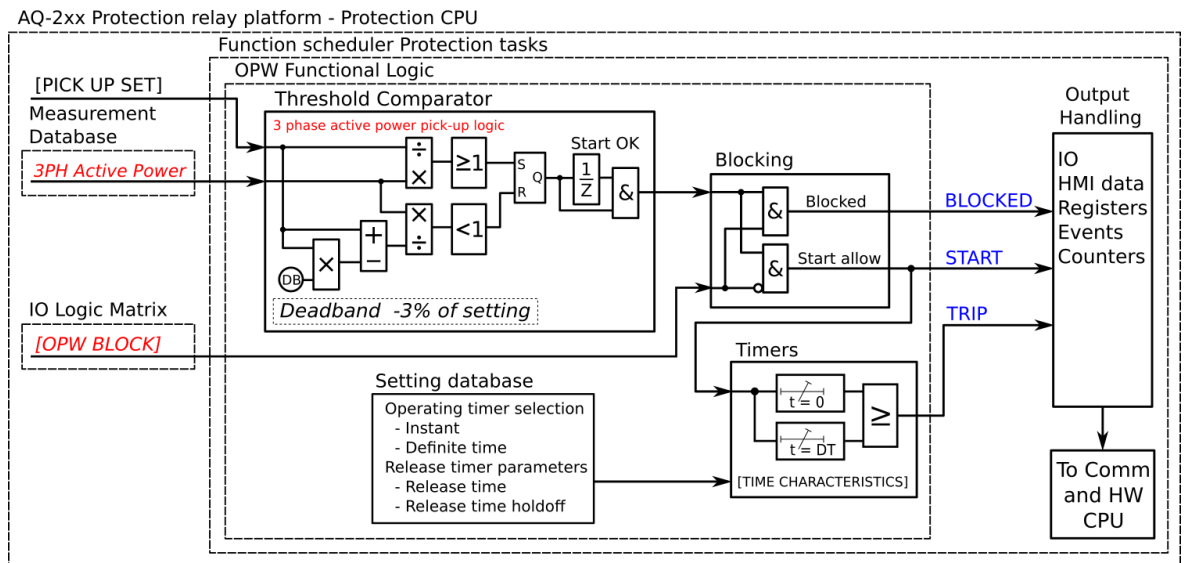
Figure. 4.4.16 - 148. Simplified function block diagram of the P> function.
