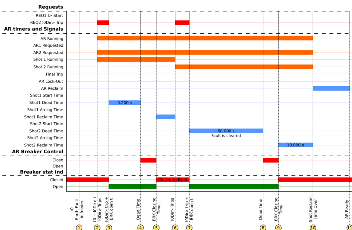
Figure. 4.5.5 - 184. Signal status graph of the semi-permanent earth fault auto-recloser cycle.
