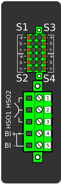
Figure. 7.5.3 - 250. Arc protection module.
