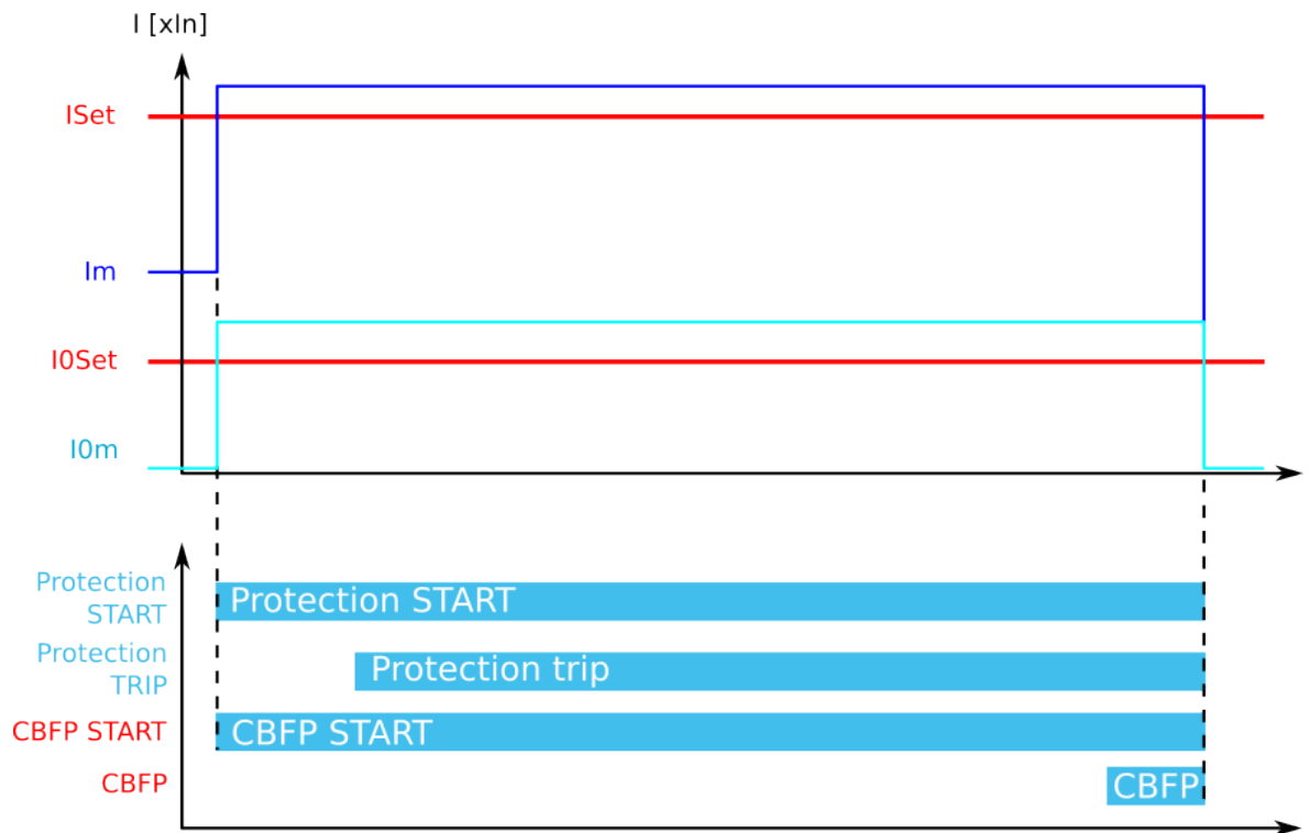
Figure. 4.4.8 - 112. CBFP when "Current" is the selected criterion.
