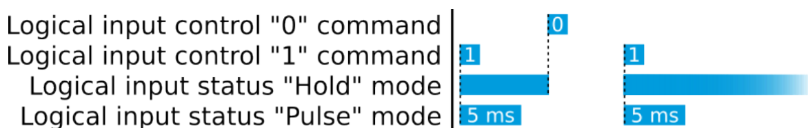
Figure. 4.5.13 - 209. Operation of logical input in "Hold" and "Pulse" modes.
