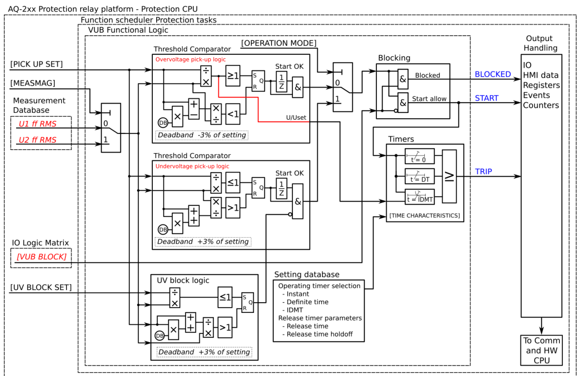
Figure. 4.4.13 - 141. Simplified function block diagram of the U1/U2>/< function.
