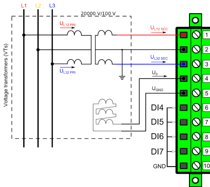
Figure. 4.2.2 - 73. Example connections for 2LL+U0 (open delta 2LL) voltage measurement.
