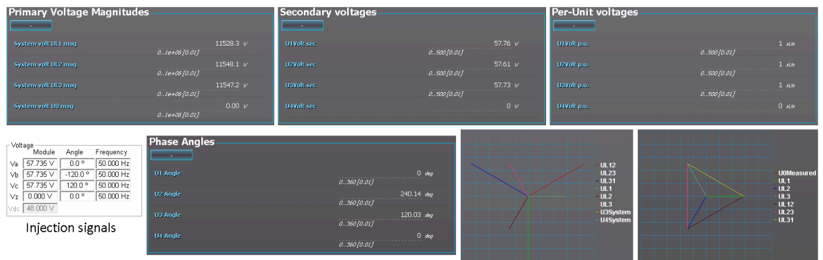
Figure. 4.2.2 - 75. Measurement behavior when nominal voltage injected during LN voltage measurements.
