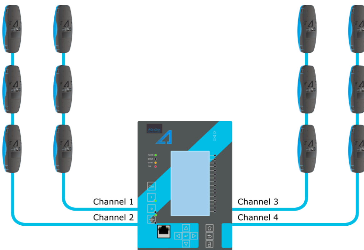
Figure. 4.4.21 - 167. Protection relay equipped with arc protection.
