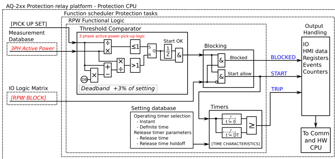
Figure. 4.4.18 - 153. Simplified function block diagram of the Pr function.
