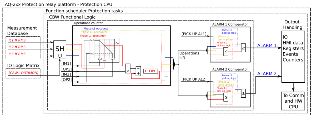
Figure. 4.6.3 - 225. Simplified function block diagram of the circuit breaker wear function.
