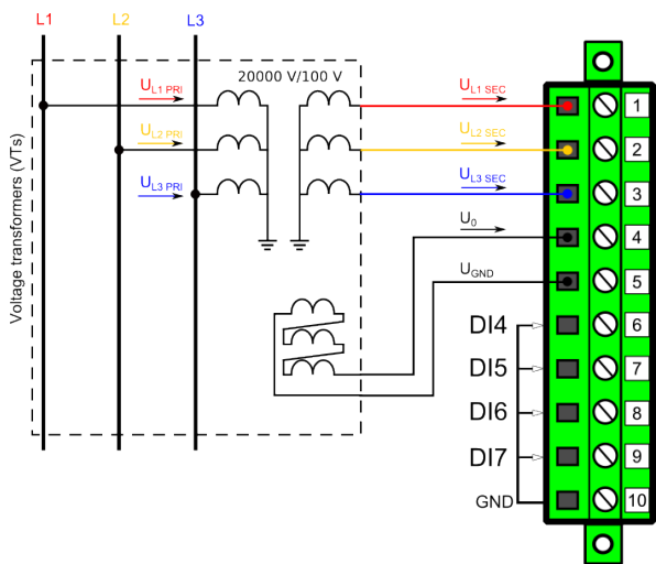
Figure. 4.2.2 - 68. Connections.
