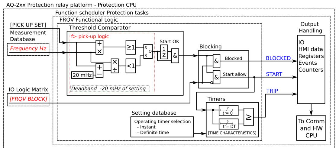
Figure. 4.4.14 - 143. Simplified function block diagram of the f> function.
