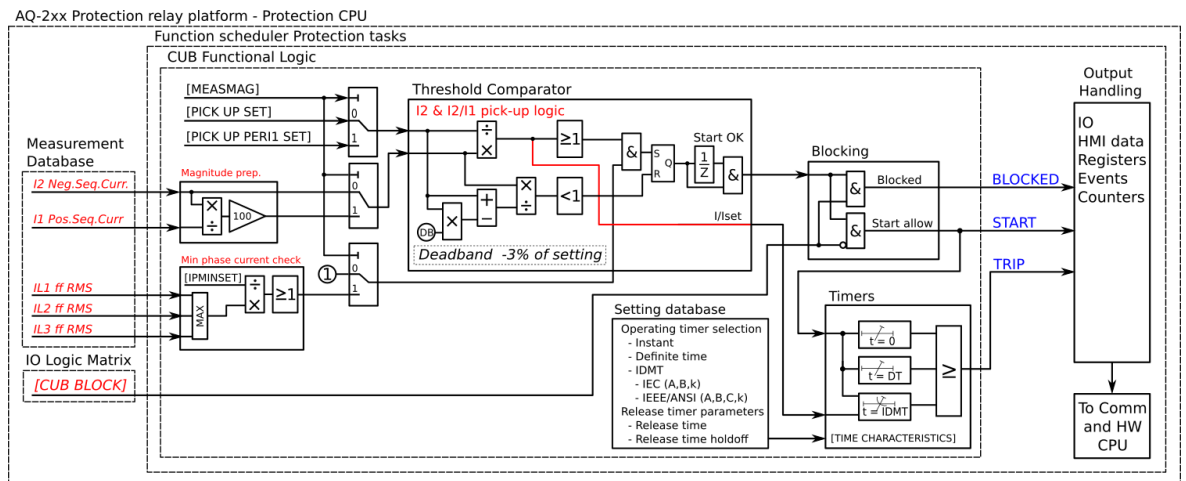
Figure. 4.4.6 - 103. Simplified function block diagram of the I2> function.
