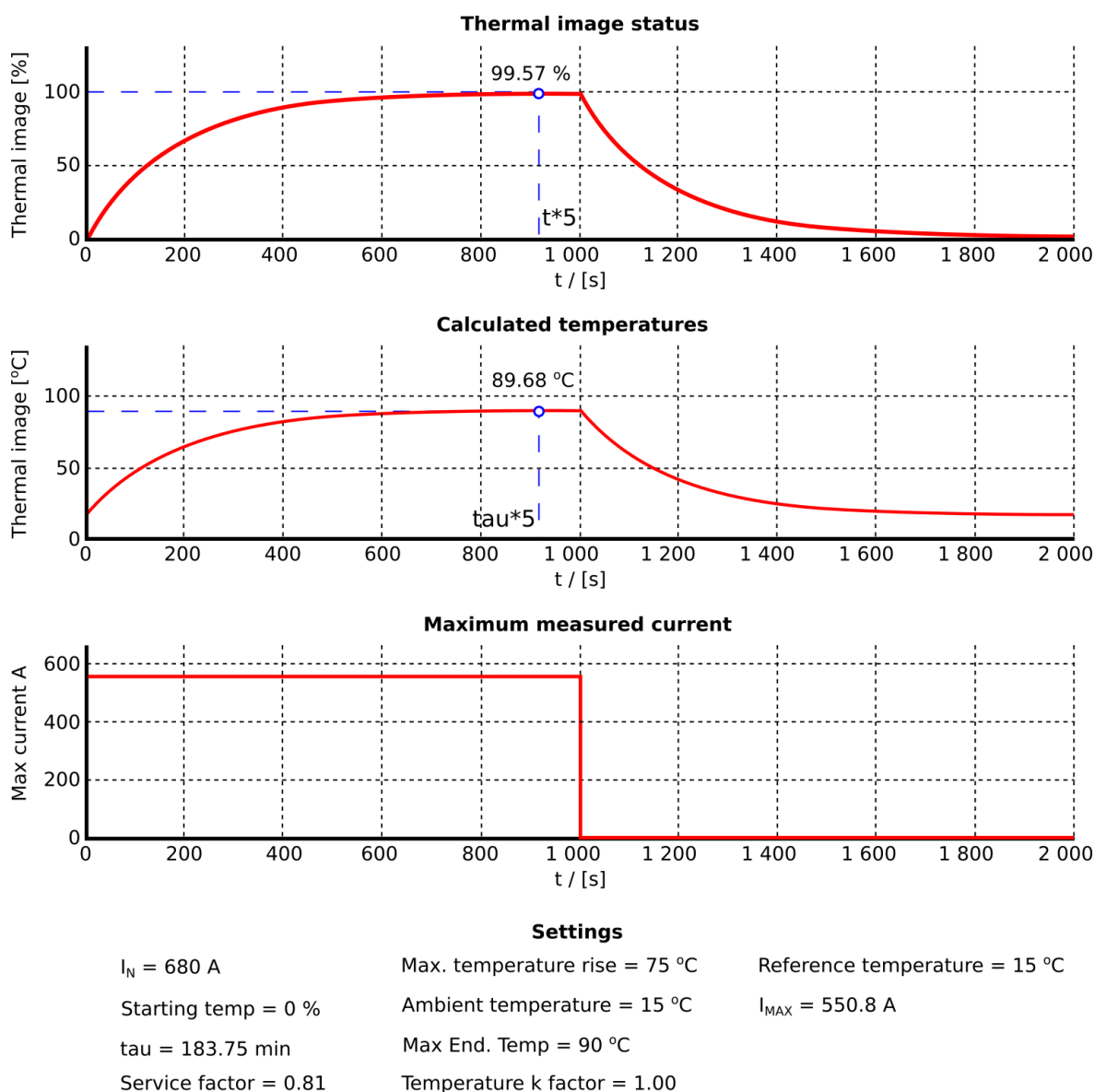
Figure. 4.4.19 - 165. Thermal response with k SF factor correctly set.
