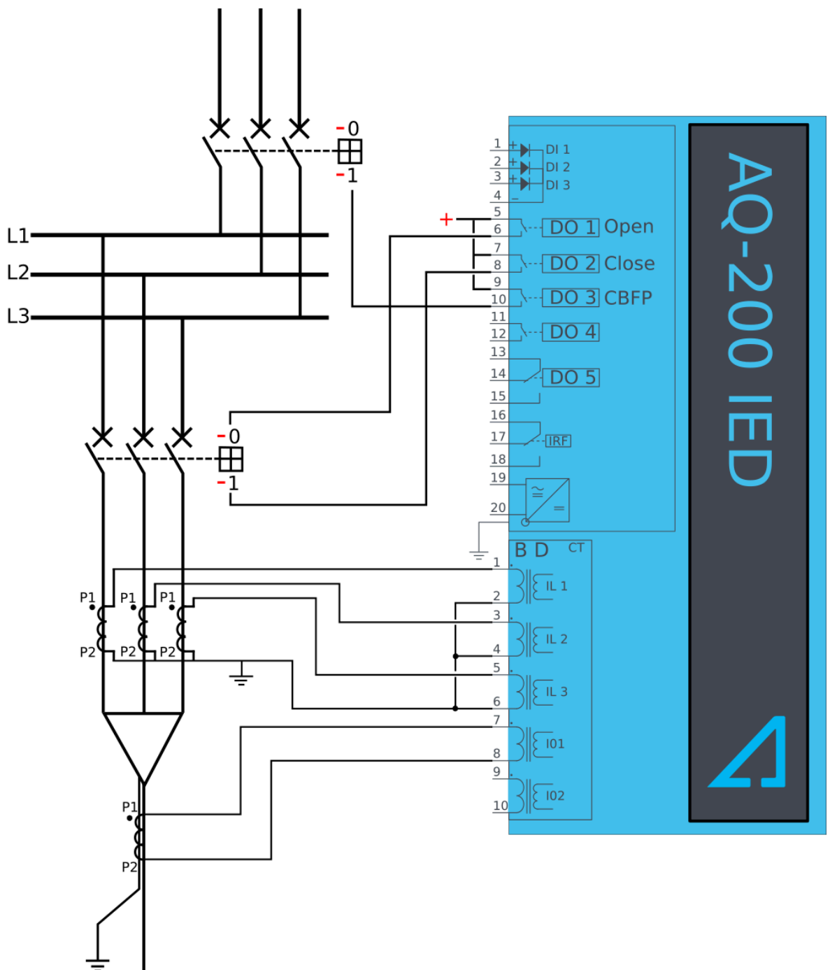
Figure. 4.4.8 - 111. Wiring diagram when Trip and CBFP are configured to the device.
