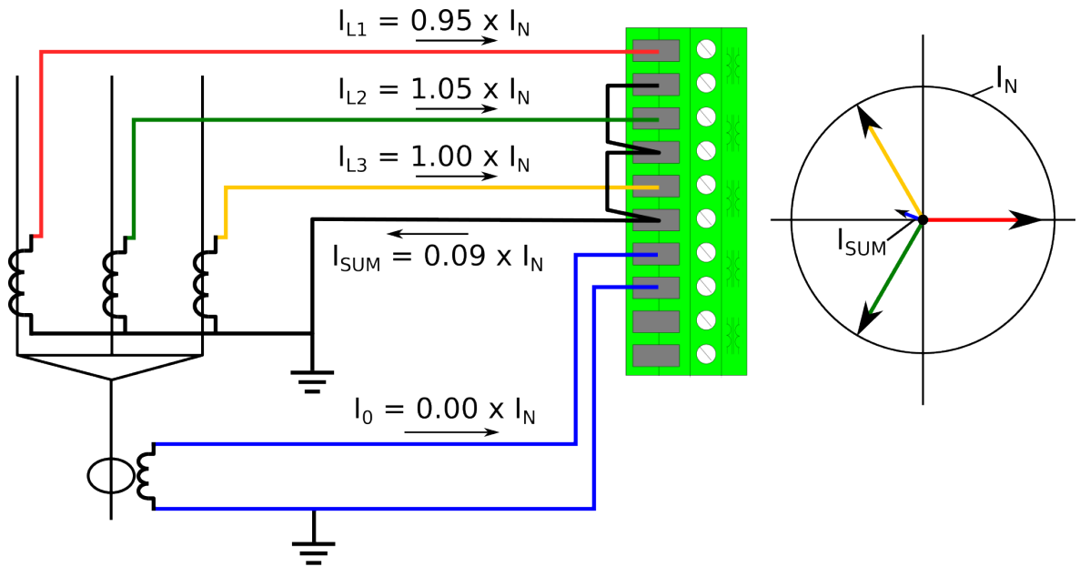
Figure. 4.4.9 - 124. Cable end differential with natural unbalance in the phase current measurement.
