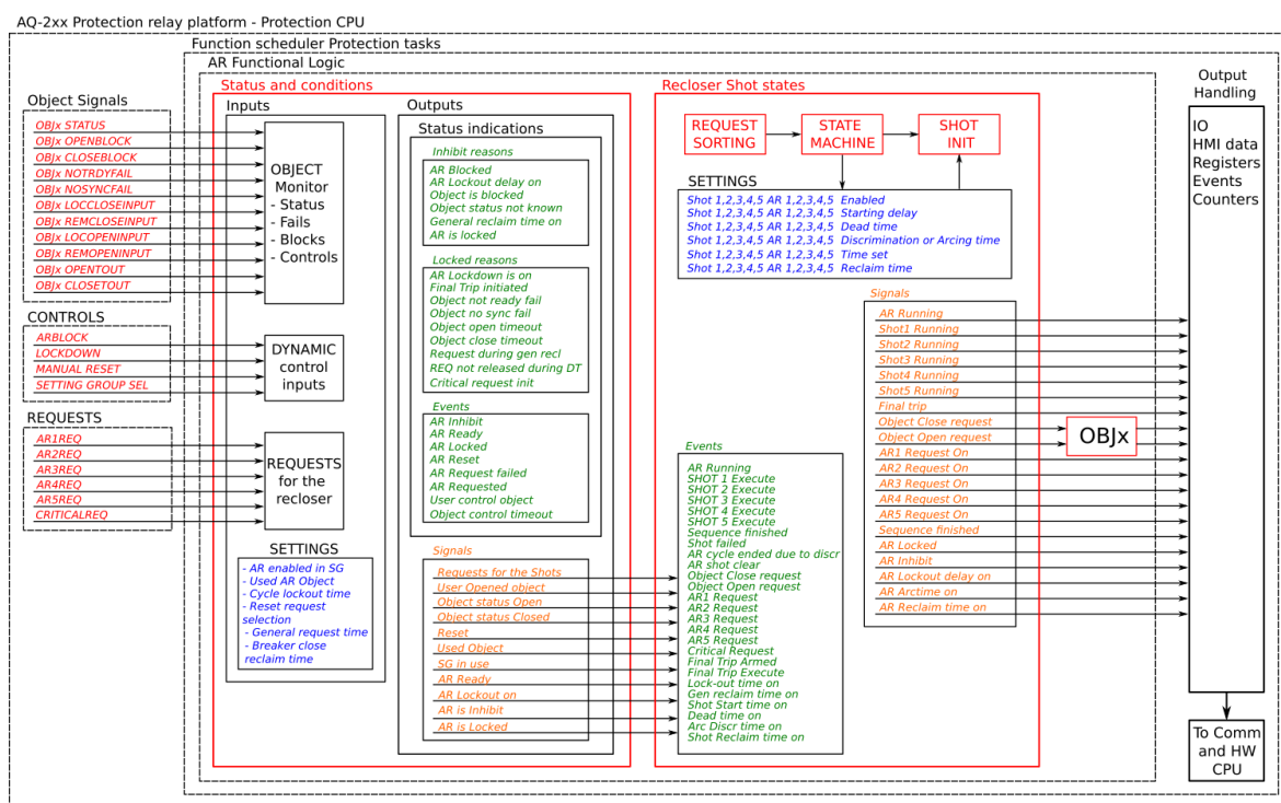
Figure. 4.5.5 - 194. Simplified function block diagram of the auto-recloser function.
