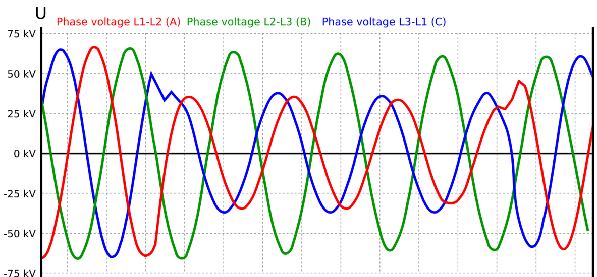
Figure. 4.5.9 - 206. Generator islanding.
