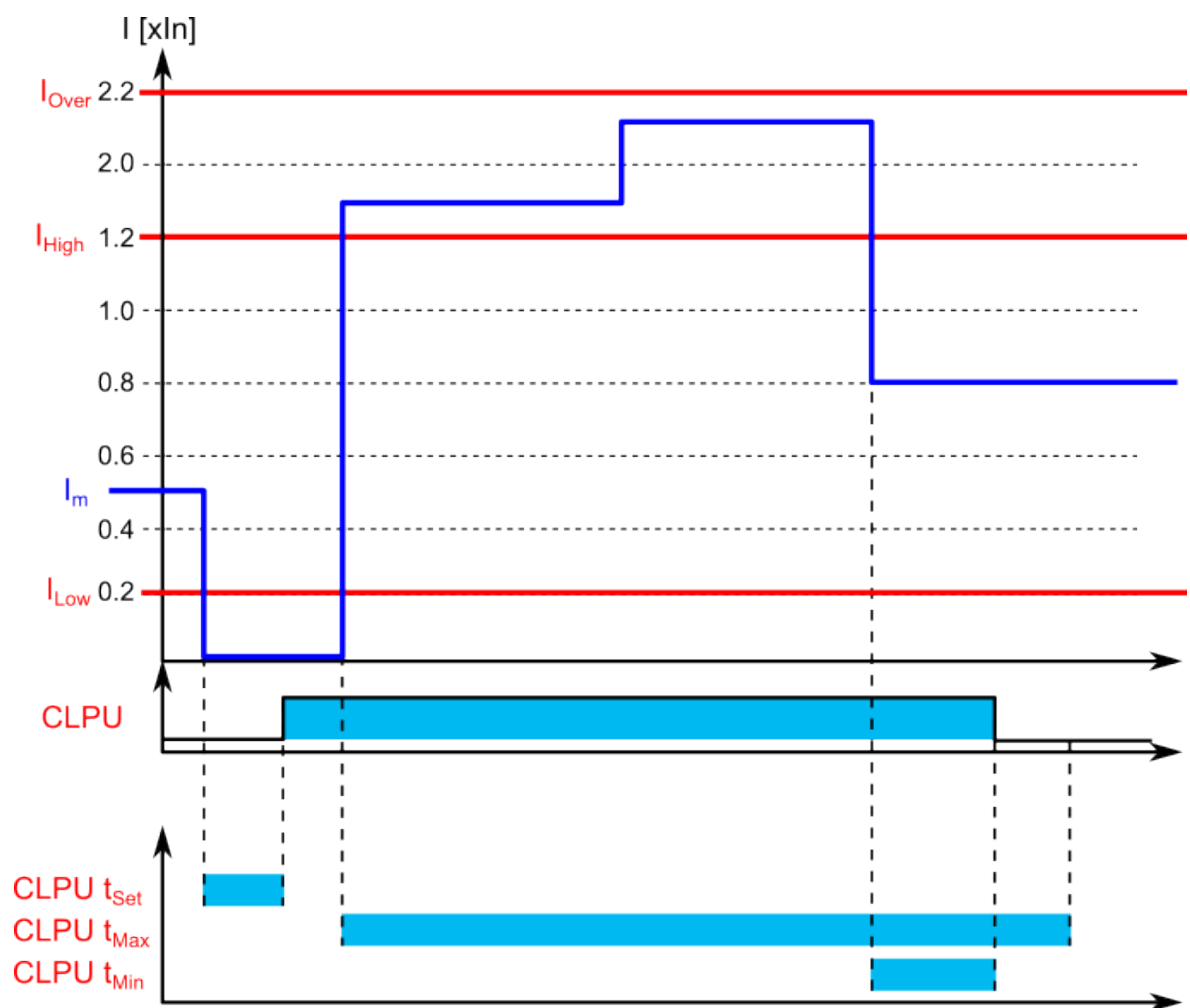
Figure. 4.5.6 - 197. Example of timers and pick-up parameters (normal CLPU situation).
