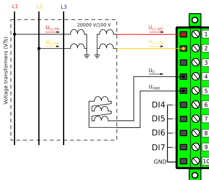
Figure. 4.2.2 - 74. Example connections for 1LL+U0 voltage measurement.
