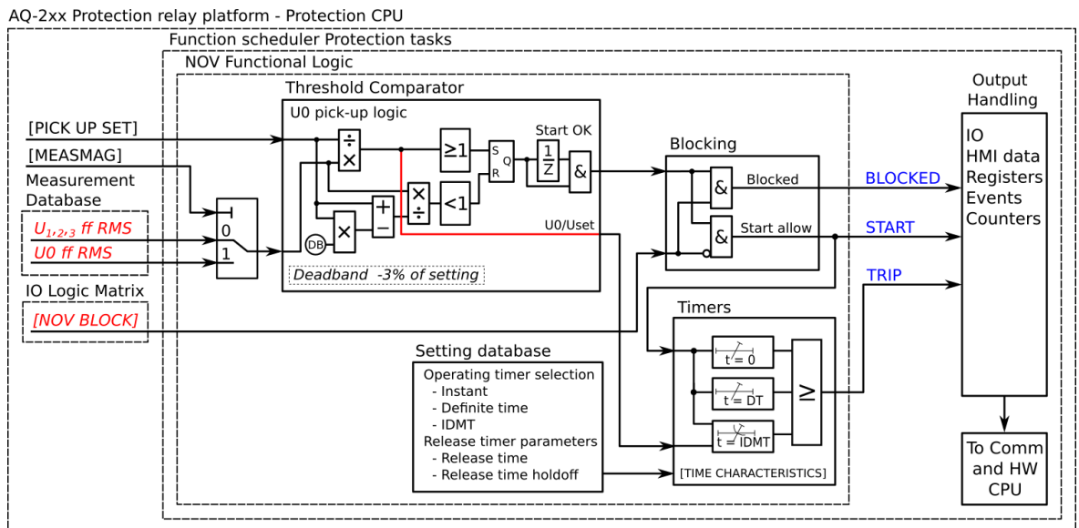
Figure. 4.4.12 - 134. Simplified function block diagram of the U0> function.
