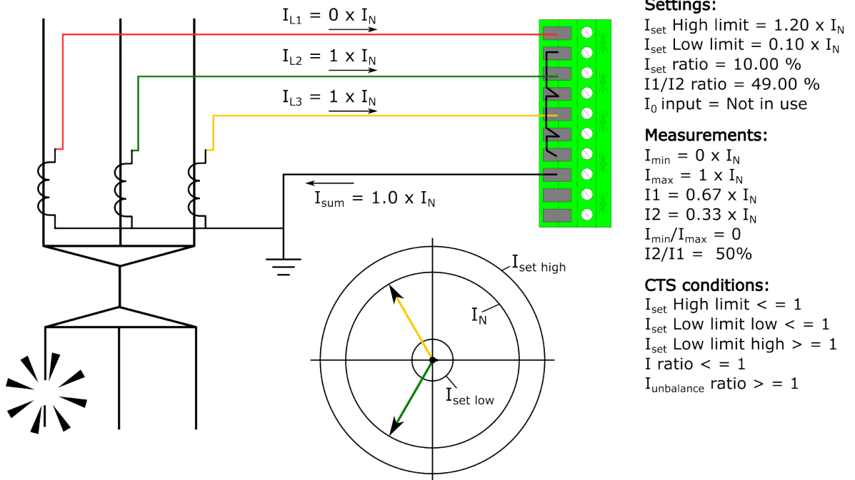
Figure. 4.6.1 - 215. Primary circuit fault in phase L1 wiring.
