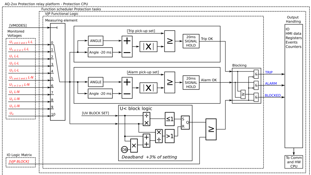
Figure. 4.5.9 - 205. Simplified function block diagram of the \Delta\phi function.
