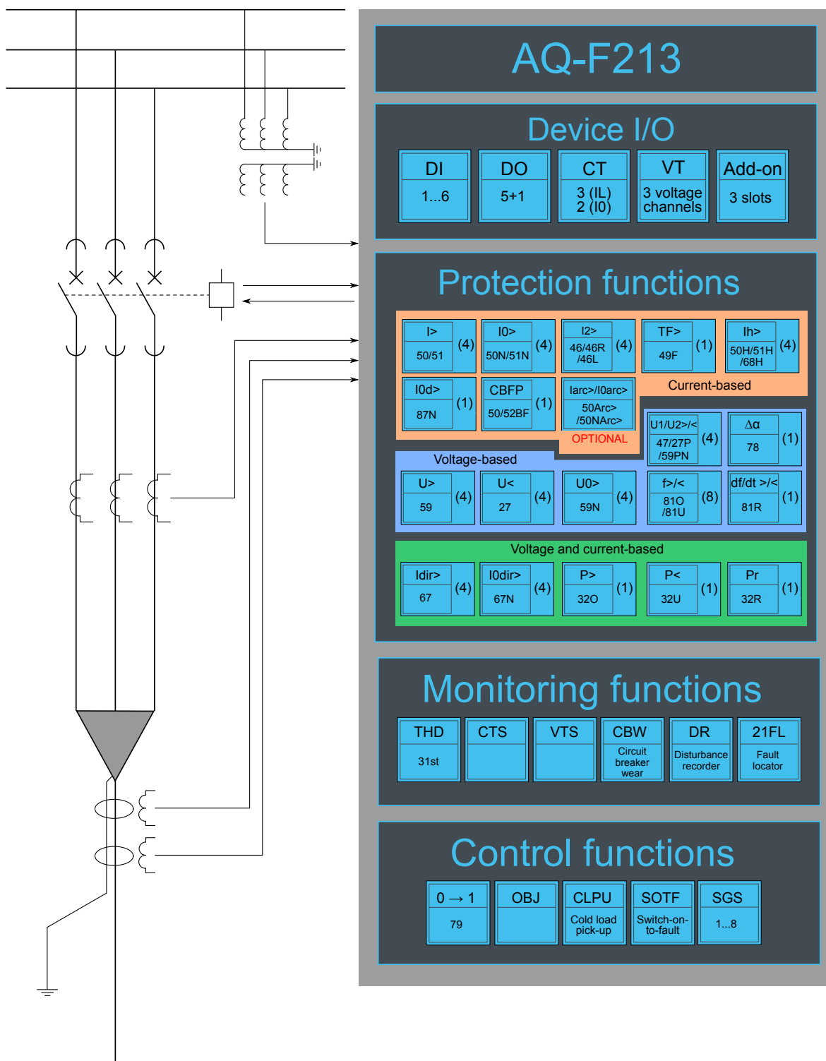
Figure. 6.1 - 234. AQ-F213 application example with function block diagram.
