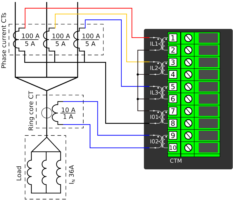
Figure. 4.2.1 - 57. Connections.
