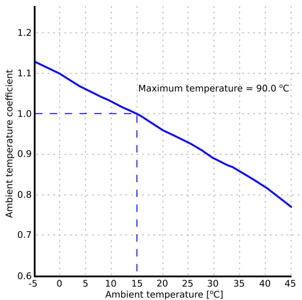
Figure. 4.4.19 - 158. Set correction curve for ambient temperature.
