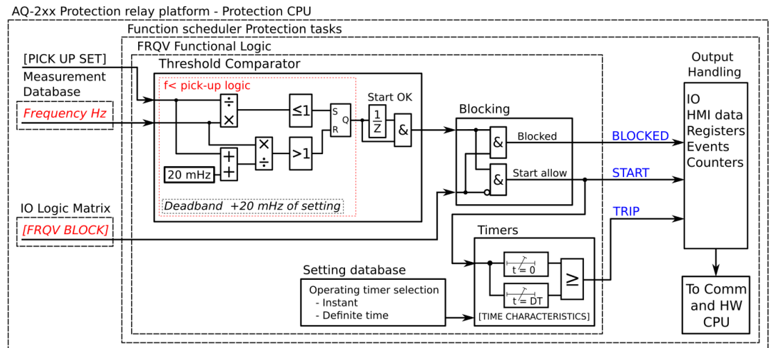
Figure. 4.4.14 - 144. Simplified function block diagram of the f< function.
