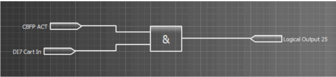
Figure. 4.5.12 - 208. Logic output example. Logical output is connected to an output relay in matrix.
