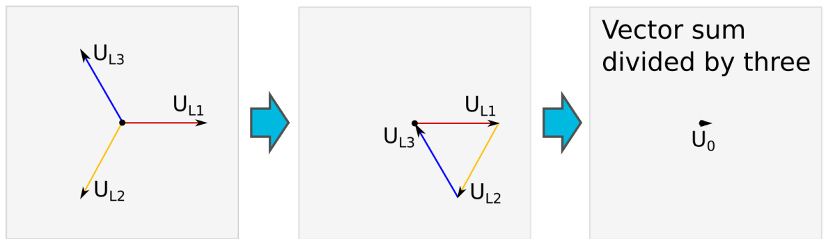
Figure. 4.4.12 - 131. Normal situation.
