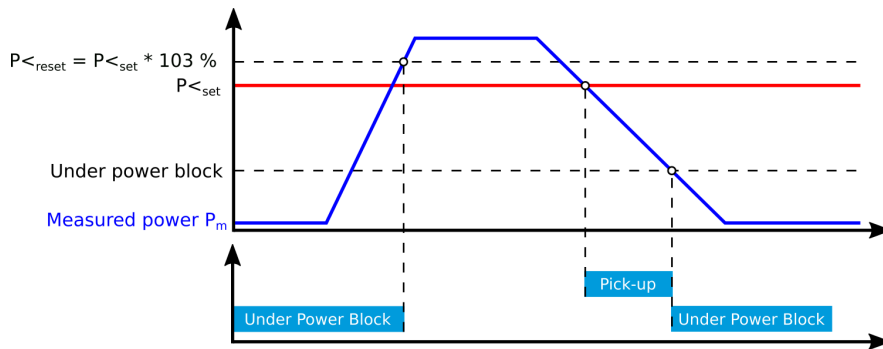
Figure. 4.4.17 - 151. Activation and deactivation characteristics of low power blocking.
