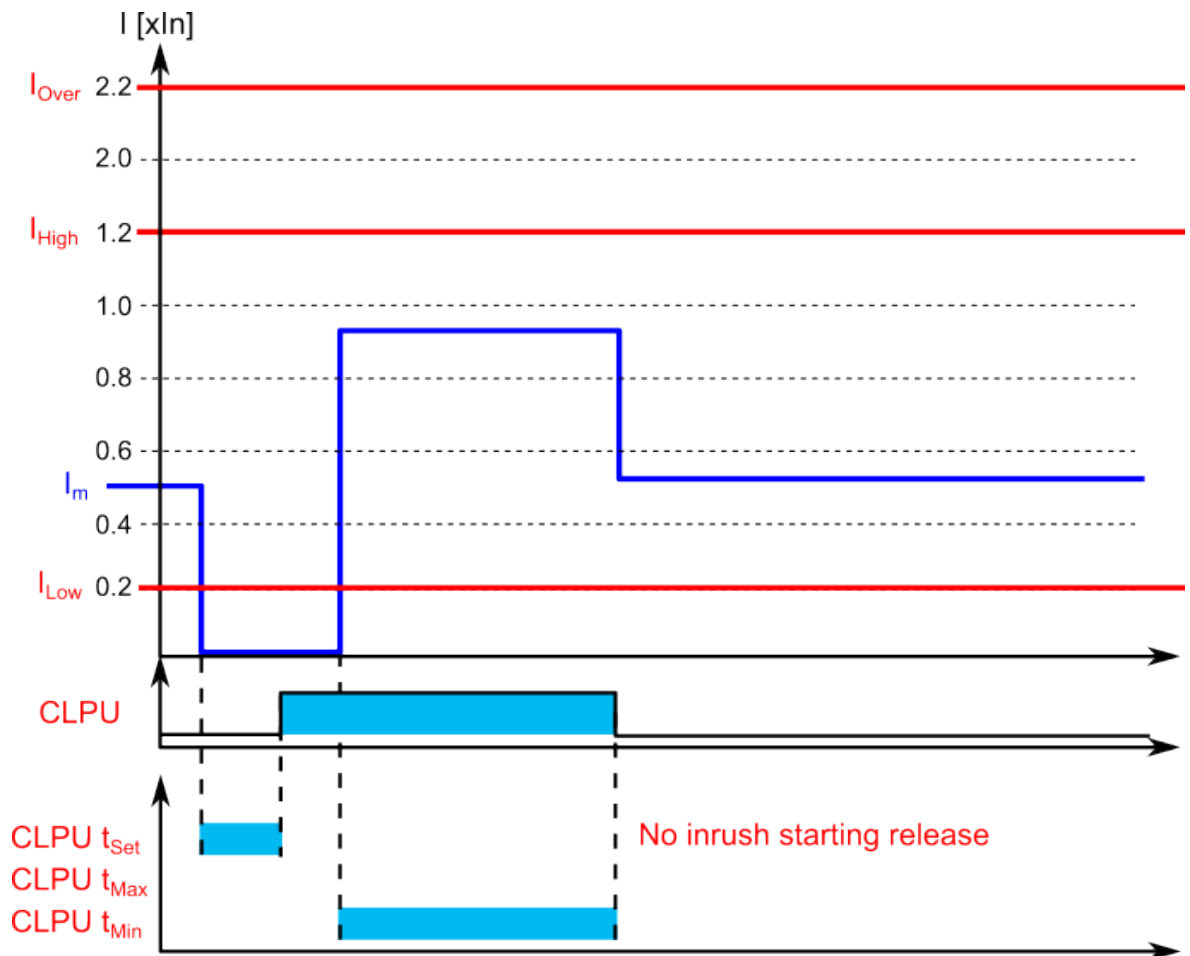
Figure. 4.5.6 - 201. Example of timers and pick-up parameters (no inrush current detected in the starting).
