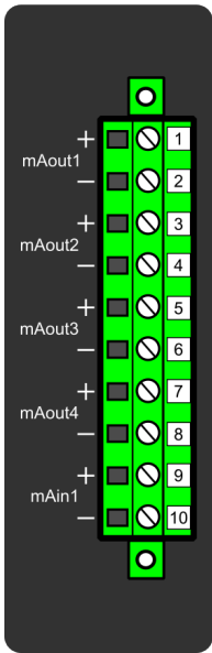
Figure. 7.5.9 - 260. Milliampere (mA) I/O module connections.
