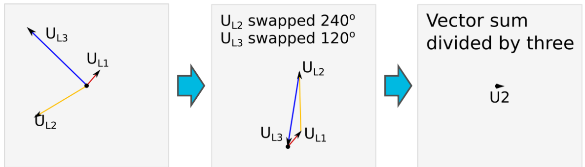
Figure. 4.4.13 - 139. Earth fault in isolated network.
