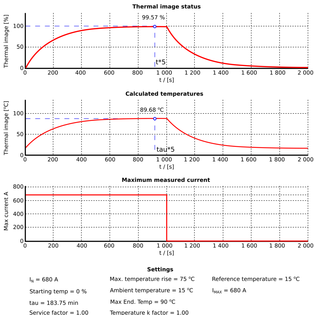
Figure. 5.3.8 - 105. Thermal image response with maximum load (installation according presumptions).
