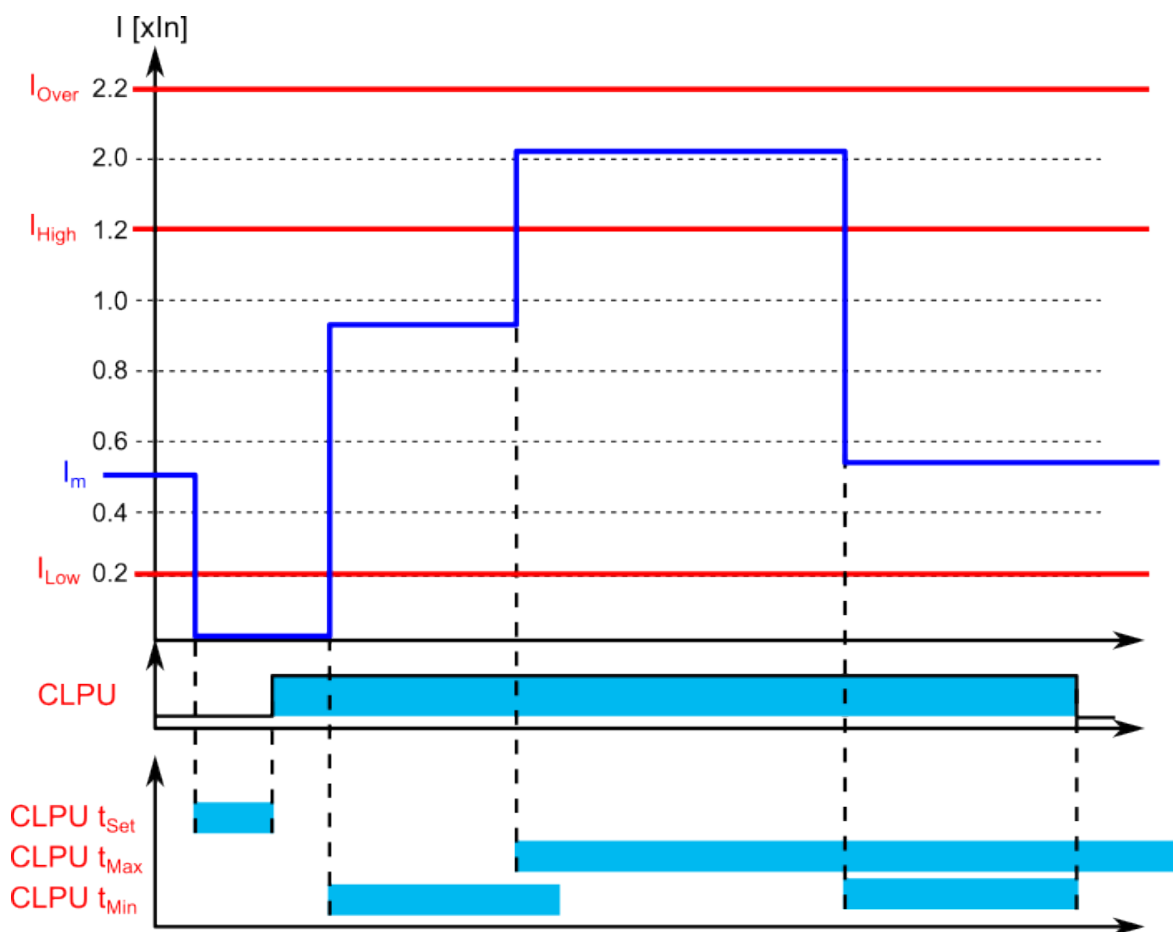
Figure. 5.4.5 - 145. Example of timers and pick-up parameters (an inrush current detected during T_{min} time).
