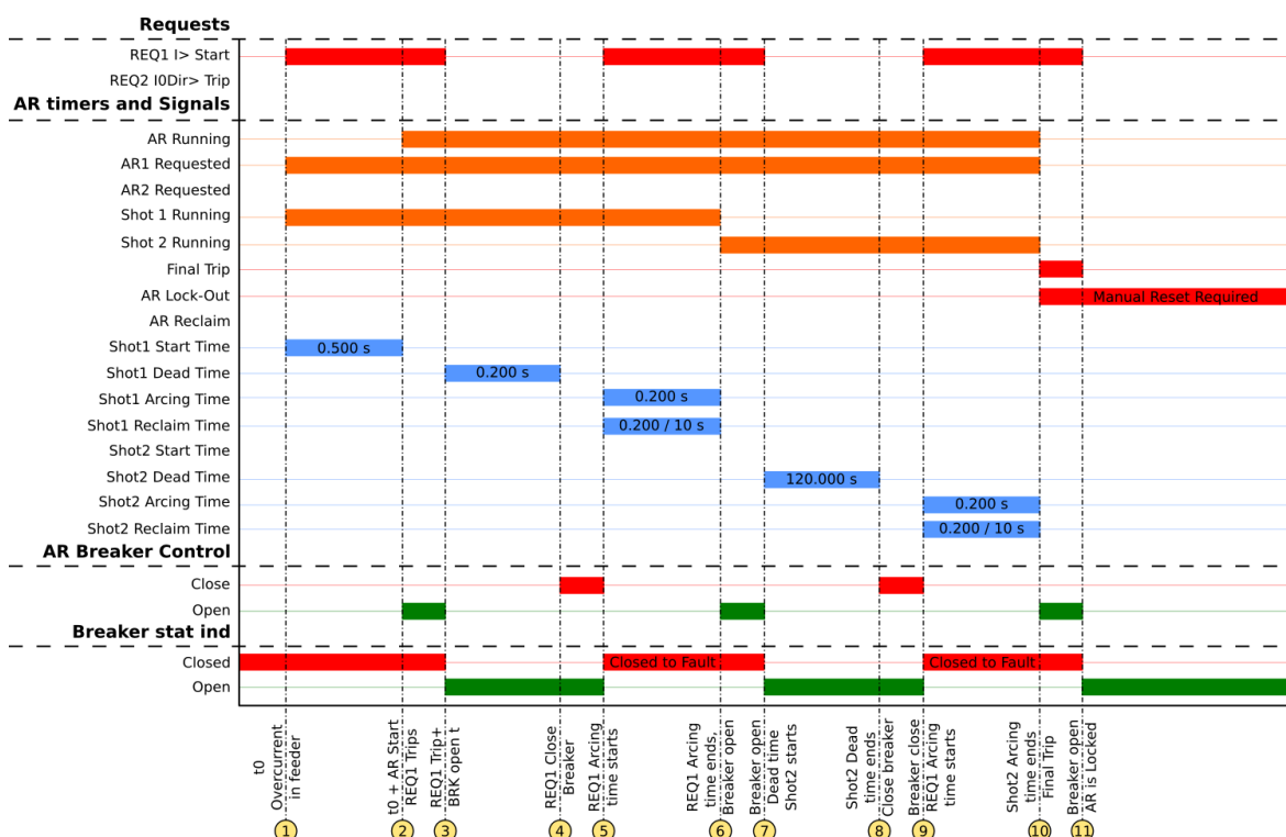
Figure. 5.4.4 - 131. Signal status graph of the permanent overcurrent auto-recloser cycle.
