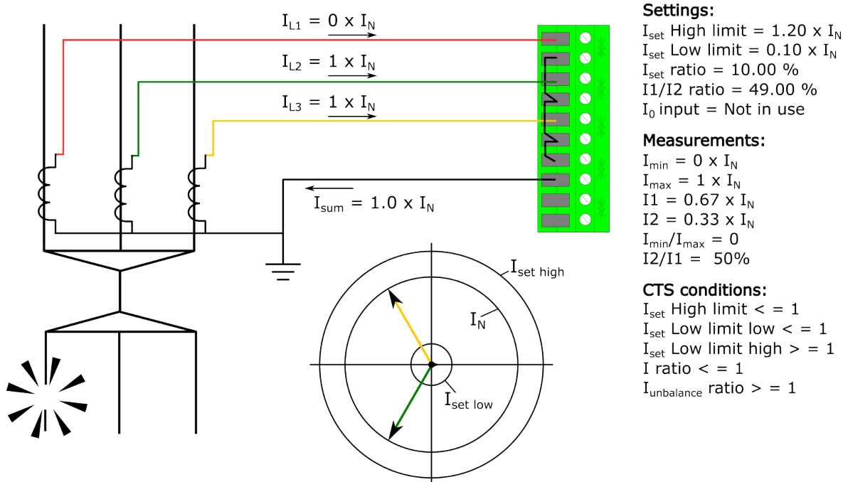
Figure. 5.5.1 - 156. Primary circuit fault in phase L1 wiring.
