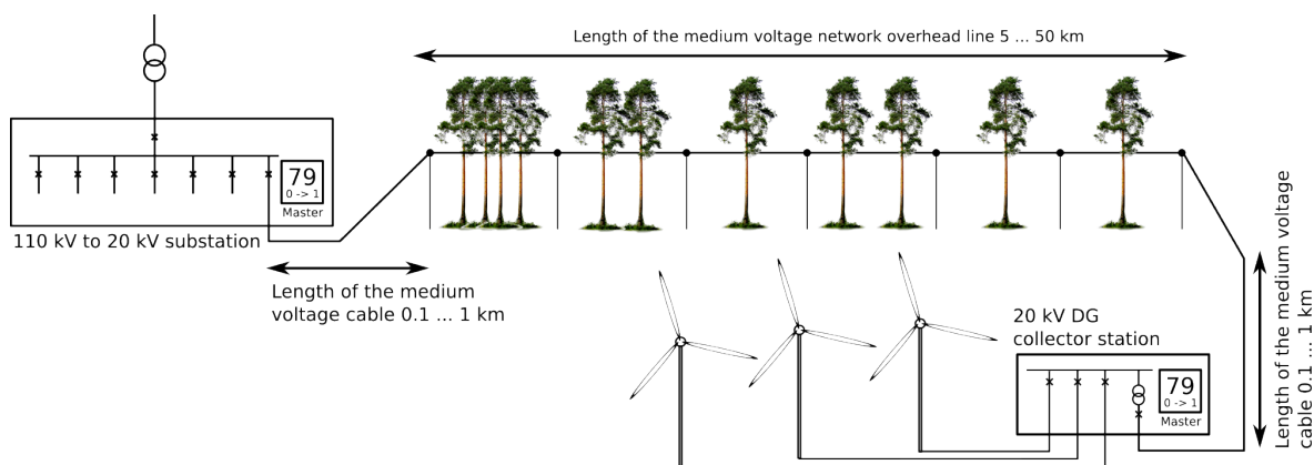
Figure. 5.4.4 - 136. Auto-reclosing with distributed generation in the line.
