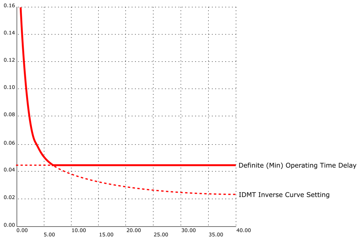
Figure. 5.3.1 - 65. Operating time delay: Definite (Min) and the minimum for tripping.
