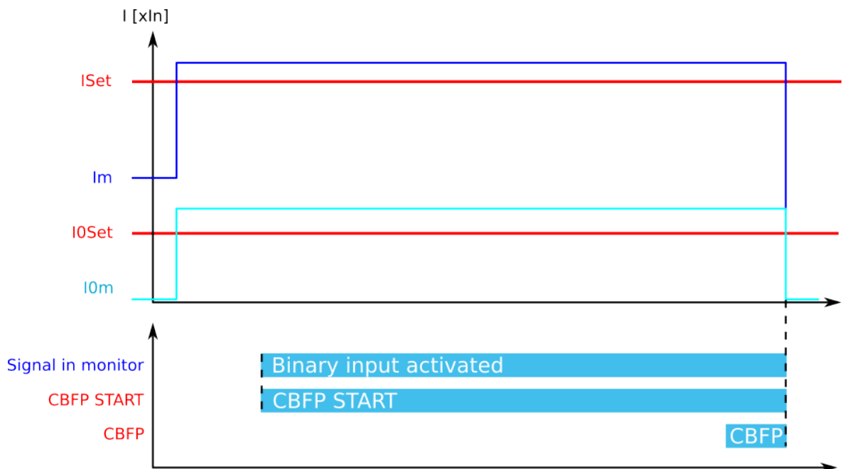
Figure. 5.3.6 - 86. Dedicated CBFP operation from digital input signal.
