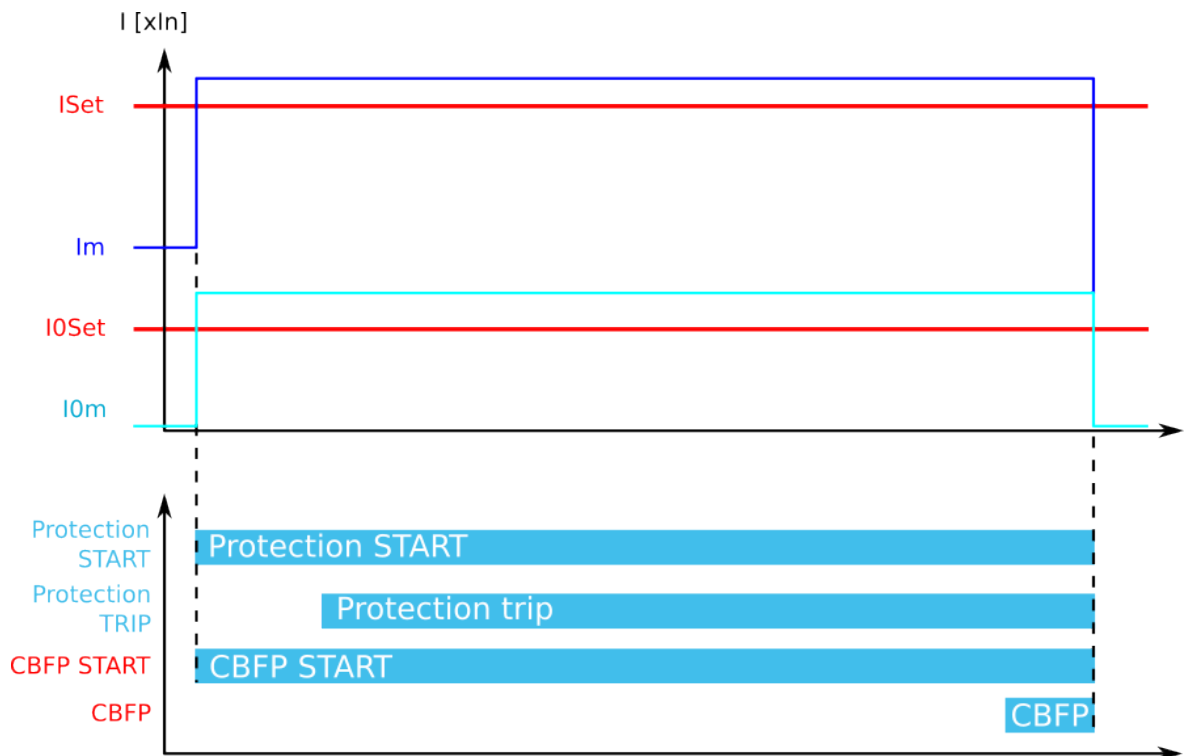
Figure. 5.3.6 - 82. CBFP when "Current" is the selected criterion.
