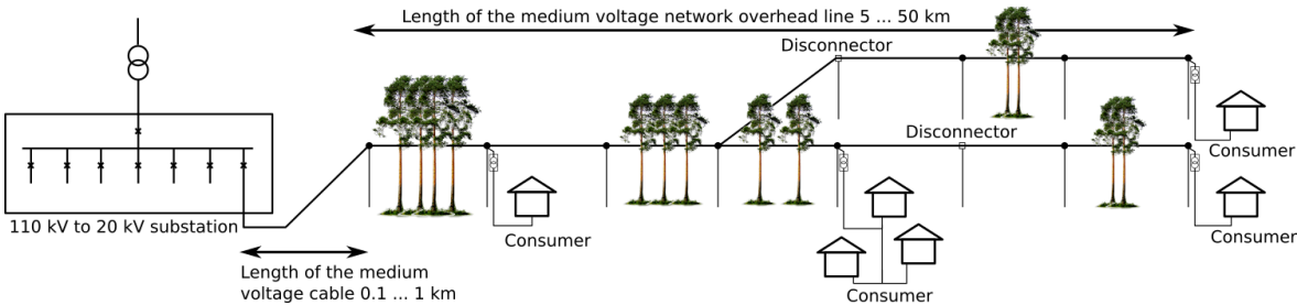
Figure. 5.4.4 - 121. Diagram of a typical radial medium-voltage network in rural areas.
