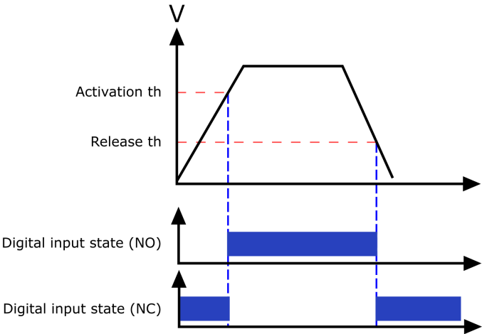
Figure. 8.4 - 186. Digital input state when energizing and de-energizing the digital input channels.
