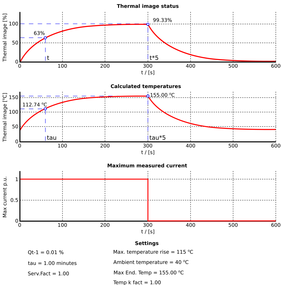
Figure. 5.3.8 - 96. Example of thermal image calculation with nominal conditions.
