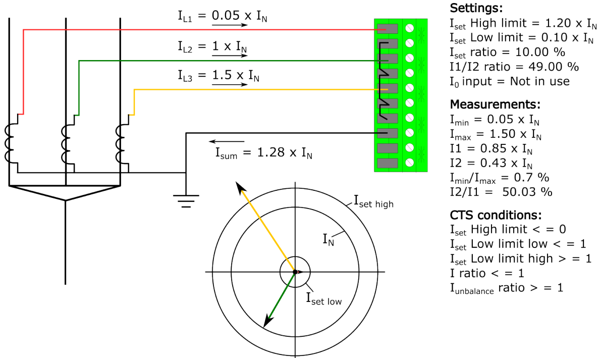
Figure. 5.5.1 - 157. No wiring fault but heavy unbalance.
