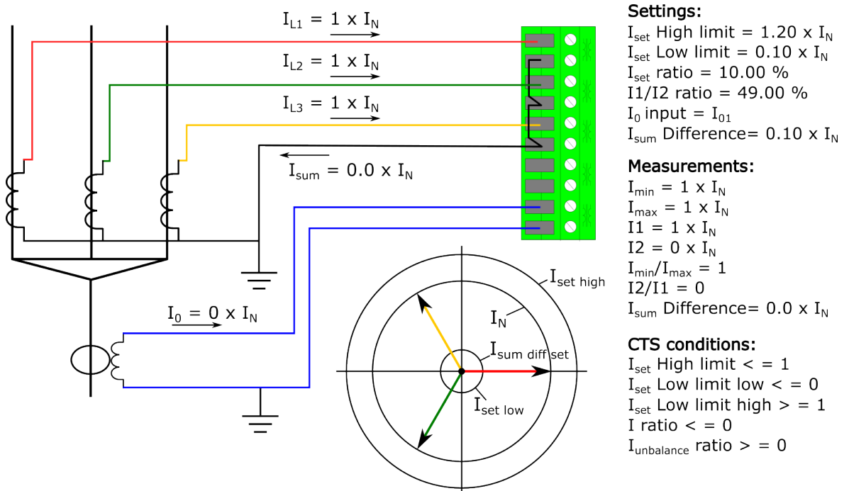
Figure. 5.5.1 - 159. Normal situation, residual current also measured.
