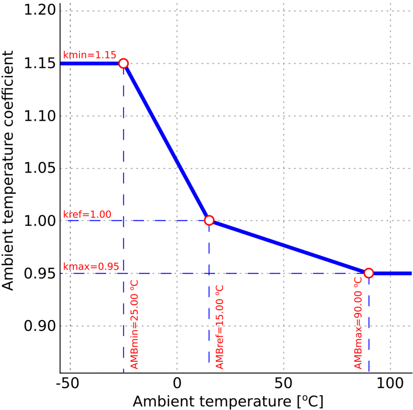
Figure. 5.3.8 - 97. Ambient temperature coefficient calculation (a three-point linear approximation and a settable correction curve).
