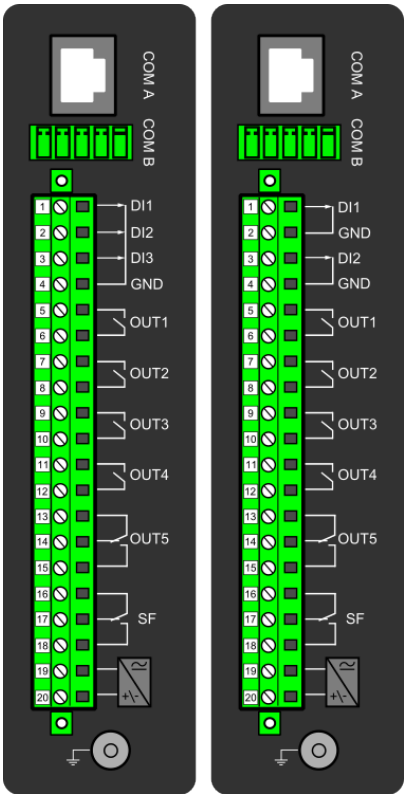
Figure. 8.2 - 183. CPU module.
