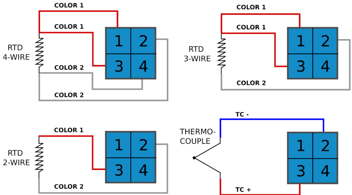
Figure. 8.7 - 190. Different sensor types and their connections.
