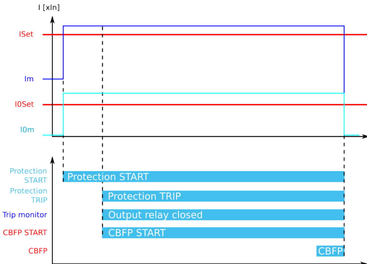
Figure. 5.3.6 - 83. CBFP when "Current and DO" is the selected criterion.
