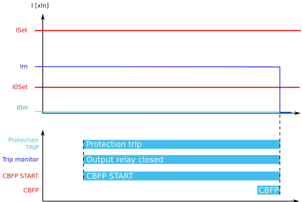
Figure. 5.3.6 - 84. CBFP when "Current or DO" is the selected criterion.
