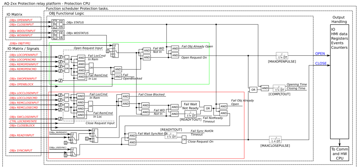
Figure. 5.4.2 - 119. Simplified function block diagram of the object control and monitoring function.
