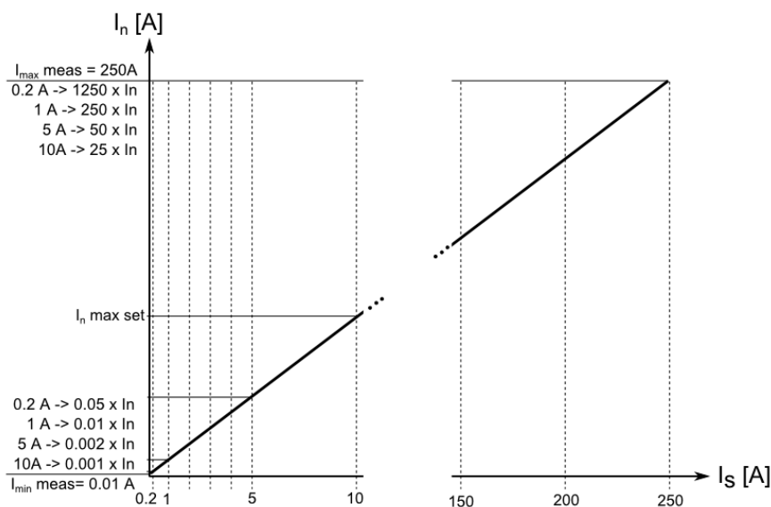
Figure. 5.3.1 - 64. Measurement range in relation to the nominal current.
