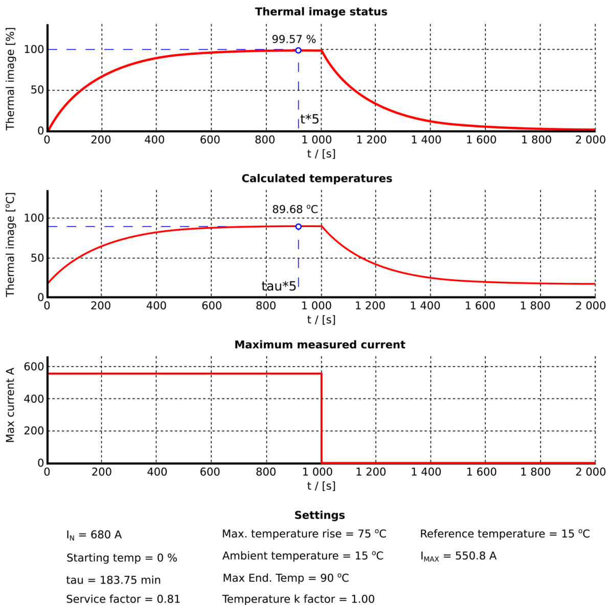
Figure. 5.3.8 - 107. Thermal response with k_{SF} factor correctly set.
