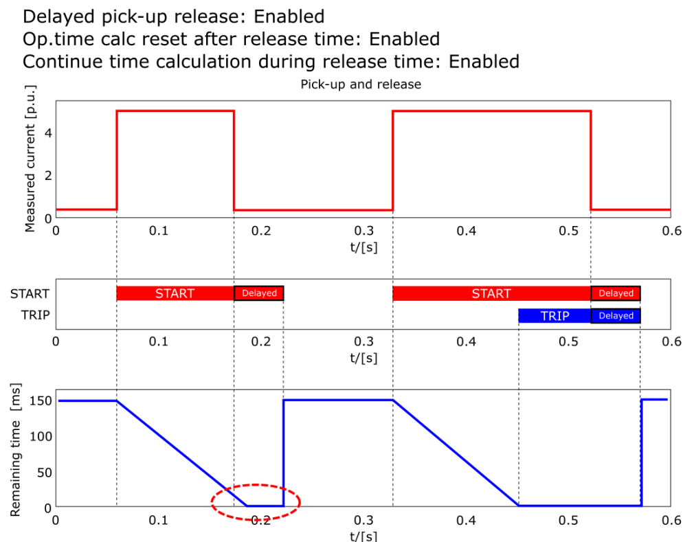
Figure. 5.3.1 - 70. Delayed pick-up release, delay counter value is decreasing during the release time.
