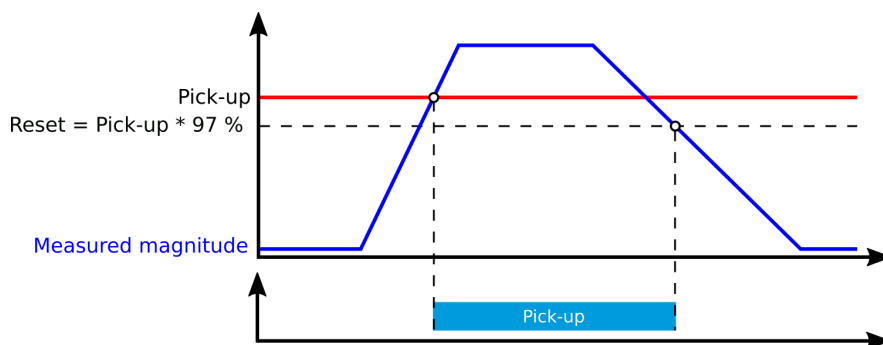
Figure. 5.3.1 - 63. Pick up and reset.
