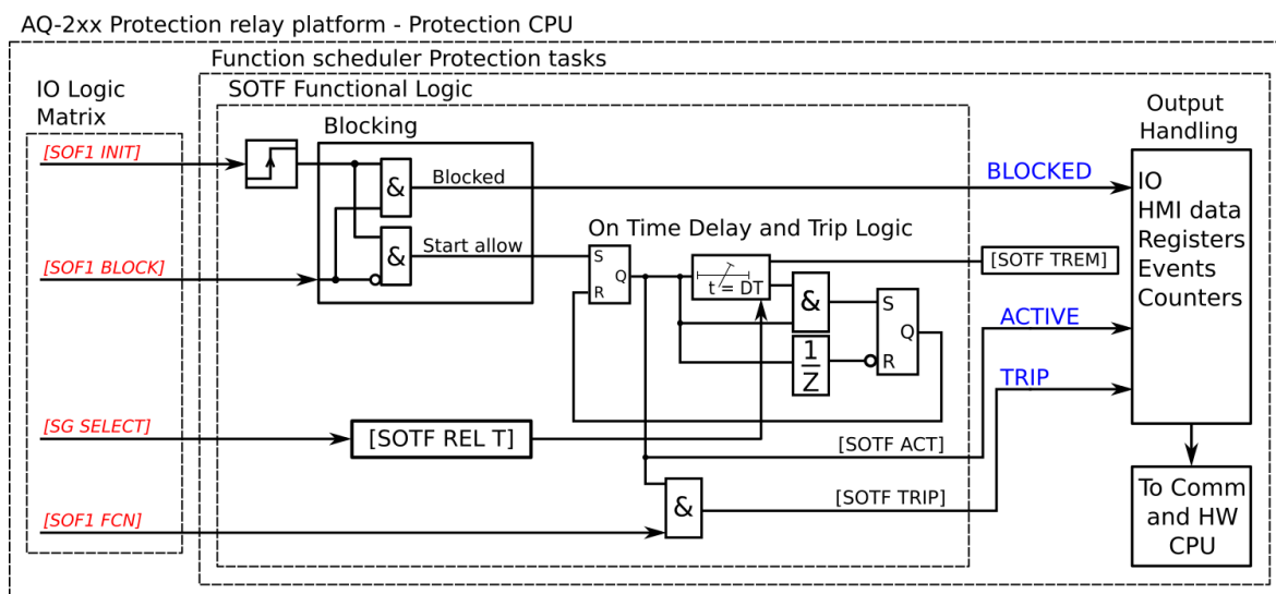
Figure. 5.4.6 - 146. Simplified function block diagram of the switch-on-to-fault function.
