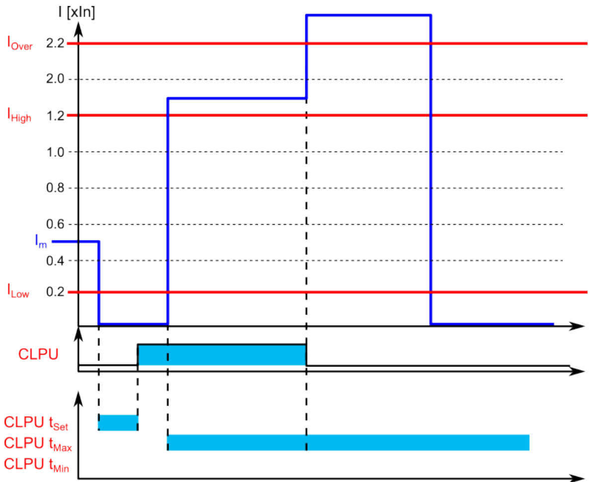
Figure. 5.4.5 - 142. Example of timers and pick-up parameters (activated pick-up and instant release due to overcurrent).
