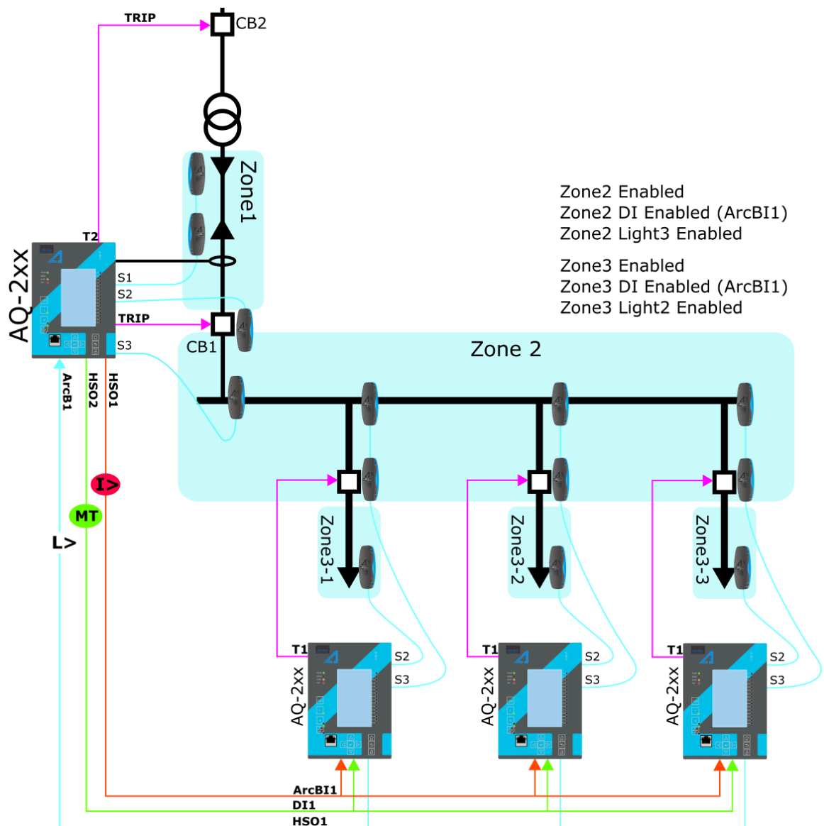
Figure. 5.3.10 - 112. Scheme IA1 (with AQ-200 protection relays).
