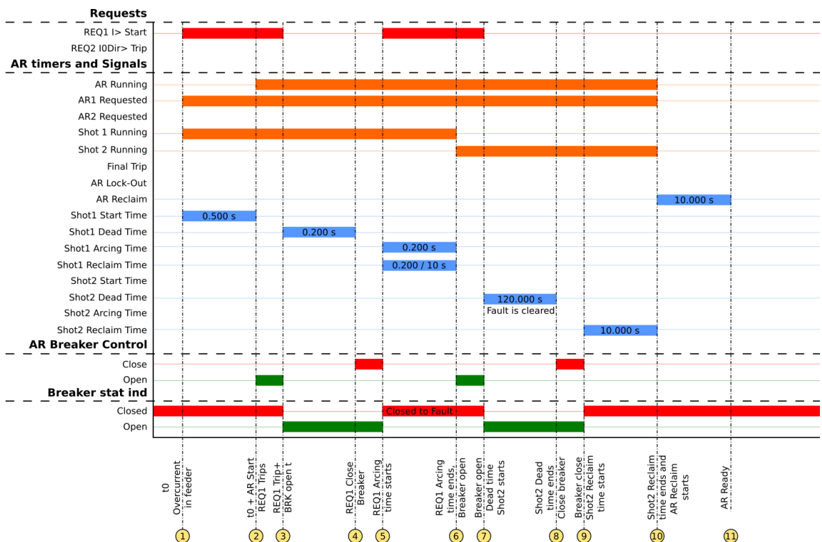
Figure. 5.4.4 - 133. Signal status graph of the semi-permanent overcurrent auto-recloser cycle.
