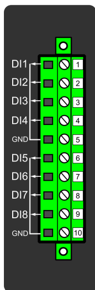
Figure. 8.4 - 185. Digital input module (DI8) with eight add-on digital inputs.
