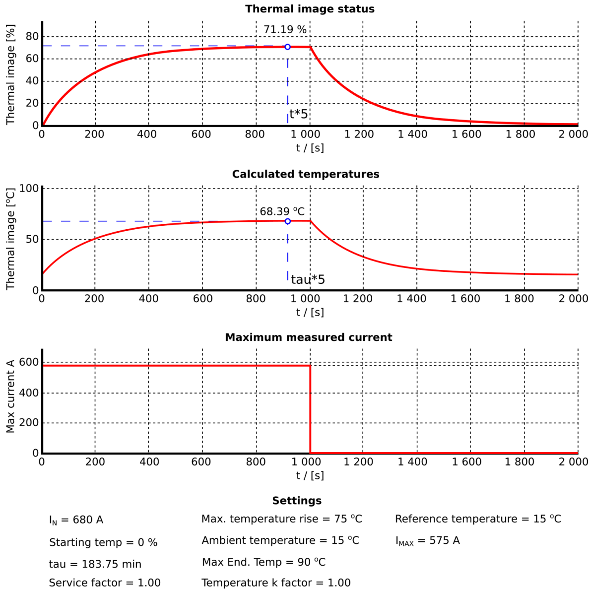
Figure. 5.3.8 - 104. Thermal image response with nominal load (installation according to presumptions).
