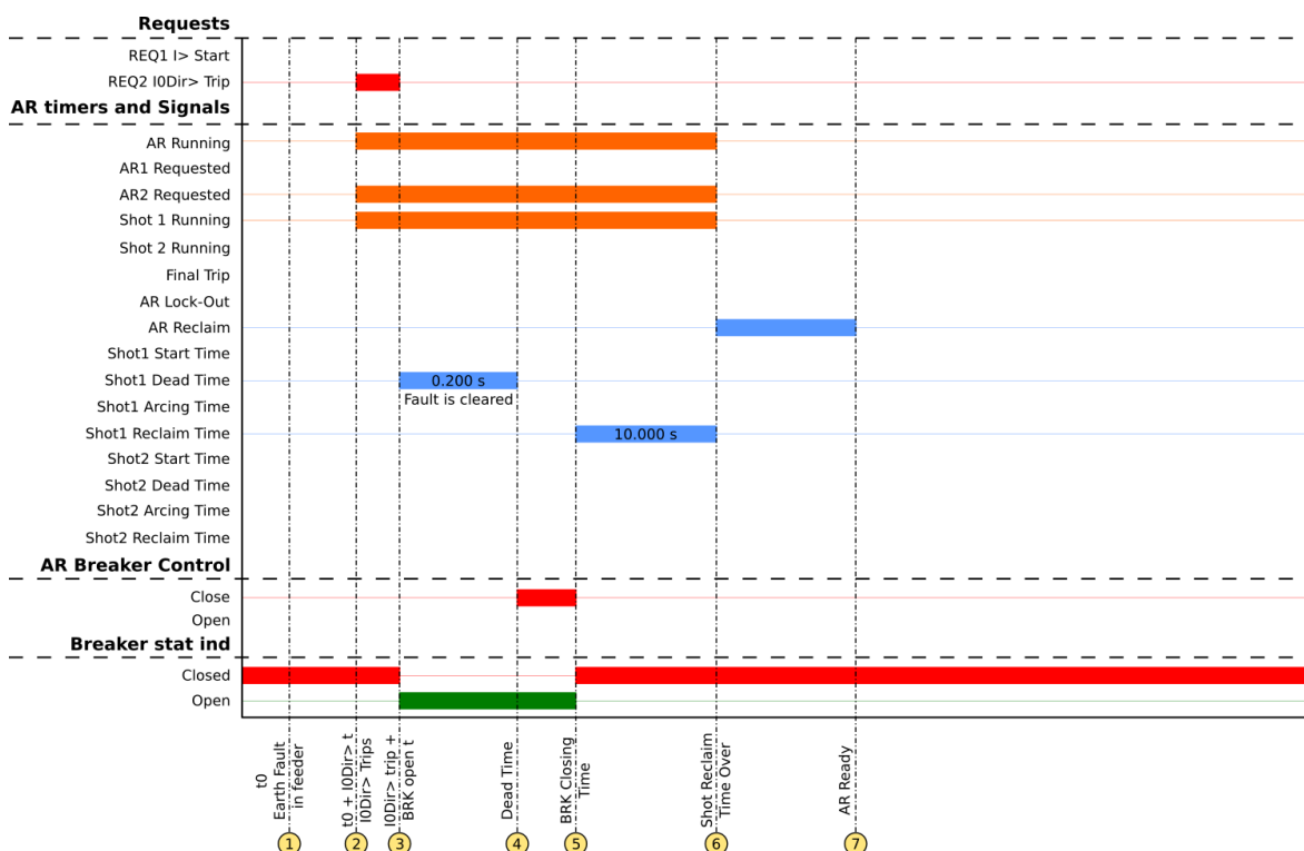
Figure. 5.4.4 - 129. Signal status graph of the transient earth fault auto-recloser cycle.
