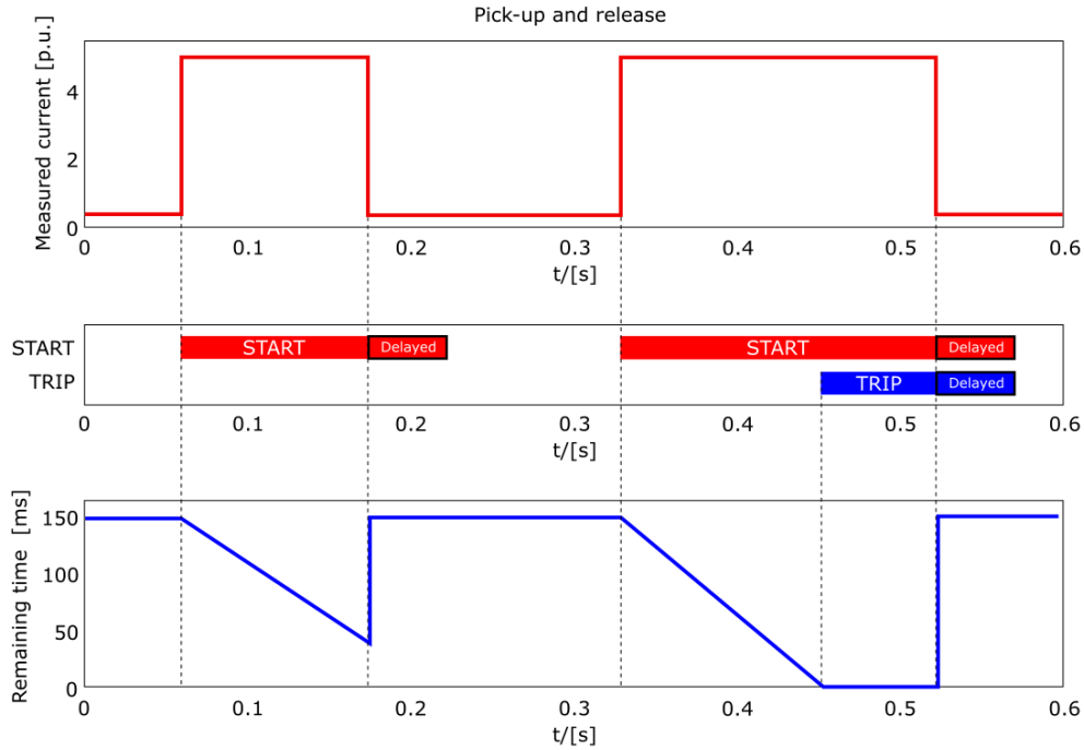
Figure. 5.3.1 - 69. Delayed pick-up release, delay counter value is held during the release time.
