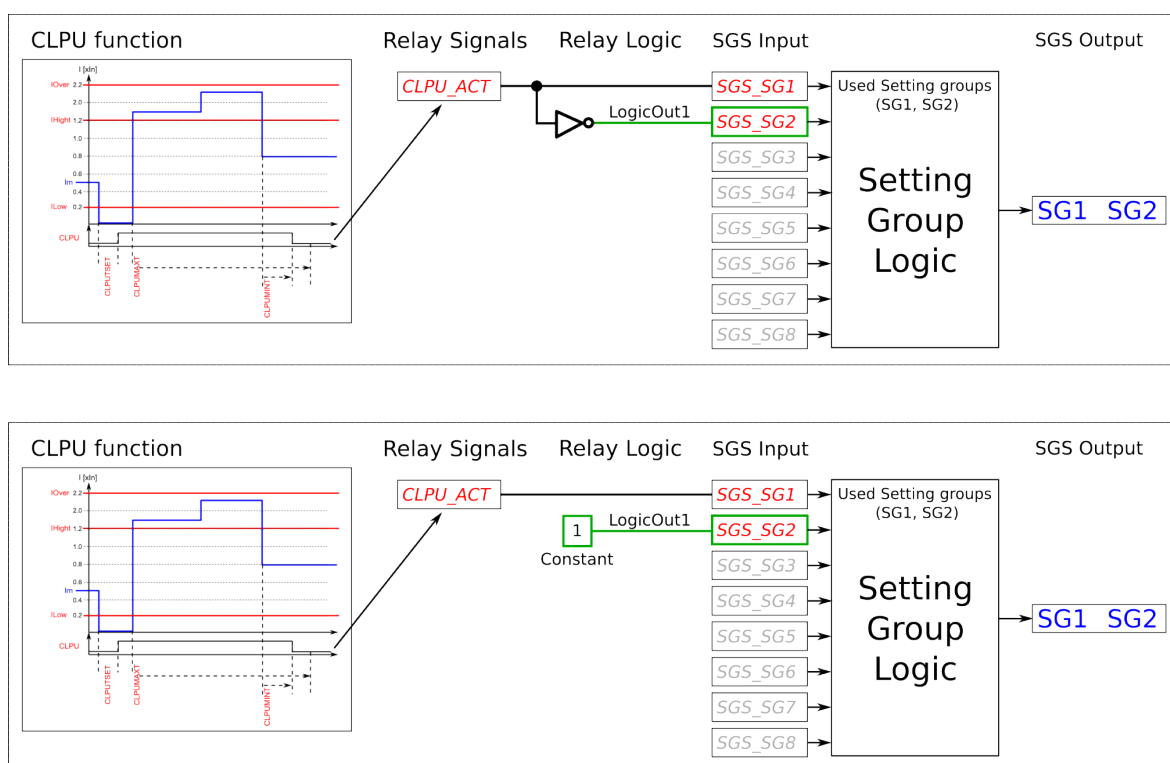
Figure. 5.4.1 - 118. Entirely application-controlled setting group change with the cold load pick-up function.
