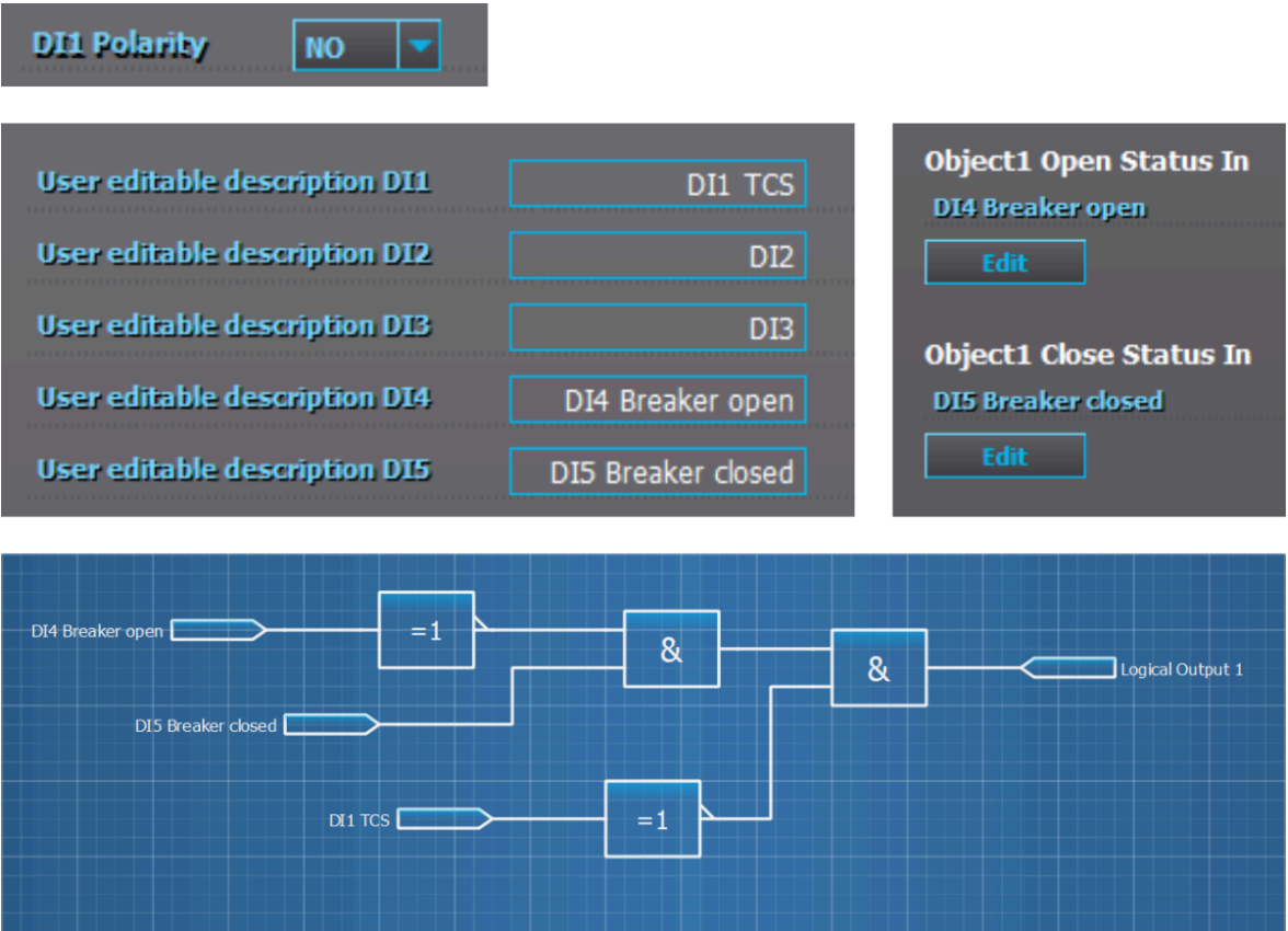
Figure. 7.4 - 180. Example block scheme.
