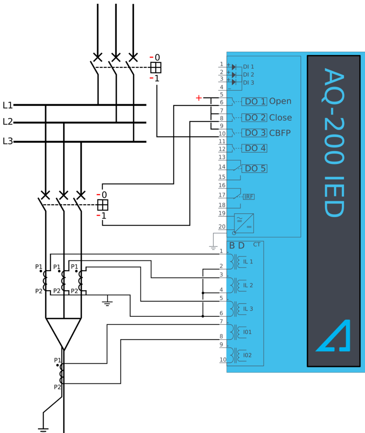
Figure. 5.3.6 - 81. Wiring diagram when Trip and CBFP are configured to the device.
