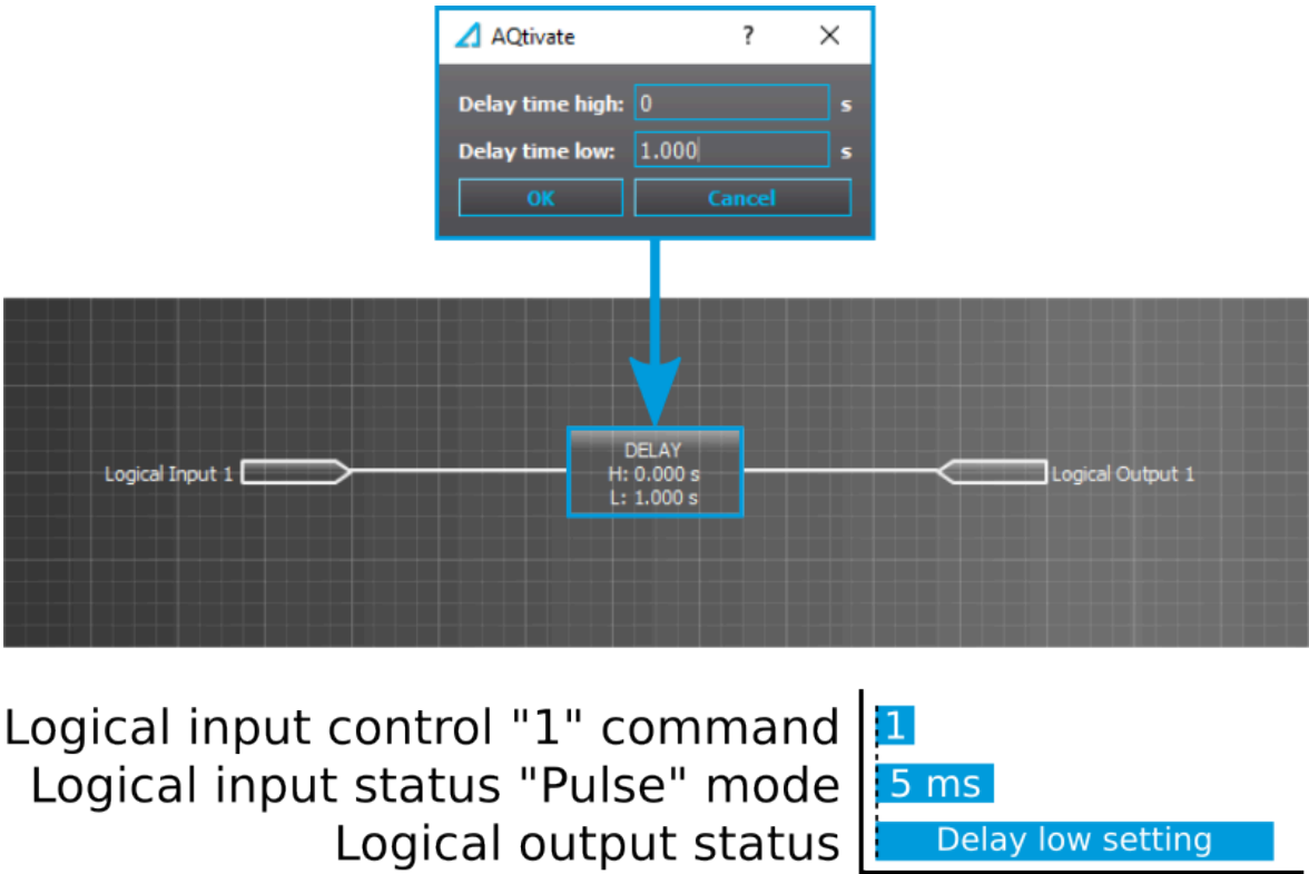
Figure. 5.4.11 - 151. Extending a logical input pulse.
