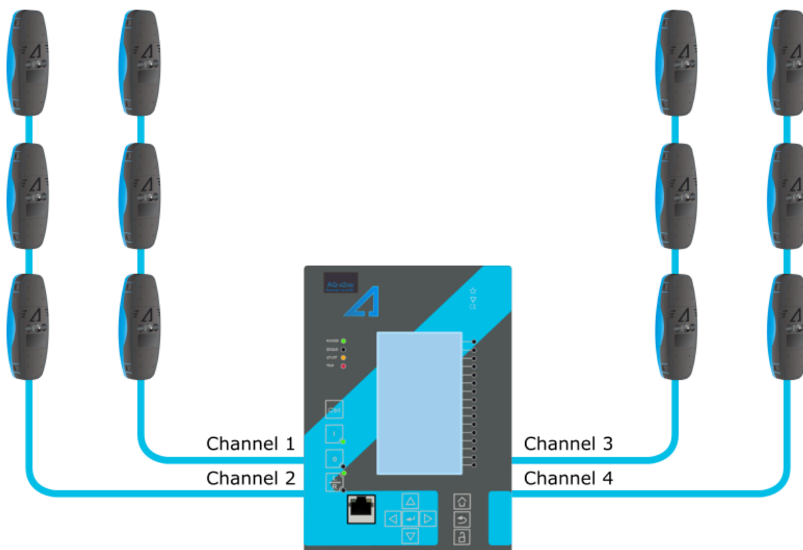
Figure. 5.3.10 - 110. IED equipped with arc protection.
