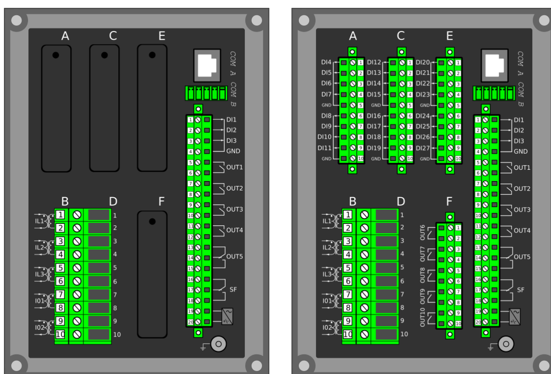
Figure. 8.1 - 181. Modular construction of AQ-X210.
