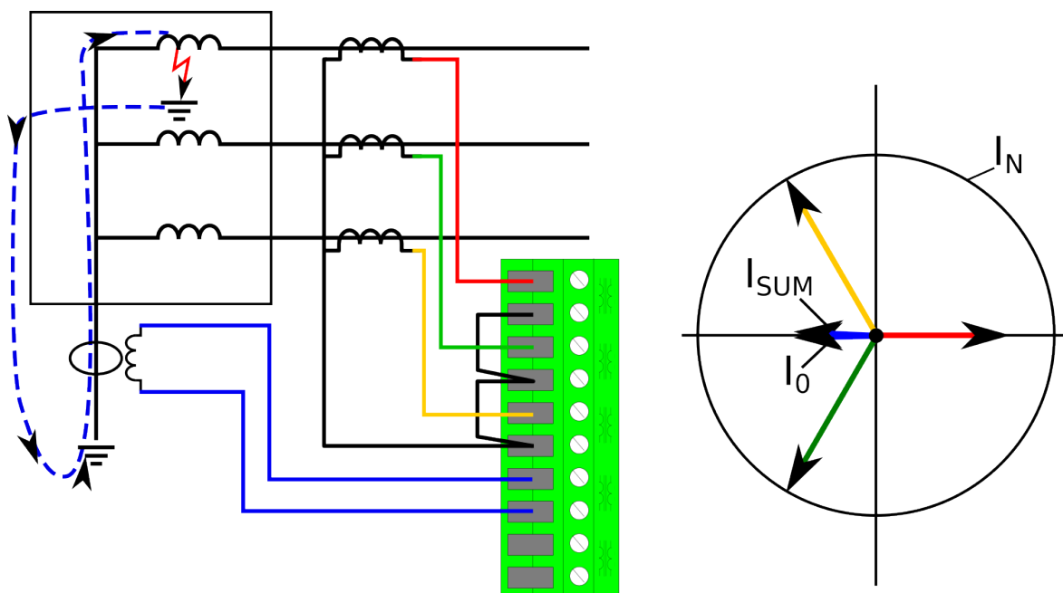
Figure. 5.3.7 - 95. Restricted earth fault inside a Y winding transformer.
