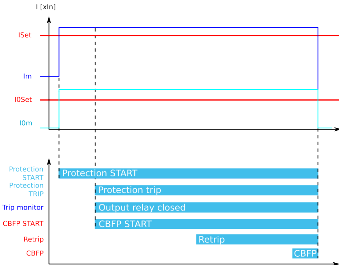
Figure. 5.3.6 - 79. Retrip and CBFP when "Current and DO" is the selected criterion.
