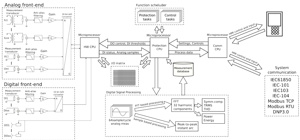
Figure. 5.3.1 - 62. Principle diagram of the protection relay platform.
