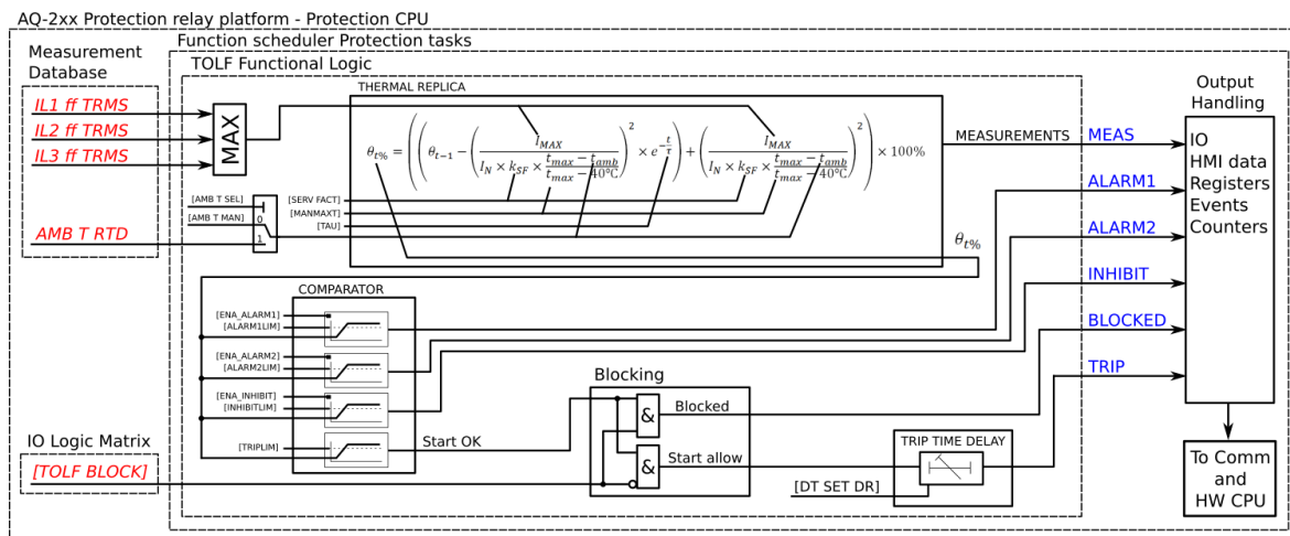
Figure. 5.3.8 - 108. Simplified function block diagram of the TF> function.
