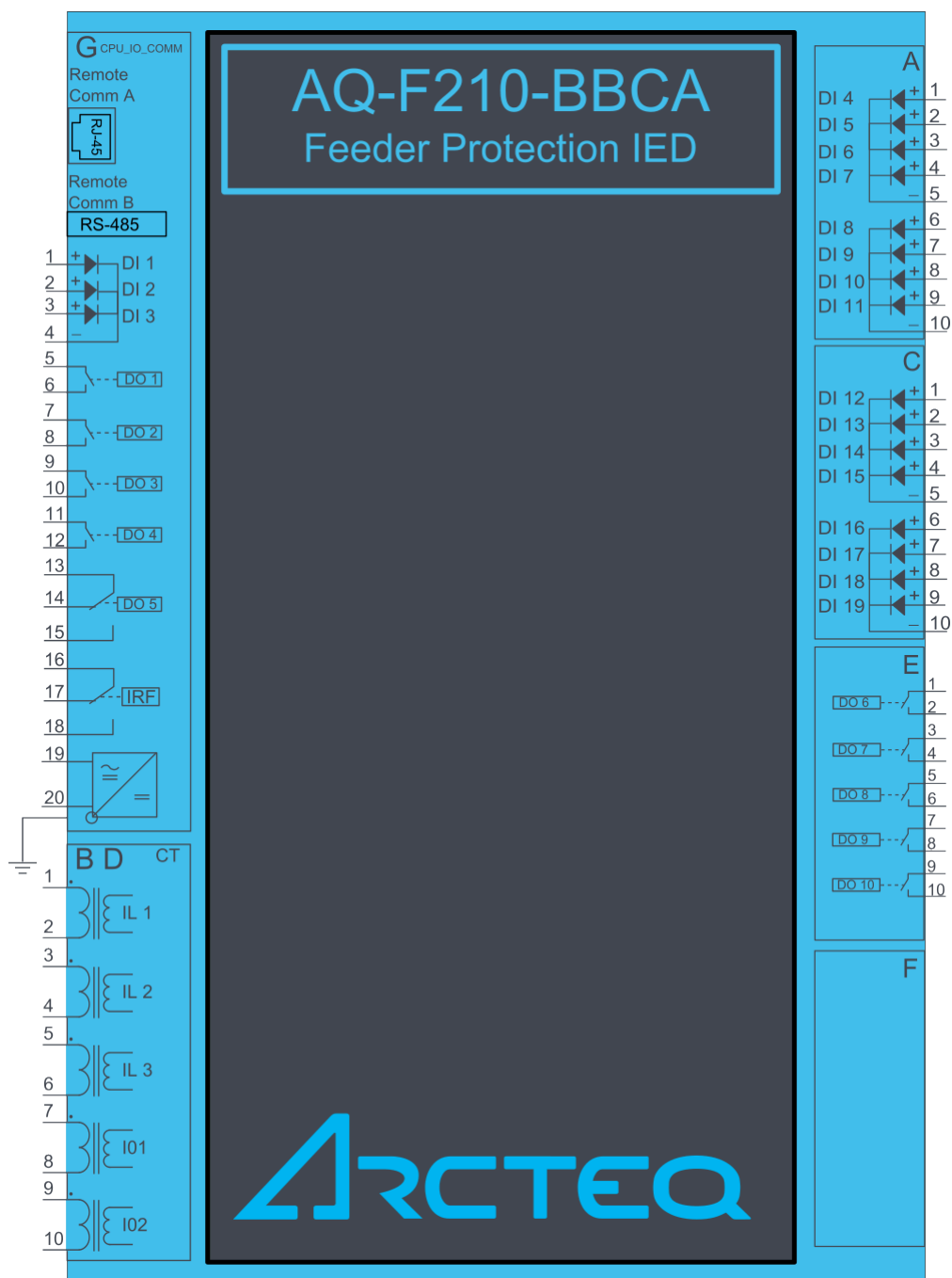
Figure. 7.1 - 172. AQ-F210 variant with digital input and output modules.
