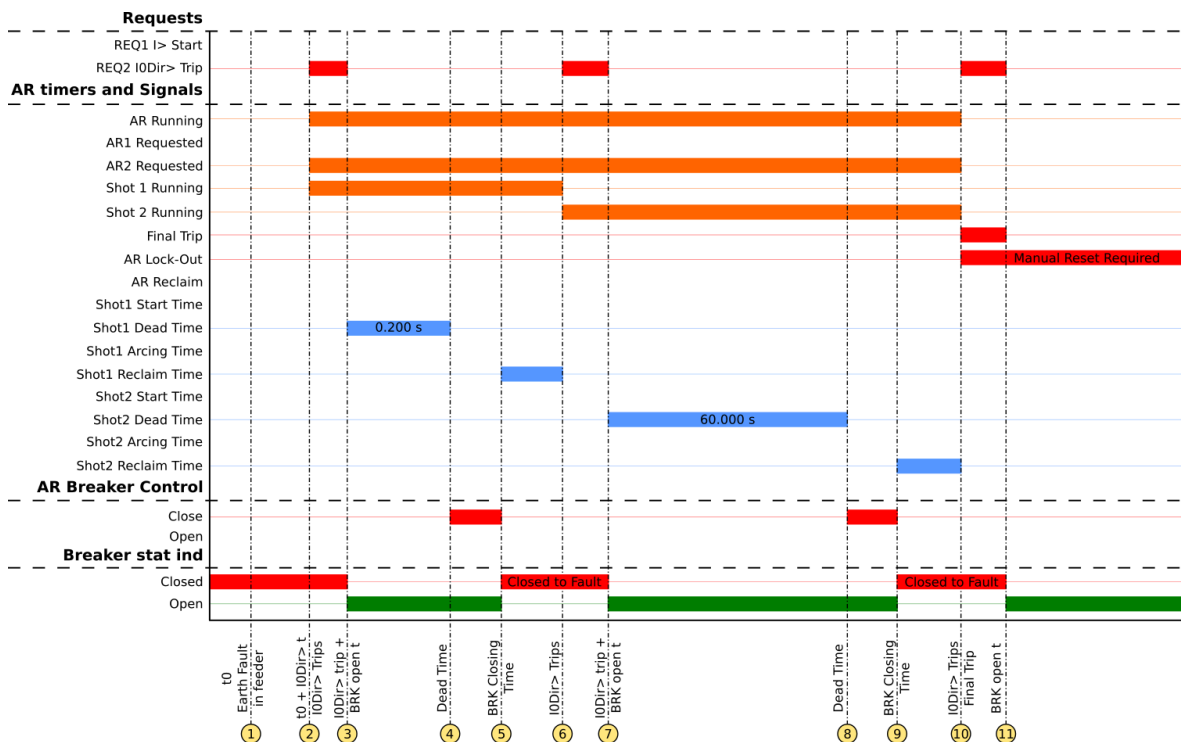
Figure. 5.4.4 - 125. Signal status graph of the permanent earth fault auto-recloser cycle.
