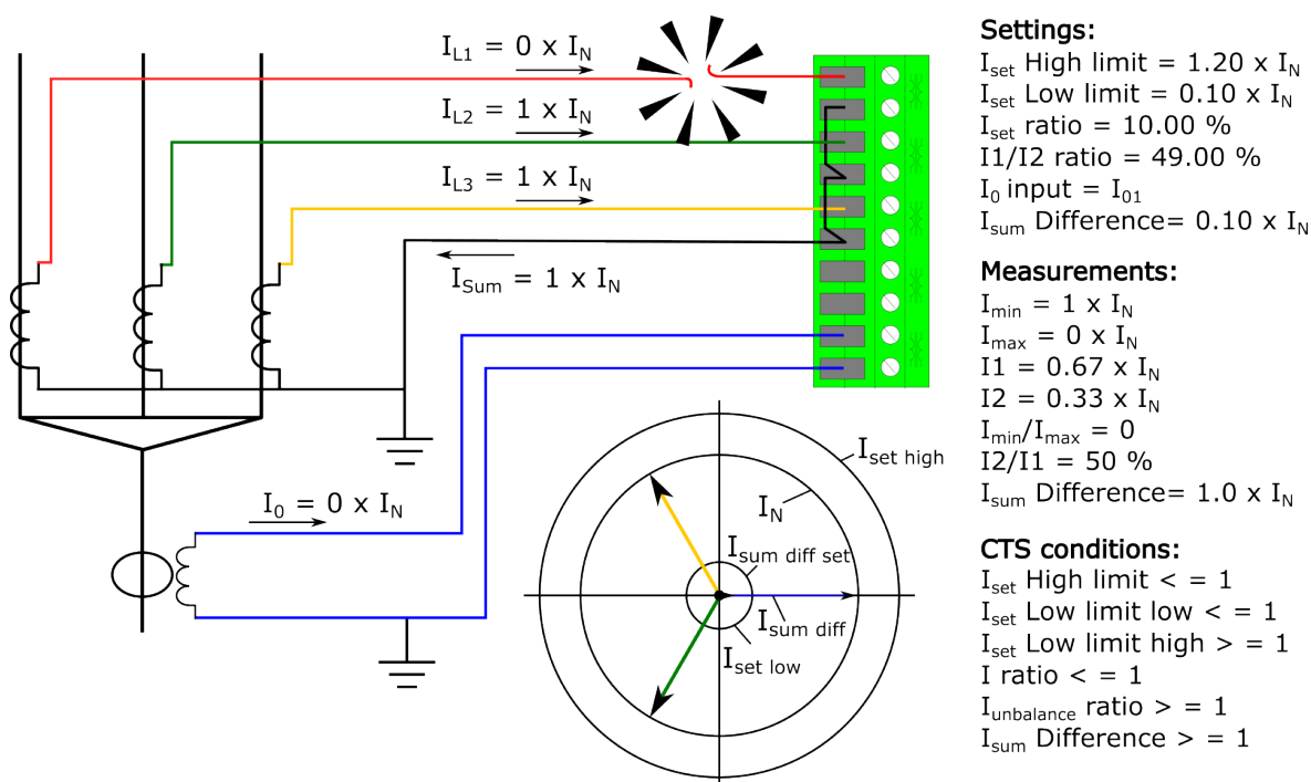
Figure. 5.5.1 - 160. Broken secondary phase current wiring.
