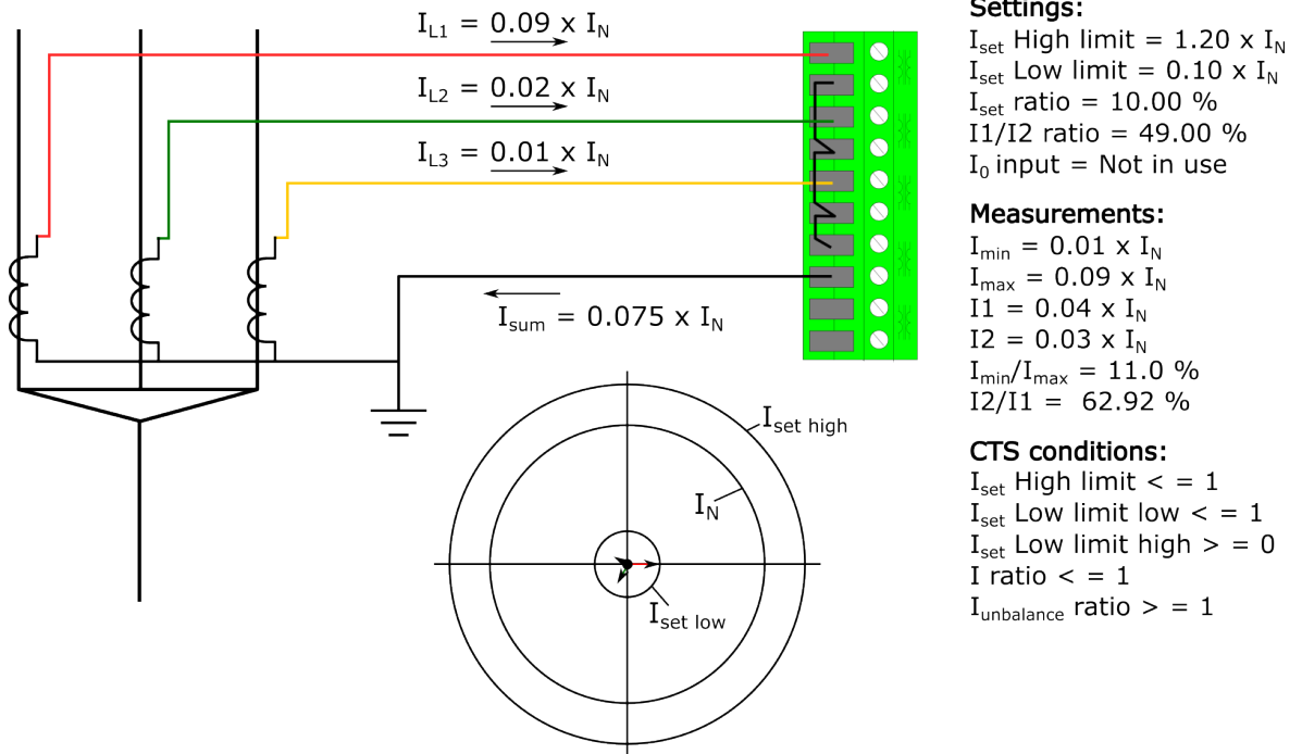
Figure. 5.5.1 - 158. Low current and heavy unbalance.
