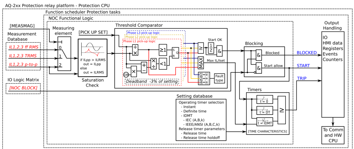
Figure. 5.3.2 - 71. Simplified function block diagram of the I> function.
