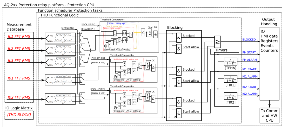
Figure. 5.5.3 - 166. Simplified function block diagram of the total harmonic distortion monitor function.
