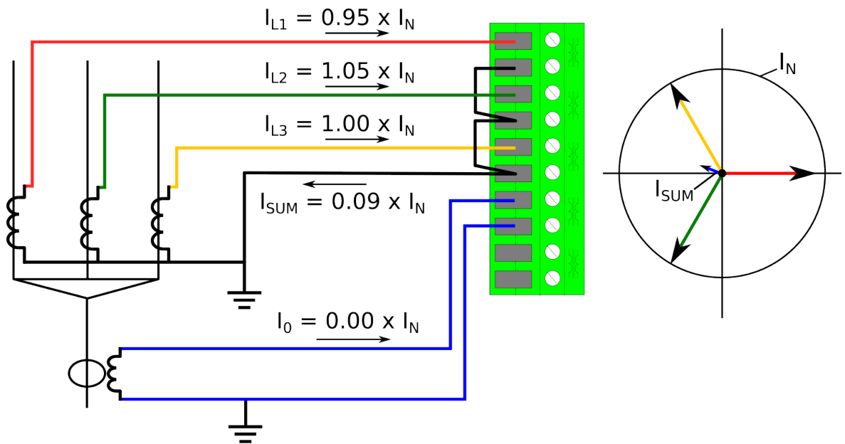
Figure. 5.3.7 - 92. Cable end differential with natural unbalance in the phase current measurement.
