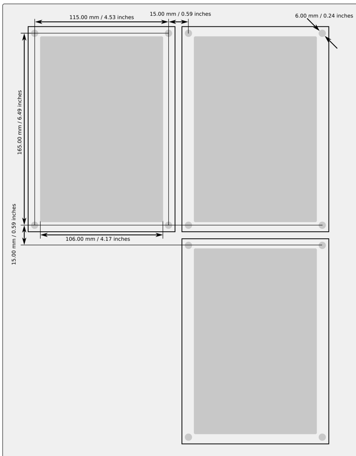
Figure. 8.13 - 202. Panel cutout dimensions and device spacing.
