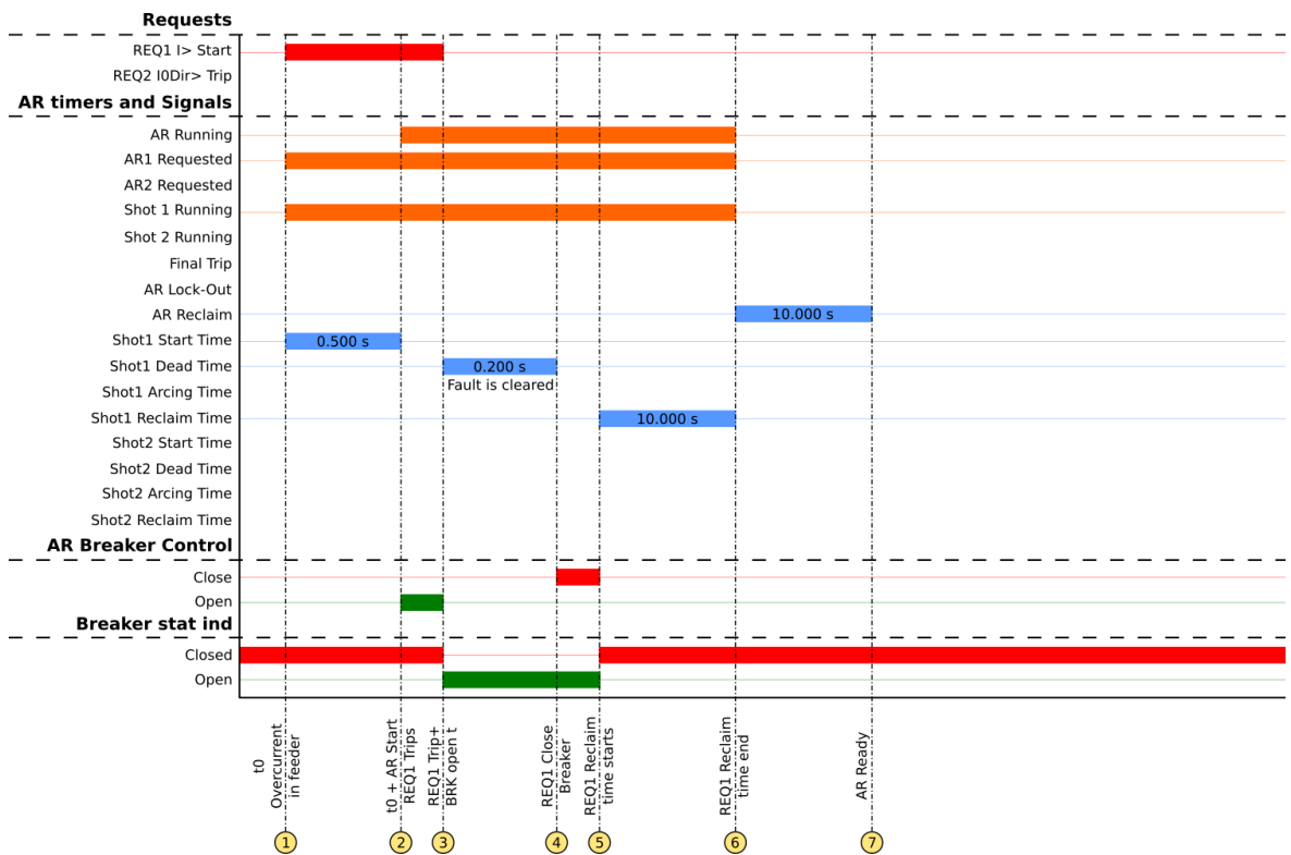
Figure. 5.4.4 - 135. Signal status graph of the transient overcurrent auto-recloser cycle.
