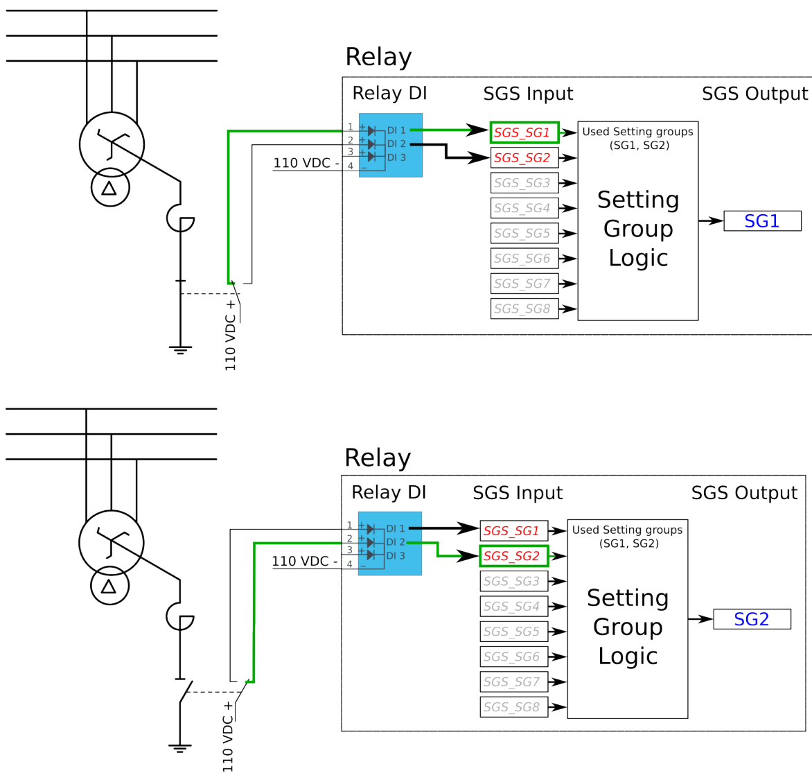
Figure. 5.4.1 - 116. Setting group control – two-wire connection from Petersen coil status.
