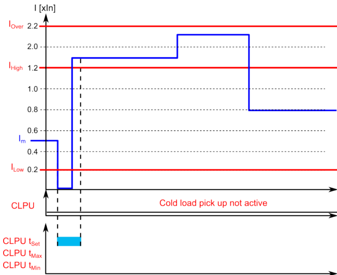
Figure. 5.4.5 - 141. Example of timers and pick-up parameters (no cold load pick-up, I_{low} too short).
