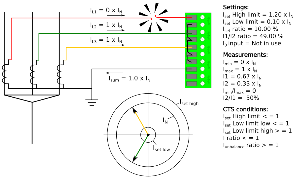
Figure. 5.5.1 - 155. Secondary circuit fault in phase L1 wiring.
