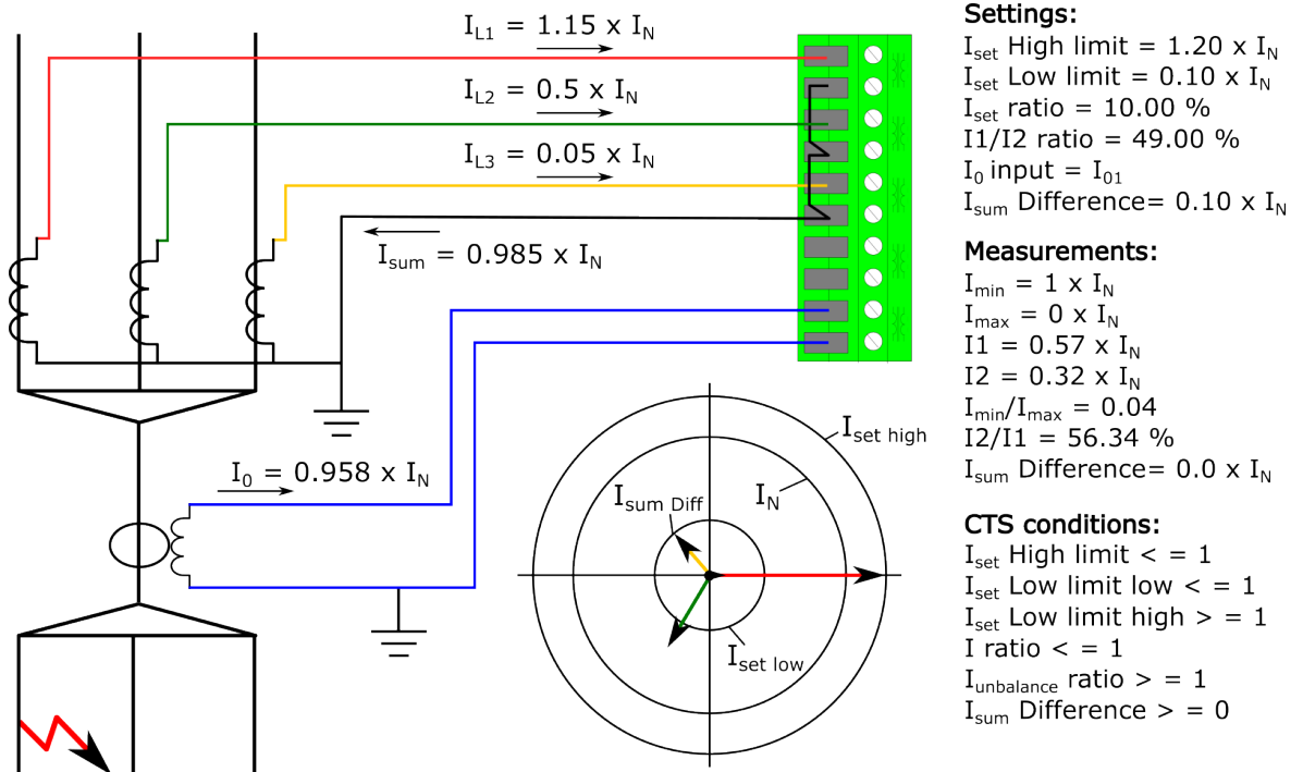
Figure. 5.5.1 - 162. Primary side high-impedance earth fault.
