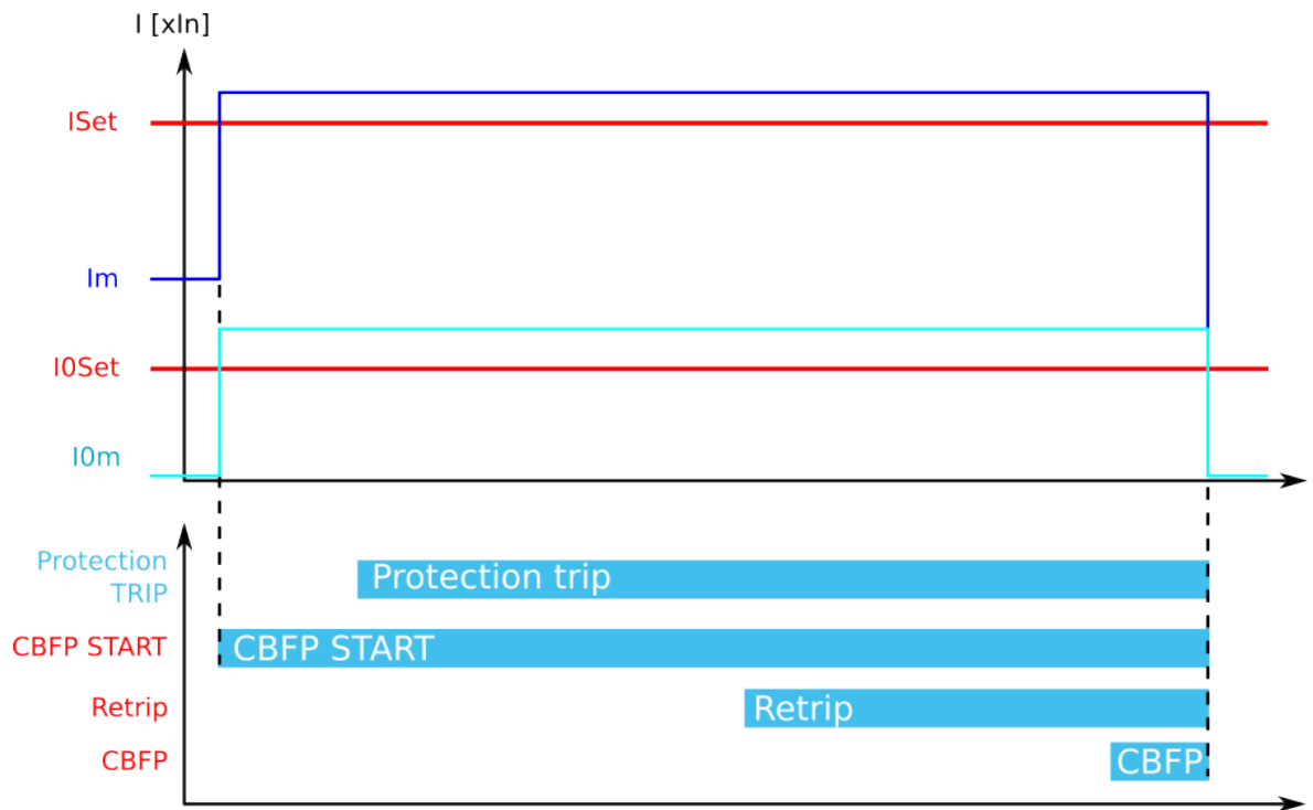
Figure. 5.3.6 - 78. Retrip and CBFP when "Current" is the selected criterion.
