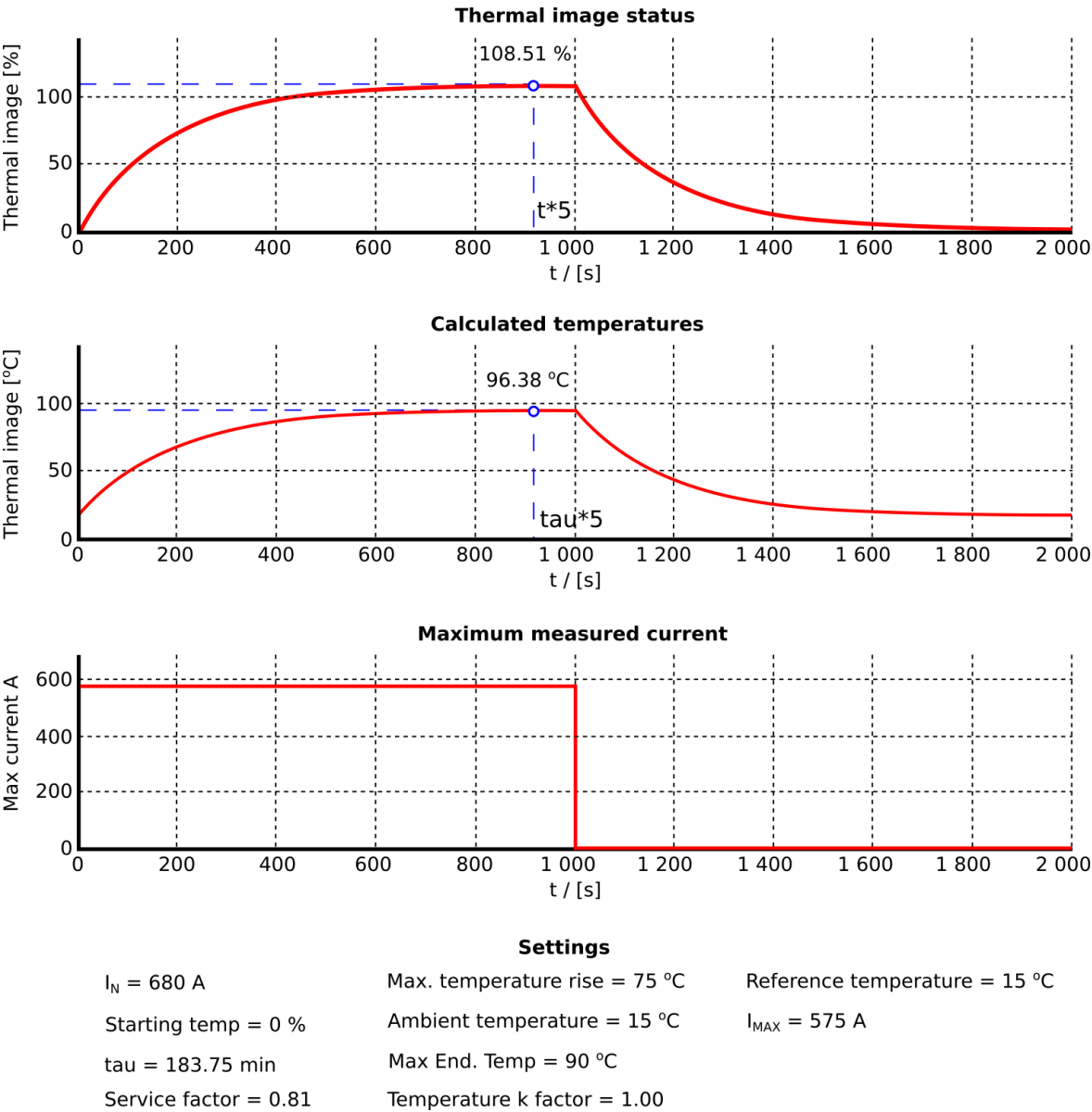
Figure. 5.3.8 - 106. Thermal image response with nominal currents and fine-tuned k_{\text{SF}} correction factor.
