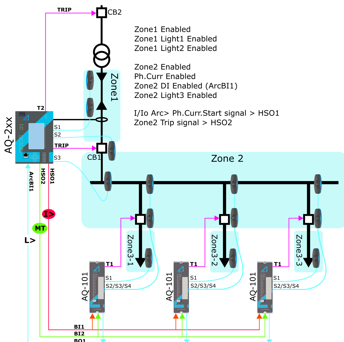
Figure. 5.3.10 - 111. Scheme IA1 (with AQ-101 arc protection relays).
