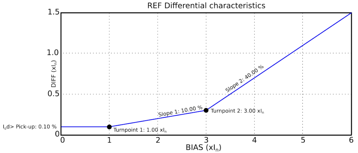
Figure. 5.3.7 - 88. Differential characteristics for the I0d> function with default settings.
