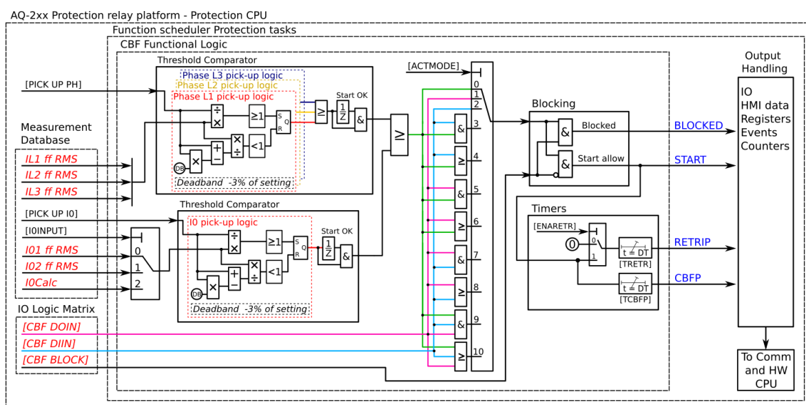
Figure. 5.3.6 - 76. Simplified function block diagram of the CBFP function.
