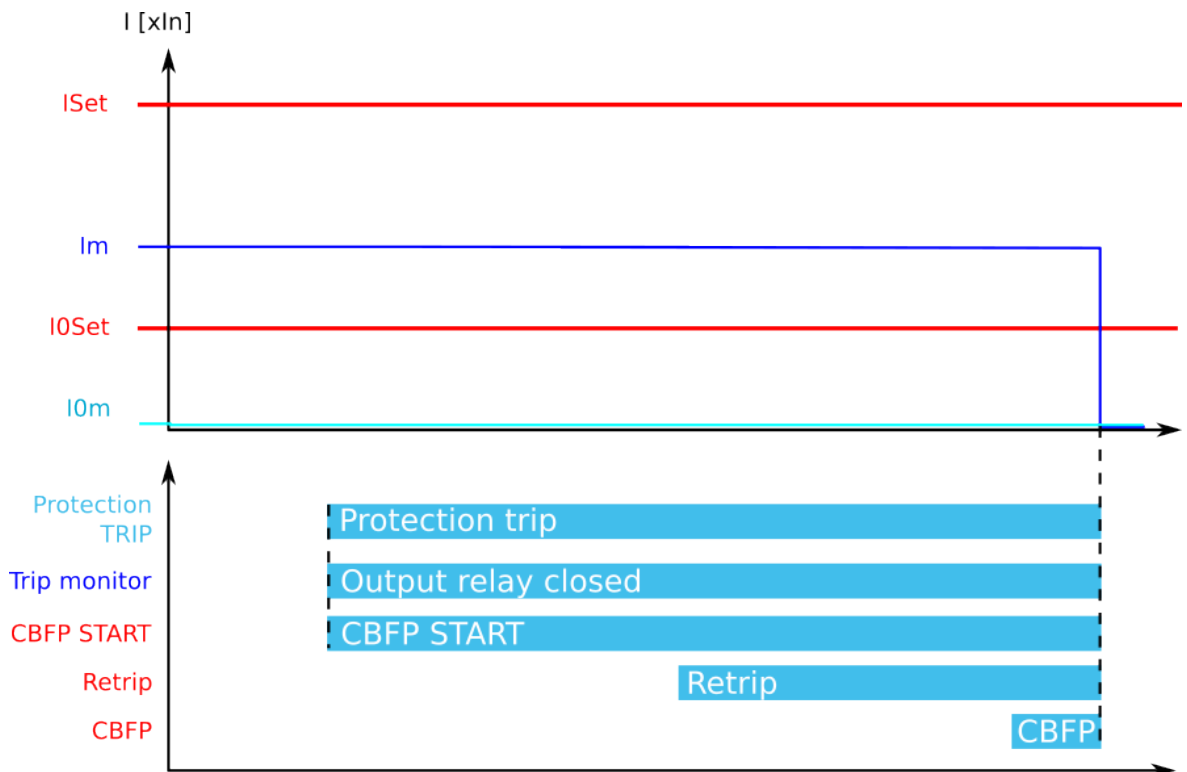
Figure. 5.3.6 - 80. Retrip and CBFP when "Current or DO" is the selected criterion.
