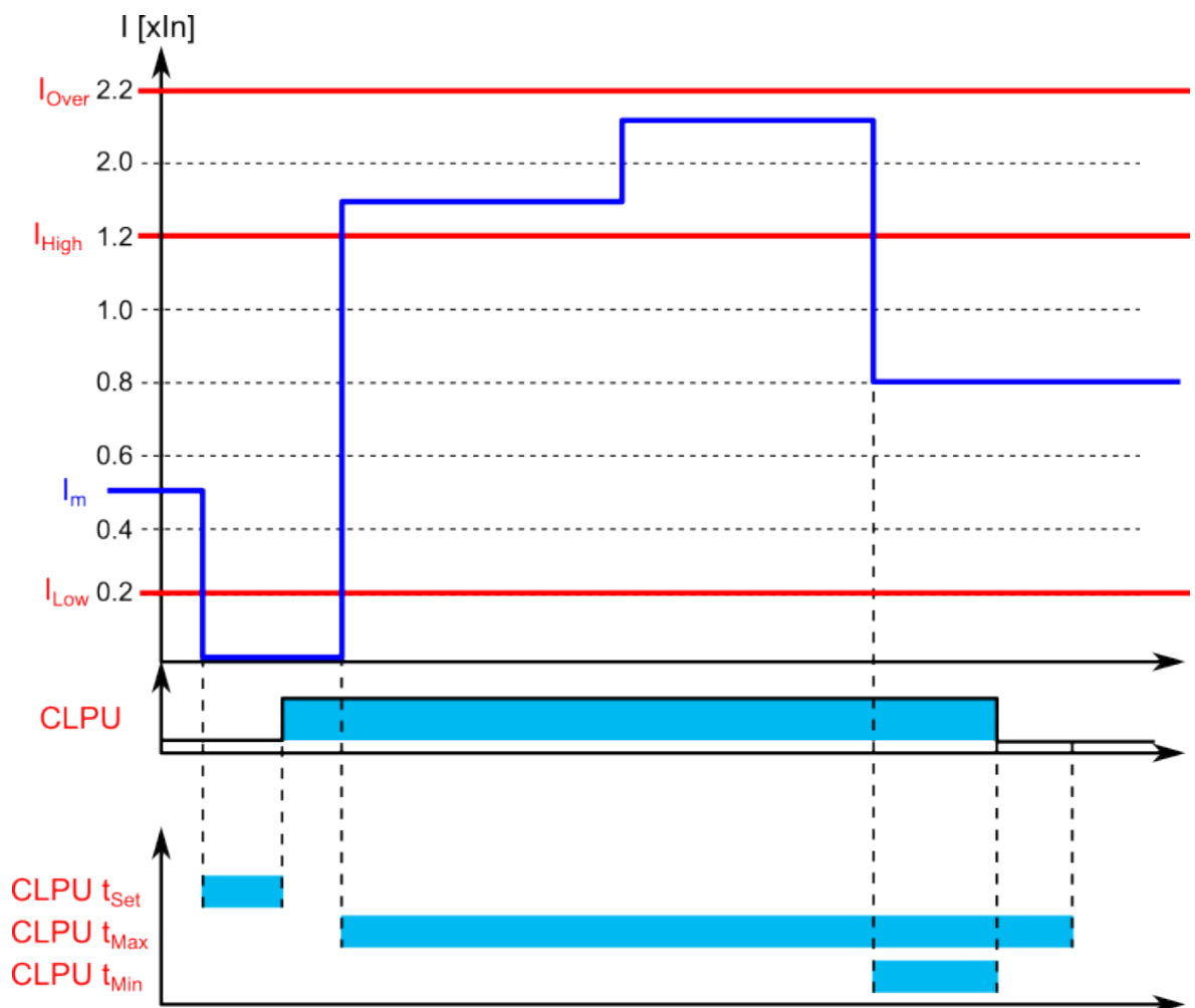
Figure. 5.4.5 - 140. Example of timers and pick-up parameters (normal CLPU situation).
