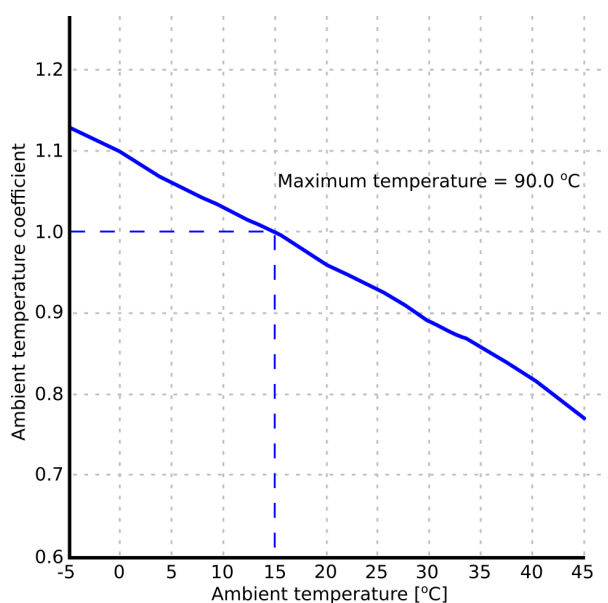
Figure. 5.3.8 - 100. Set correction curve for ambient temperature.
