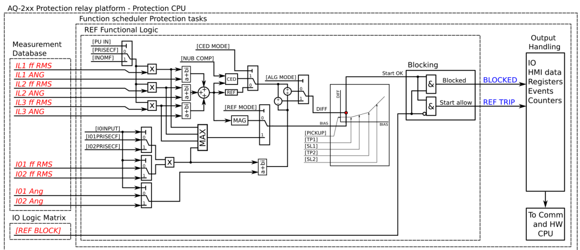
Figure. 5.3.7 - 87. Simplified function block diagram of the I0d> function.
