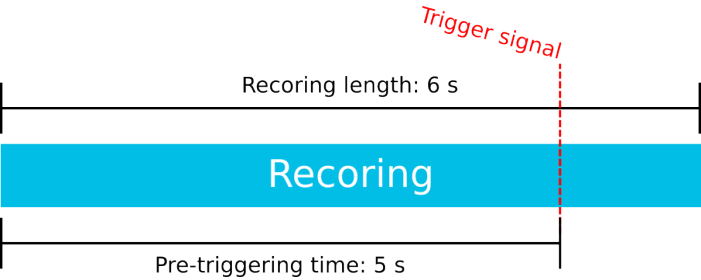
Figure. 5.5.4 - 168. Effects of recording length and pre-triggering time signals. This example is based on the settings shown above.
