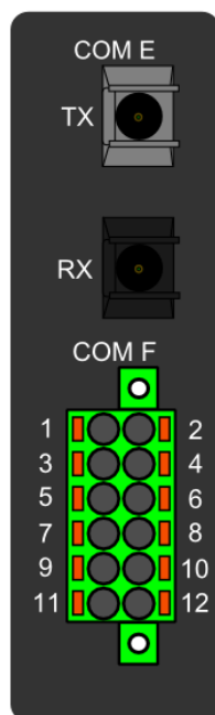
Figure. 8.8 - 191. Serial RS-232 module connectors.
