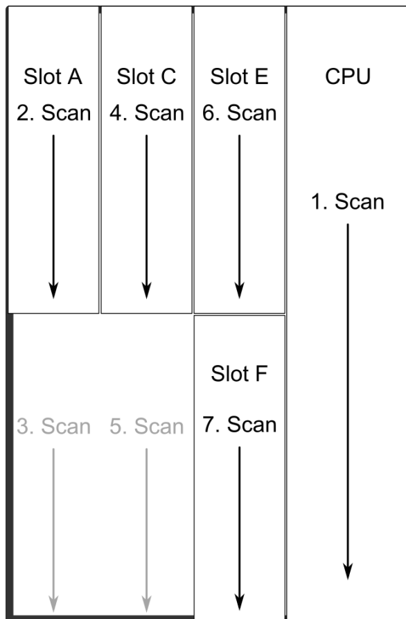
Figure. 8.1 - 182. AQ-X210 hardware scanning and I/O naming principles.
