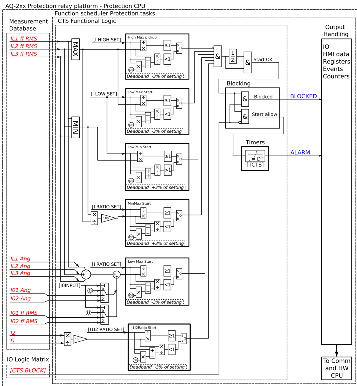
Figure. 5.5.1 - 153. Simplified function block diagram of the CTS function.
