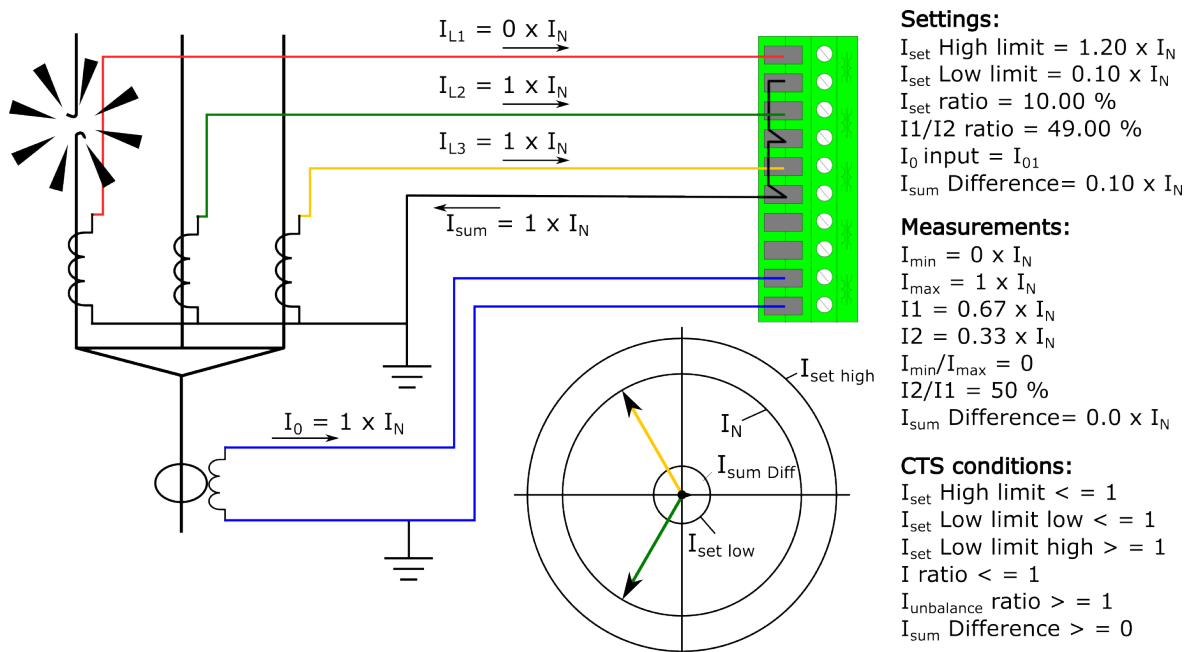
Figure. 5.5.1 - 161. Broken primary phase current wiring.
