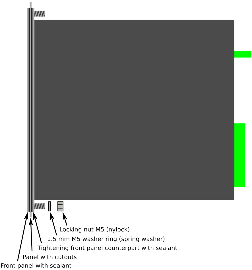
Figure. 8.13 - 201. Device installation.
