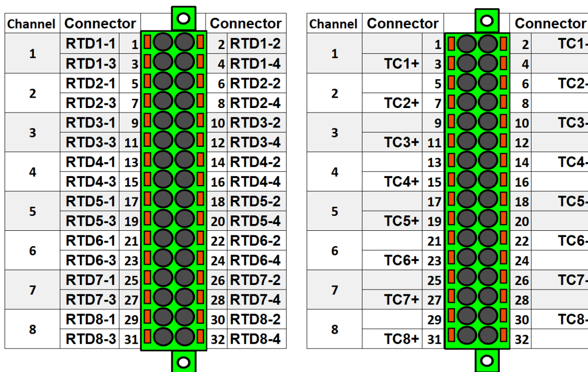
Figure. 8.7 - 189. RTD input module connectors.
