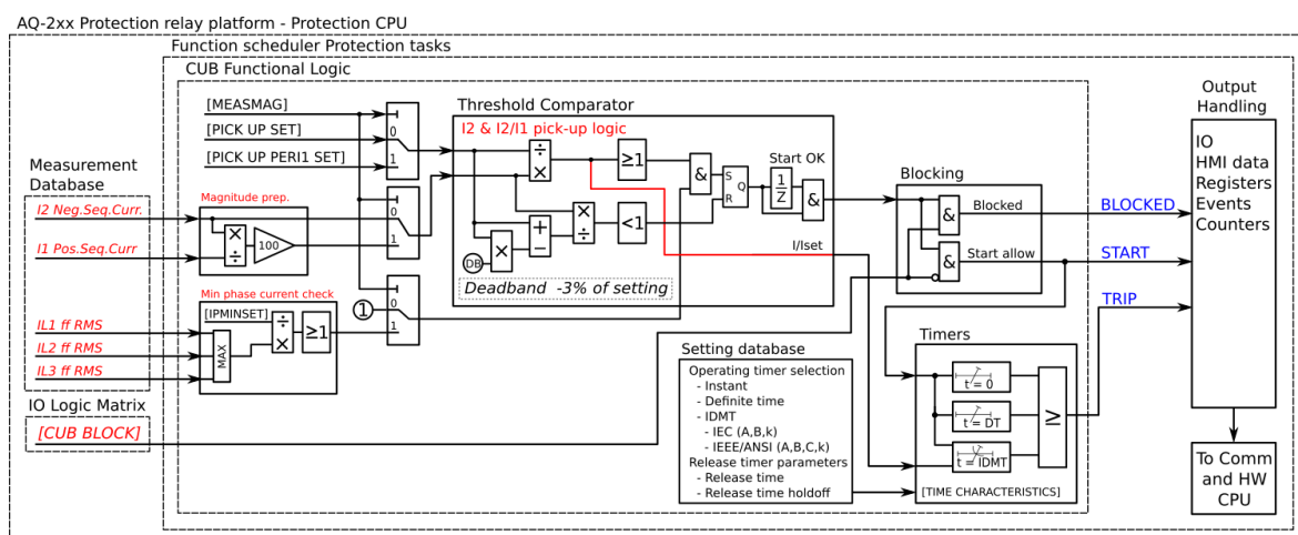
Figure. 5.3.4 - 73. Simplified function block diagram of the I2> function.
