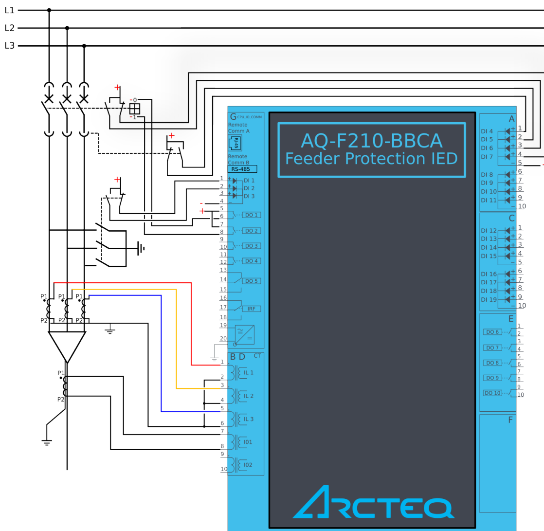
Figure. 7.2 - 174. Application example and its connections.
