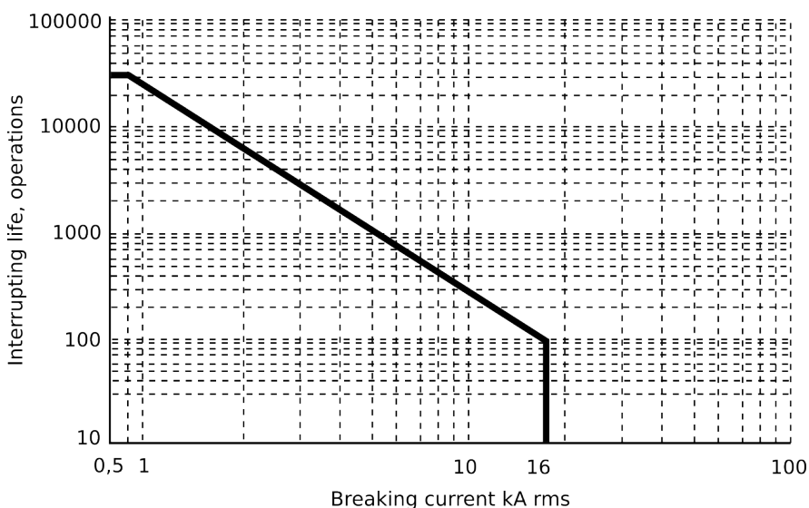
Figure. 5.5.2 - 163. Example of the circuit breaker interrupting life operations.
