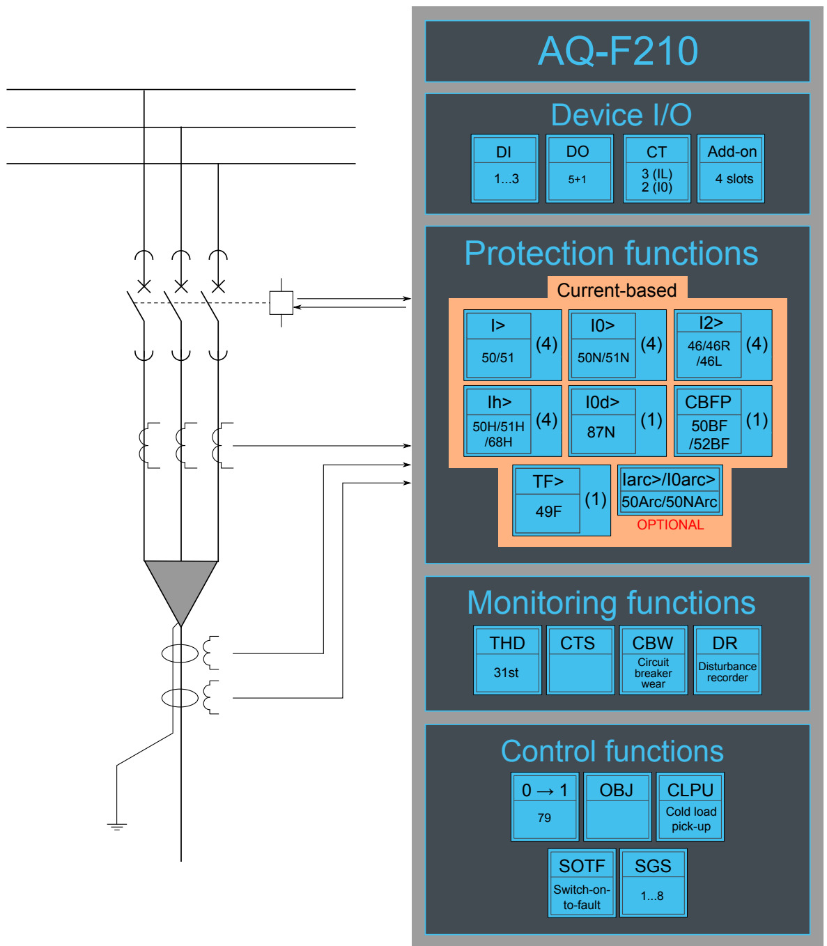
Figure. 7.1 - 173. AQ-F210 application example with function block diagram.
