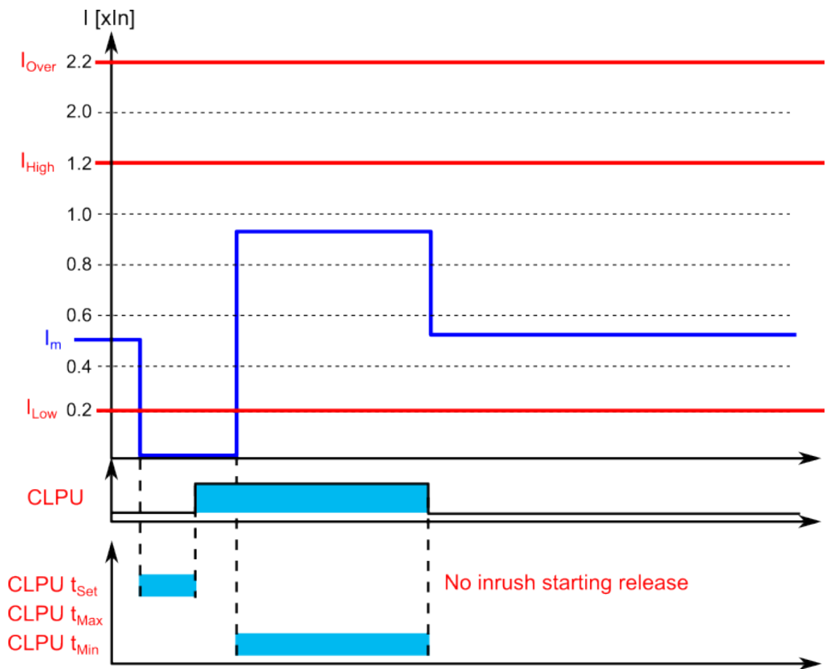
Figure. 5.4.5 - 144. Example of timers and pick-up parameters (no inrush current detected in the starting).
