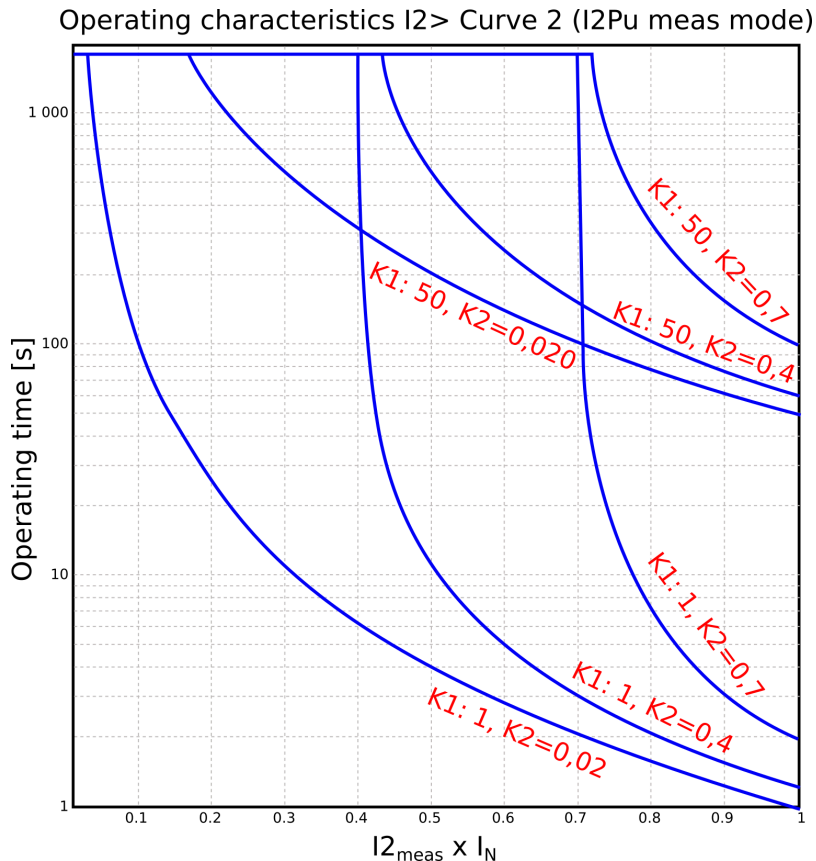
Figure. 5.3.4 - 74. Operation characteristics curve for I2&gt; Curve2.
