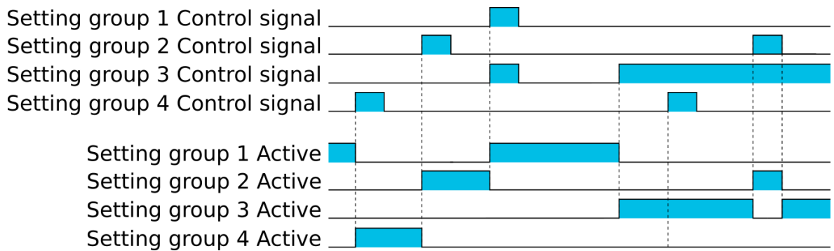
Figure. 5.4.1 - 114. Example sequences of group changing (control with pulse only, or with both pulses and static signals).
