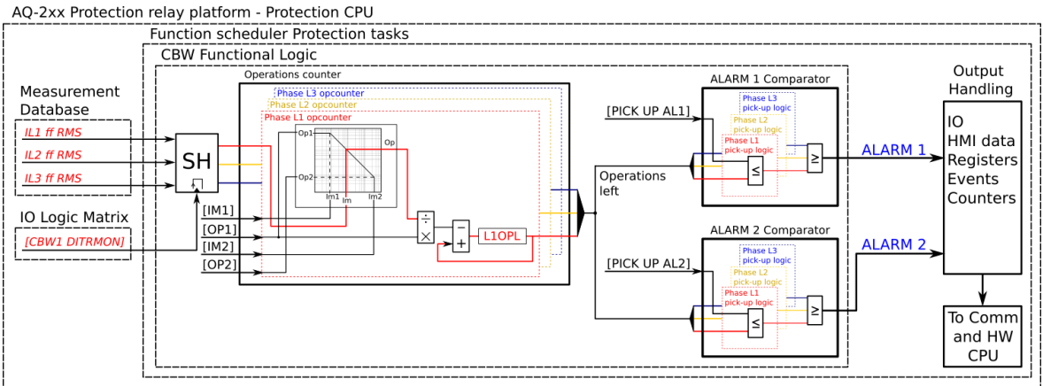
Figure. 5.5.2 - 164. Simplified function block diagram of the circuit breaker wear function.
