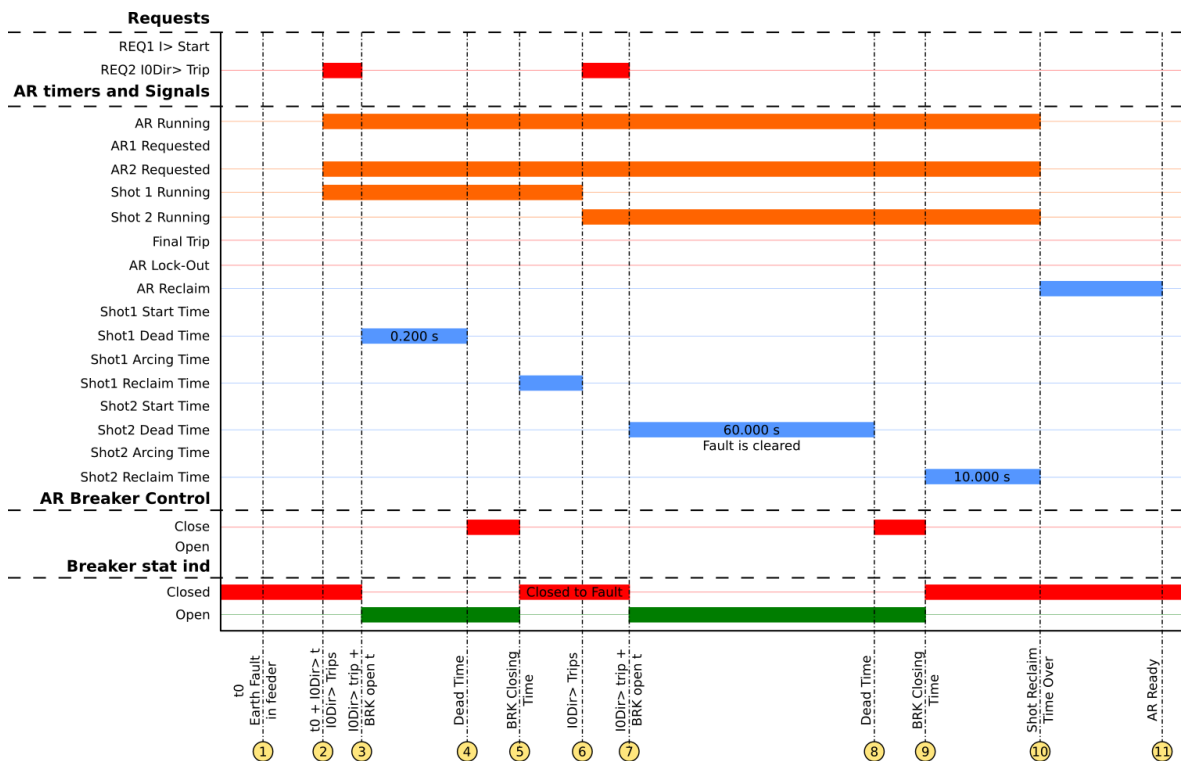
Figure. 5.4.4 - 127. Signal status graph of the semi-permanent earth fault auto-recloser cycle.
