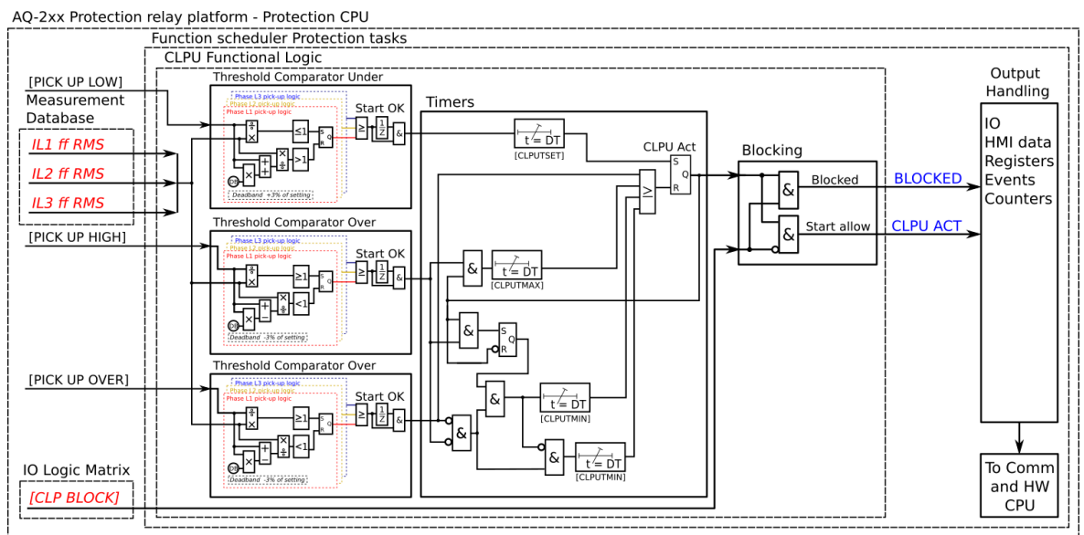
Figure. 5.4.5 - 139. Simplified function block diagram of the cold load pick-up function.
